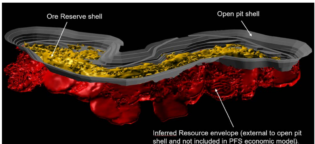
Figure 3 Kalkaroo PFS conceptual open pit, showing Ore Reserve shell (yellow) within the open pit and Inferred Resources (red) external to the open pit and not included in the PFS economic model.
