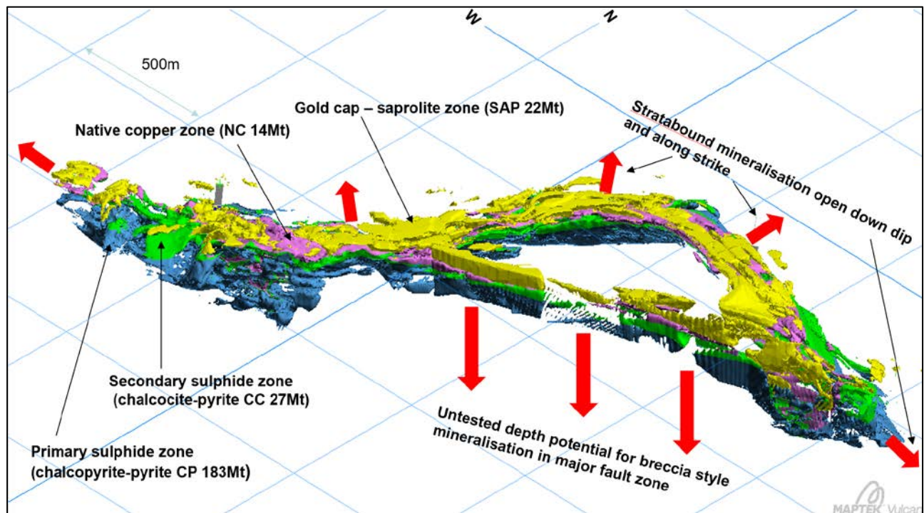
Figure 2 3D view of the Kalkaroo orebody showing the different copper-gold mineralisation types.
