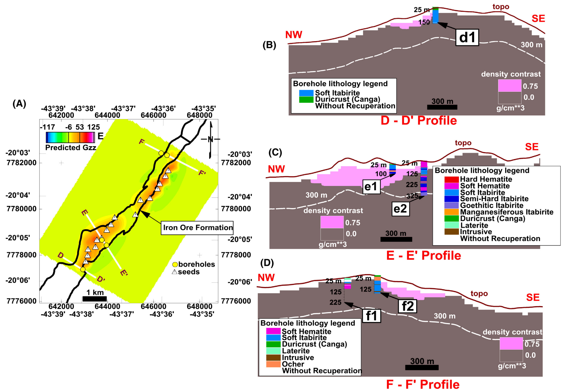
Fig. 11. Area 2. (A) The predicted g_{zz} -component of the gravity gradient tensor. The white lines DD', EE', and FF' display the locations of the vertical cross sections described in (B), (C) and (D), respectively. The yellow dots and the white triangles show the horizontal coordinates of, respectively, the boreholes and the seeds used in the inversion. (B), (C), and (D) show vertical cross sections along profiles DD', EE', and FF', respectively, displaying the estimated density-contrast distribution (in pink) with density contrast 0.75 g/cm 3 . The color ribbons in (B)–(D) represent the lithological intervals intersected by boreholes (d1, e1, e2, f1 and f2). (For interpretation of the references to color in this figure legend, the reader is referred to the web version of this article.)
