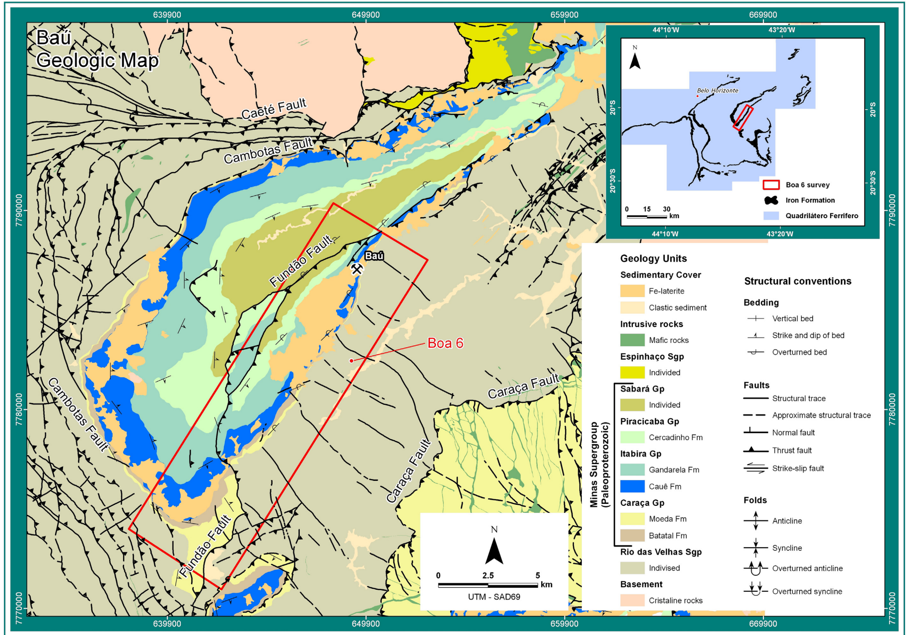
Fig. 3. Detailed geological and structural map of the Gandarela syncline area. The blue areas represent Cauê Formation (banded iron formation). The study area, named Boa 6, is outlined in red rectangle. The inset on the right shows the Quadrilátero Ferrífero area. (For interpretation of the references to color in this figure legend, the reader is referred to the web version of this article.) After Lobato et al. (2005).
