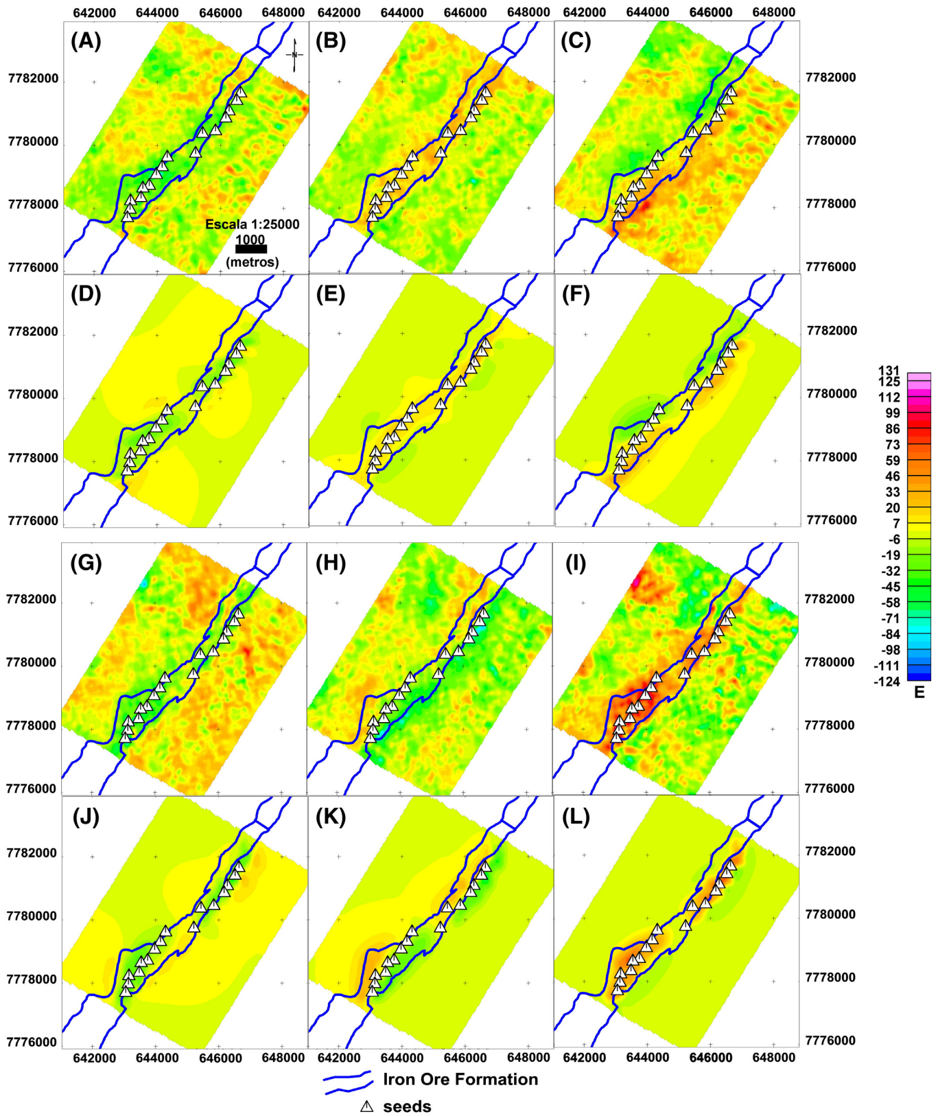
Fig. 7. Area 2. The observed (A–C and G–I panels) and predicted (D–F and J–L panels) g_{xx} -, g_{xy} -, g_{xz} -, g_{yy} -, g_{yz} - and g_{zz} -components of the gravity gradient tensor. The latter were produced by the estimated density-contrast distribution shown in Fig. 9A. The white triangles represent the horizontal coordinates of the seeds used in the inversion. The blue lines delineate the mapped boundaries of the iron formation according to Dorr (1969). The location of Area 2 is shown in Fig. 5B. (For interpretation of the references to color in this figure legend, the reader is referred to the web version of this article.)
