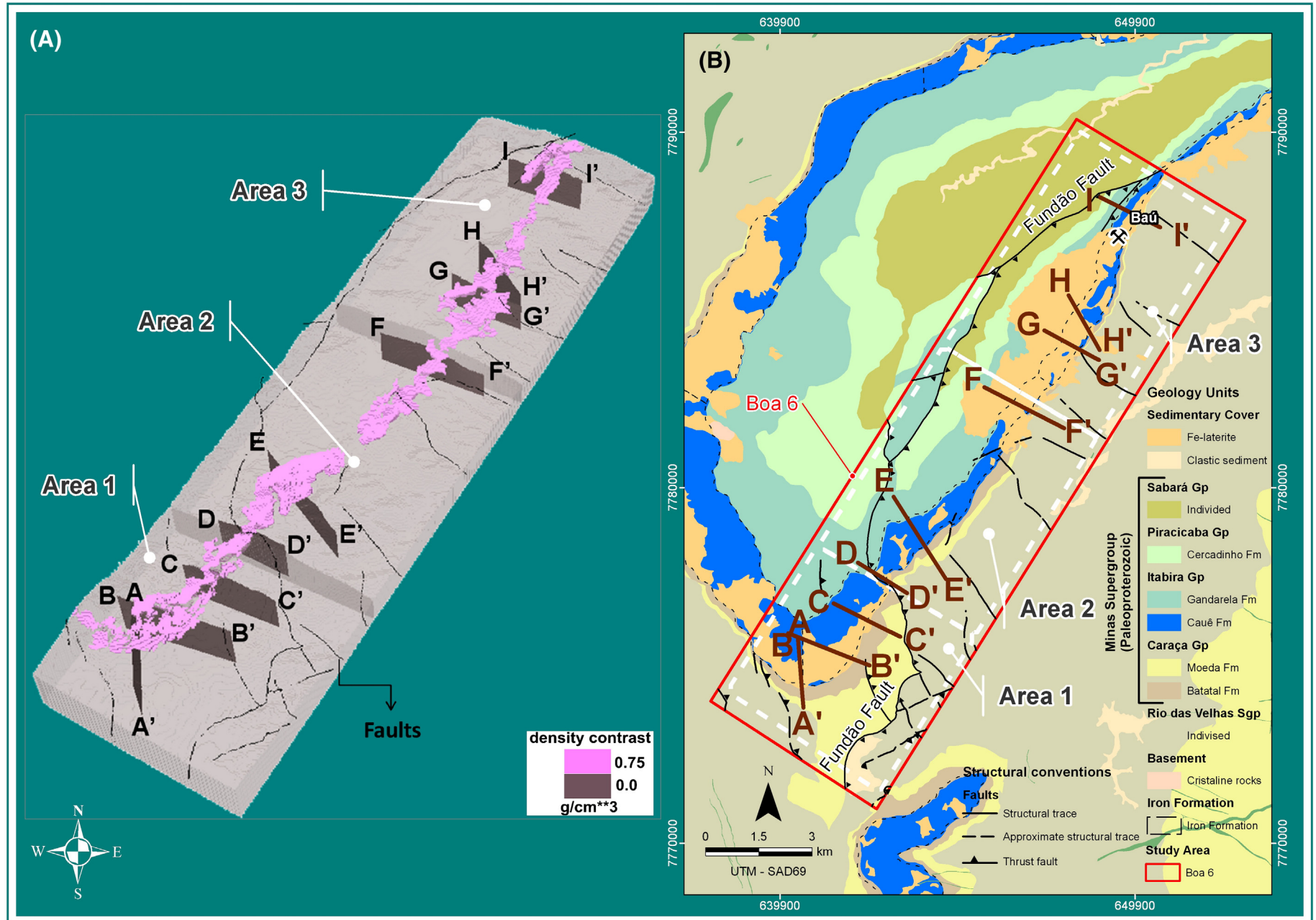
Fig. 9. (A) Tridimensional view of the estimated density-contrast distribution (in pink) with density contrast 0.75 \text{ g/cm}^3 , corresponding to the iron-ore body of the Cauê Formation. This estimate is obtained by inverting the gravity-gradient data sets from Areas 1–3 shown in Figs. 6–8 (color-scaled maps in panels A–C and G–I). (B) Geologic map of the study area showing Areas 1–3 which were used by applying Uieda and Barbosa's (2012a) method. The brown lines AA'–II' display the locations of the vertical cross sections described in Figs. 10–12. (For interpretation of the references to color in this figure legend, the reader is referred to the web version of this article.)
