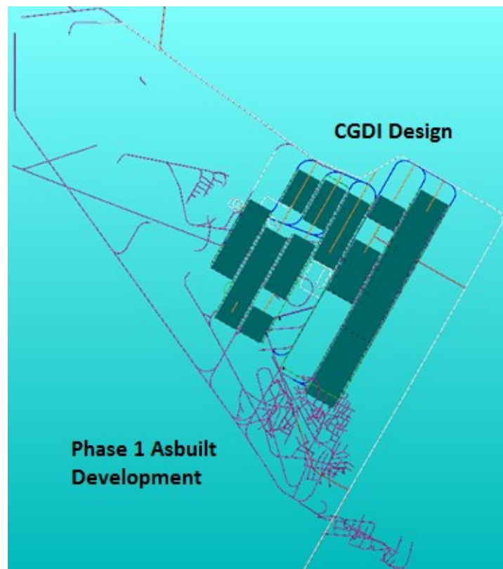
Figure 15-3: CGDI Designed Stopes in Relation to As-built Development
