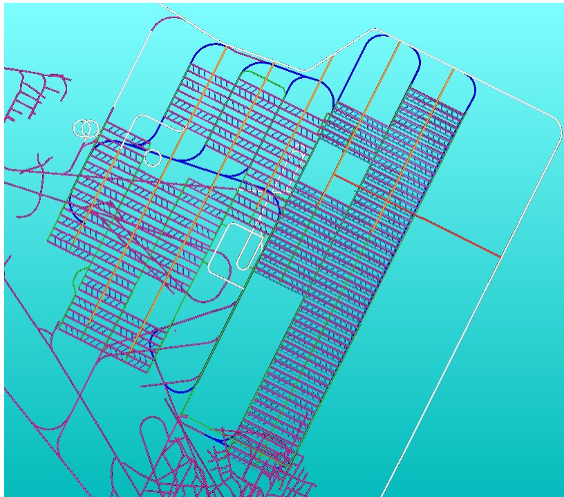
Figure 15-10: CGDI Development Design showing Bogging Levels and Rail System (dark blue)
