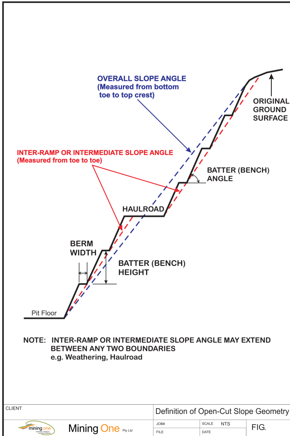
Figure 15-37: Pit Section
