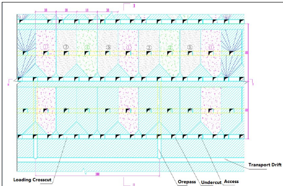
Figure 15-8: CGDI Stoping Cross-section with Mining Sequence
