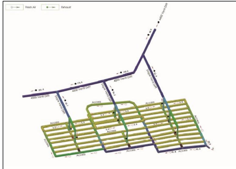
Figure 15-14: Ventilation 4,450 mRL
