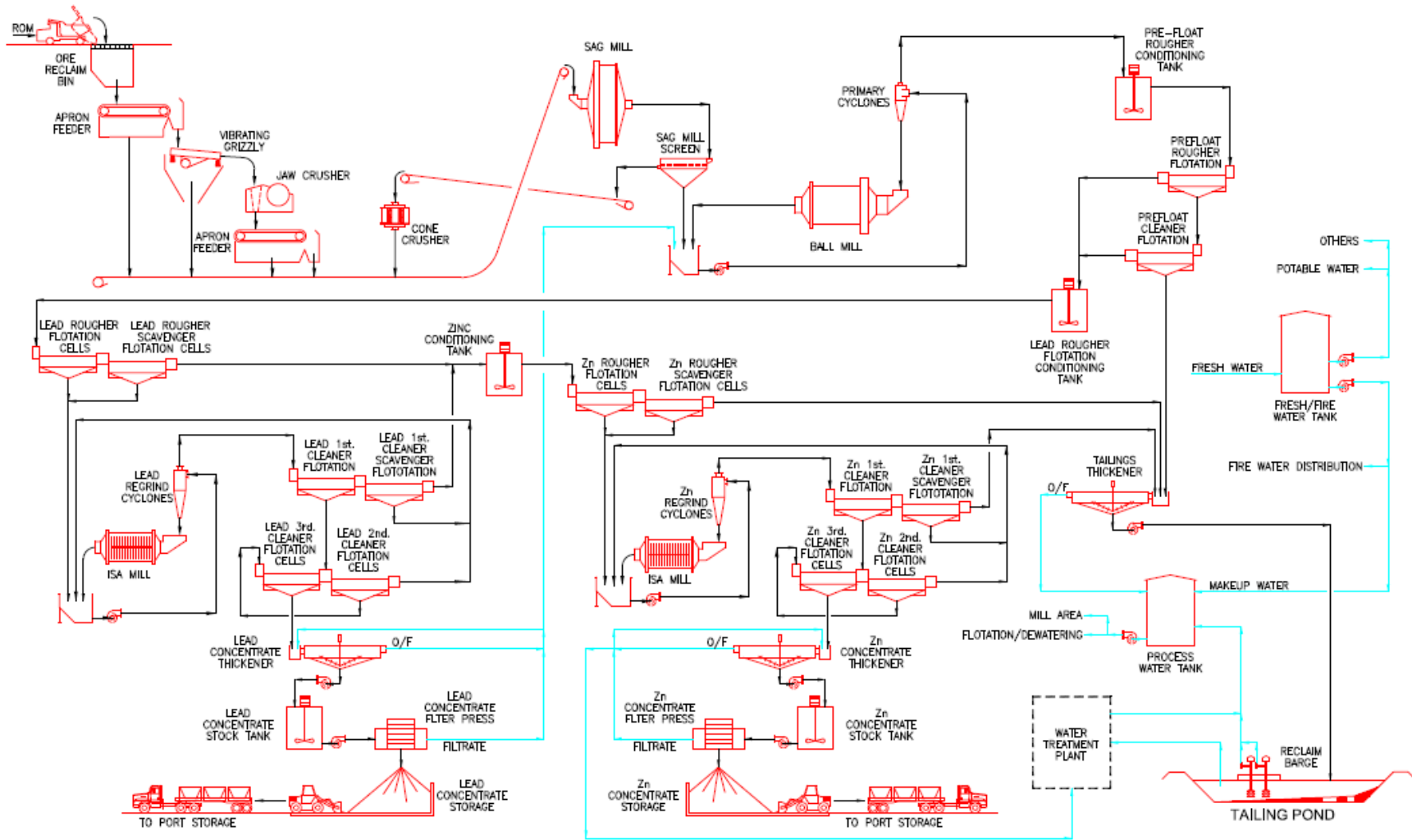
Figure 17-1: Simplified Flow Sheet
