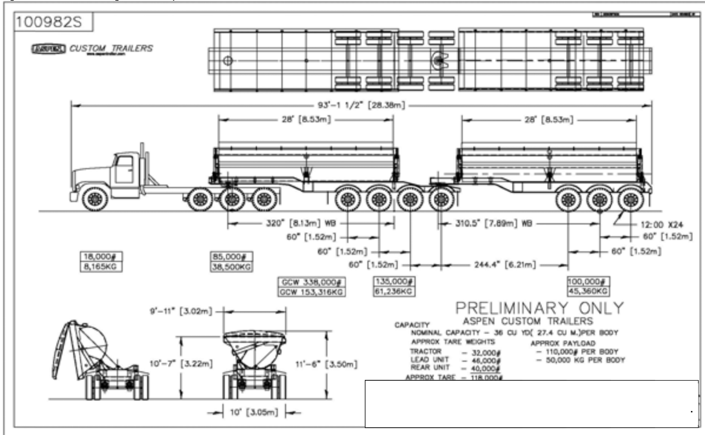
Figure 18-2 Concentrate Haulage Truck Concepts
