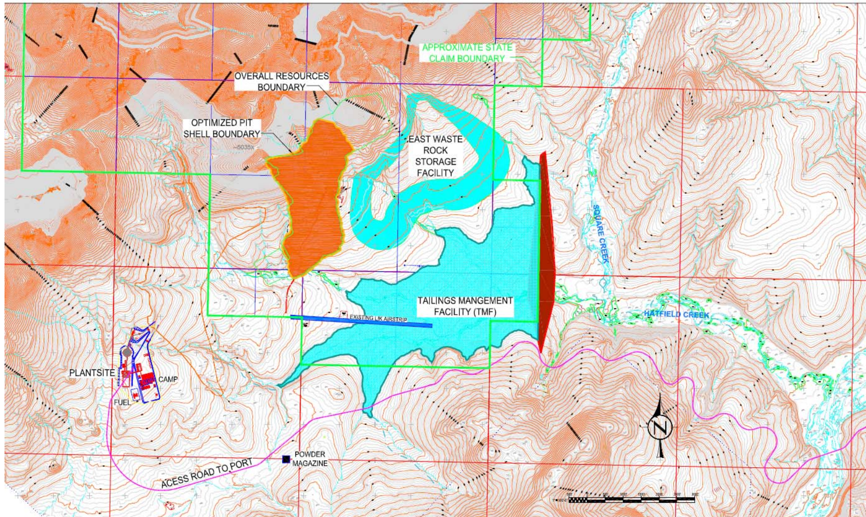
Figure 18-3: Overall Site Plan
