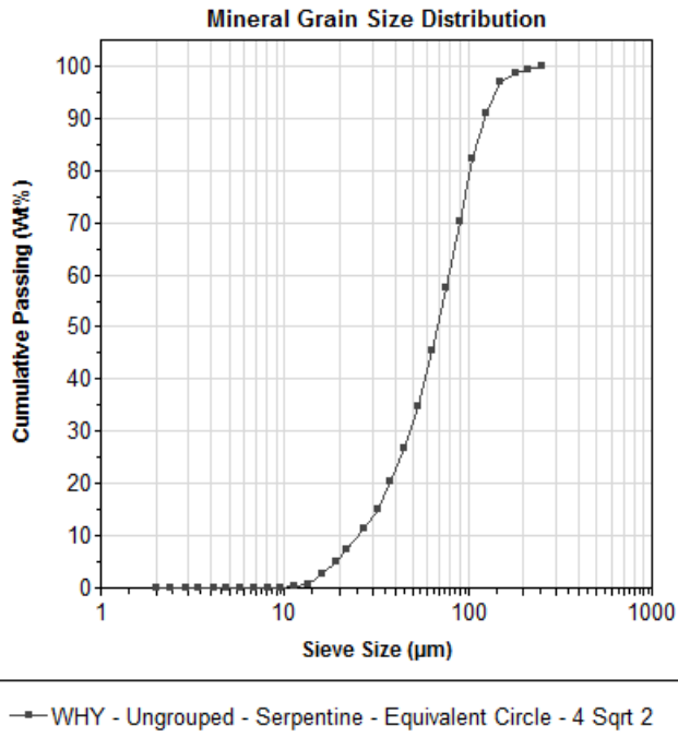
Figure 12. Serpentine grain size distribution in the WHY Resources sample.
