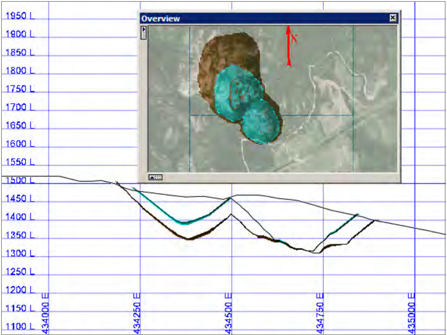
Comparison of the economic Whittle™ pit shell 8 (blue color, smaller) to 13 (brown color, larger) in the section view
