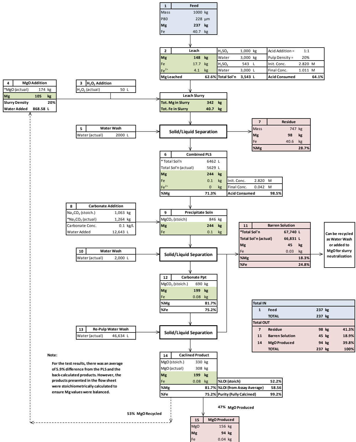
Figure 9. Process Flow Sheet of Metallurgical Test Work
