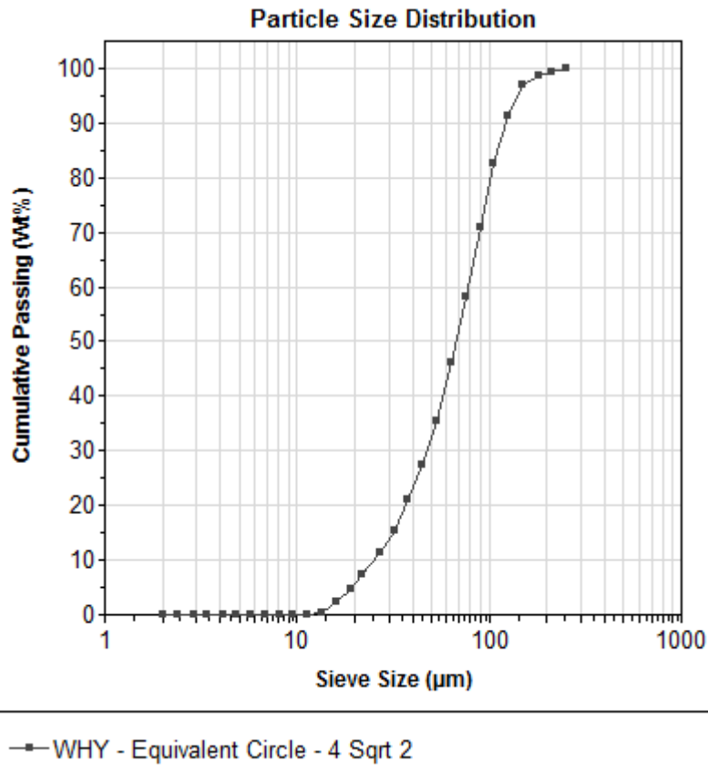
Figure 1. MLA-determined particle size distribution for the WHY Resources sample.
