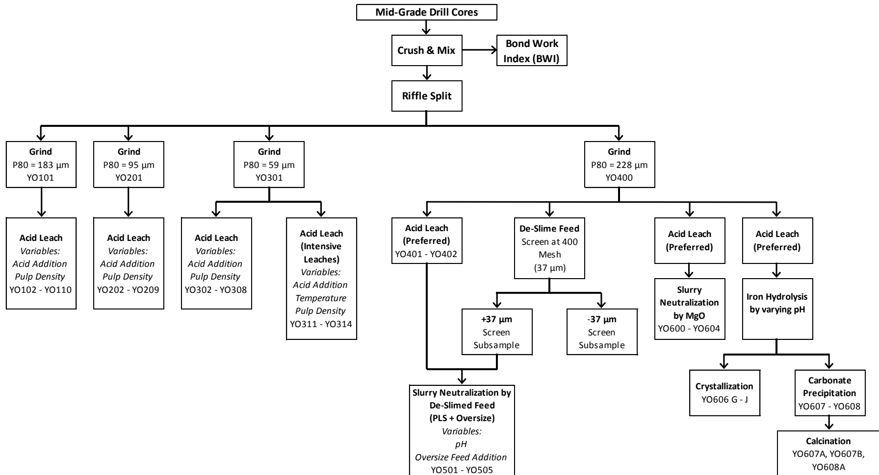
Figure 1. General Flow Sheet of Test Program for WHY Resources
