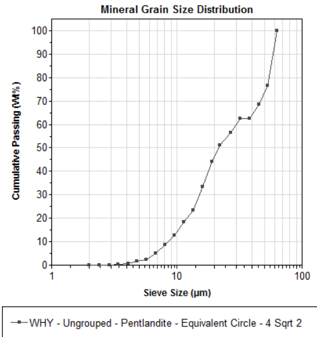
Figure 5. Pentlandite grain size distribution in the WHY Resources sample.
