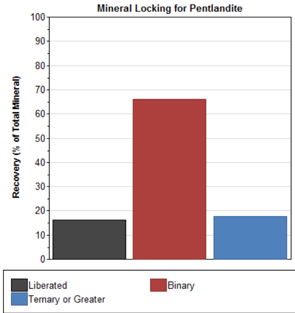
Figure 6. Mineral locking for pentlandite from the WHY Resources sample.
