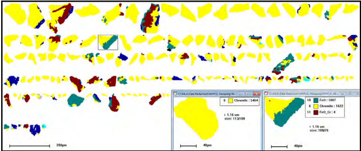
Figure 9. Selected chromite-containing particles from the WHY Resources sample.
