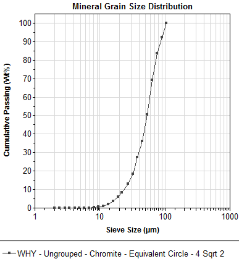
Figure 10. Chromite grain size distribution in the WHY Resources sample.
