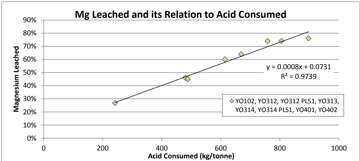
Figure 4. Magnesium Leached and its Relation to Acid Consumed
