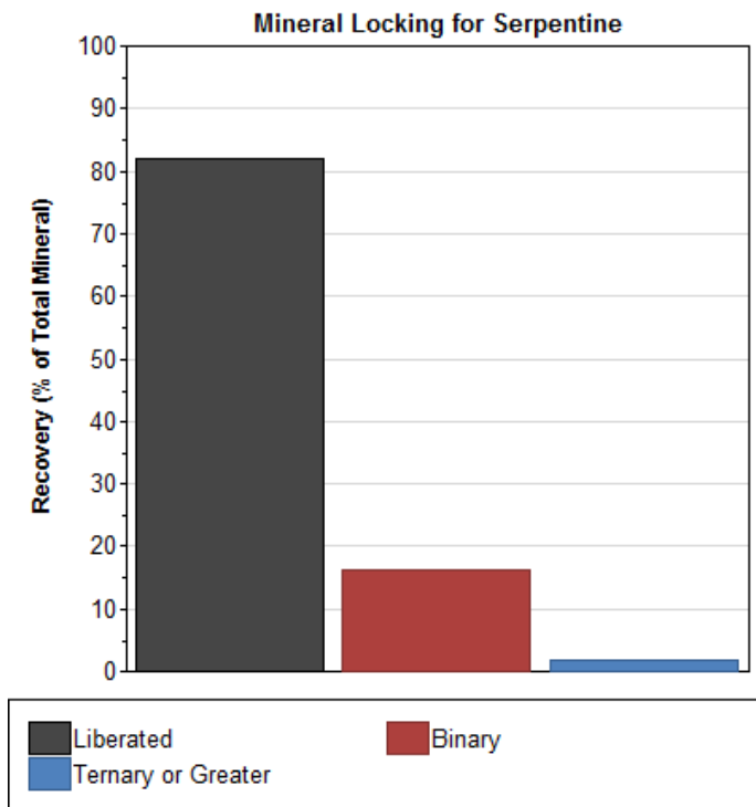
Figure 13. Mineral locking for serpentine from the WHY Resources sample.
