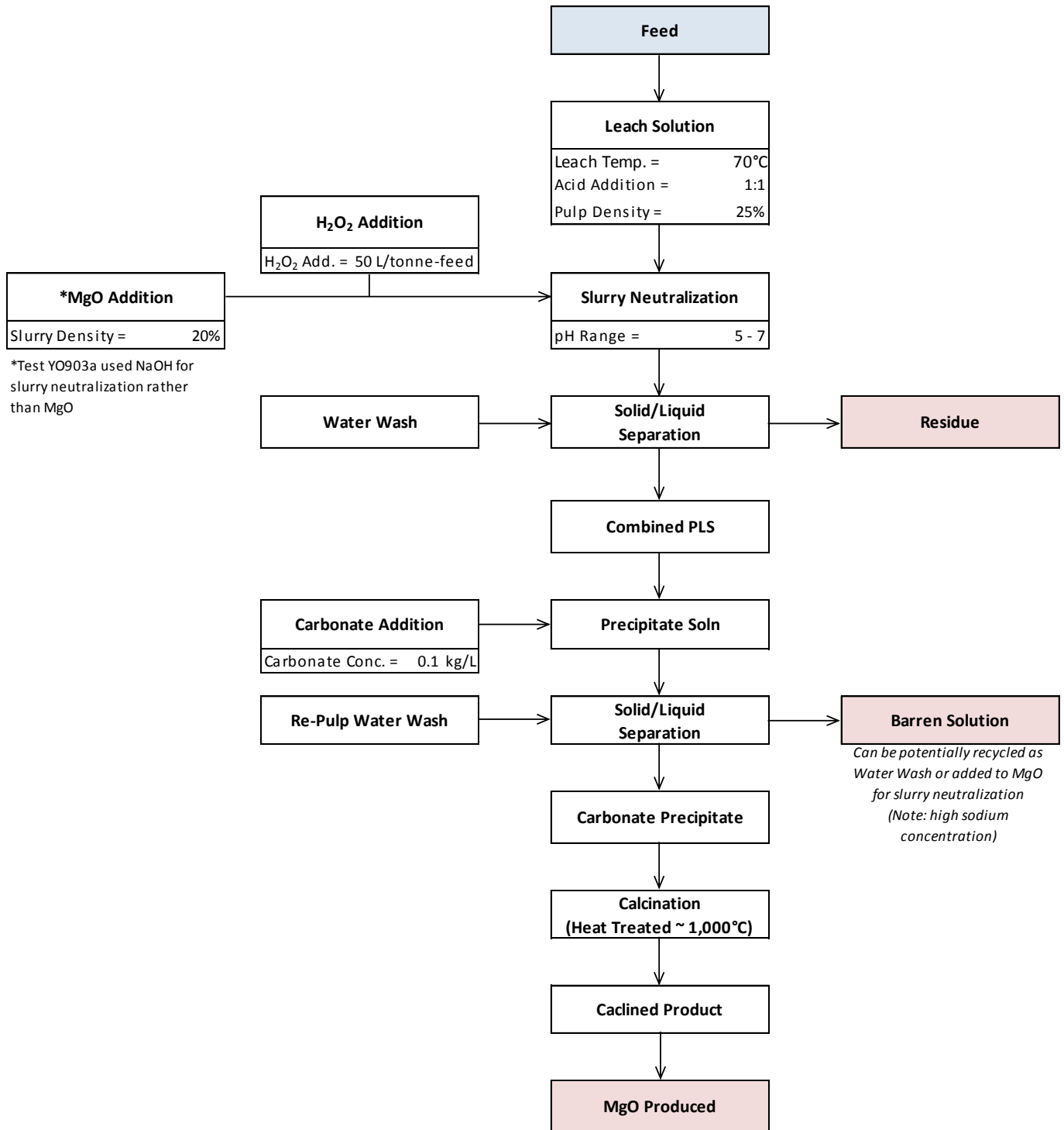
Figure 1: Overall Process Flow Sheet
