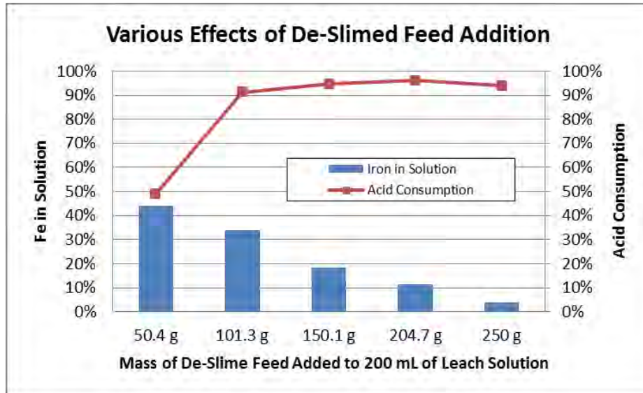
Figure 6. Various Effects of De-Slimed Feed Addition
