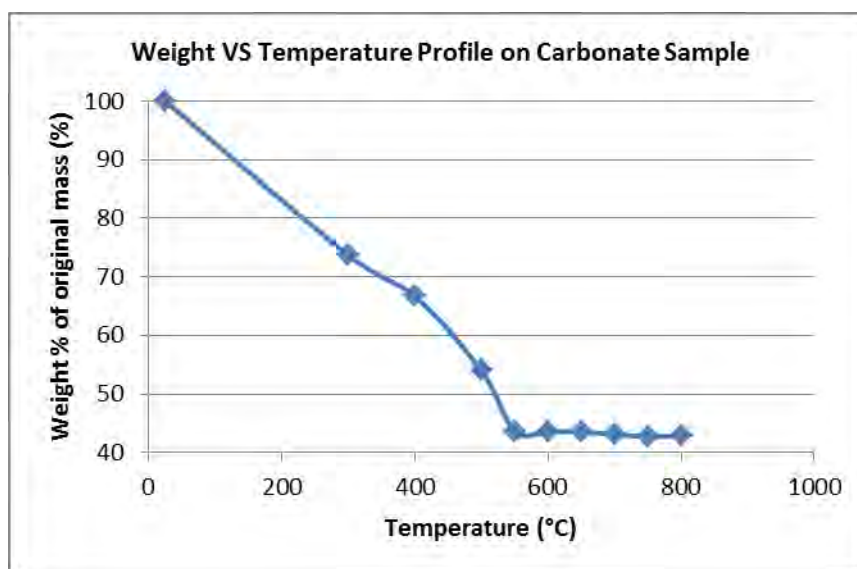
Figure 8. Weight VS Temperature Profile on Carbonate Sample
