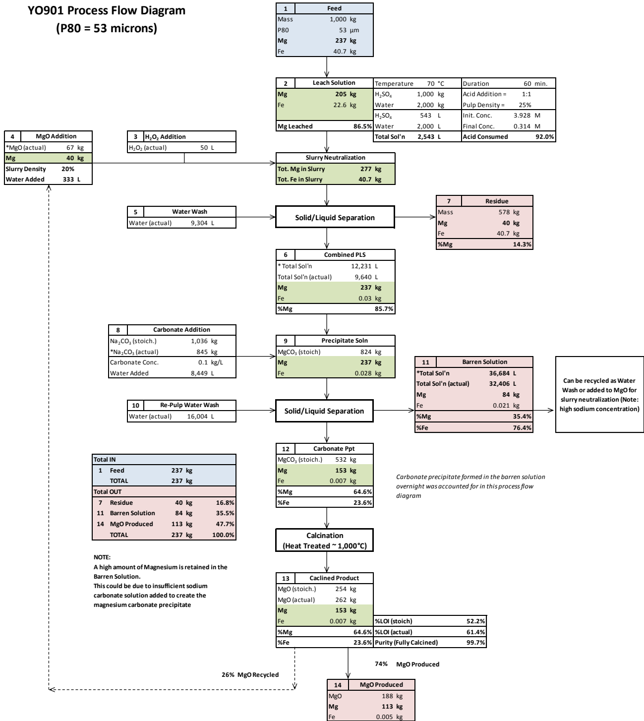
Figure 1: Process Flow Sheet of Test Work YO901 (P 80 = 53 μm, MgO Slurry Neutralization)
