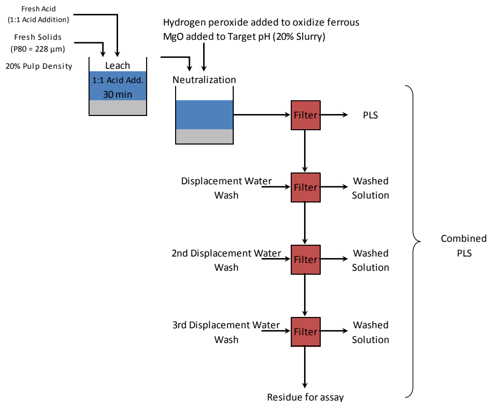
Figure 7. General Flow Sheet for Leach Test with MgO Addition
