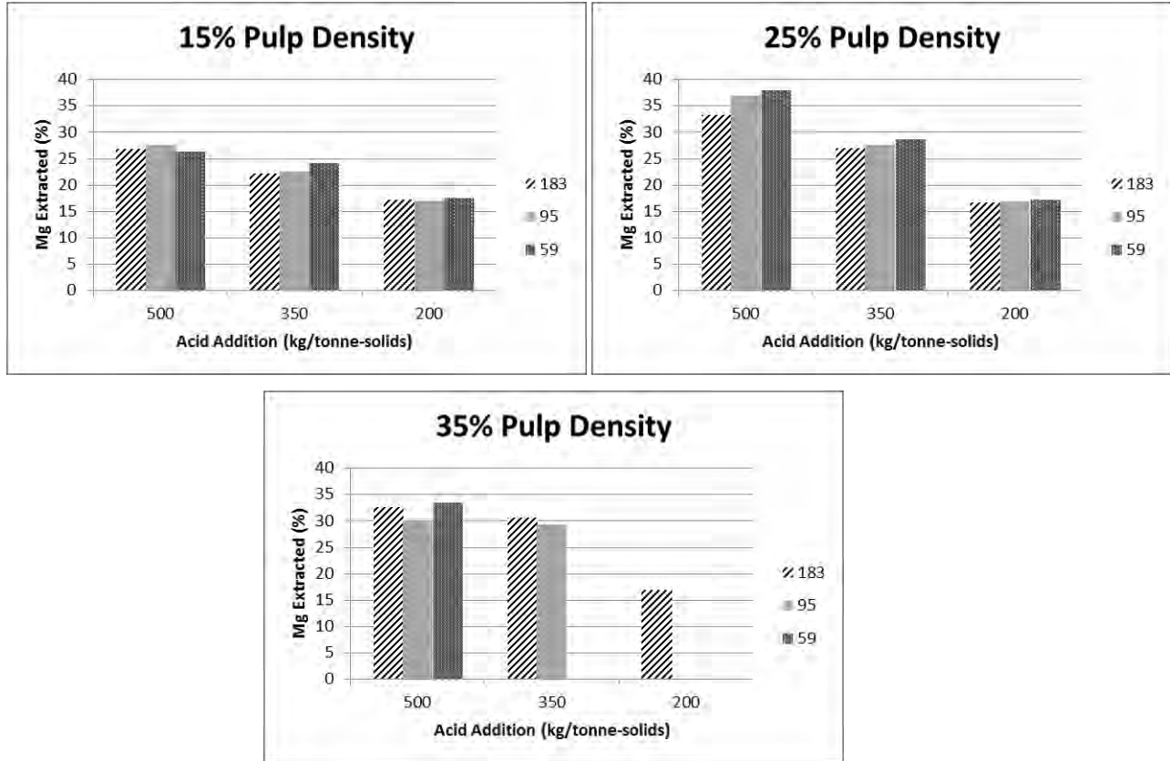
Figure 3. Magnesium Extracted as a Function of Acid Addition at Various Grind Sizes and Pulp Densities
