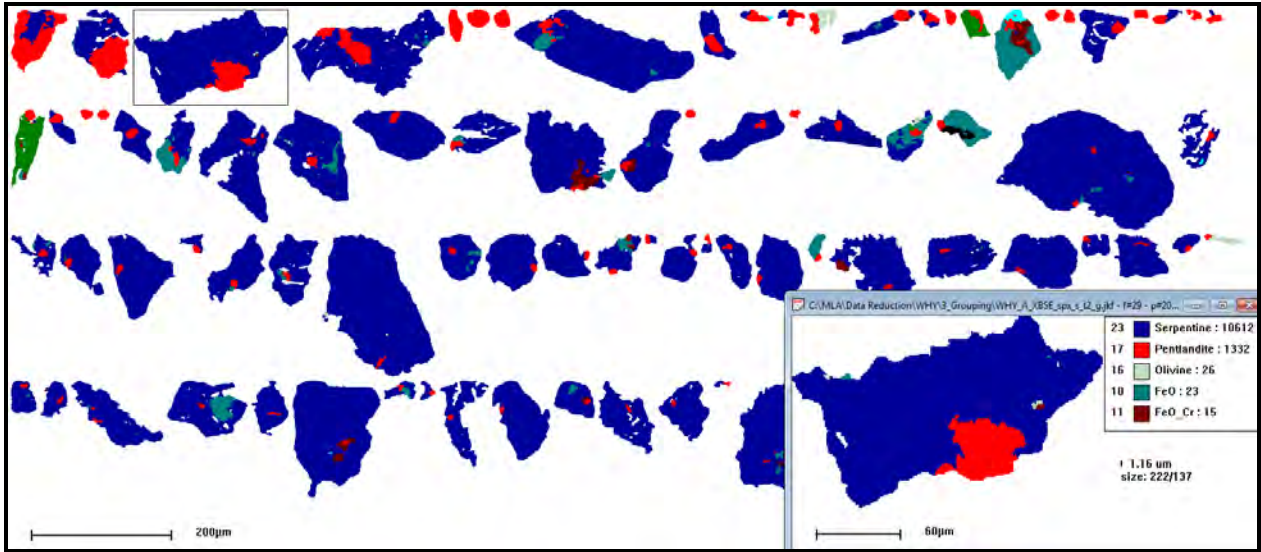
Figure 4. Selected pentlandite-containing particles from the WHY Resources sample.
