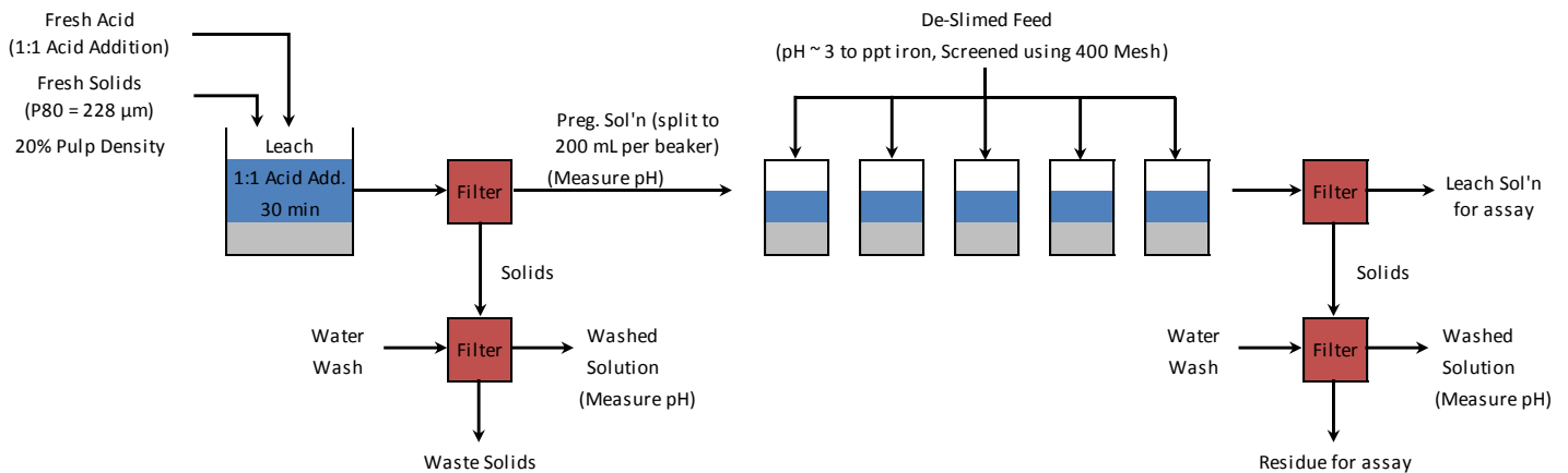
Figure 5. General Flow Sheet for Leach Test with De-Slimed Feed Addition
