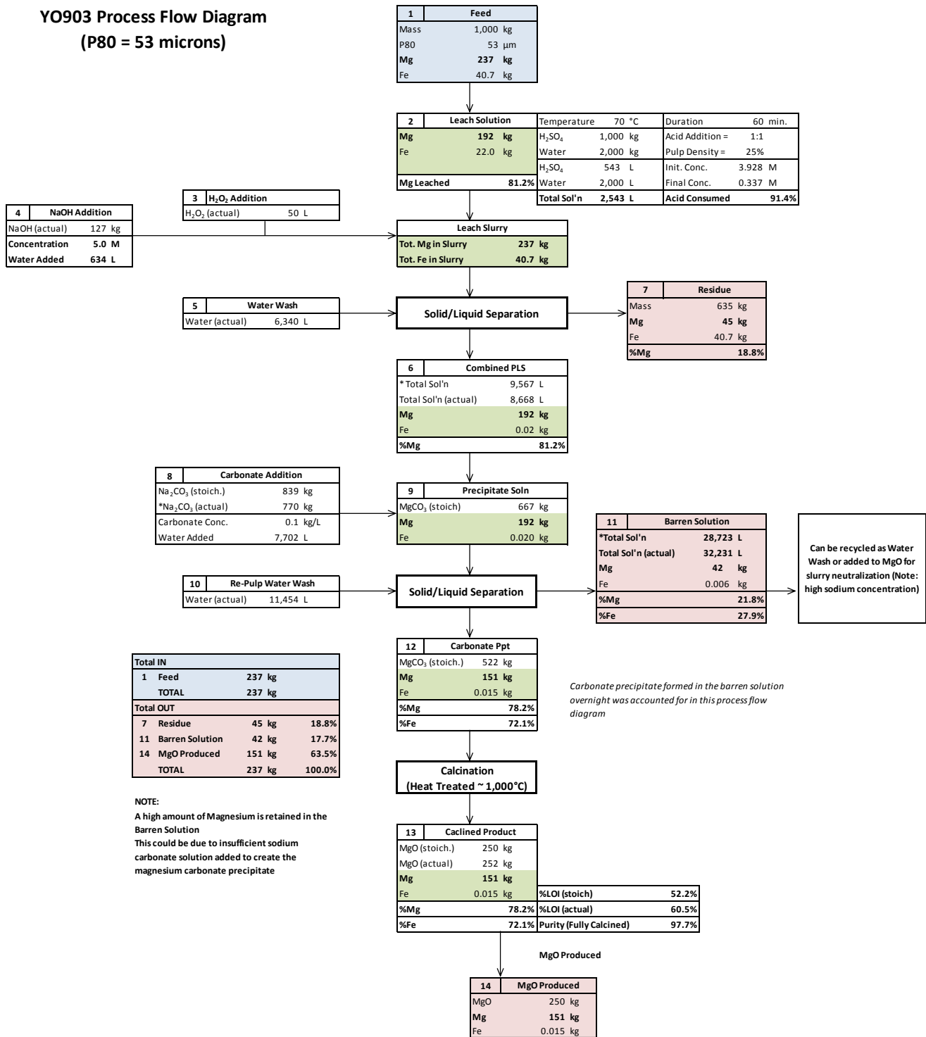
Figure 3: Process Flow Sheet of Test Work YO903 (P 80 = 53 μm, NaOH Slurry Neutralization)
