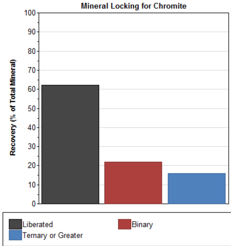
Figure 11. Mineral locking for chromite from the WHY Resources sample.
