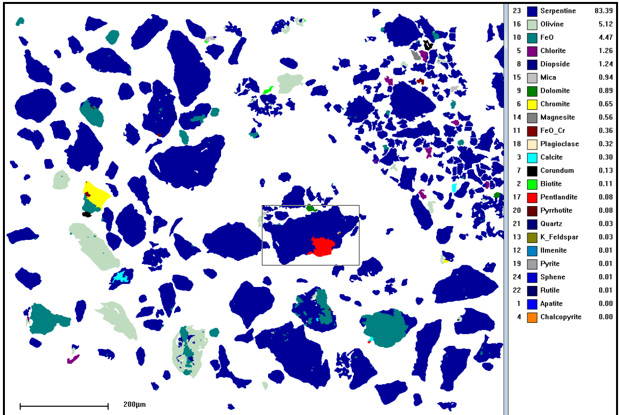
Figure 2. Classified MLA image from the WHY Resources sample. Inset shows overall mineral surface area percentages.
