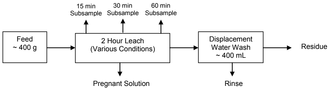
Figure 2. Acid Leach Test Flow Sheet
