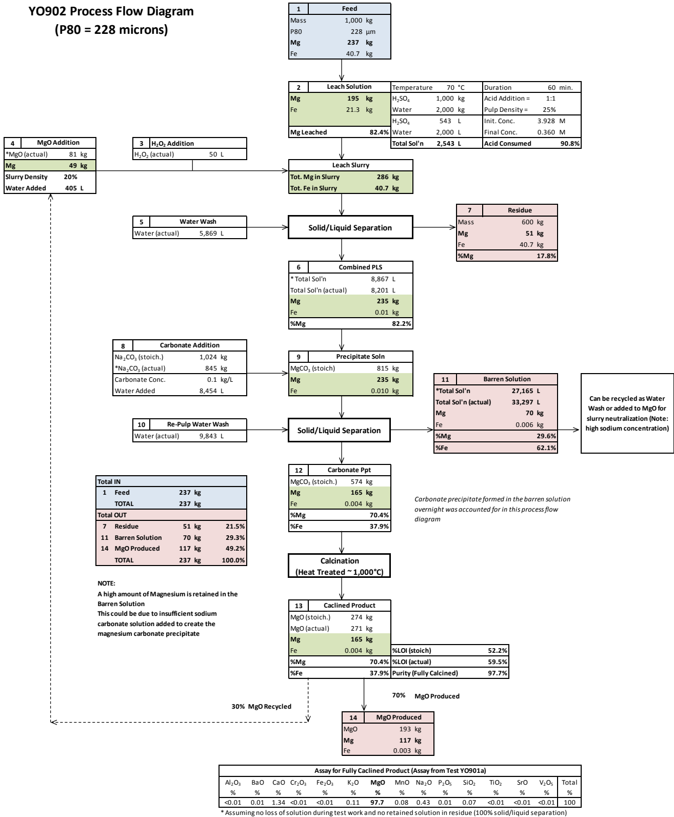
Figure 2: Process Flow Sheet of Test Work YO902 (P 80 = 228 μm, MgO Slurry Neutralization)
