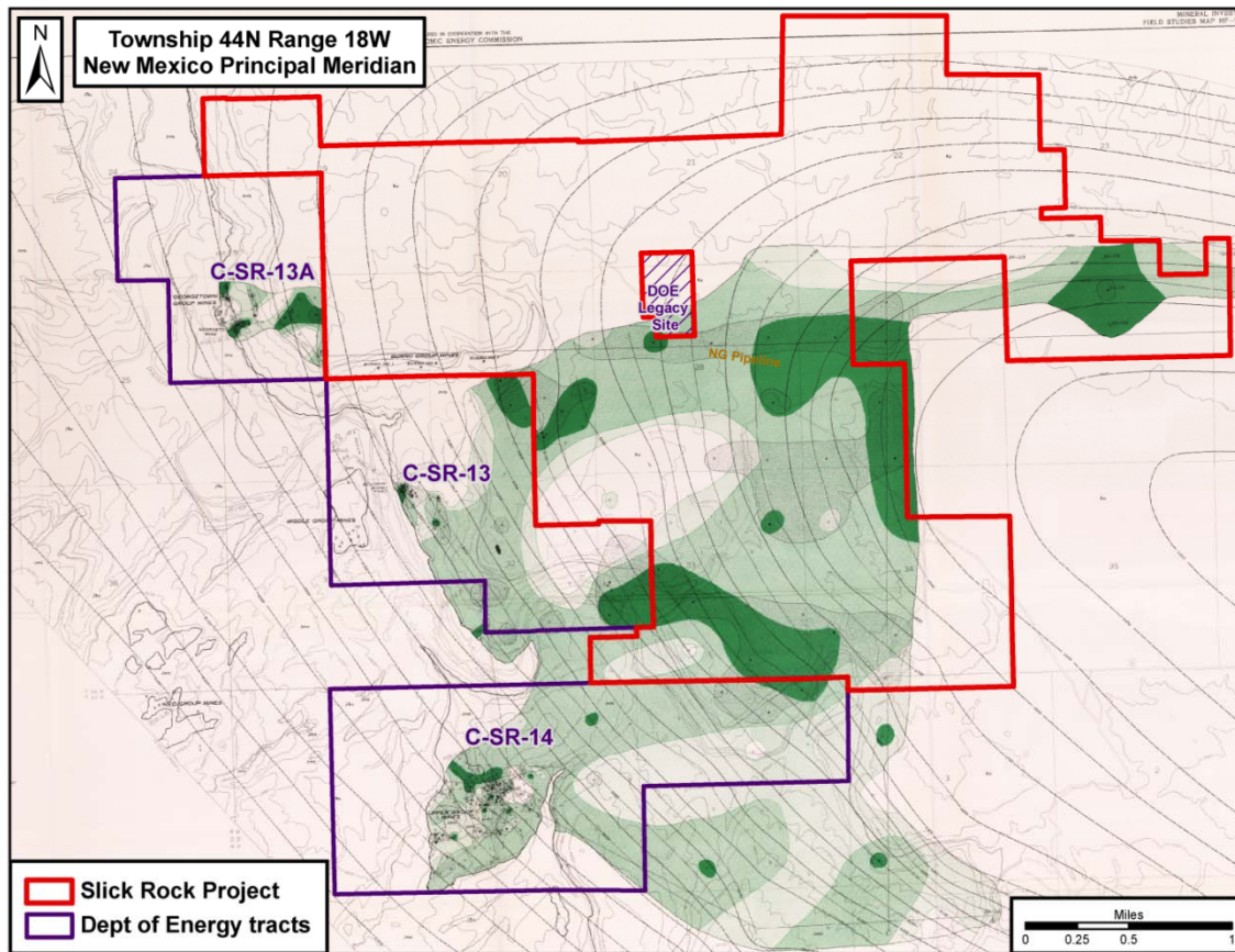
FIGURE 7.3: URANIUM FAVORABILITY MAP (ROGERS AND SHAW, 1962)
