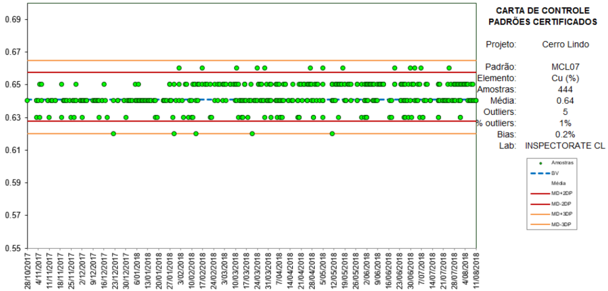
FIGURE 11-4 CRM “MCL07” RESULTS FOR COPPER – MINE AND CERTIMIN LABORATORIES – (2017-2018)
