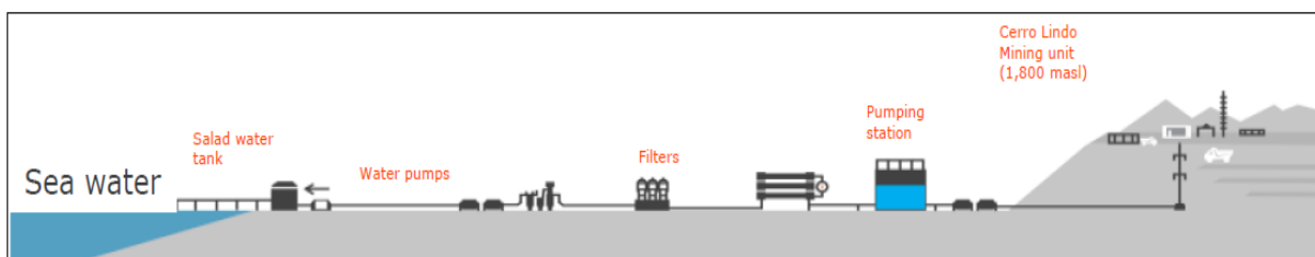
FIGURE 20-1 WATER SUPPLY SYSTEM FOR CERRO LINDO MINE
