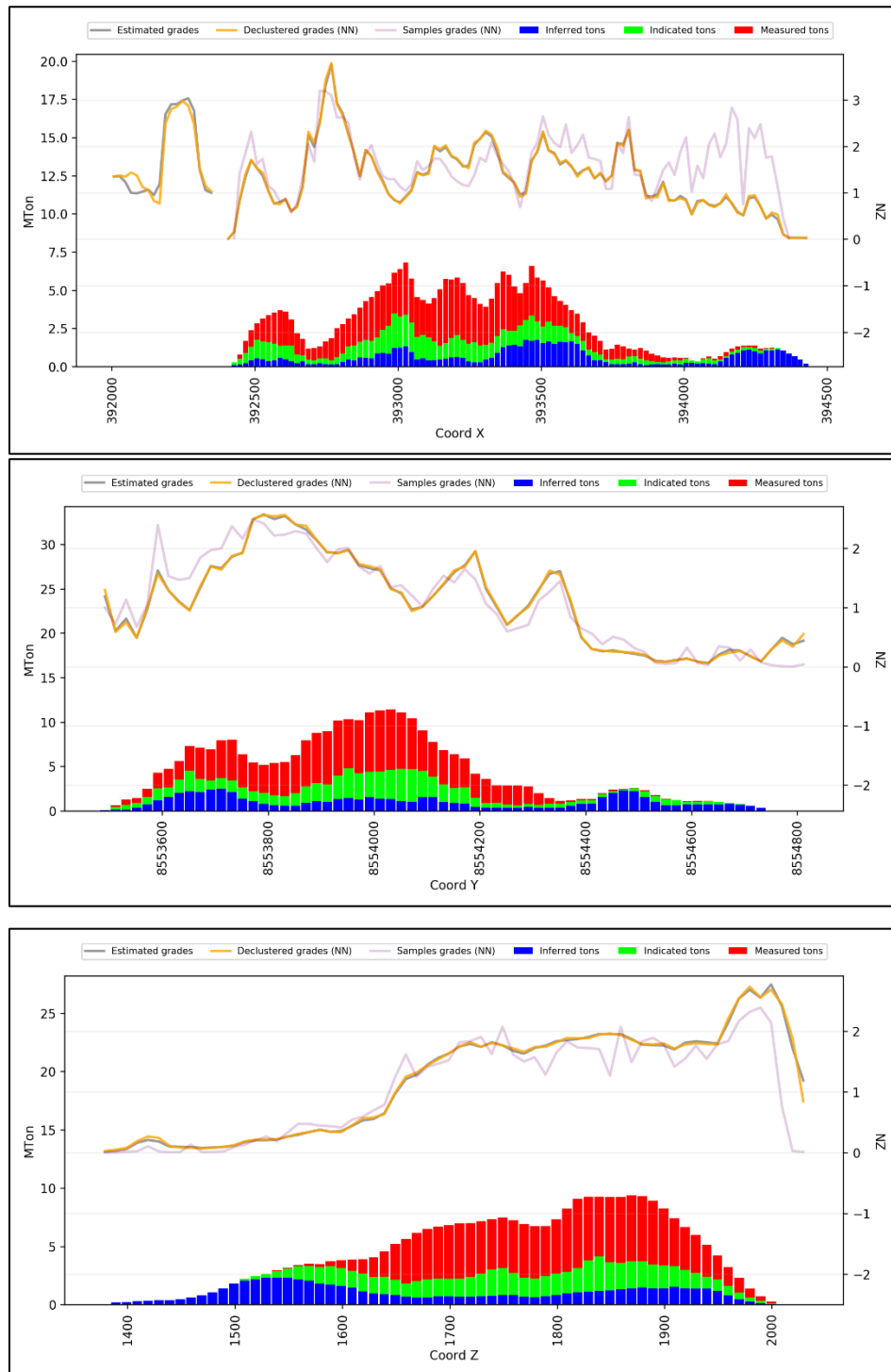
FIGURE 14-33 SWATH PLOT: ZN GRADE VARIATION ALONG X, Y, AND Z
