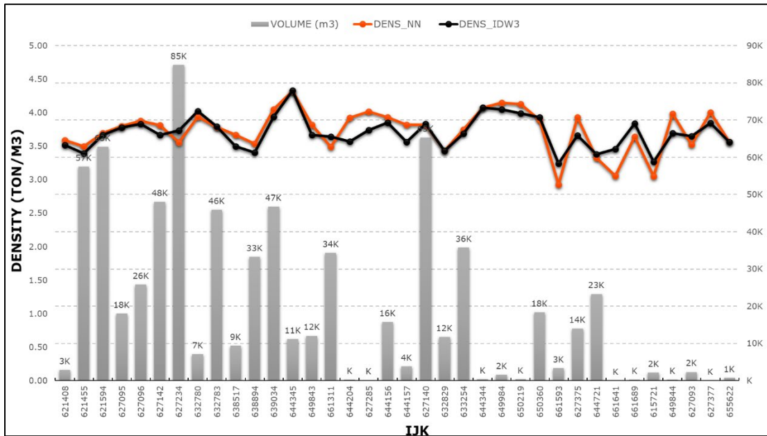
FIGURE 14-25 SSM SWATH PLOTS – DENSITY VALUES
