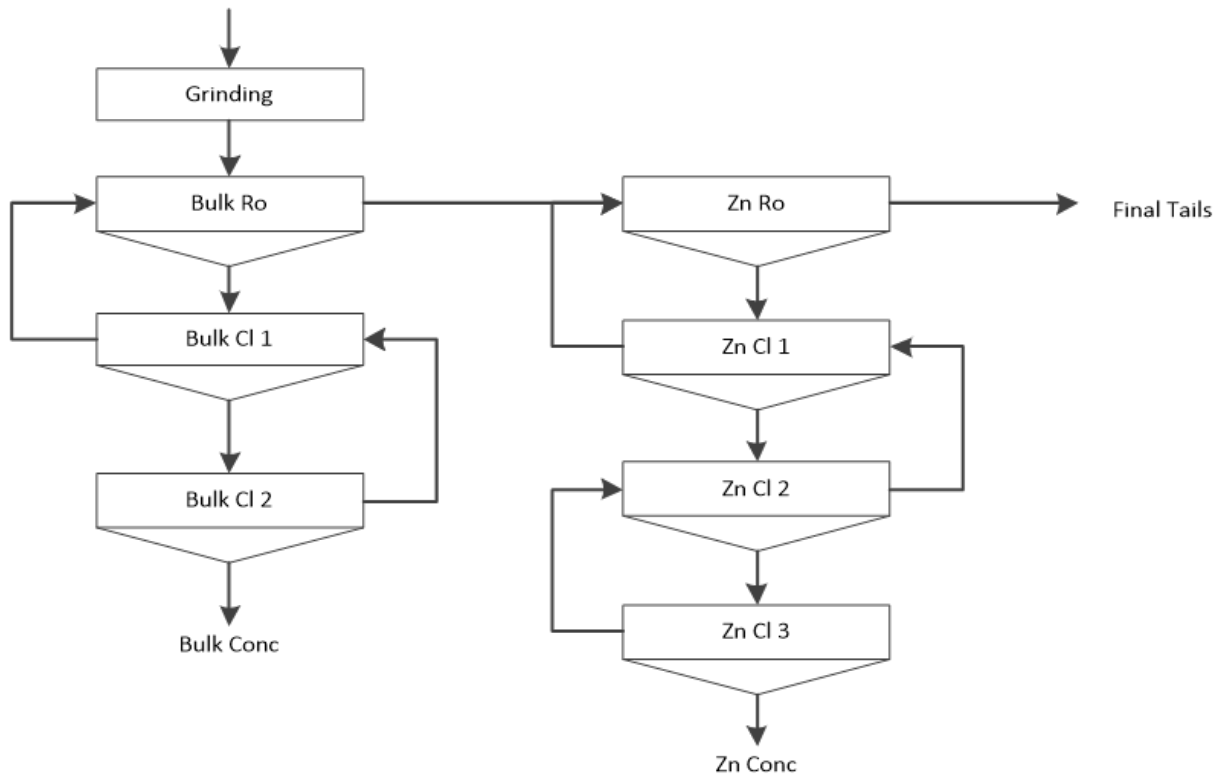
FIGURE 13-4 LOCKED CYCLE FLOTATION TEST FLOWSHEET
