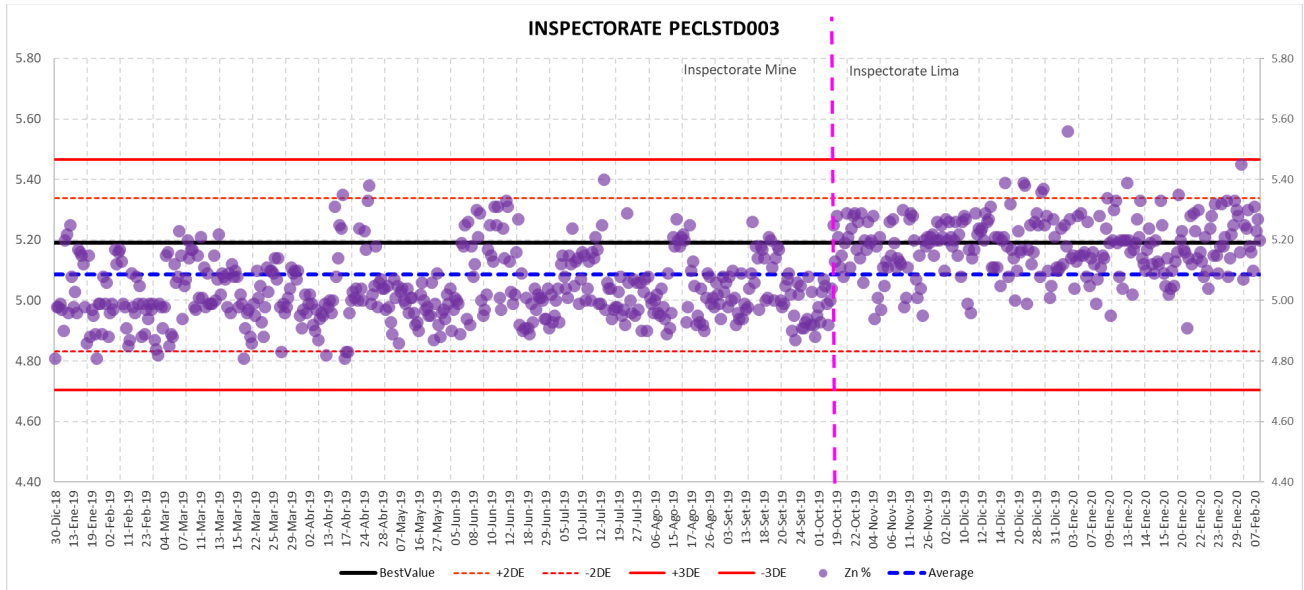
FIGURE 11-5 CERRO LINDO CRM ZN PERFORMANCE FOR PECLSDT003 (2018-2020)
