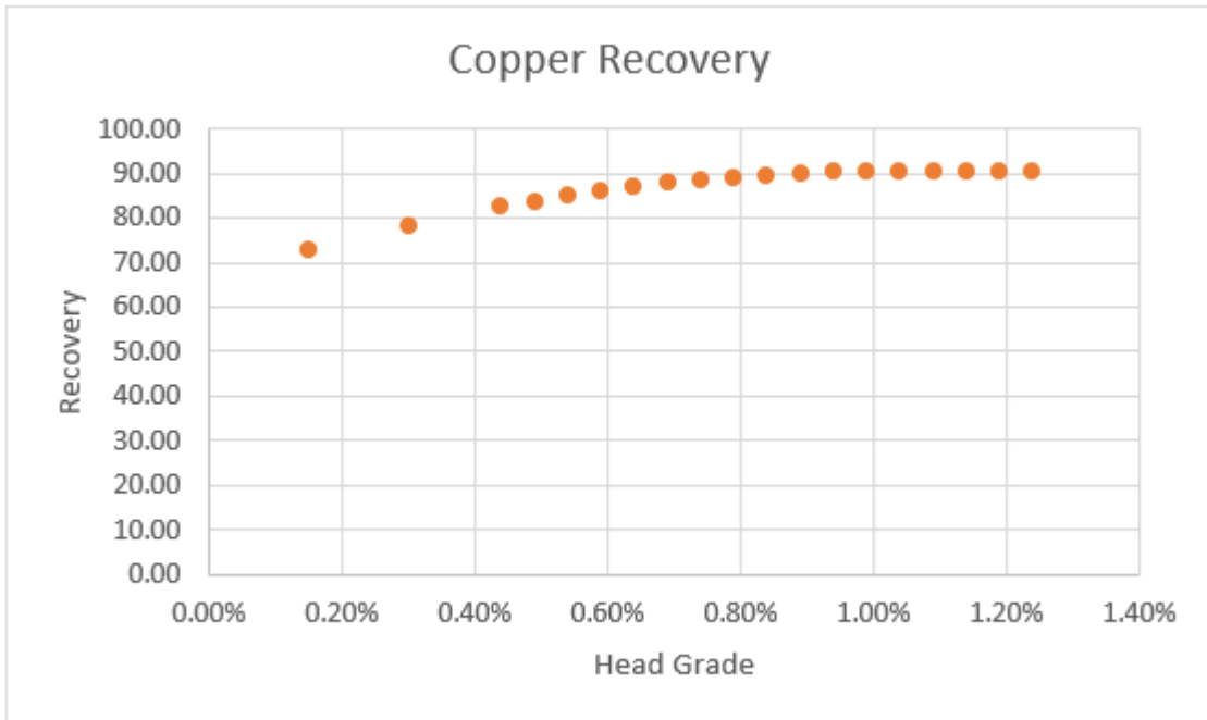
FIGURE 14-28 COPPER RECOVERY
