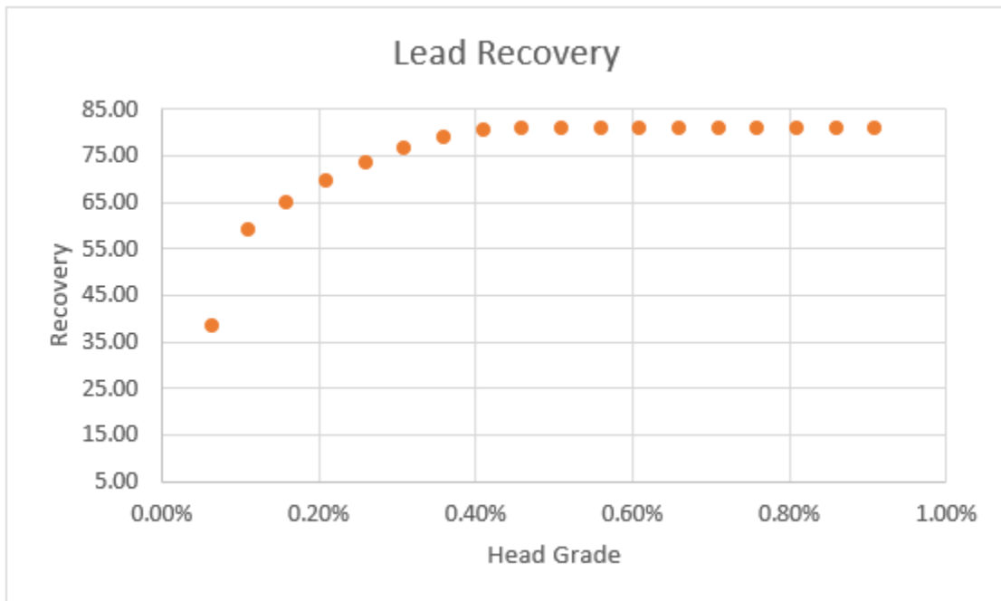
FIGURE 14-29 LEAD RECOVERY
