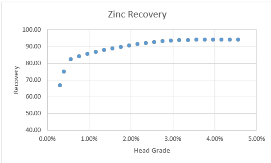
FIGURE 15-1 ZINC RECOVERY
