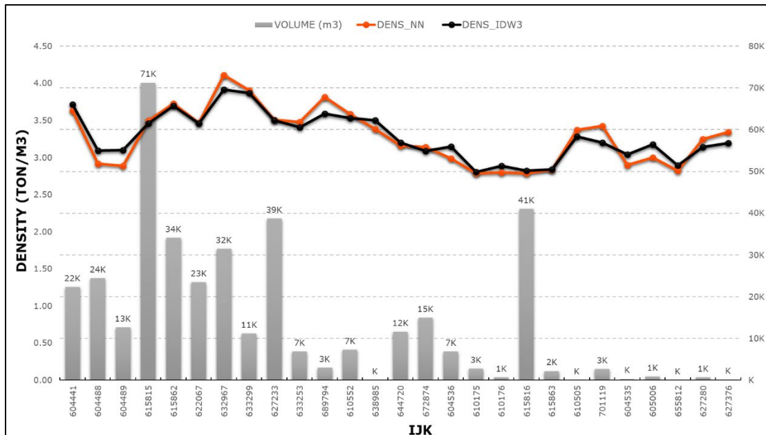
FIGURE 14-26 VM SWATH PLOTS – DENSITY VALUES
