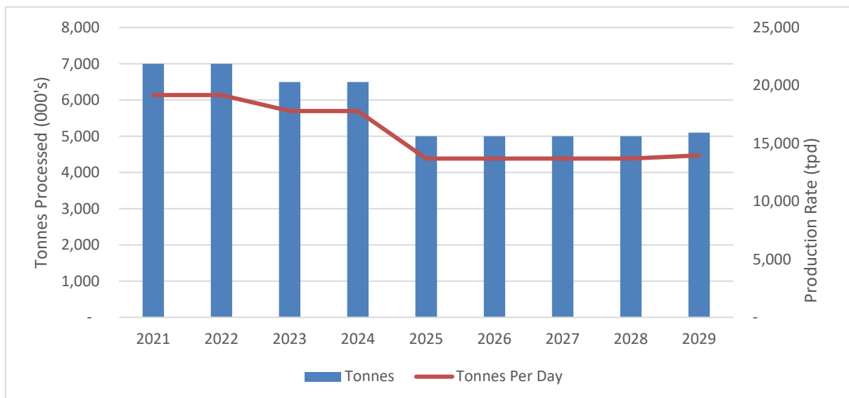
FIGURE 16-8 LOM PRODUCTION PROFILE
