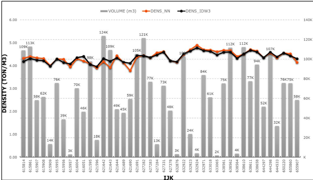
FIGURE 14-23 SPB SWATH PLOTS – DENSITY VALUES
