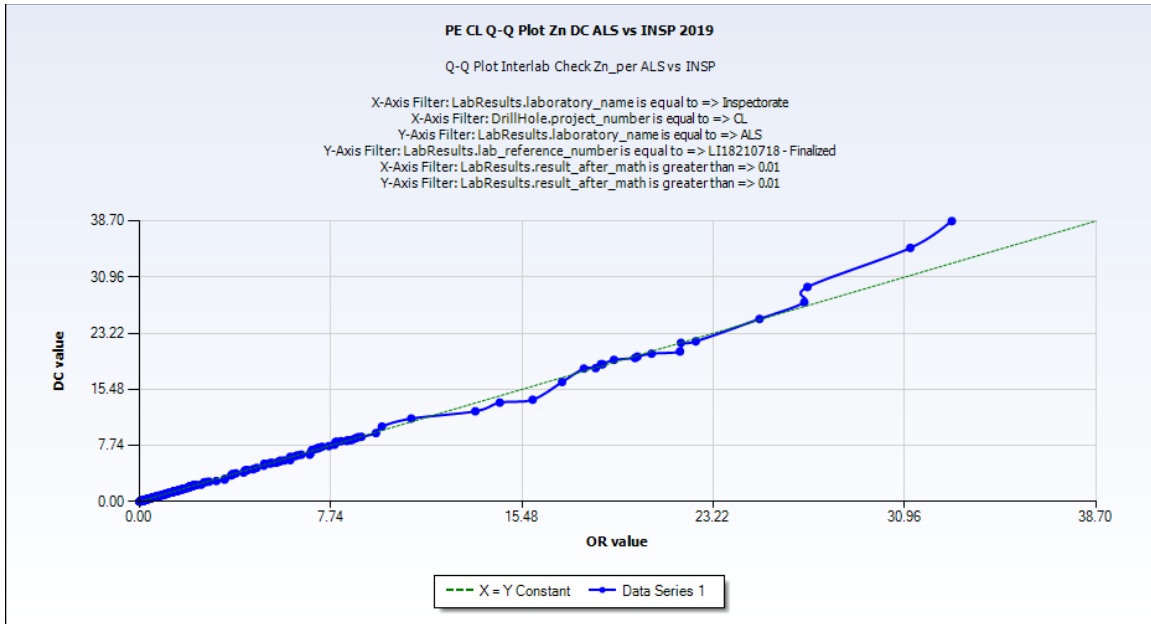
FIGURE 11-9 2018-2019 2020 CERRO LINDO ZN AND CU EXTERNAL CHECK ASSAYS – INSPECTORATE MINE LABORATORY
