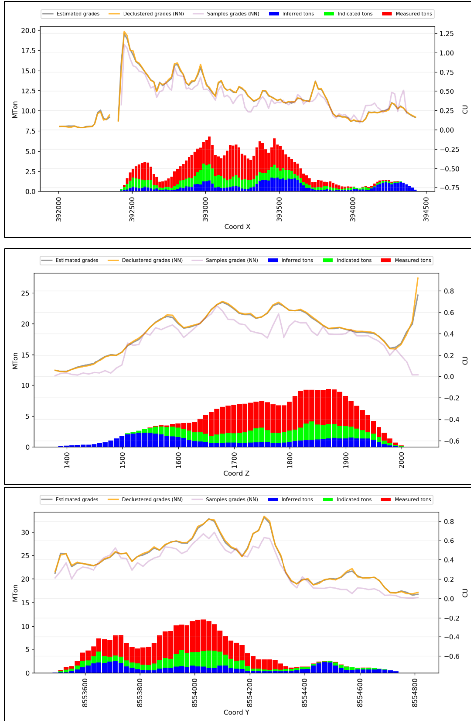
FIGURE 14-34 SWATH PLOT: CU GRADE VARIATION ALONG X, Y, AND Z
