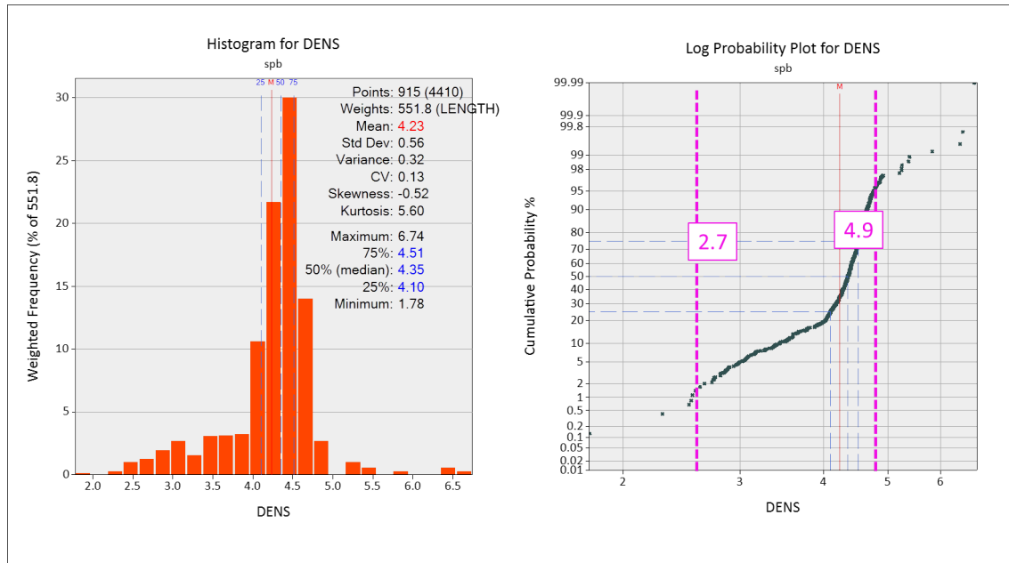
FIGURE 14-21 DENSITY CAPPING ANALYSIS FOR SPB DOMAIN
