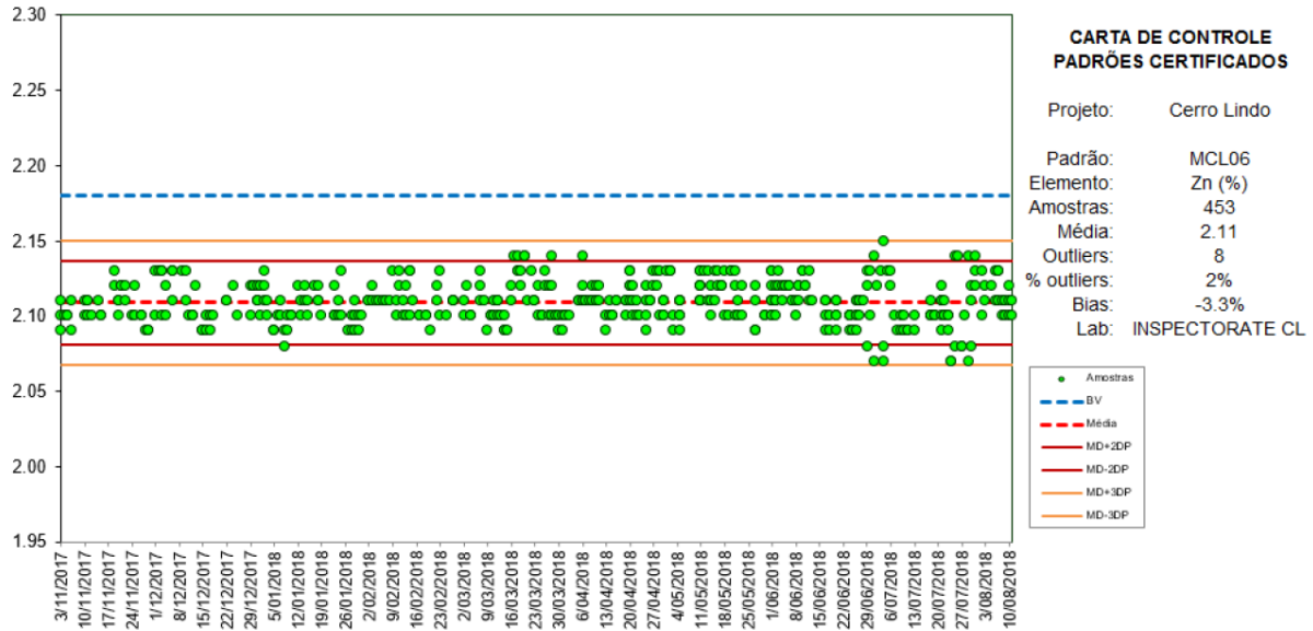
FIGURE 11-3 CRM “MCL06” RESULTS FOR ZINC – MINE AND CERTIMIN LABORATORIES – (2017-2018)
