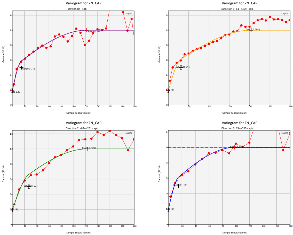
FIGURE 14-18 ZN VARIOGRAM FOR MINERALIZATION SPB DOMAIN
