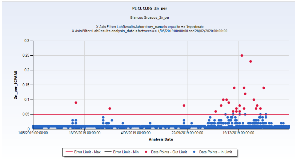
FIGURE 11-7 2019-2020 CERRO LINDO BLANK ZN AND CU ASSAYS – INSPECTORATE MINE LABORATORY
