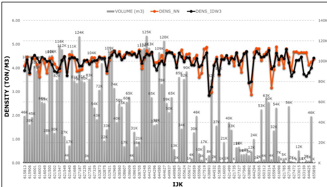
FIGURE 14-24 SPP SWATH PLOTS – DENSITY VALUES
