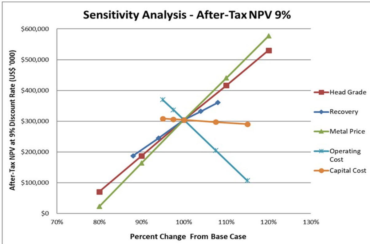
FIGURE 22-1 AFTER-TAX NPV SENSITIVITY GRAPH
