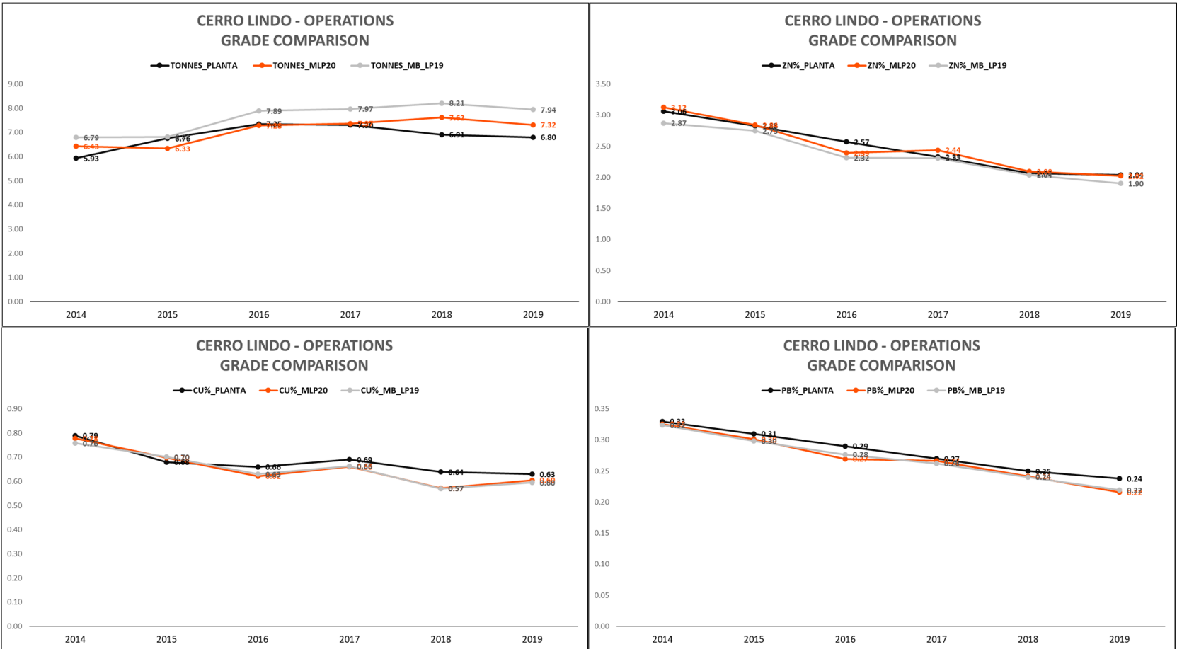
FIGURE 14-37 PLANT VERSUS RESOURCE MODEL RECONCILIATION
