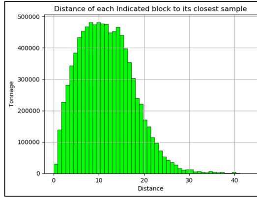
FIGURE 14-30 VALIDATION OF CLASSIFICATION (SPB AND SPP) SPB
