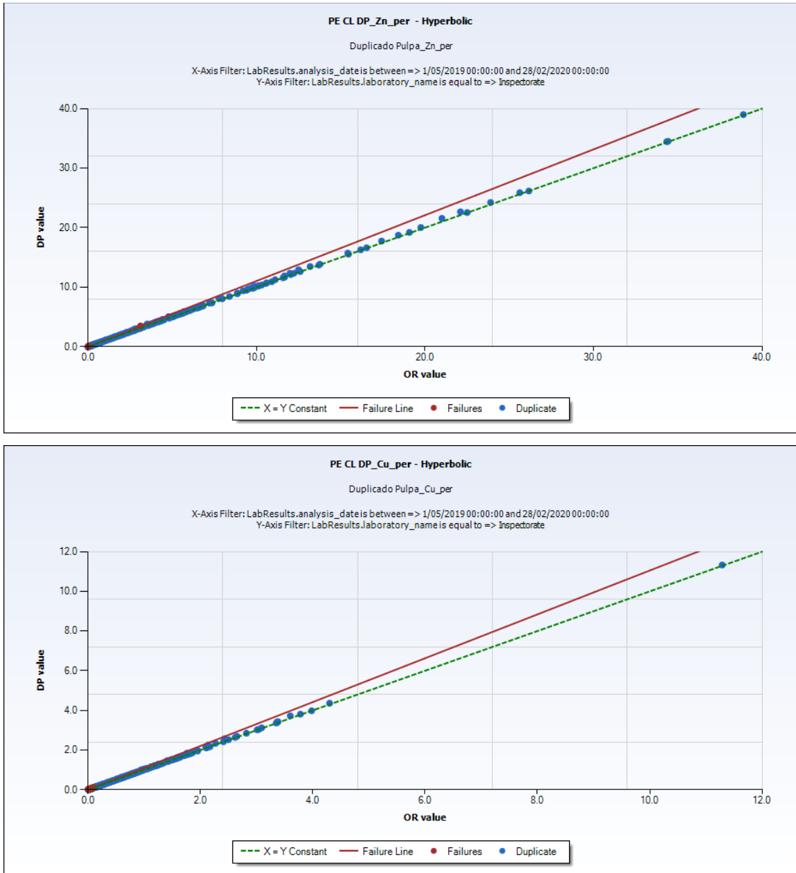
FIGURE 11-8 2019-2020 CERRO LINDO PULP DUPLICATES ZN AND CU ASSAYS – INSPECTORATE MINE LABORATORY
