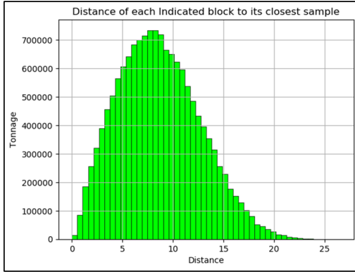
FIGURE 14-31 VALIDATION OF CLASSIFICATION (SSM AND VM) SSM
