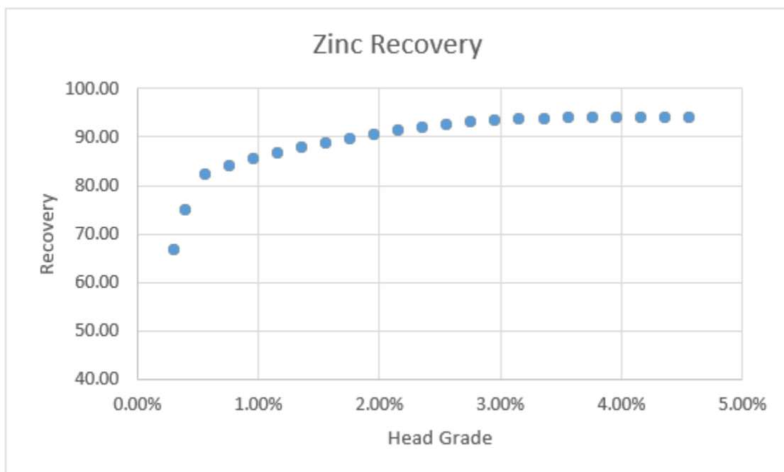
FIGURE 14-27 ZINC RECOVERY
