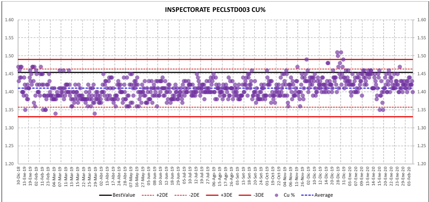
FIGURE 11-6 CERRO LINDO CRM “PECLSDT003 (2018-2020)” RESULTS FOR COPPER – INSPECTORATE MINE LABORATORY
