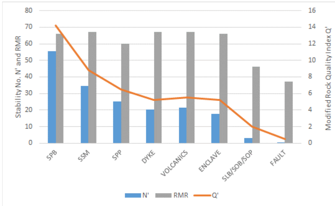
FIGURE 16-5 STABILITY AND ROCK QUALITY INDICES
