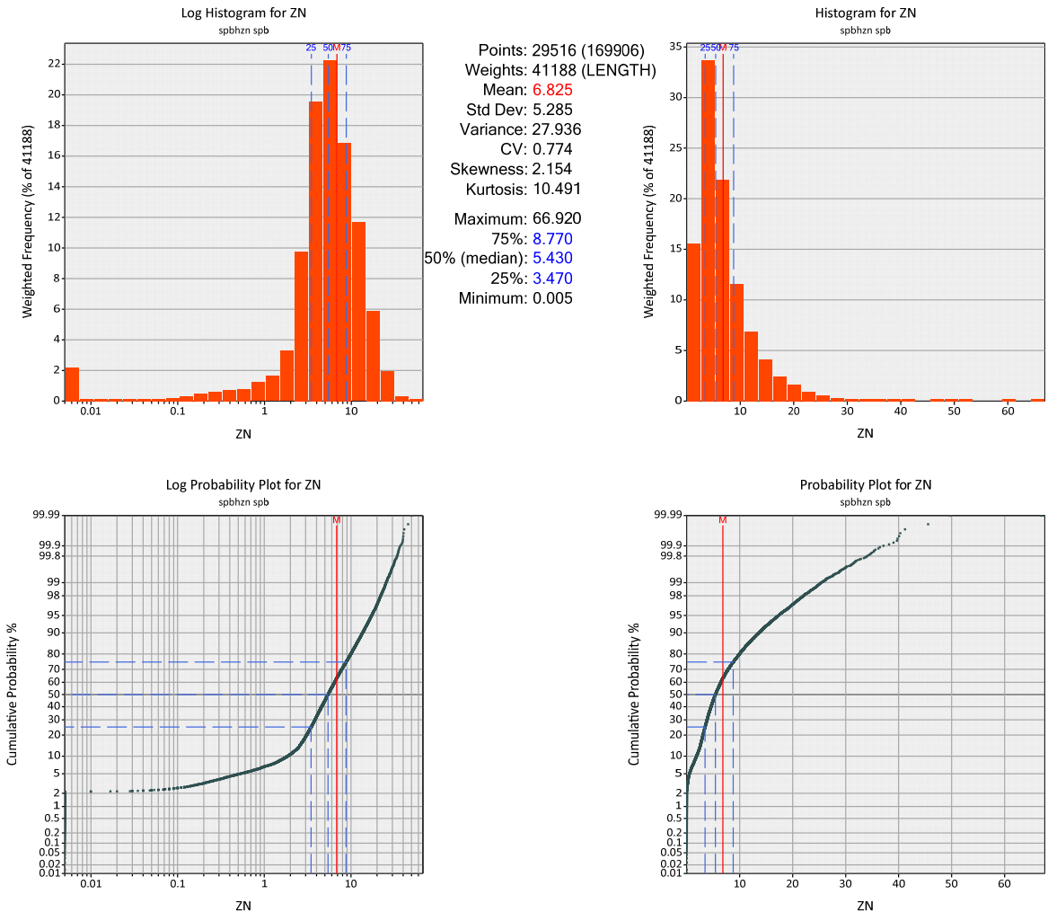
FIGURE 14-13 CAPPING ANALYSIS FOR SPB ZN HIGH GRADE MINERALIZATION
