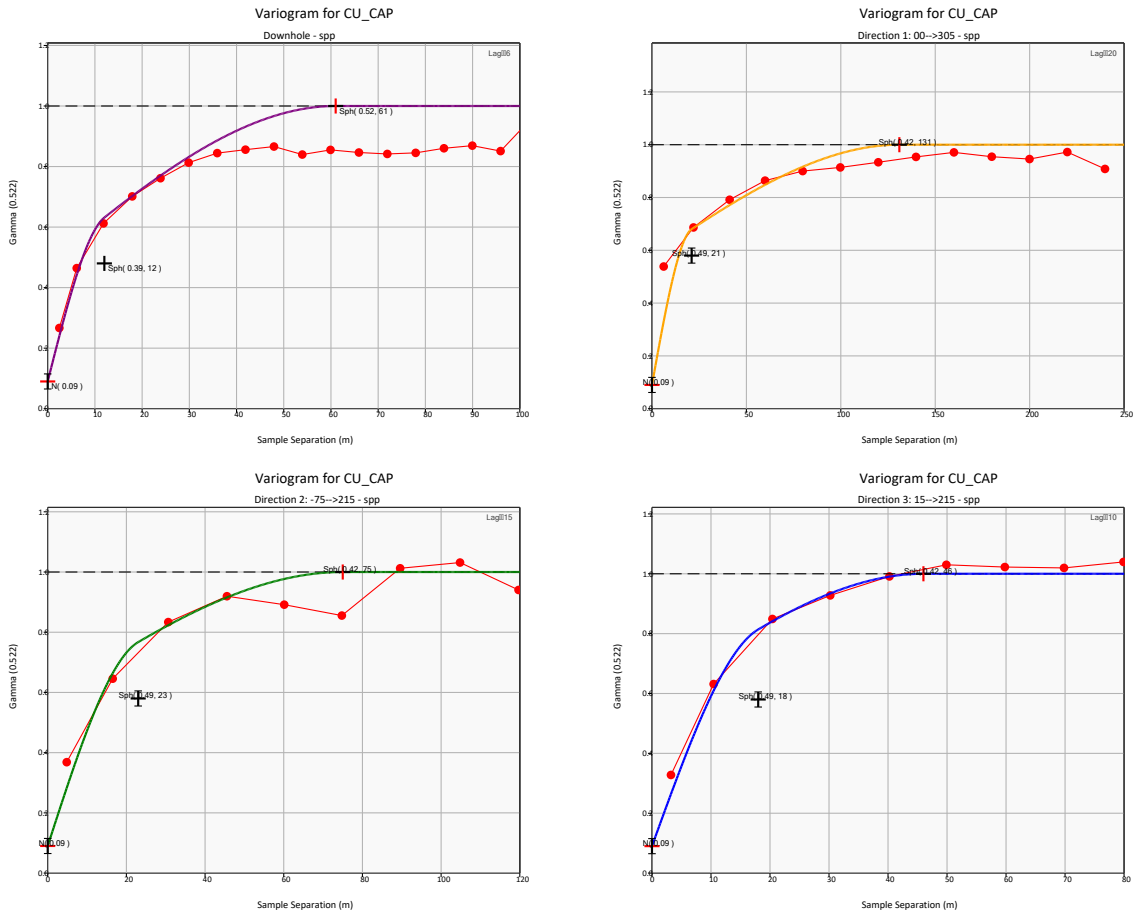
FIGURE 14-19 CU VARIOGRAM FOR MINERALIZATION SPP DOMAIN
