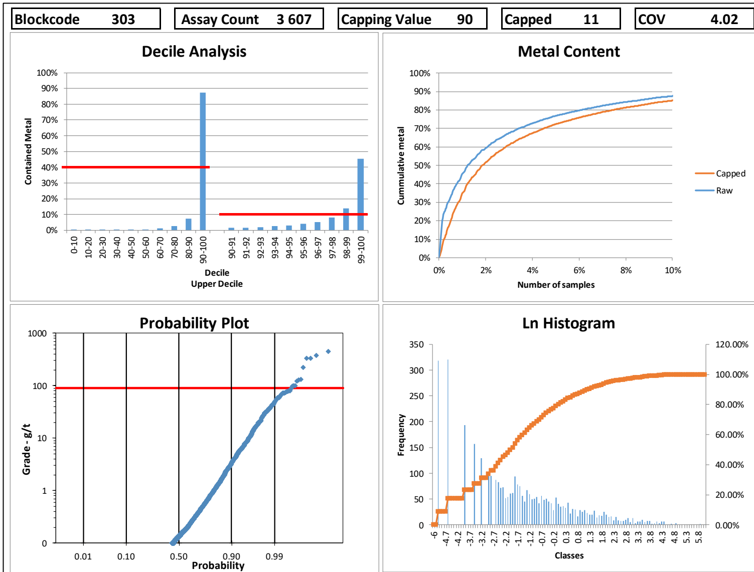
Figure 14.5 – Graphs supporting a capping value of 90 g/t Au for Zone 3
