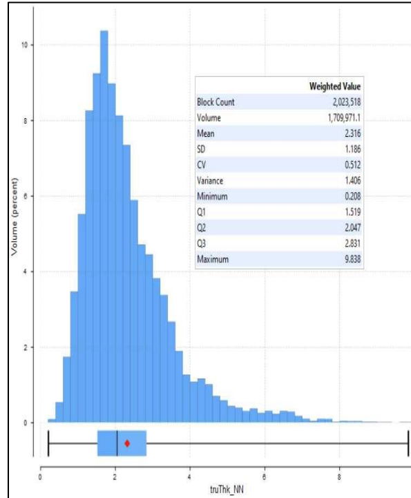
Figure 14.2: Histogram of T_T Where GT_T > 4.0
