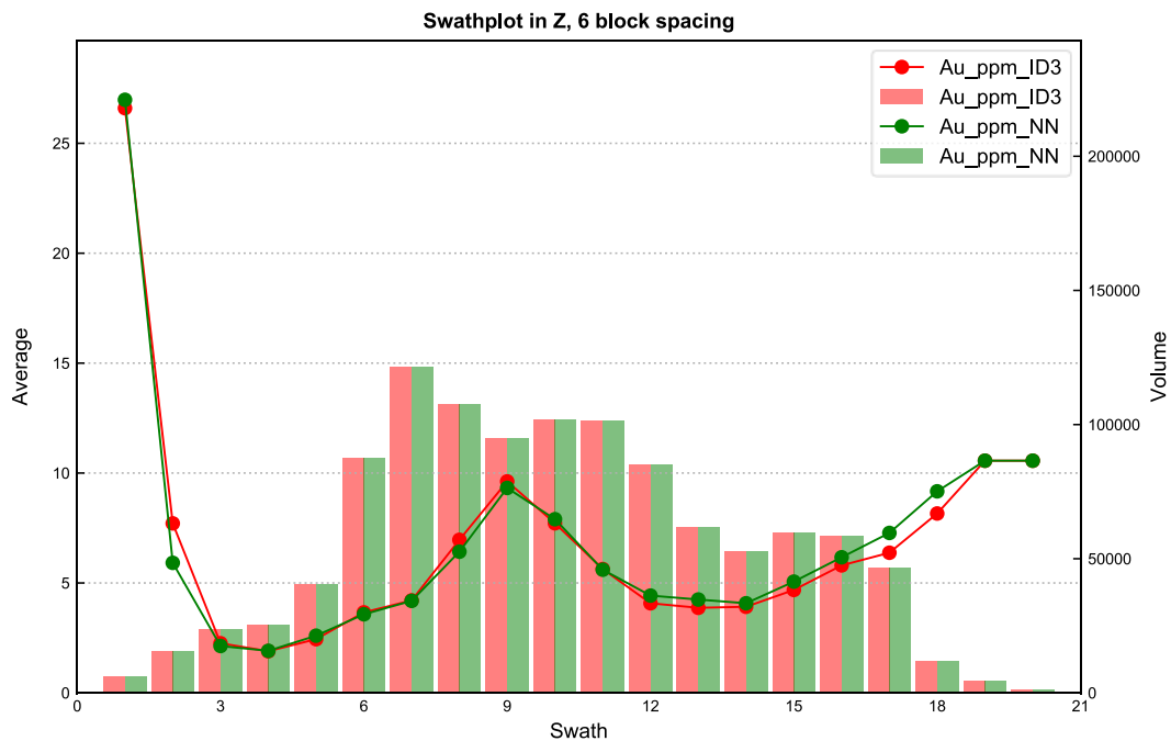
Figure 14.7: Swath Plot Example (HM Y and Z, Width 30 m)
