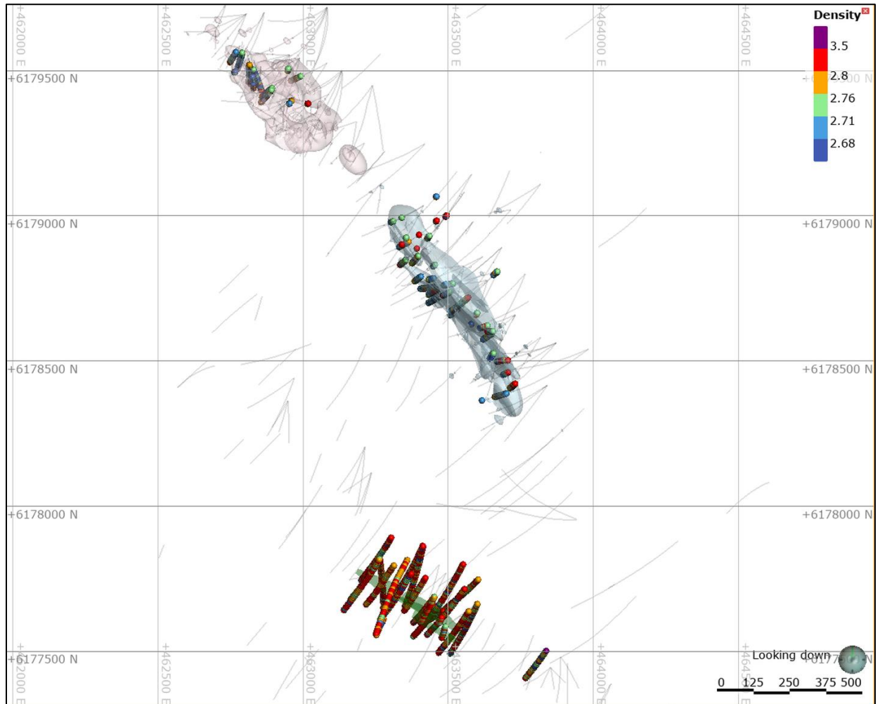
Figure 14.4: Plan View of Bulk Density Sample Distribution
