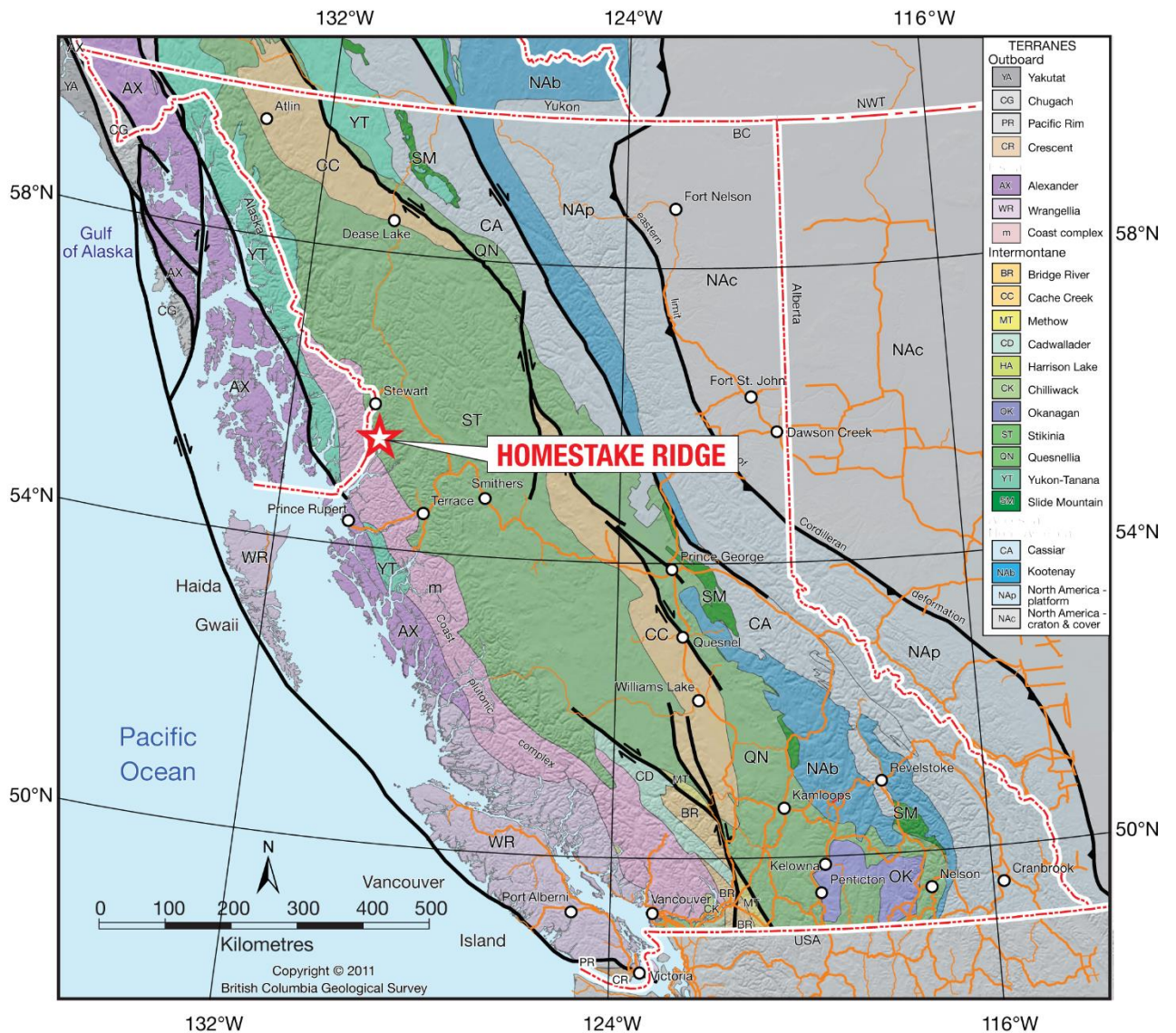
Figure 7.1: Regional Geology
