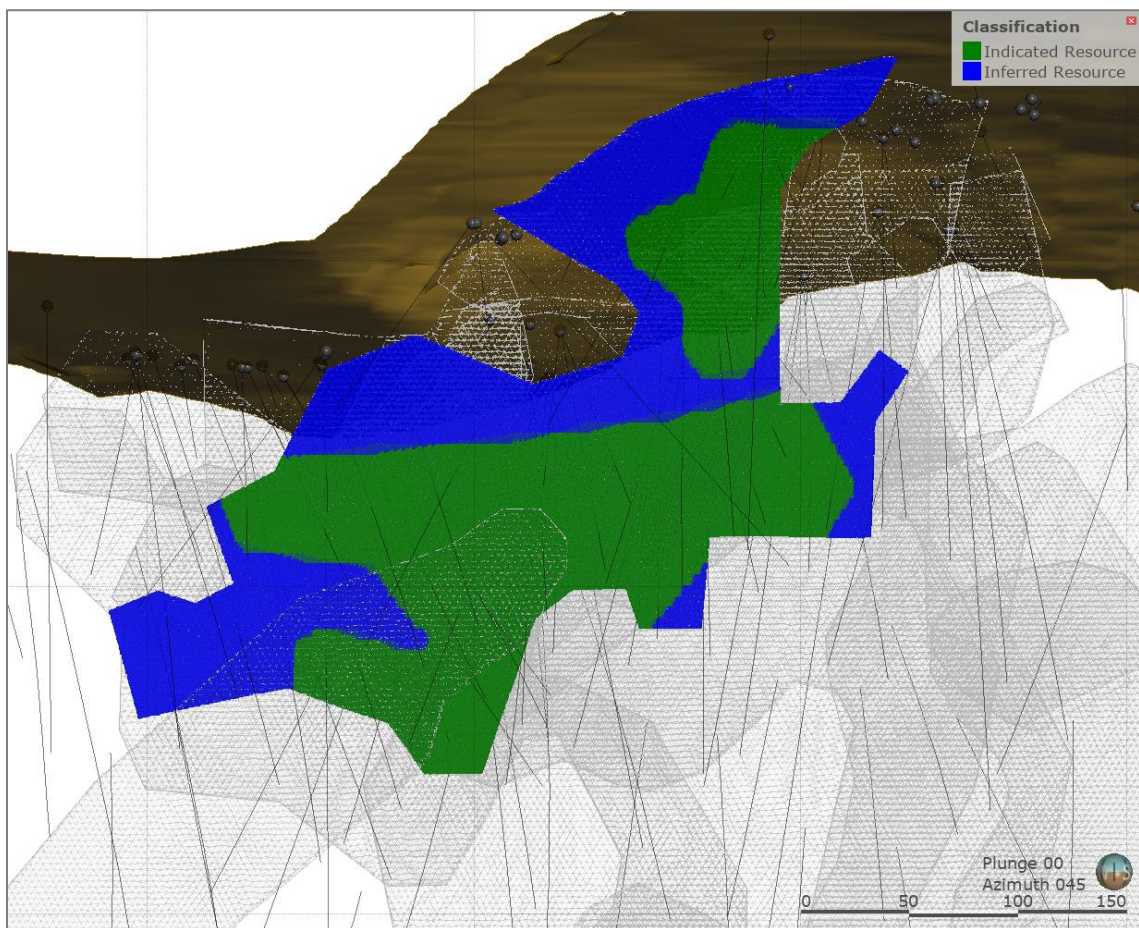
Figure 14.8: Indicated Resource and Inferred Resource. HM02 vein of HM zone Example. Vertical Section Looking NE
