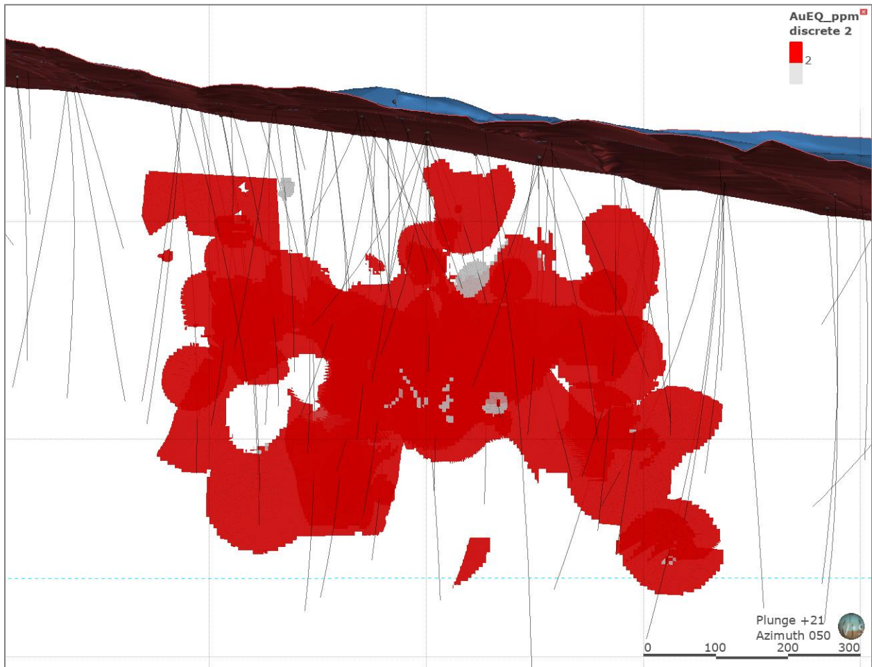
Figure 14.3: Inferred and Indicated Mineral Resource Blocks \geq 4.0 g/t AuEq* T_T : HS Zone Example, Vertical Section Looking NE
