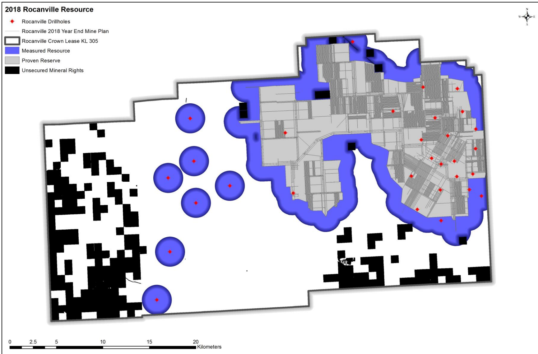
Figure 20: Map showing Rocanville Mineral Reserve with mine workings to December 2018.
