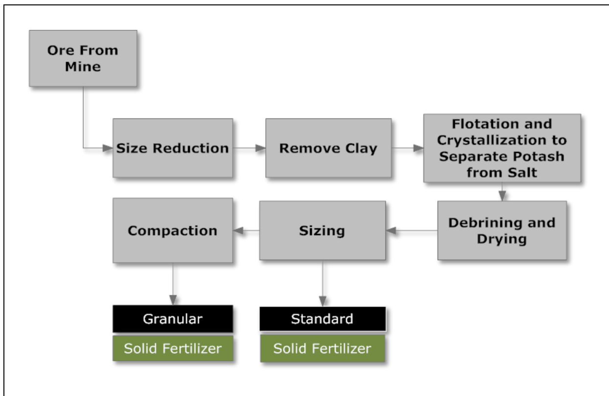
Figure 23: Simplified flow diagram for potash flotation and crystallization milling methods used at Rocanville.
