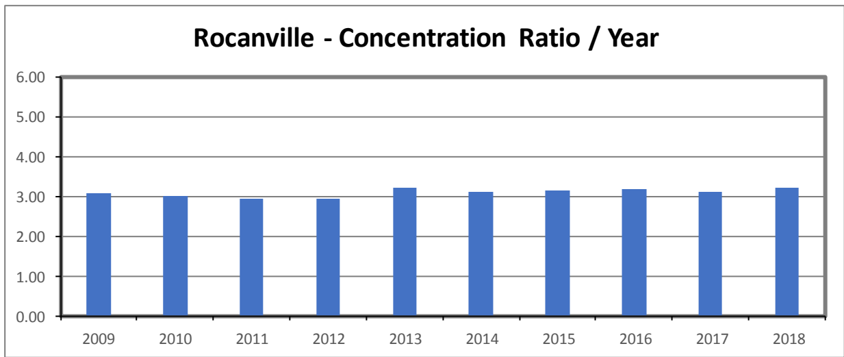
Figure 22: Actual mining, production and concentration ratio for the Rocanville mine over the past 10 years.
