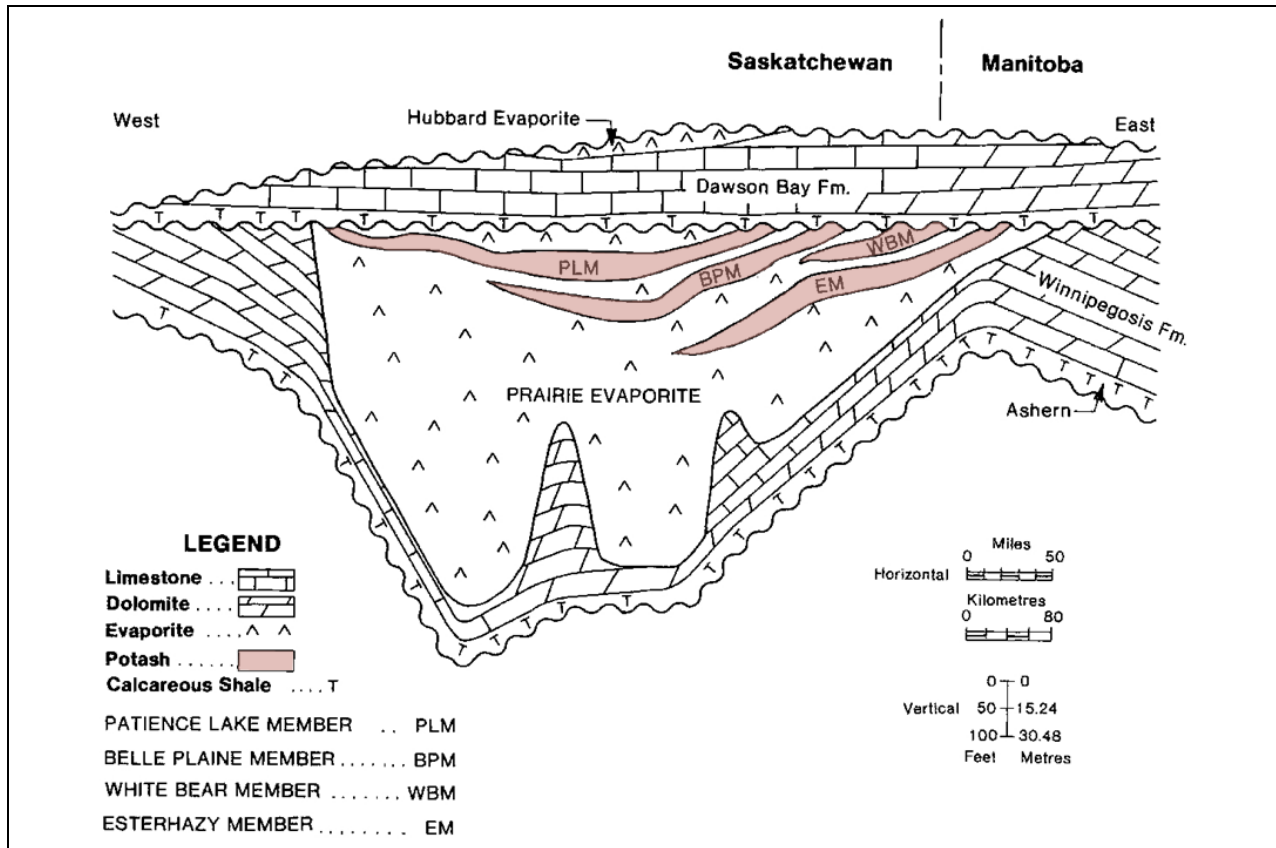
Figure 9: Schematic cross-section across southern Saskatchewan of the Prairie Evaporite Formation showing relative position of potash members. At Rocanville, potash is mined from the Esterhazy Member, labeled “EM” (from Fuzesy, 1982).
