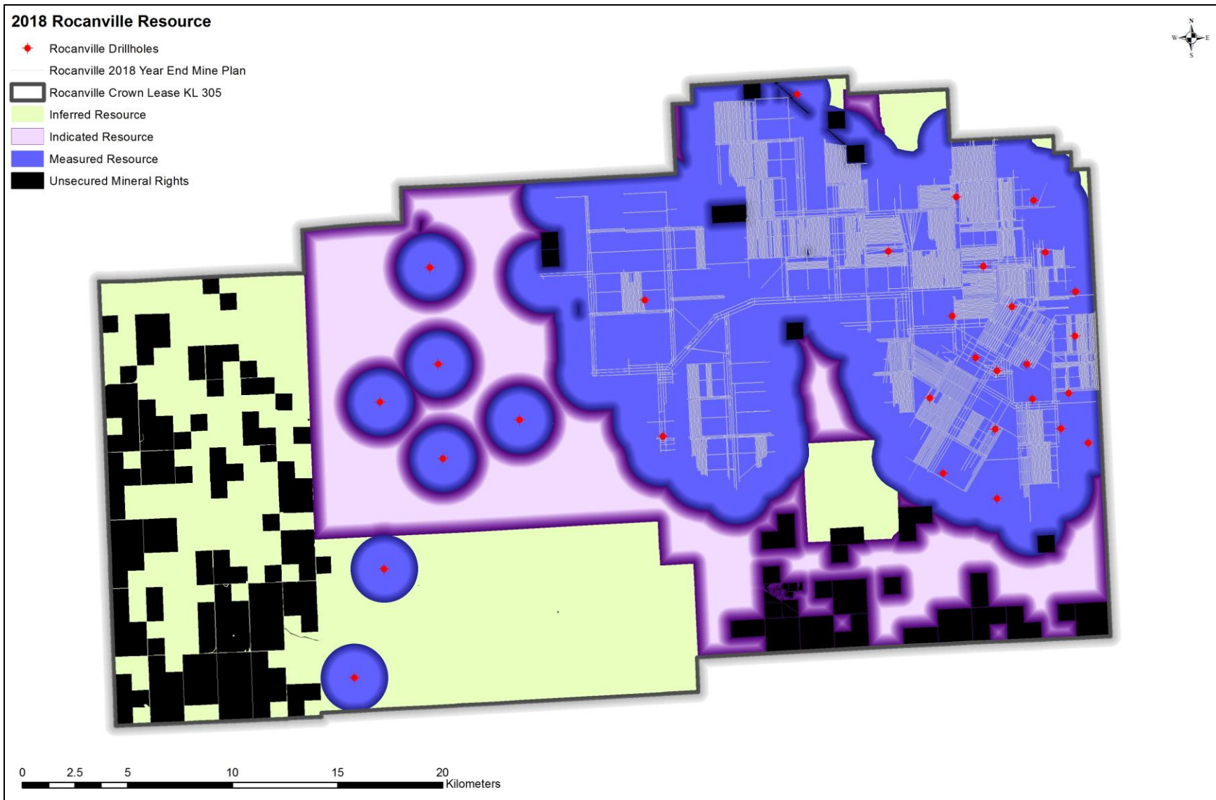
Figure 19: Map showing Rocanville Mineral Resource with mine workings to December 2018.
