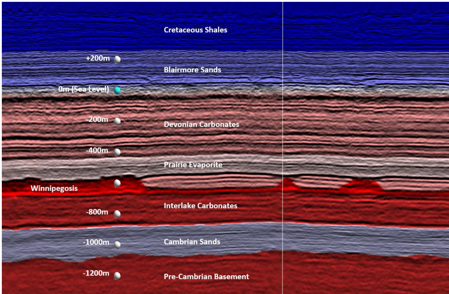
Figure 13: Seismic section from the Rocanville 2007 3D seismic data volume showing relative rock velocities of fast (red), slow (blue) and in between (white/pink). Vertical exaggeration is 2X, Sea Level (SL) is marked in metres, and major geological units are labeled.
