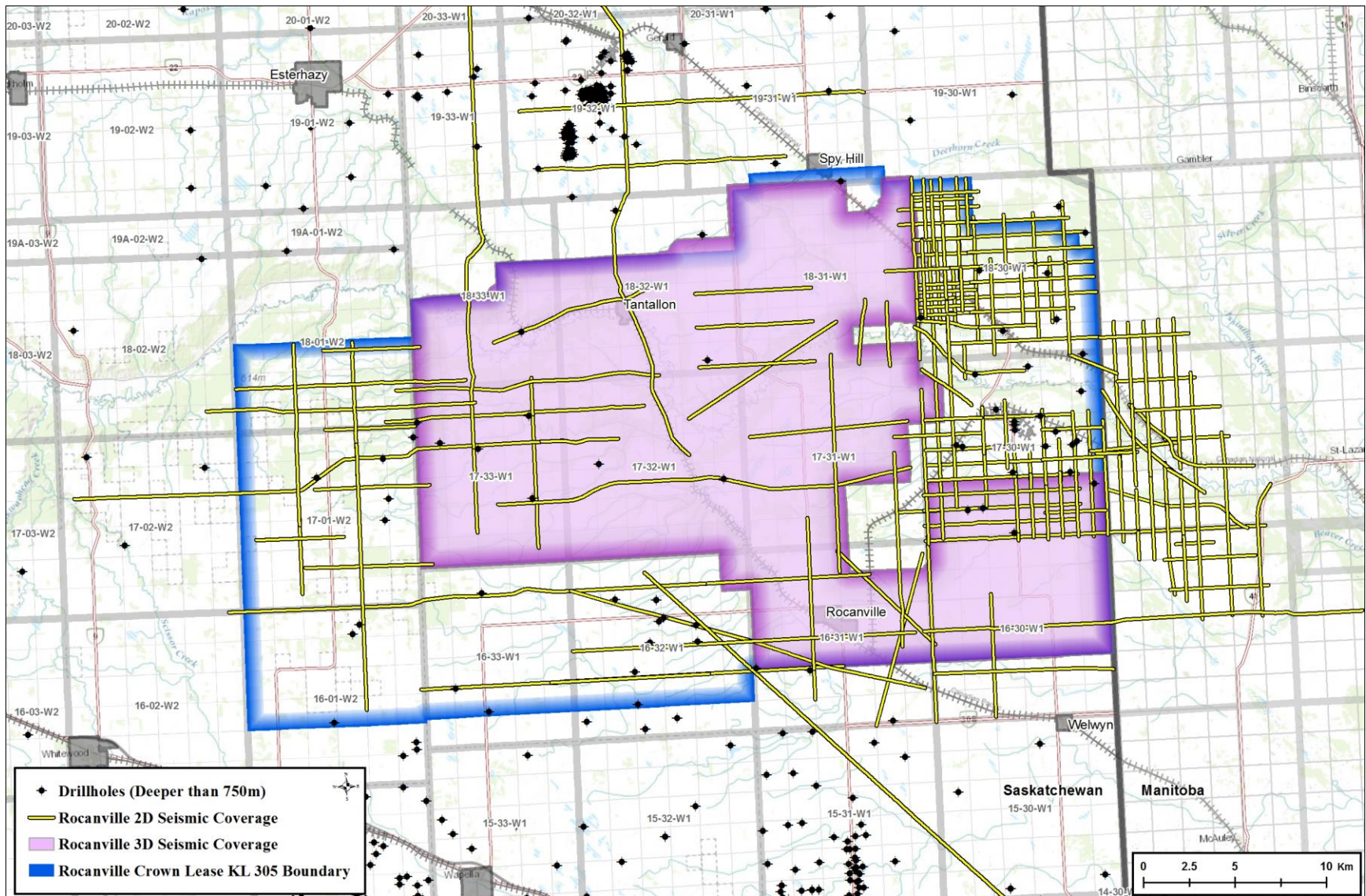
Figure 10: Potash exploration at Rocanville (2D & 3D surface seismic and drillholes deeper than 750 m).
