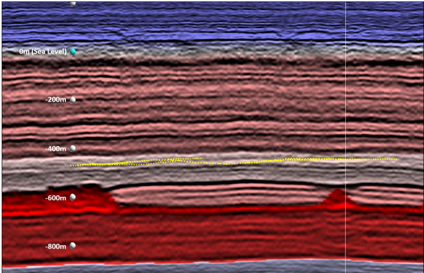
Figure 14: Detail of seismic section from the Rocanville 3D seismic data volume (see text for explanation). Mine room is marked in yellow. Ground surface is at approximately +500 m above Sea Level.
