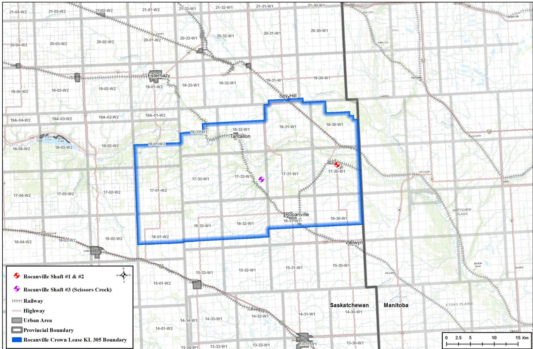
Figure 6: Map showing infrastructure (towns, rivers, roads, and railways) near Rocanville Potash. Rocanville shaft locations are shown in red and purple.
