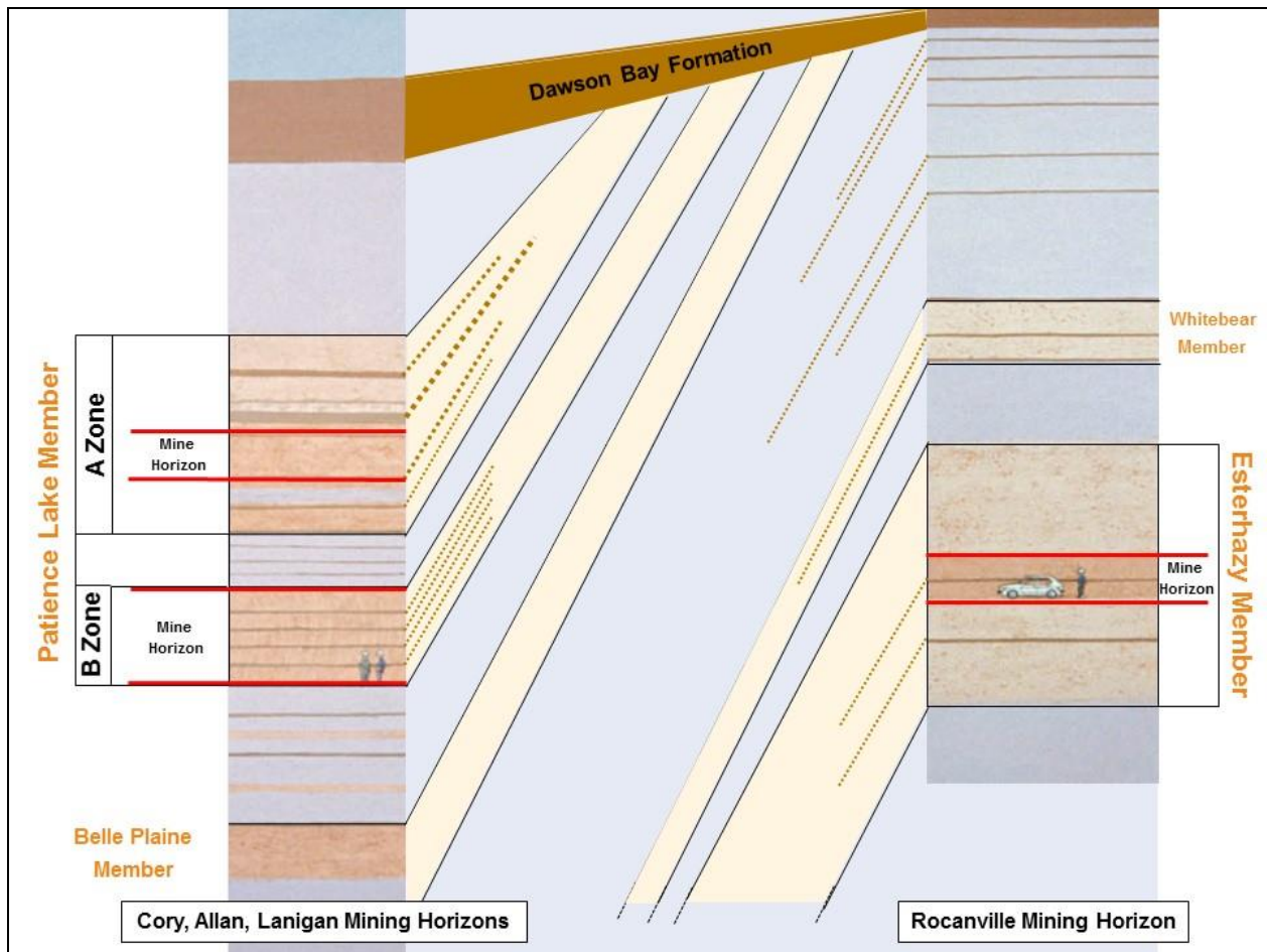
Figure 21: Typical stratigraphic section correlated with composite photos covering both the Patience Lake Member and the Esterhazy Member potash production intervals. At Rocanville, mining takes place in the Esterhazy Member.
