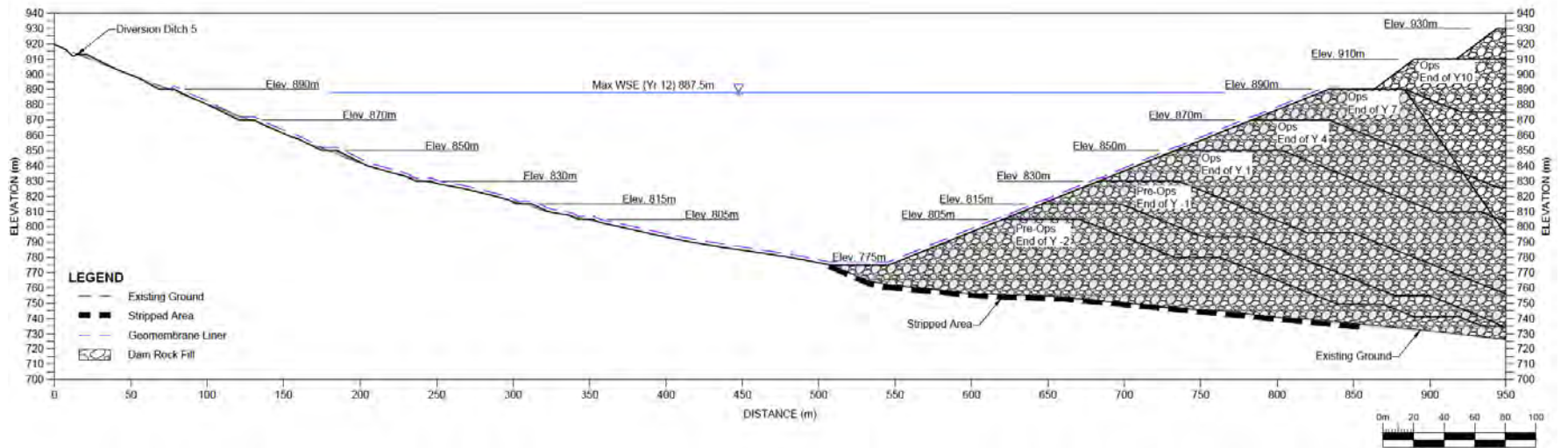
Figure 18-11 Cross Section of the TMF and raises to Final Design Elevation (SRK, 2020)
