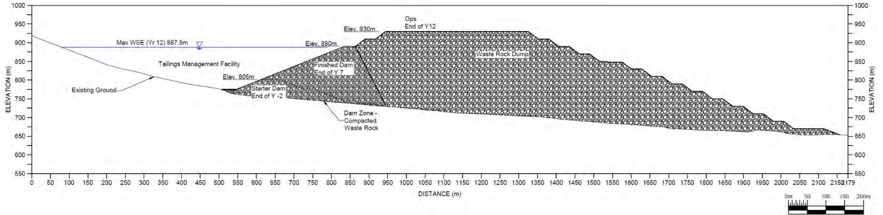
Figure 18-10 Cross Section through the TMF & WRF showing Starter Dam to Elevation 805 m (SRK, 2020)
