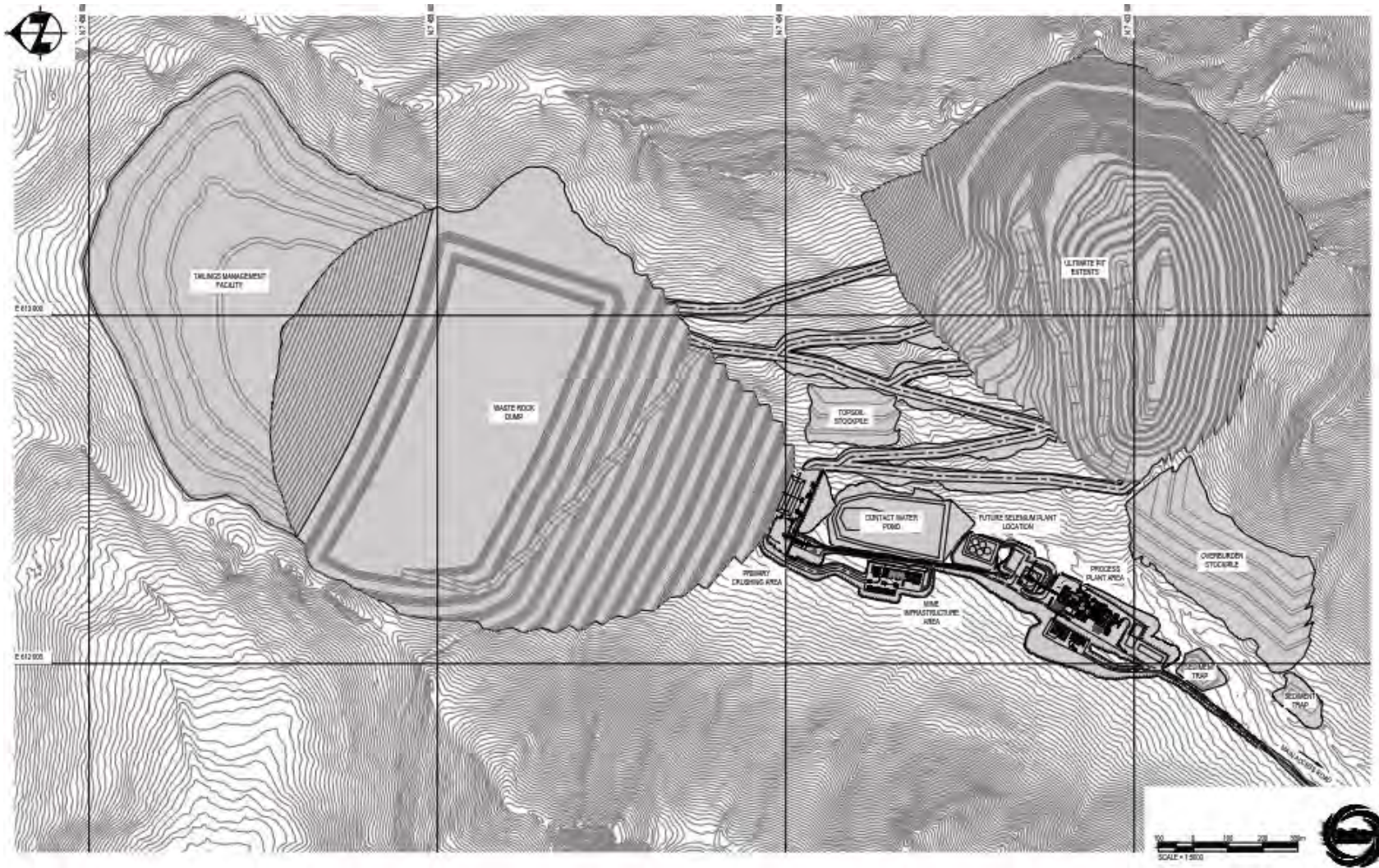
Figure 18-1 Proposed Site Layout (Ausenco, 2020)
