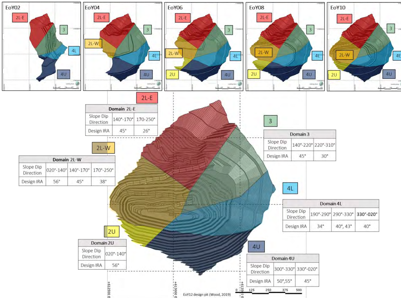
Figure 9-8 Recommended Inter-Ramp Angles by Slope Design Sector (Wood, 2019)
