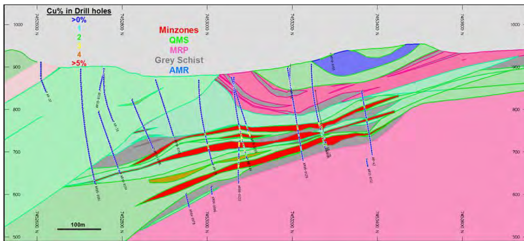
Figure 14-7 Cross Section 745300N Showing Lithology Domains at Arctic (Sim, 2019)
