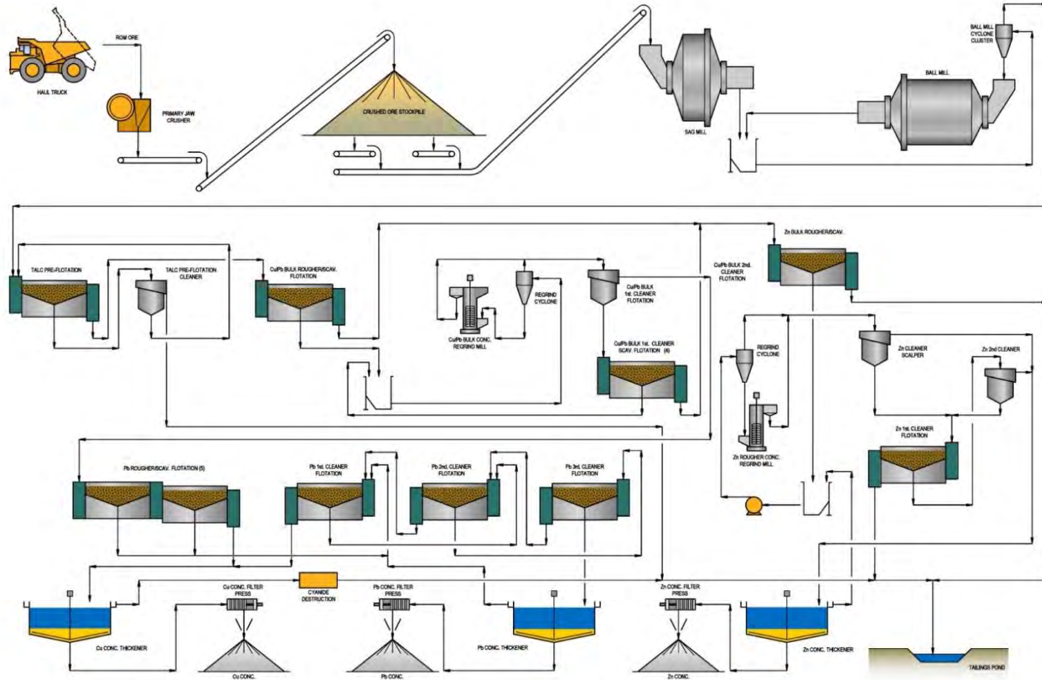
Figure 17-1 Simplified Process Flowsheet (Ausenco 2020)
