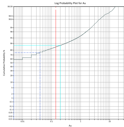
Figure 14.1 Example log probability plot from Kilosegui showing grade threshold for mineralised zone definition at 0.2g/t
