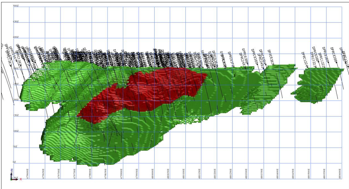
Figure 14.20: Long section View of Nokpa Indicated and Inferred.
