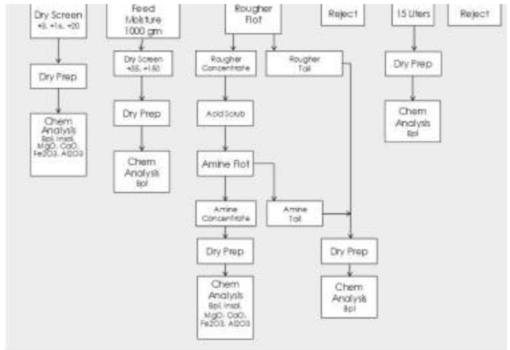
Figure 8-1: Core Sample Preparation Flow Sheet
