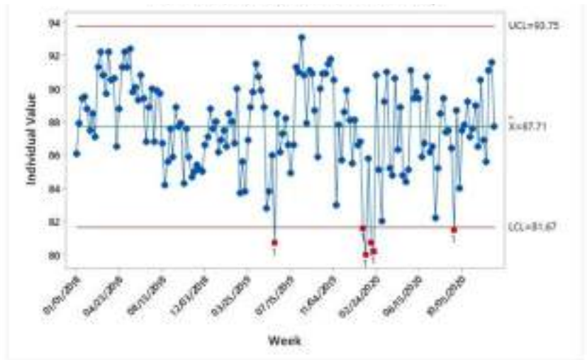
Figure 10-4: South Fort Meade Plant Recovery Control Chart
