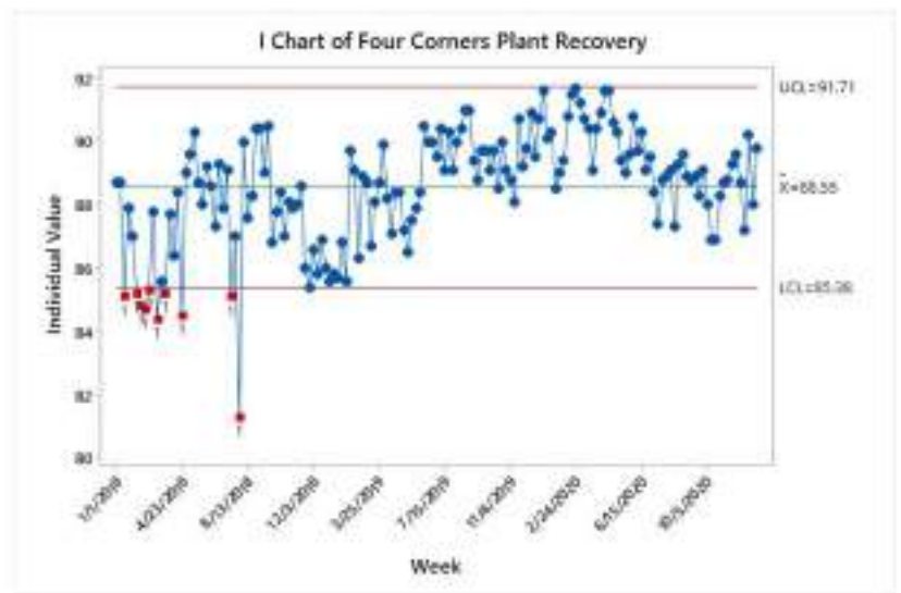
Figure 10-5: Four Corners Plant Recovery Control Chart
