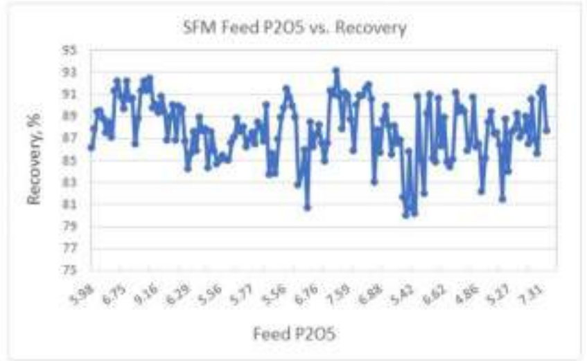
Figure 10-1: South Fort Meade Feed P 2 O 5 Grade vs. Recovery%
