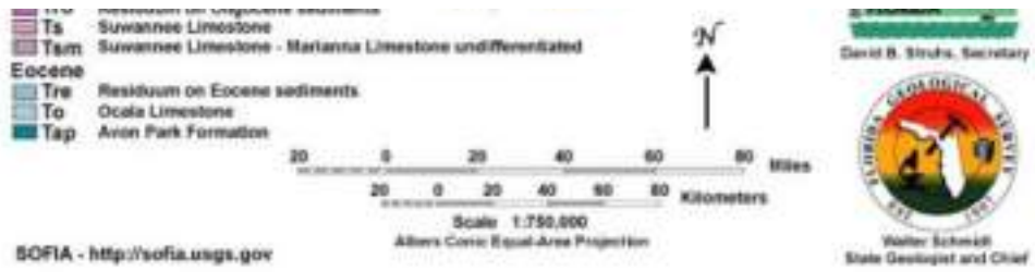
Figure 6-1: Regional Geology
