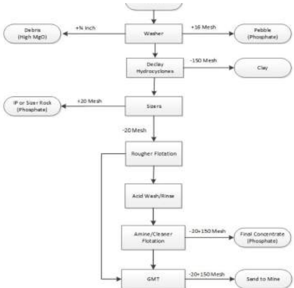
Figure 14-1: Phosphate Beneficiation Process Flowsheet
