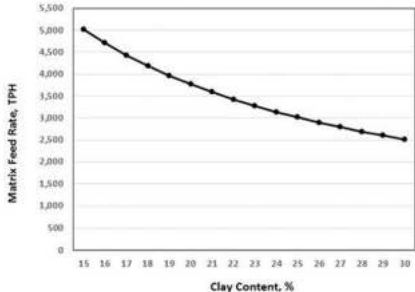
Figure 14-2: Matrix Clay Content vs. Maximum Feed
