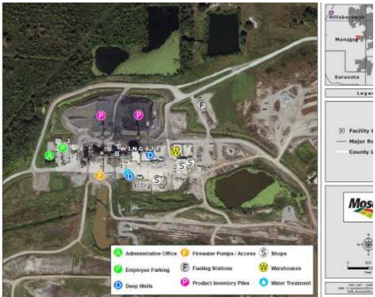
Figure 15-6: Wingate Facility Beneficiation Plant and Related Infrastructure
