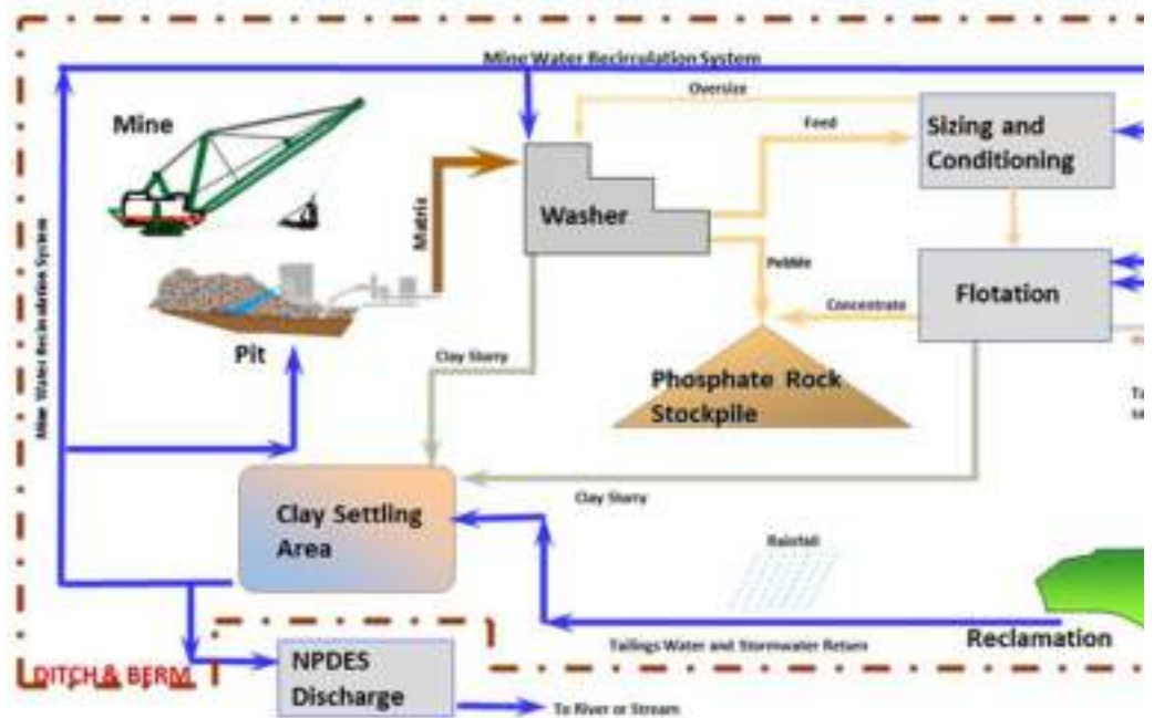
Figure 17-1: Mine Process Flow Diagram
