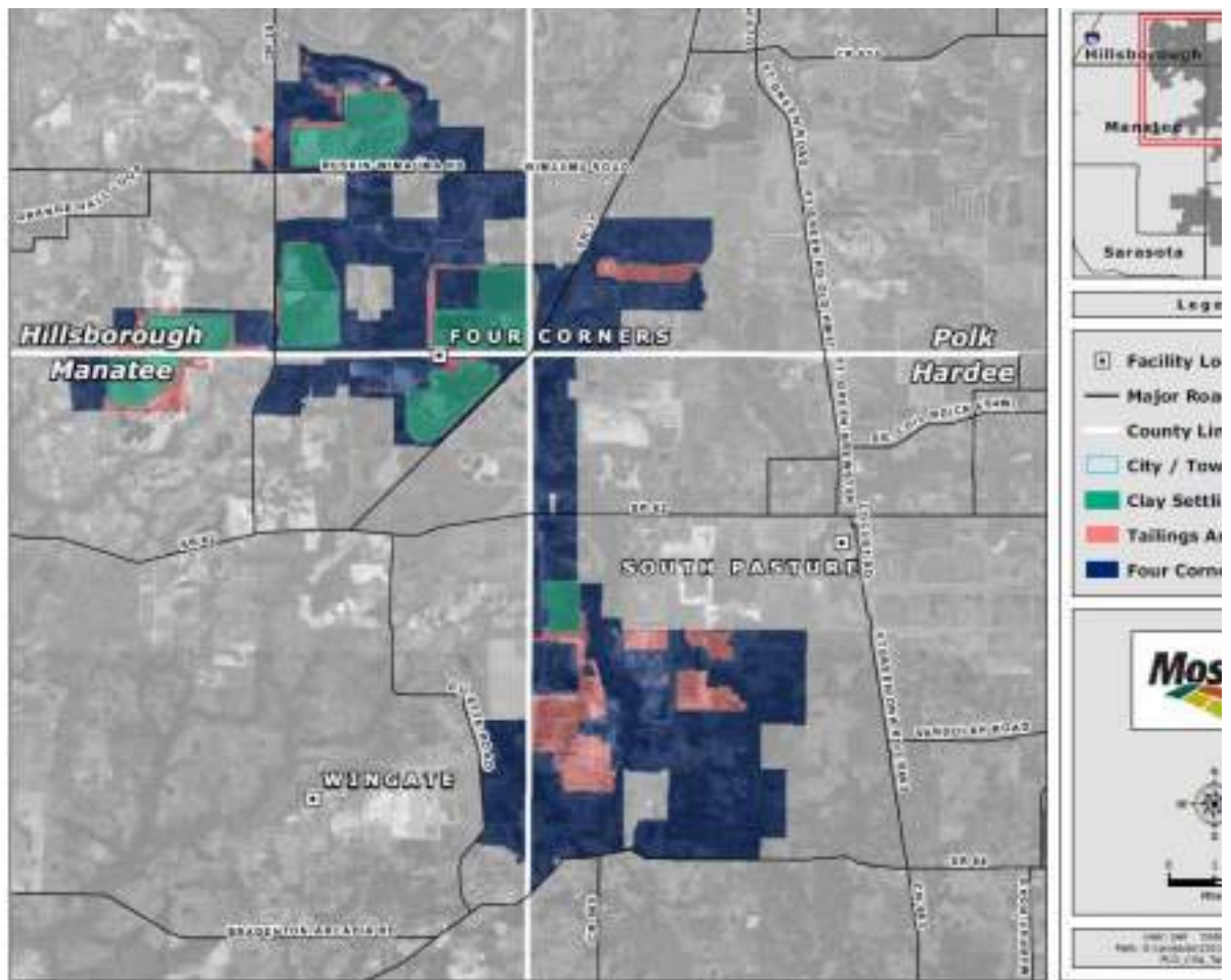
Figure 15-8: Four Corners Facility Clay Settling and Sand Tailings Locations
