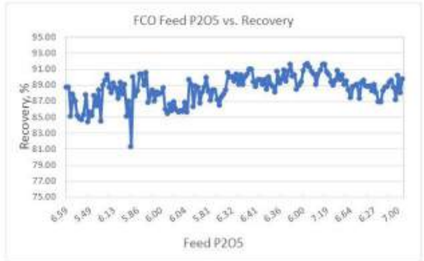
Figure 10-2: Four Corners Feed P 2 O 5 Grade vs. Recovery%
