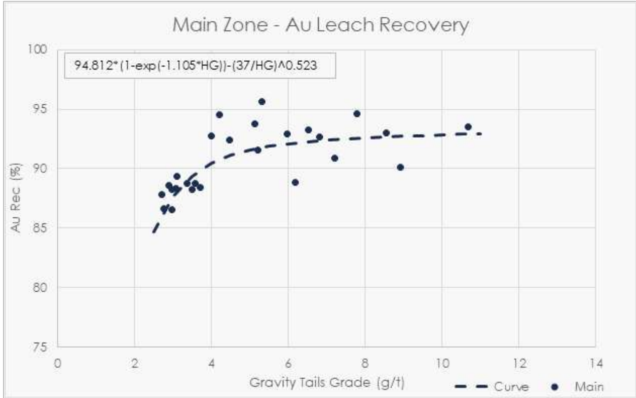
Figure 13-35: Main zone gold recovery curve
