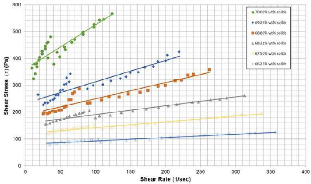
Figure 13-25: Flow loop data summary
