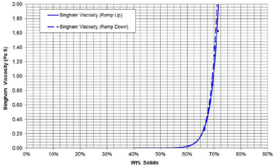
Figure 13-24: Bingham viscosity results for sample Tailings 37 µm sample
