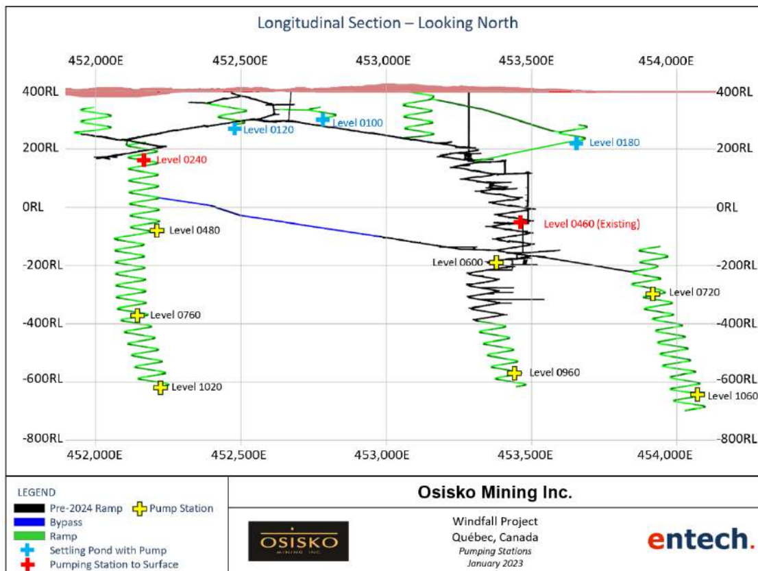
Figure 16-17: Pumping stations
