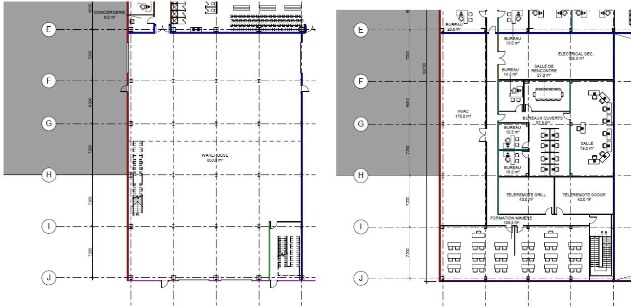
Figure 18-12: Plan view of warehouse and control centre
