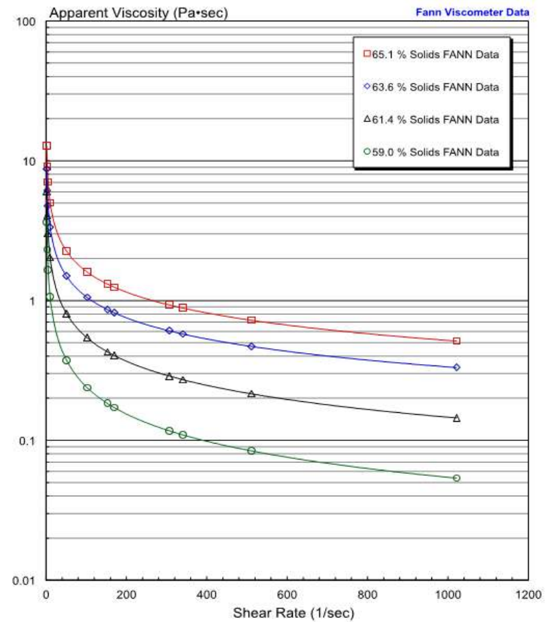
Figure 13-6: Apparent viscosity vs. shear rate
