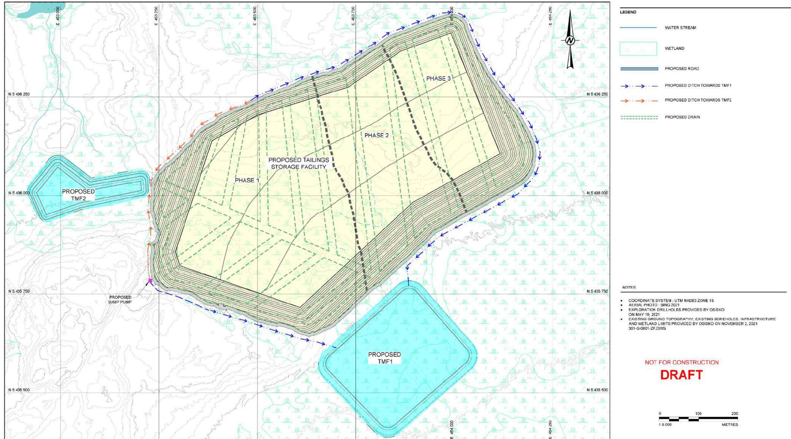
Figure 18-16: Plan view of the tailings management facility
