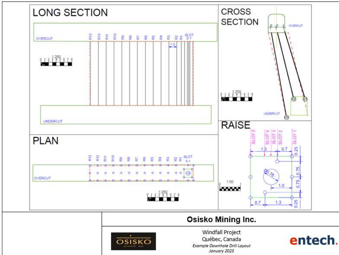
Figure 16-13: General arrangement for downhole stope design
