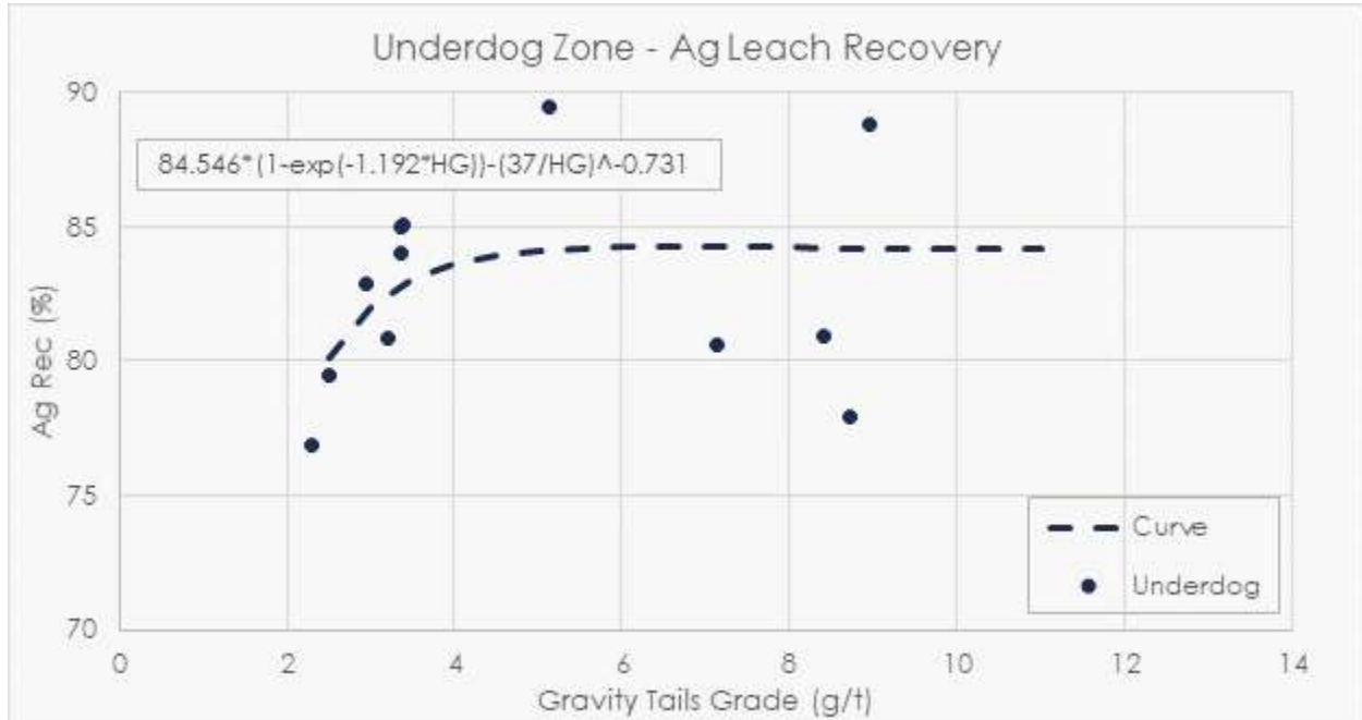
Figure 13-42: Underdog zone silver recovery curve
