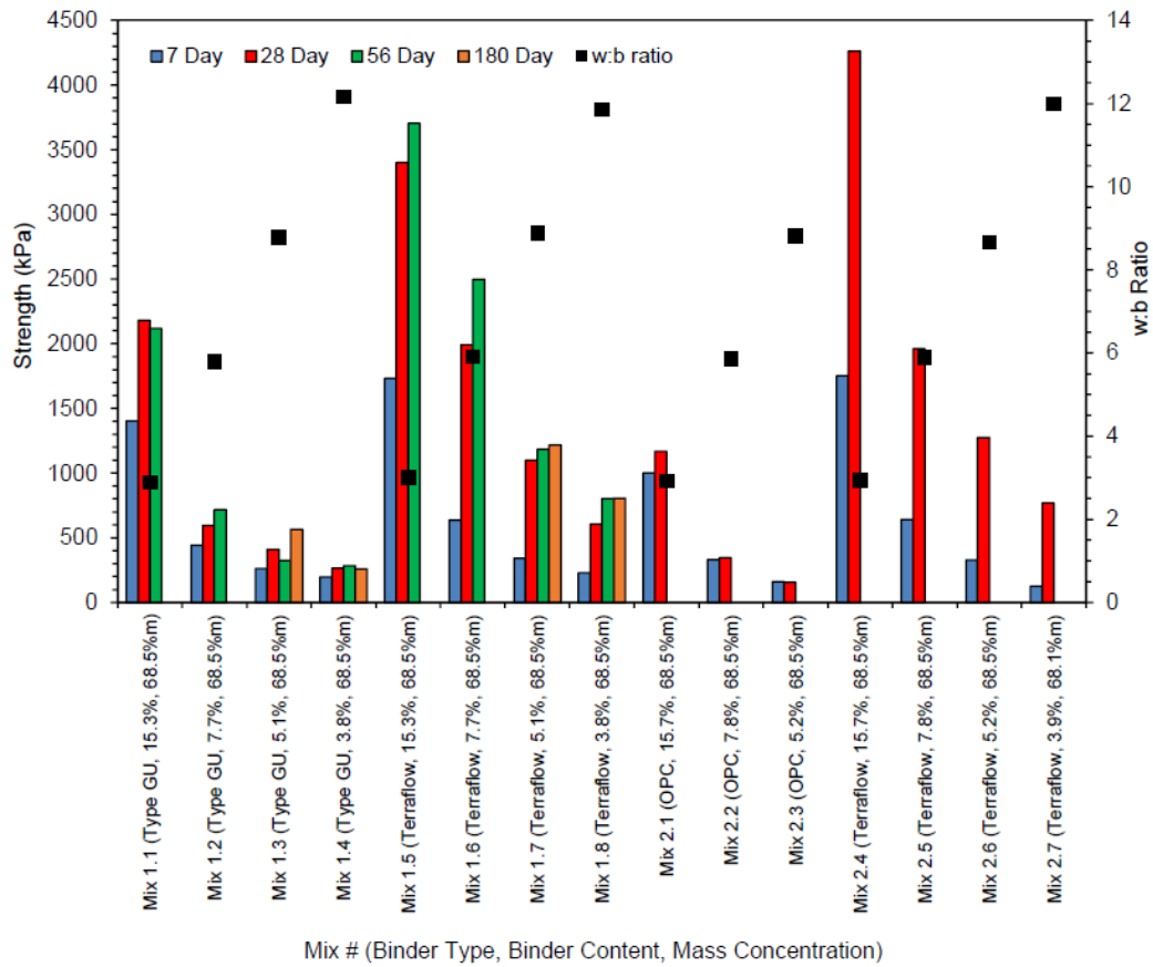
Figure 13-16: UCS test results
