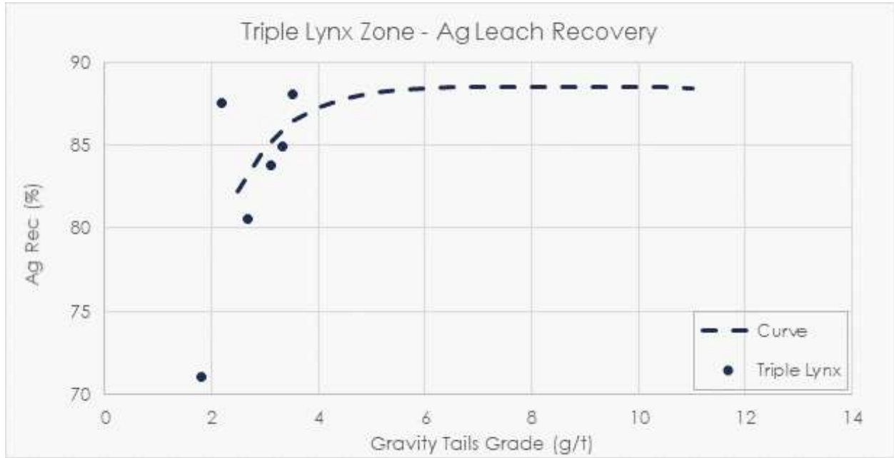
Figure 13-44: Triple Lynx zone silver recovery curve
