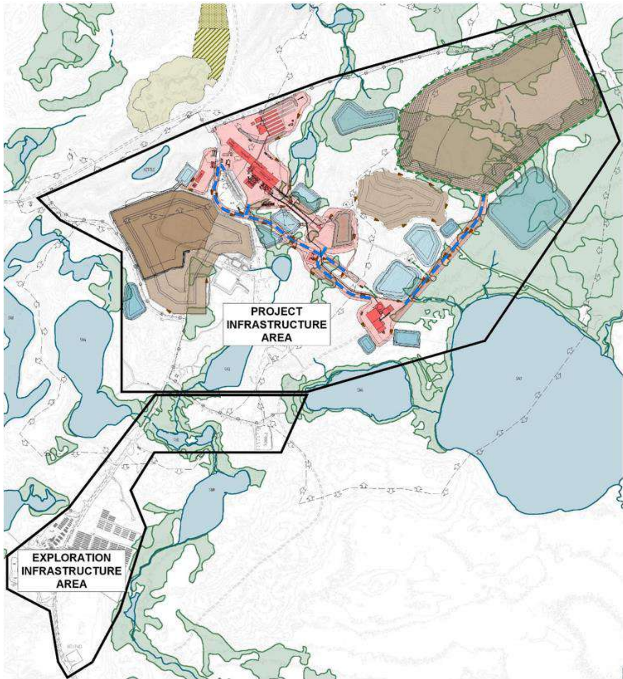
Figure 18-1: Windfall complete site layout
