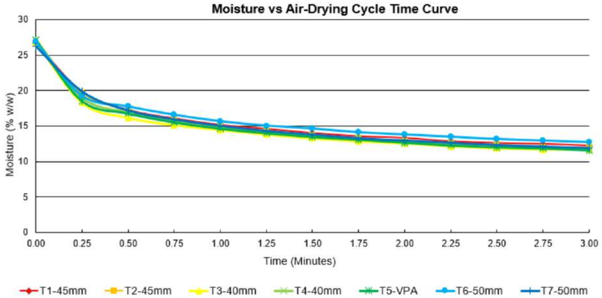
Figure 13-33: Drying time effect on cake moisture
