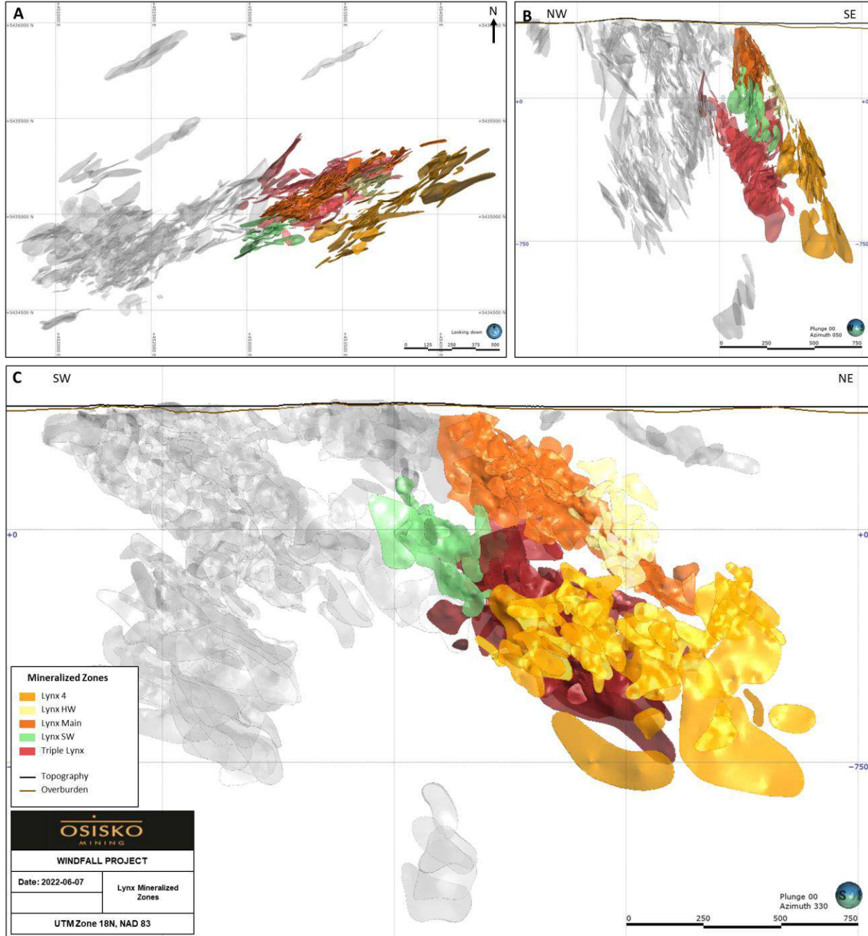
Figure 14-4: Lynx mineralized zones in the Windfall deposit A) Plan view; B) Cross-section view (looking northeast); and C) Longitudinal view (looking northwest)
