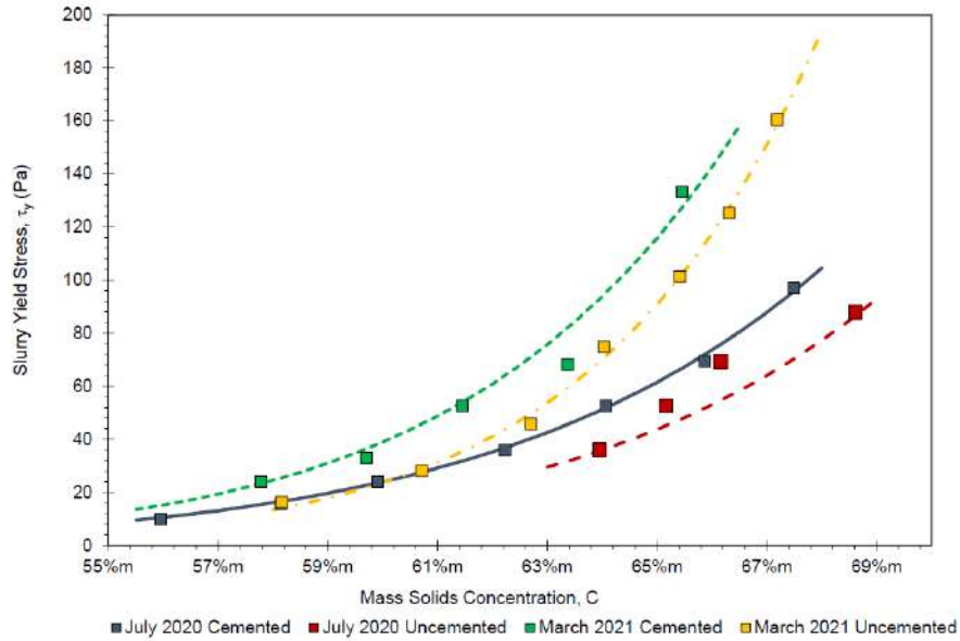
Figure 13-14: Bingham yield stress vs. mass solids concentration
