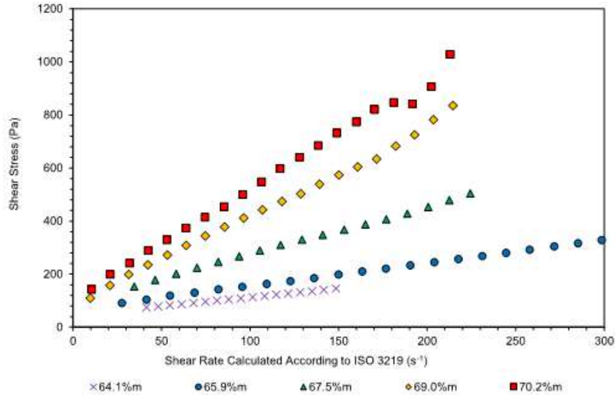
Figure 13-10: Cemented July 2020 tailings rheogram
