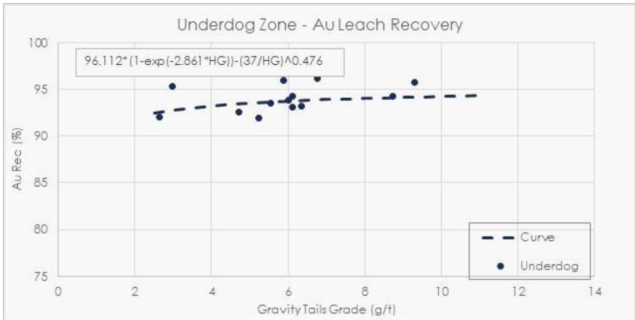
Figure 13-37: Underdog zone gold recovery curve
