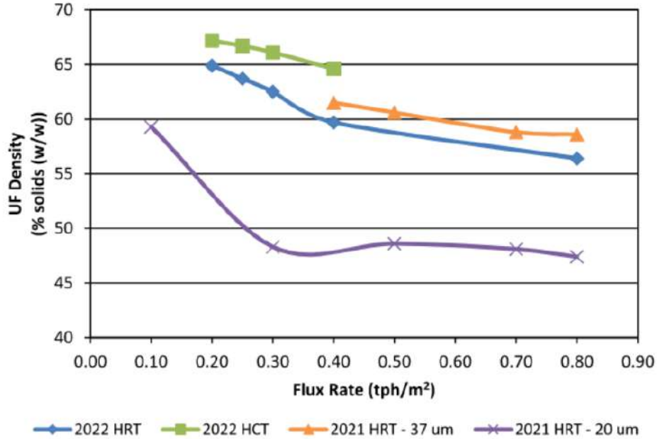
Figure 13-30: Historical underflow solids content comparison for different P 80
