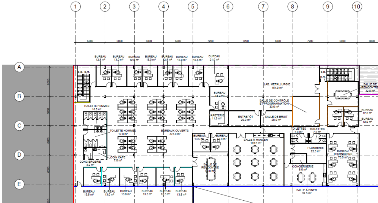
Figure 18-11: Plan view of 1 st floor office
