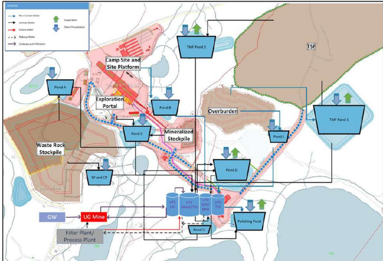
Figure 20-3: Water balance conceptual flow diagram – Phase 1
