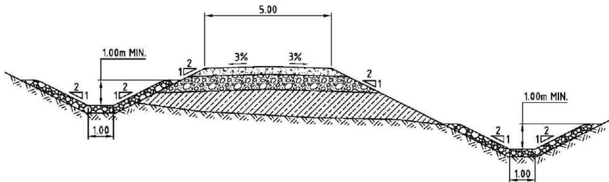
Figure 18-14: Service road – Typical cross-section
