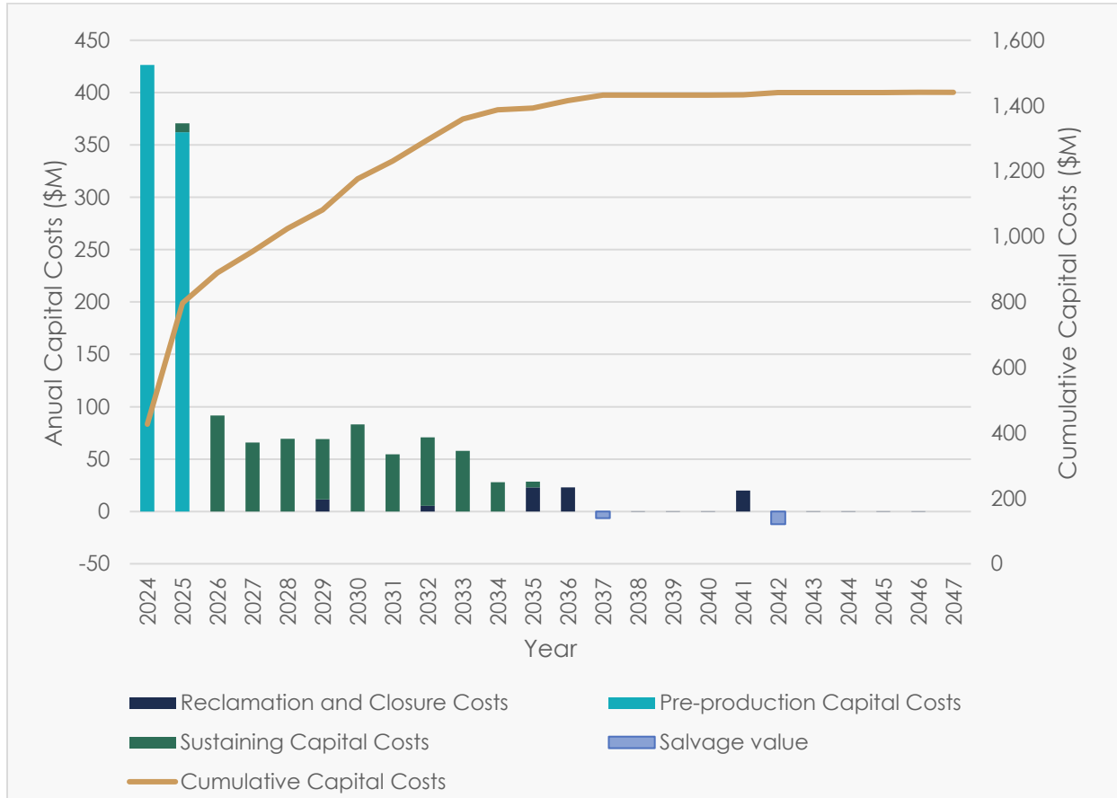
Figure 21-1: Annual and cumulative project capital costs
