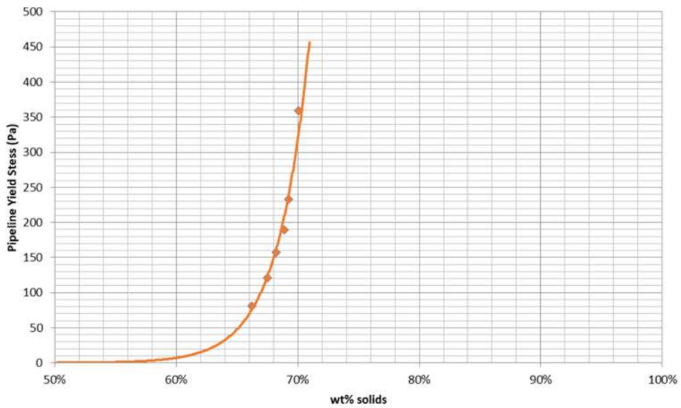
Figure 13-26: Pipeline yield stress vs. wt% solids
