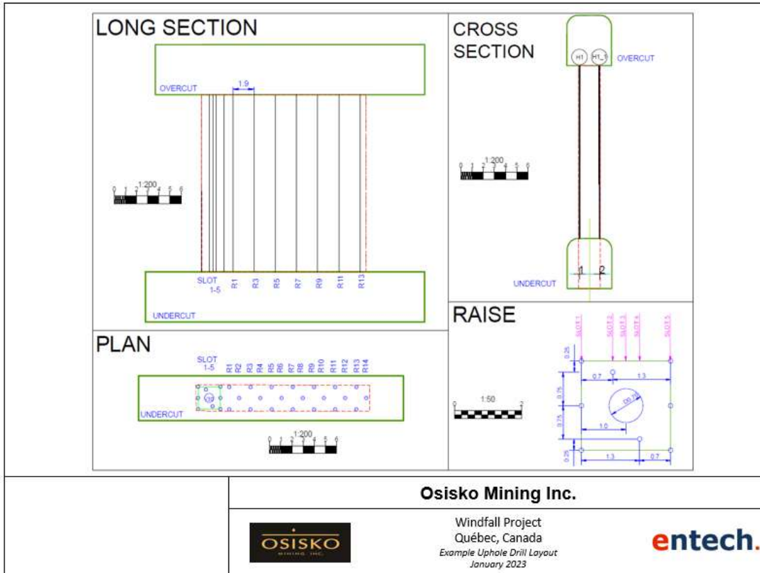
Figure 16-14: General arrangement for uphole stope design
