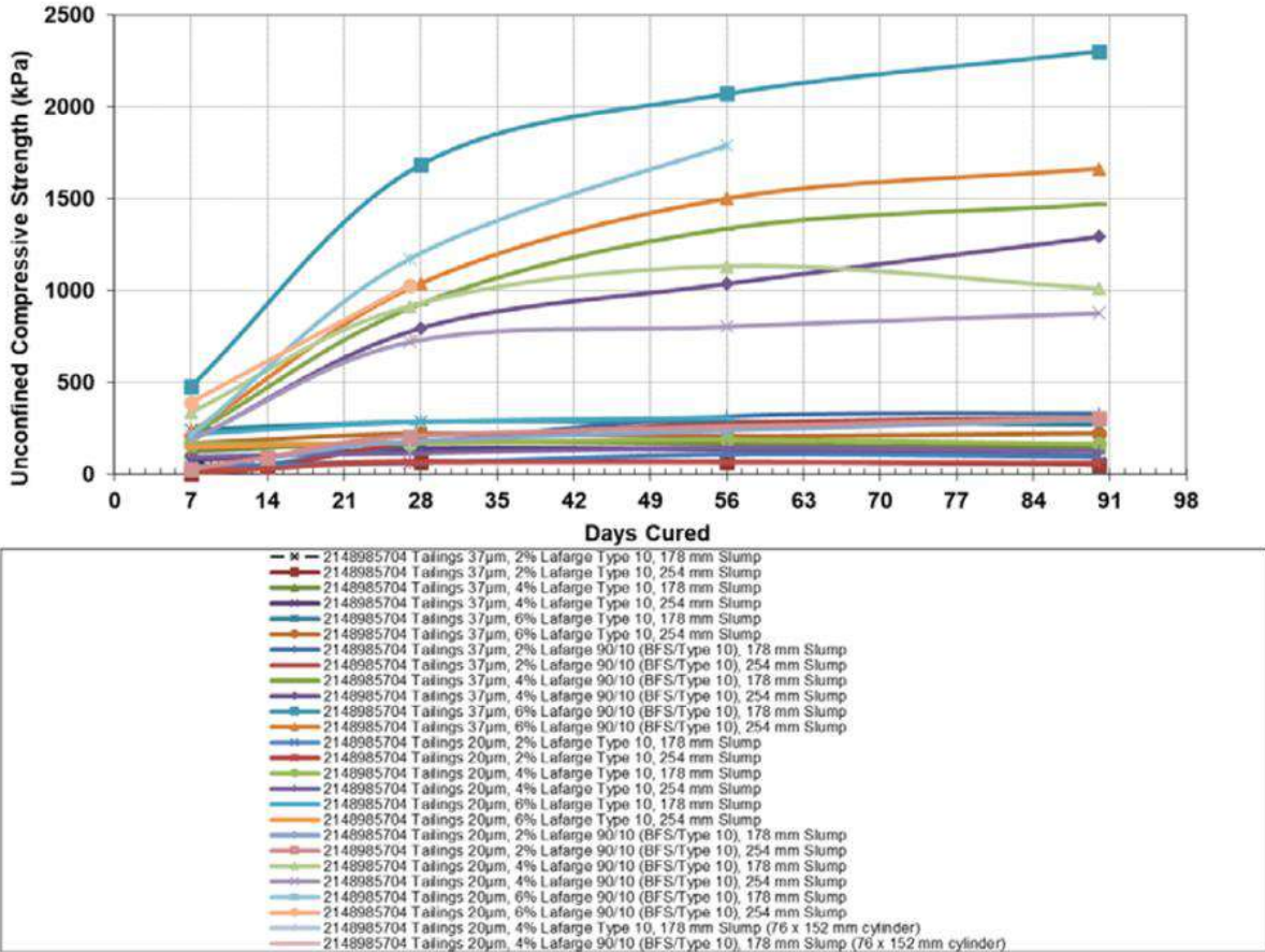
Figure 13-28: UCS results for samples Tailings 37 and 20 µm
