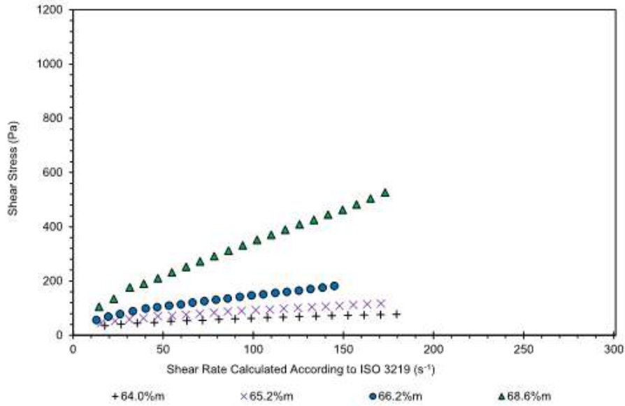
Figure 13-12: Uncemented July 2020 tailings rheogram
