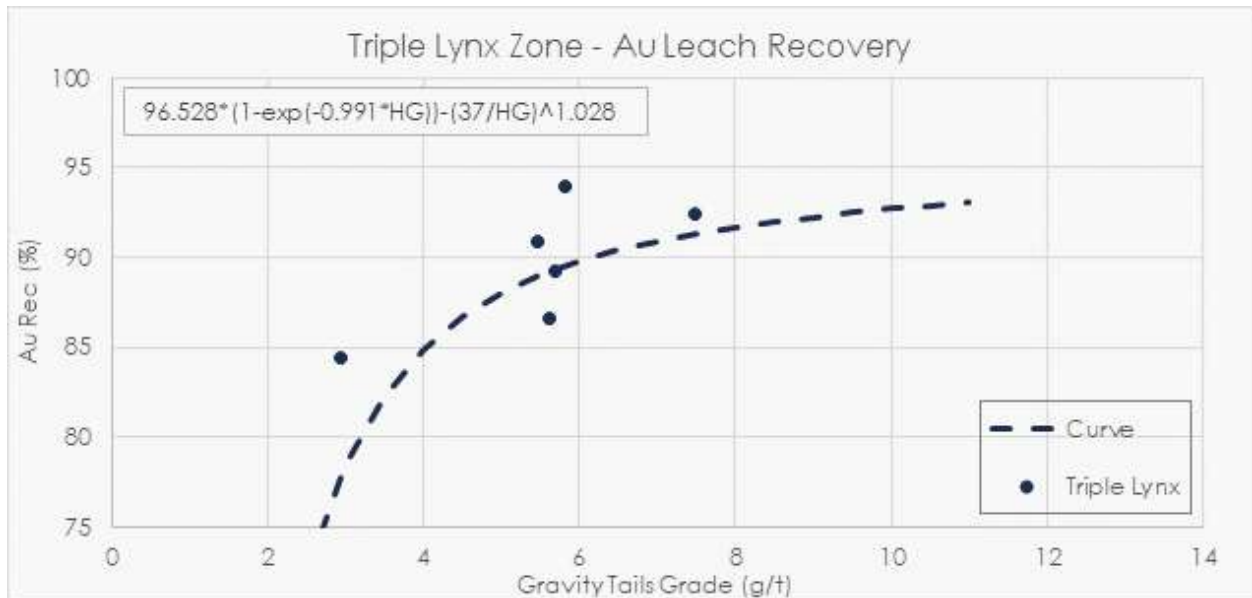
Figure 13-39: Triple Lynx zone gold recovery curve
