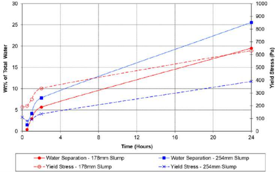
Figure 13-21: Water bleed and yield stress vs. time for Tailings 37 µm sample
