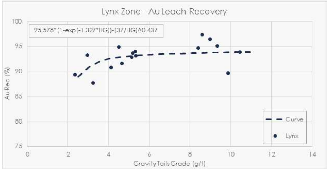
Figure 13-36: Lynx zone gold recovery curve
