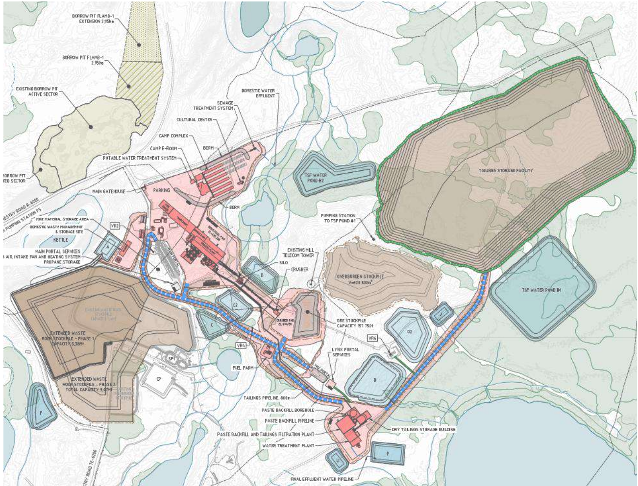
Figure 18-2: Windfall Project layout
