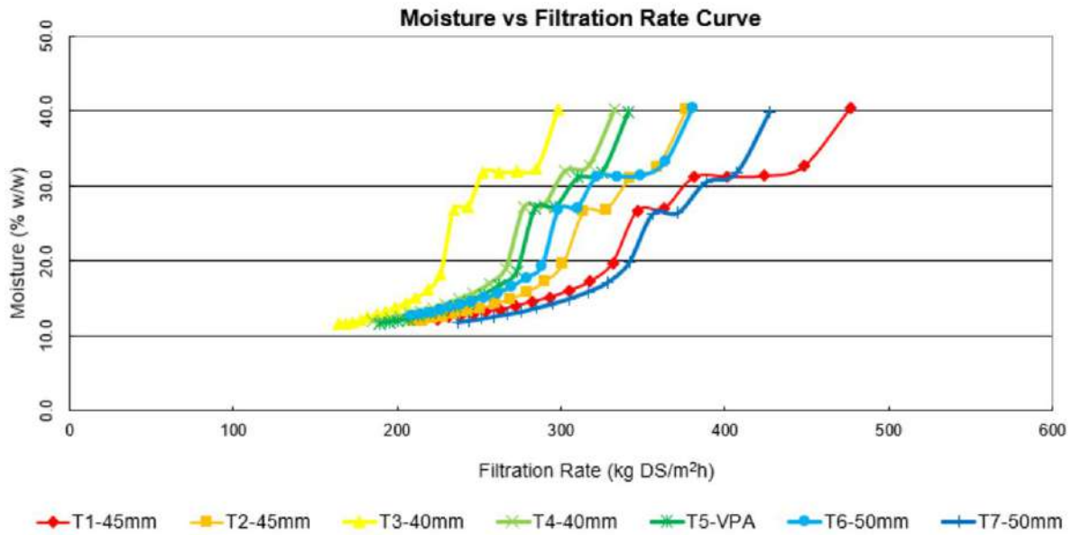
Figure 13-34: Filtration rate vs. cake moisture
