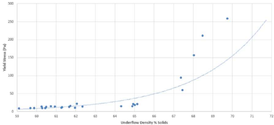
Figure 13-32: 190-mm pilot yield stress vs. underflow solids content
