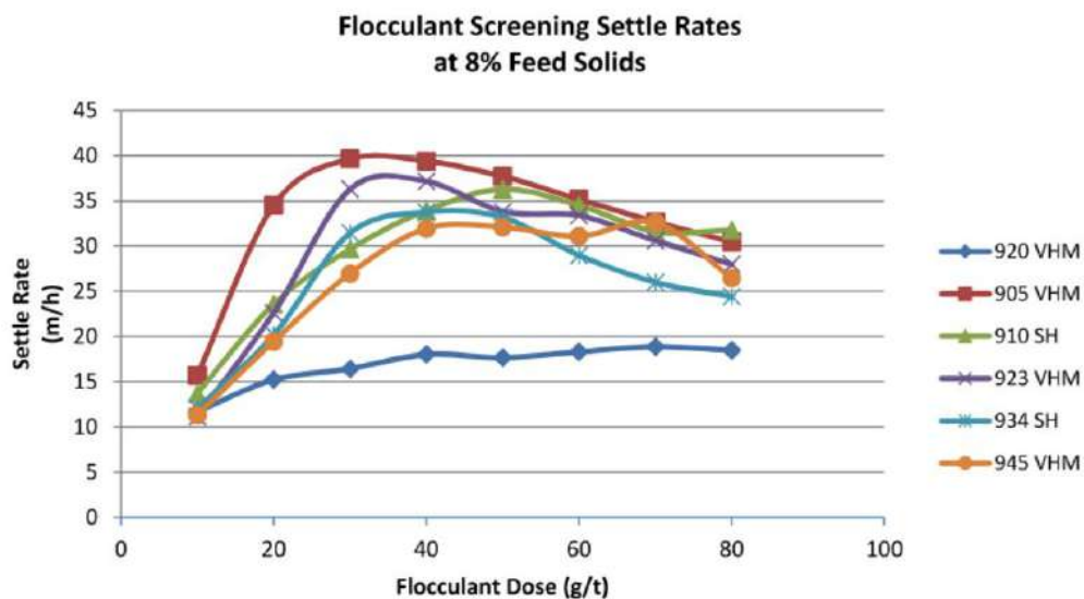
Figure 13-29: Lynx bulk tailings flocculant screening results
