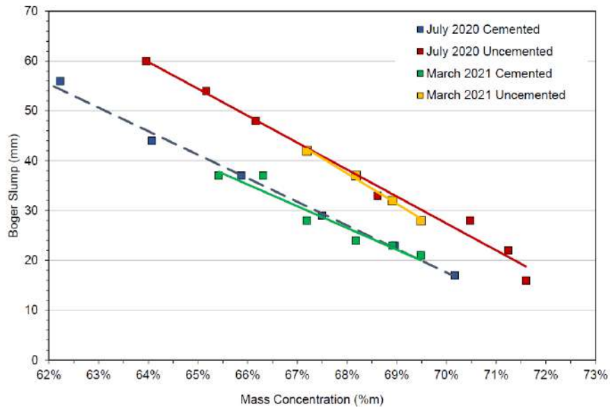
Figure 13-9: Boger slump vs. mass concentration
