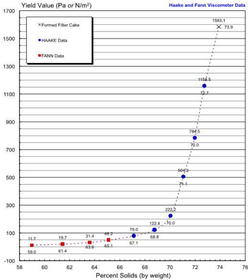
Figure 13-5: Yield stress vs. wt% solids
