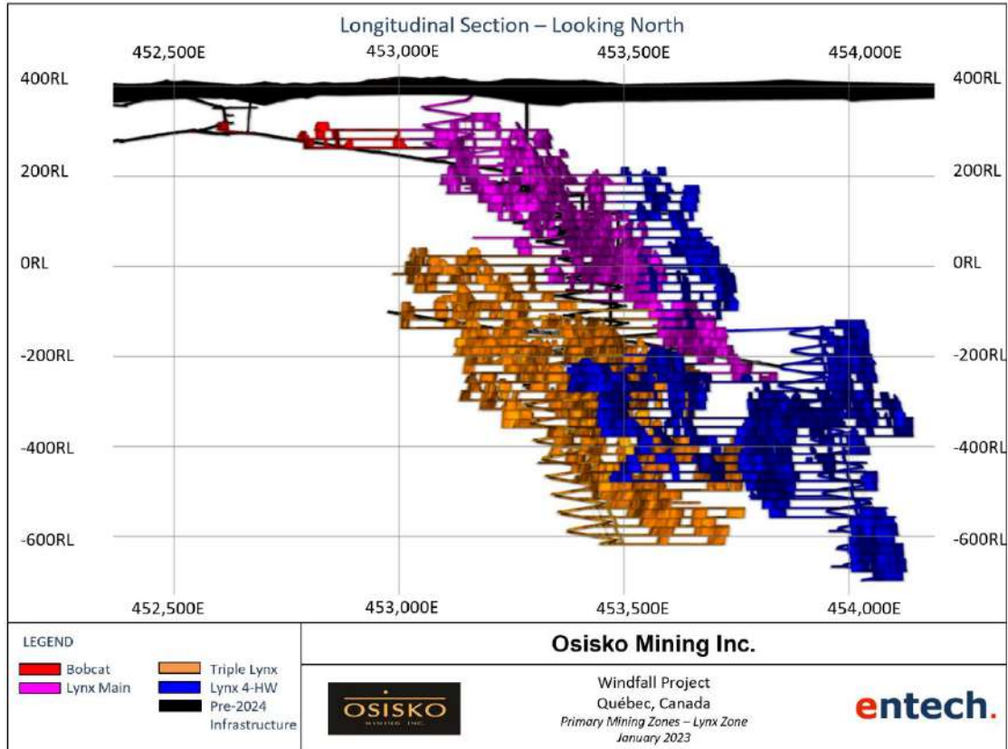
Figure 16-7: Lynx zone development design
