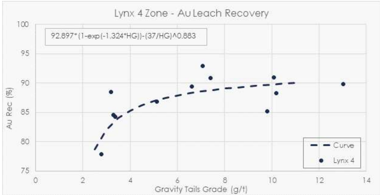
Figure 13-38: Lynx 4 zone gold recovery curve
