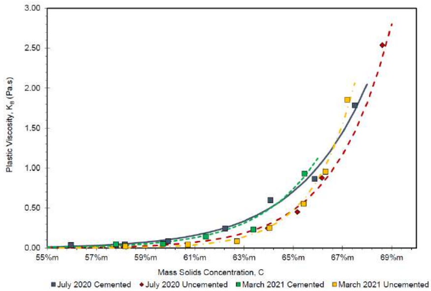
Figure 13-15: Plastic viscosity vs. mass solids concentration
