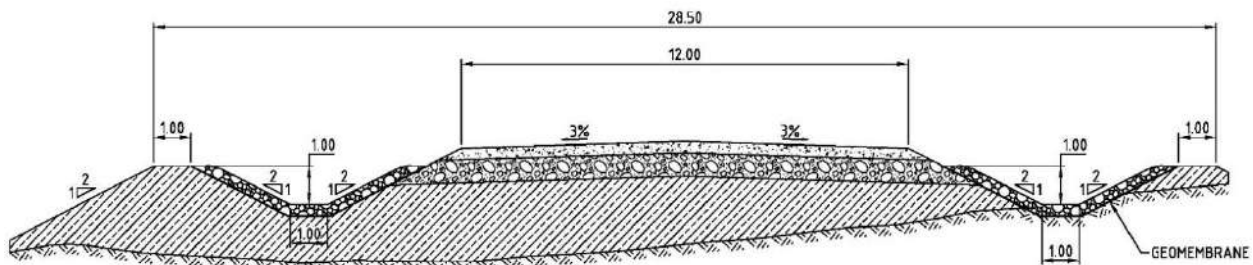
Figure 18-15: Haulage road – Typical cross-section
