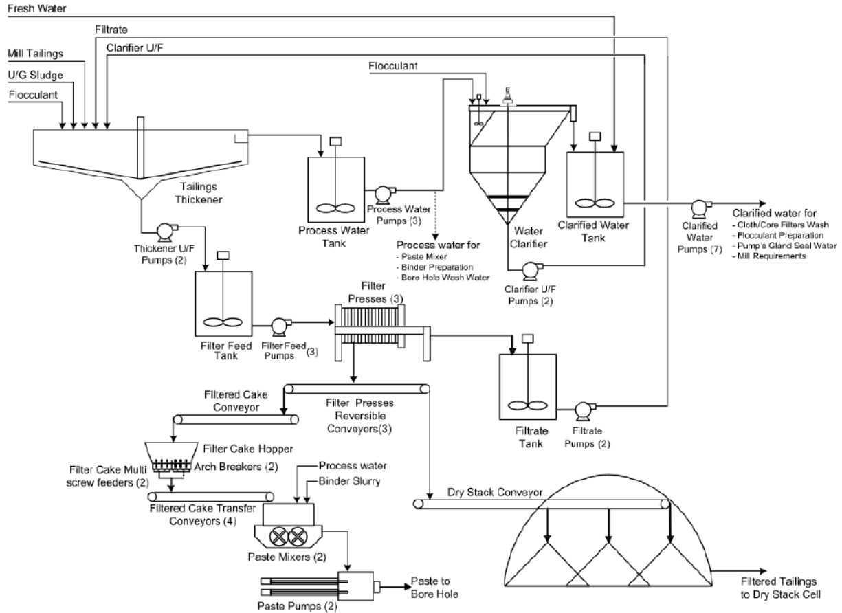
Figure 17-6: Tailings filtration plant simplified flowsheet
