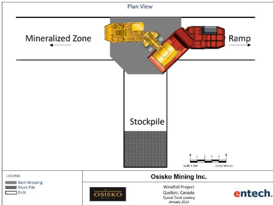
Figure 16-11: Typical level truck loading arrangement
