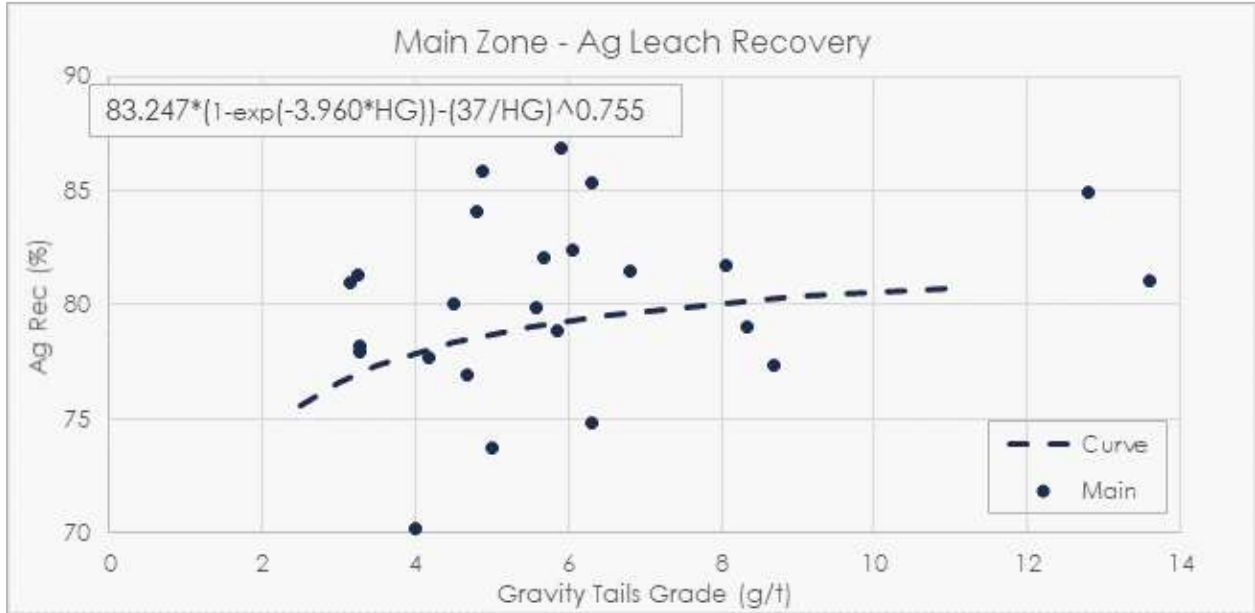
Figure 13-40: Main zone silver recovery curve
