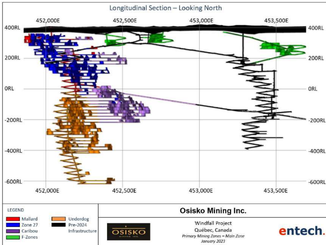
Figure 16-8: Main zone development design
