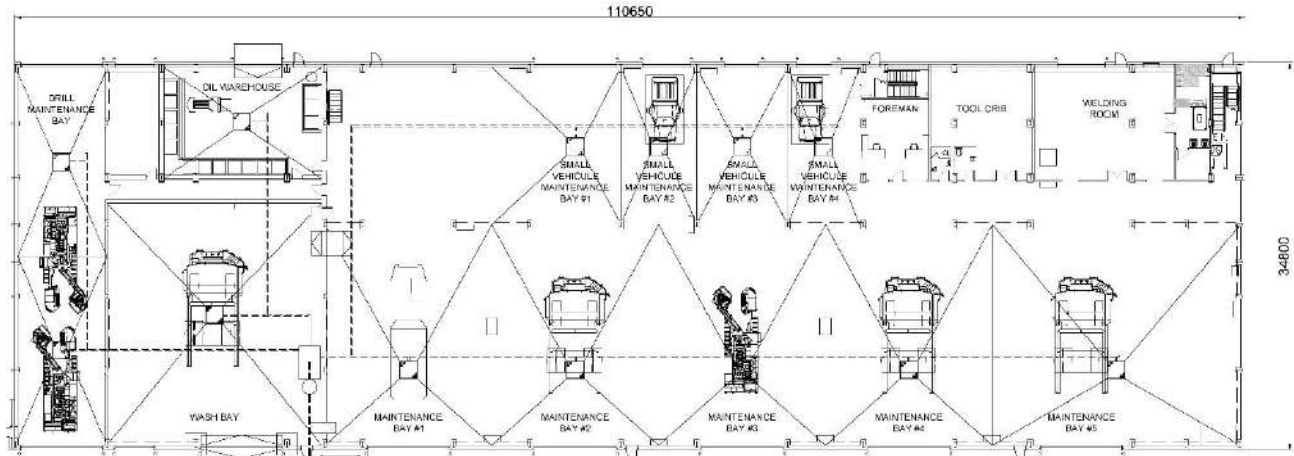
Figure 18-7: Truck shop layout (first floor)
