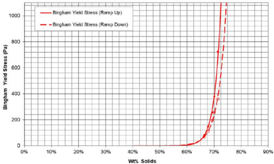
Figure 13-23: Bingham yield stress results for sample Tailings 37 \mu\text{m} sample
