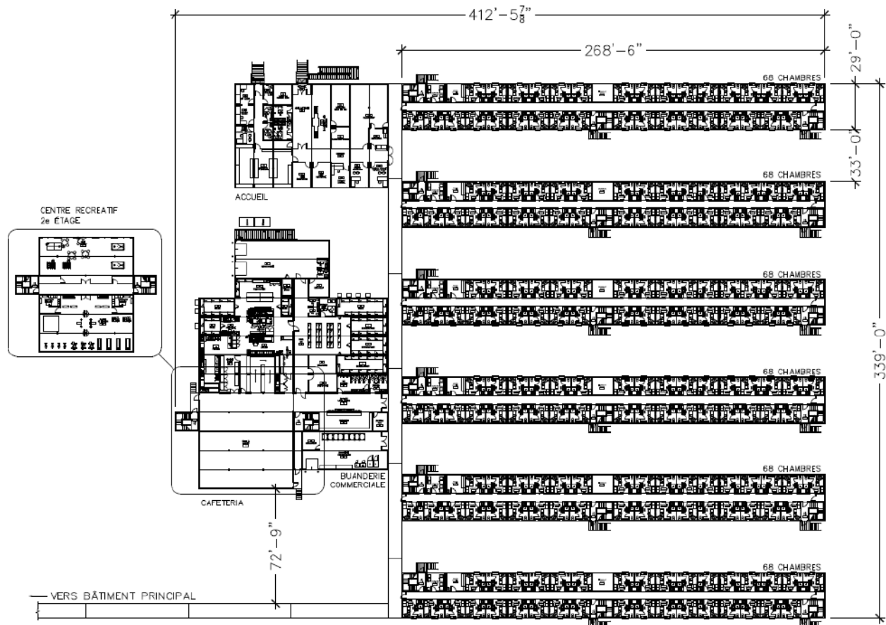
Figure 18-3: Camp complex layout
