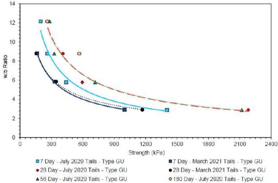
Figure 13-17: Water-to-binder ratio curves with "Type GU" binder
