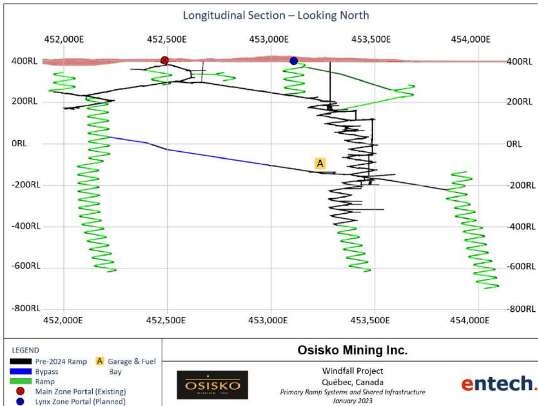
Figure 16-9: Primary ramp systems and shared infrastructure
