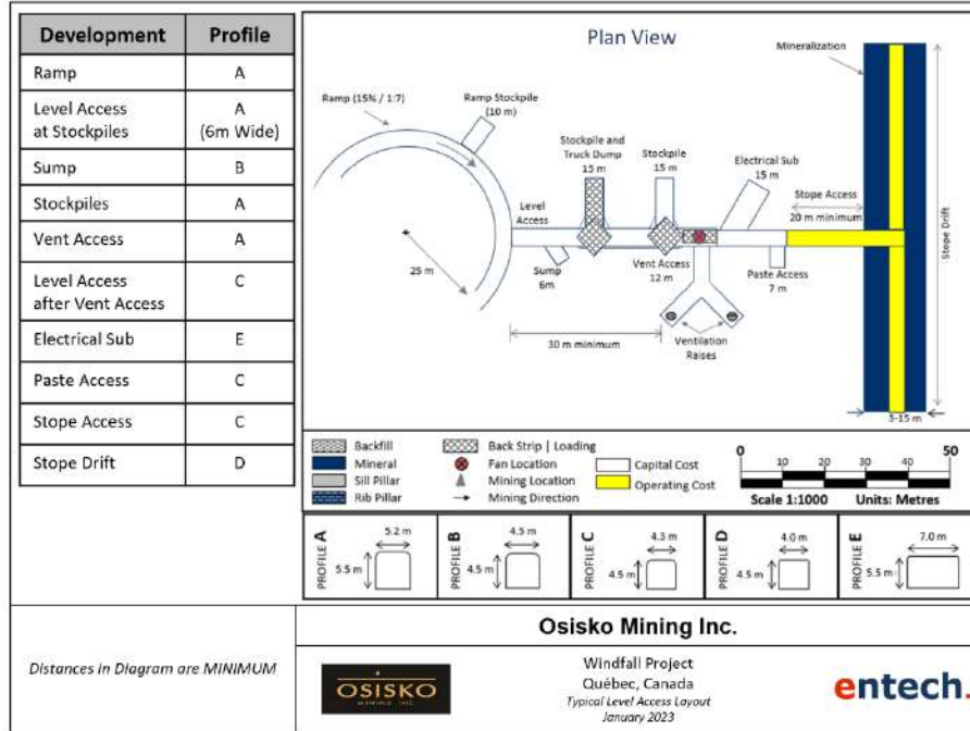
Figure 16-10: Typical level layout
