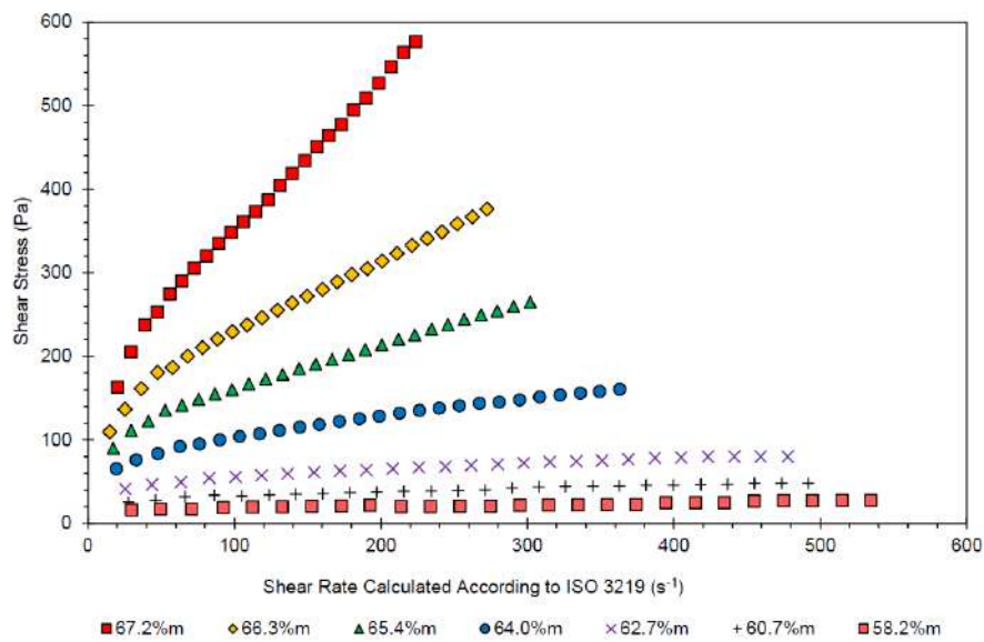
Figure 13-13: Uncemented March 2021 tailings rheogram
