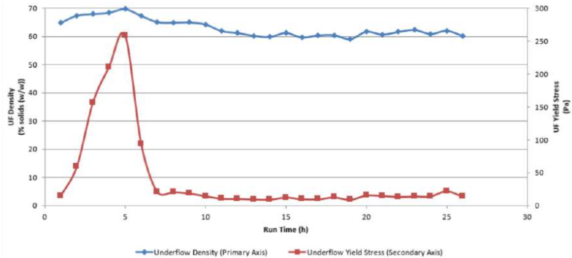
Figure 13-31: 190-mm pilot yield stress and underflow values produced during run time
