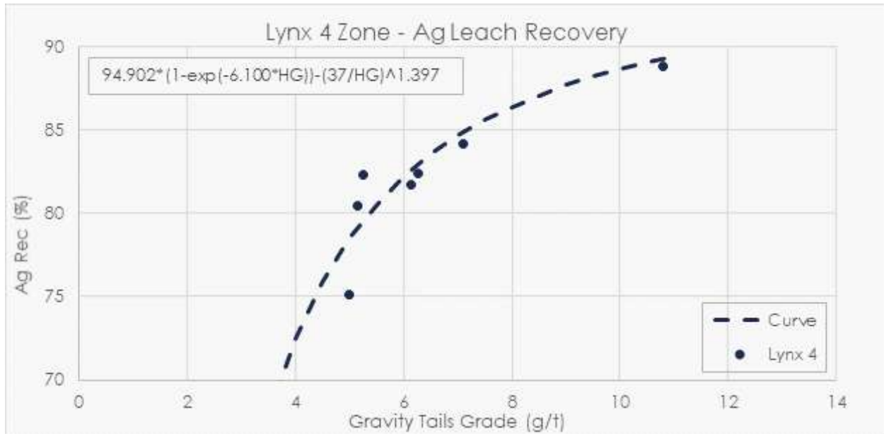
Figure 13-43: Lynx 4 zone silver recovery curve
