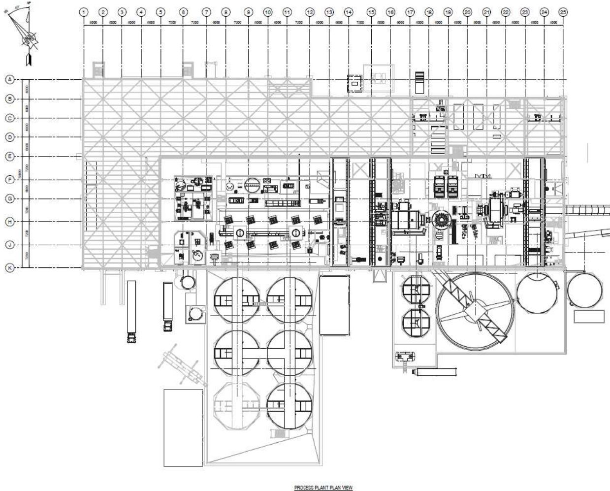
Figure 18-9: Plan view of the process plant
