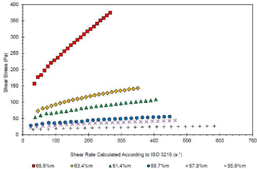
Figure 13-11: Cemented March 2021 tailings rheogram
