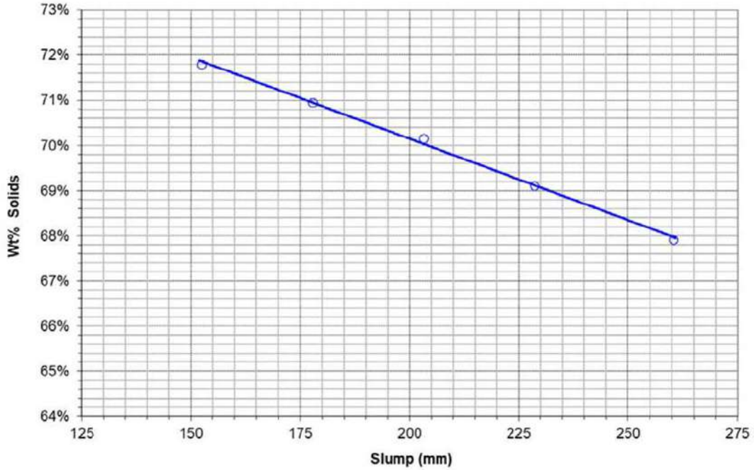
Figure 13-19: %Solids vs. slump for Tailings 37 µm sample
