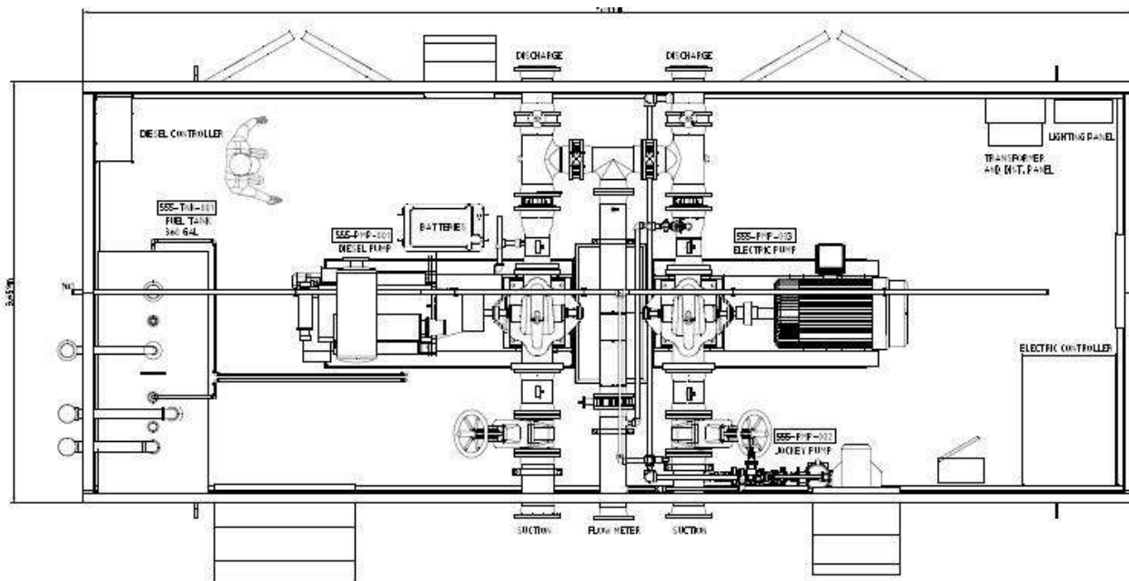
Figure 18-6: Fire water pump station layout
