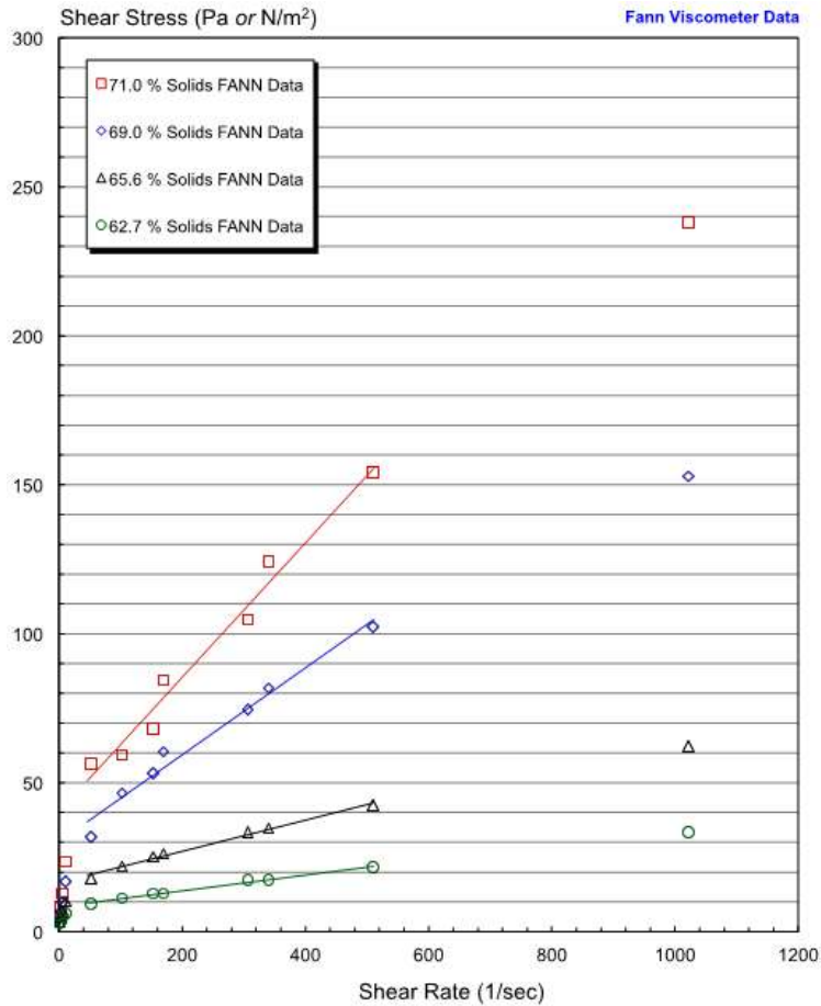
Figure 13-7: Shear stress vs. shear rate
