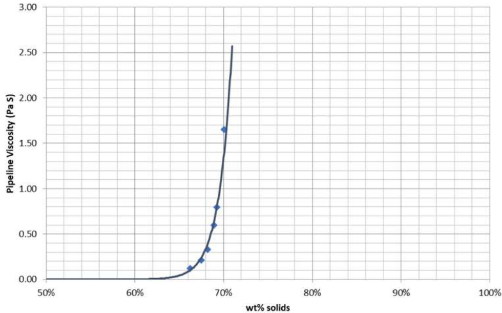
Figure 13-27: Pipeline viscosity vs. wt% solids
