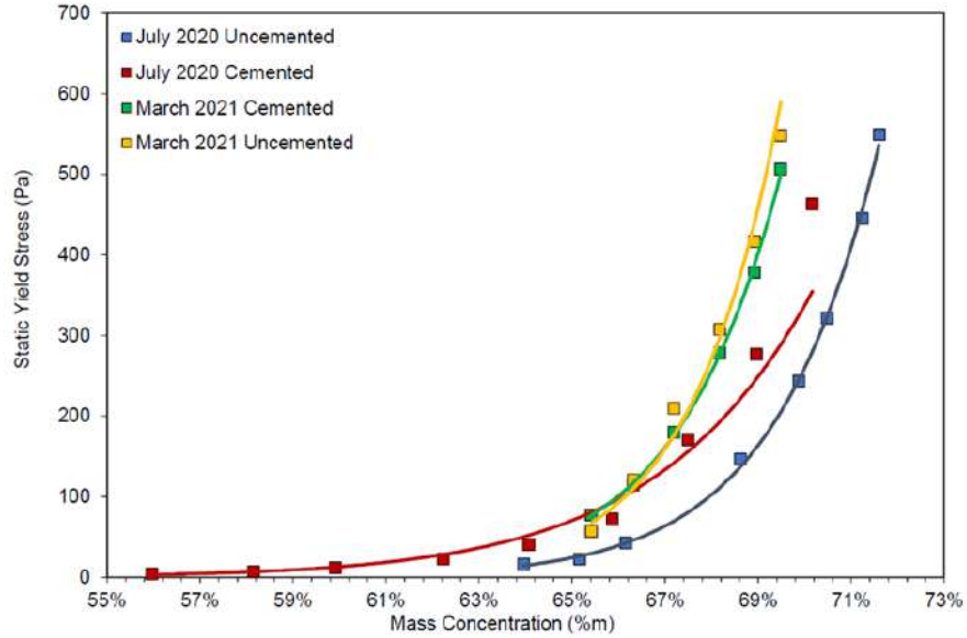
Figure 13-8: Static yield stress vs. mass concentration
