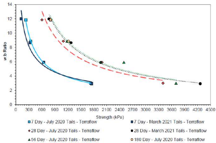
Figure 13-18: Water-to-binder ratio curves with "TerraFlow" binder
