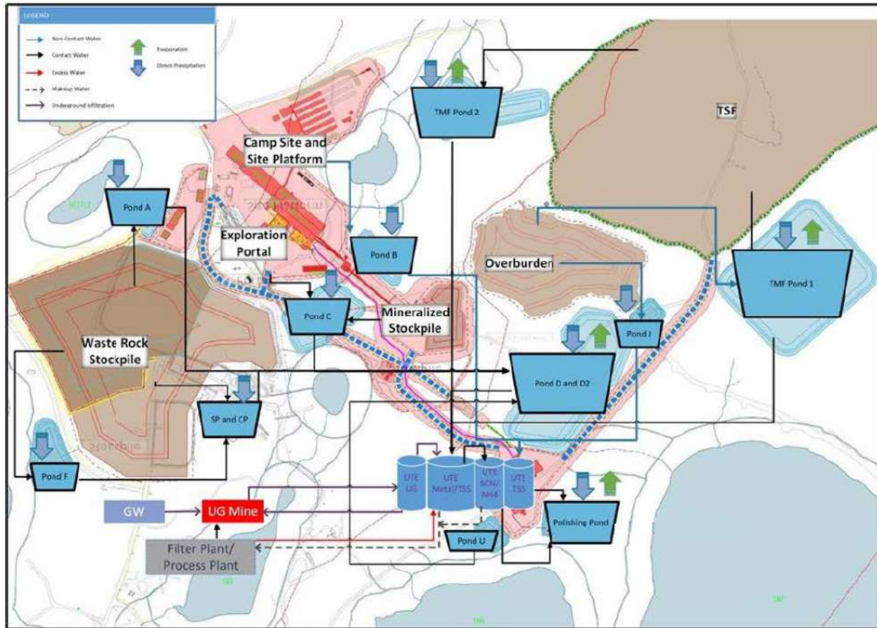
Figure 20-4: Water balance conceptual flow diagram – Phase 2
