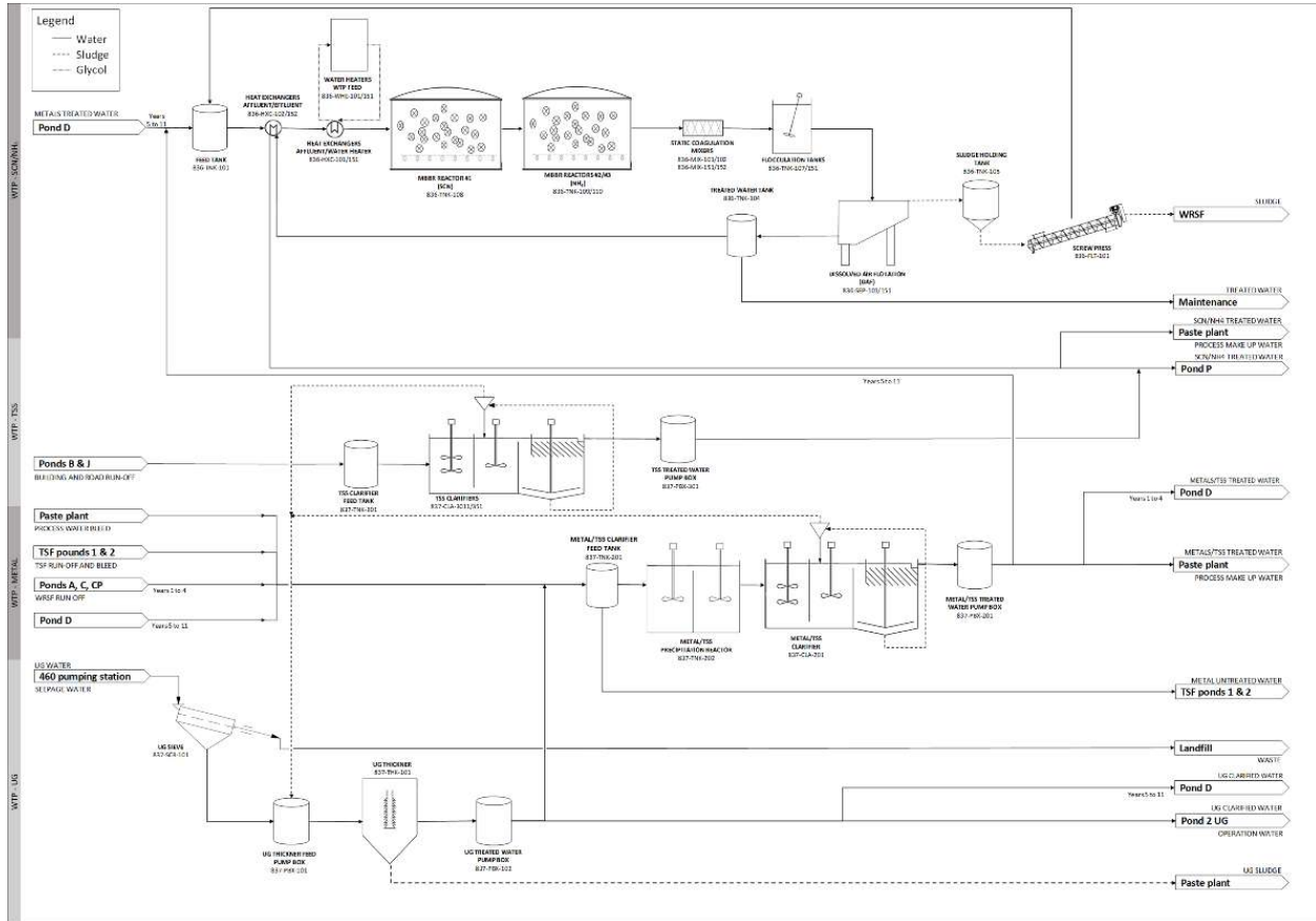
Figure 18-19: Simplified water treatment process diagram
