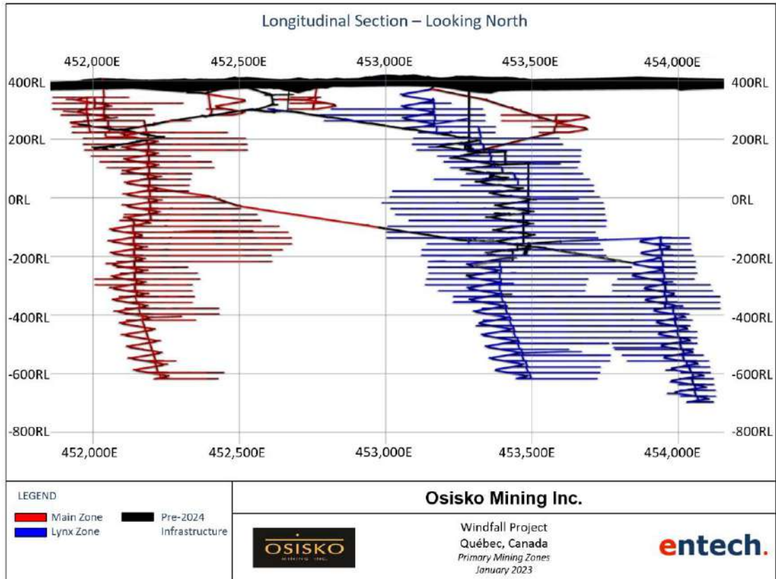
Figure 16-6: Windfall development design
