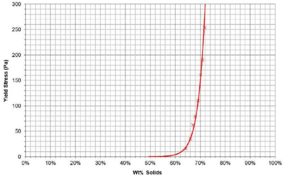
Figure 13-20: Static yield stress vs. %solids for Tailings 37 µm sample
