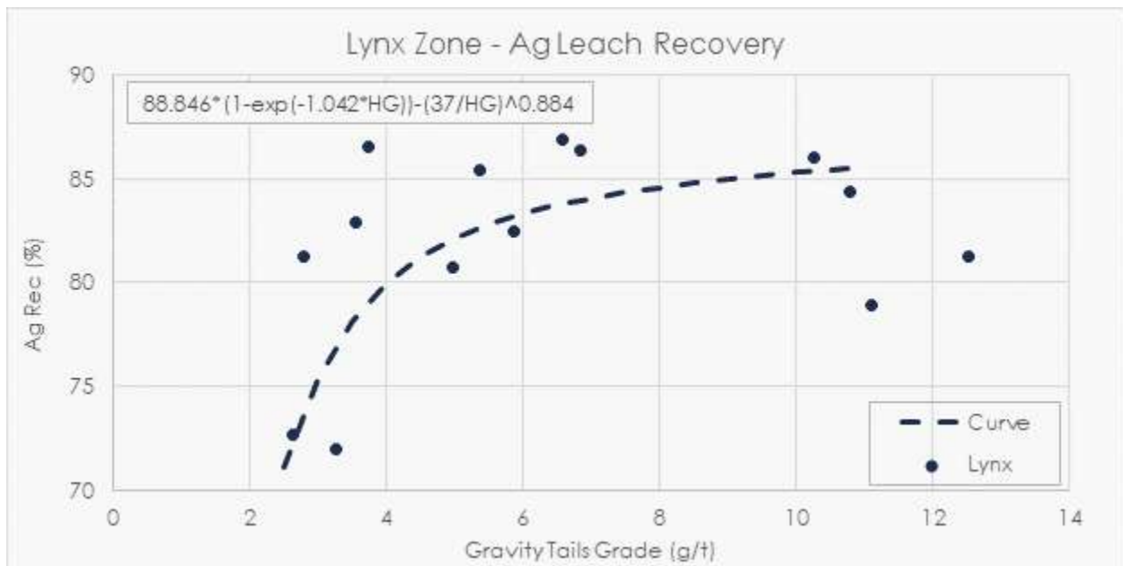
Figure 13-41: Lynx zone silver recovery curve
