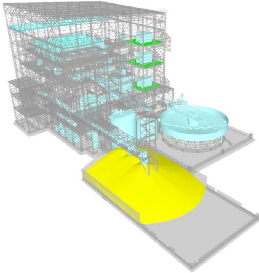
Figure 18-13: Tailings filtration and paste backfill plant layout
