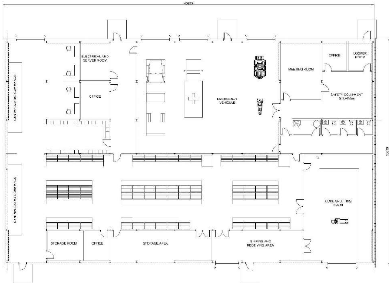
Figure 18-8: Production core shack and emergency vehicle storage layout
