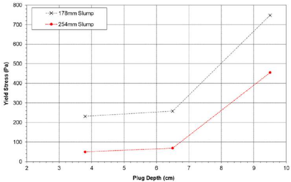
Figure 13-22: Plug yield stress for Tailings 37 µm sample
