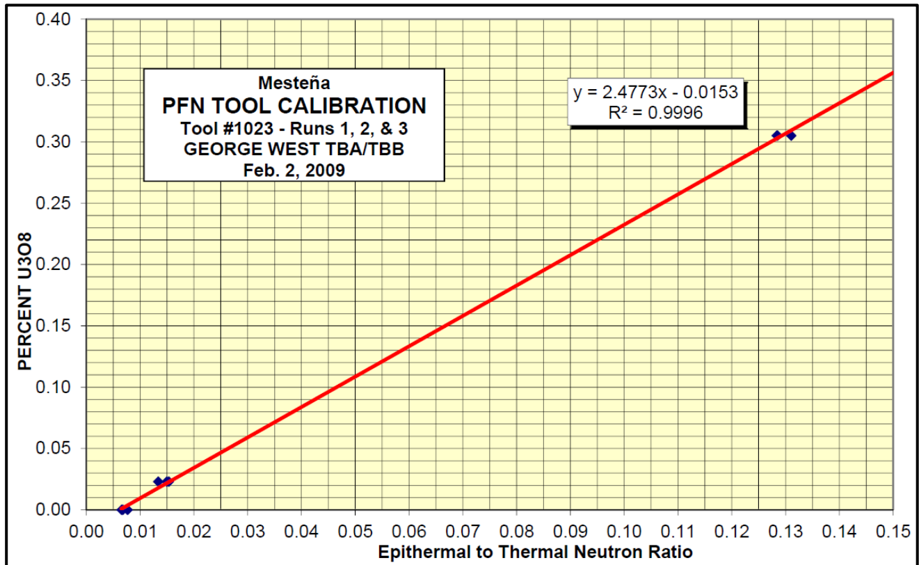
Figure 11-1. PFN Tool Calibration
