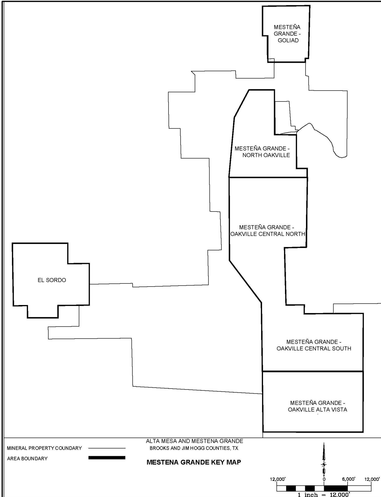
Figure 14-9 Mestena Grande Key Map
