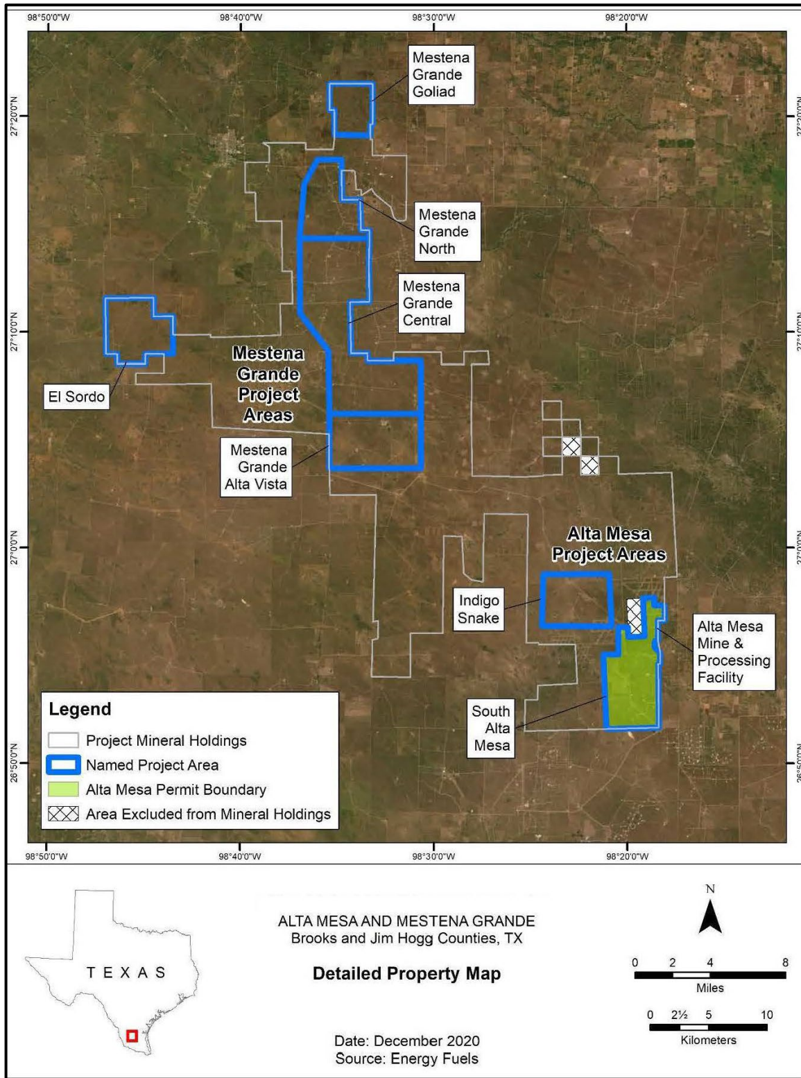
Figure 3-2. Alta Mesa and Mestena Grande Property Map
