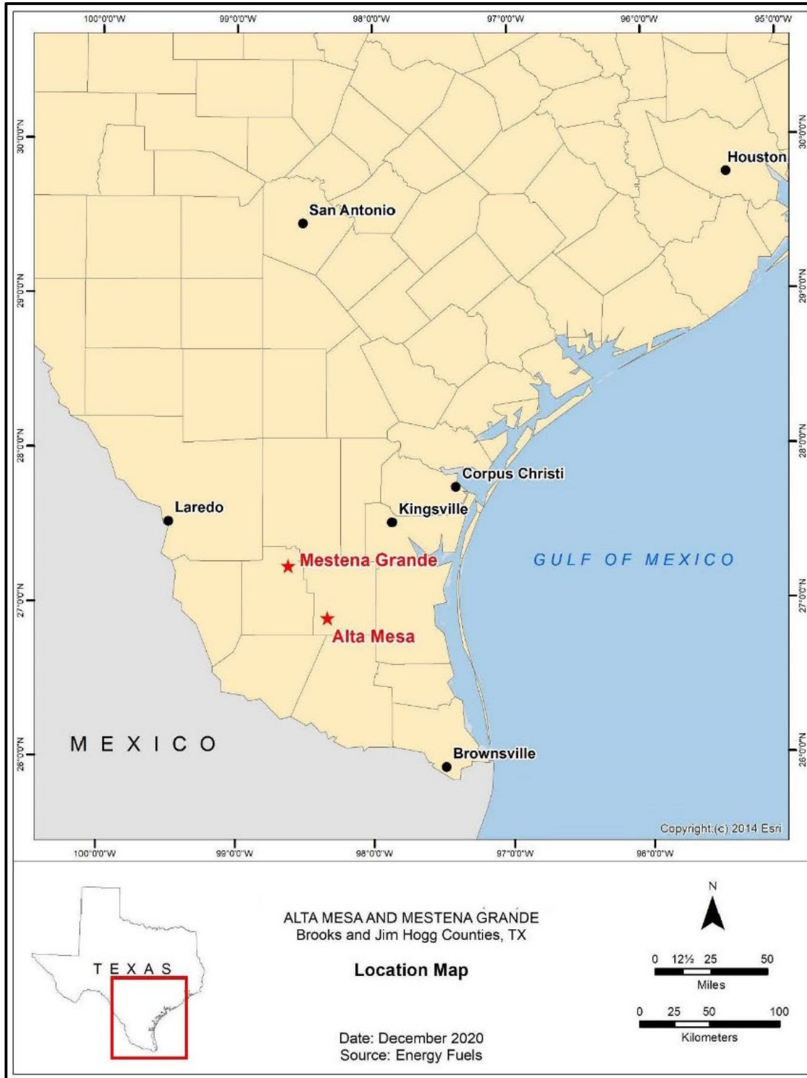
Figure 3-1. Alta Mesa and Mestena Grande Location Map
