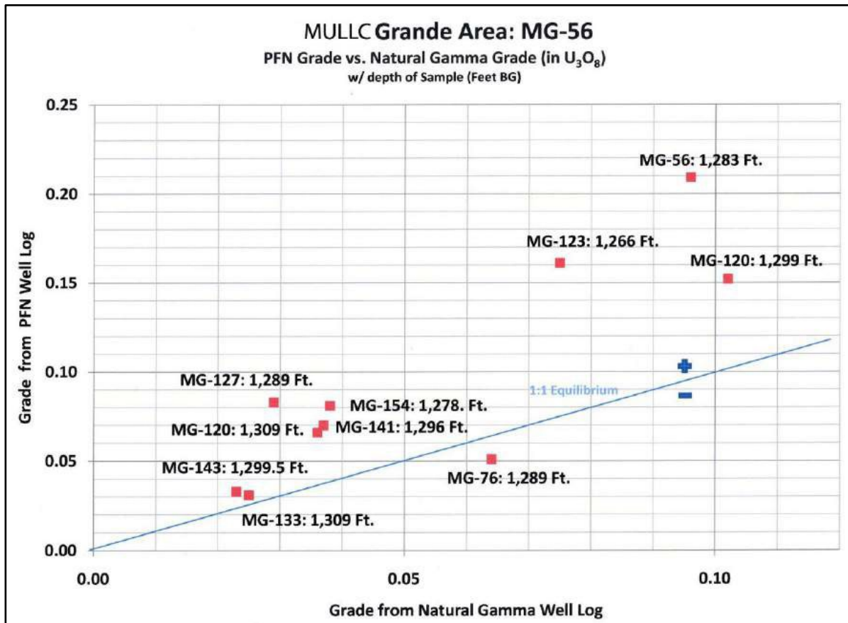
Figure 11-2. Disequilibrium Graph: Natural Gamma vs PFN Grade
