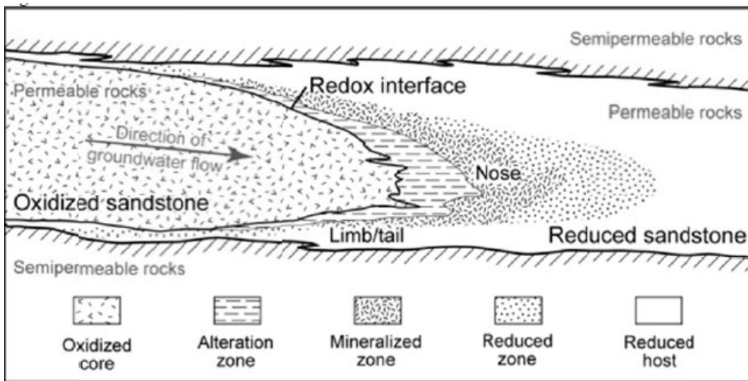
Figure 8-1 Idealized Cross Section of a Sandstone Hosted Uranium Roll-Front Deposit (Modified from Granger and Warren -1974 and De Voto- 1978)
