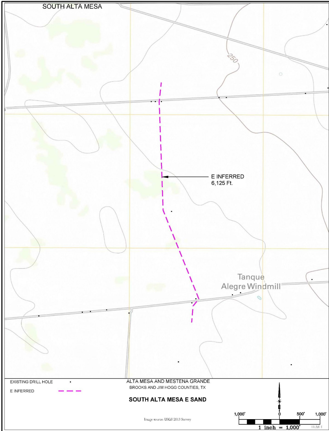
Figure 14-8 Sam and E Sand
