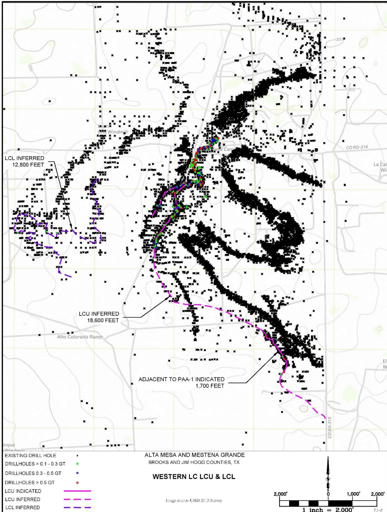
Figure 14-5 Western LC LCU and LCL
