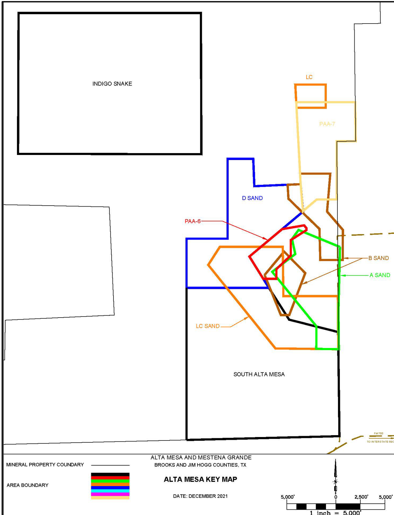
Figure 14-1 Alta Mesa Key Map
