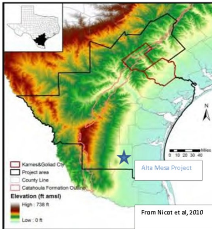
Figure 4-1. Topography of the South Texas Uranium Province
