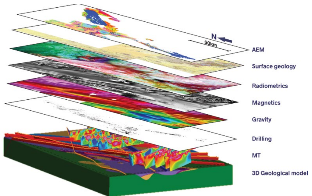
Figure 38: Paterson Province data syntheses layers
