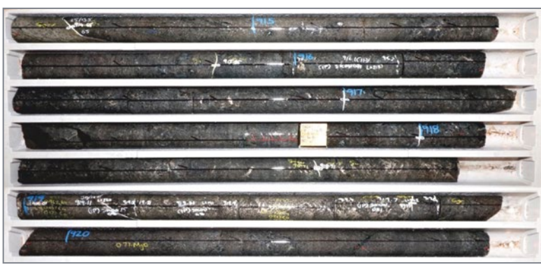
Figure 15: SKDD081 minor massive sulphides intersected in the Firehawk Horizon
