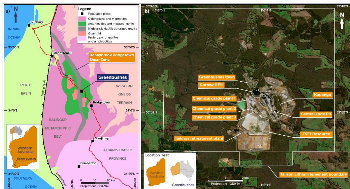
Figure 4: Greenbushes location, regional geology, and infrastructure
