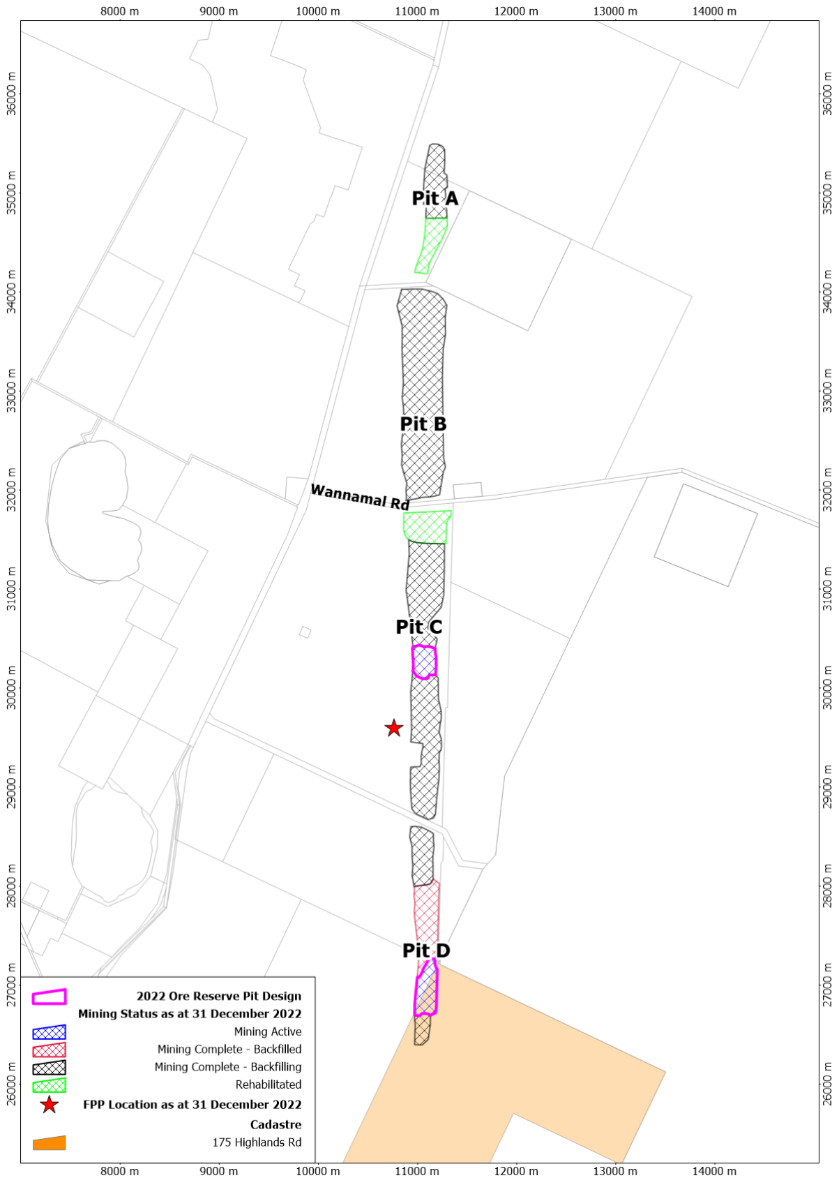
Figure 3 - Mining Status as at 31 December 2022
