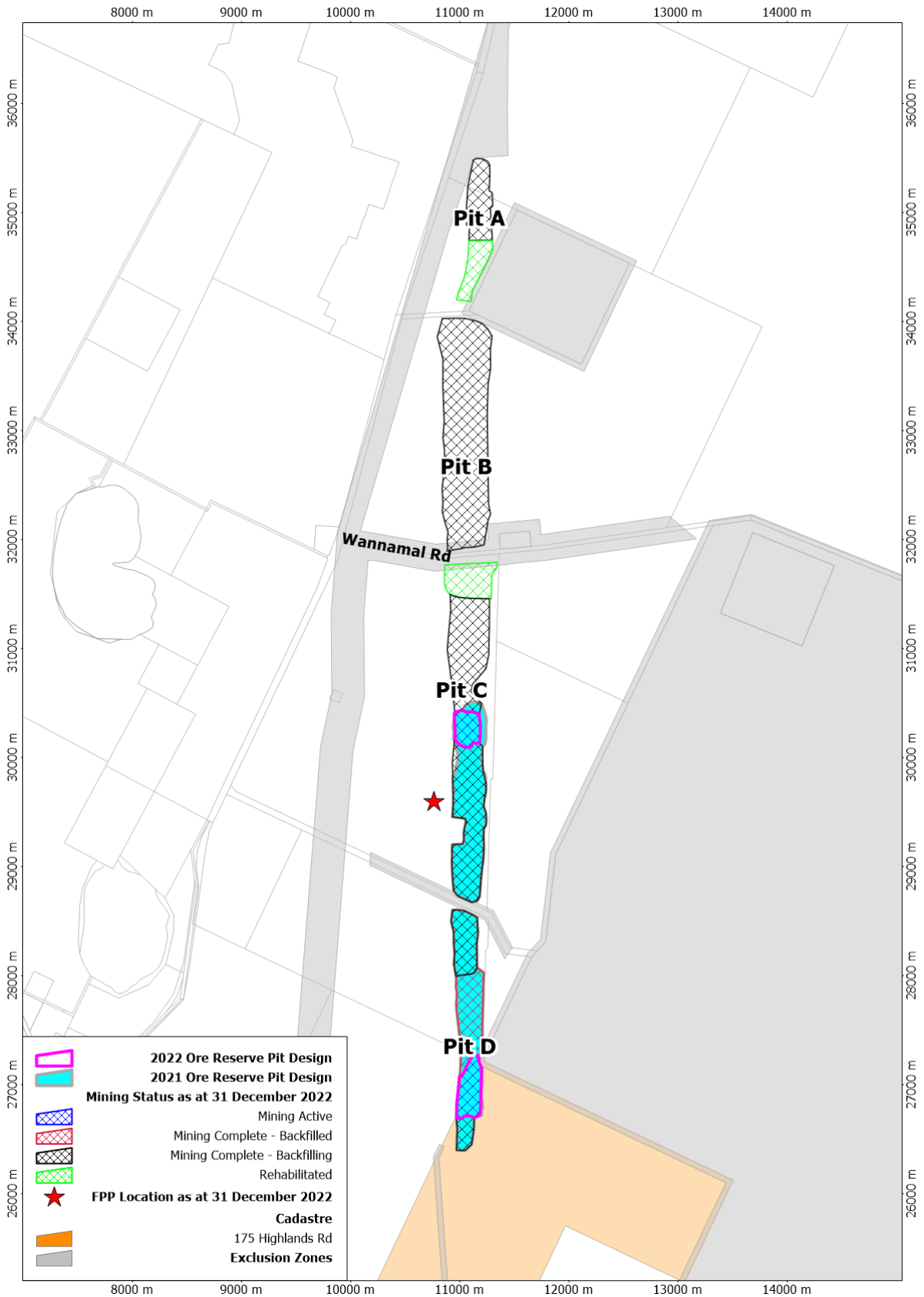
Figure 5 - 2021 and 2022 Ore Reserve Pit Outlines
