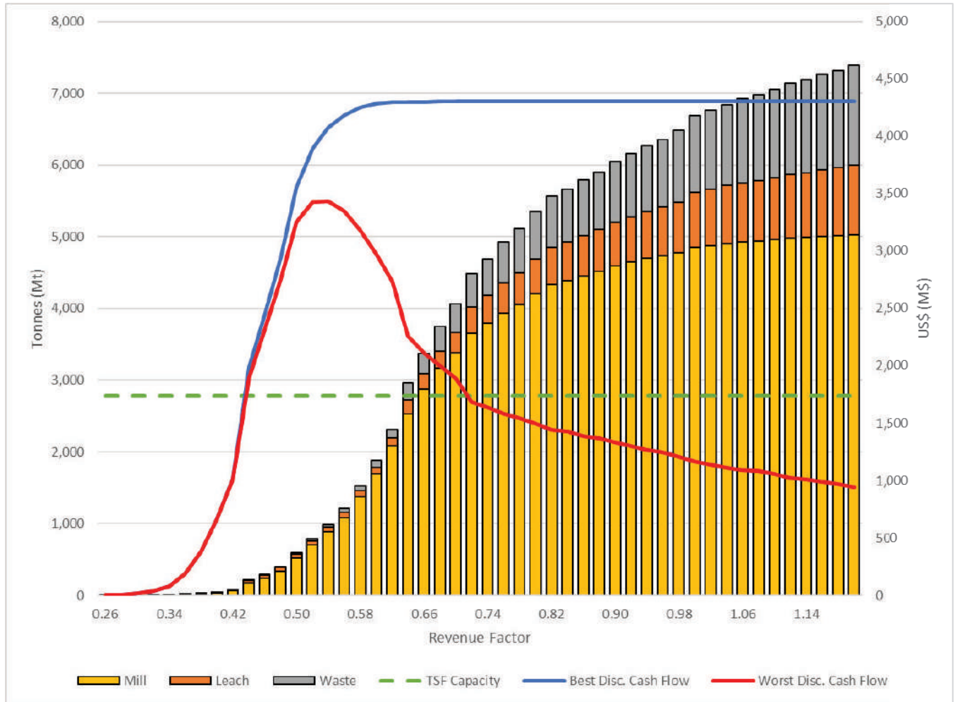
Figure 12.2: Summary of LC Nested Pit Analysis
