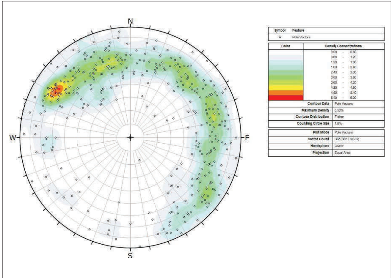
Figure 7.11: Stereographic Project of Major Faults
