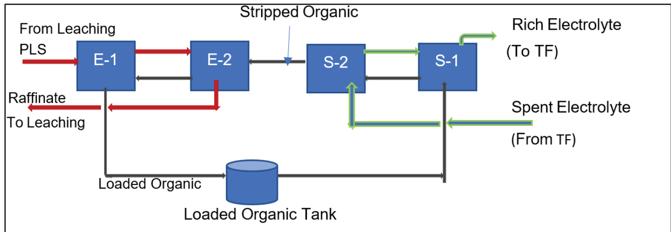
Figure 14.8: Original Series SX Configuration
