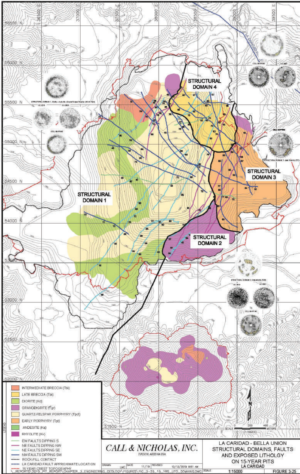
Figure 7.10 : CNI Structural Domain Map
