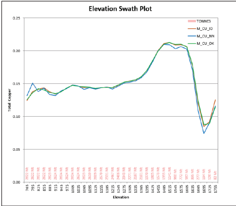
Figure 11.16: Plan Cu Swath Plot
