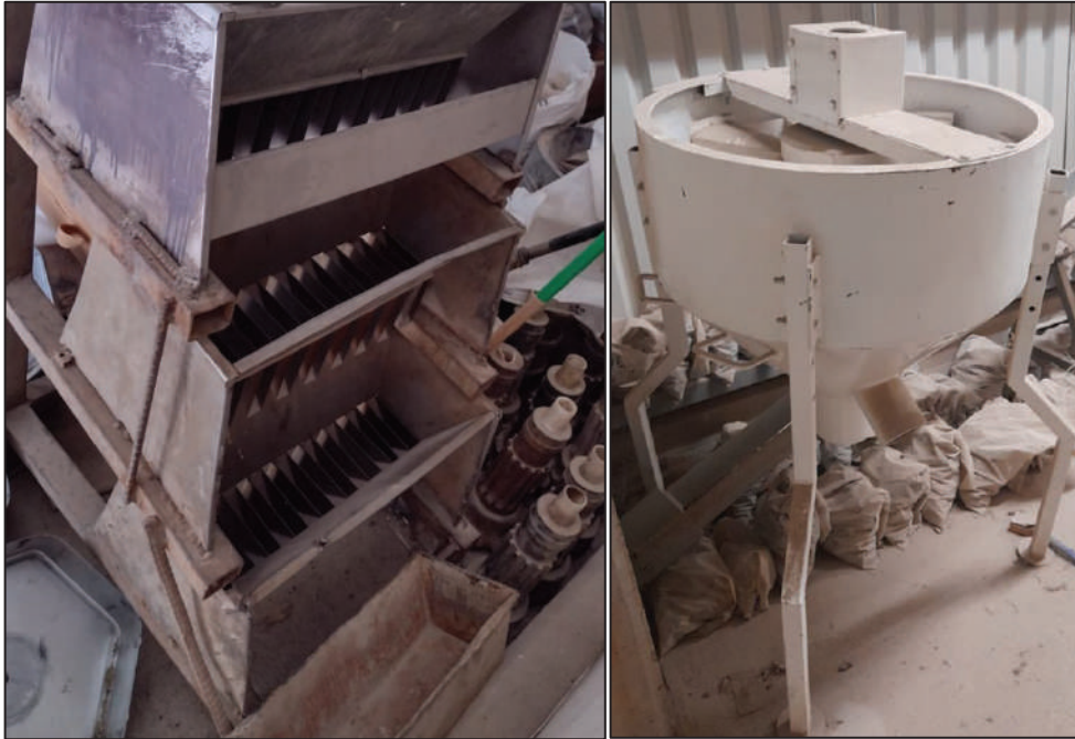
Figure 8.1: Jones Splitter – RC Sample Splitter, Left, Mechanical Splitter, Right
