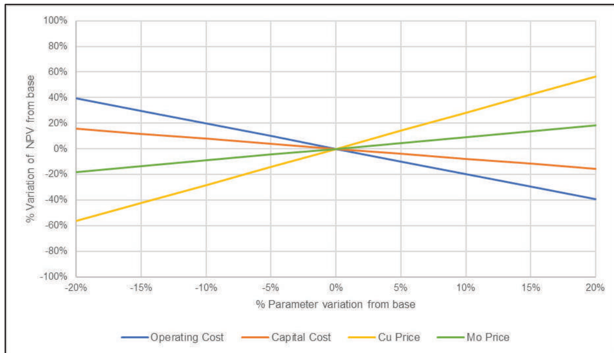
Figure 19.1: Sensitivity Analysis
