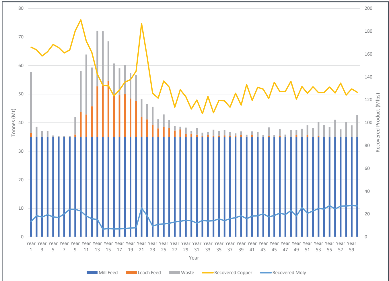
Figure 13.4: LOM Plan Production Statistics
