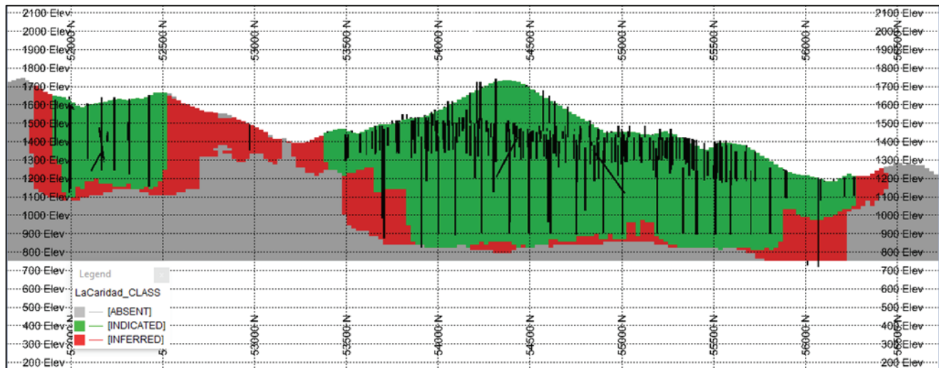
Figure 11.19: S-N Section (38,000 E) of Resource Classification Assigned to the Block Model
