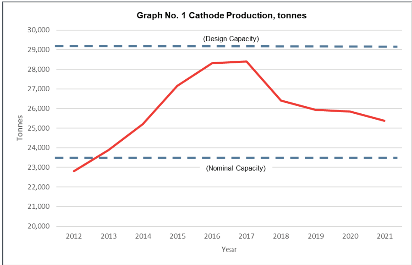
Figure 14.11: Cathode Production (tonnes)
