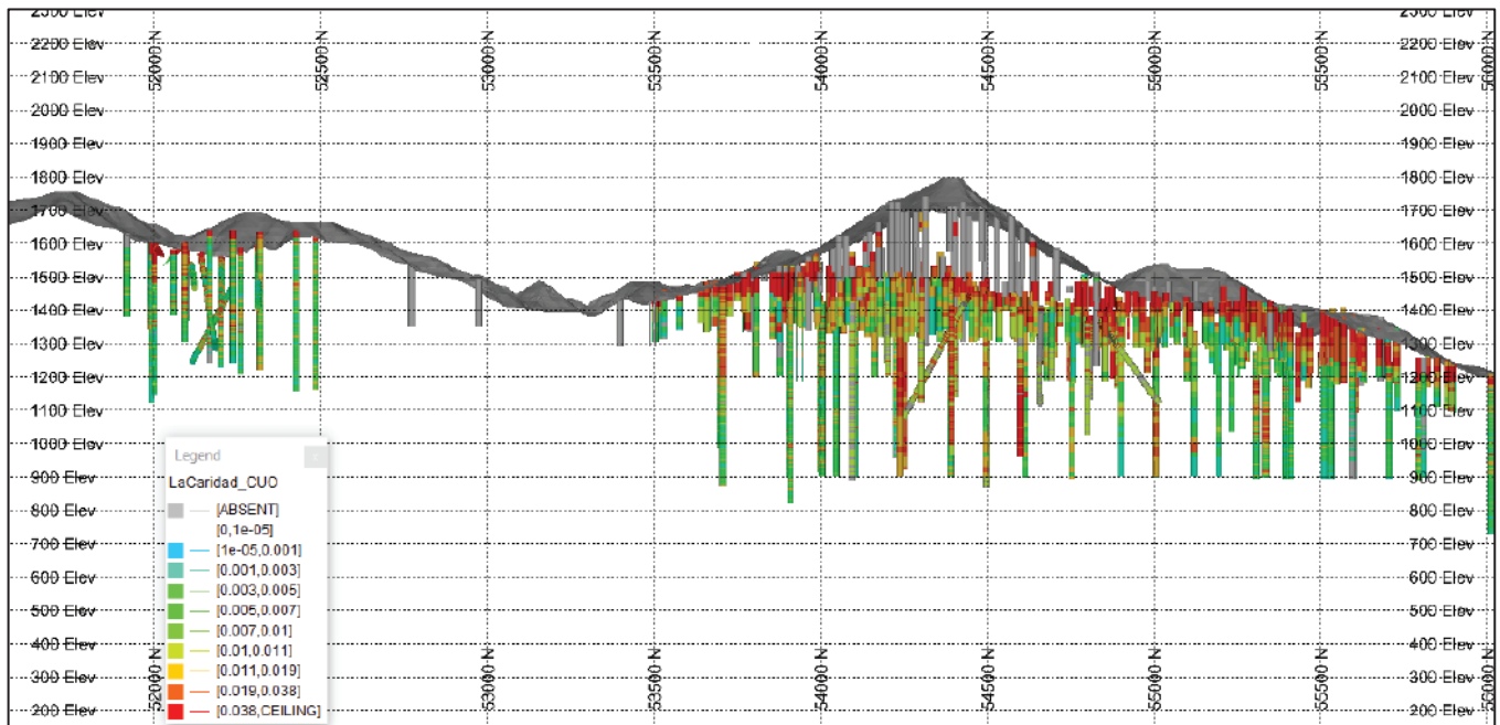
Figure 11.5: South-North Section (38,000 E) of Drill Holes Showing CuO
