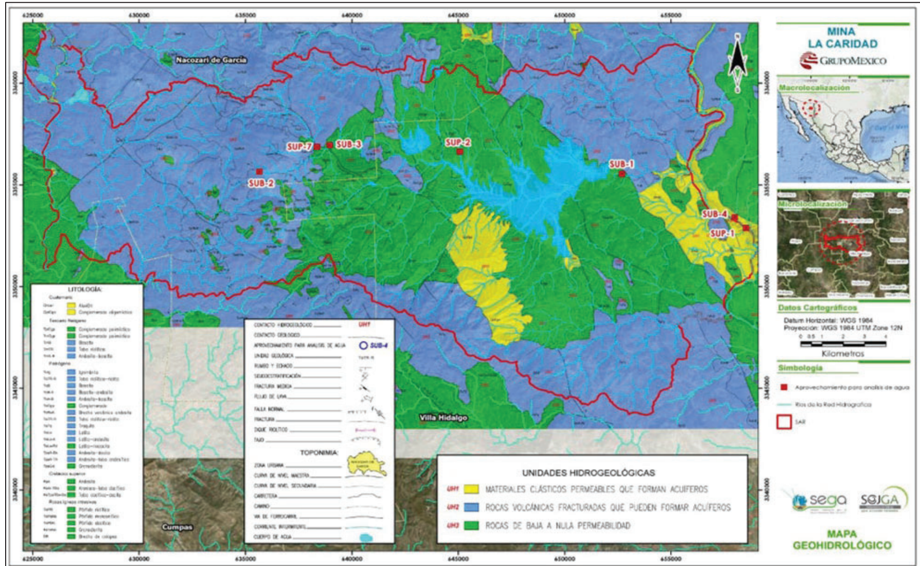
Figure 7.9: Hydrogeological Units
