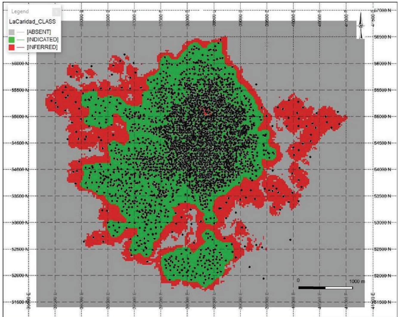
Figure 11.18: Plan View of Resource Classification Assigned to the Block Model
