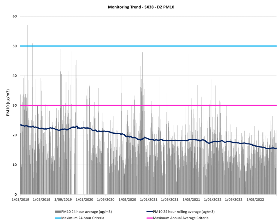
Figure 6-17 SX38 D2 TEOM monitoring trend 2019-2022
