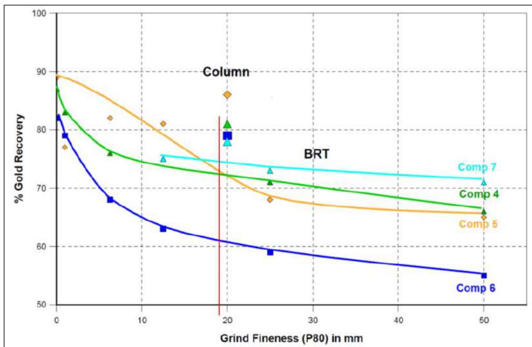
Figure 13-3 – Gold extraction vs. P80 size.
