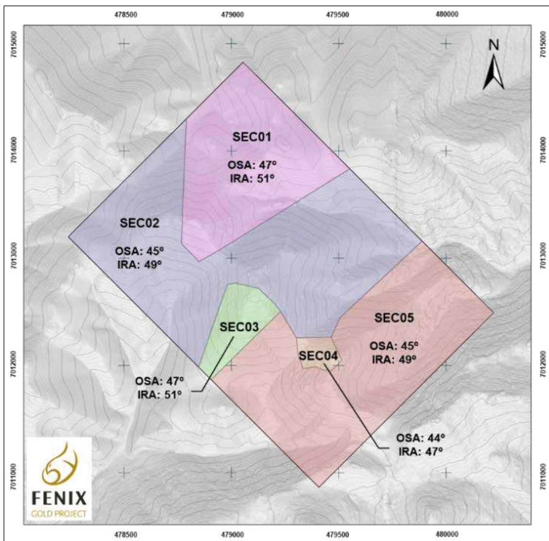
Figure 15-2 – Overall slope angle for pit optimization.
