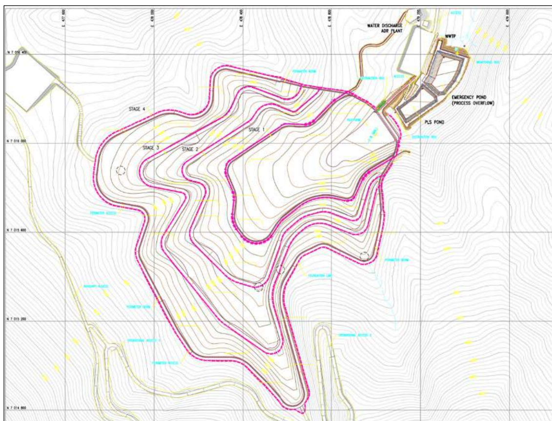
Figure 17-5 – Heap leach pad layout.
