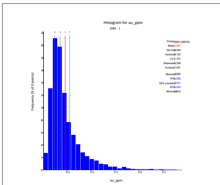
Figure 14-16 – Histogram of gold composite grades of Fenix Central A – BX.
