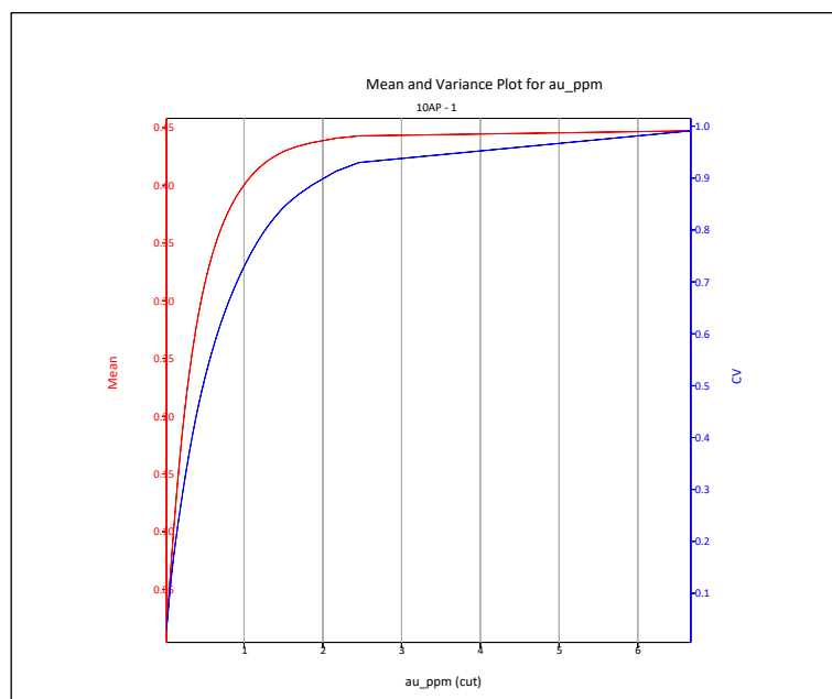
Figure 14-6 – Mean and coefficient of variation plot for Fenix North AP.
