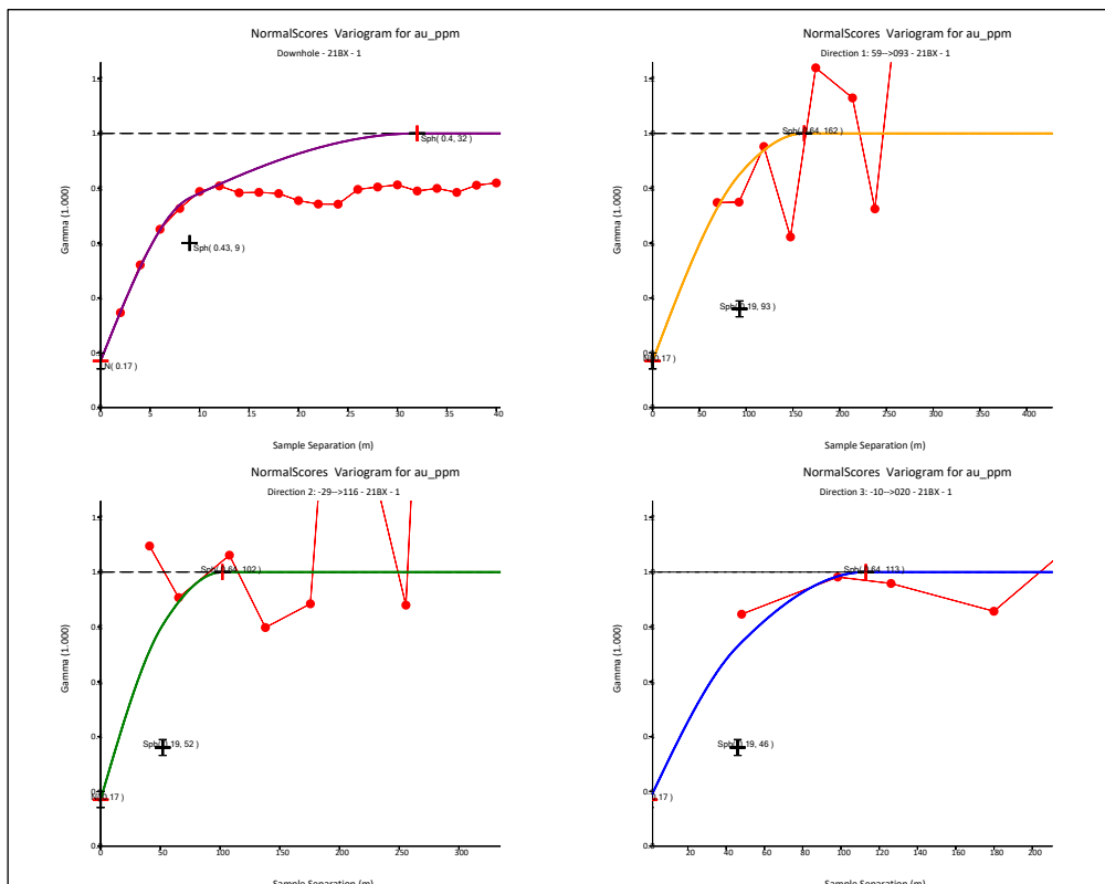
Figure 14-61 – Directional variogram model, Fenix Central B – BX.
