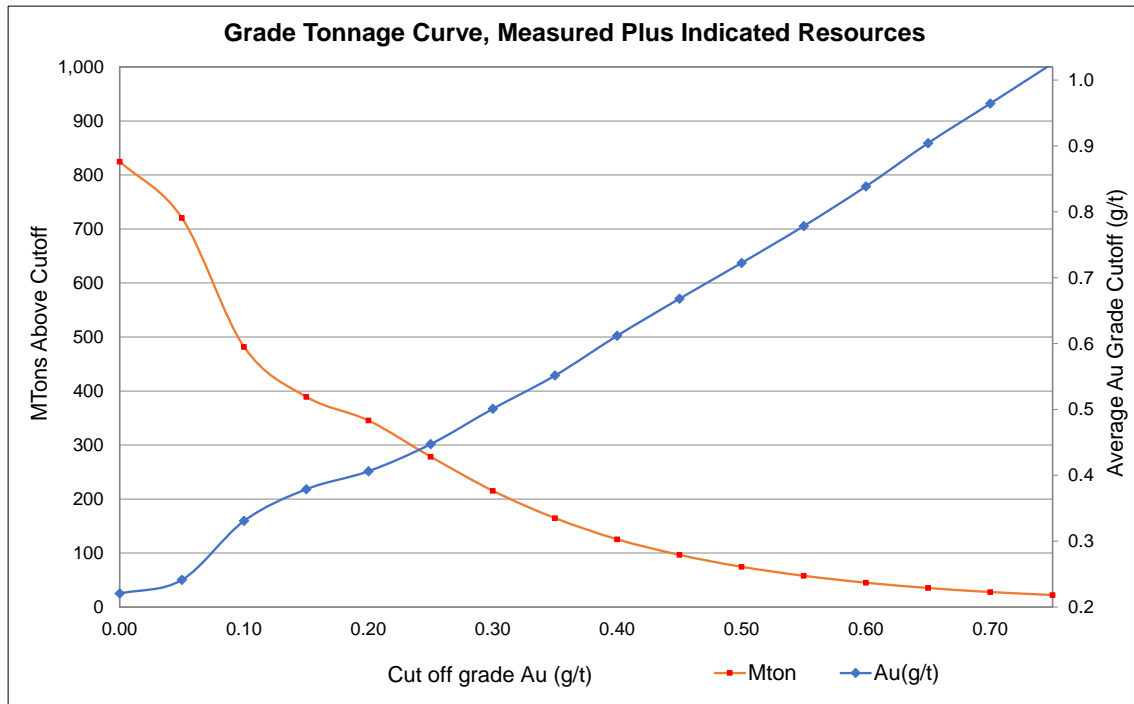
Figure 14-78 – Grade-Tonnage Curve, Measured + Indicated Resources, Fenix Gold Project.
