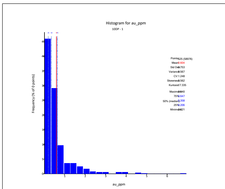
Figure 14-10 – Histogram of gold composite grades of Fenix North DP.
