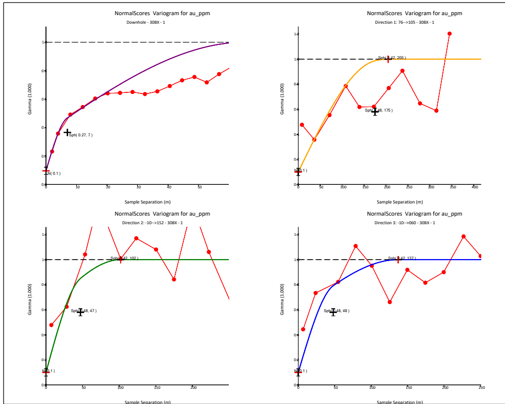
Figure 14-64 – Directional variogram model, Fenix South BX.
