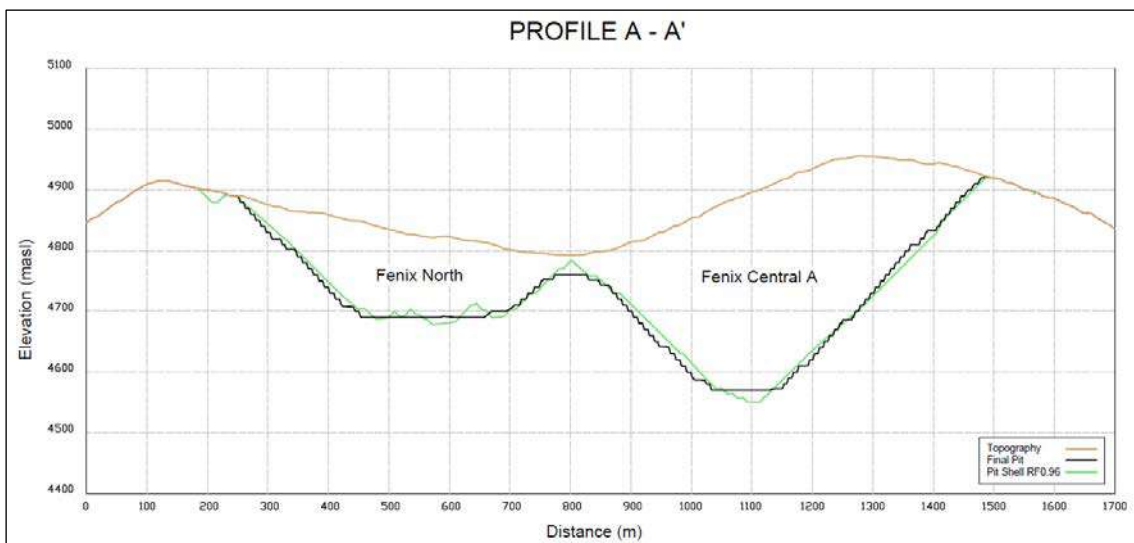
Figure 16-4 – Profile A-A' - Pit design and pit shell.
