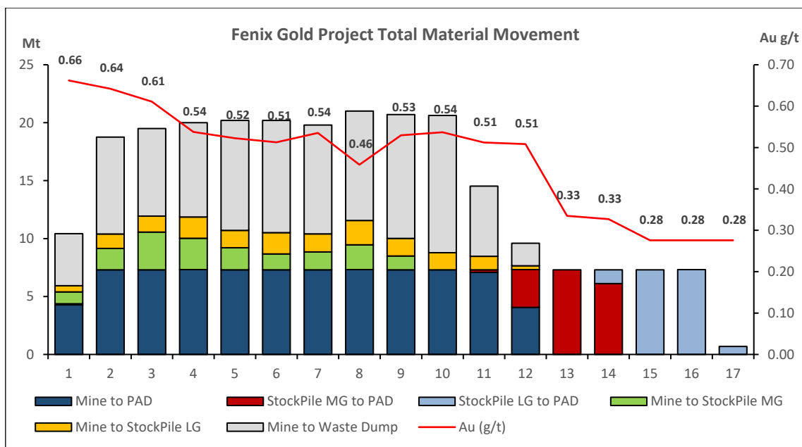
Figure 1-3 – Fenix Gold Project, Mine schedule.
