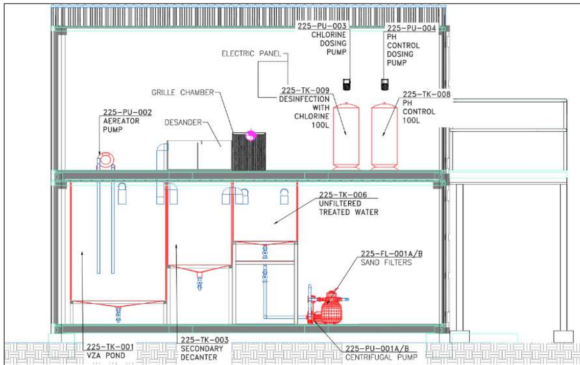
Figure 18-8 – Sewage treatment plant.
