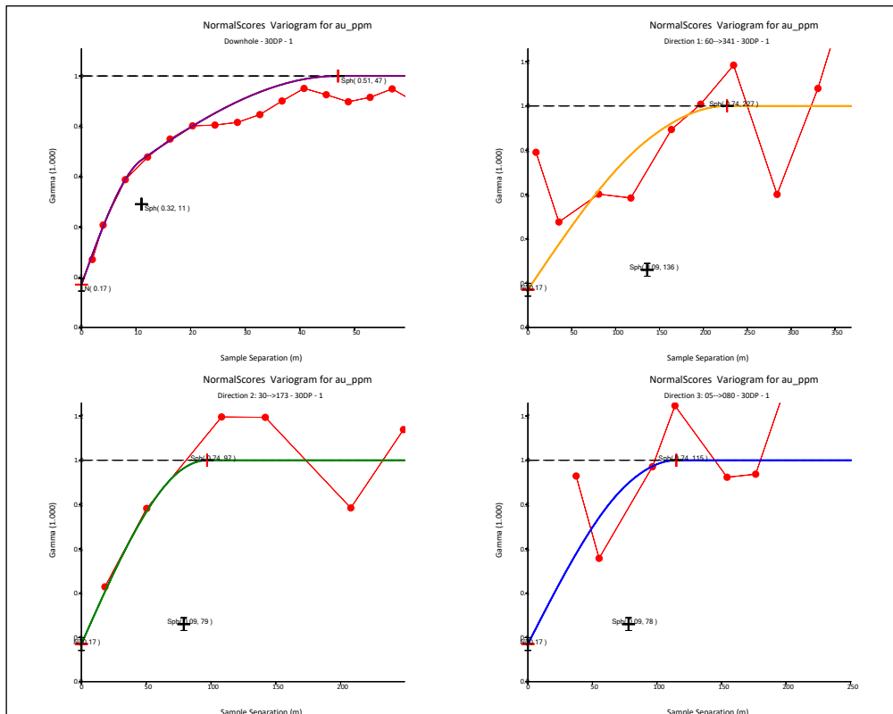
Figure 14-65 – Directional variogram model, Fenix South DP.
