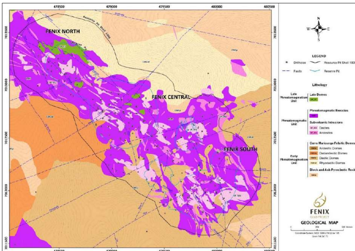
Figure 7-3 – Geologic map of the Fenix Gold Project.
