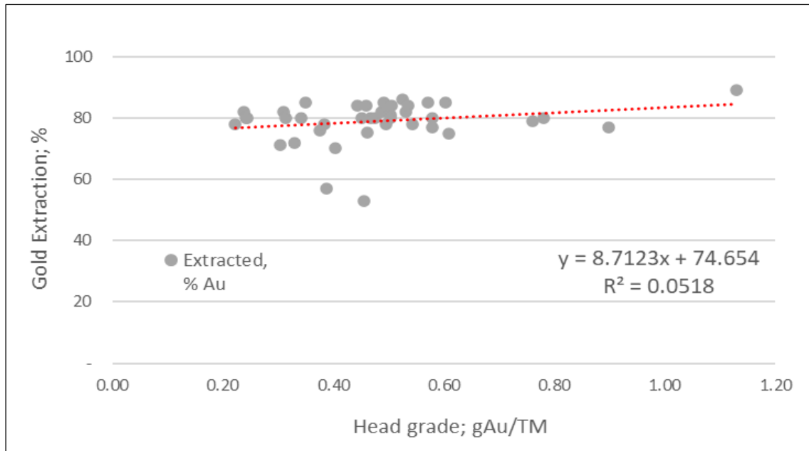
Source: HLC Ingeniería y Construcción SpA, 2023, NI 43-101 Technical Report Fenix Gold Project. Figure 13-7 – Gold extraction vs. Gold head grade (P100: 19 mm/150 mm).
