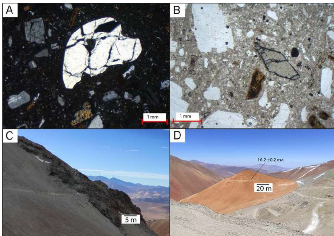
Figure 7-4 – Corroded quartz eye, hornblende, biotite a), and sphene phenocrysts in a vitreous fundamental mass altered to smectites (b). View of a felsic dome on the NE slope of Fenix North and (c) view of dacitic dome SW of Fenix South (d).
