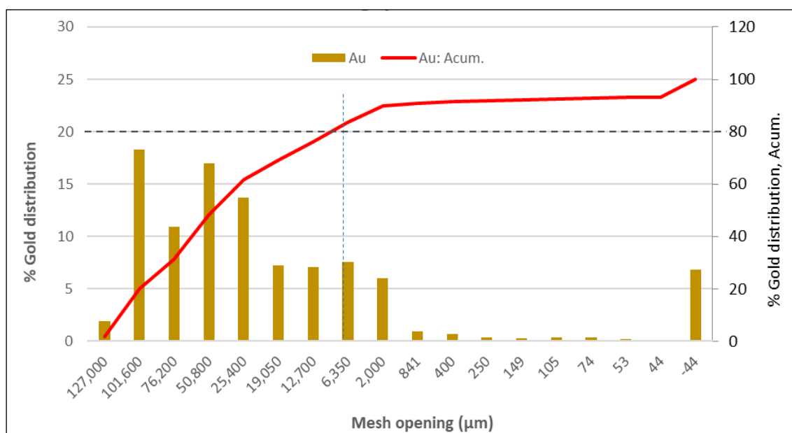
Figure 13-6 – Gold distribution by leach residue size range analysis.
