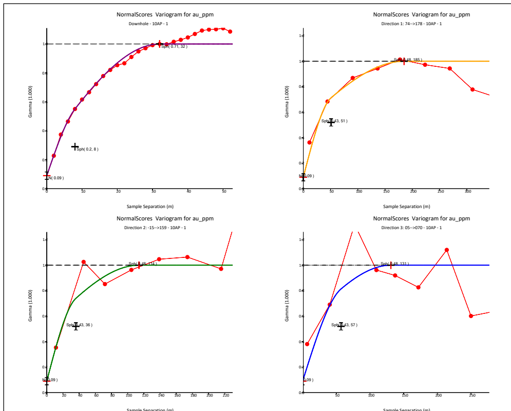
Figure 14-54 – Directional variogram model, Fenix North AP.
