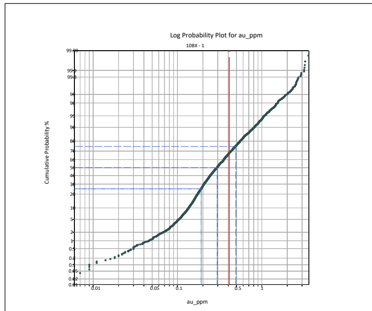
Figure 14-8 – Probability plot of gold composites, Fenix North BX.
