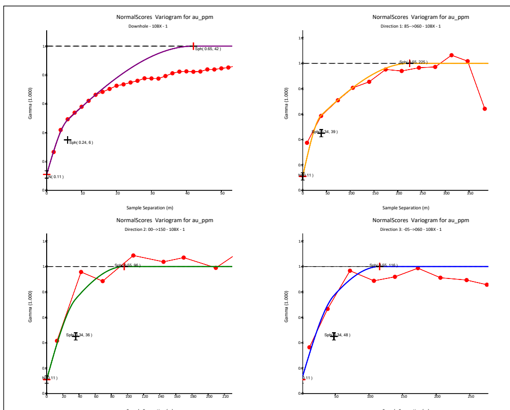
Figure 14-55 – Directional variogram model, Fenix North BX.
