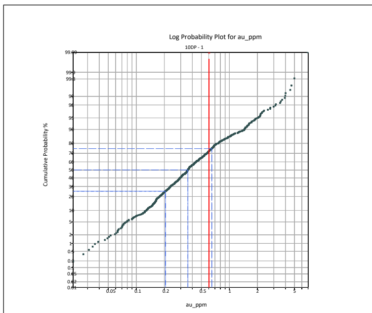
Figure 14-11 – Probability plot of gold composites, Fenix North DP.
