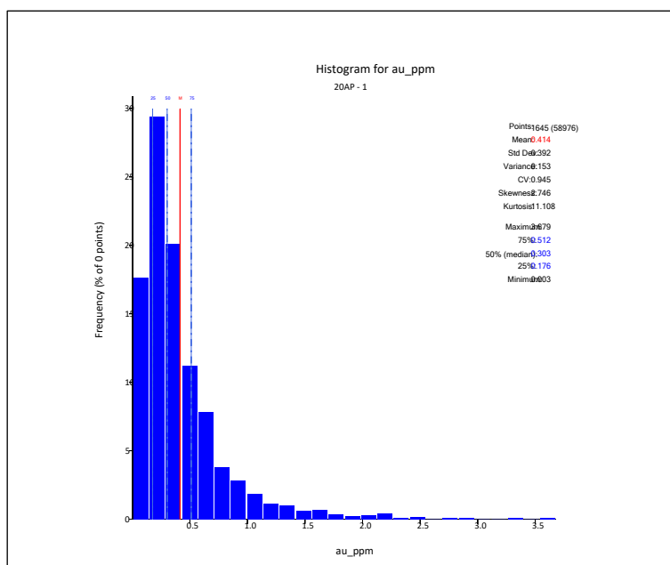
Figure 14-13 – Histogram of gold composite grades of Fenix Central A – AP
