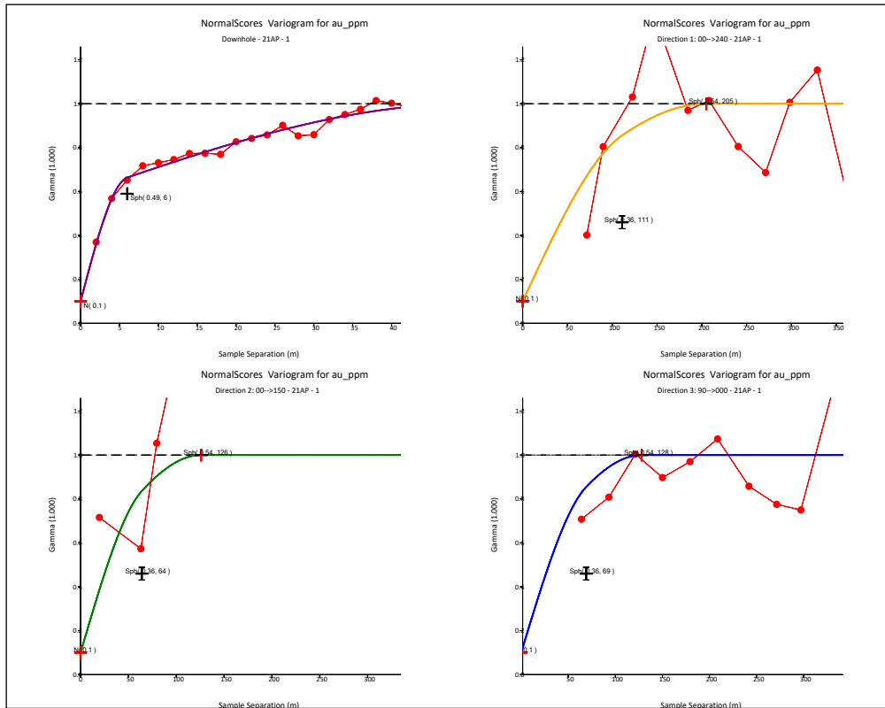
Figure 14-60 – Directional variogram model, Fenix Central B – AP.
