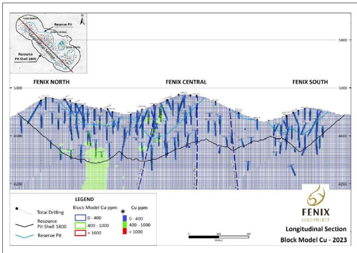
Figure 14-77 – Longitudinal section (looking NE), estimated Cu grades and composites.
