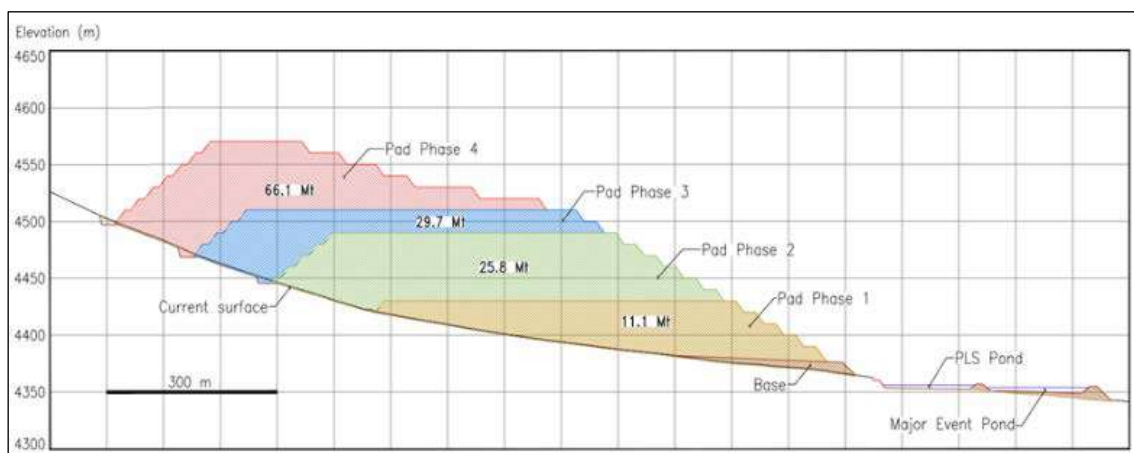
Figure 16-23 – Leach Pad (PAD), PLS Pond, Major Event Pond – Section.
