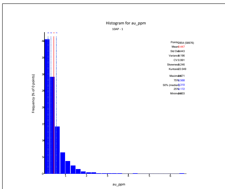
Figure 14-4 – Histogram of gold composite grades of Fenix North AP.
