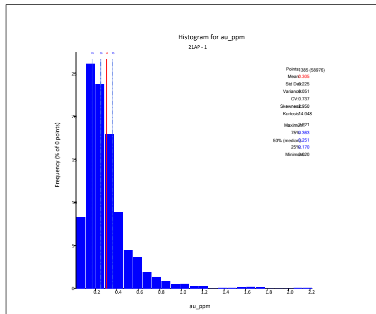
Figure 14-22 – Histogram of gold composite grades of Fenix Central B-AP.
