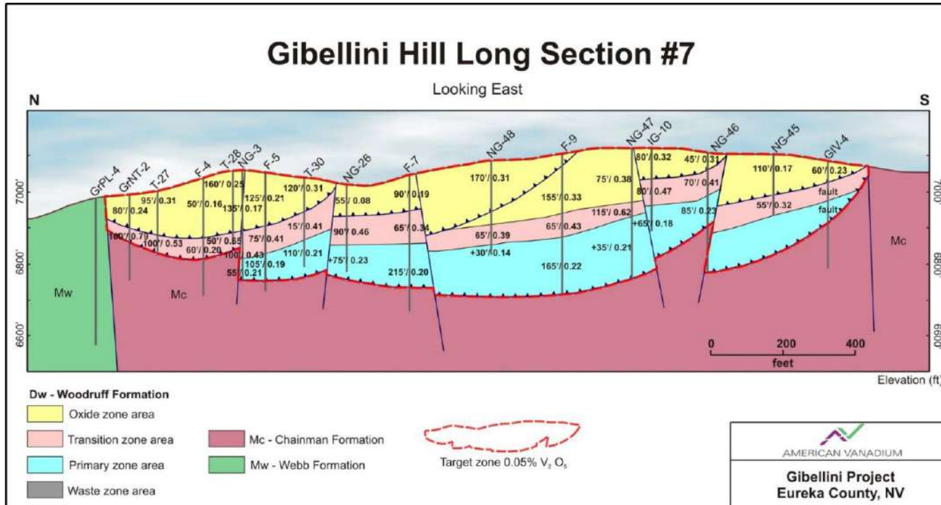
Figure 7-4: Long-section Across Gibellini (looking northeast)
