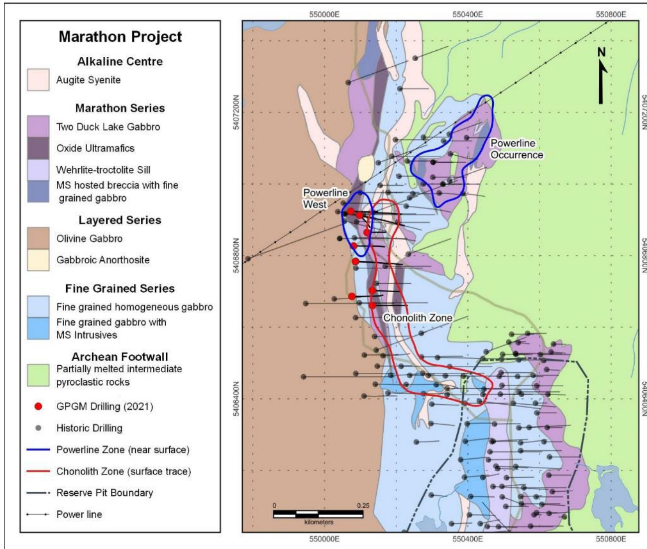
Figure 7.18: North End of the Marathon Deposit Showing the Biowobik Prospect including the Chonolith and Power Line Occurrences
