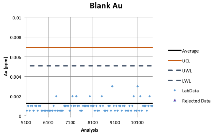
Figure 11.35: Performance of Blanks for Pt
