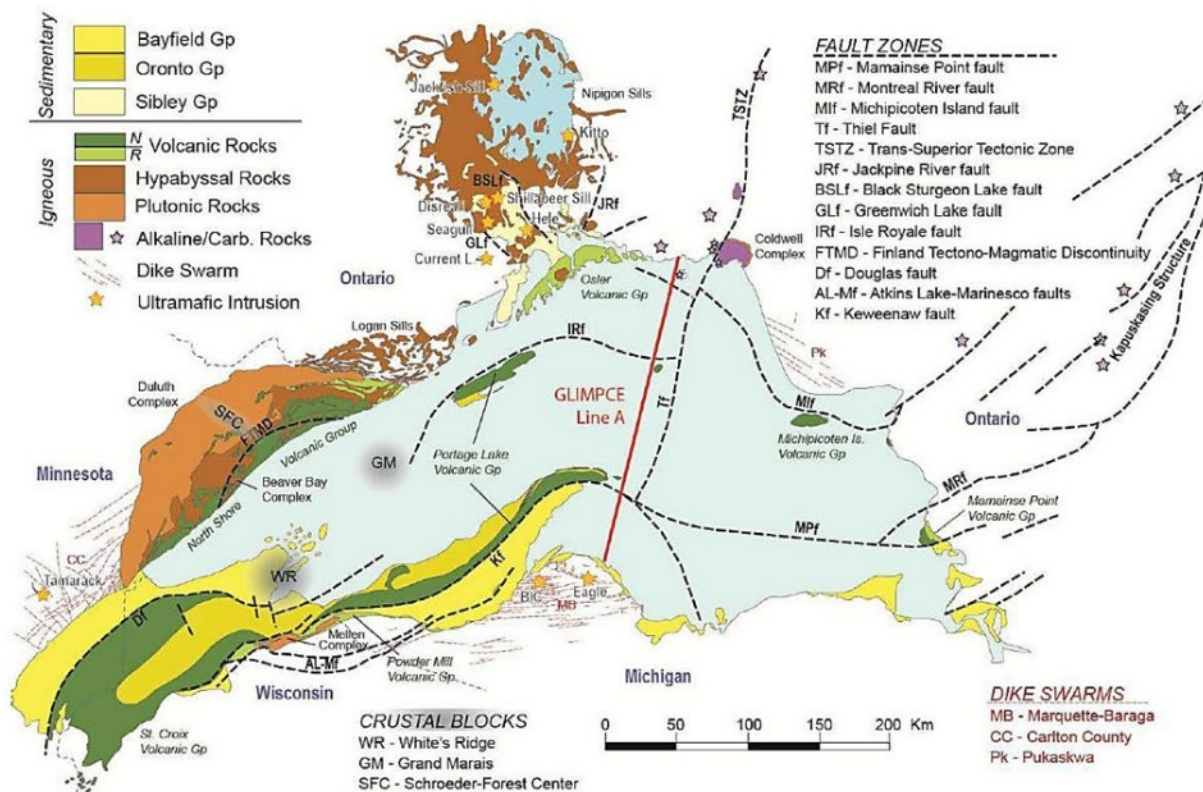
Figure 1.3: Regional Structural Geology
