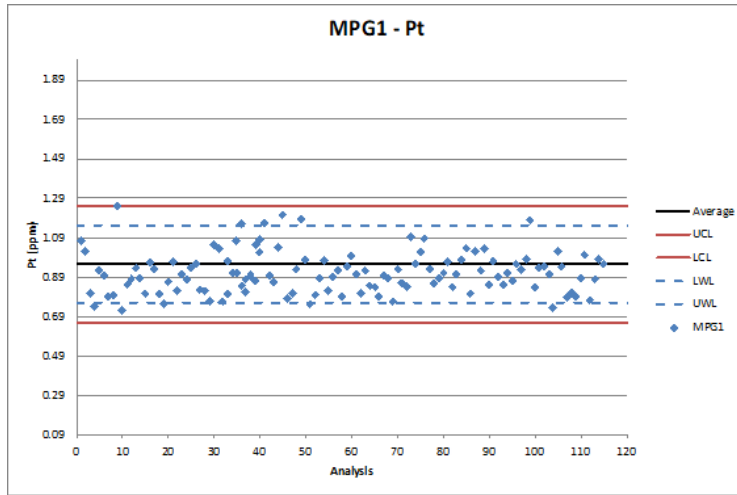
Figure 11.2: Performance of CRM MPG1 for Pt
