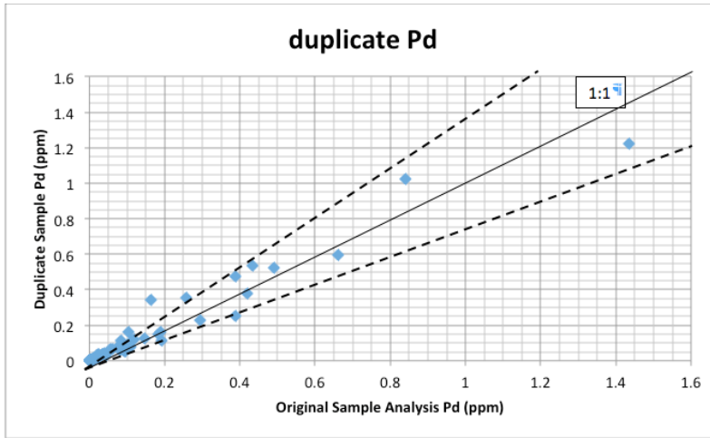
Figure 11.41: Performance of Field Duplicates for Pd
