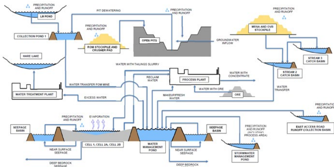
Figure 18.12: Site Wide Water Balance (KP)
