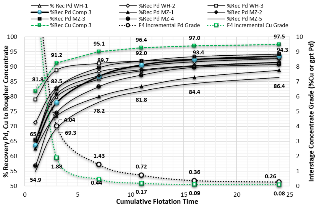
Figure 13.5: Rougher Flotation Rate Kinetics and Interstage Grade
