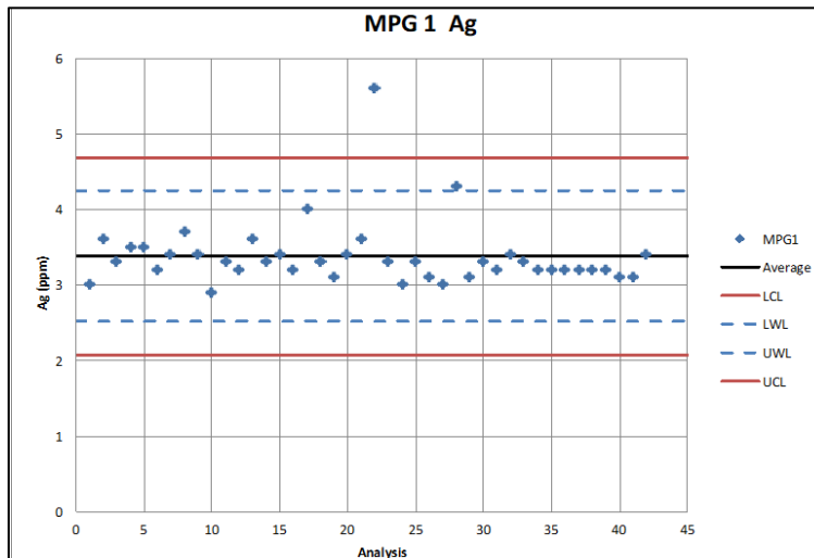
Figure 11.62: Performance of CRM MPG1 for Ag
