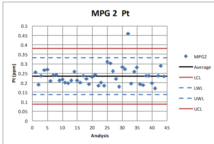
Figure 11.65: Performance of CRM MPG2 for Pt
