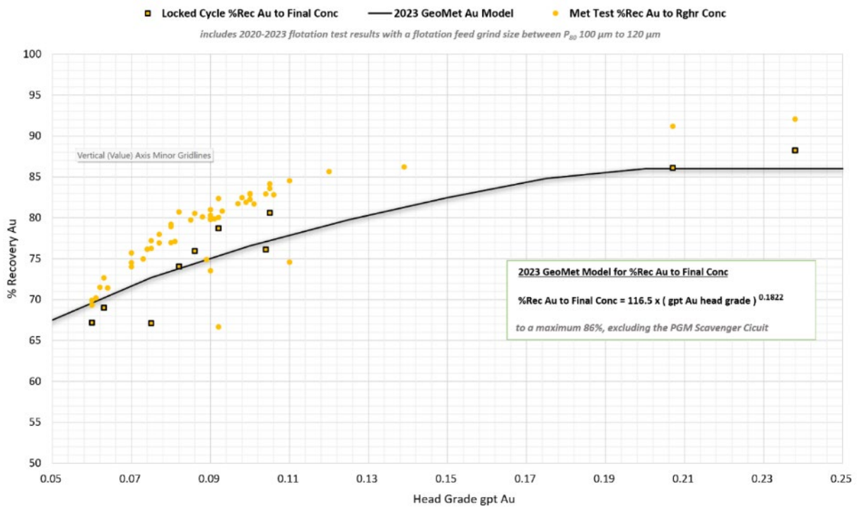
Figure 13.12: GeoMet Model for Gold Recovery to Final Concentrate
