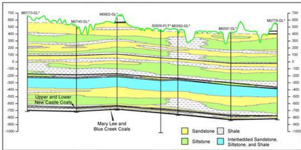
Figure 6-2: Generalized Geologic Profile Indicating Dominant Overburden Lithologies
