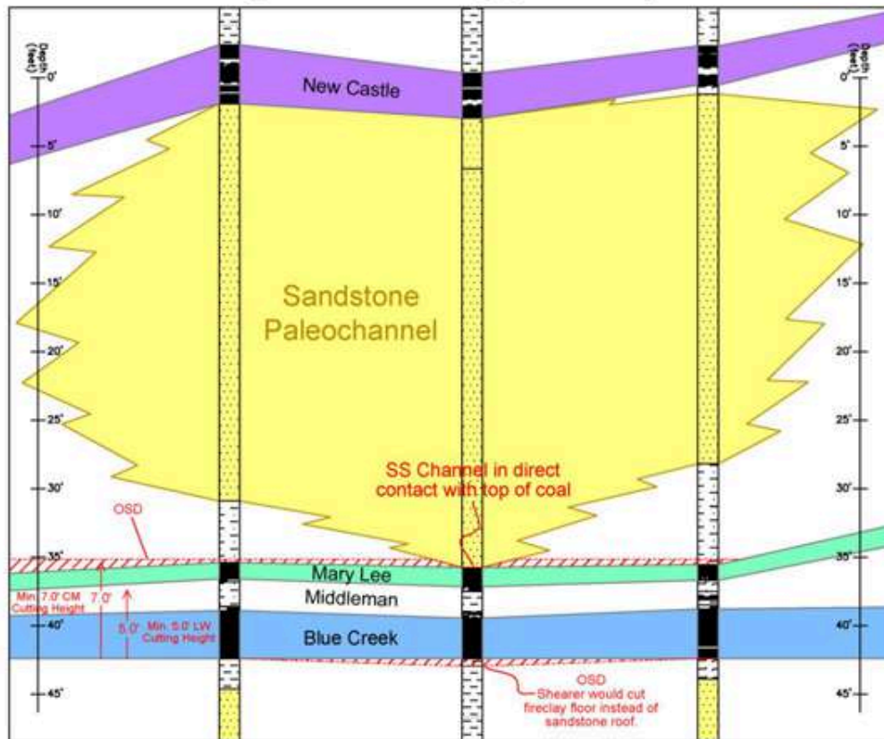
Figure 6-3: Mine No. 4 Stratigraphic Relationships
