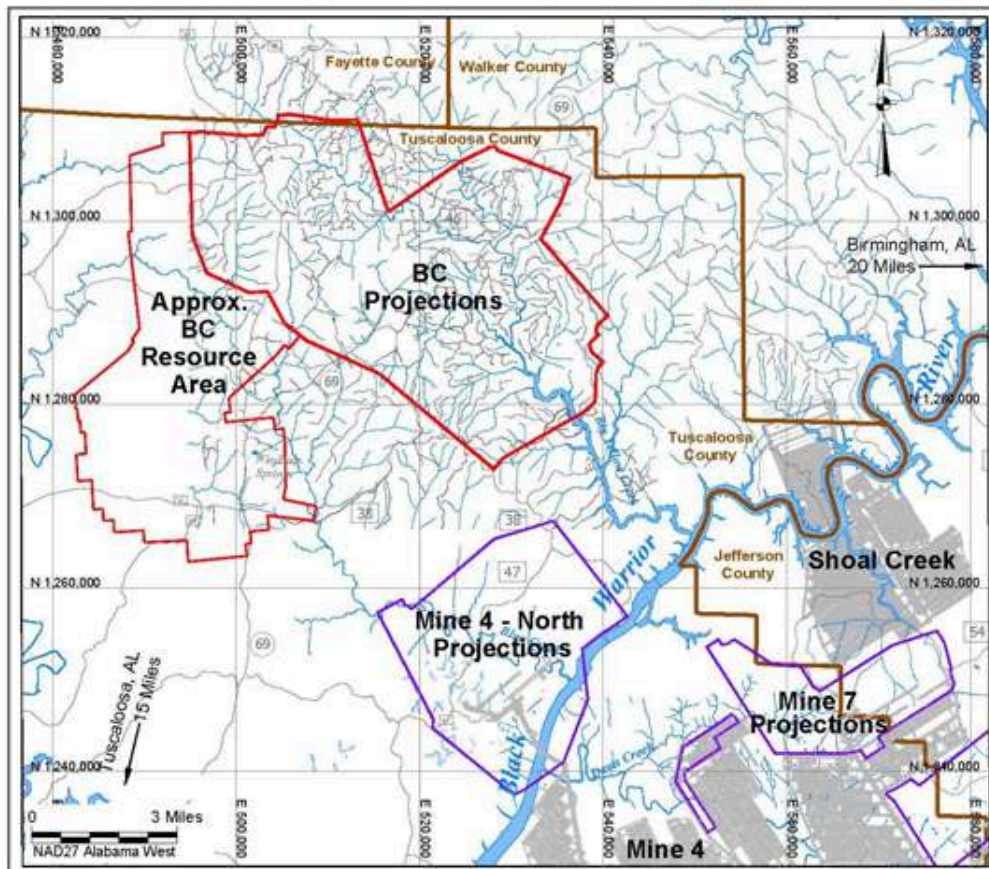
Figure 1-1: Blue Creek Project Location Map
