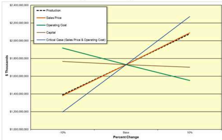
Figure 19-2: Sensitivity of NPV
