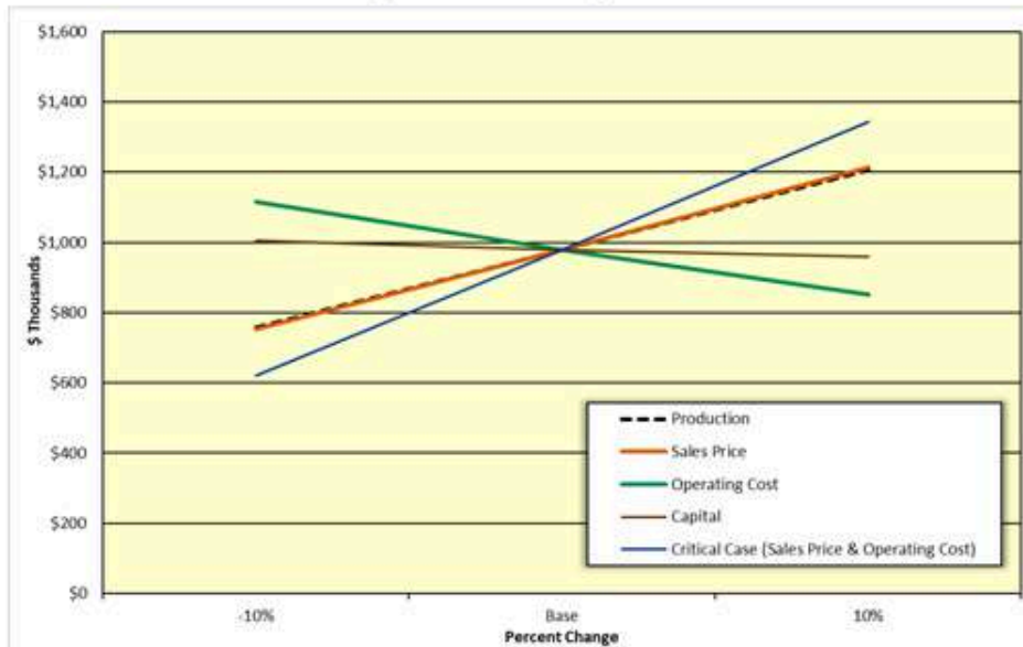
Figure 19-3: Sensitivity of NPV
