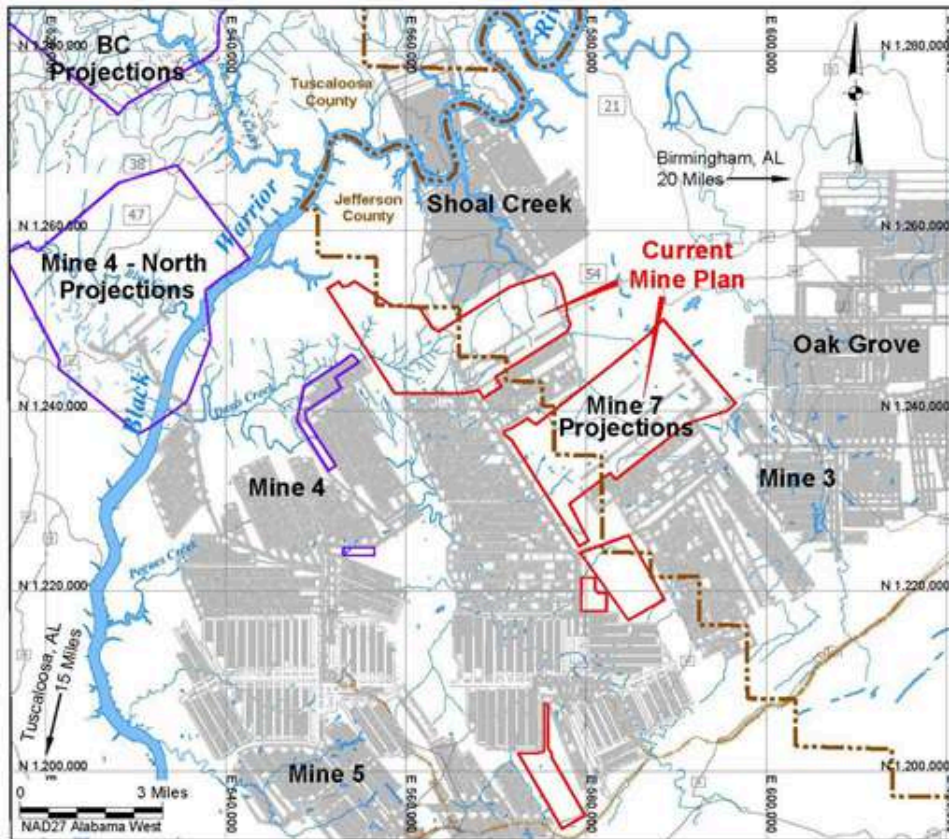
Figure 3-1: Warrior Met Mine No. 7 Complex Property Location Map
