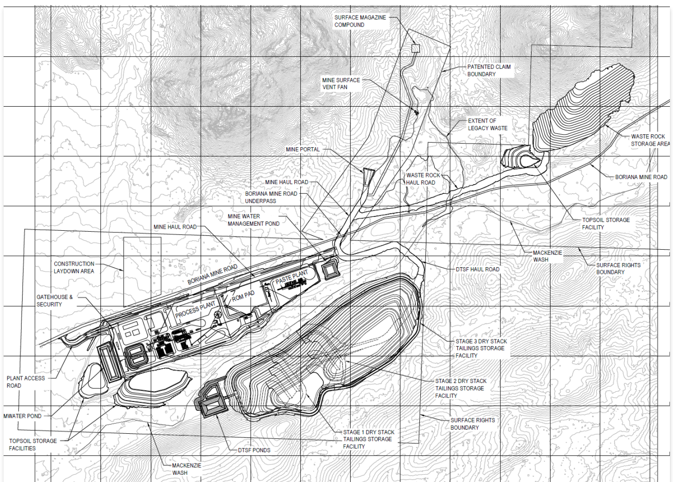
Figure 10 Project layout
