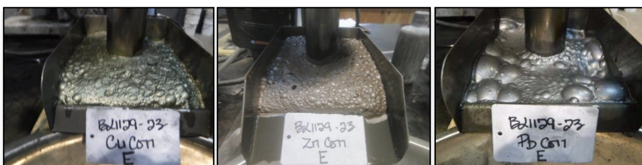
Figure 8 Photos of Copper, Zinc and Lead-Silver concentrate from Locked Cycle Testing
