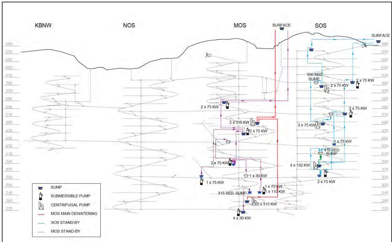
Figure 16-10: Dewatering System
