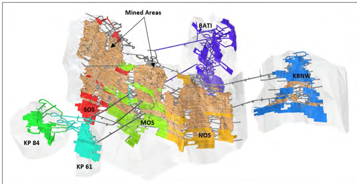
Figure 16-1: Isometric View Showing Mine Areas and Vein Wireframe (Eldorado, 2023)
