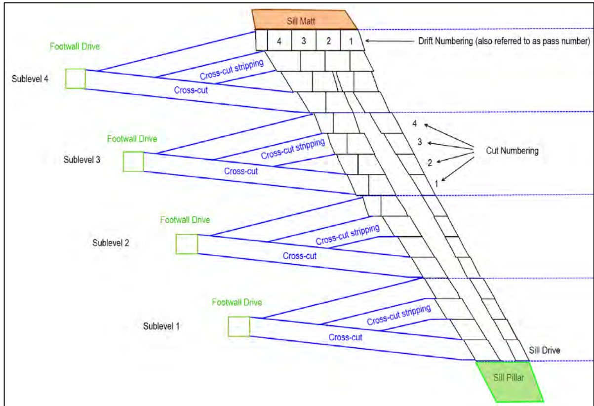
Figure 16-2: Schematic Cross Section Showing DAF Production Block Layout
