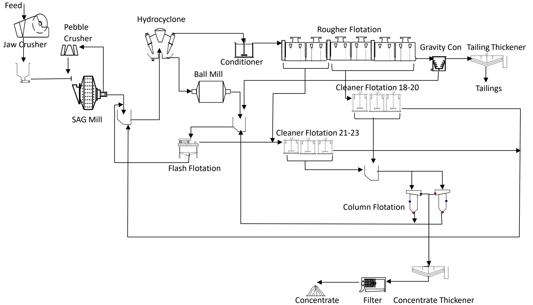
Figure 17-1: Simplified Plant Process Flow Diagram with Column Flotation Cells
