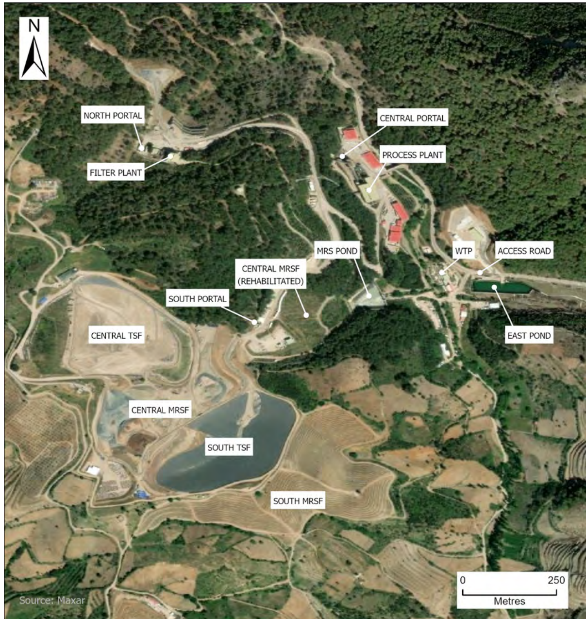
Figure 18-2: Project Layout (Eldorado 2023)
