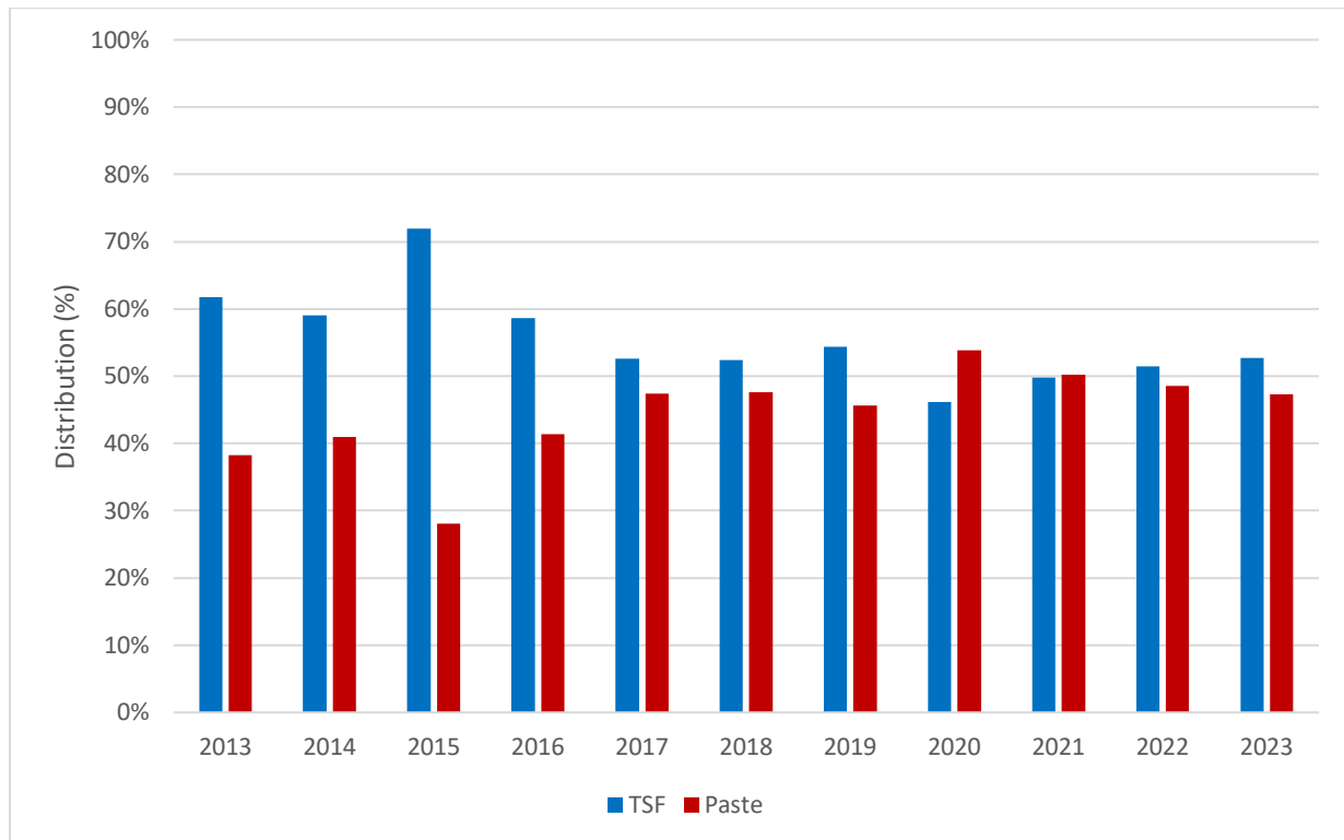
Figure 17-3: Distribution of Flotation Tailings to TSF and Paste Plant
