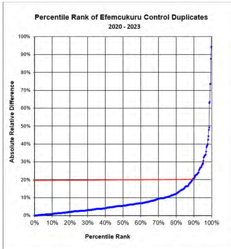
Figure 11-4: Percentile Rank Plot, Efemçukuru 2020-2023 Duplicate Data
