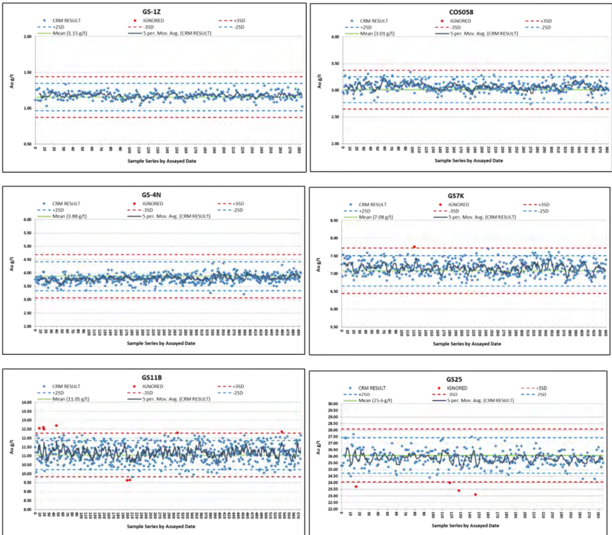
Figure 11-1: CRM Charts, 2020 to 2023, Efemçukuru Mine
