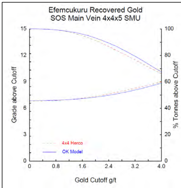
Figure 14-15: HERCO plot, SOS domain
