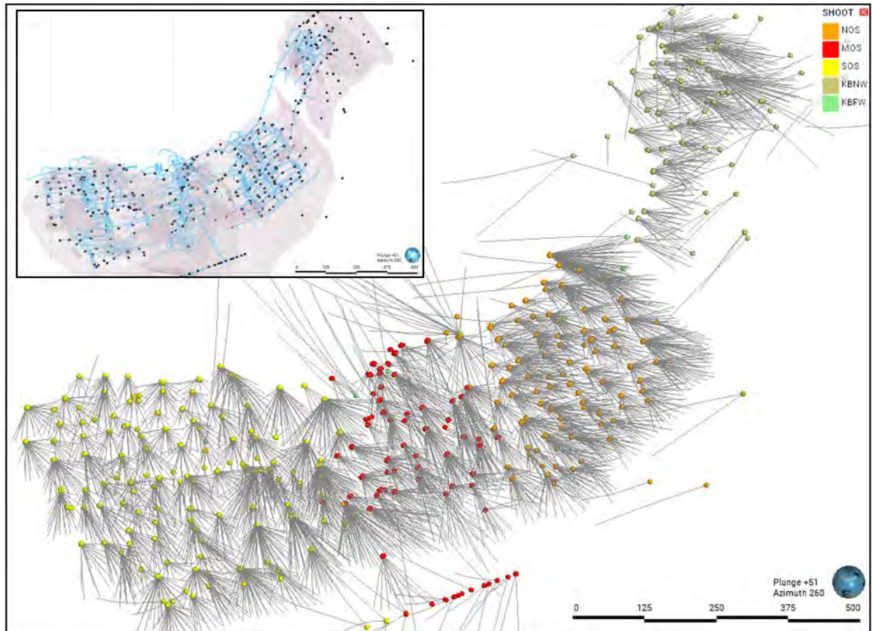
Figure 10-2: Oblique 3-D view (facing west) of Infill Drillhole Collars and Traces, Kestanebeleni
