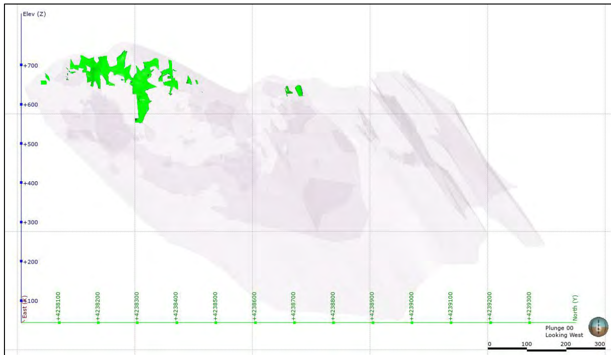
Figure 14-2: Modeled voids in the Kestanebeleni Vein System (Eldorado, 2019)
