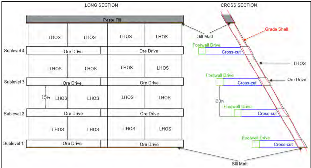
Figure 16-3: Schematic Long and Cross Sections Showing LHOS Production Block Layout
