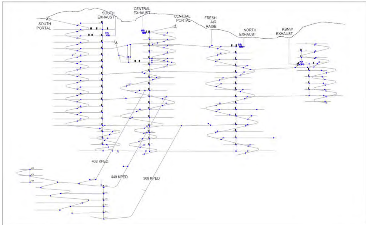
Figure 16-9: Primary Ventilation Components
