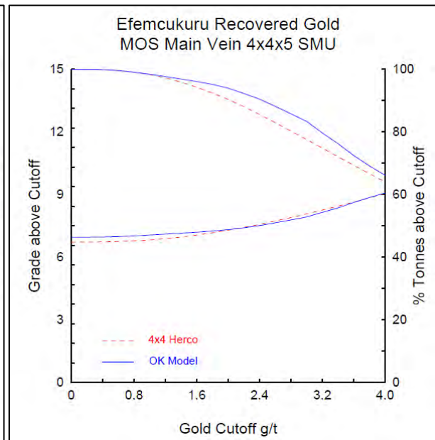
Figure 14-16: HERCO plot, MOS domain
