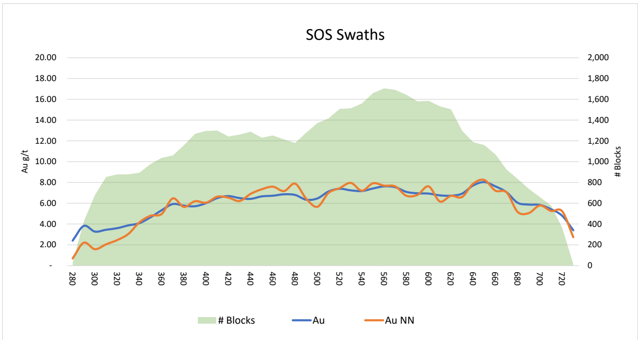
Figure 14-12: Model Trend Plot showing 10 m Binned Averages along Elevations for OK and NN Gold Grade Estimates, SOS Domain
