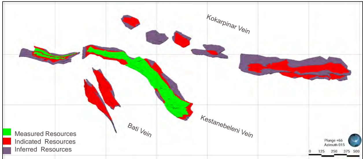
Figure 14-18: Mineral Resources Classification, Efemçukuru Mine (Eldorado, 2023)
