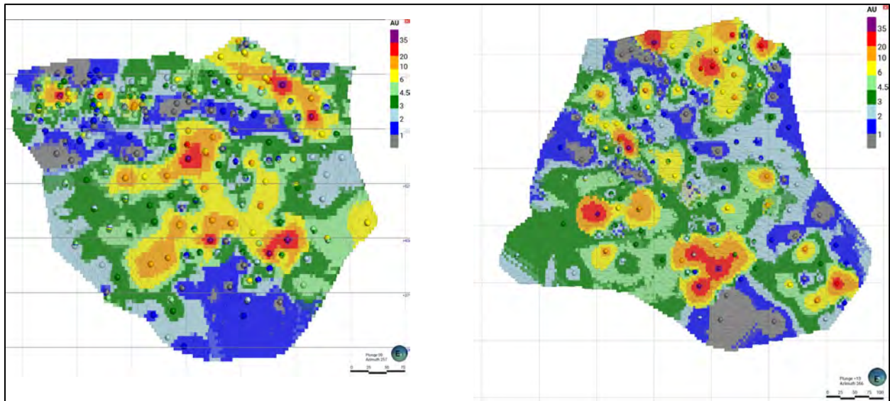
Figure 14-11: Batı Veins (#1 on Left, #2 on Right) Modeled Grades and Composited Drill Hole Samples (Au, g/t) (Eldorado, 2023)
