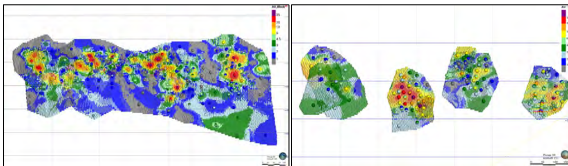
Figure 14-10: Modeled Kokarpınar Domains (KPS on left; KPM on right) and Composited Drill Hole Samples (Au, g/t) (Eldorado, 2023)
