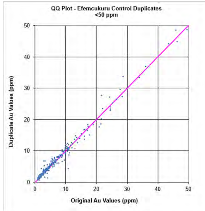
Figure 11-5: QQ Plot for Efemçukuru Duplicate Data
