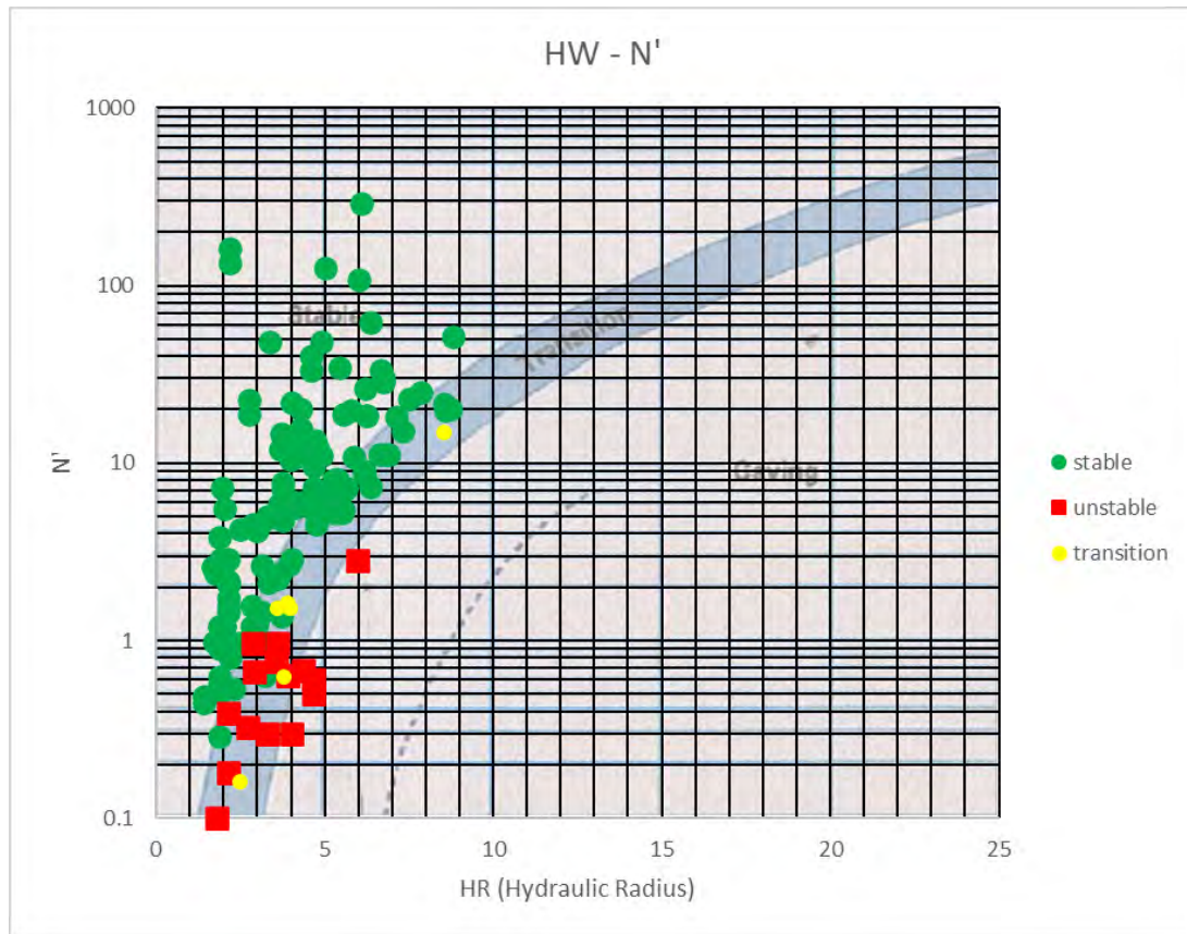
Figure 16-5: Back Analysis of Stope Performance (The Mathews Stability Graph)
