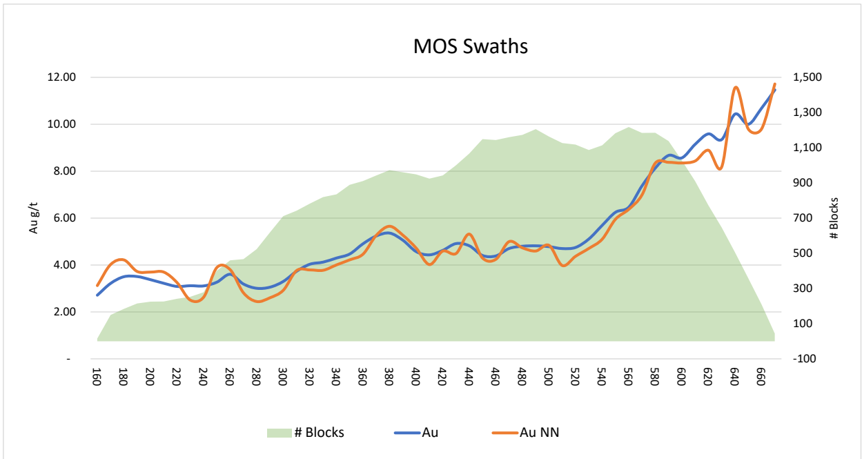
Figure 14-13: Model Trend Plot showing 10 m Binned Averages along Elevations for OK and NN Gold Grade Estimates, MOS Domain
