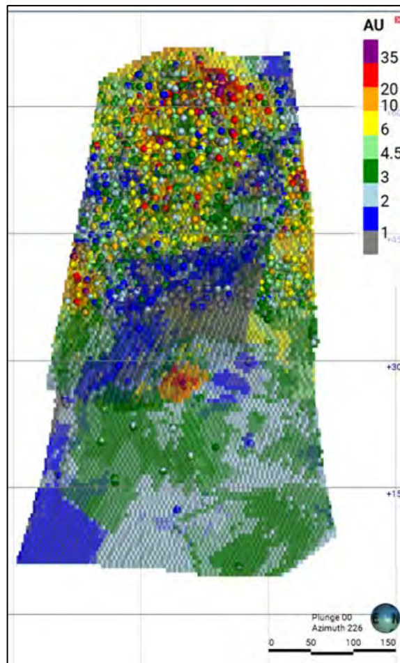
Figure 14-7: MOS Modeled Grades and Composited Drill Hole Samples (Au, g/t) (Eldorado, 2023)
