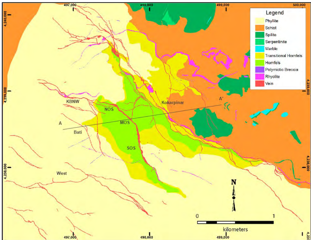
Figure 7-2: Geological Map of the Efemçukuru Deposit (from Eldorado, 2023)
