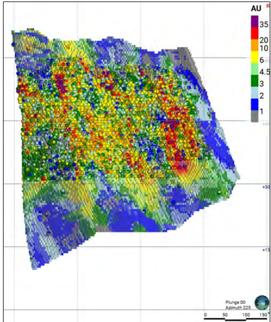
Figure 14-8: NOS Modeled Grades and Composited Drill Hole Samples (Au, g/t) (Eldorado, 2023)
