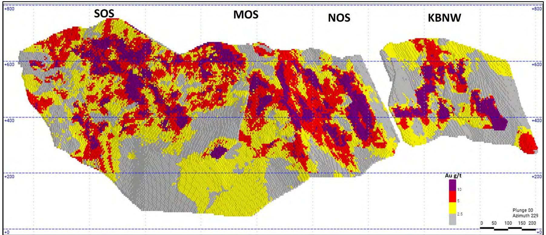
Figure 8-1: Longitudinal Projection of the Mineral Resource Block Model, Illustrating Gold Distribution and High-Grade Shoots at Kestanebeleni (Eldorado, 2023)
