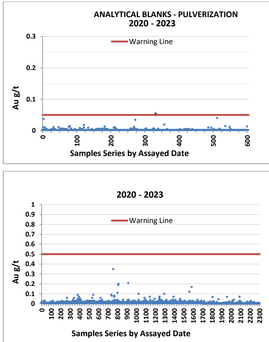
Figure 11-2: Efemçukuru Blank Data – 2020-2023 Drill Programs
