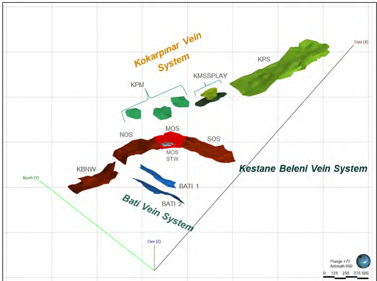
Figure 14-1: Kestanebeleni, Kokarpınar and Batı System Modeling Domains (Eldorado, 2023)
