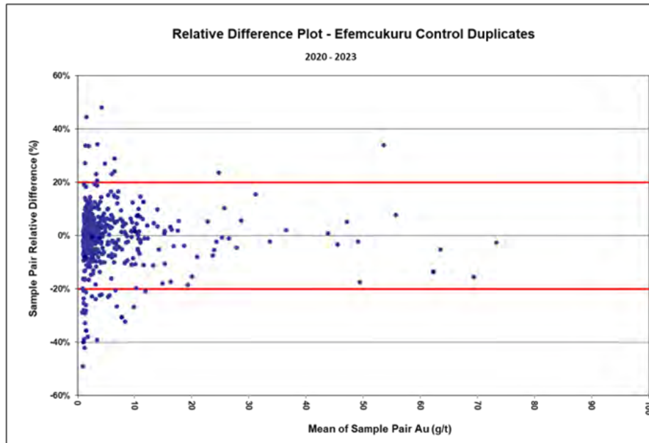
Figure 11-3: Relative Difference Chart, Efemçukuru 2020-2023 Duplicate Data
