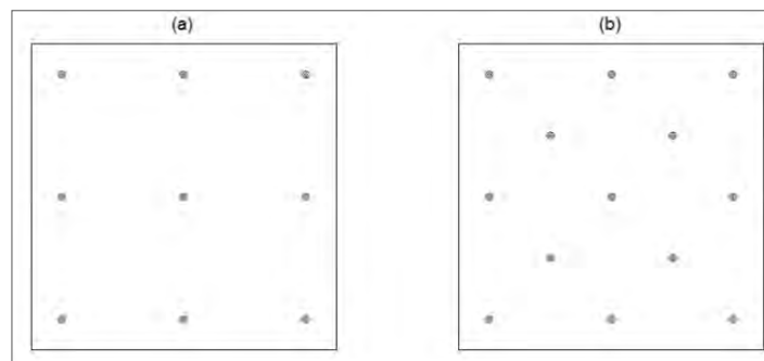
Figure 10-4: Infill Drilling Pattern a) 10 m × 10 m grid b) five dice pattern
