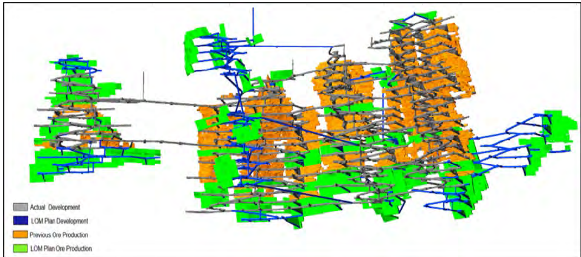
Figure 16-8: Current and LOM Plan Mine Development
