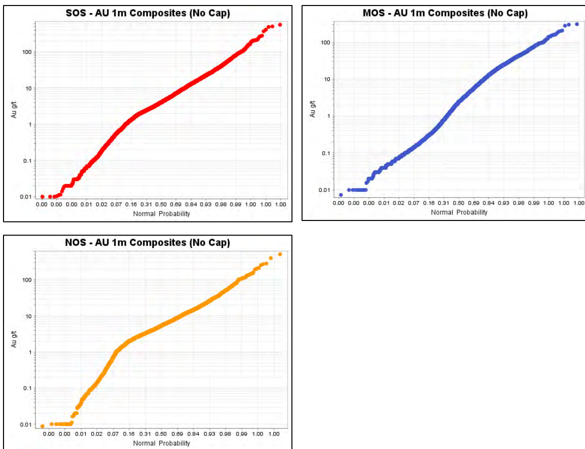
Figure 14-4: Cumulative Probability Plots, Kestanebeleni Vein System
