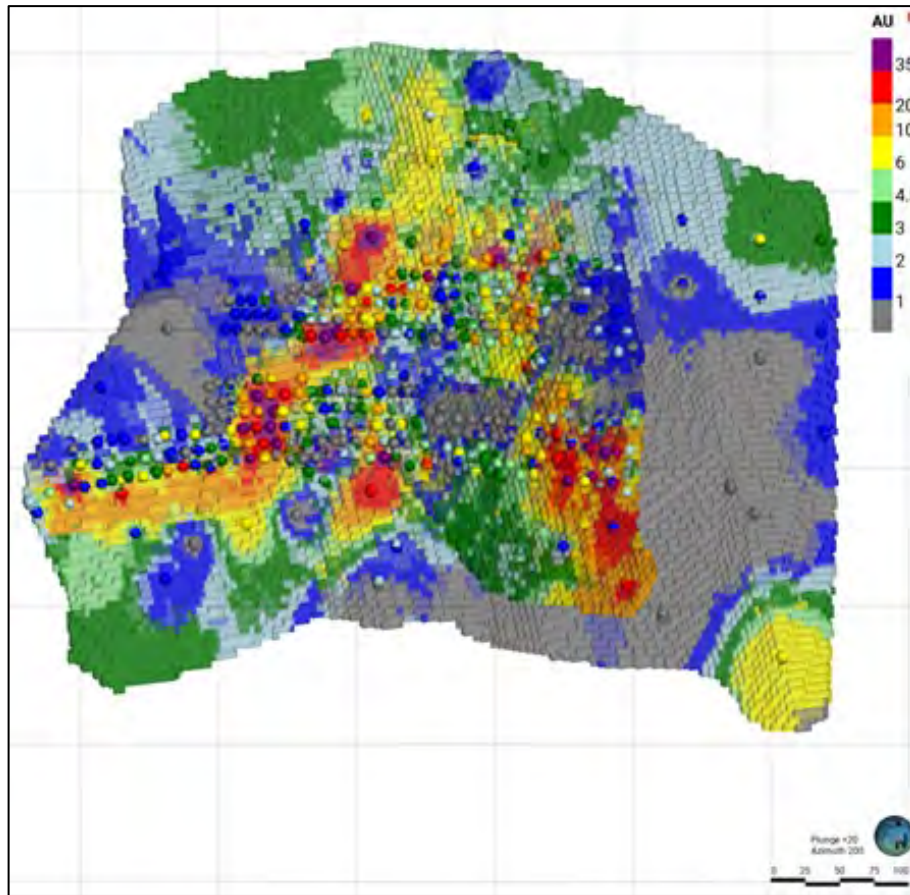
Figure 14-9: KBNW Modeled Grades and Composited Drill Hole Samples (Eldorado, 2023)
