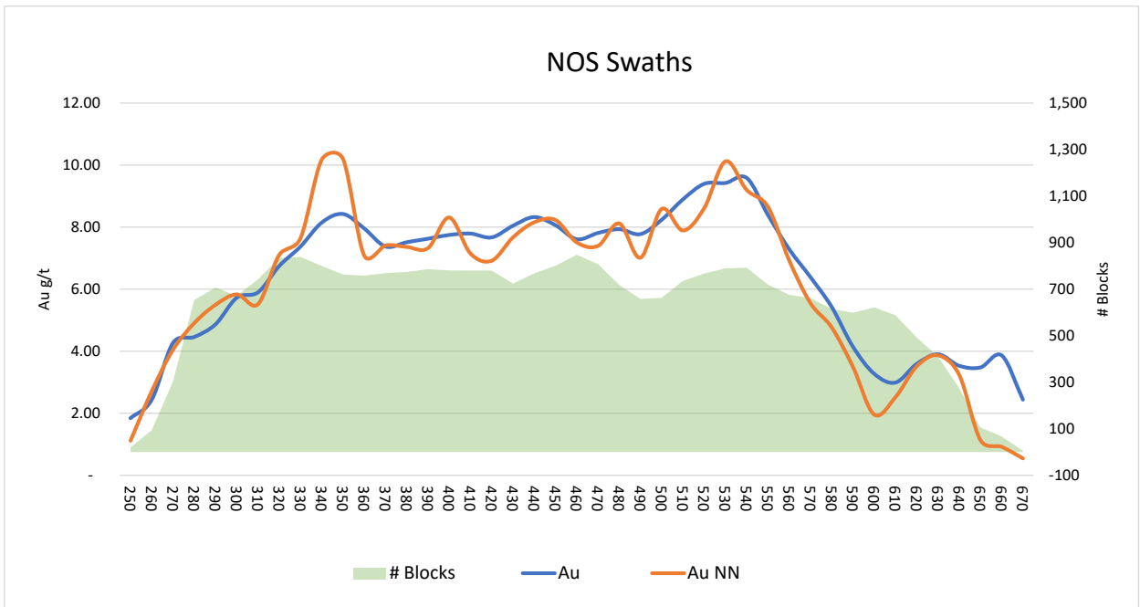
Figure 14-14: Model Trend Plot showing 10 m Binned Averages along Elevations for OK and NN Gold Grade Estimates, NOS Domain
