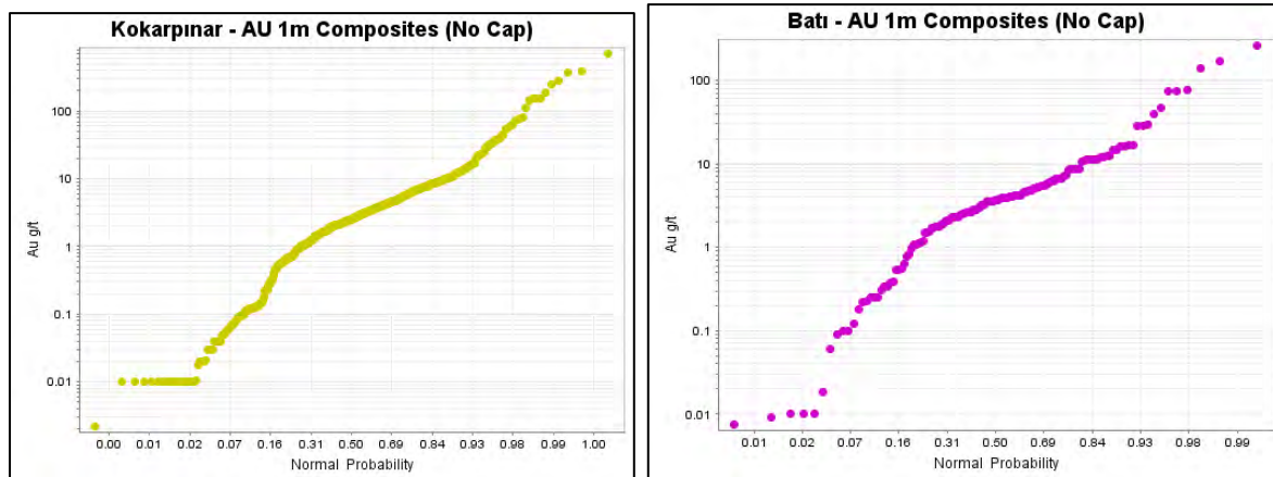
Figure 14-5: Cumulative Probability Plots, Kokarpınar and Batı Systems
