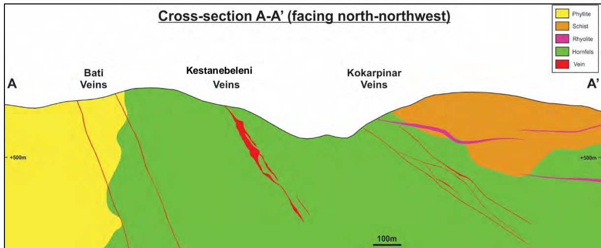
Figure 7-3: Geological cross section through the Bati, Kestanebeleni (MOS) and Kokarpinar Veins (from Eldorado, 2023)
