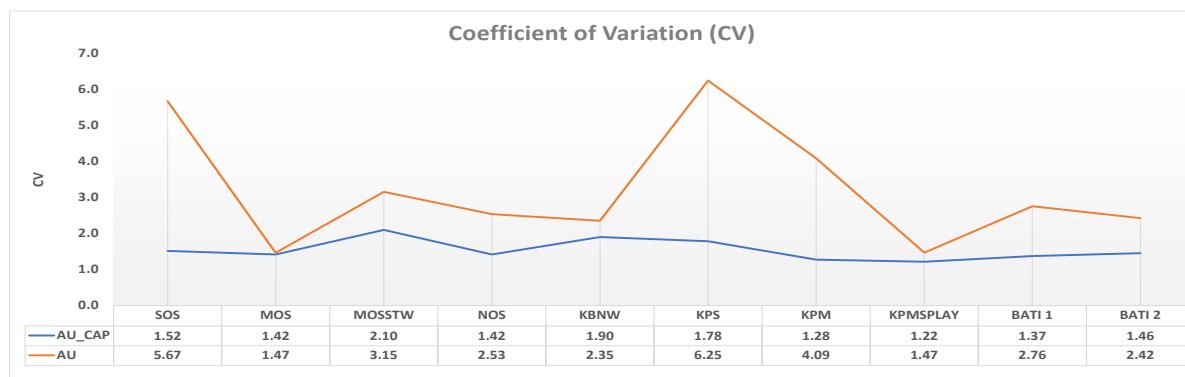
Figure 14-3: Average Coefficient of Variation for Capped and Uncapped Data a by Domain
