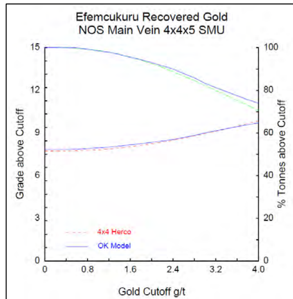
Figure 14-17: HERCO plot, NOS domain
