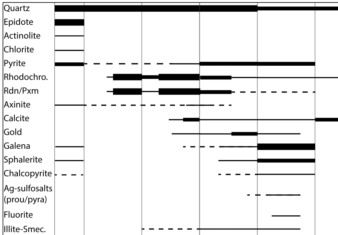
Figure 8-2: Mineral Paragenesis at Efemçukuru (Boucher, 2016)
