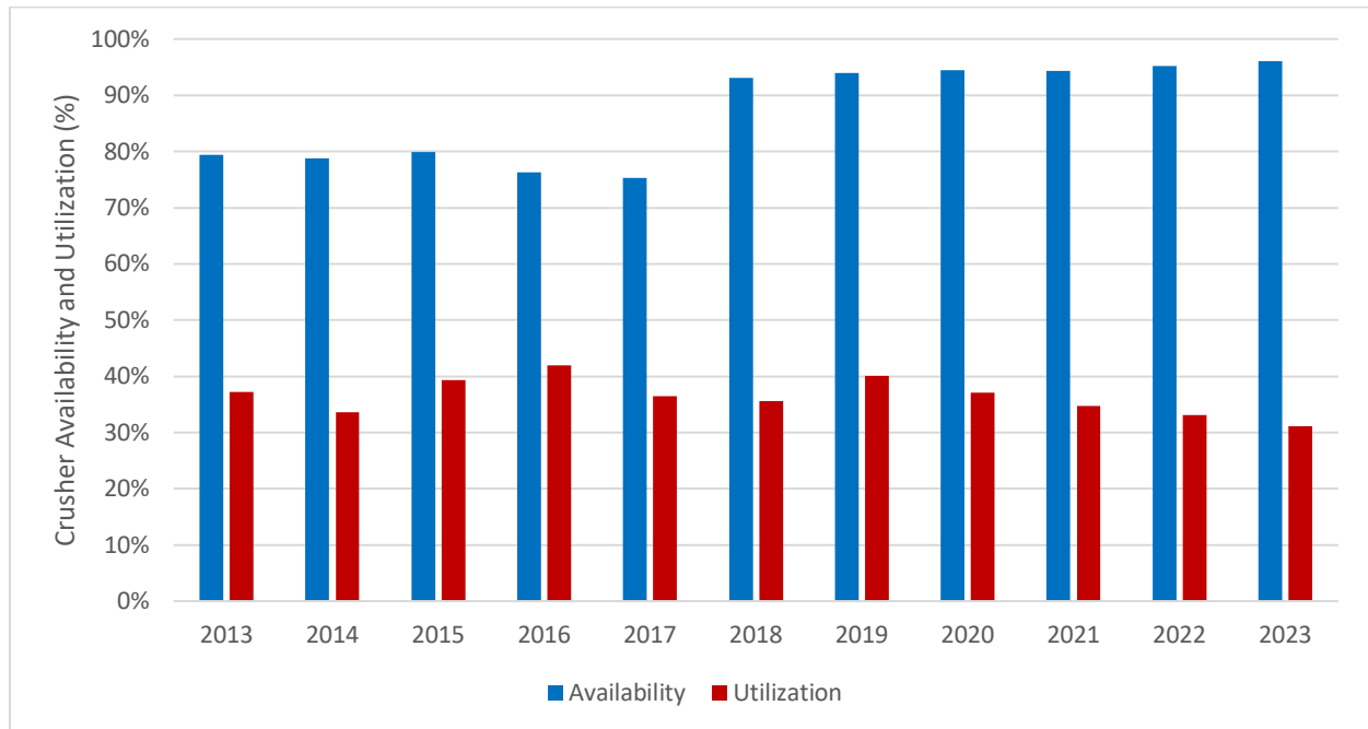
Figure 17-2: Crusher availability and utilization between 2013 and 2023
