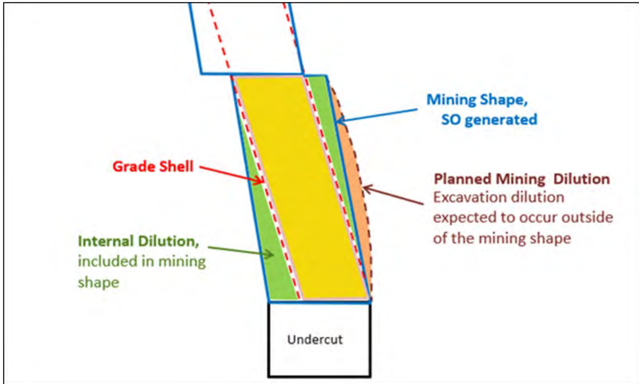
Figure 15-1: Schematic Showing Dilution Encapsulated by SO Mining Shape
