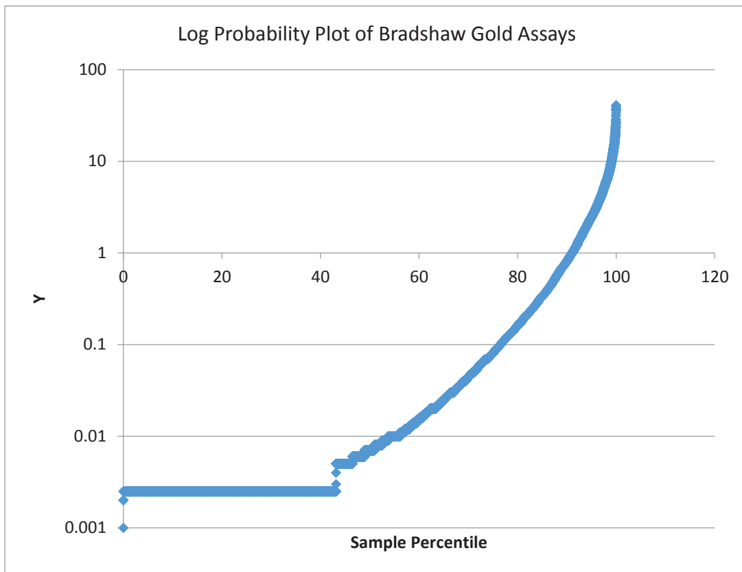
Figure 14.3: Log Probability Plot of Bradshaw Gold Assays
