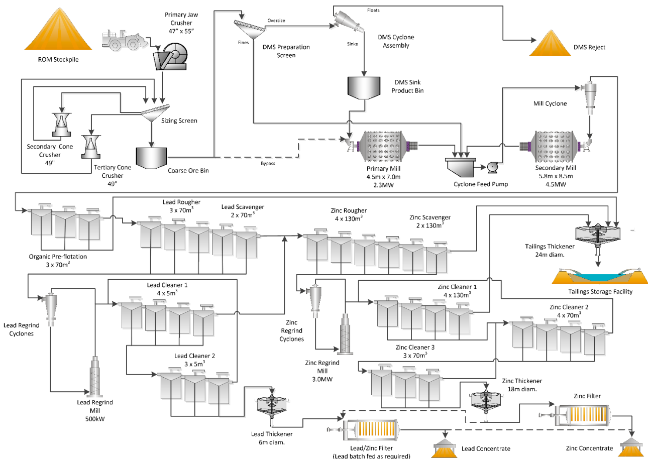
Figure 7 – Updated Process Flow Sheet
