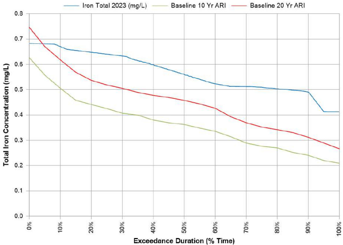
Chart 45 Total Iron Performance Indicator Woronora Reservoir 2023
