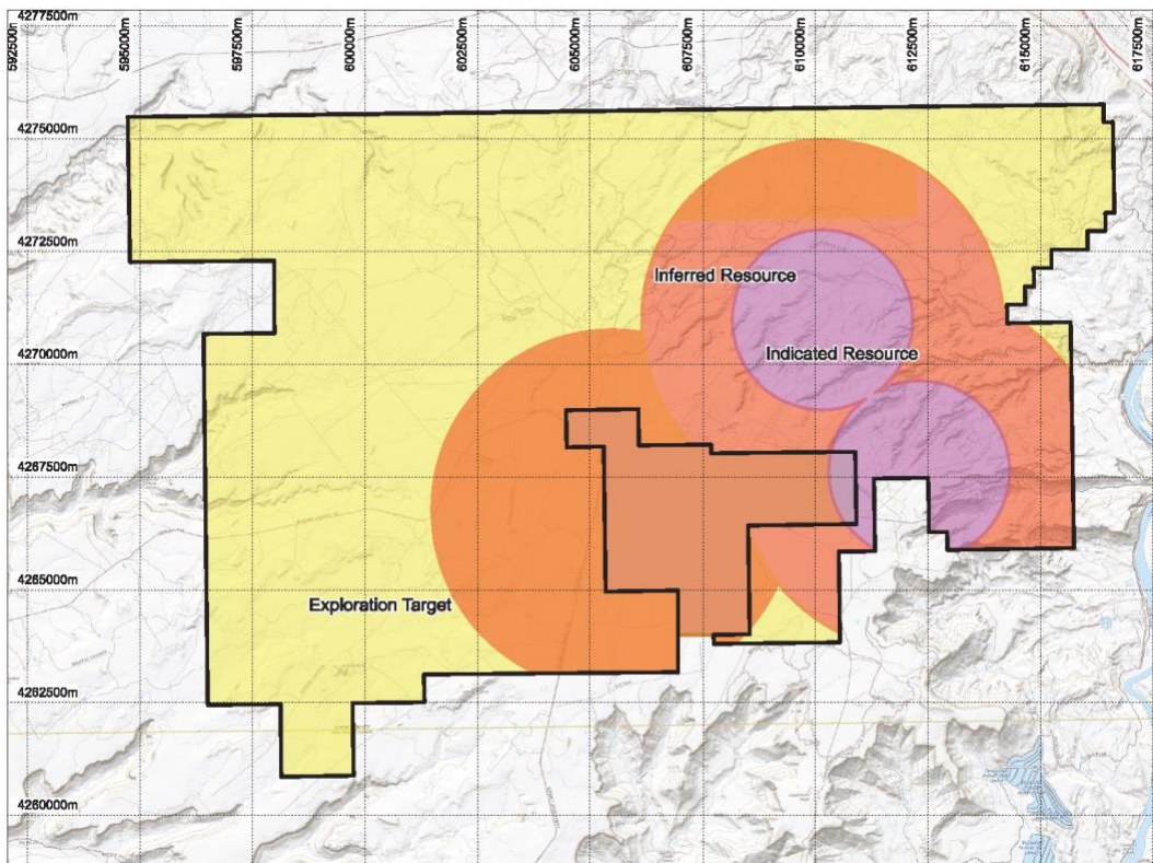
Figure 13: The Mississippi Resource Classification.
