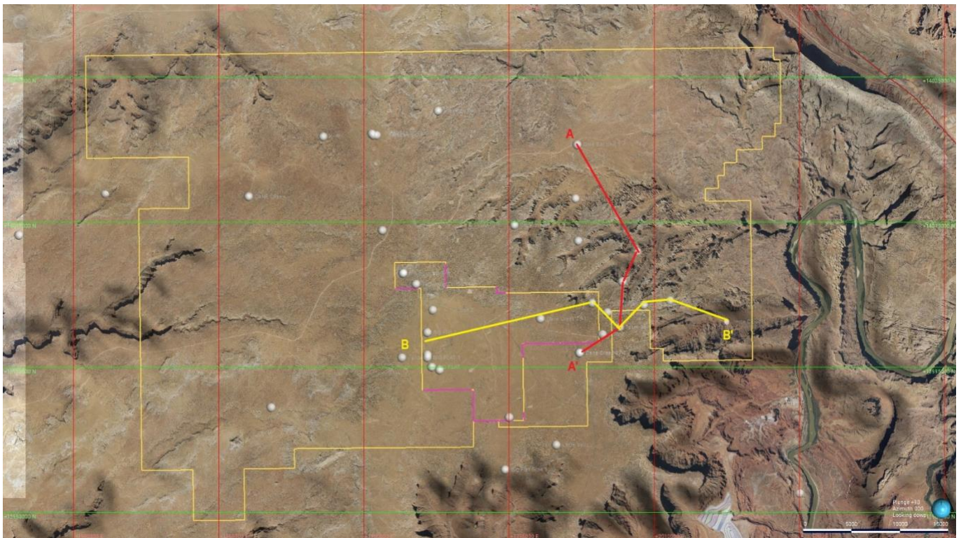
Figure 4: Plan view showing claim area, topography and section lines.
