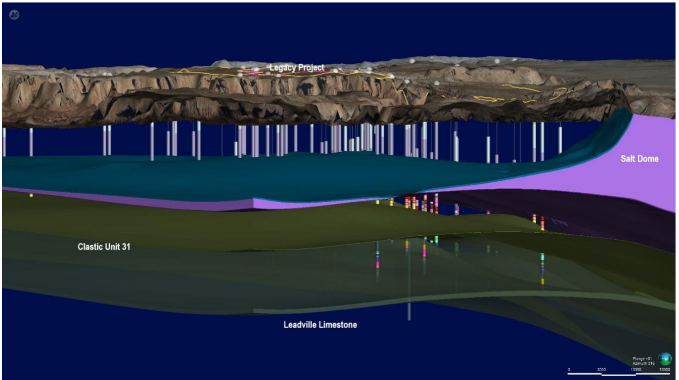
Figure 5: View showing surface topography, wells and modelled clastic zones.
