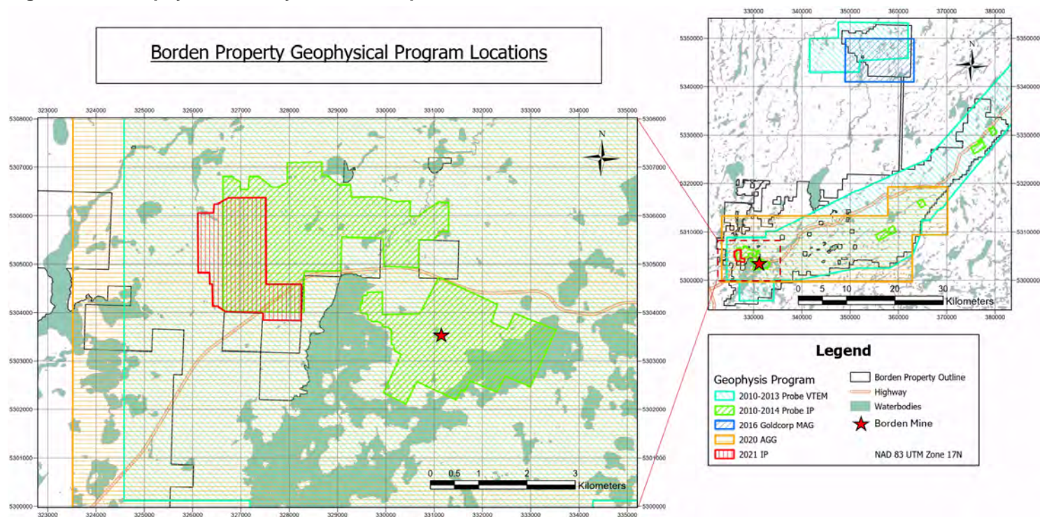
Figure 9-12: Geophysical Survey Location Map, Borden Area
