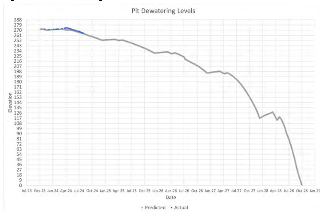
Figure 16-8: Pit Dewatering Forecasts, Pamour
