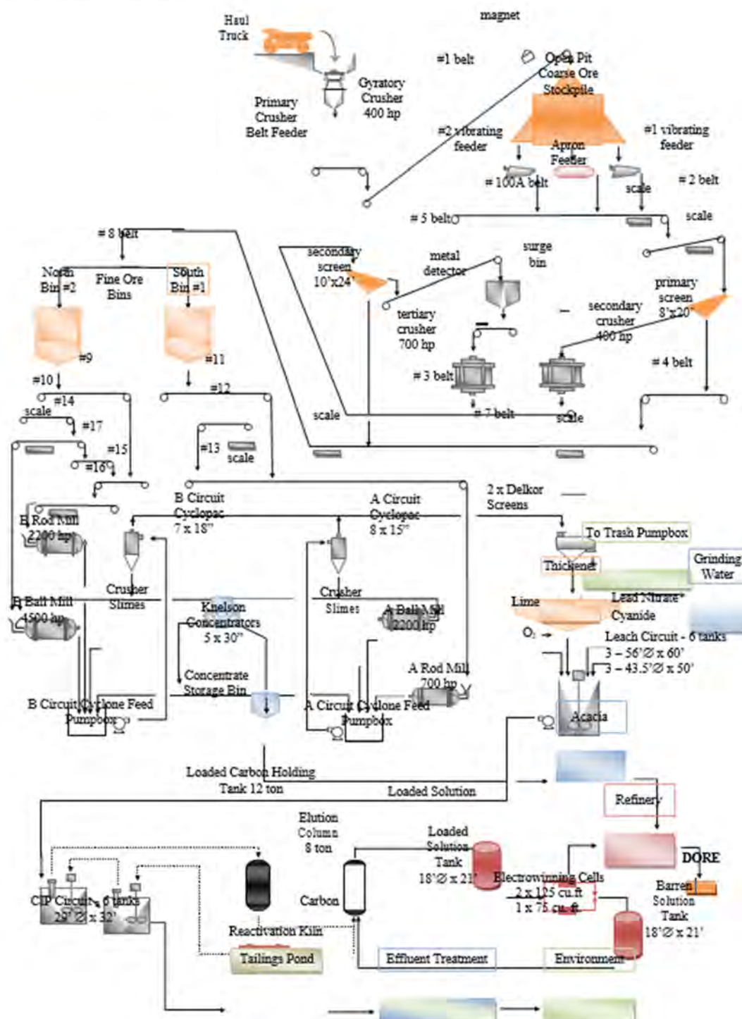
Figure 17-1: Process Flowsheet
