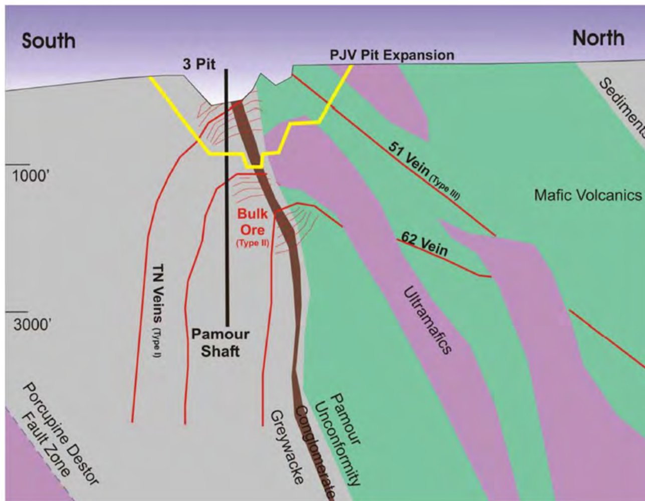
Figure 7-23: Example Cross-Section, Pamour
