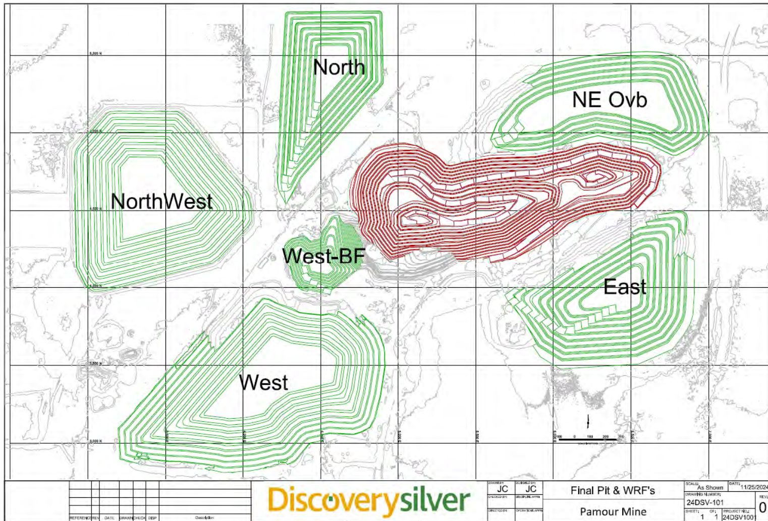
Figure 16-9: Waste Rock Storage Facilities, Pamour
