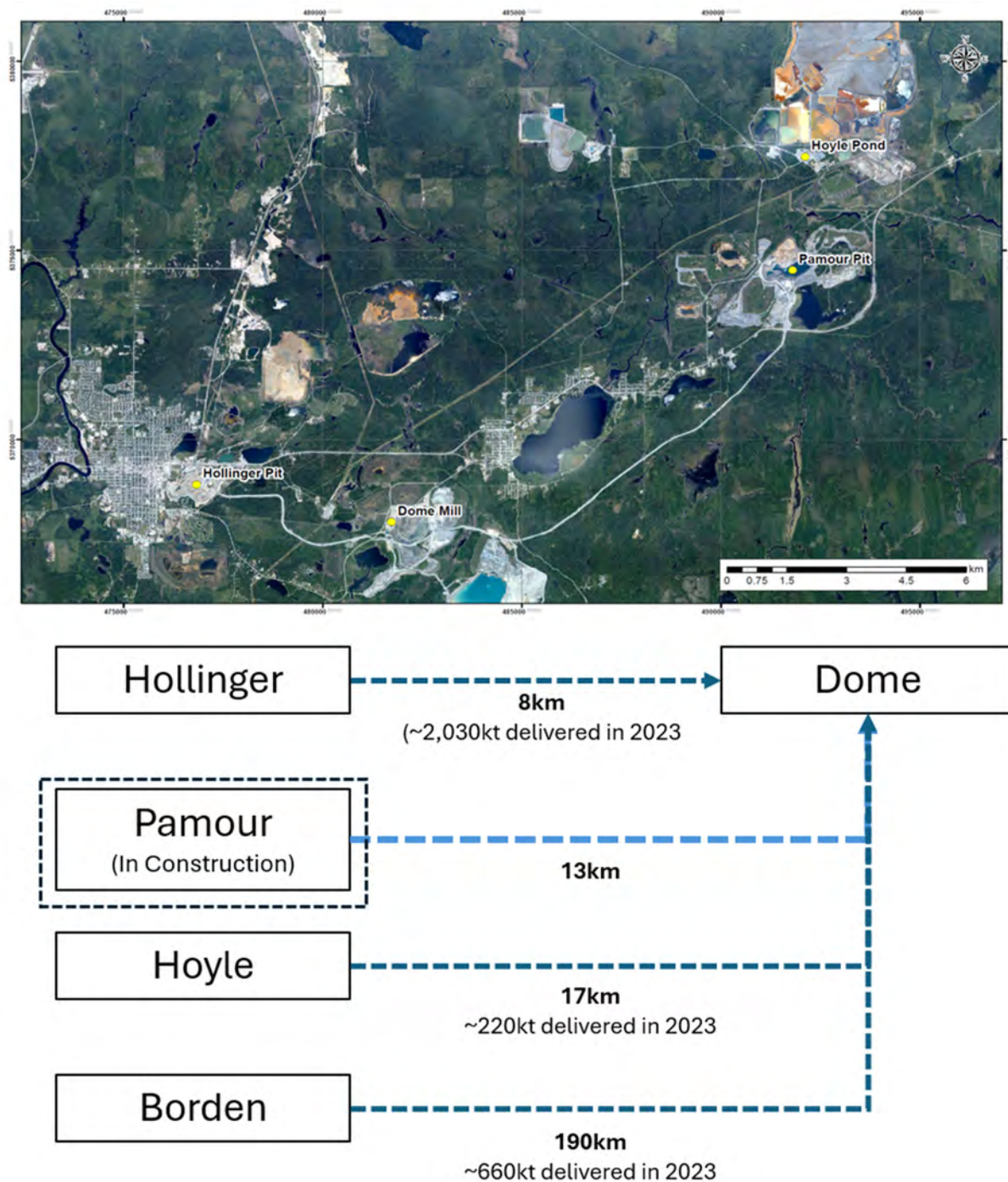
Figure 16-1: Process Plant Feed Sources
