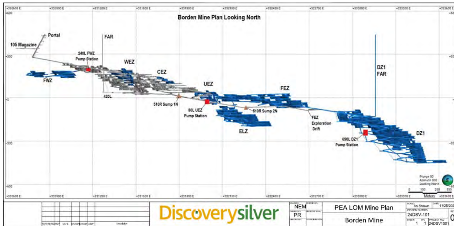
Figure 16-2: Mine Cross-Section, Borden
