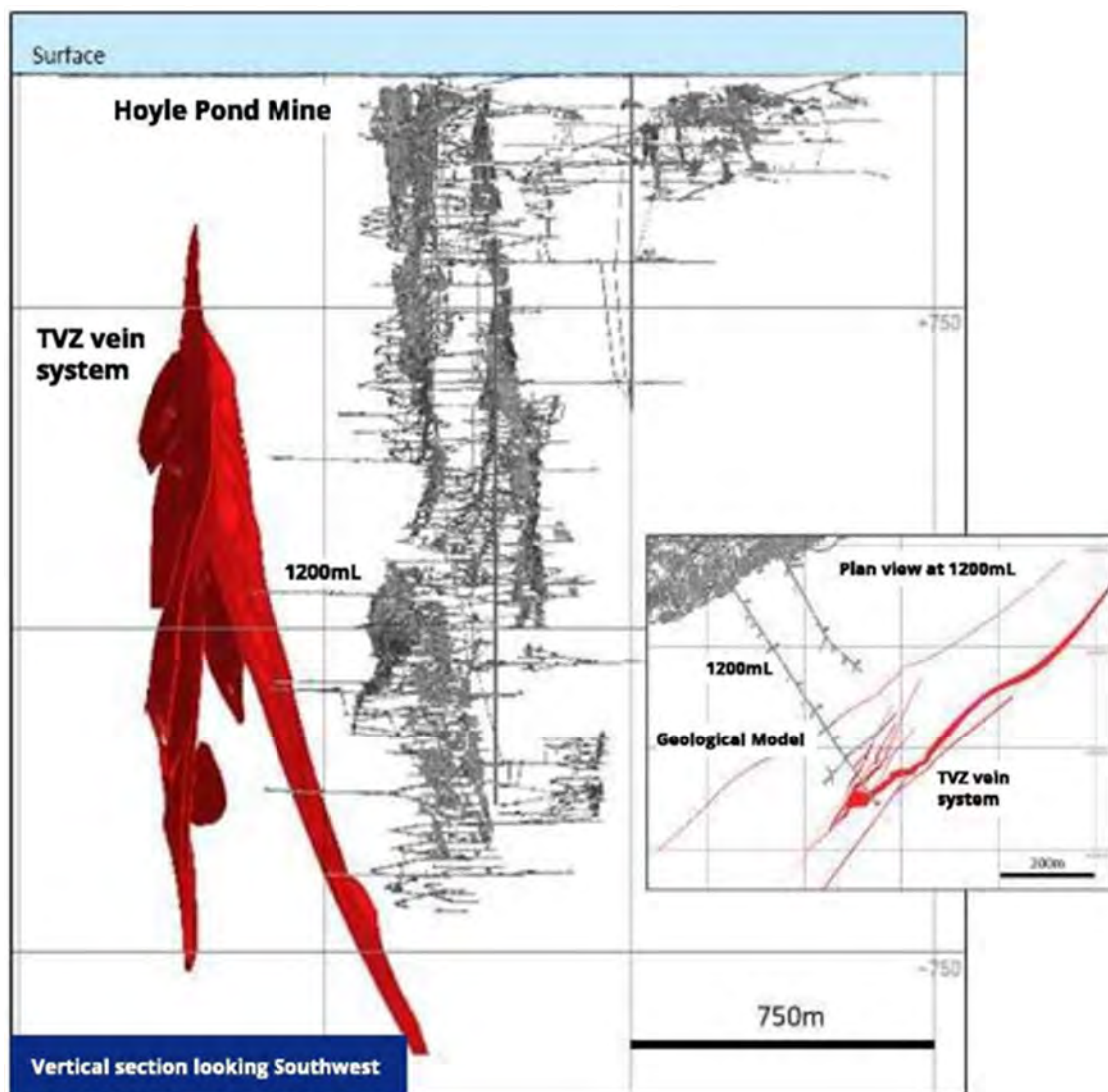
Figure 9-18: TVZ Zone Prospective Area, Hoyle Pond
