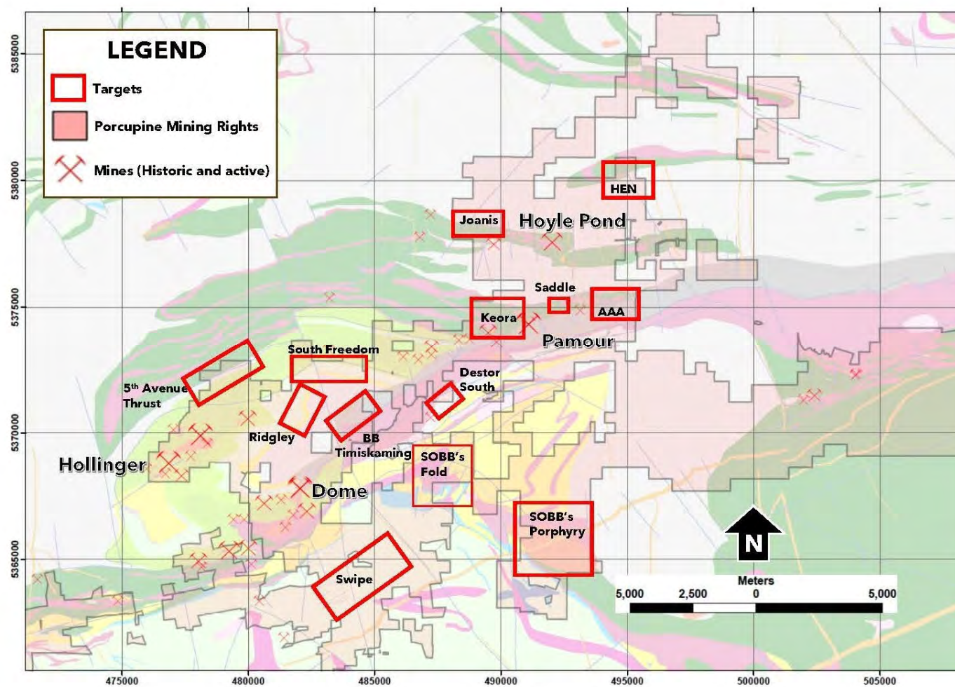
Figure 9-13: Prospectivity Targeting Map, Timmins Area
