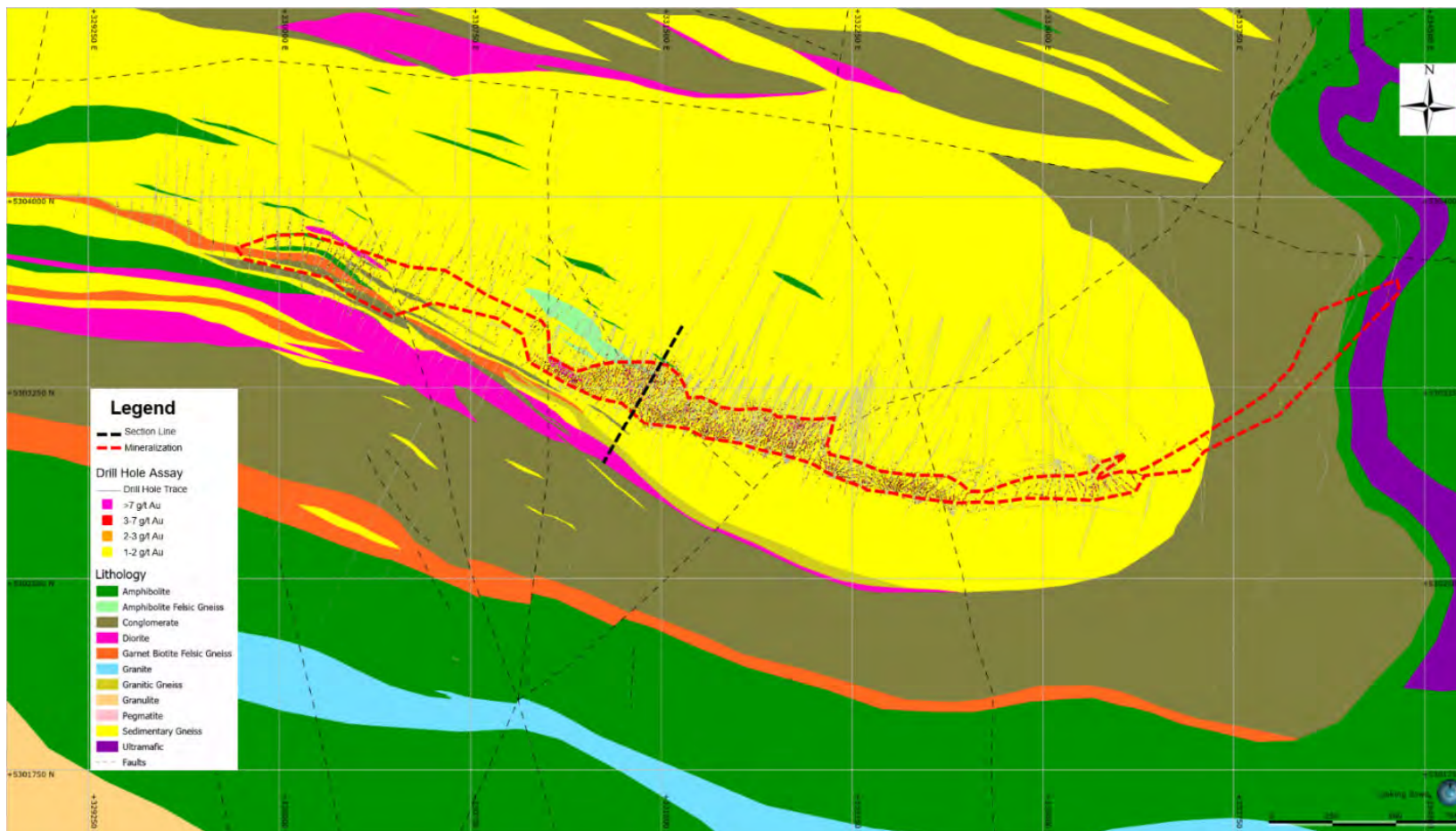
Figure 7-10: Geology Plan, Borden
