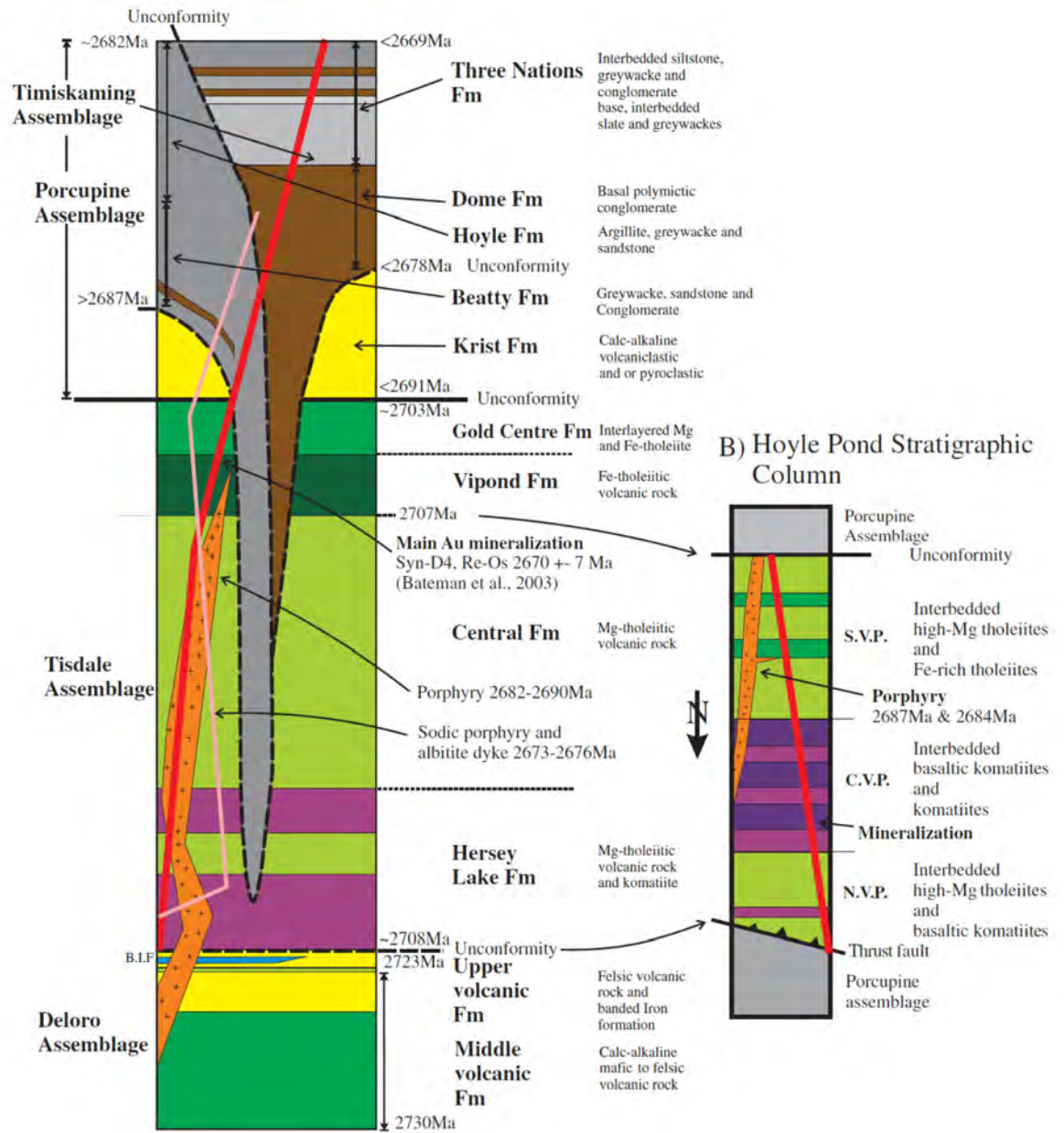
Figure 7-6: Stratigraphic Column, Timmins Area
