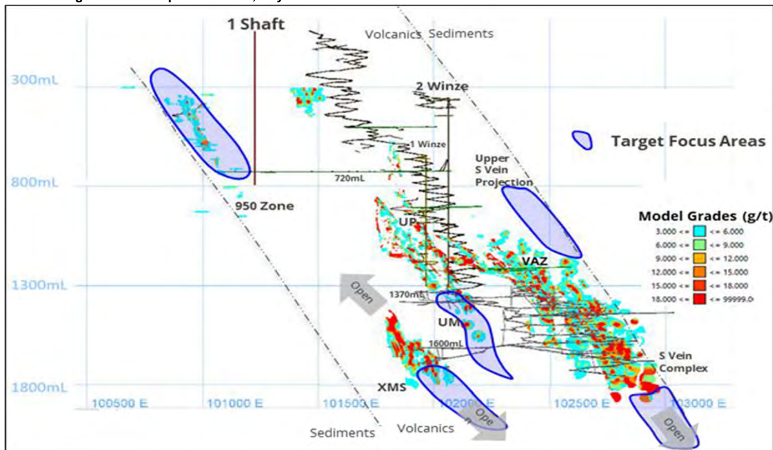
Figure 9-17: Prospective Areas, Hoyle Pond
