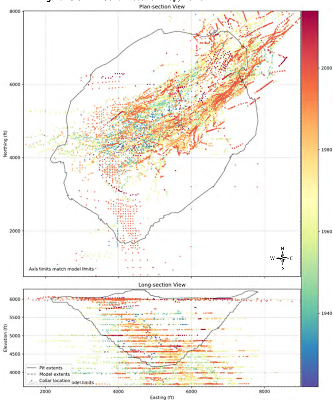
Figure 10-6: Drill Collar Location Map, Dome
