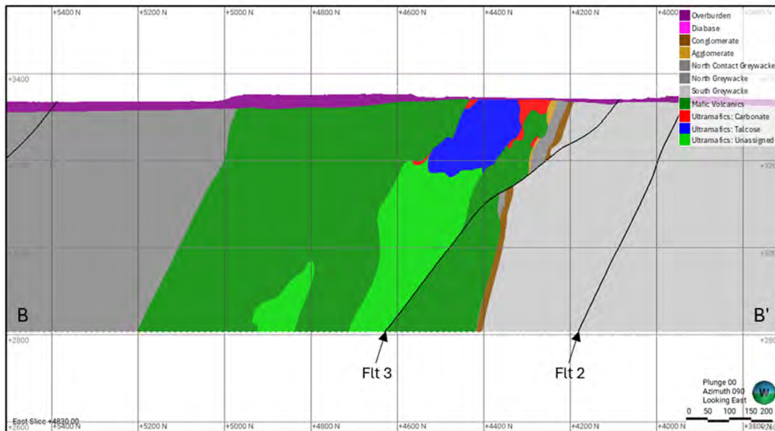
Figure 14-12: Example Cross-Section, Geology Model, Pamour
