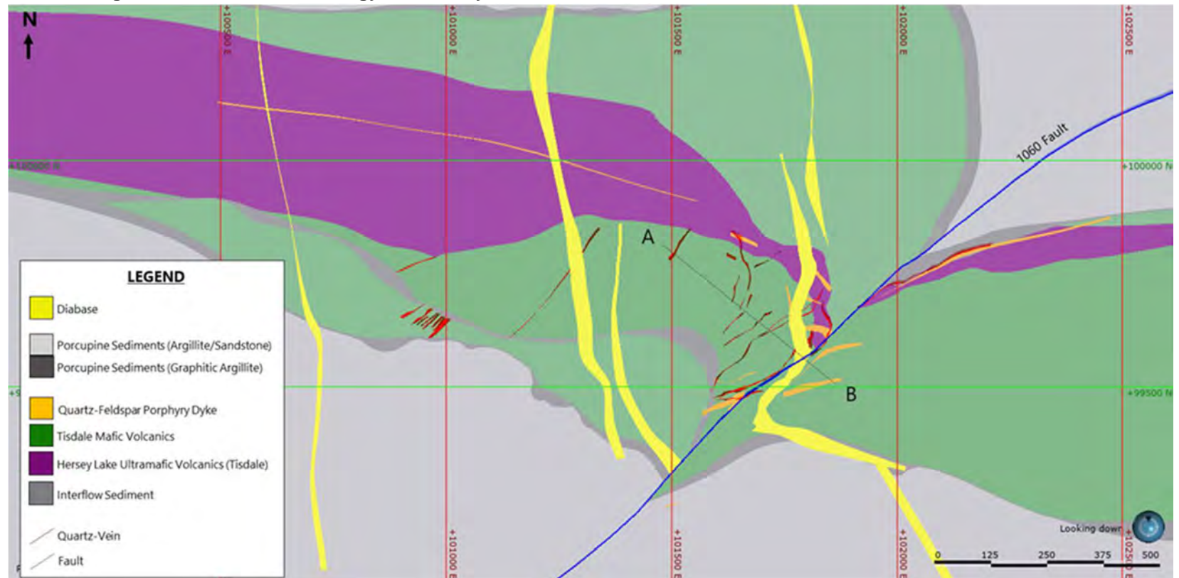
Figure 14-8: Plan View, Geology Model, Hoyle Pond
