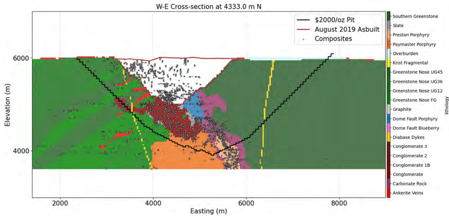
Figure 14-4: Example, Dome West–East Section Displaying Flagged Lithologies
