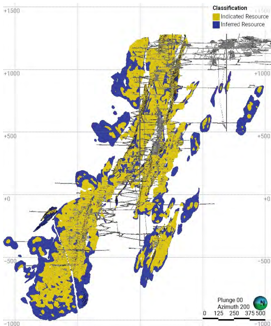
Figure 14-10: Confidence Classification, Hoyle Pond
