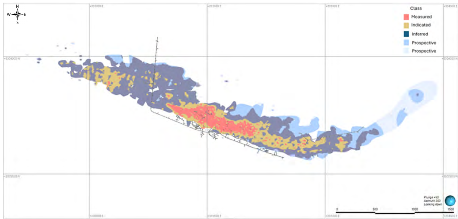
Figure 9-16: Prospective Areas, Borden
