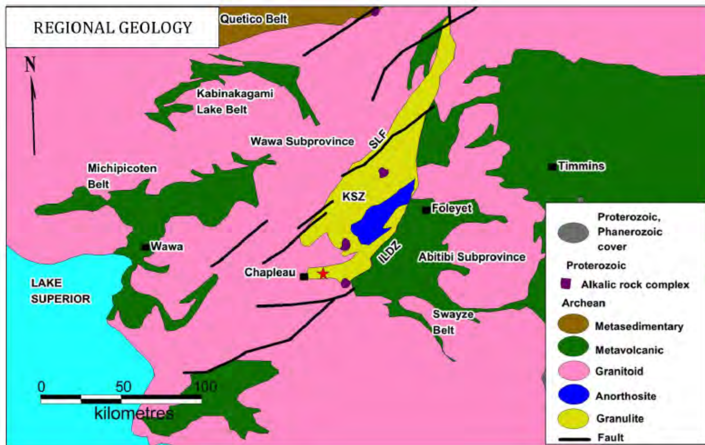
Figure 7-3: Regional Geology Plan, Kapuskasing Structural Zone
