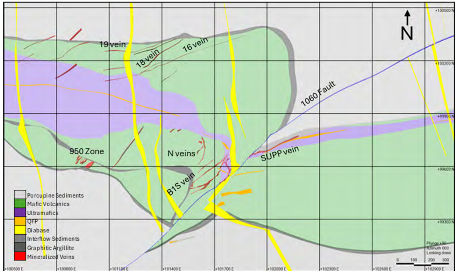
Figure 7-19: Vein System and Geology Plan, Hoyle Pond
