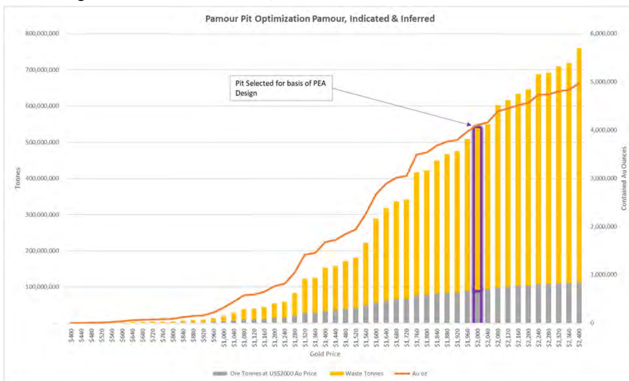
Figure 16-5: Pit Shell Evaluation, Pamour
