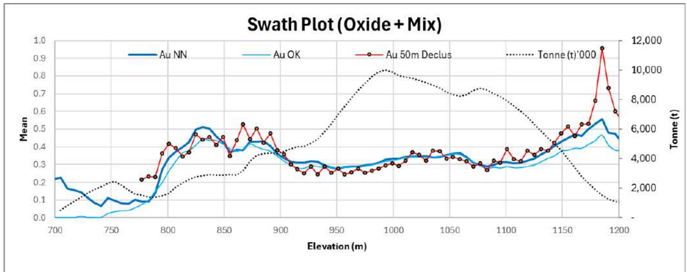
Figure 14-24: Swath Plot Elevation: Drill Hole Grades, OK and NN Grade Estimation
