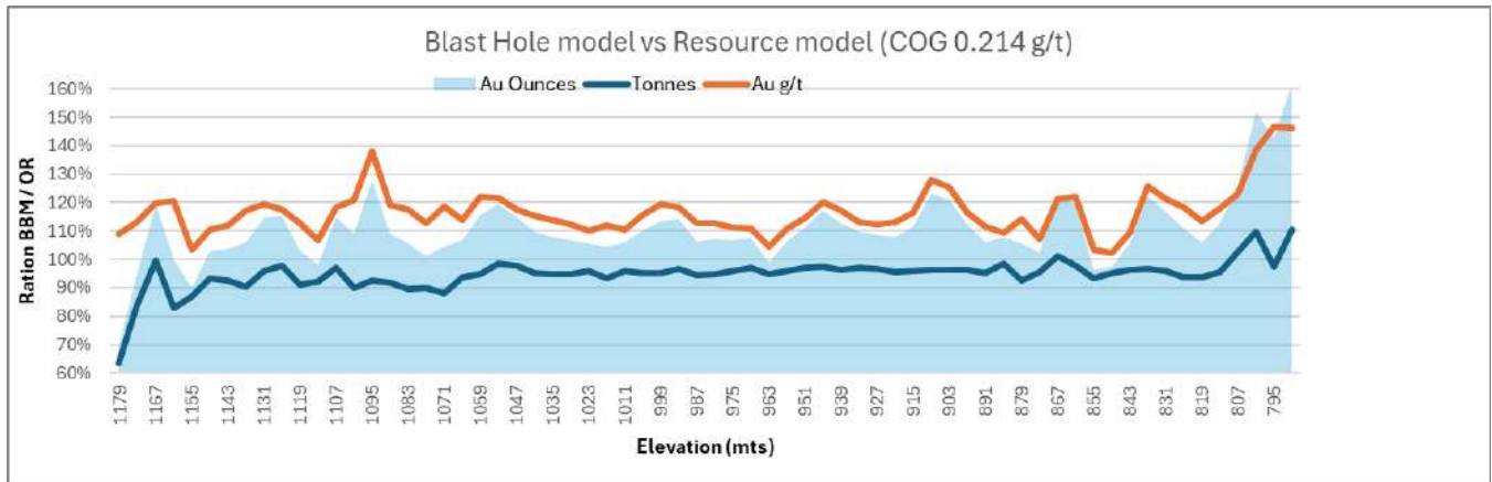
Figure 14-29: Tonnes, Grade, and Contained Metal Comparison between 2024 Resource Model vs. Blast Hole Block Model
