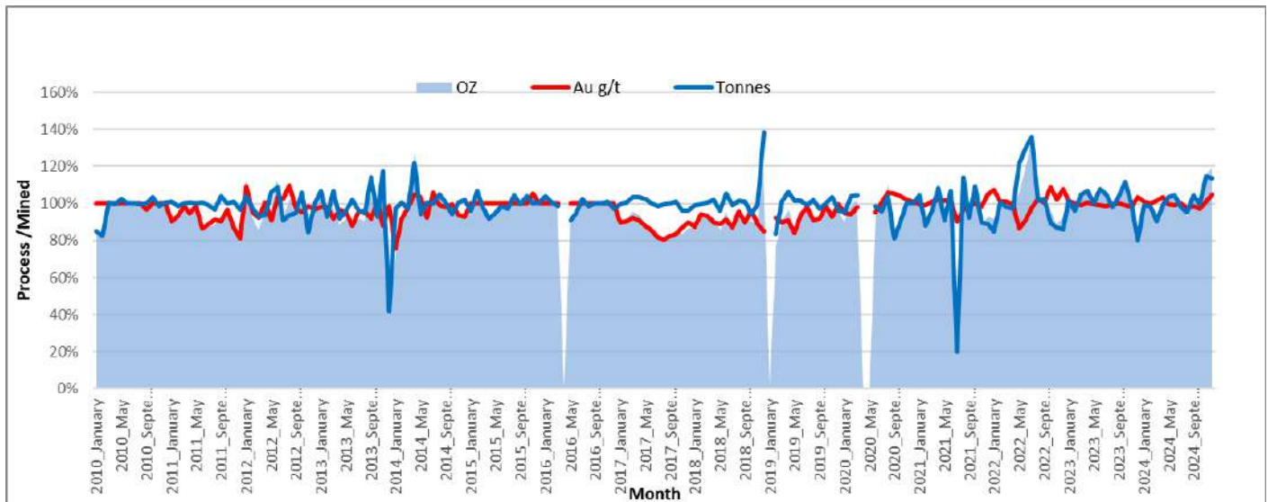
Figure 14-37: Reconciliation Trend from 2010 to 2024 of Process Plant vs. Ore Mined (Tonnes, Gold Grade, and Ounces)
