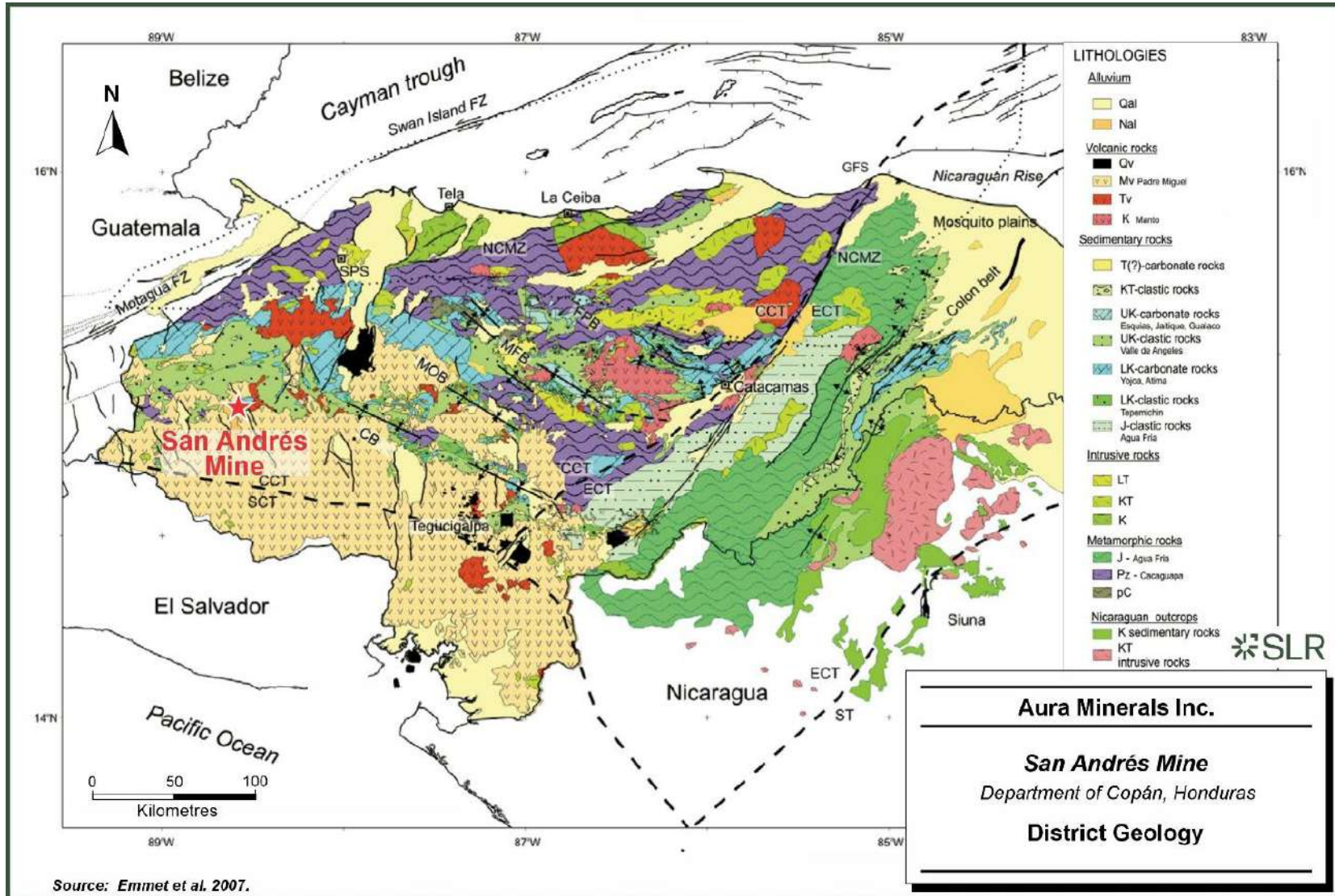
Figure 7-2: District Geology
