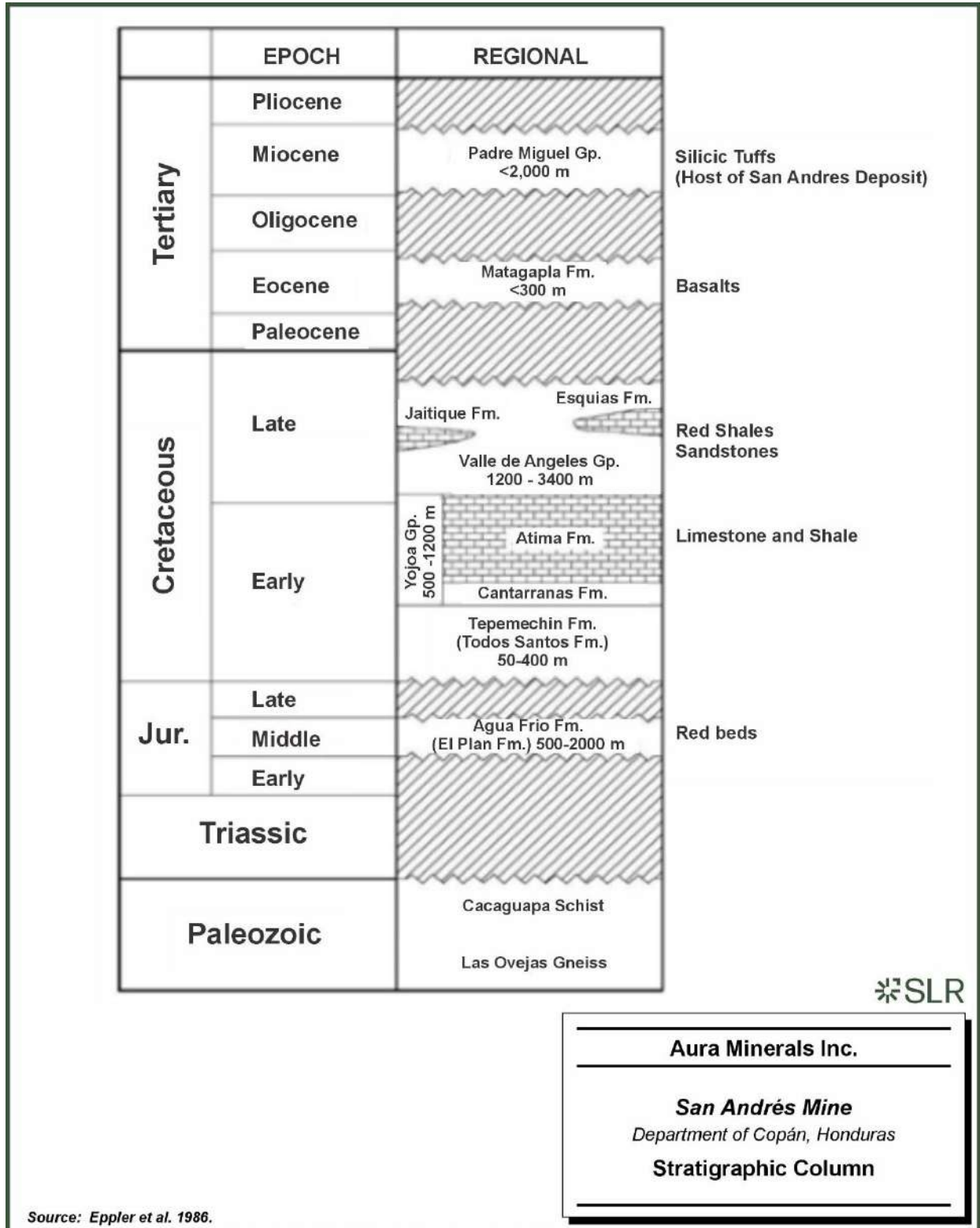
Figure 7-3: Stratigraphic Column
