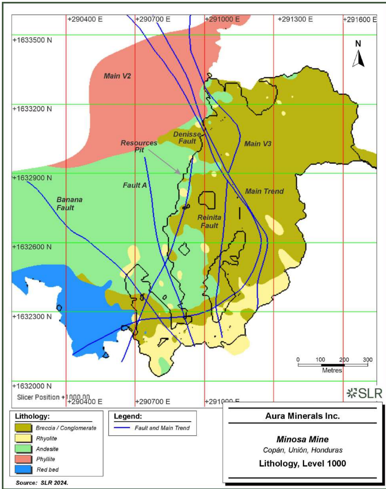
Figure 14-3: Lithology, Level 1000
