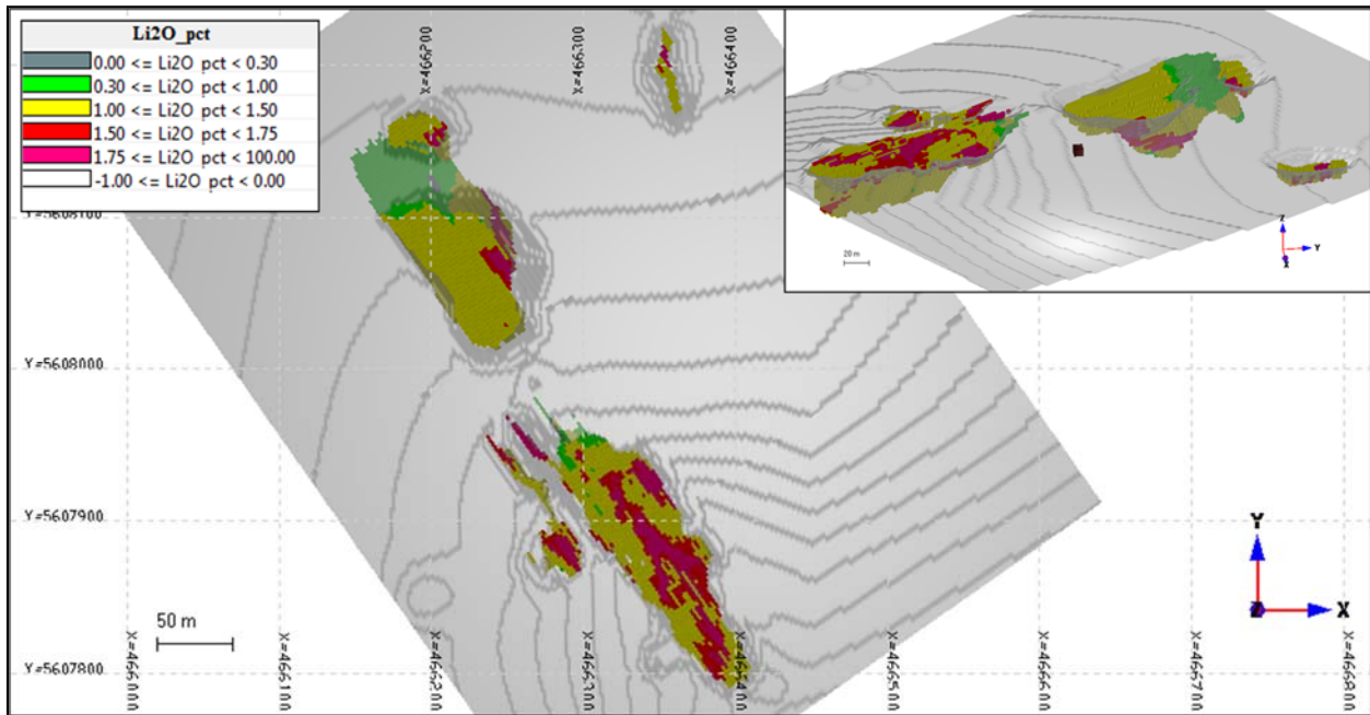
Figure 61 – Pit outline and resource block model.
