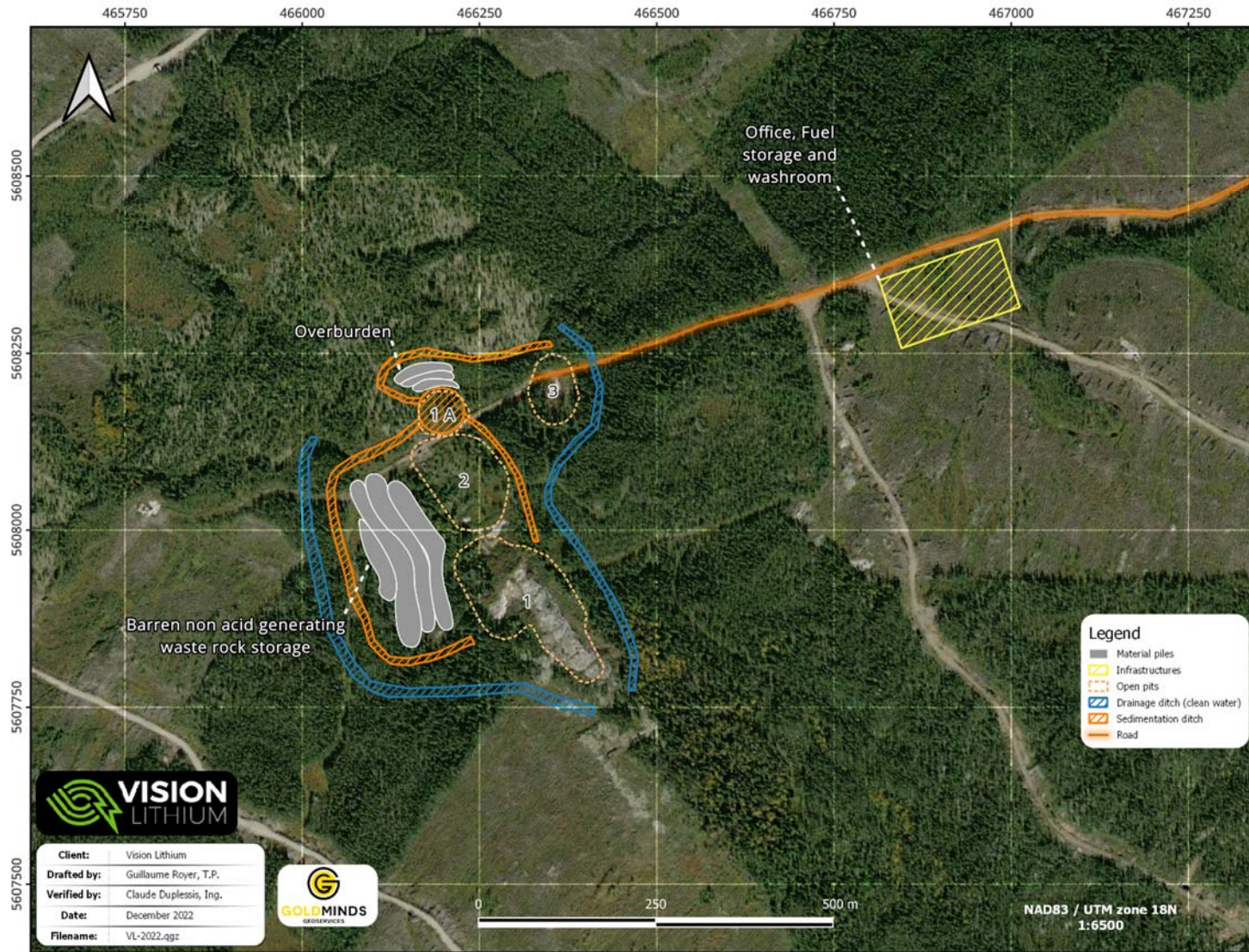
Figure 64 - Site surface plan.
