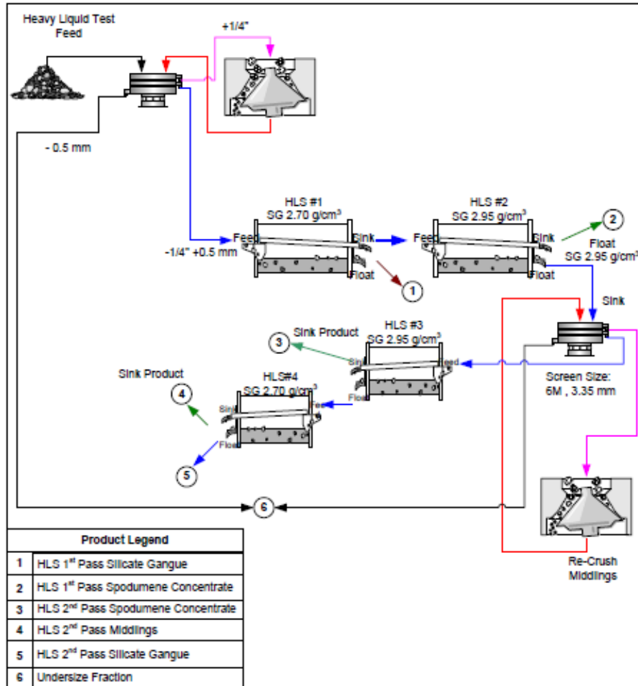
Figure 38: HLS test flowsheet performed on the drill cores
