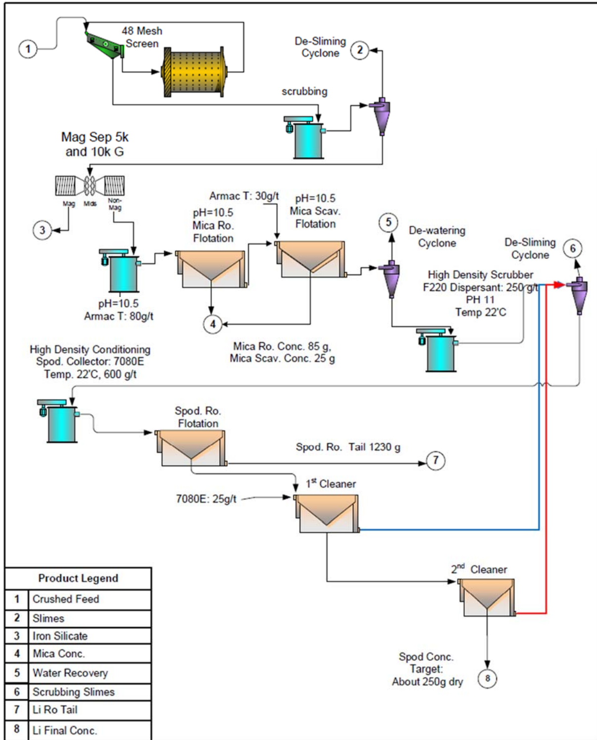
Figure 43 – Locked-Cycle Test Flowsheet (SGS, 2019).
