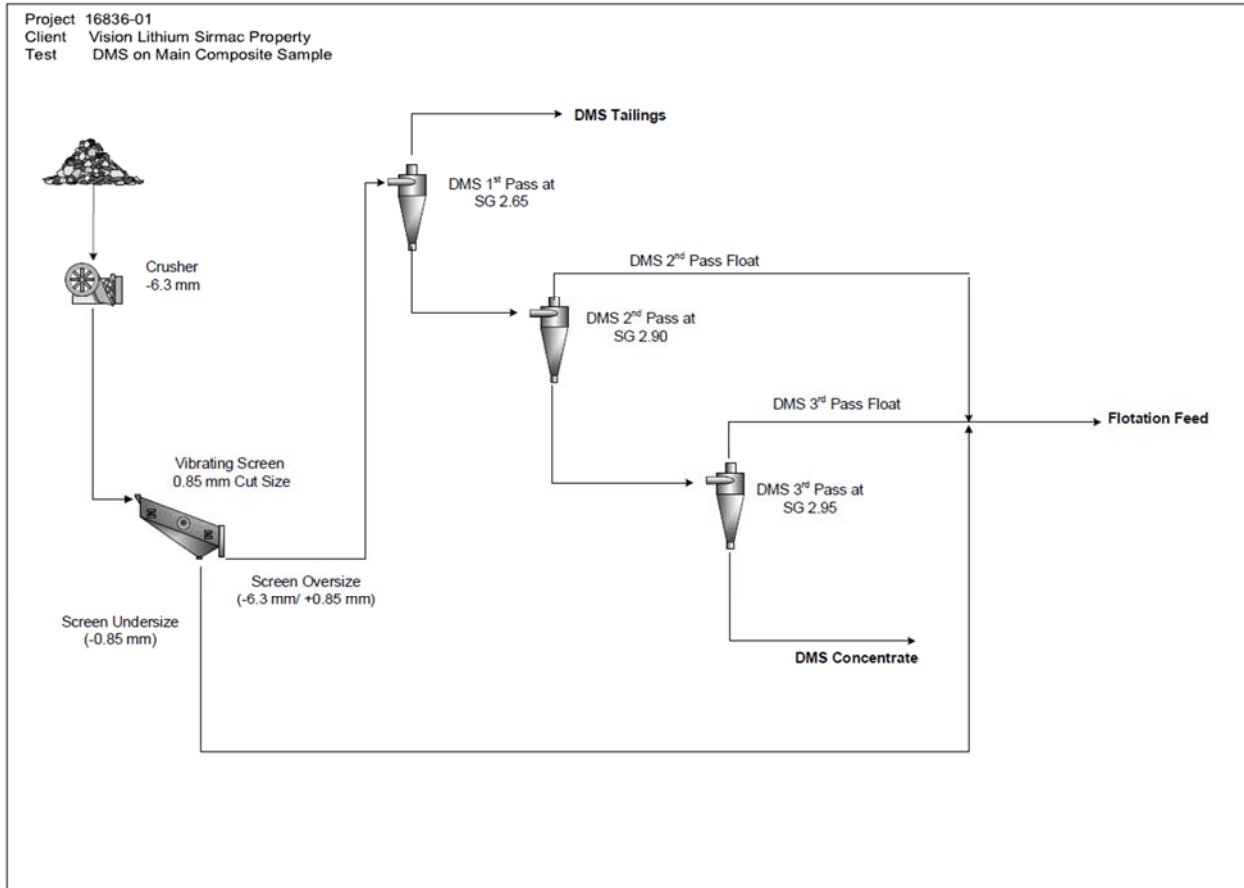
Figure 44 – Final Developed DMS + Flotation Flowsheet for Main Outcrop Composite (Part 1 – DMS; SGS, 2019).
