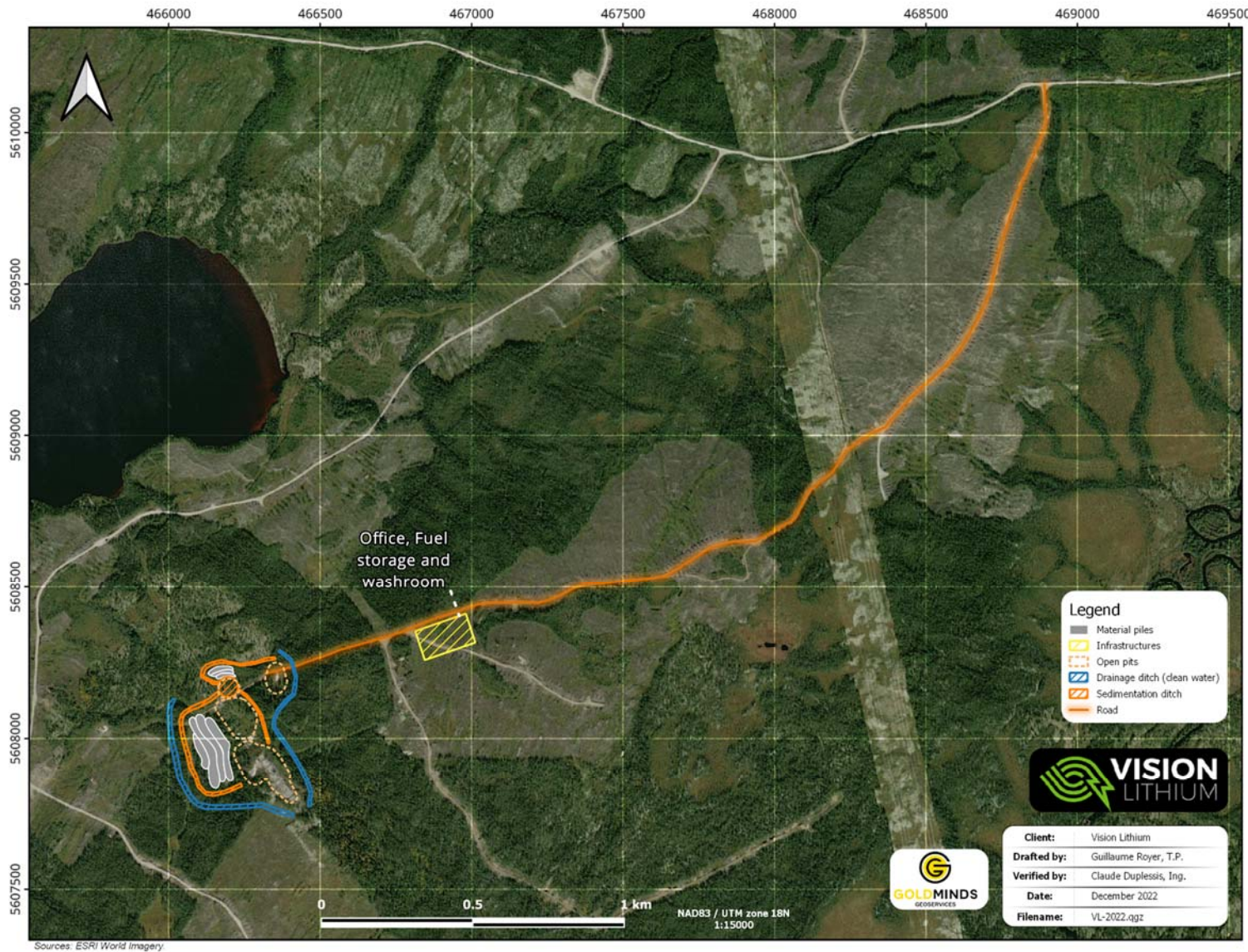
Figure 65 – Site surface plan with access road.
