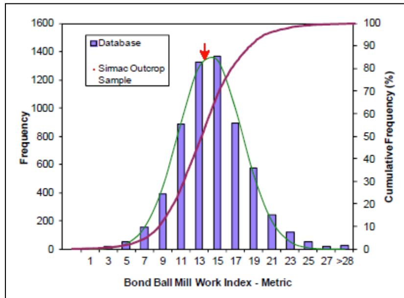
Figure 37: Outcrop composite Bond Ball Mill Work Index comparison to SGS Database
