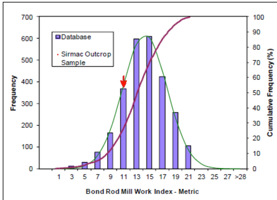
Figure 36: Outcrop composite Bond Rod Mill Work Index comparison to SGS Database
