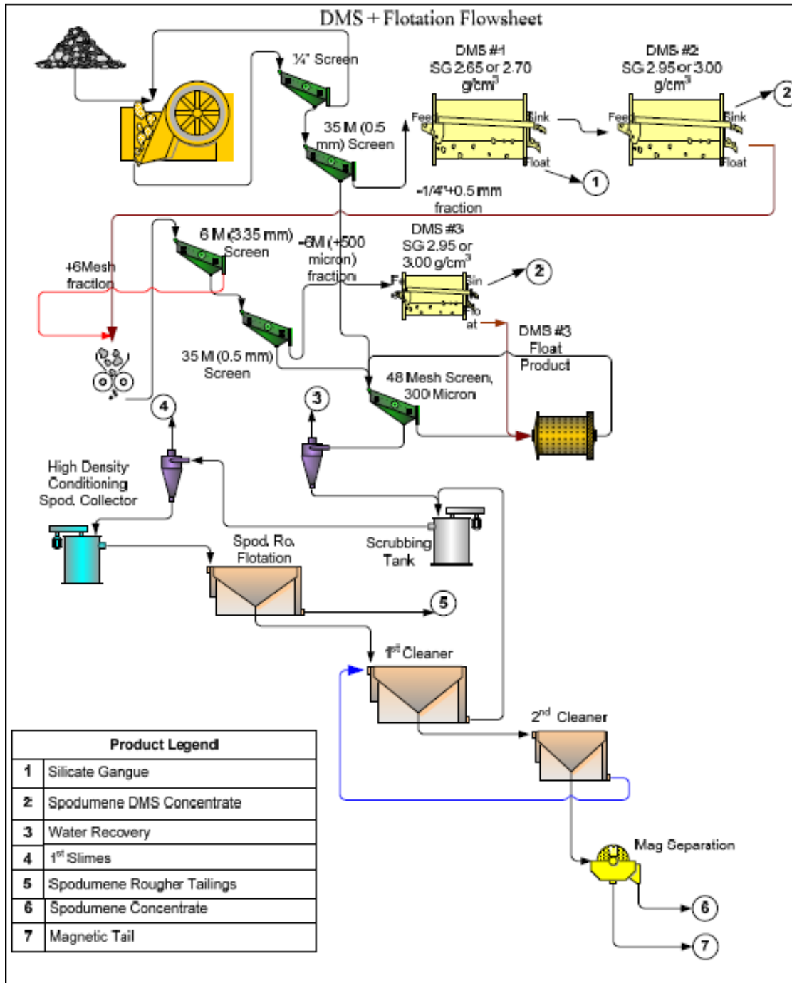
Figure 39: Preliminary flowsheet
