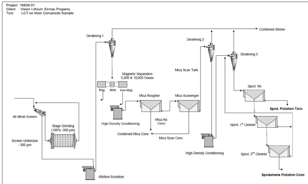
Figure 45 – Final Developed DMS + Flotation Flowsheet for Main Outcrop Composite (Part 2 – Flotation).
