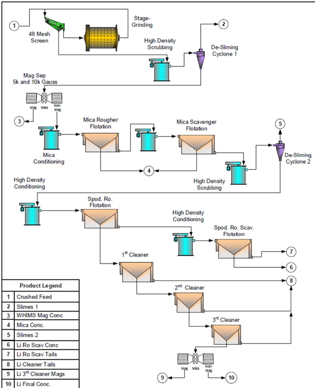
Figure 42 – Optimized Batch Flotation Test Flowsheet (SGS, 2019).
