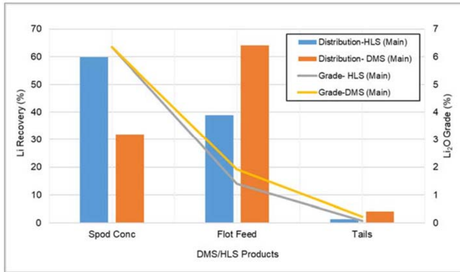
Figure 41 – Comparison of Lithium Department in the HLS Test and the DMS Test (Main Composite).
