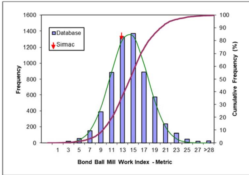
Figure 40: BWI of the Main Composite Flotation Feed Compared to the SGS Database (SGS, 2019).
