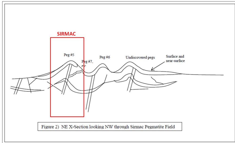
Figure 49 – Schematic interpretation from Pearse, 2010.
