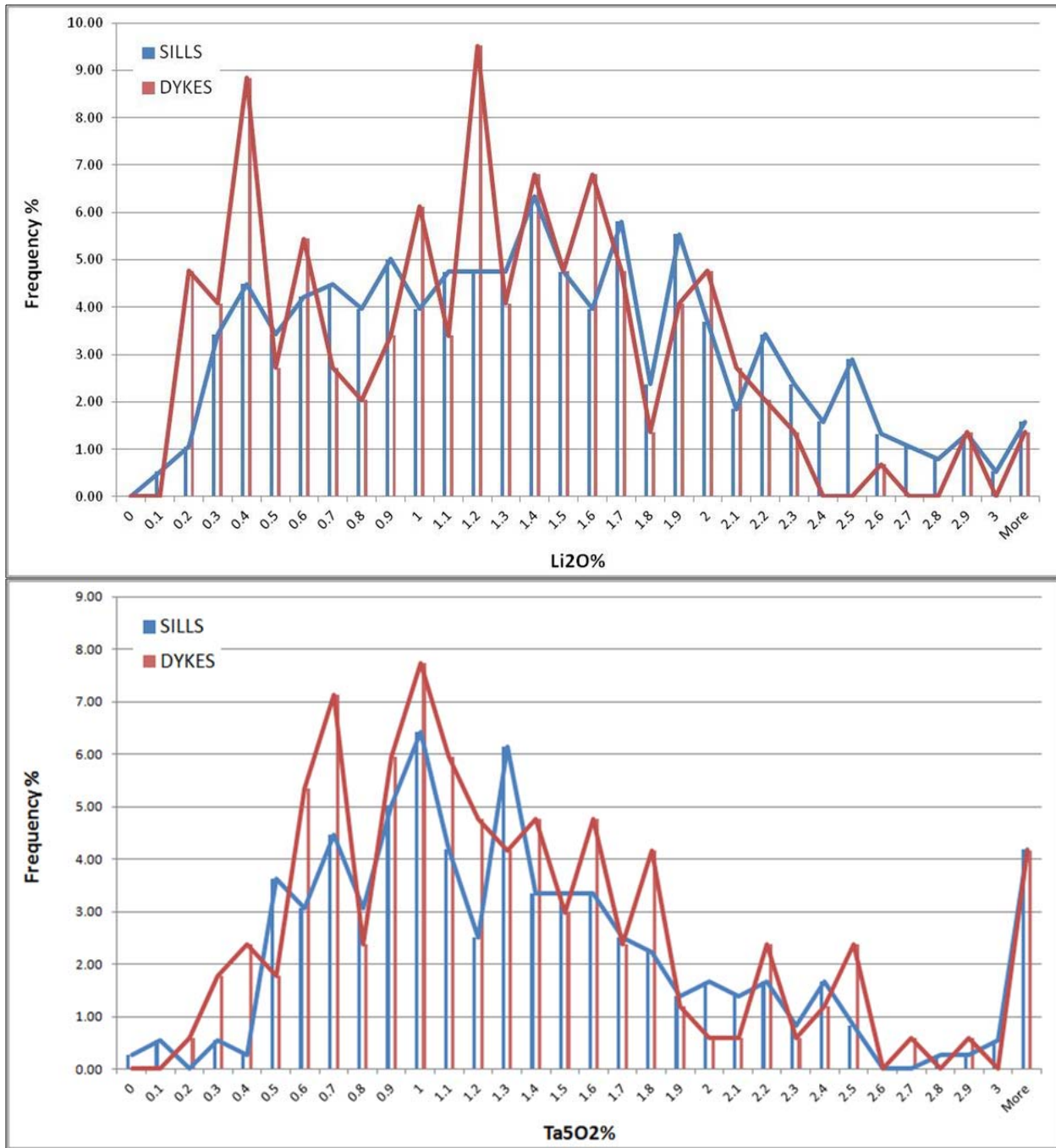
Figure 54 – Histogram distribution comparing composites from the sills and feeder dykes.
