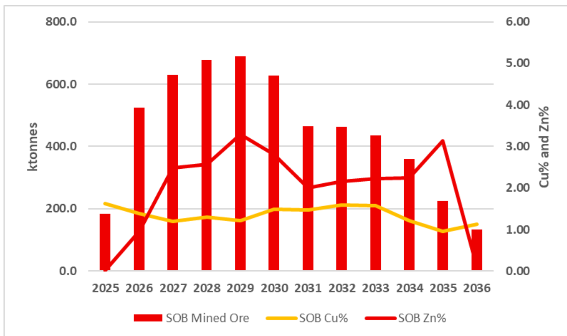
Figure 16.23 South Orebody; annual schedule of stope tonnes and grades
