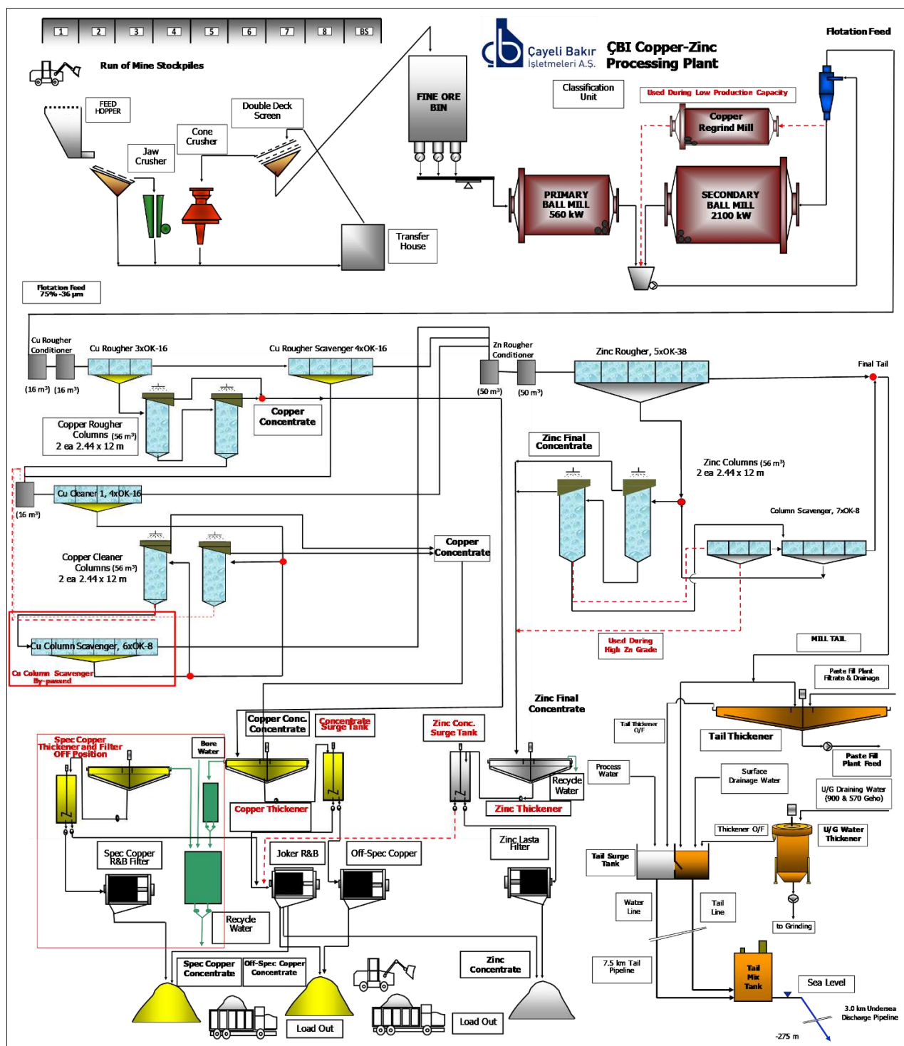
Figure 17.2 Pictorial flowsheet for the ÇBI ore processing facilities
