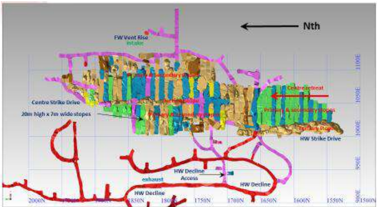
Figure 16.4 Example (completed) development and stoping layout, 940 mRL sublevel, Main Orebody
