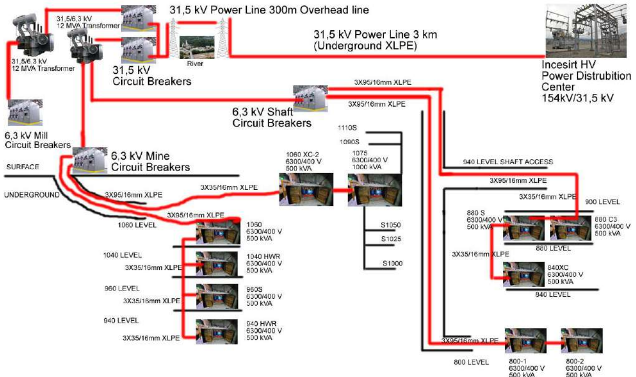
Figure 16.18 Underground power distribution diagram
