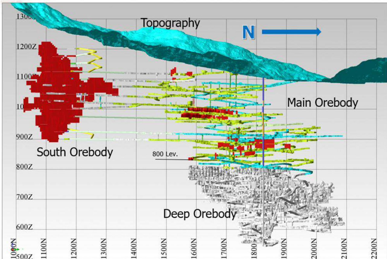
Figure 16.15 Longitudinal schematic (3D) view through the Main, Deep and South Orebodies
