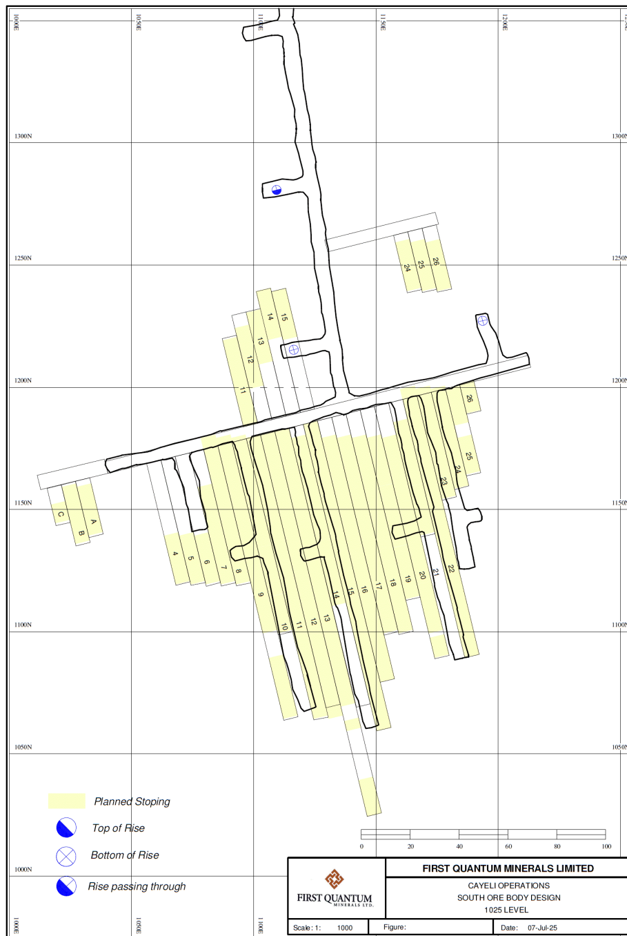
Figure 16.5 Example (planned) sublevel development and stoping layout, 1025 mRL sublevel, South Orebody
