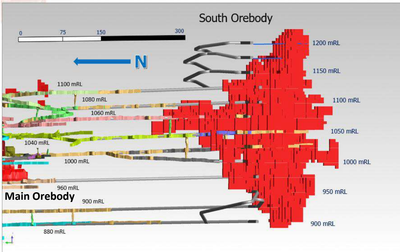
Figure 16.2 Oblique view of Main and South Orebody access development
