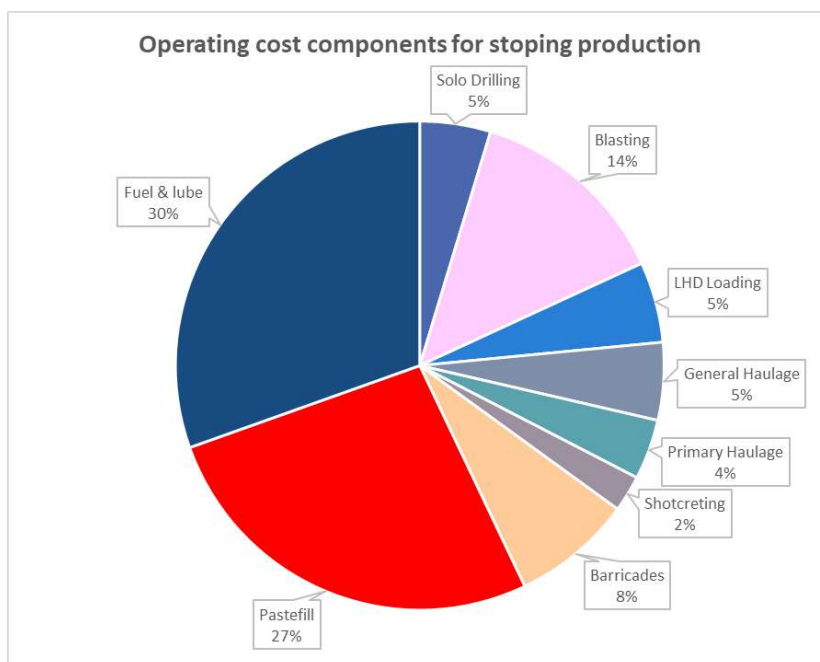
Figure 21.2 Operating cost chart (LOM averages) for stoping production
