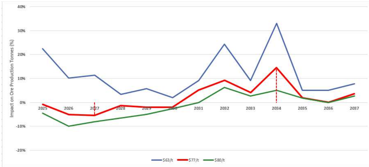
Figure 15.1 Production ore tonnes sensitivity to operating cost averaging
