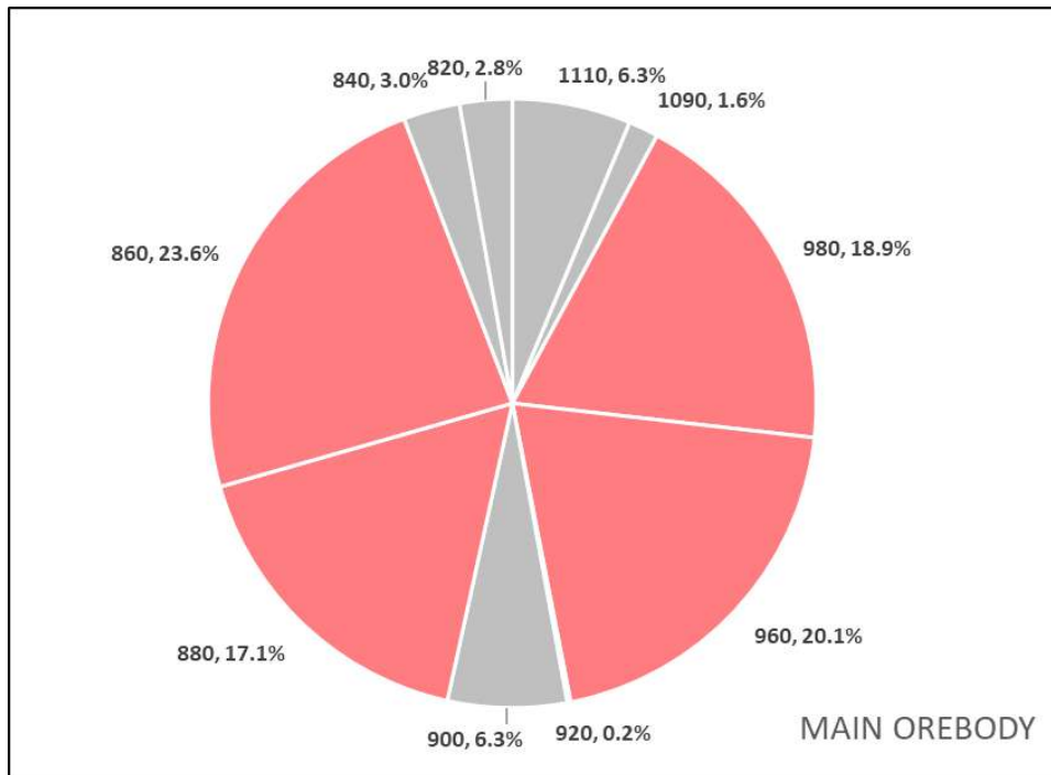
Figure 15.13 Main Orebody, Mineral Reserve tonnage (%) by sublevel
