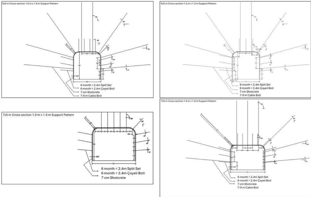
Figure 16.11 Typical rock reinforcement patterns (source: ÇBI 2025)
