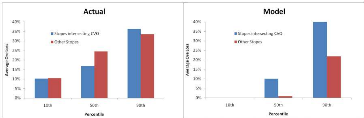
Figure 16.14 Actual overbreak vs modelled ore loss results comparison (source: AMC, 2014)
