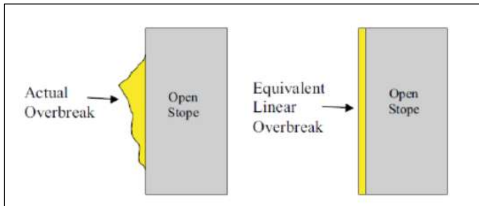
Figure 16.13 Unplanned mining dilution; equivalent linear overbreak (source: AMC, 2014)
