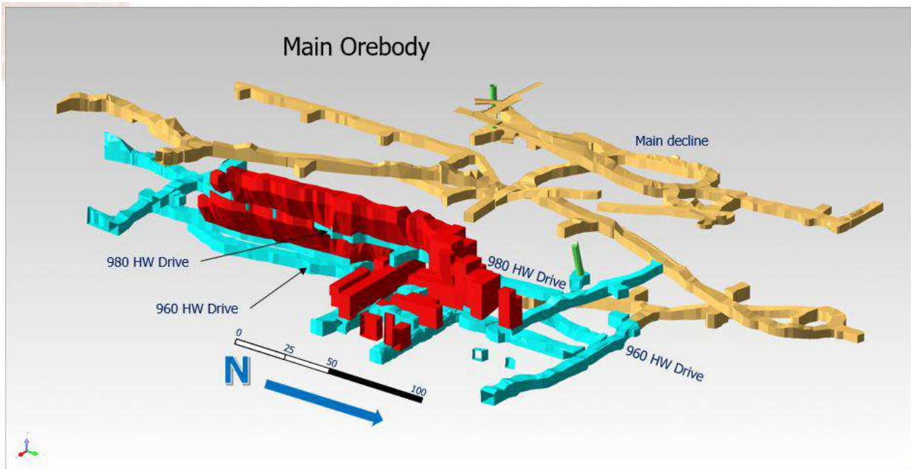
Figure 15.5 Main Orebody, 980 mRL and 960 mRL sublevels
