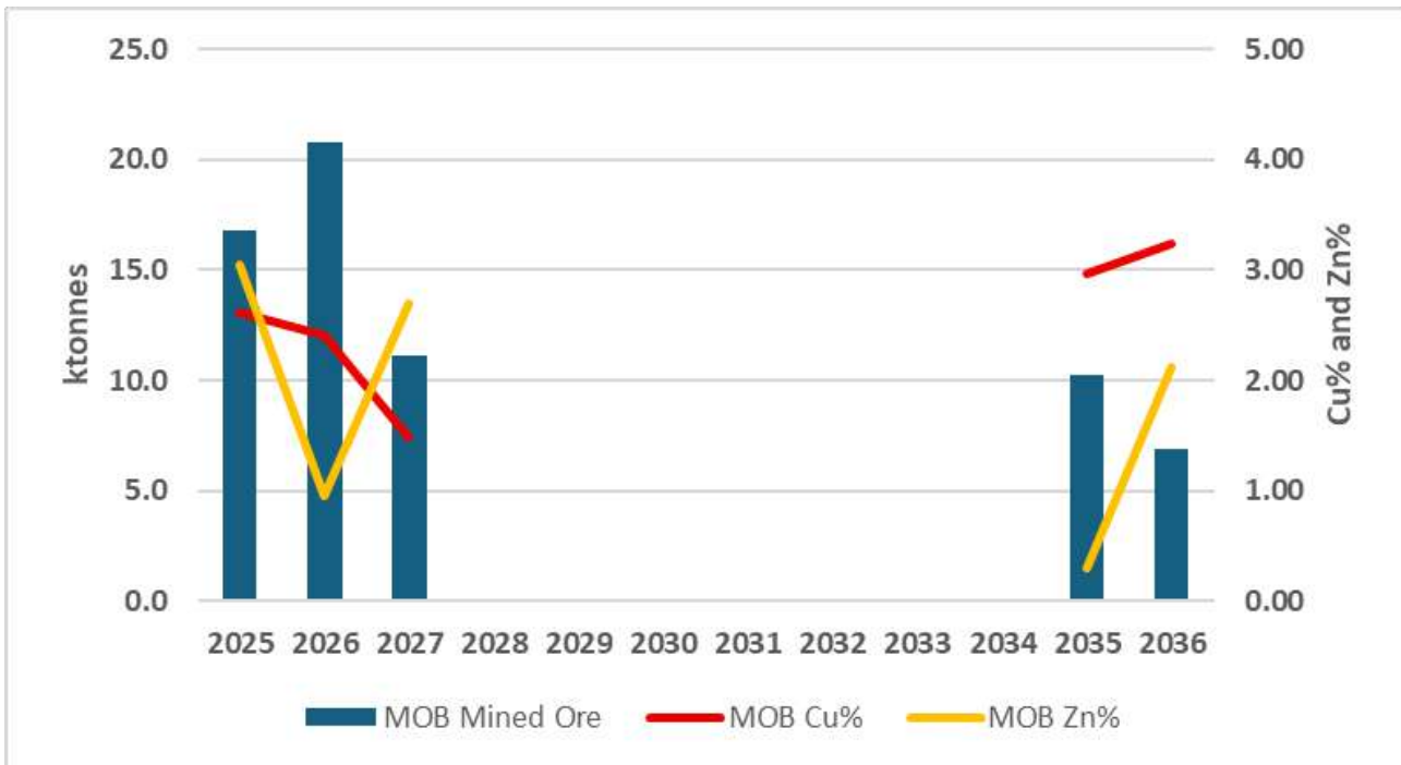
Figure 16.20 Main Orebody; annual schedule of development ore tonnes and grades
