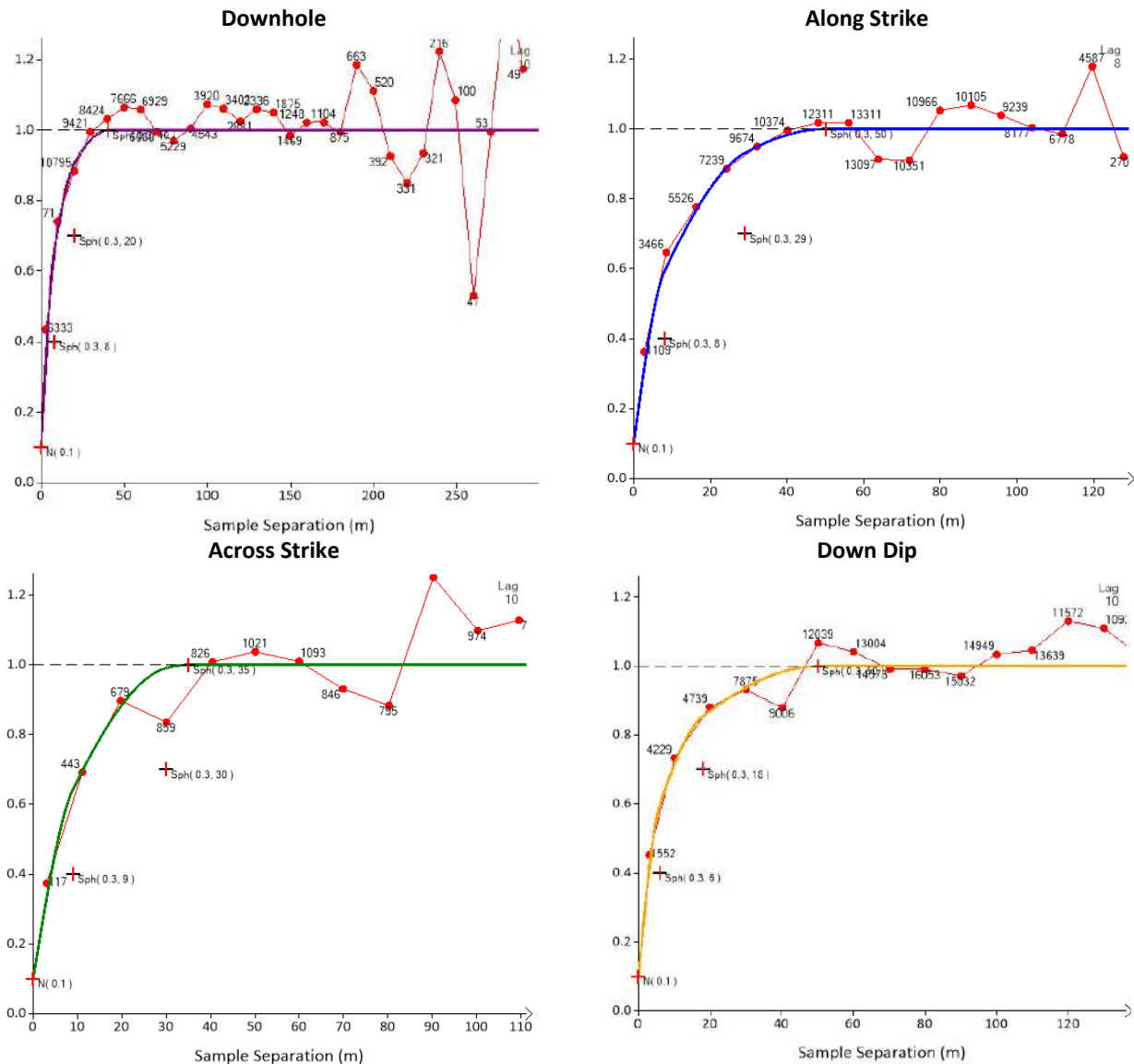
Figure 14.5 Example of normal scores variograms for Cu (ESTFLAGCU=5501)
