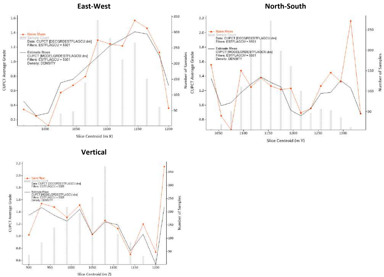
Figure 14.6 Disseminated stockwork estimate, South Orebody (ESTFLAGCU=5501)
