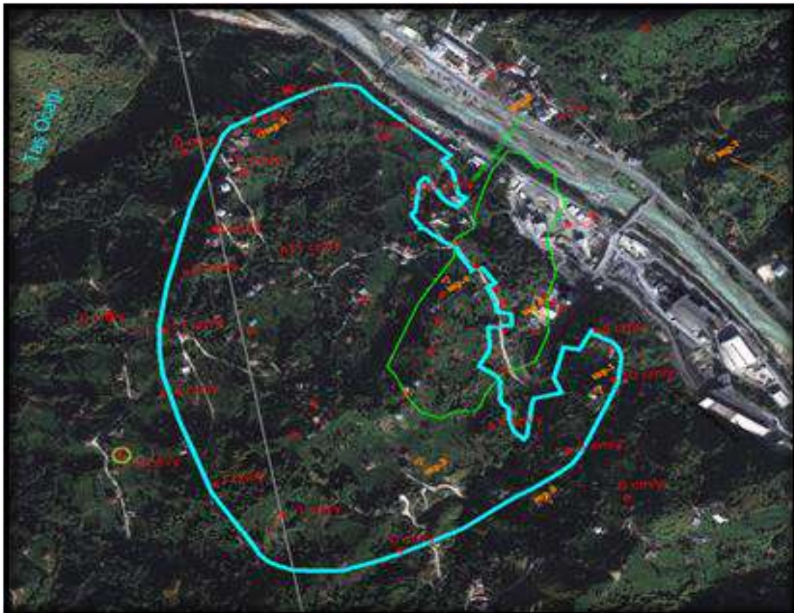
Figure 20.3 Defined landslide zone (source: ÇBI)
