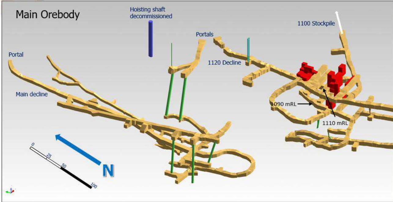
Figure 15.4 Main Orebody, 1100 mRL and 1080 mRL sublevels
