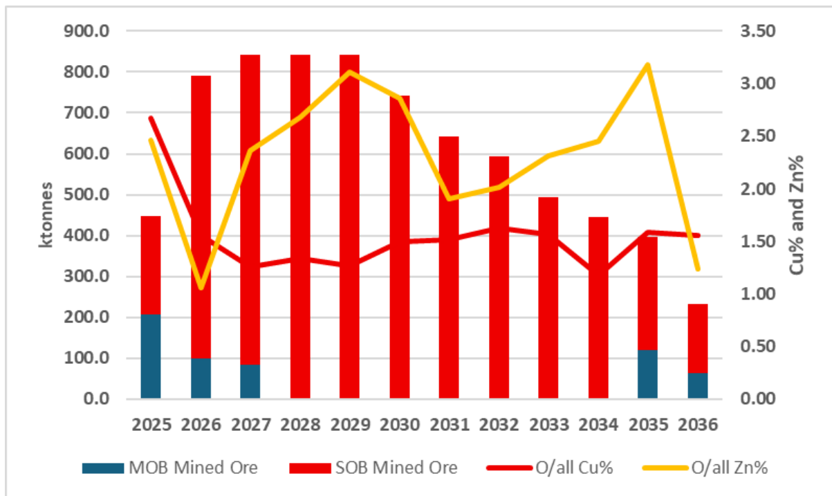
Figure 16.24 Annual schedule of combined development and stope tonnes and grades
