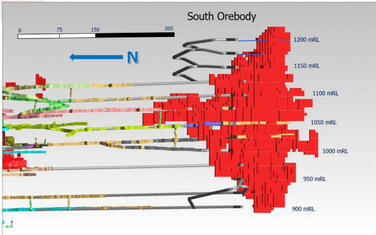
Figure 15.12 South Orebody, 1200 mRL to 900 mRL
