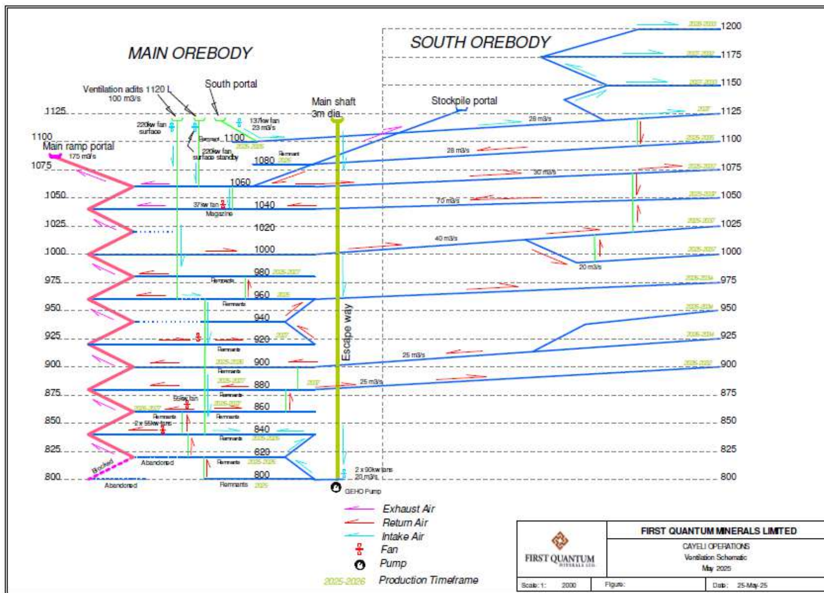
Figure 16.17 Ventilation network diagram; Main Orebody and South Orebody during development
