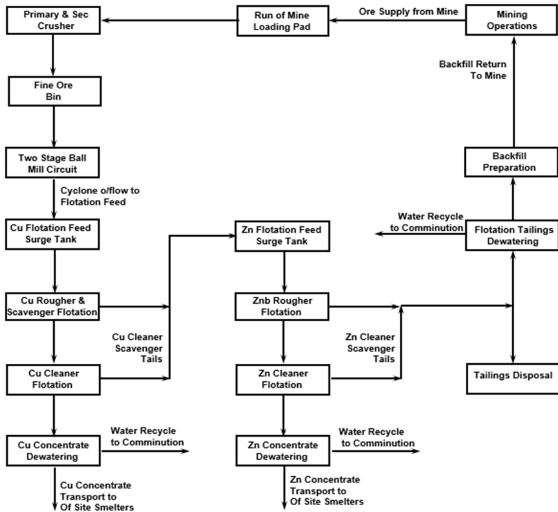
Figure 1.2 Simplified block flowsheet for the ÇBI processing facilities
