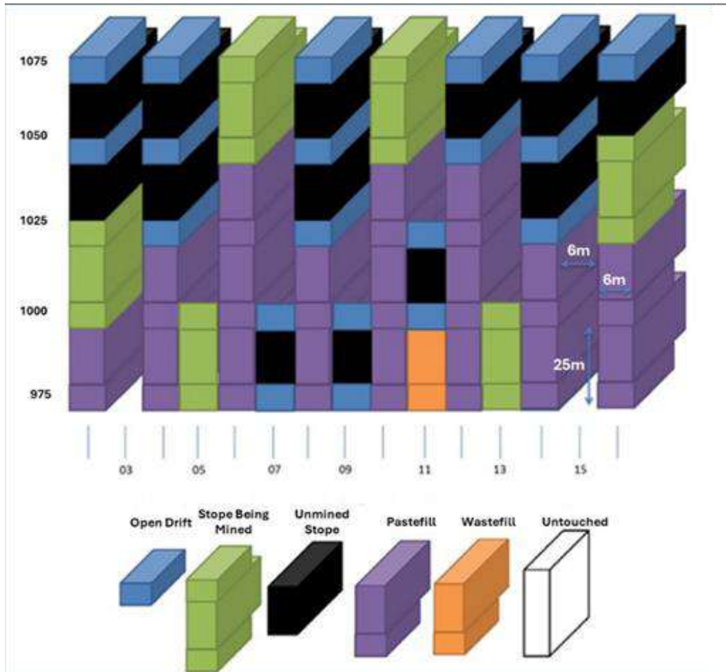
Figure 16.7 Mining sequence across multiple sublevels (source: ÇBI, January 2025)
