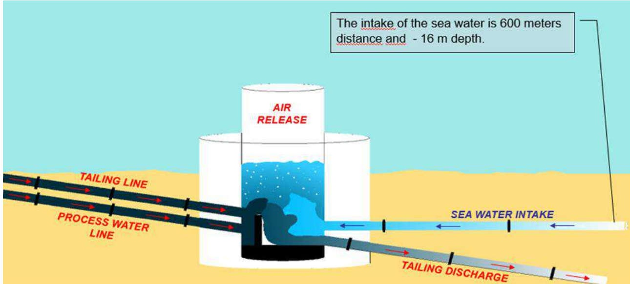
Figure 18.3 DST mix tank arrangement (source: ÇBI)
