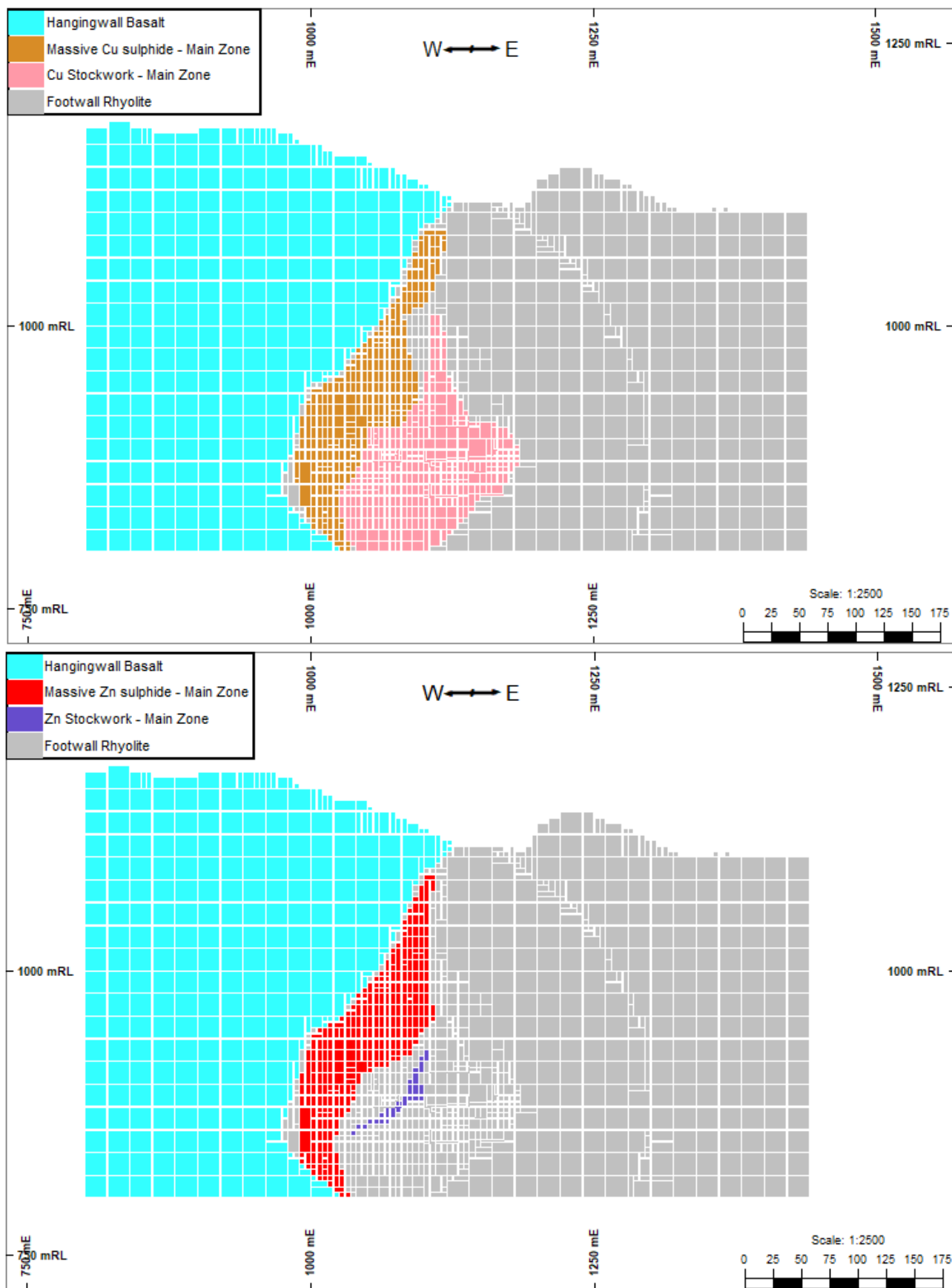
Figure 7.3 East-west Section (1800 mN) through the Main Orebody illustrating the Cu and Zn zones
