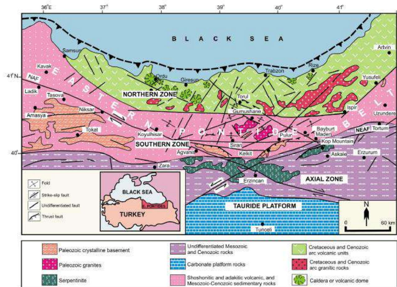
Figure 7.1 Geological and tectonic map of the Eastern Pontides Orogenic Belt (Eyuboglu et al 2006)
