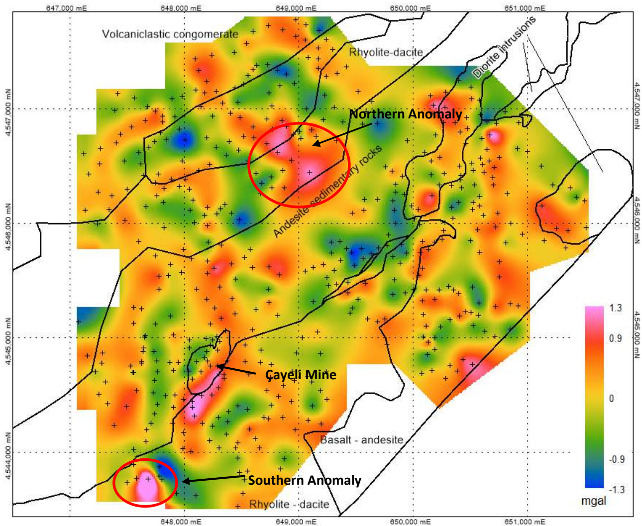
Figure 9.2 Gravity anomalies in the vicinity of the Çayeli mine (FQM, 2020)
