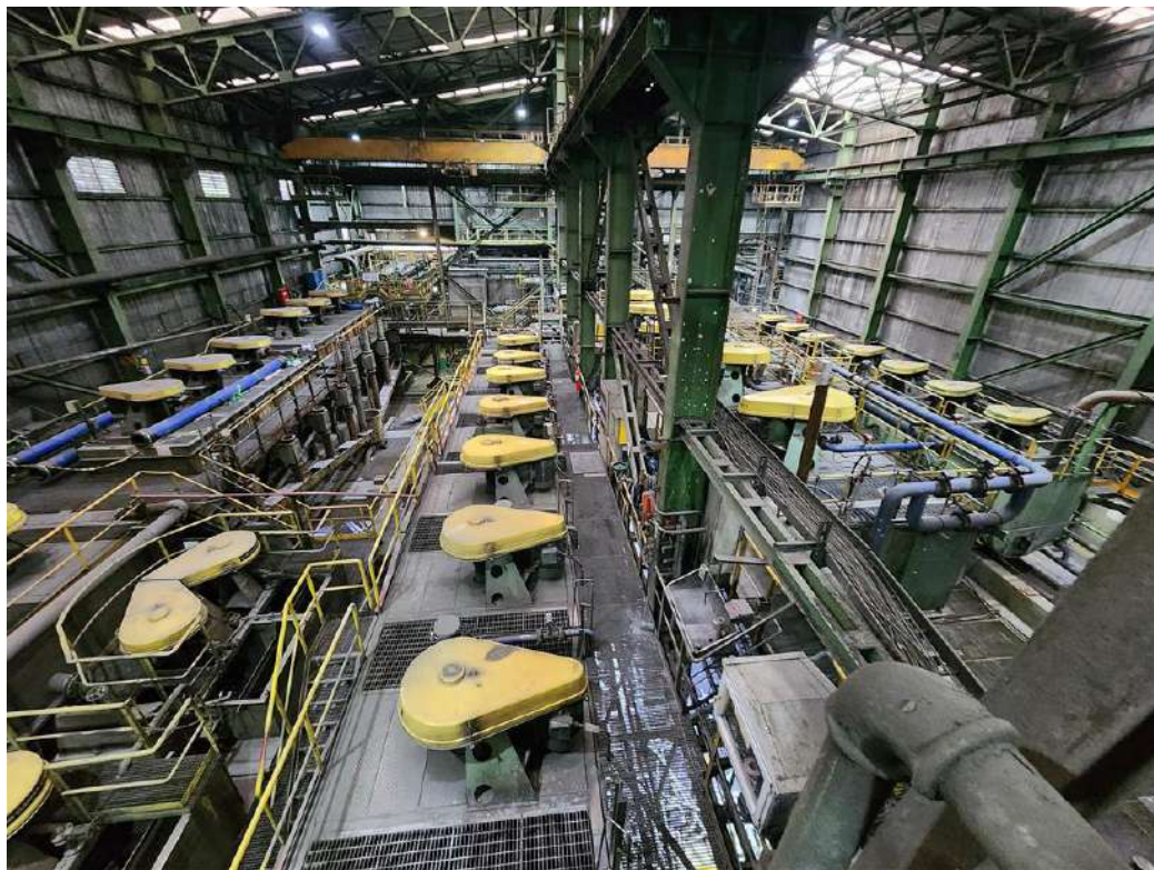
Figure 17.7 Flotation circuit
