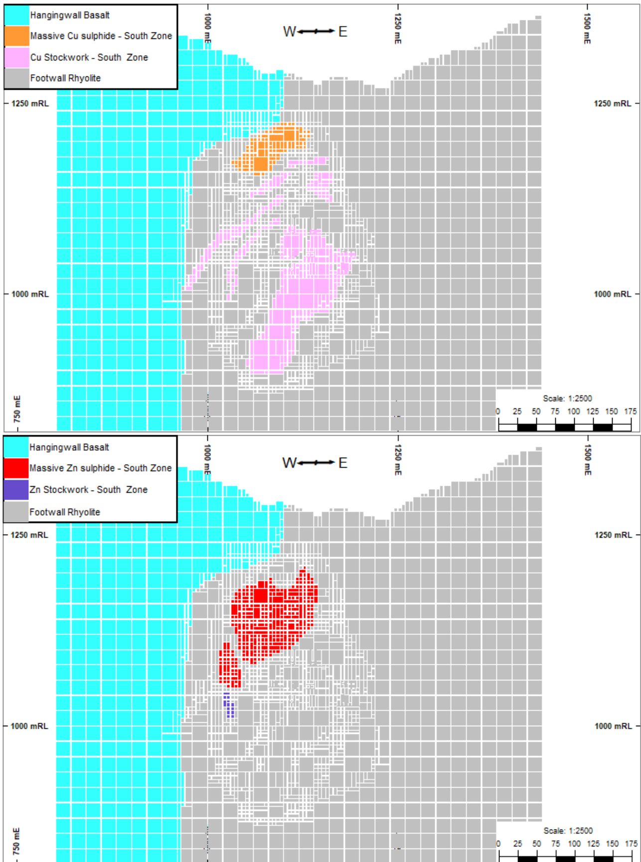
Figure 7.4 East-west Section (1100 mN) through the South Orebody illustrating the Cu and Zn zones
