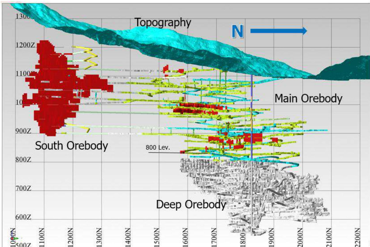
Figure 1.3 Longitudinal schematic (3D) view through the Main, Deep and South Orebodies
