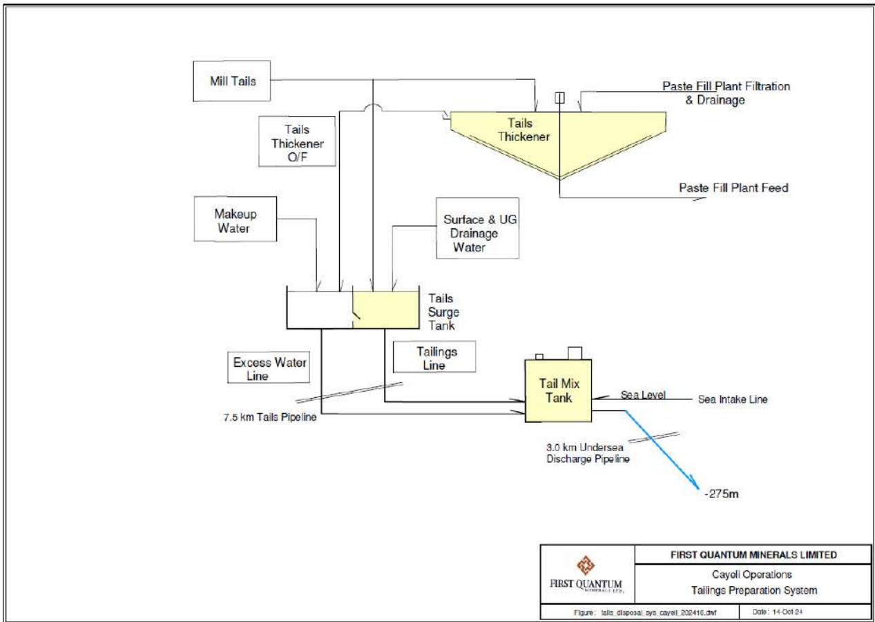
Figure 18.1 Çayeli tailings preparation system (source: FQM)
