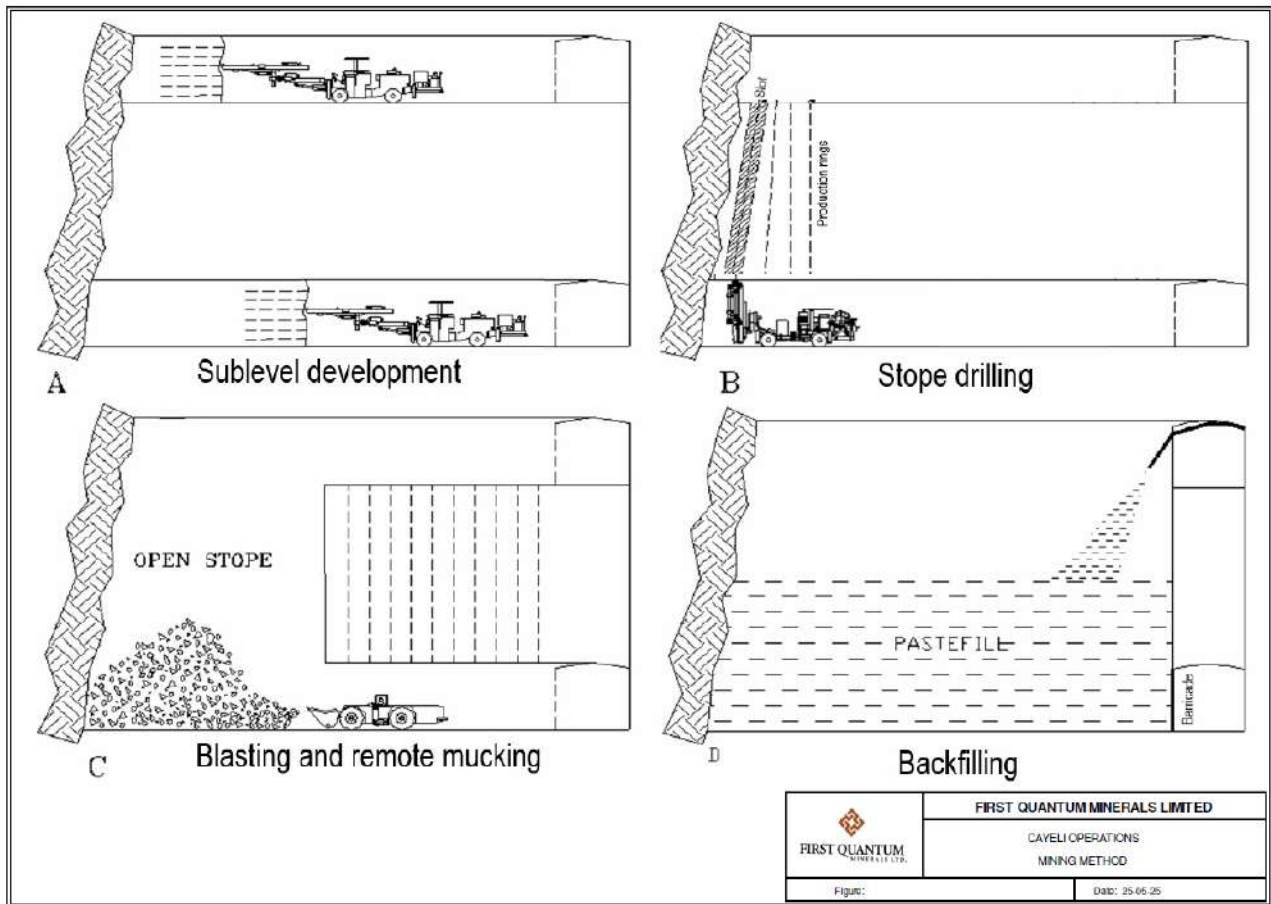
Figure 16.6 Sequence of individual stope production activities
