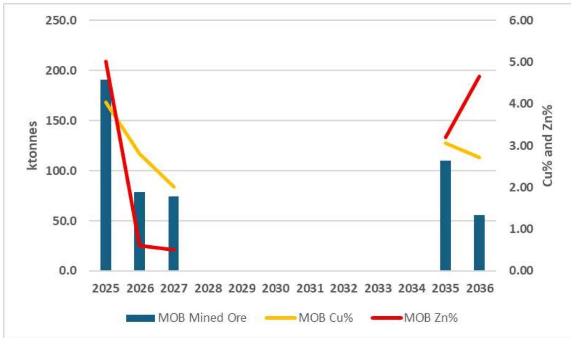
Figure 16.22 Main Orebody; annual schedule of stope tonnes and grades
