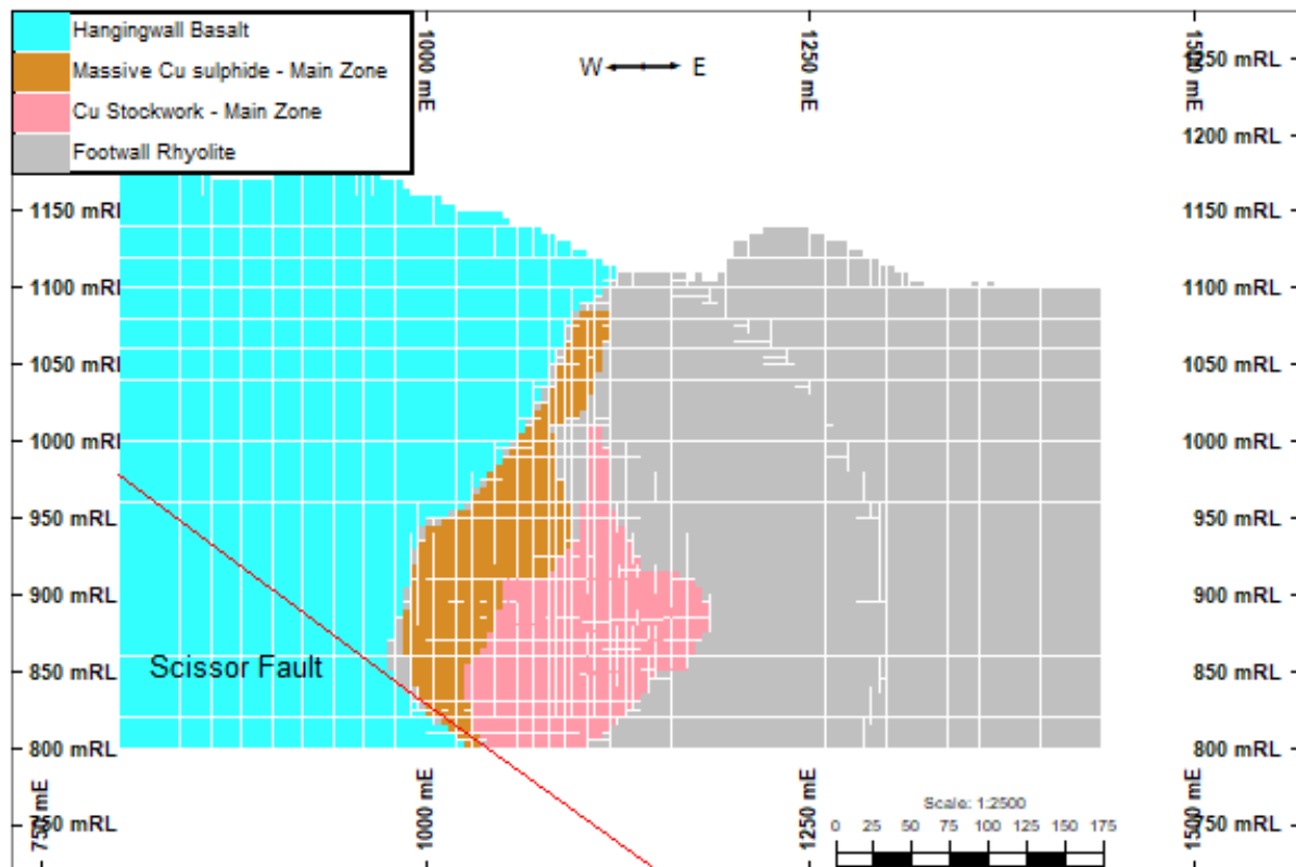
Figure 16.9 Location of the Scissor Fault, separating the Main and Deep Orebodies on section 1120 mN
