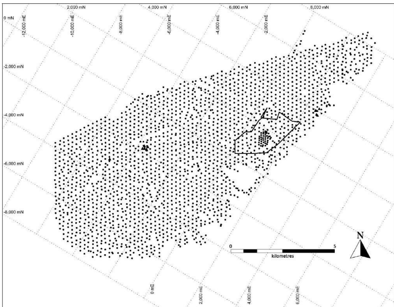
Figure 9.1 Plan of soil sampling locations and the current lease boundary
