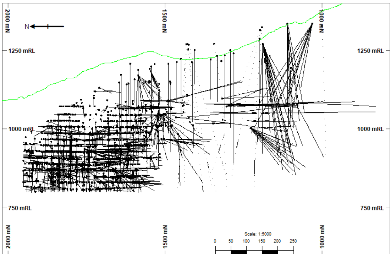
Figure 14.1 North-South Section (1000 mN) showing the clipped Çayeli drilling and topography
