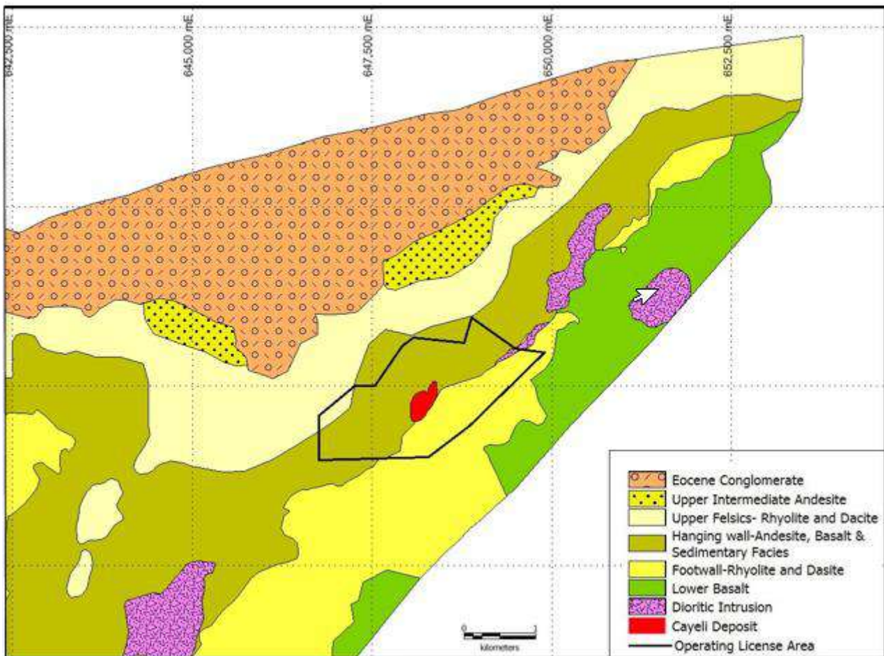
Figure 7.2 Çayeli, geology map (source: RPA, 2006)
