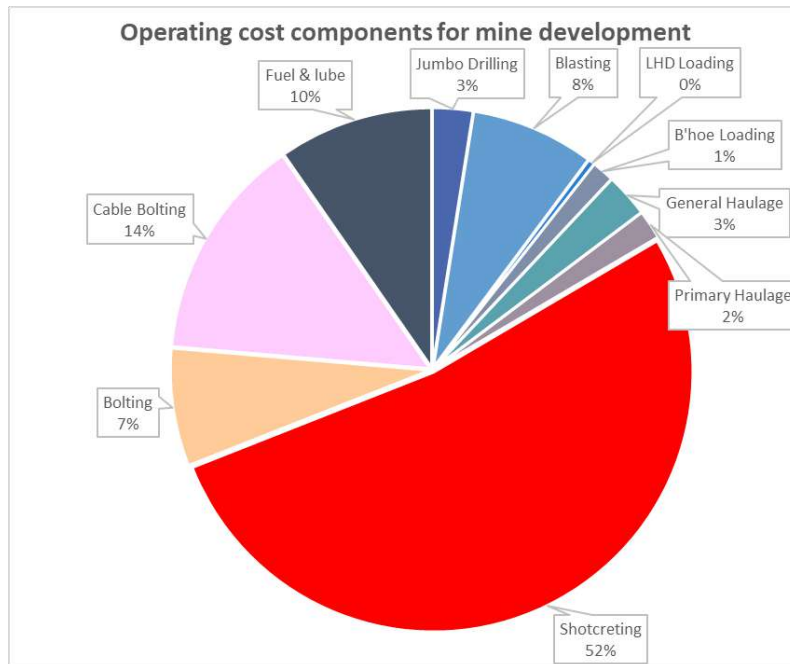
Figure 21.1 Operating cost chart (LOM averages) for mine development
