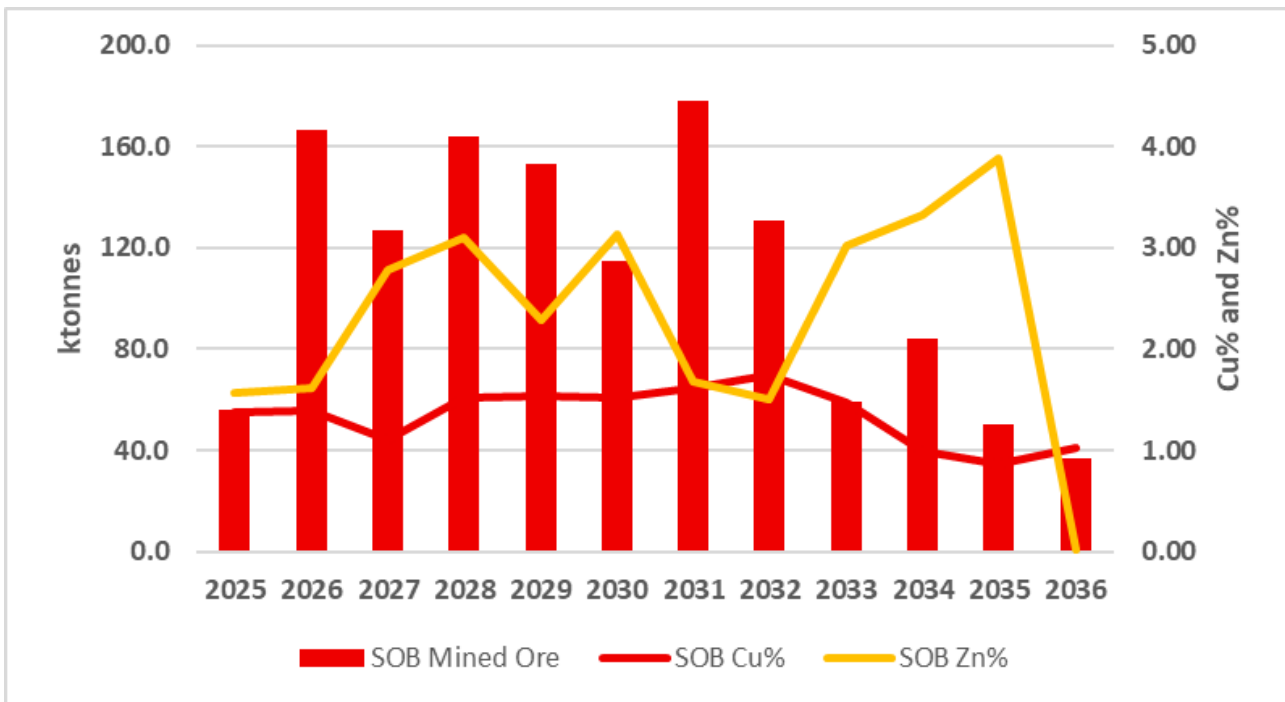
Figure 16.21 South Orebody; annual schedule of development ore tonnes and grades
