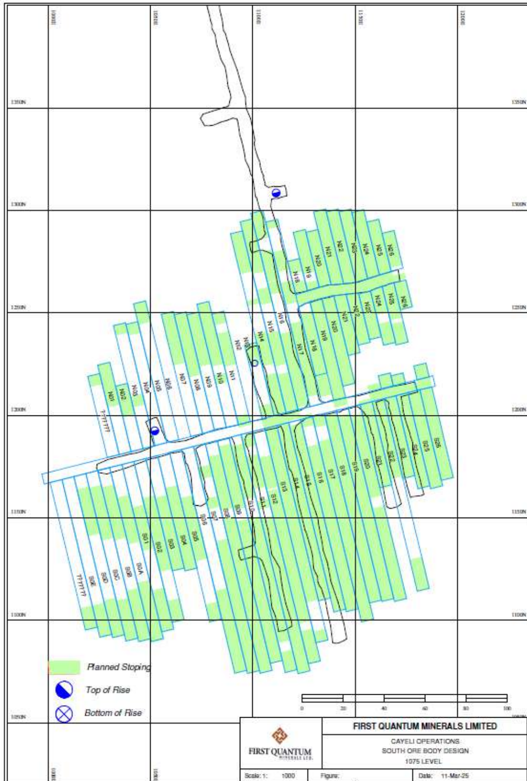
Figure 15.3 South Orebody, sublevel design example
