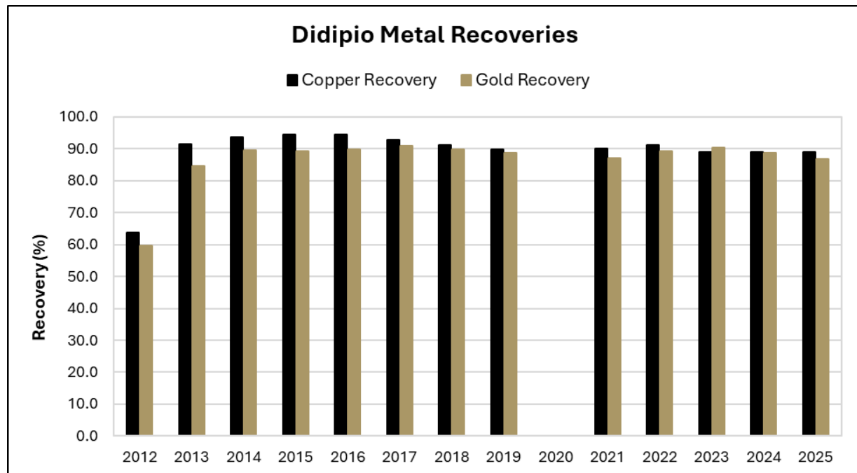
Figure 17-4: Annual Gold and Copper Recovery Data
