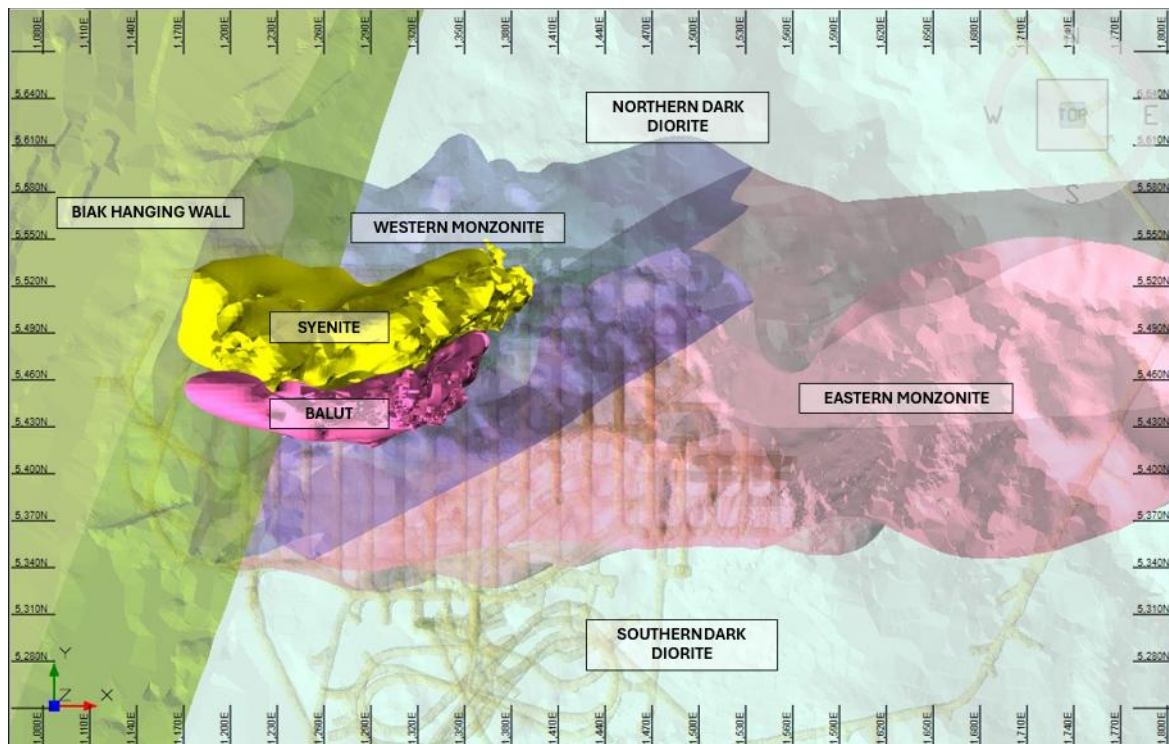
Figure 16-5: Didipio Geotechnical Domains (Plan View: 2280 mRL and below)
