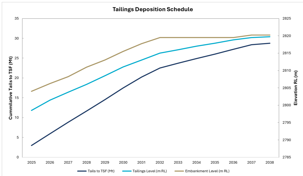
Figure 18-2: LoM Storage Requirements and Scheduled TSF Development
