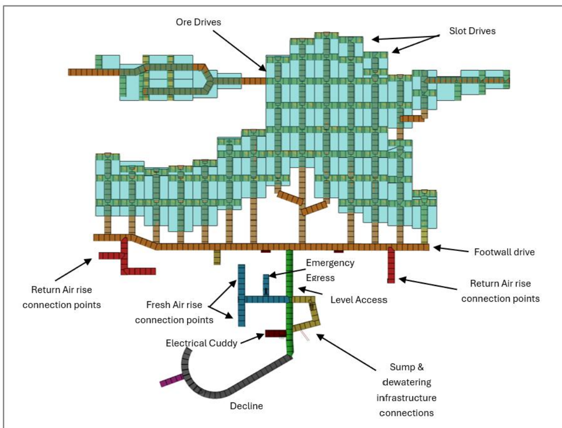
Figure 16-12: Plan View - Didipio Underground Level Layout (2100 mRL Level Plan View)
