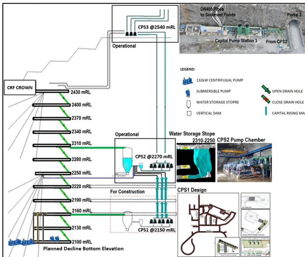
Figure 16-7: Didipio Dewatering Schematic
