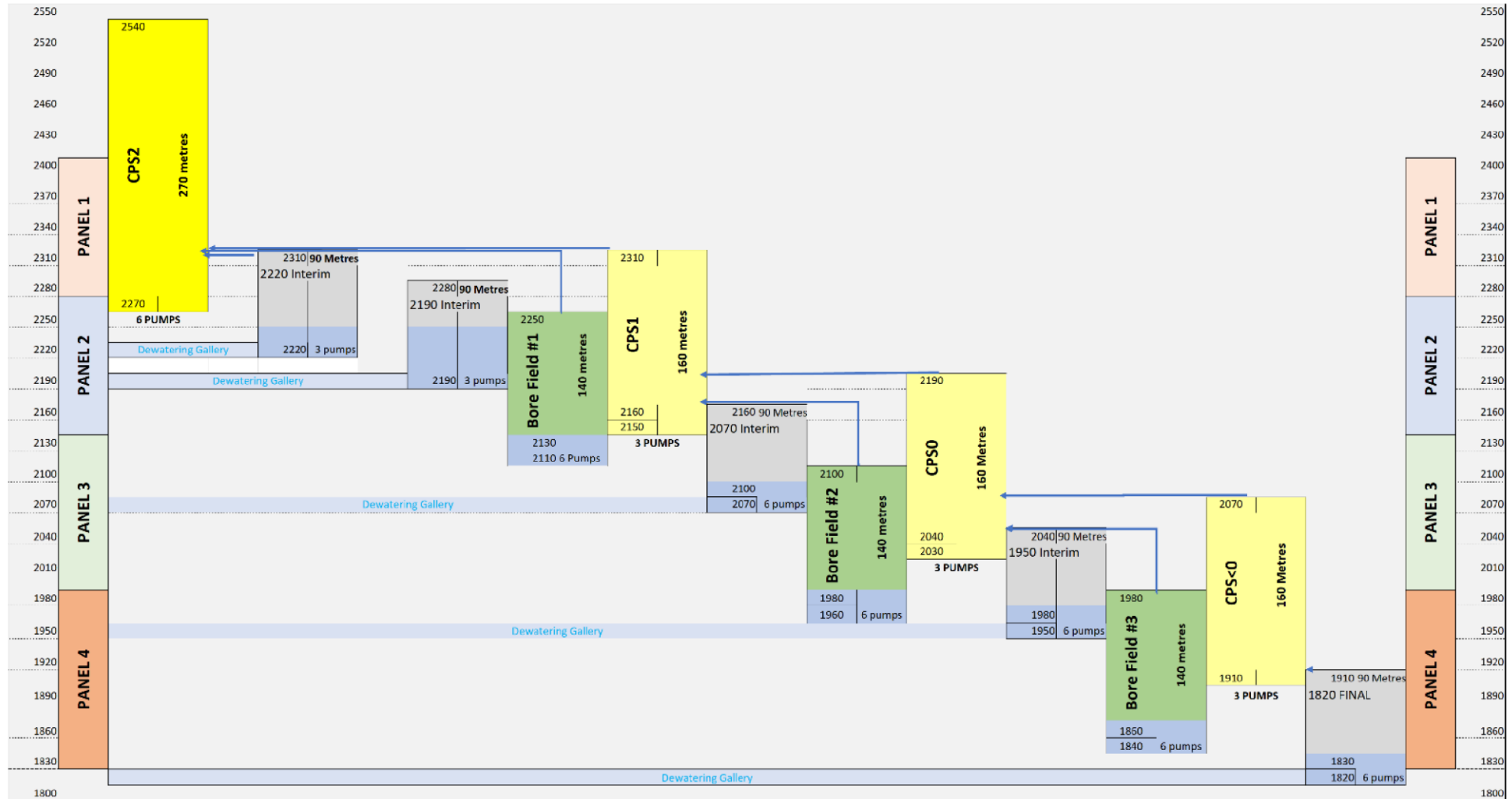
Figure 16-6: Underground Dewatering Strategy Schematic
