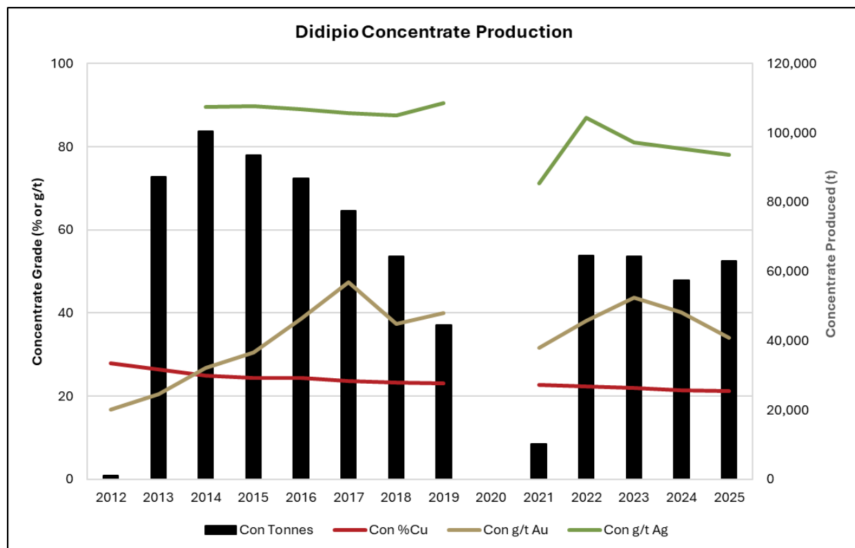
Figure 17-3: Annual Didipio Concentrate Production Data
