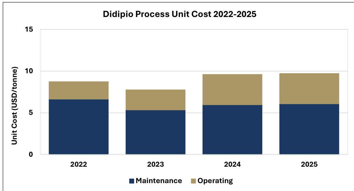
Figure 17-6: Processing Plant Unit Cost Performance
