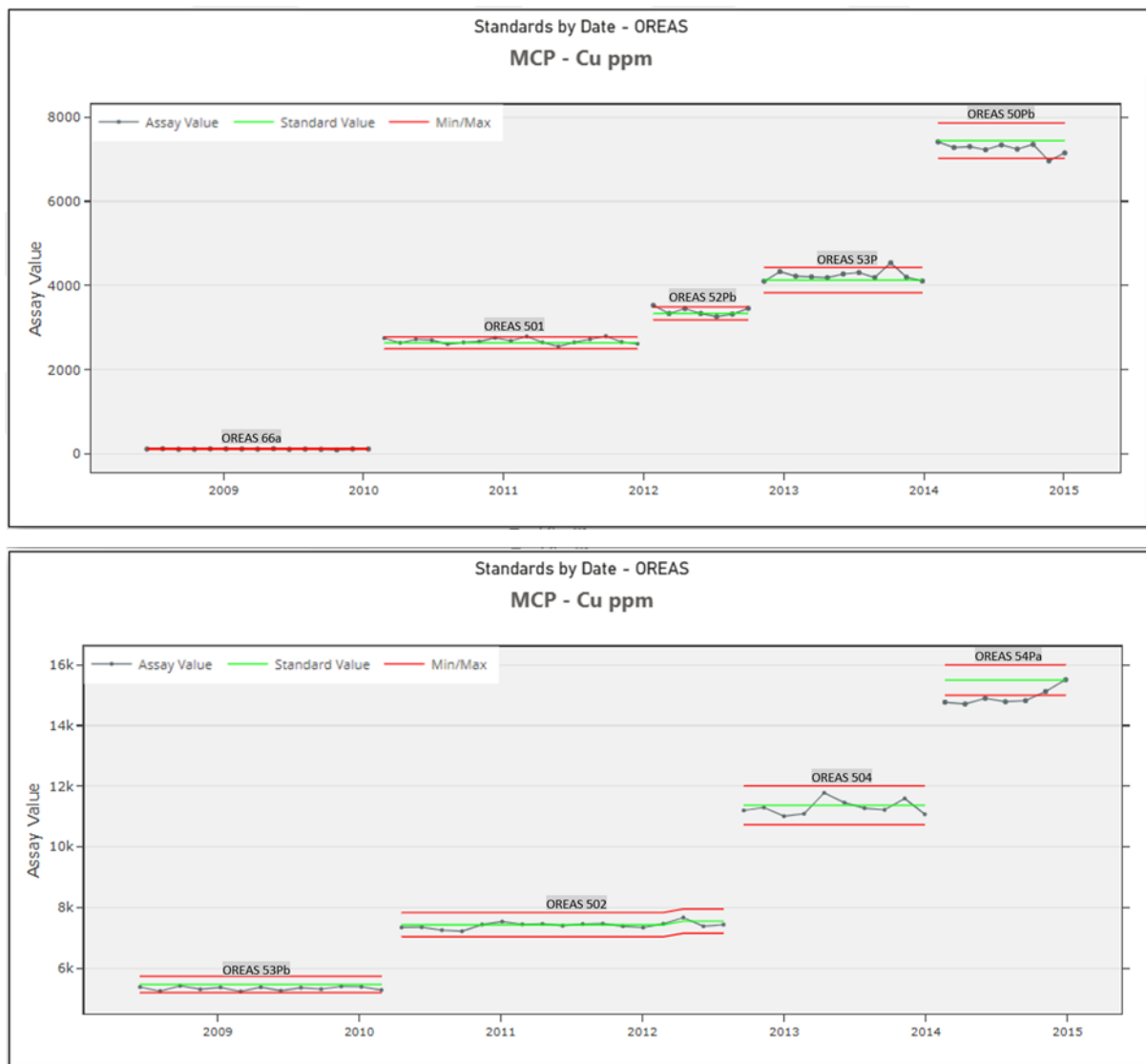
Figure 12-5: Cu Standards - McPhar-Intertek (9 Standards Used – 2 Charts)
