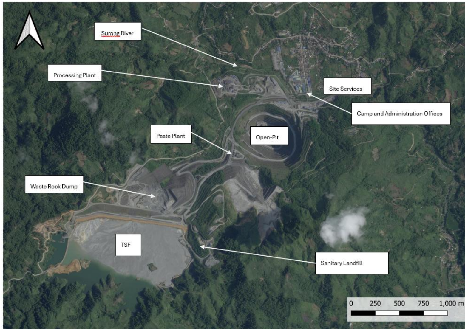
Figure 18-1: Didipio Site Plan with Major Surface Infrastructure Including TSF
