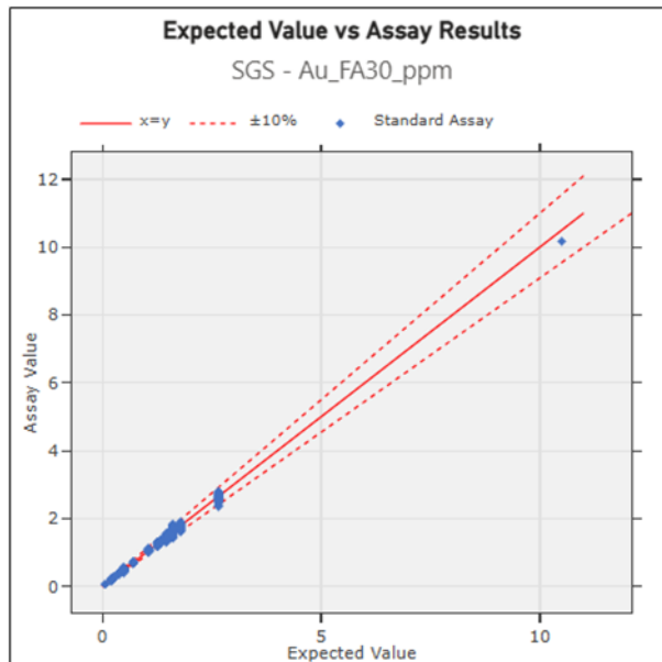
Figure 12-1: Gold (g/t Au) Standards - SGS
