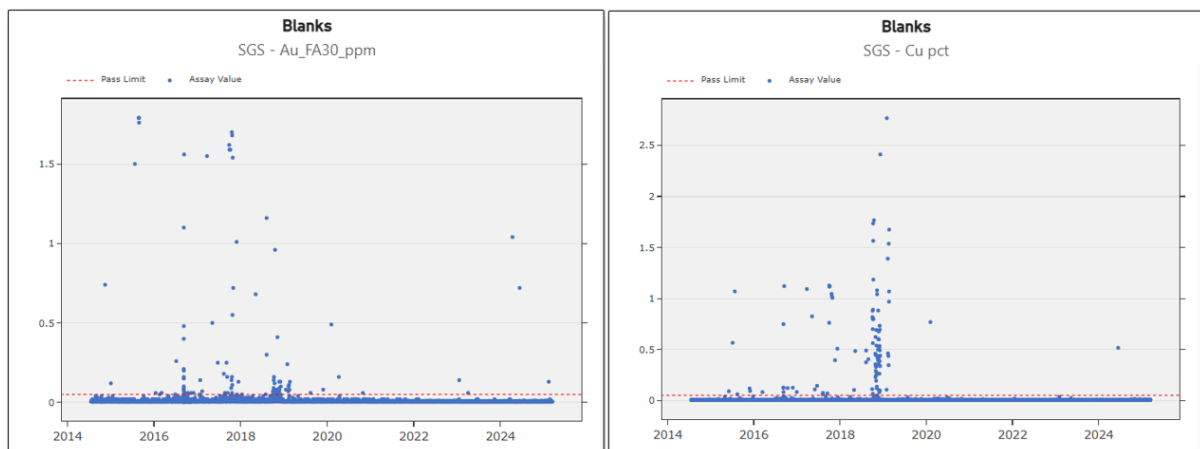
Figure 12-9: Standard Blank for Au and Cu – SGS
