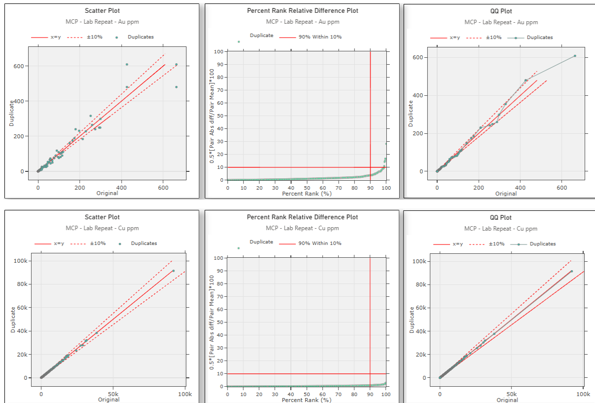
Figure 12-11: Lab Repeat Metrics for Au and Cu (McPhar-Intertek Laboratory)
