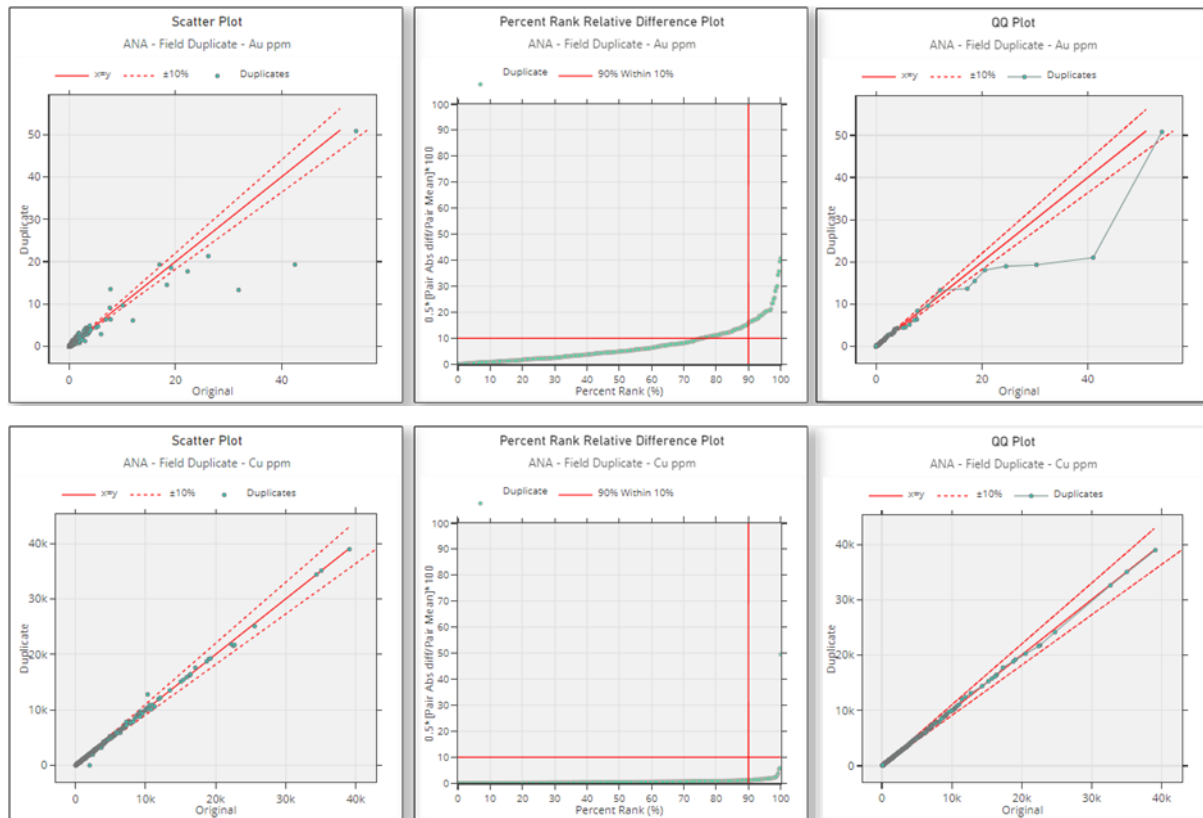
Figure 12-13: Field Duplicates for Cu and Au (Analabs Laboratory)
