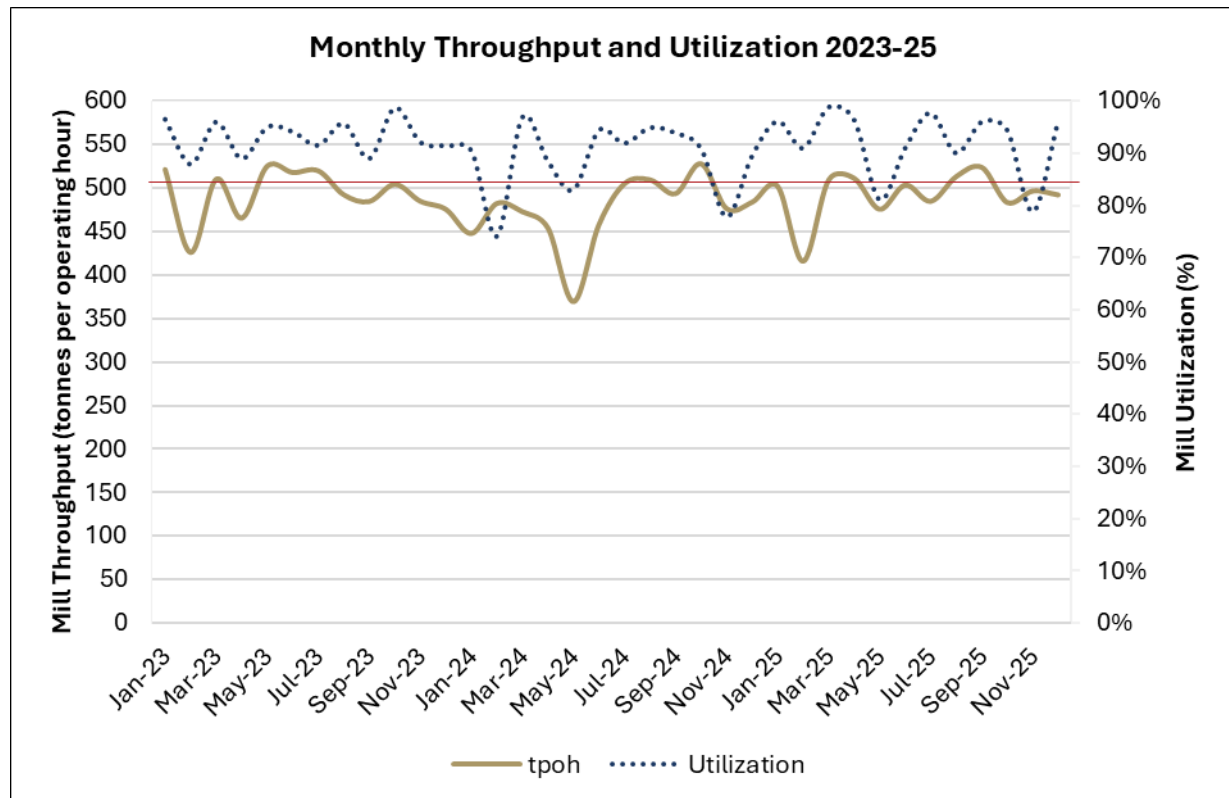
Figure 17-7: Historic Throughput and Utilisation
