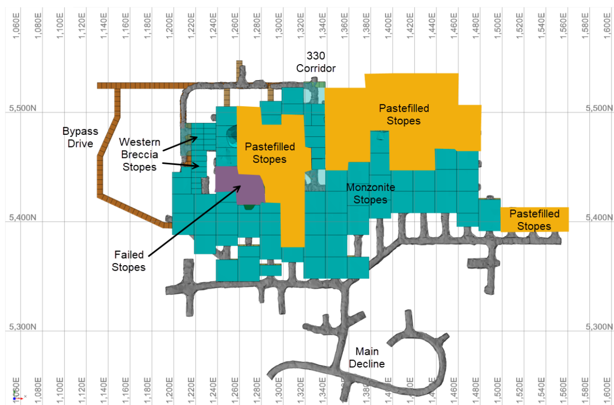
Figure 16-13: 2370 Level Plan View
