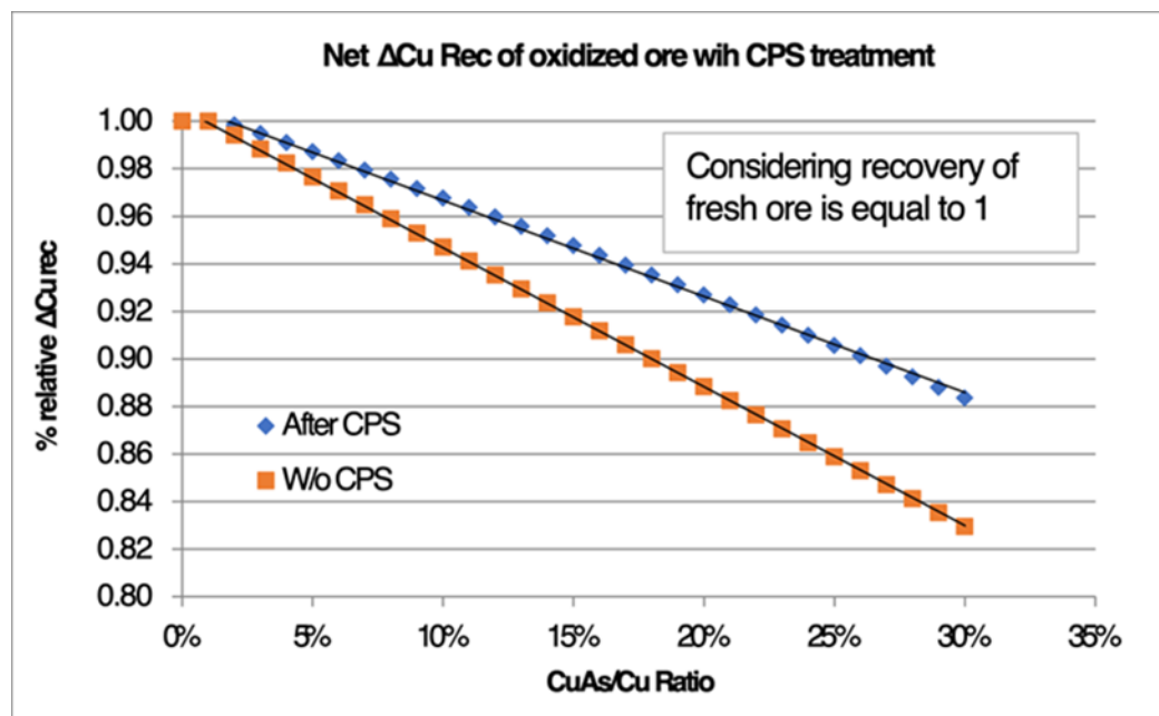
Figure 13-3: Relative Copper Recovery Change (With and Without CPS Compared to Fresh Ore)
