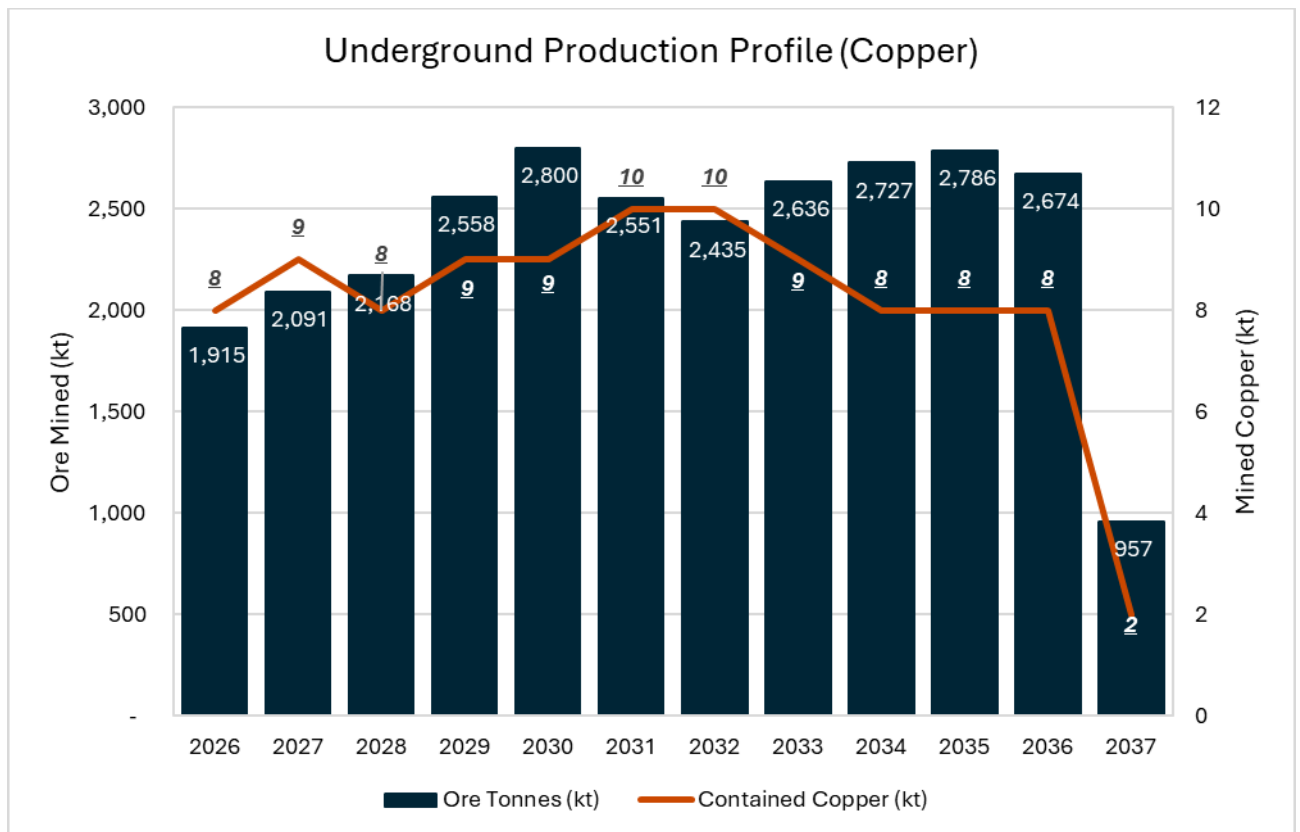
Figure 16-22: Annual Underground Production - Copper
