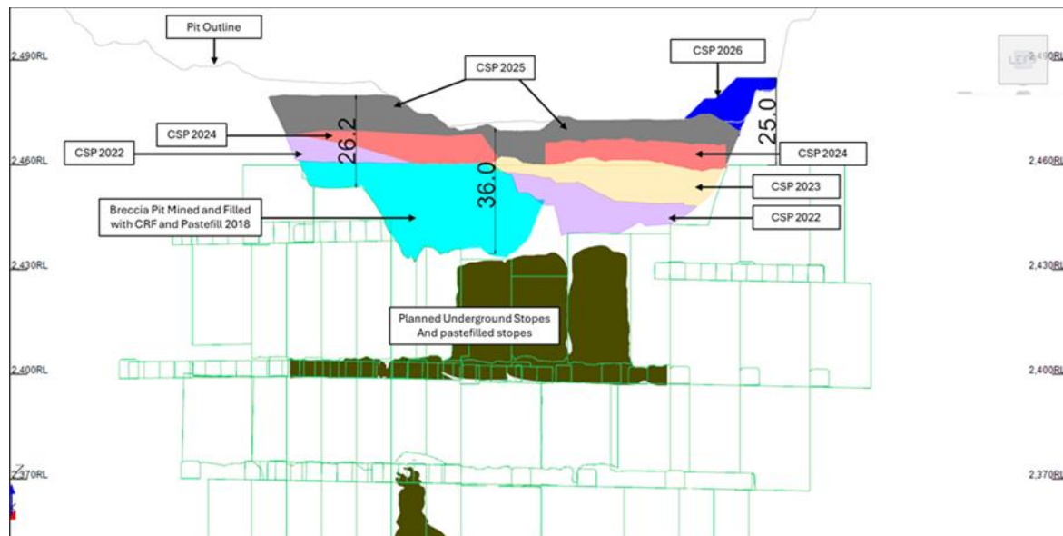
Figure 16-2: Section View of CSP (Looking East)
