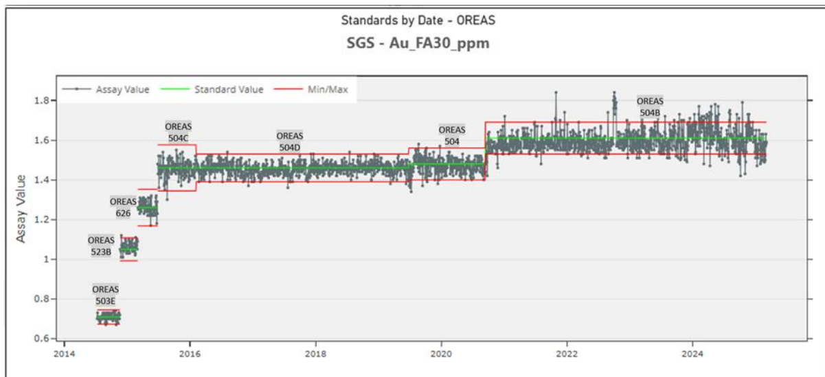
Figure 12-6: Au Standard – SGS (Shown Over 2 Charts)
