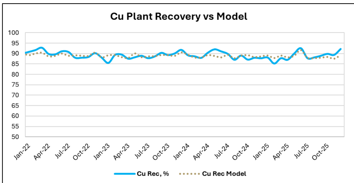
Figure 13-5: Didipio Copper Recovery vs Model
