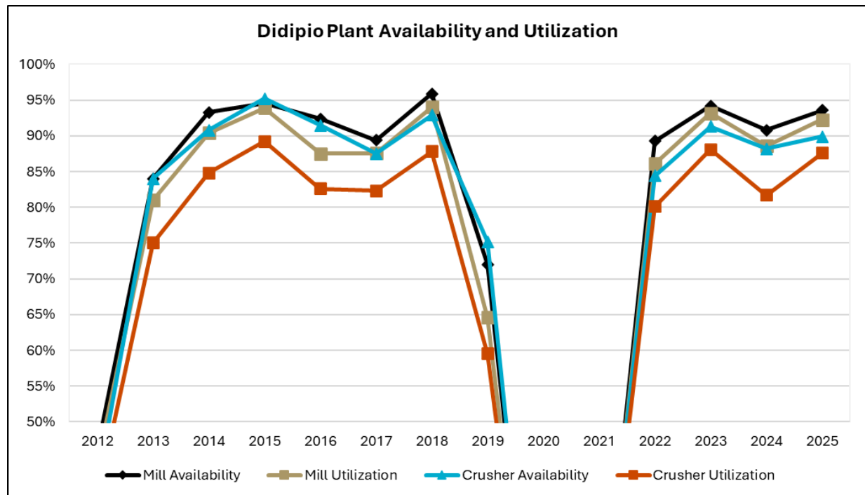
Figure 17-5: Annual Plant Availability and Utilisation
