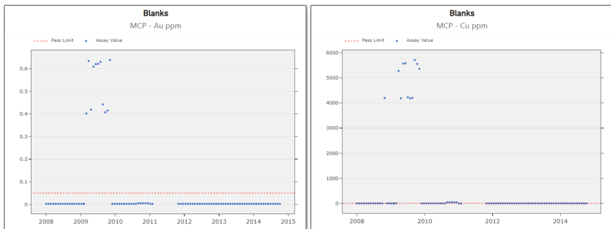
Figure 12-8: Blanks for Au and Cu - McPhar Intertek
