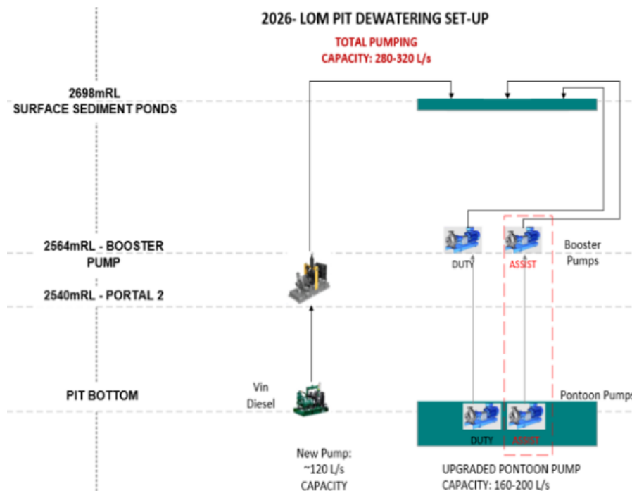
Figure 16-10: 2026 In-Pit Dewatering Set-Up
