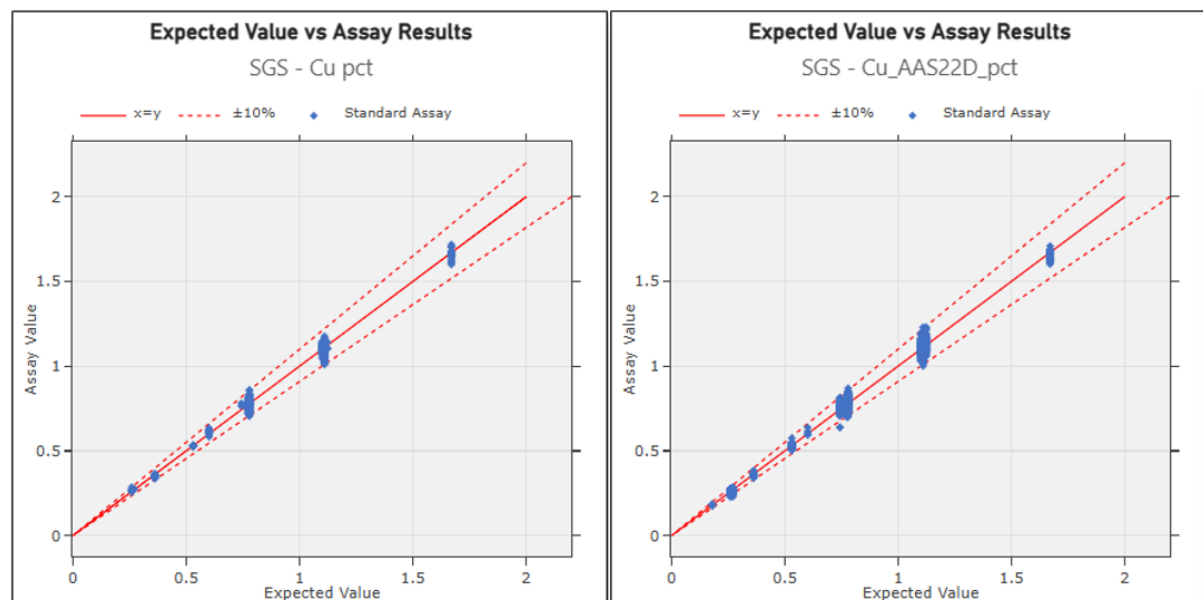
Figure 12-2: Copper (% Cu) XRF - Left, % CU AAS - (Right) Standards – SGS
