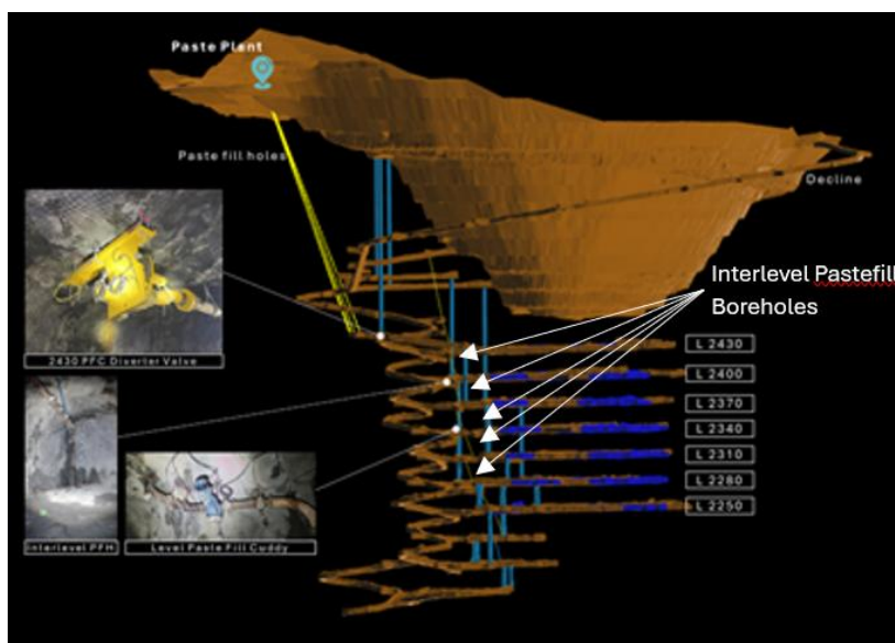
Figure 16-19: Underground Pastefill Reticulation
