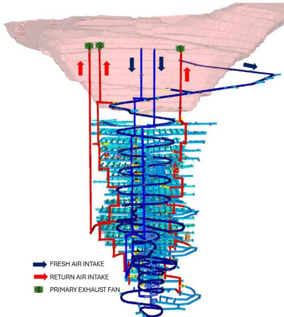
Figure 16-16: Ventsim Model - Primary Ventilation Upgrades
