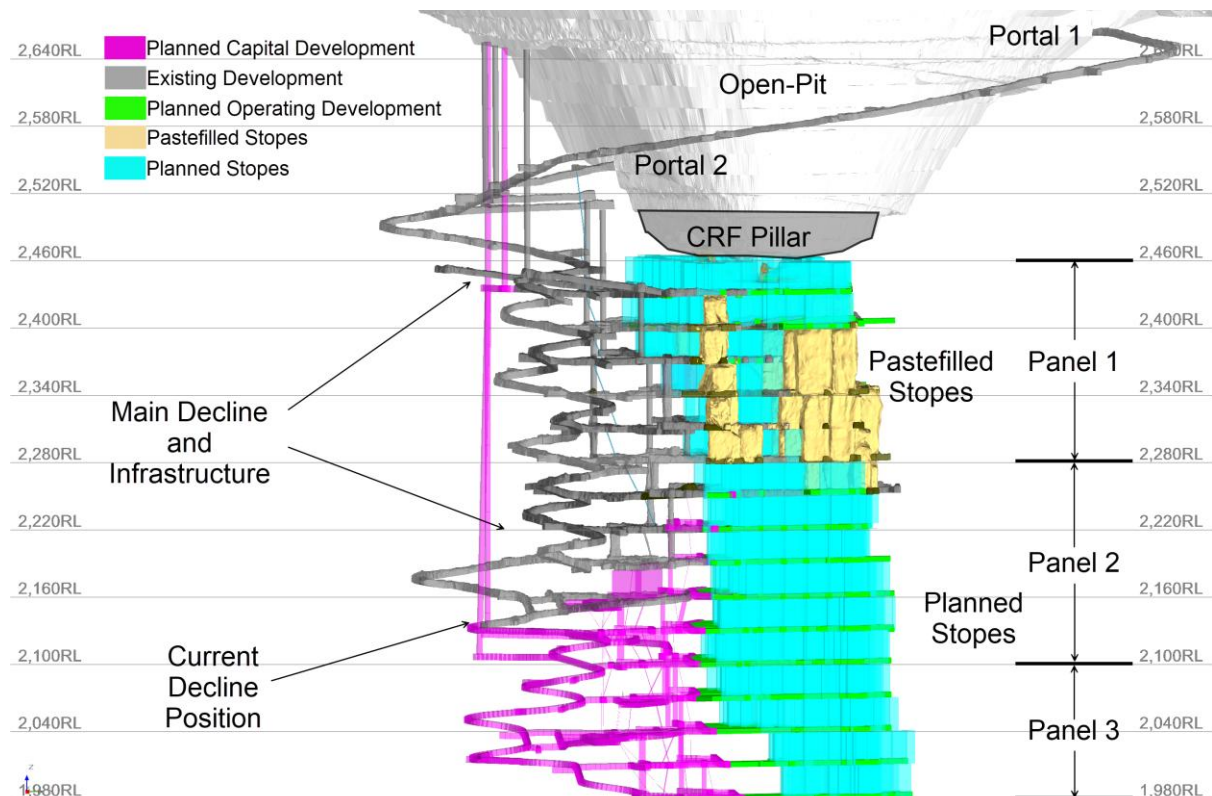
Figure 16-1: Didipio Underground – Oblique view Looking North- West
