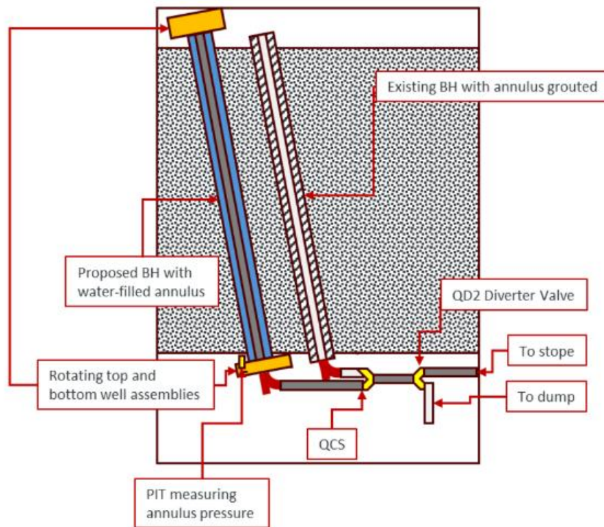
Figure 16-20: Basic Schematic of Proposed BH04 Primary Borehole
