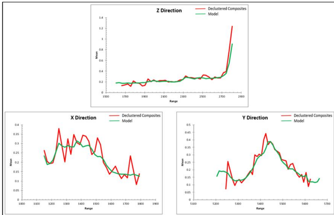
Figure 14-5: Swath Plot (cudom 1)
