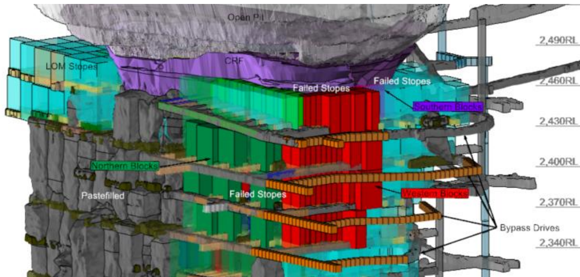
Figure 16-14: Oblique View Looking South-East of Reconfigured Breccia Mine Design (2430 to 2340 Levels)
