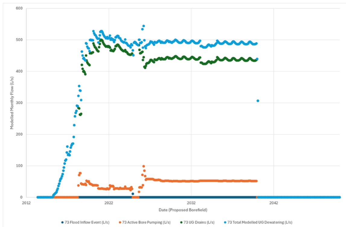
Figure 16-11: 2025 Modelled Flows with Proposed Underground Borefield
