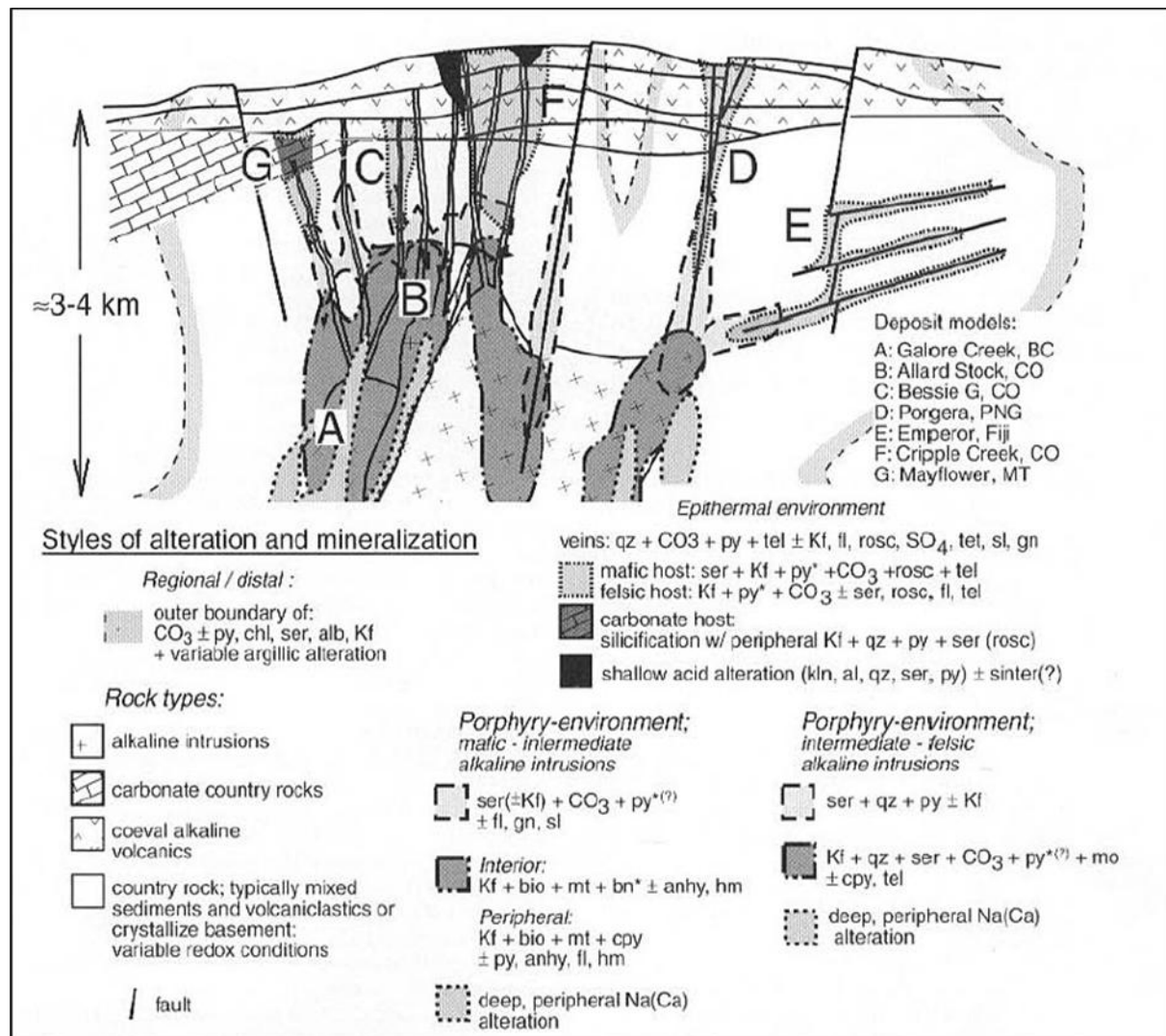
Figure 8-1: Schematic Illustration - Relationships Between Rock types
