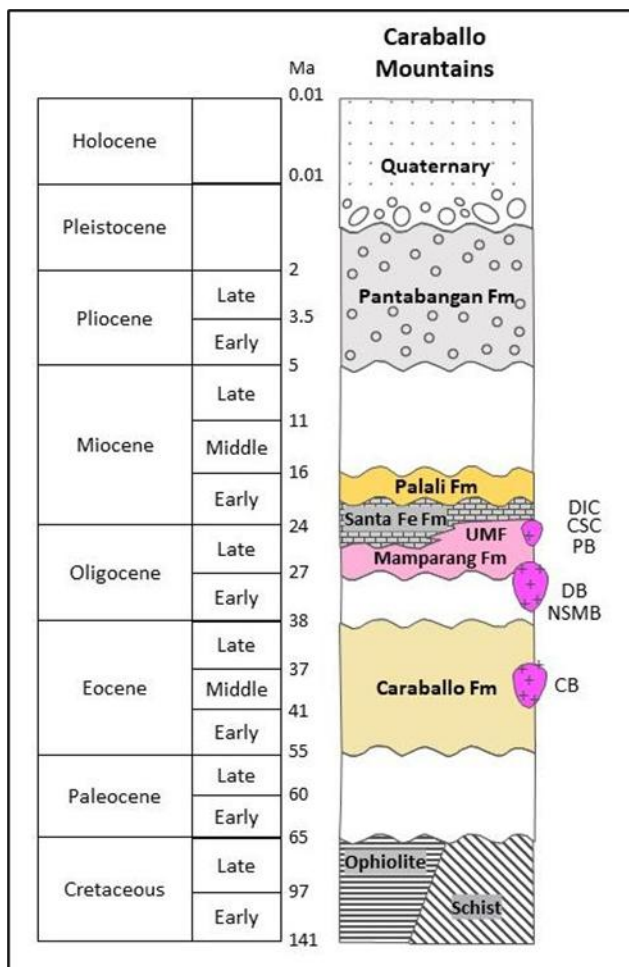
Figure 7-2: Regional Stratigraphy Caraballo Mountains
