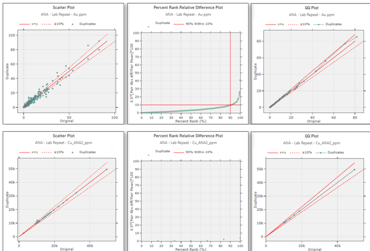
Figure 12-10: Lab Repeat Metrics for Au and Cu (Analabs Laboratory)
