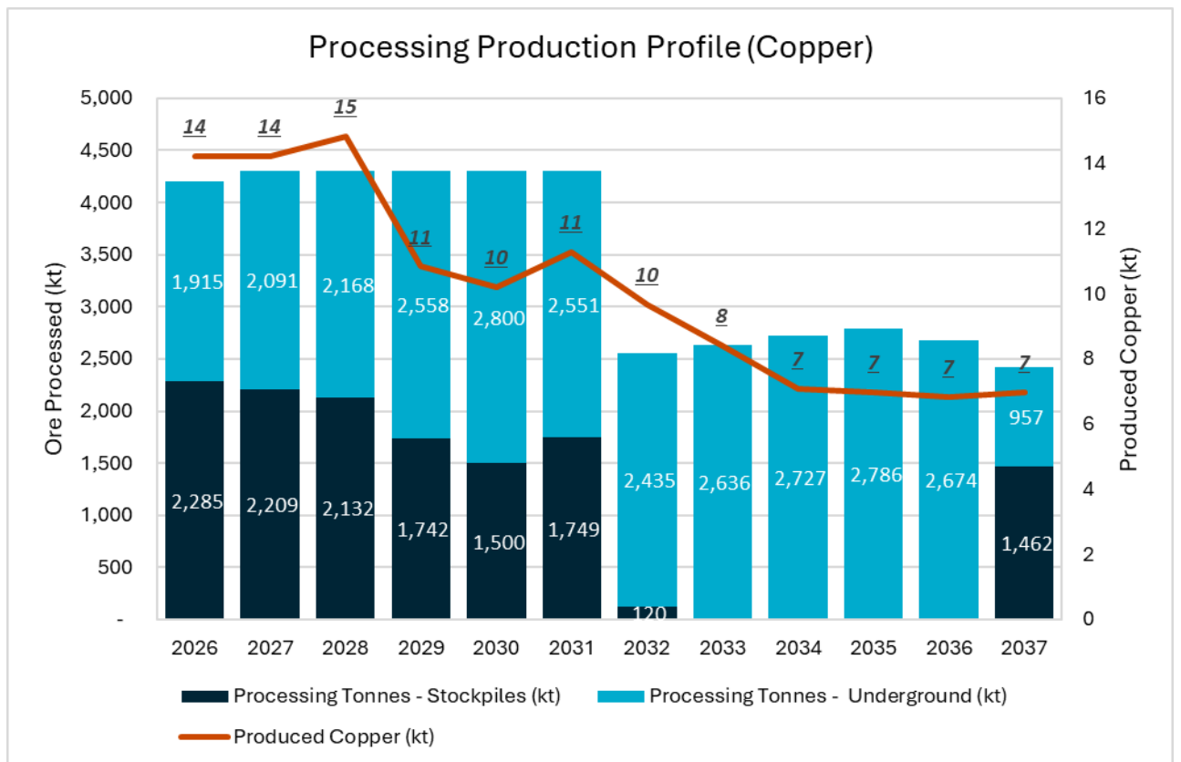
Figure 16-24: Processing Production Profile - Copper
