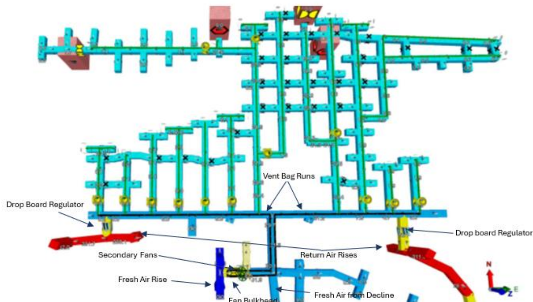
Figure 16-17: Planned Level Ventilation Layout
