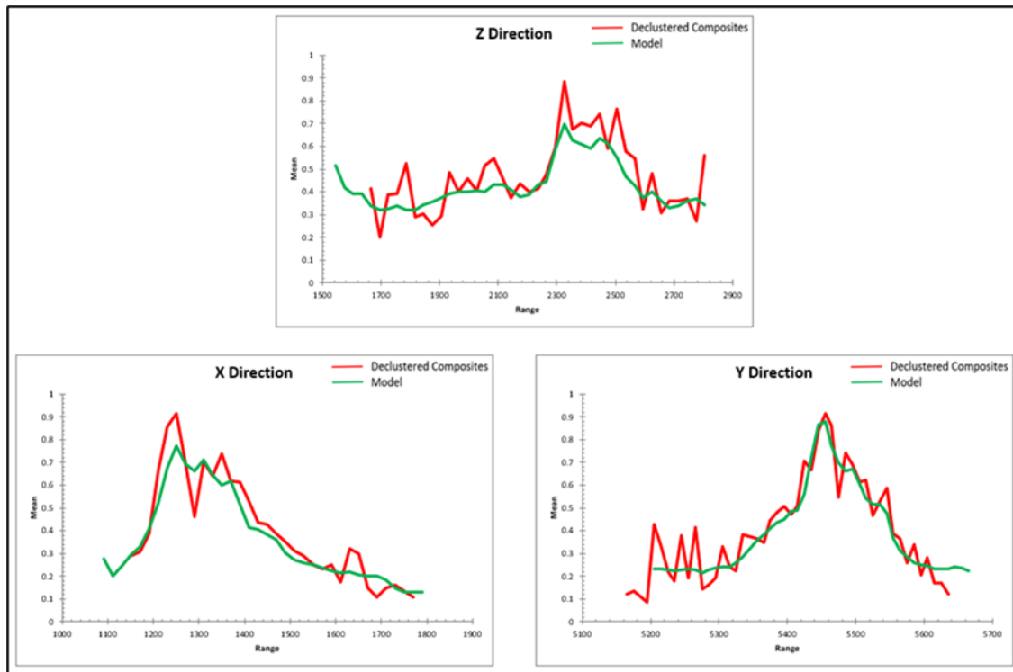
Figure 14-4: Swath Plot (audom 1)
