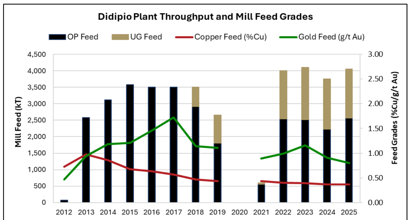
Figure 17-2: Process Plant Throughput 2012 - 2025
