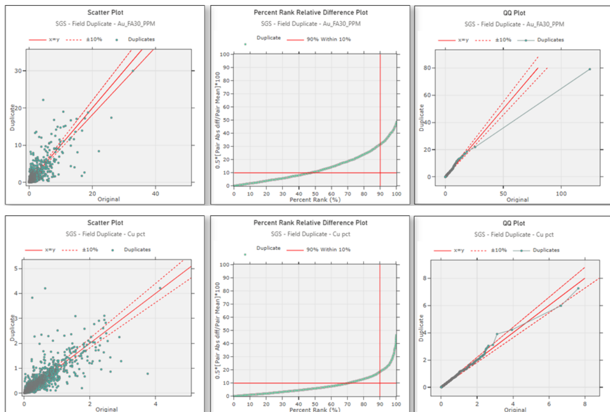
Figure 12-14: Field Duplicates for Cu and Au (SGS Laboratory)
