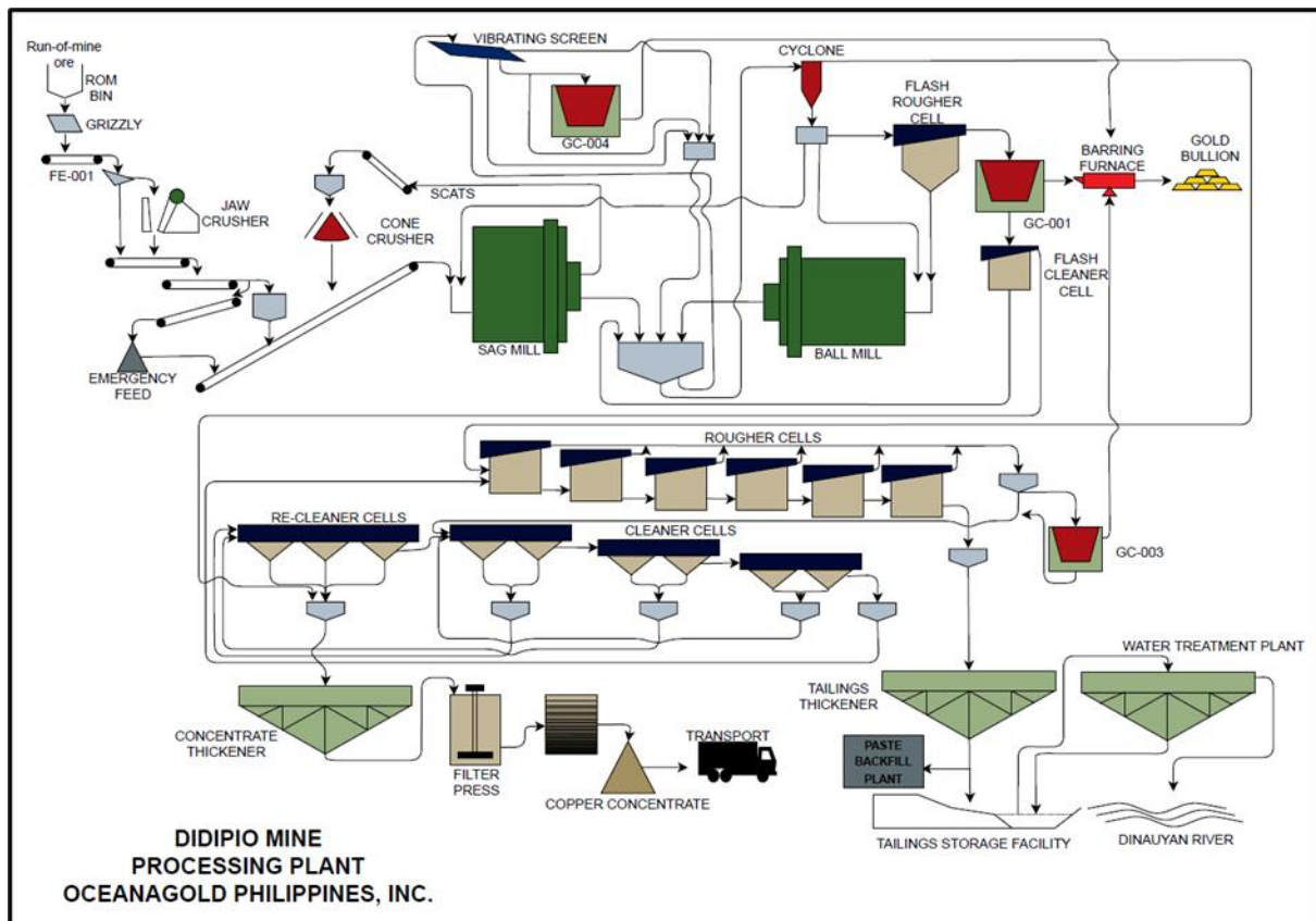
Figure 17-1: Process Plant Flowsheet 2025
