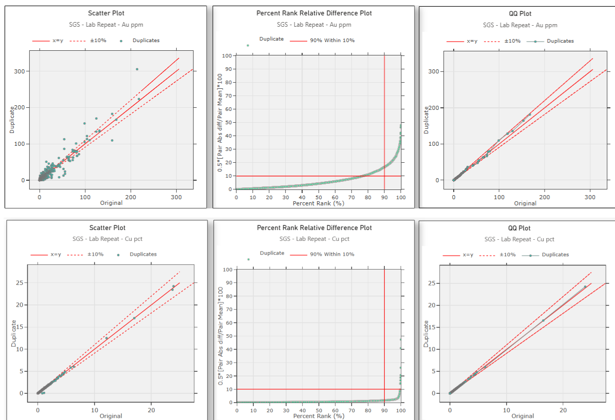
Figure 12-12: Lab Repeat Metrics for Au and Cu (SGS Laboratory)
