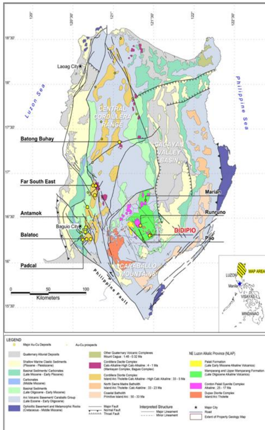
Figure 7-1: Regional Geology and Structures Northern Luzon Island
