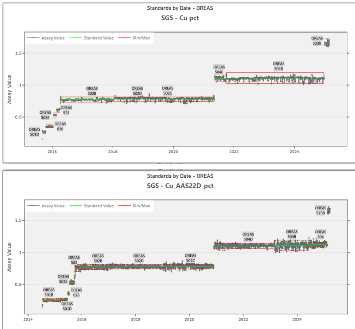
Figure 12-7: Cu Standard – SGS
