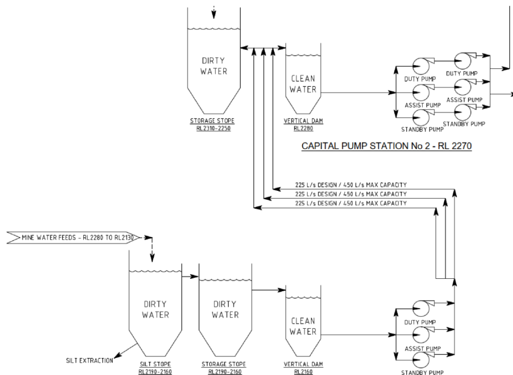
Figure 16-9: CPS1 System Flow Sheet
