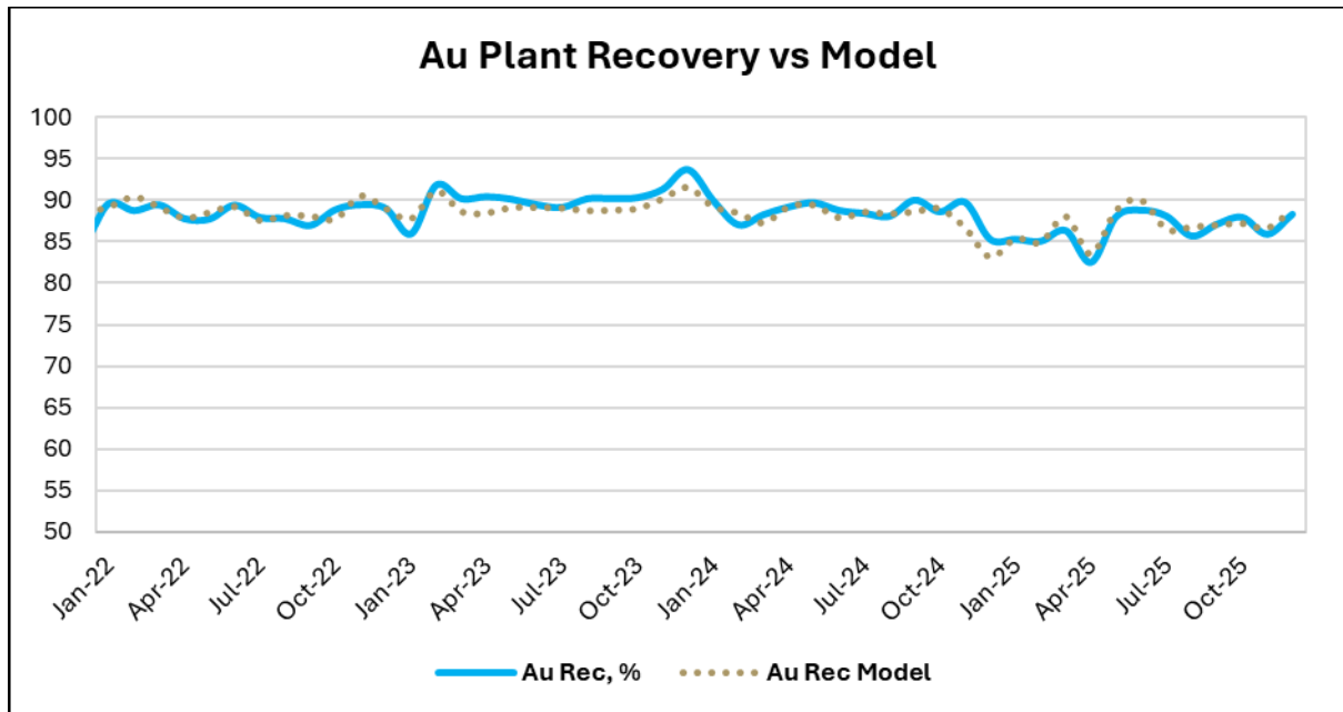
Figure 13-4: Didipio Gold Recovery vs Model
