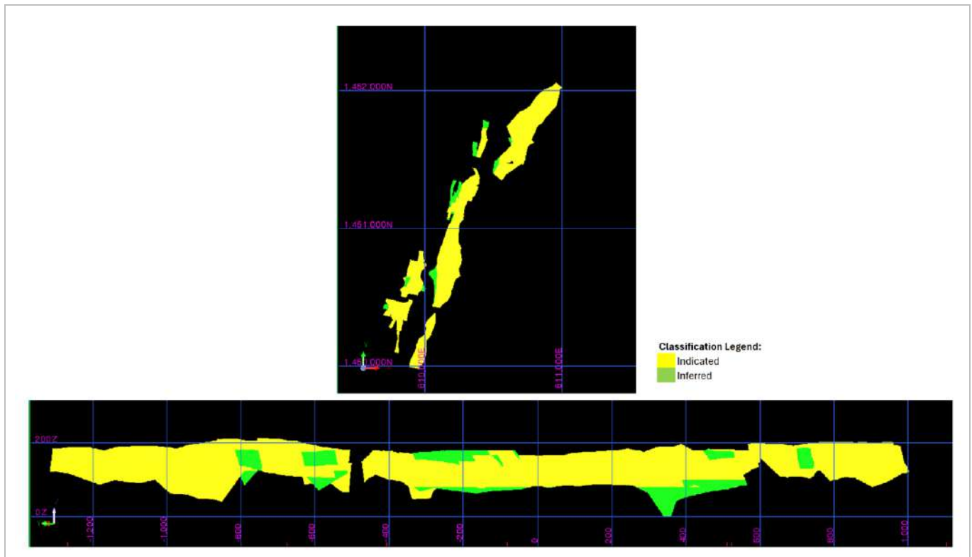
Figure 14-54: Goumbati West, Kobokoto Mineral Resource Class., N-S Long Section Looking West (EDV 2025)
