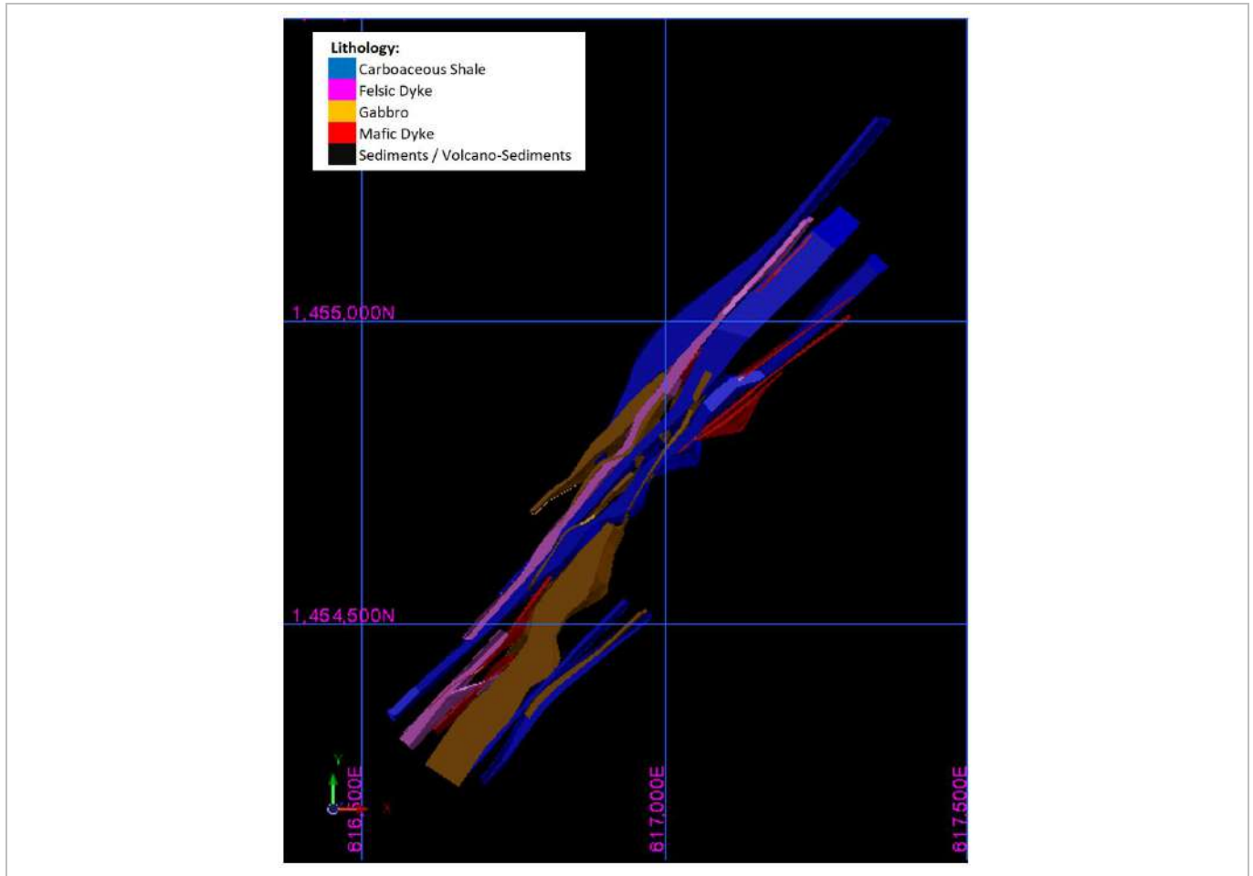
Figure 14-6: Kerekounda East Lithological Model, Plan View (EDV, 2024)
