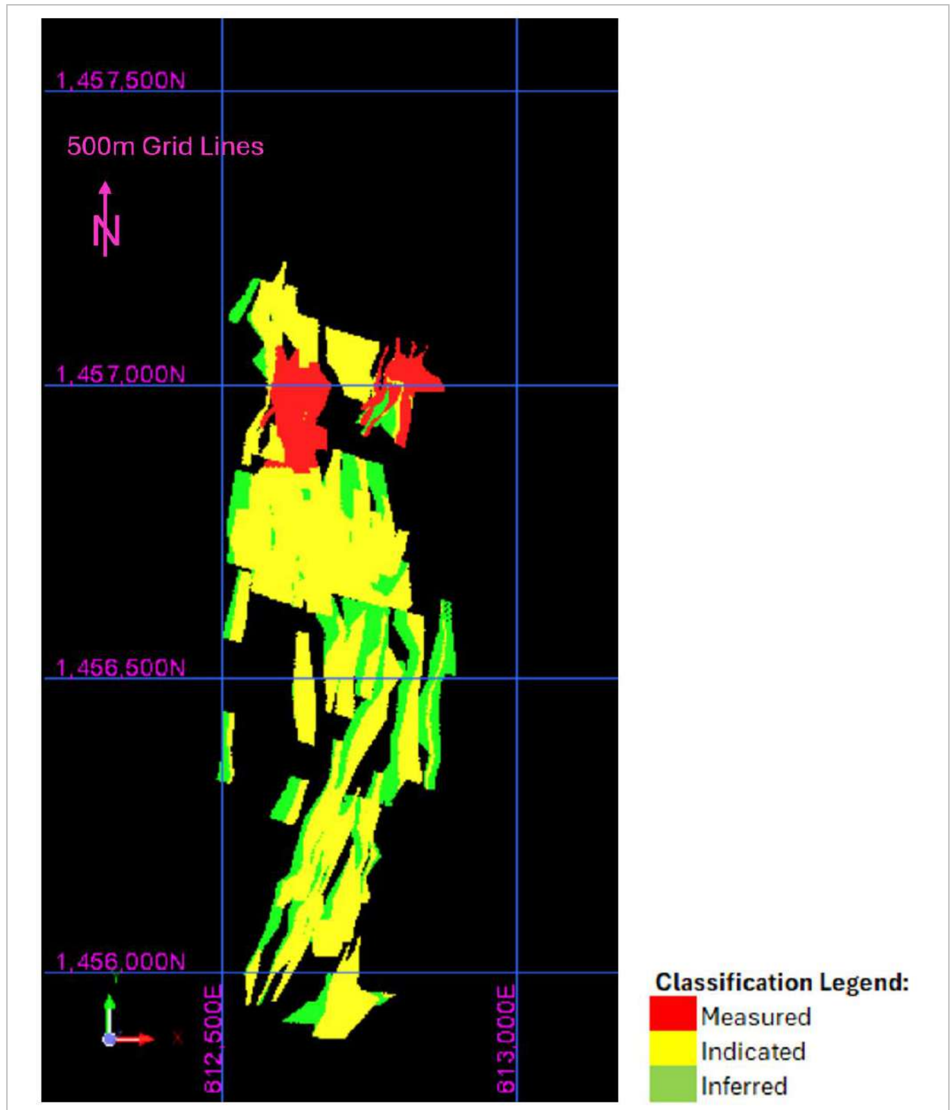
Figure 14-67: Niakafiri West Mineral Resource Classification Plan View (EDV 2025)
