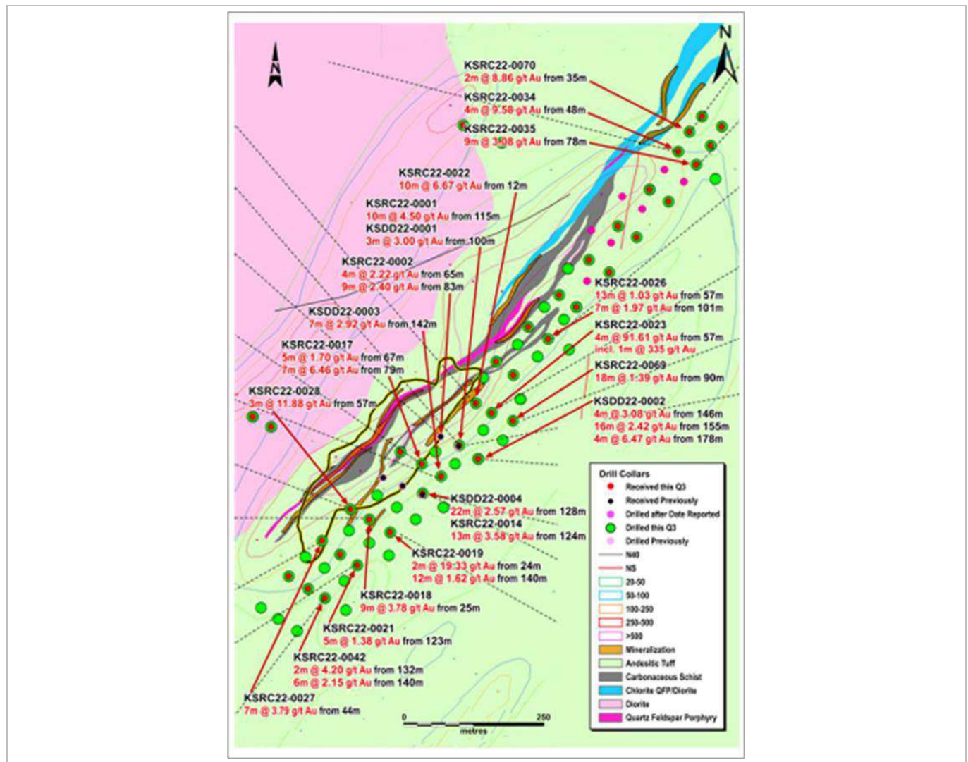
Figure 10-7: Kiesta C Drill Collar Location and Selected Assay Results
