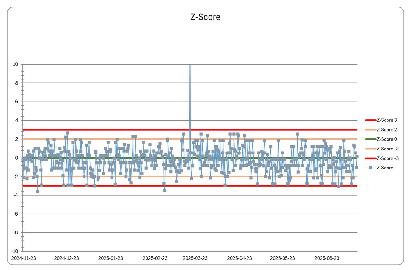
Figure 11-10: Example of a Z-Score Control Chart (ALSSB, Sabodala, all CRMs)
