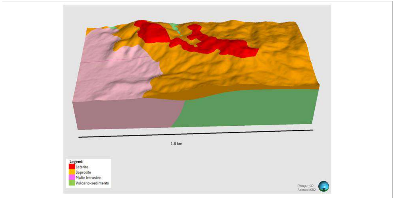
Figure 14-10: Mamasato Isometric Lithological Model Looking North (EDV, 2024)
