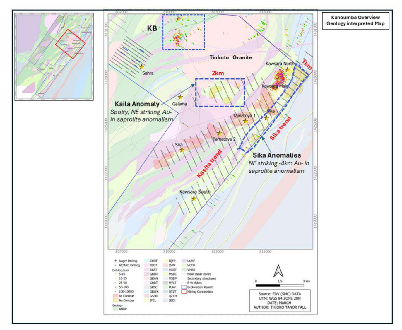
Figure 9-4: Kanoumba Geology and Exploration Activities (2022 -2025)
