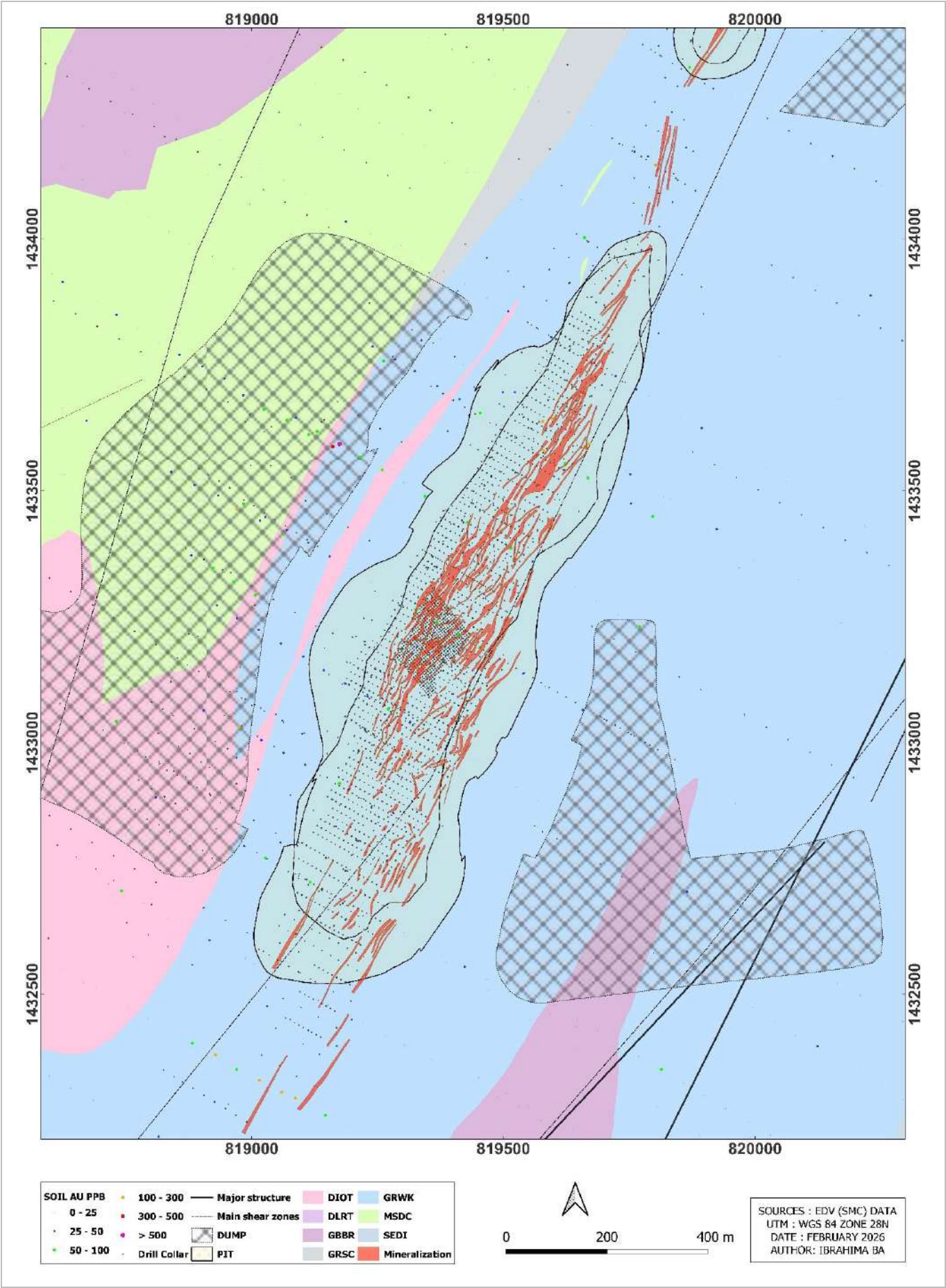
Figure 7-14: MCZ Geological Map with Mineralised Zones (EDV, 2025a)
