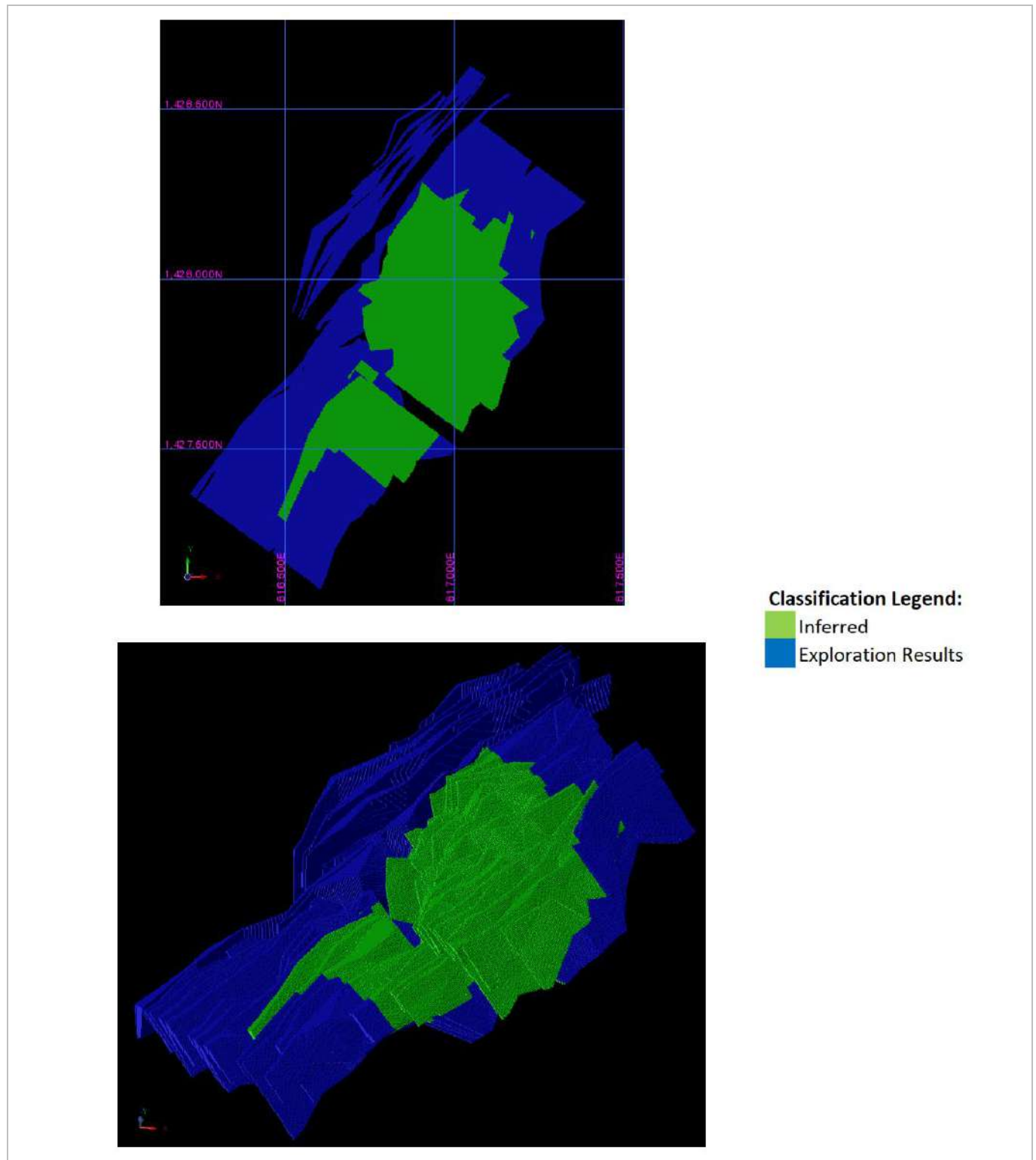
Figure 14-55: Kawsara Mineral Resource Classification Plan View and Oblique View Looking North (EDV 2025)
