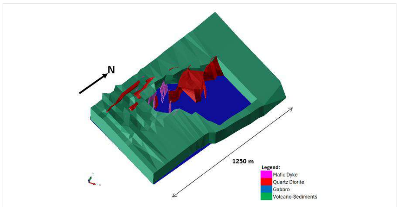
Figure 14-8: Makana 1 Lithological Model, Oblique View (EDV, 2025)
