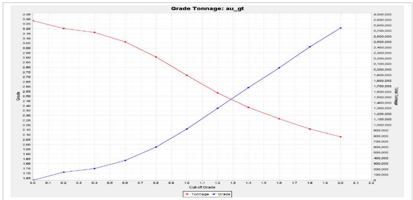
Figure 14-96: Makana 1 Grade-Tonnage Curve Within USD 2100/oz Whittle Pit (EDV 2025)
