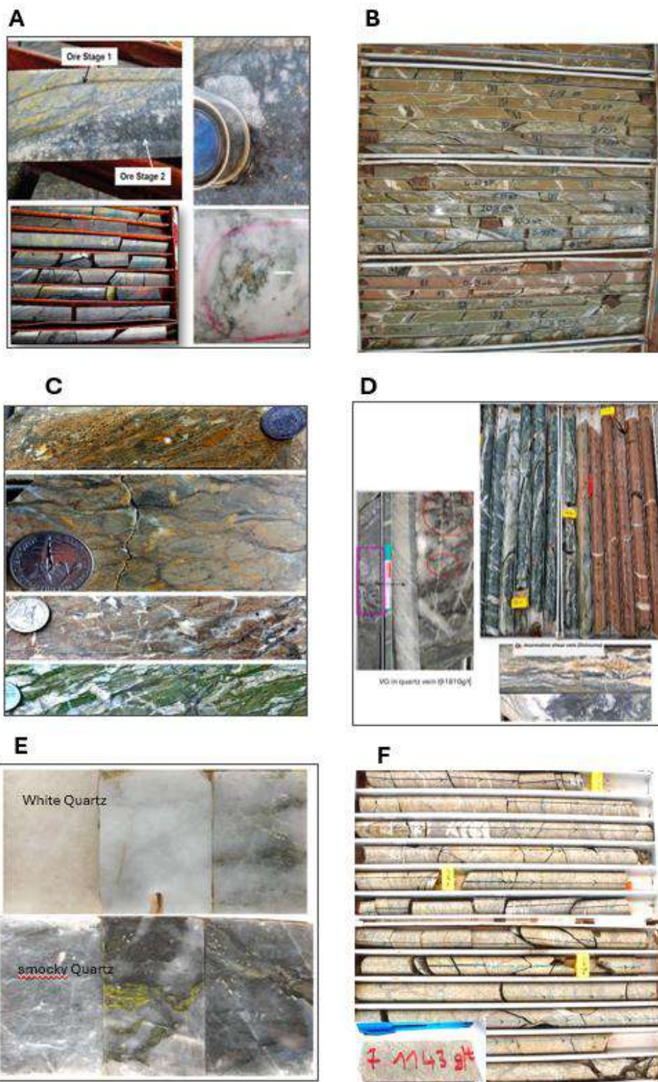
Figure 7-15: Core Photos Showing Alteration & Mineralisation Styles (EDV, 2025a)
