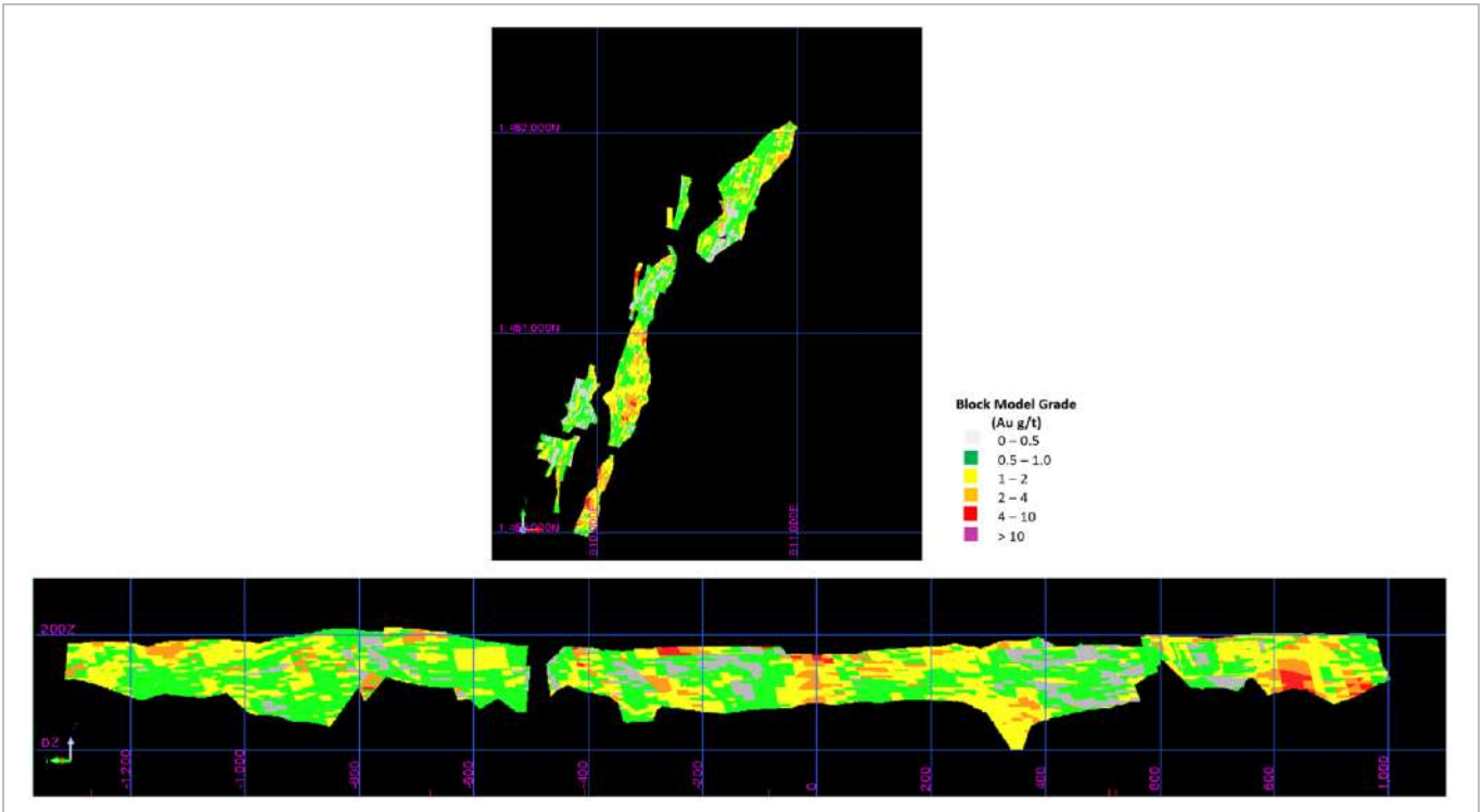
Figure 14-72: Goumbati West - Kobokoto Grade Block Model Plan and Long Section Views (EDV 2025)
