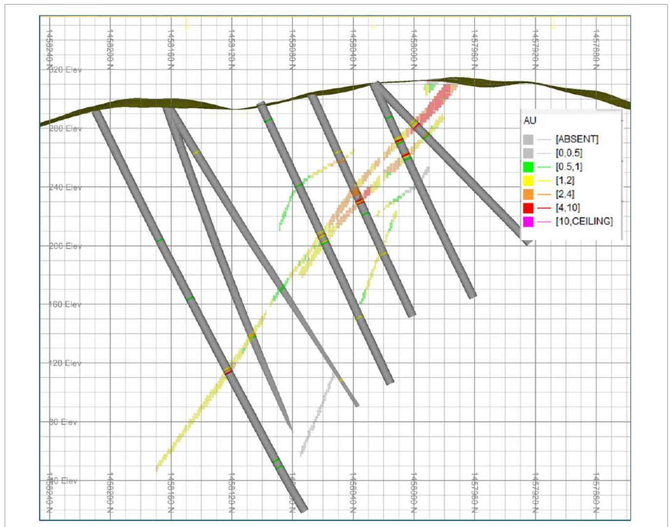
Figure 14-46: Example of Visual Validation at Golouma (EDV 2025)
