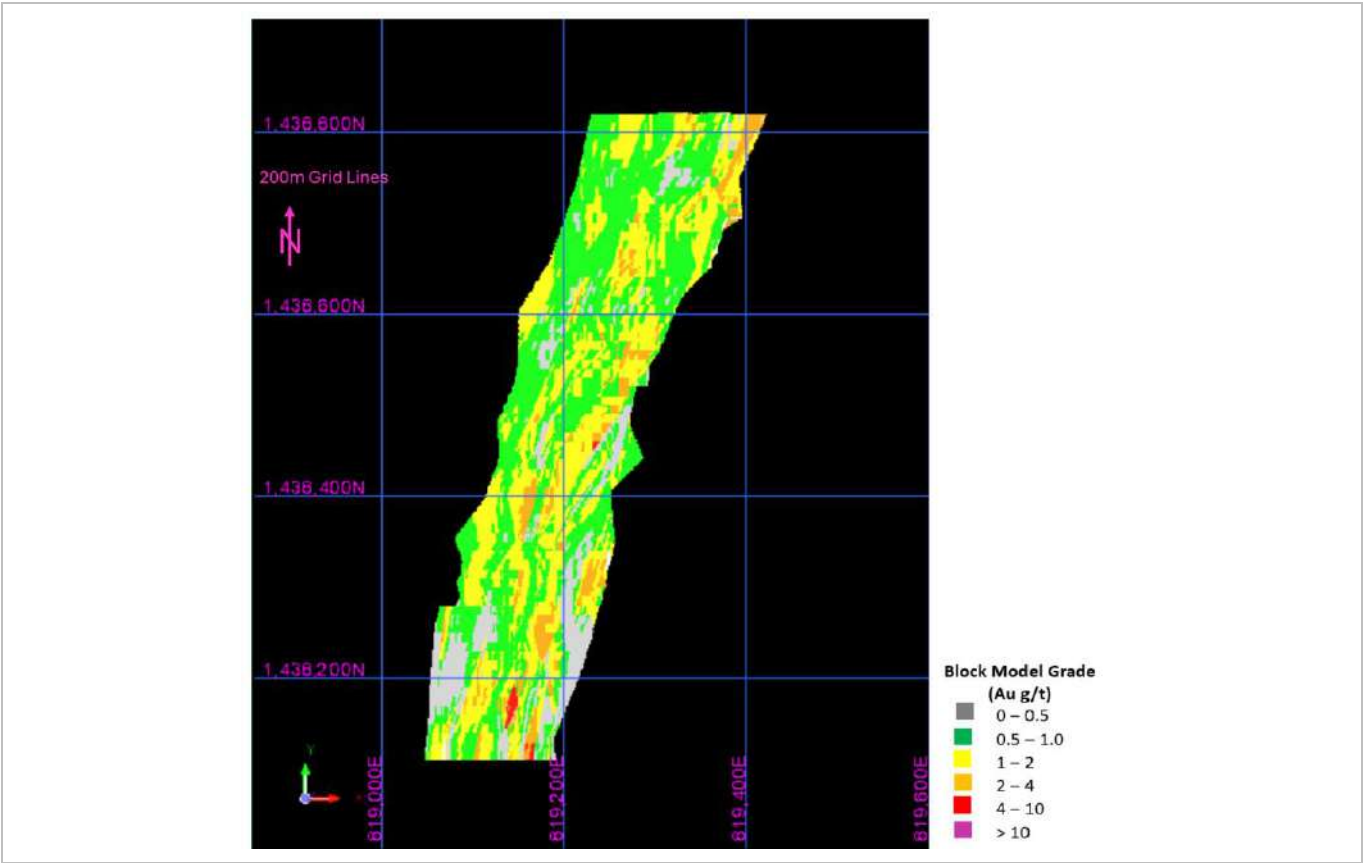
Figure 14-87: Tina Grade Block Model Plan View (EDV 2025)
