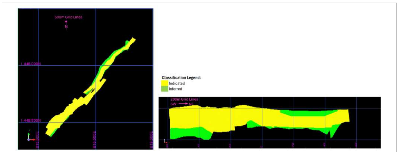
Figure 14-59: Kiesta C Mineral Resource Classification in Plan & SW-NE Long Section Looking NW (EDV 2025)
