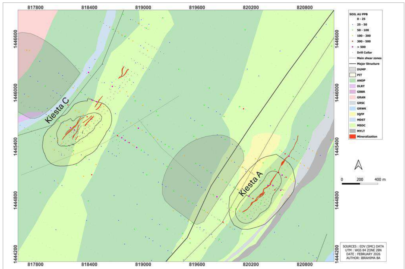
Figure 7-13: Kiesta Geology and Deposits (EDV, 2025a)
