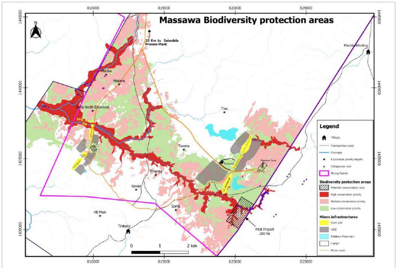
Figure 20-3: Chimpanzee habitats, nests and evidence of presence
