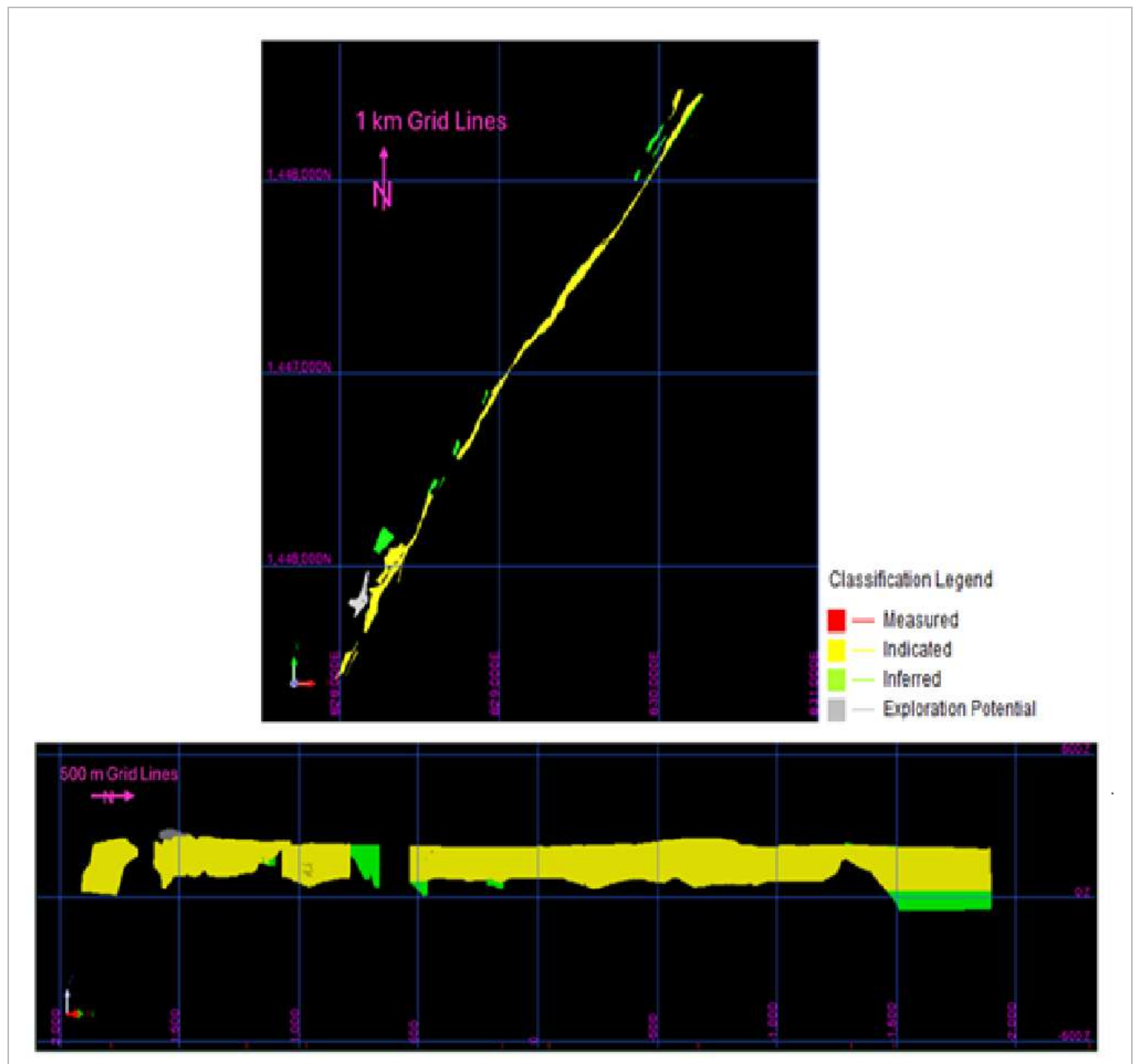
Figure 14-52: Delya-Samina Classification in Plan and S-N Long Section looking West Views (EDV 2025)
