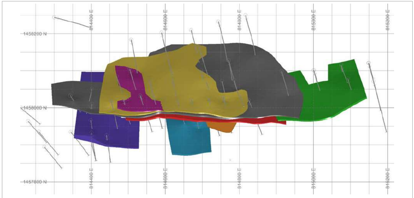
Figure 14-27: Mamasato Mineralisation, Plan View (EDV, 2025)
