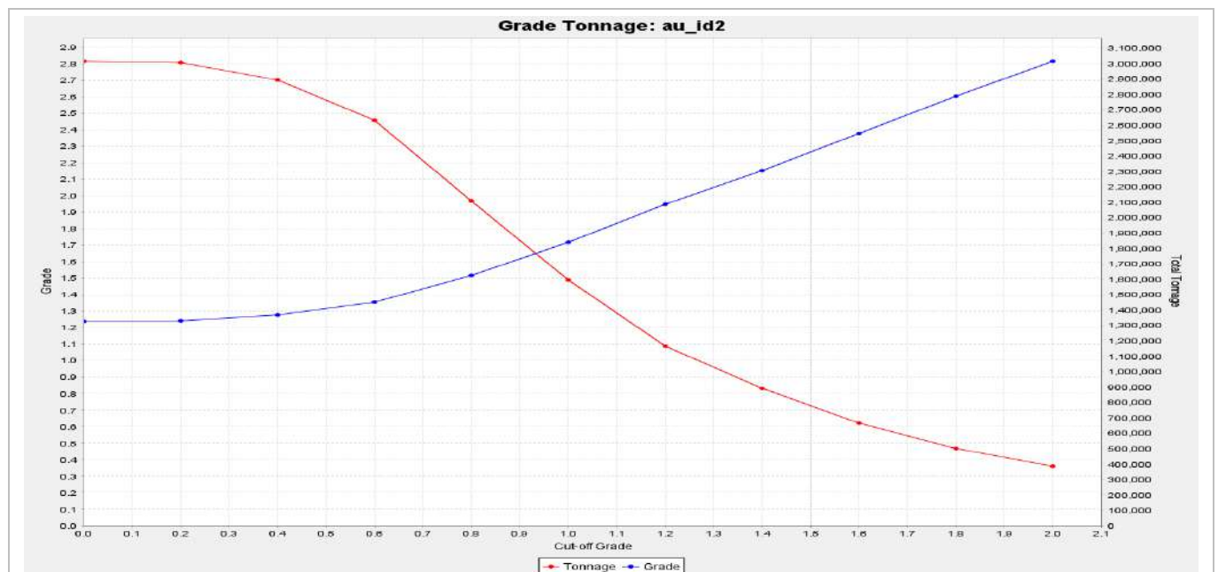
Figure 14-90: Goumbati West, Kobokoto Grade-Tonnage Curve Within USD 2100 Pit Shell (EDV 2025)
