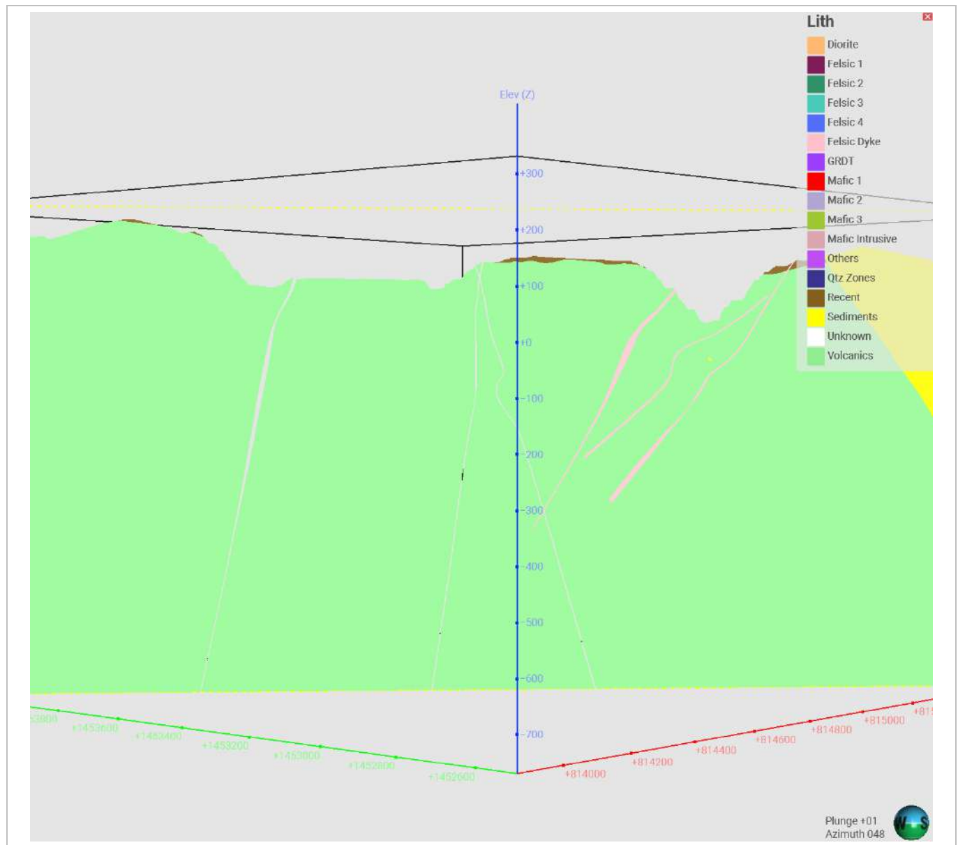
Figure 14-4: Golouma Lithological Model Cross Section (EDV, 2025)
