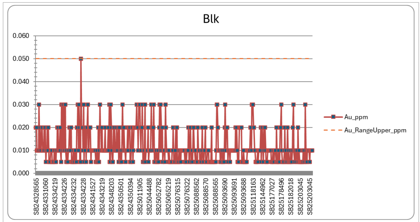
Figure 11-5: Example of a Blank Control Chart (ALSSB, Sabodala)
