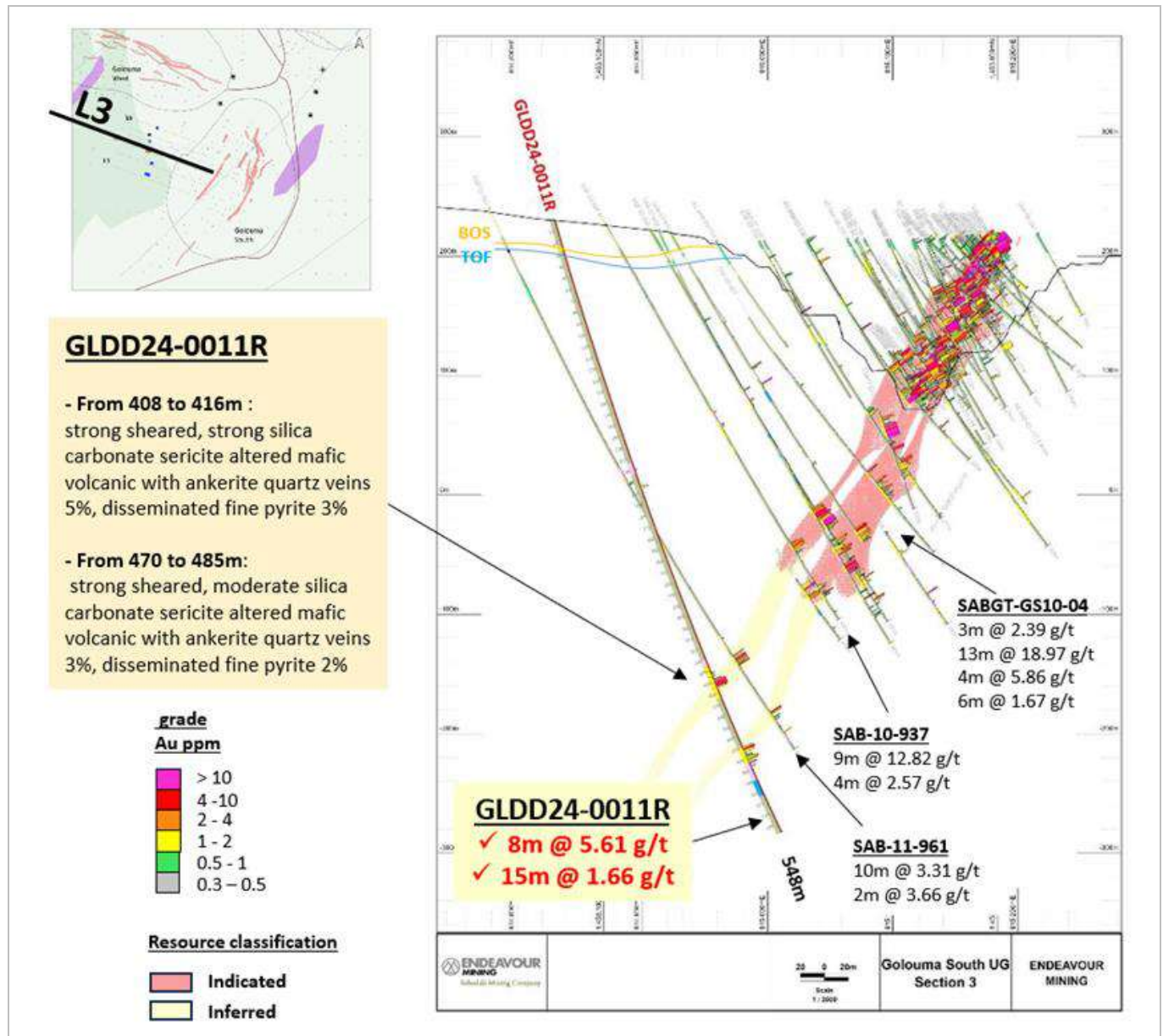
Figure 10-5: Golouma South UG Section Line 3 Drilling Results
