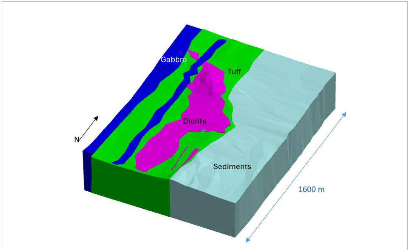
Figure 14-5: Kawsara Lithological Model Schematic (EDV, 2024)
