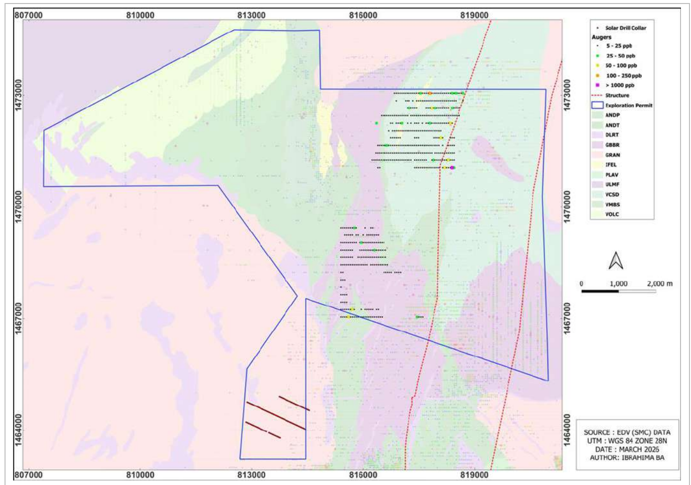
Figure 9-6: Bransan Lot A Geology and Auger Drilling 2024-2025
