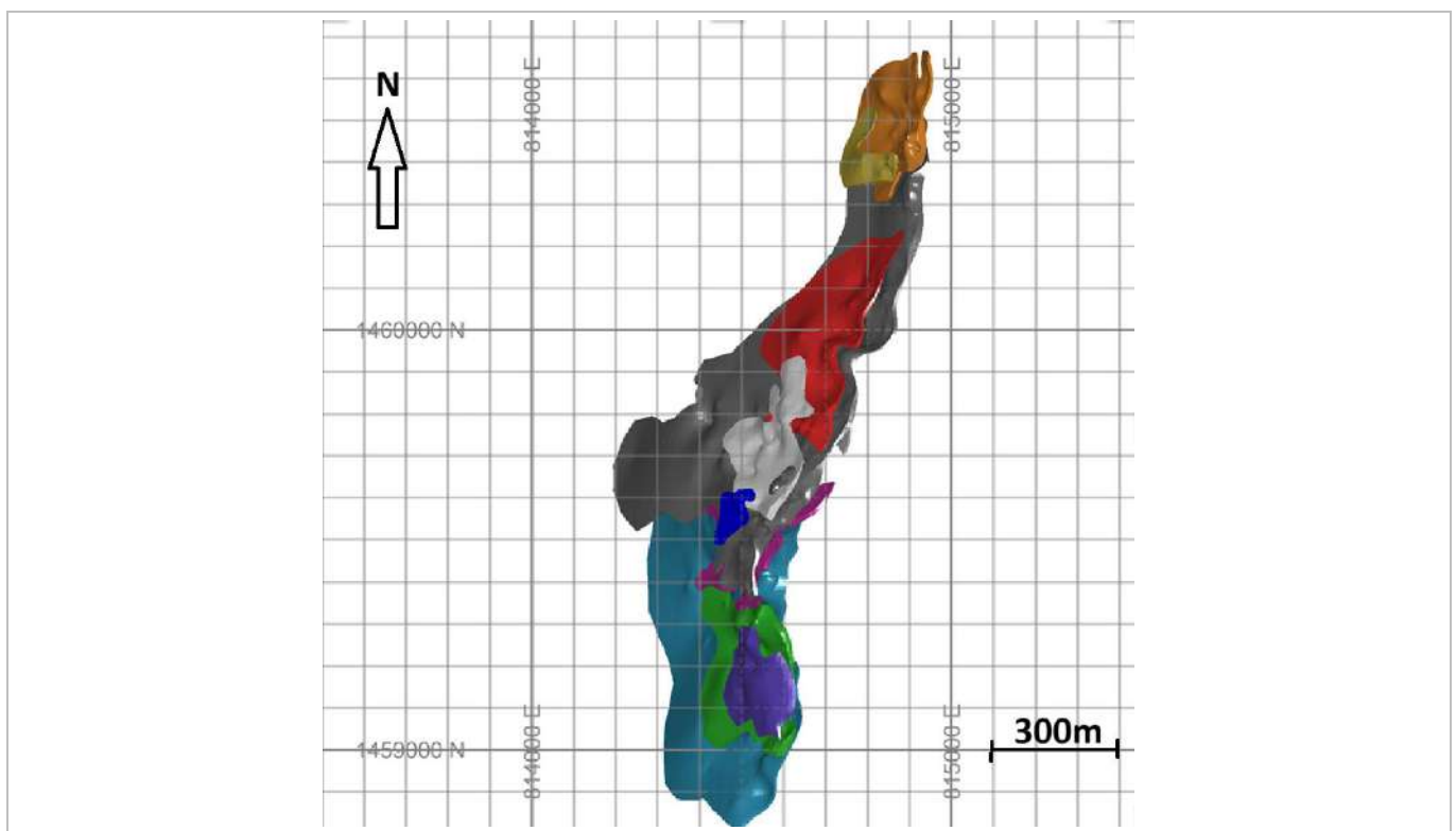
Figure 14-28: Masato Mineralisation, Plan View (EDV, 2022)
