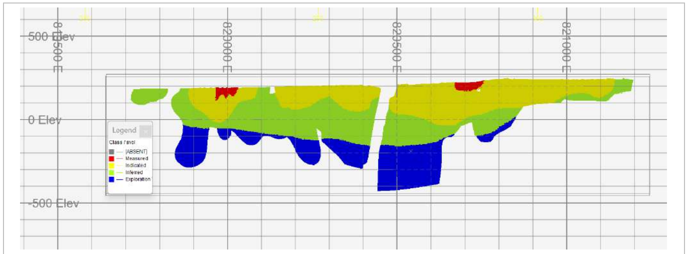
Figure 14-65: Massawa North Zone Mineral Resource Classification (EDV2025)
