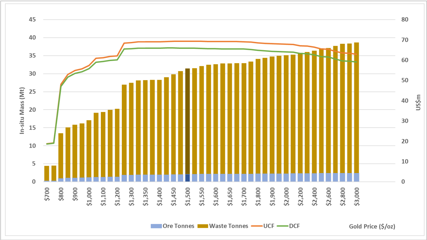
Figure 15-4: Kiesta Zone A (KIA) Optimisation Results
