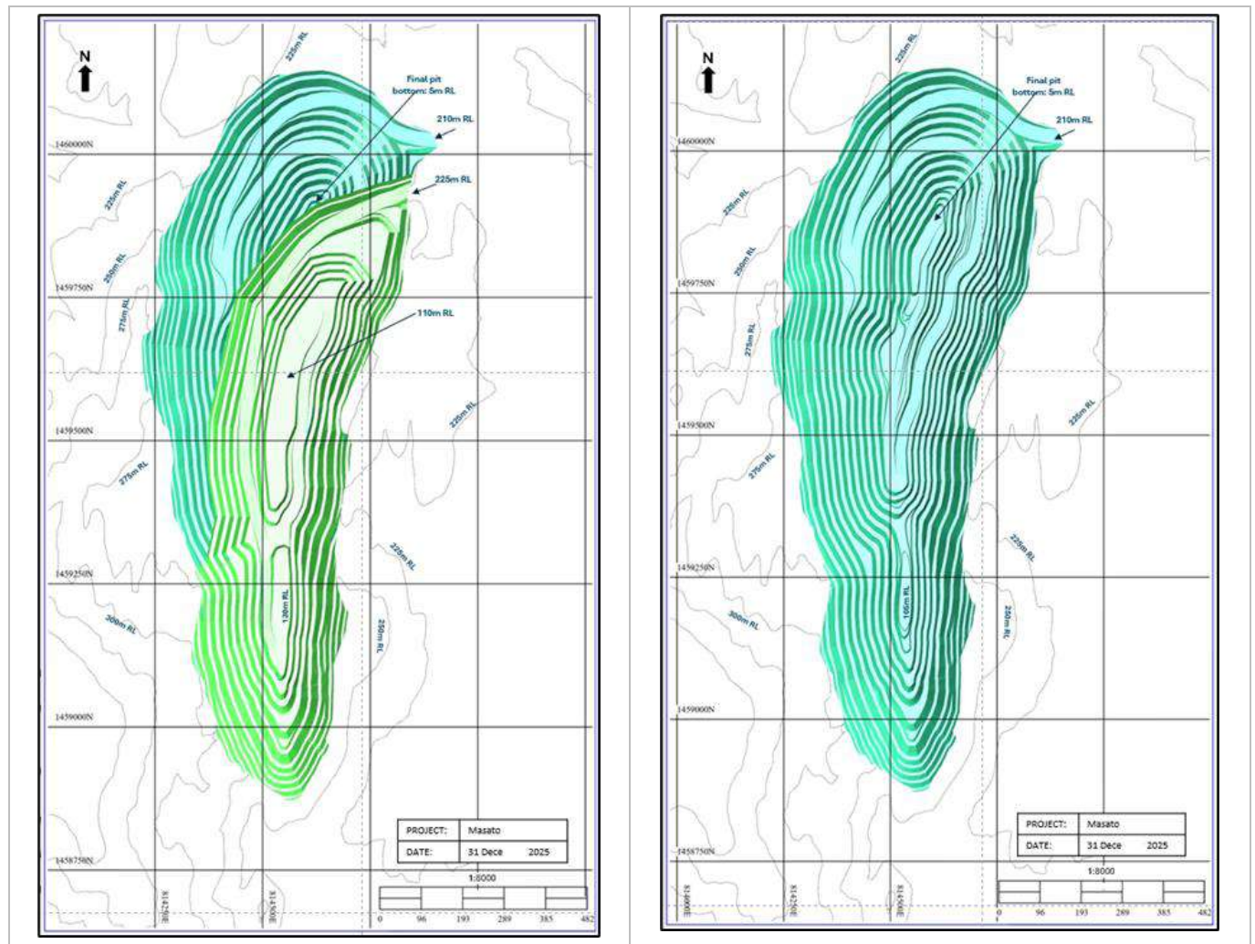
Figure 15-14: Masato Pit Design in Two Stages and Final Pit (EDV, 2025)
