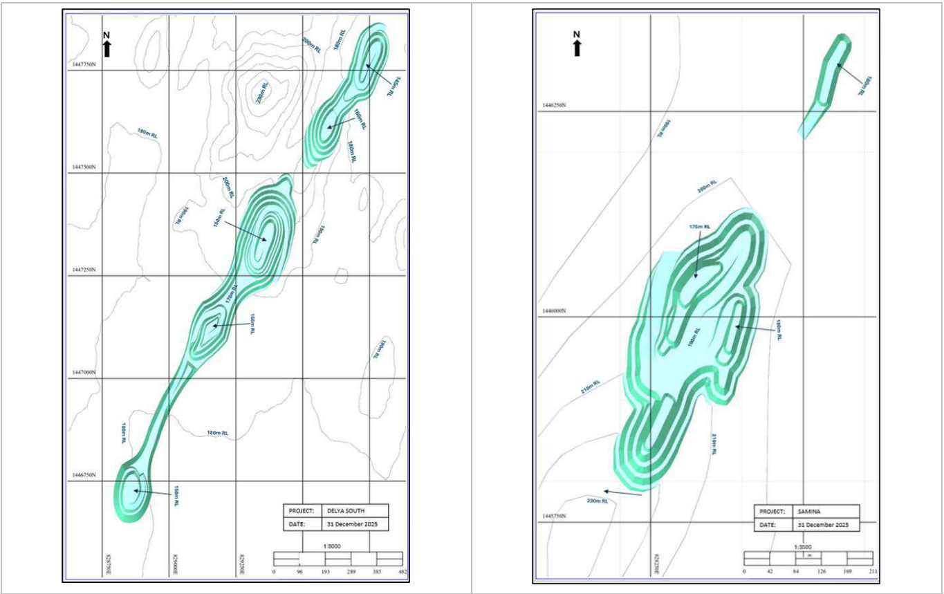
Figure 15-26: Delya South Pit Designs (EDV, 2025)
