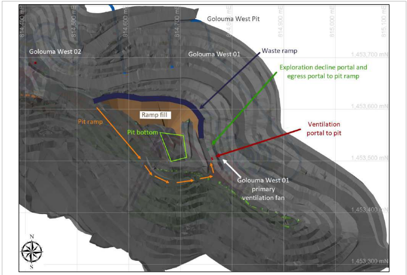
Figure 15-28: Golouma West 01 Access Portals
