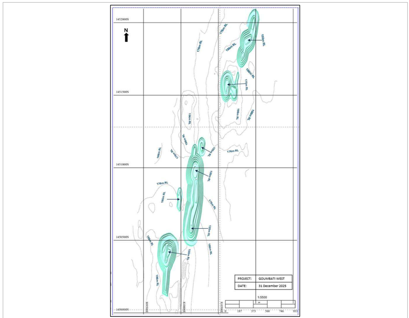
Figure 15-21: Goumbati West Pit Designs (EDV, 2025)
