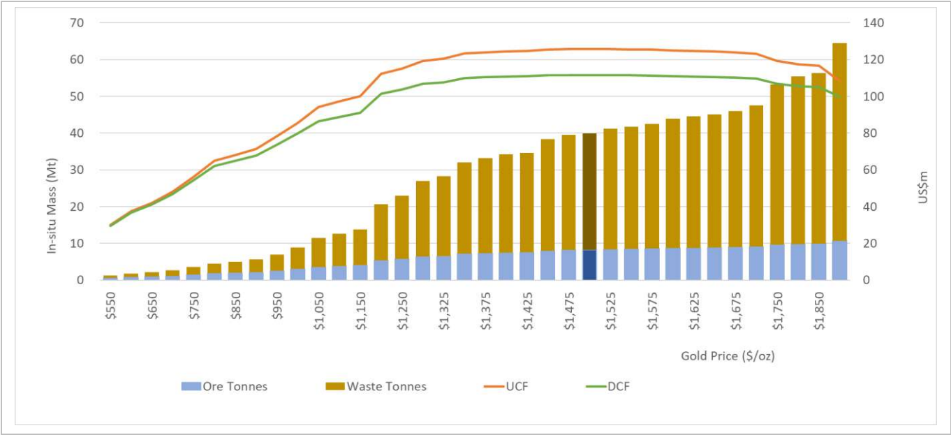
Figure 15-7: Niakifiri East Optimisation Results
