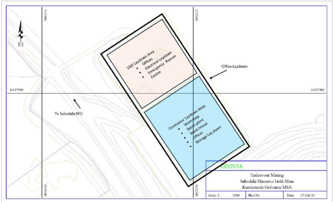
Figure 18-15: K&G UG MSA Area
