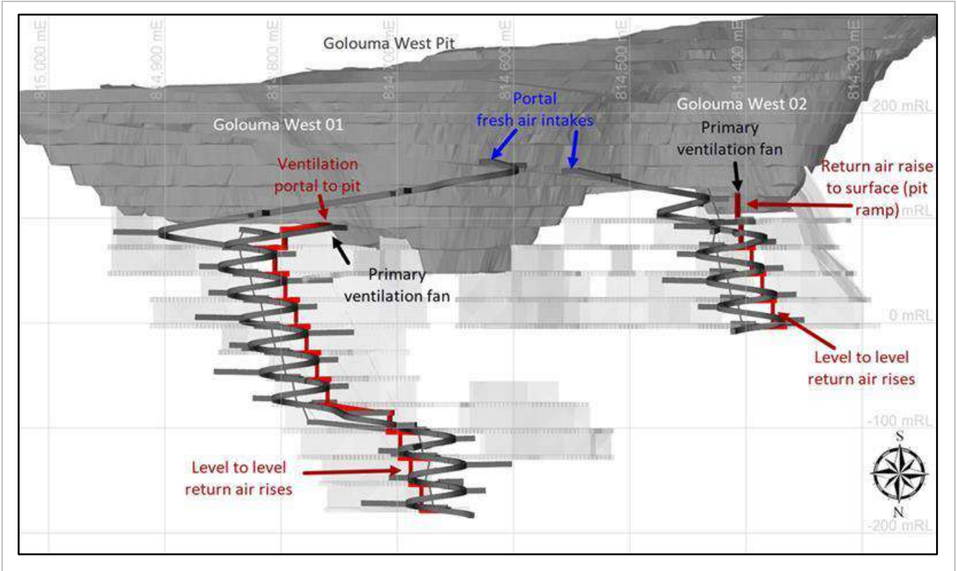
Figure 16-7: Golouma West 01 and 02 Primary Ventilation System Schematic
