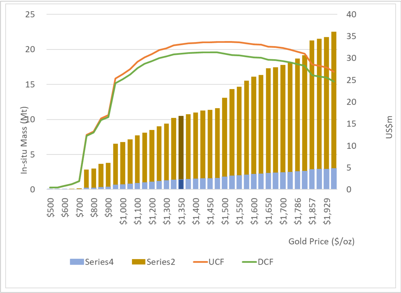
Figure 15-8: Niakifiri West Optimisation Results
