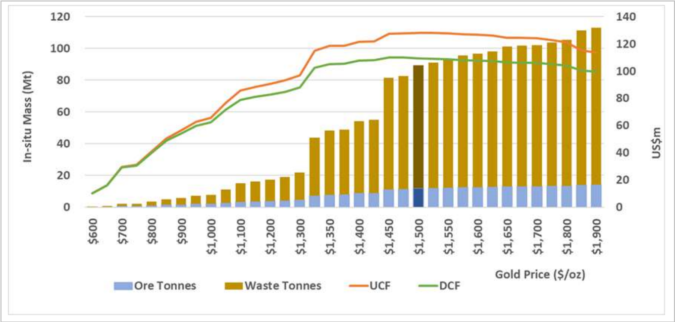
Figure 15-3: Masato (MAS) Optimisation Results
