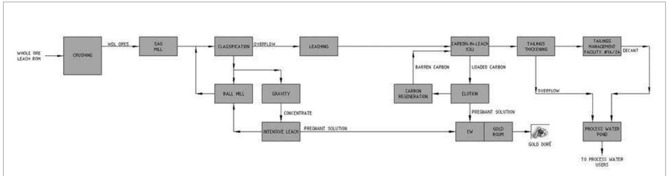
Figure 17-1: SWOLP Block Flow Diagram (BFD)
