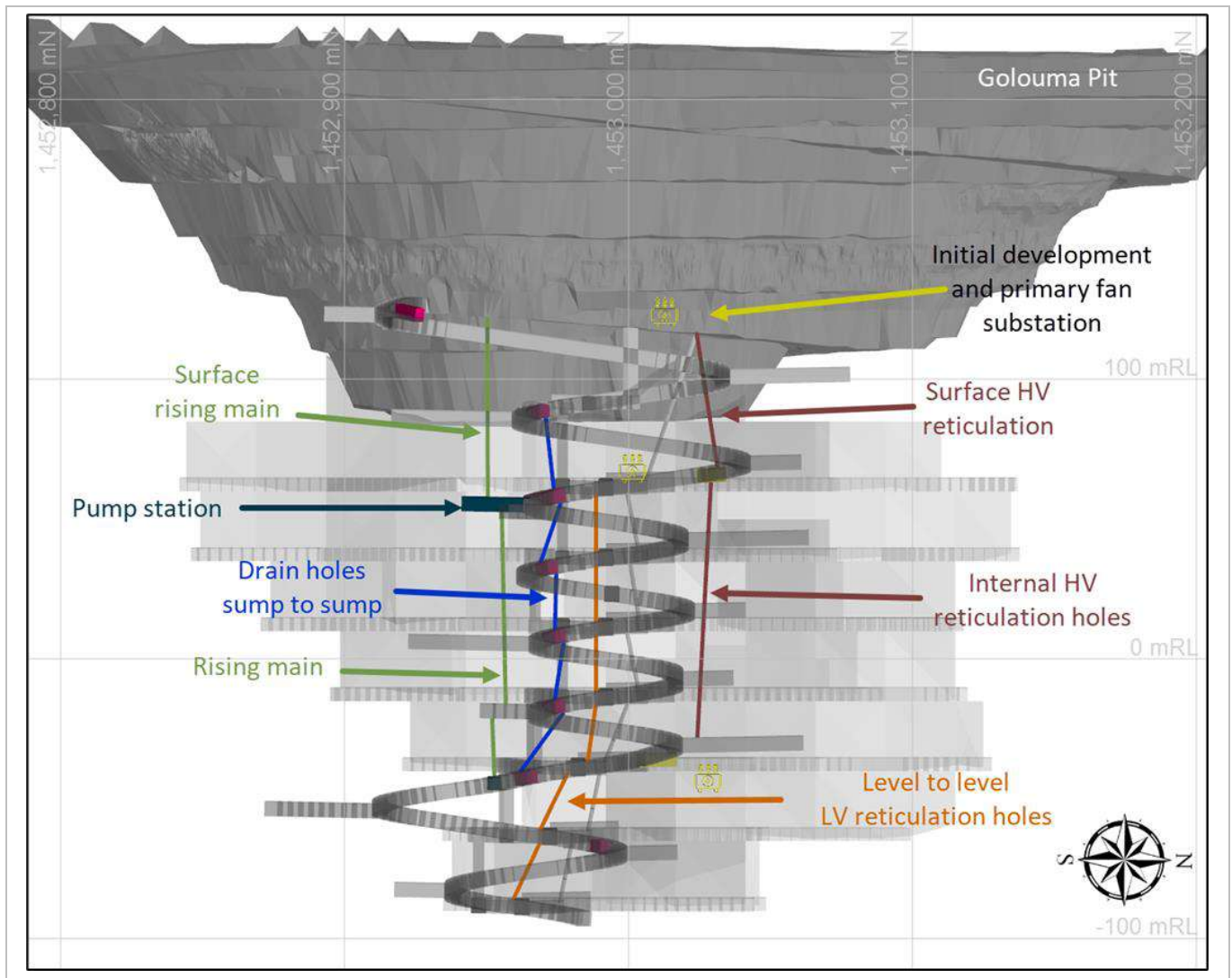
Figure 16-14: Golouma South Mine Services System Schematic
