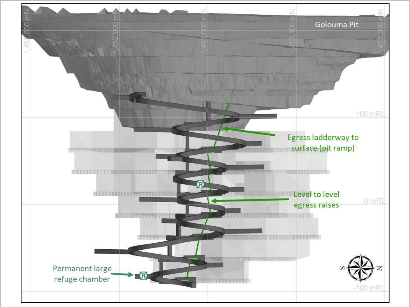
Figure 16-9: Kerekounda Egress System Schematic
