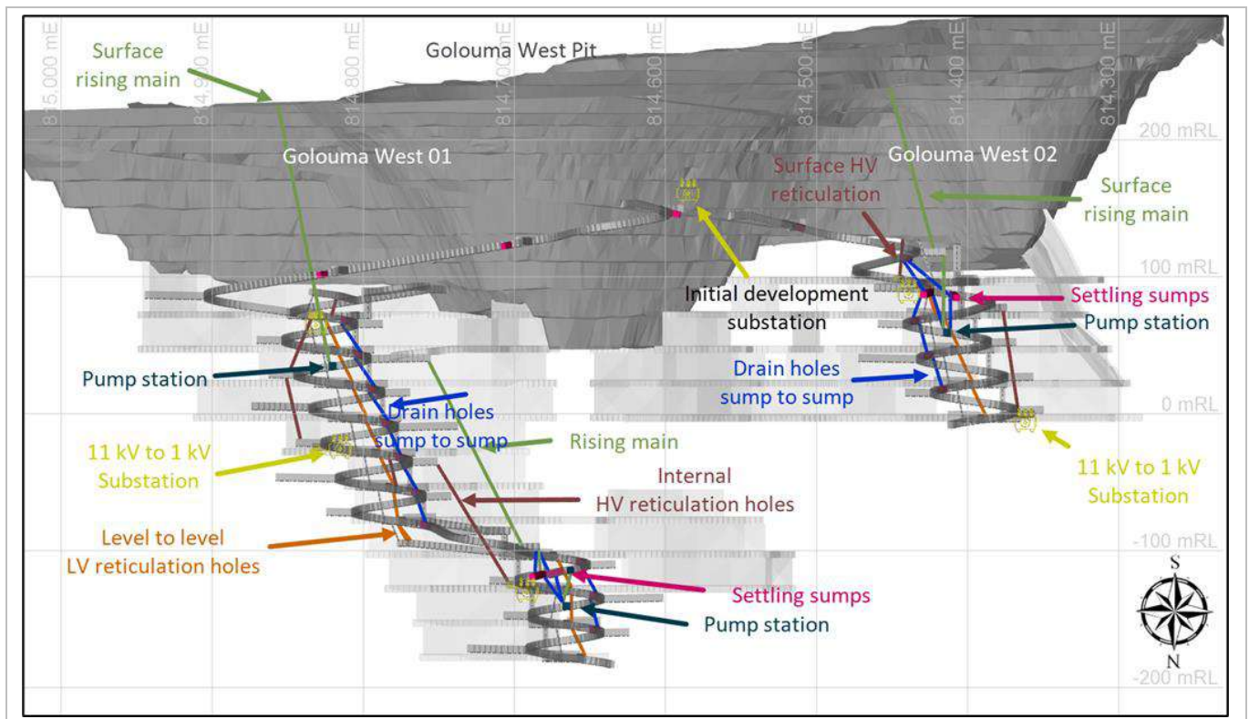
Figure 16-13: Golouma West 01 and 02 Mine Services System Schematic
