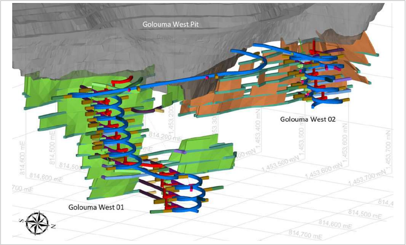
Figure 16-16: Golouma West 01 and 02 Underground Mineral Reserve Design
