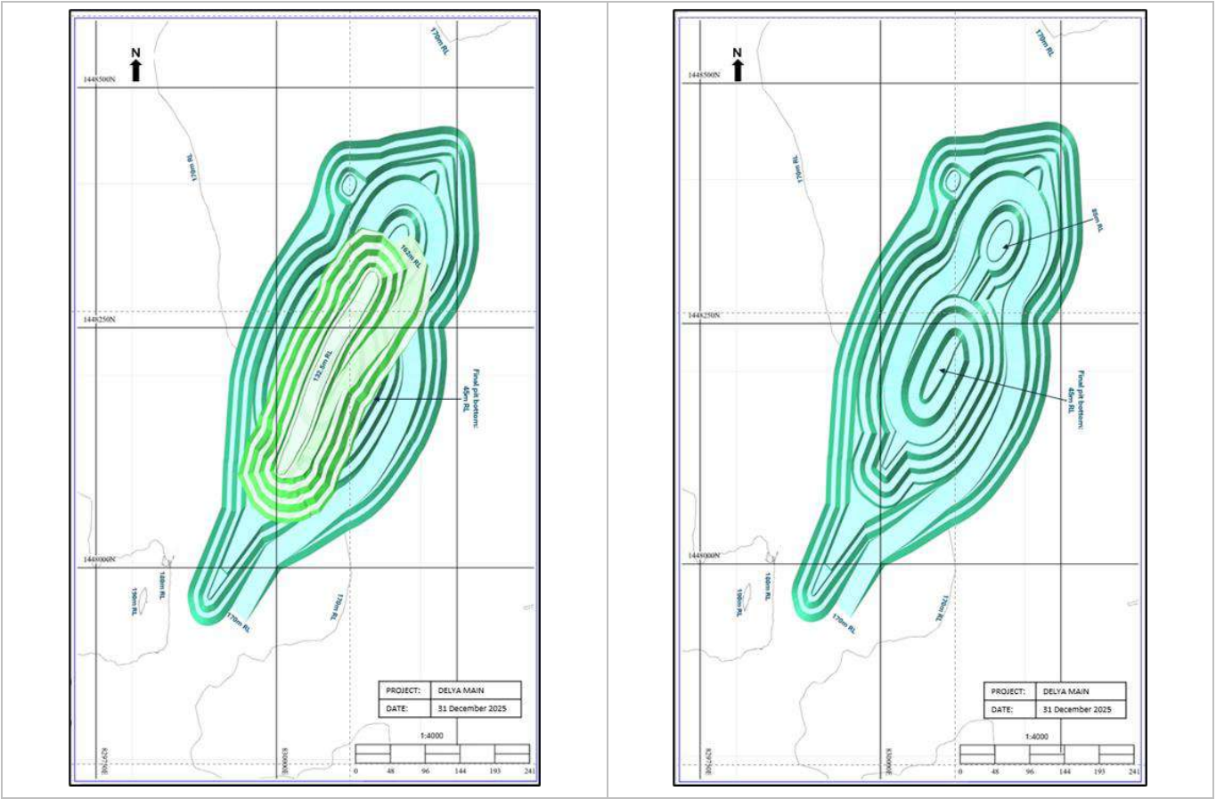
Figure 15-25: Delya Main Stage and Final Pit Designs (EDV, 2025)
