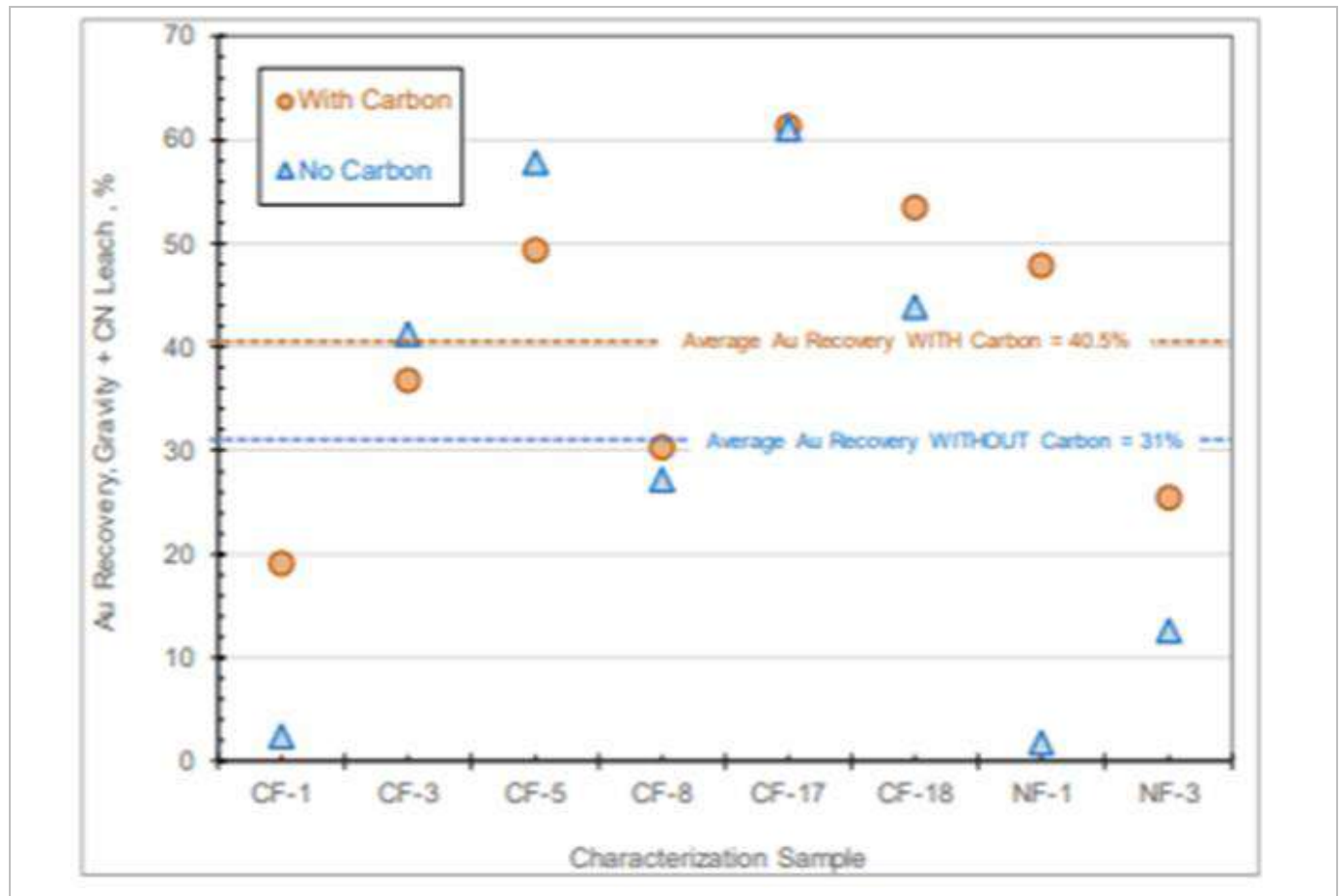
Figure 13-11: 2020 SGS Phase 1 Massawa Direct Leaching versus CIL for 6 MCZ and 2 MNZ Samples
