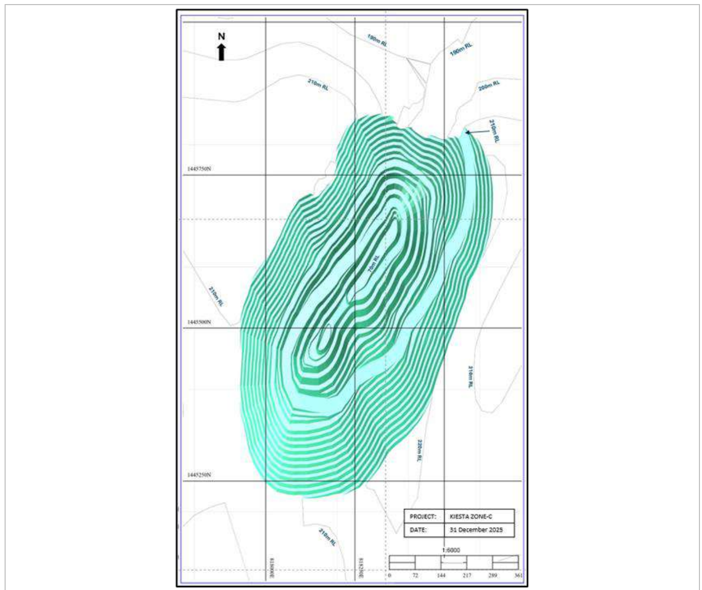
Figure 15-16: Kiesta C Pit Designs with a Stage & Final Pit (EDV, 2025)
