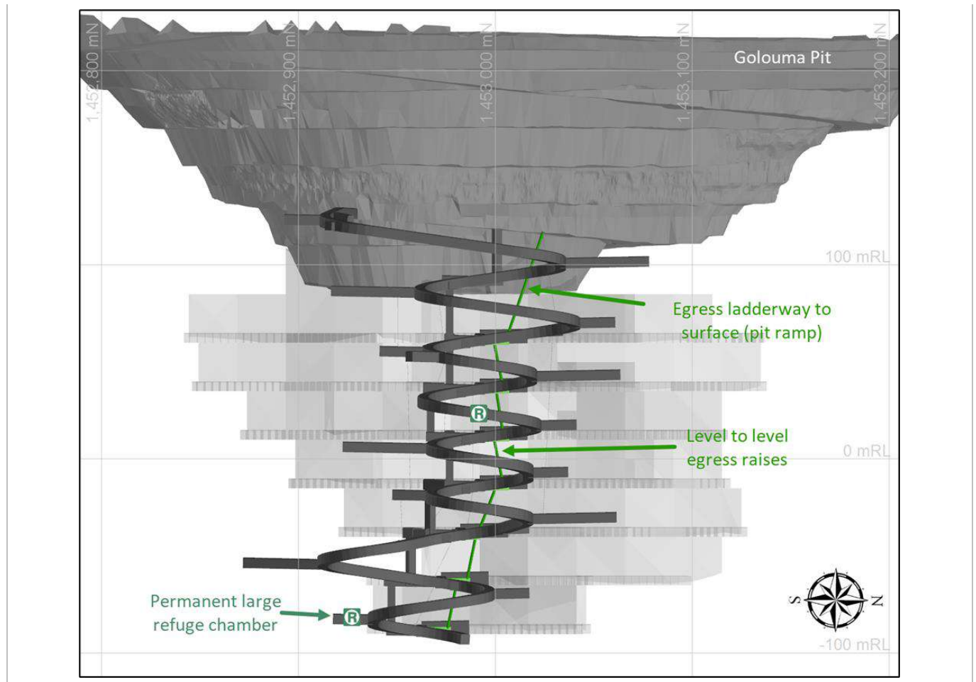
Figure 16-11: Golouma South Egress System Schematic
