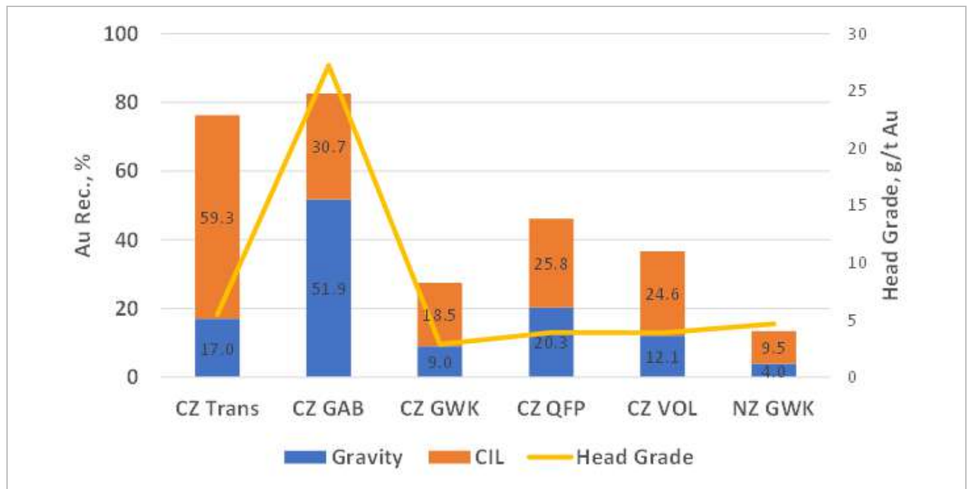
Figure 13-10: Phase 2 Massawa Avg. Sample Variability Gravity/CIL Recoveries by Lithology (2020)
