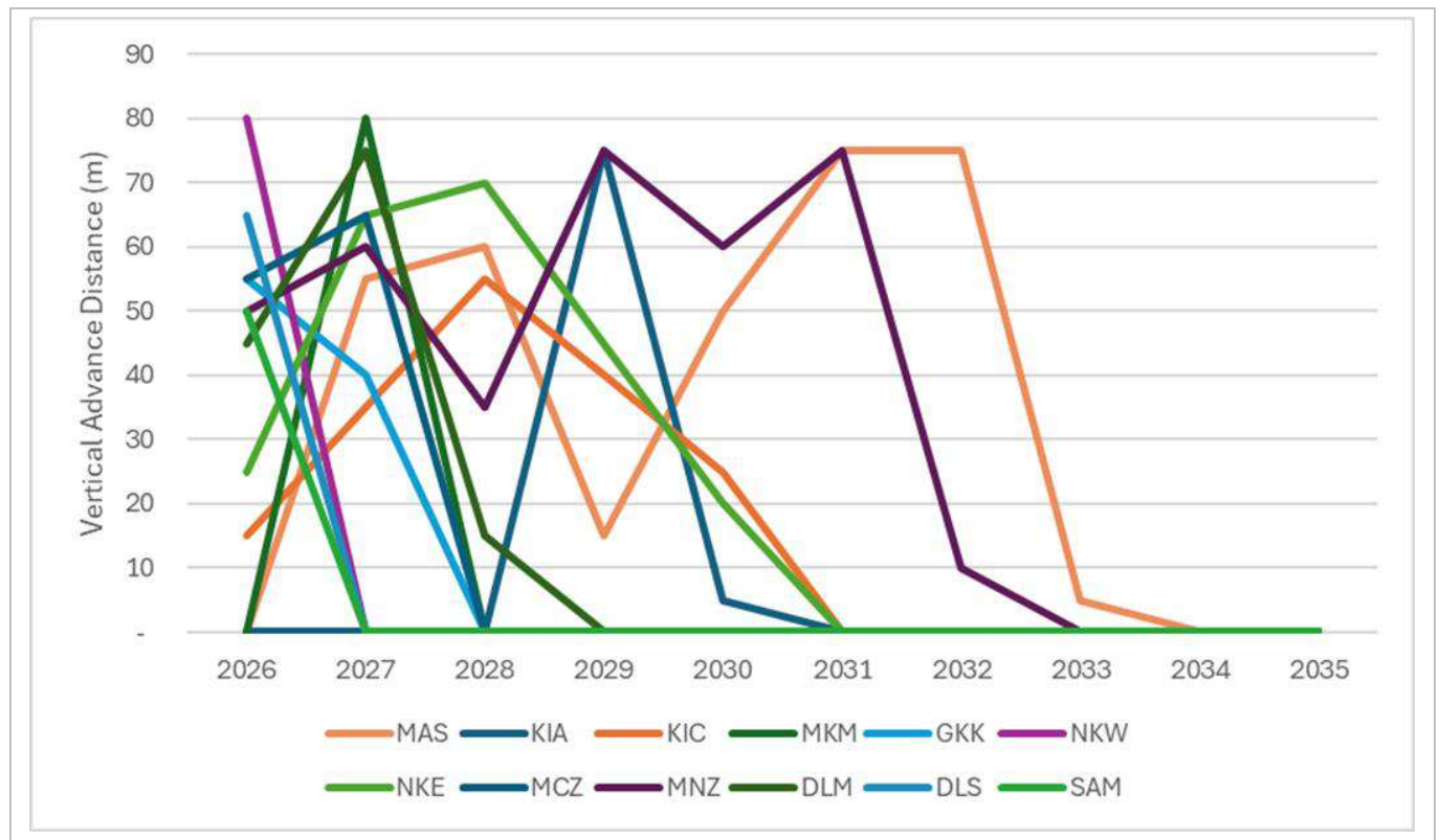
Figure 16-18 Maximum Vertical Advance Rates by Pit
