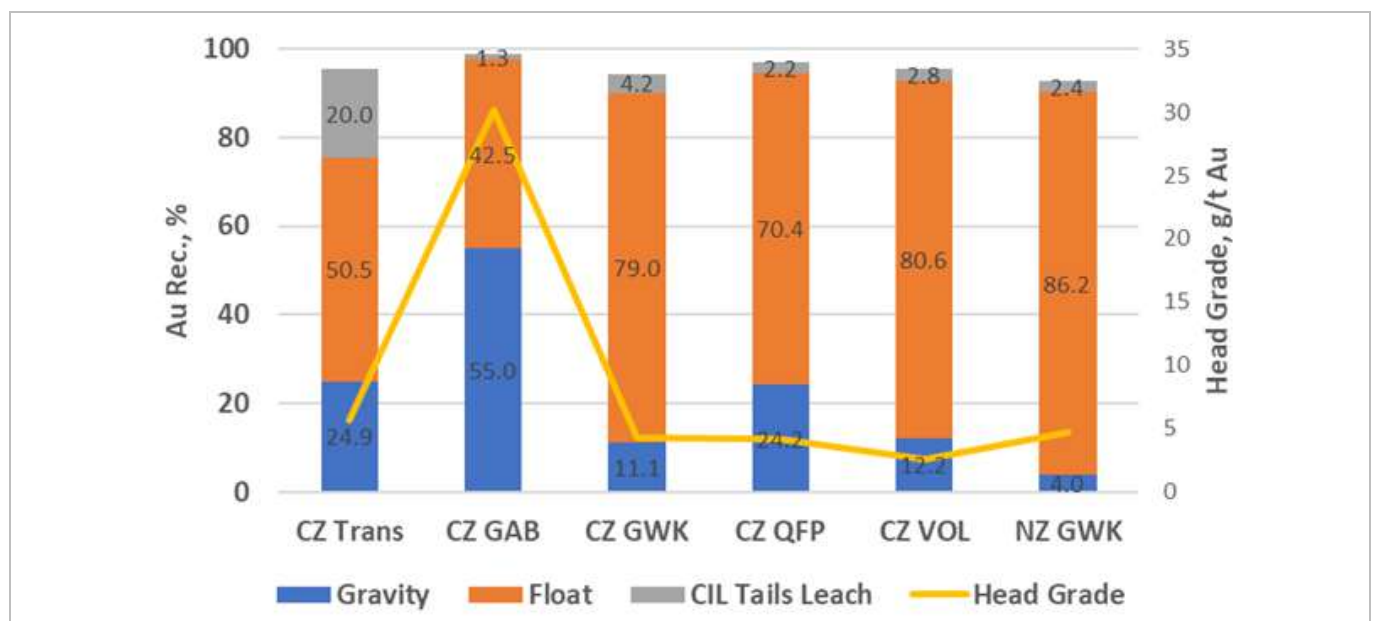
Figure 13-12: P2 Massawa Avg. Variability Sample Gravity/Flotation/Flotation Tails CIL Recoveries by Lithology
