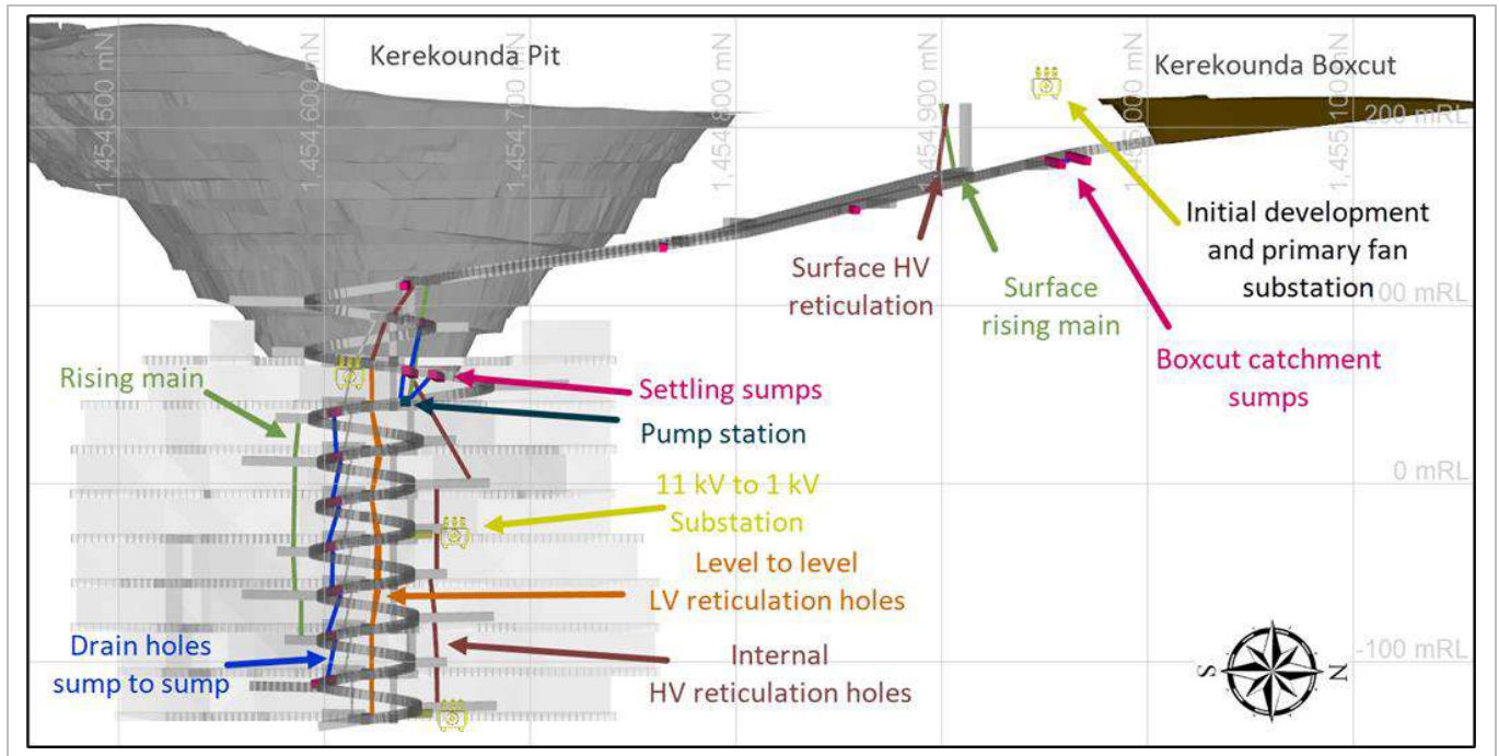
Figure 16-12: Kerekounda Mine Services System Schematic
