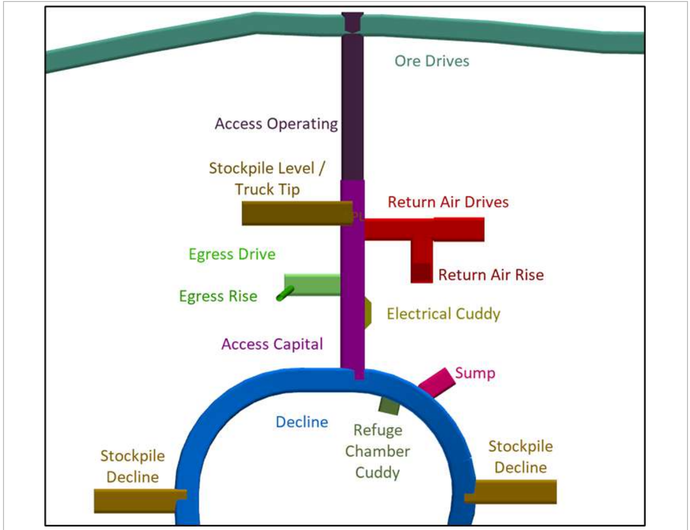
Figure 16-5: Typical K&G UG Level Layout (Plan View)
