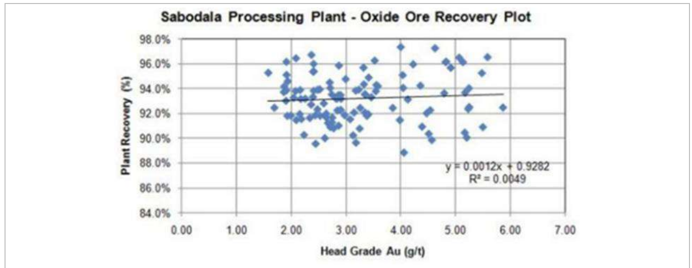
Figure 13-7: March-July 2009 Operational Data Supporting Sabodala Oxide Recovery Modelling
