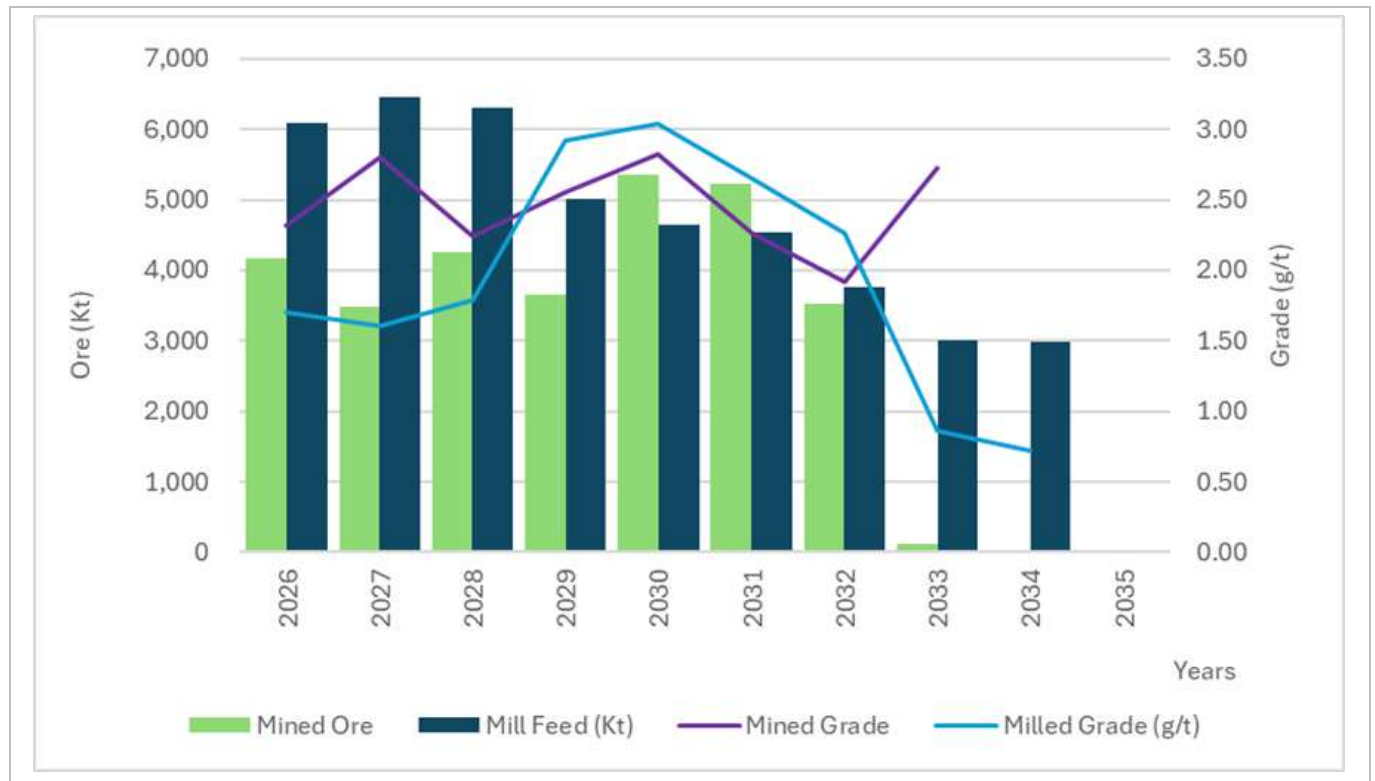
Figure 16-21: Annual Mined and Processed Ore Tonnage and Grade
