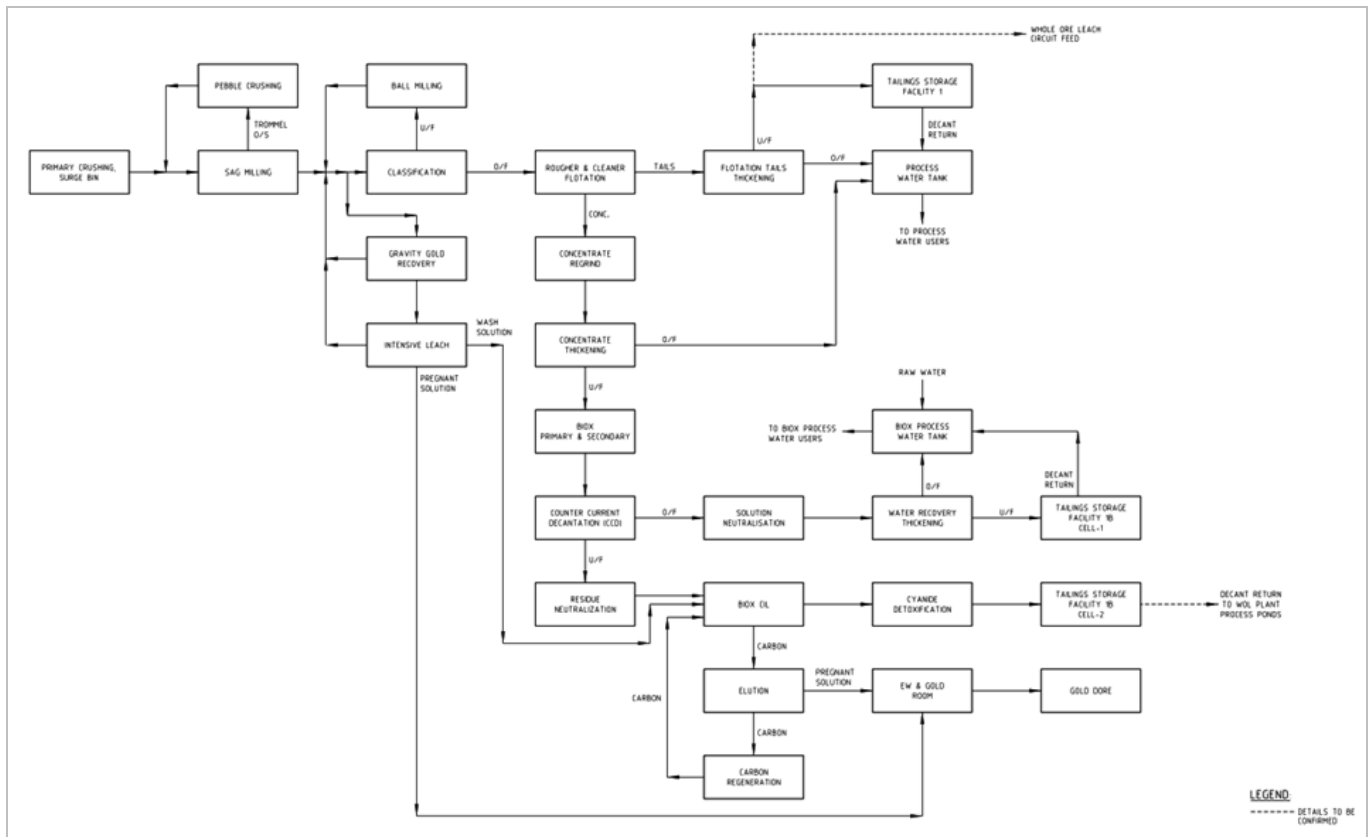
Figure 17-2: SSTP Block Flow Diagram (BFD)
