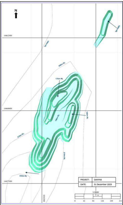
Figure 15-27: Samina Pit Designs (EDV, 2025)
