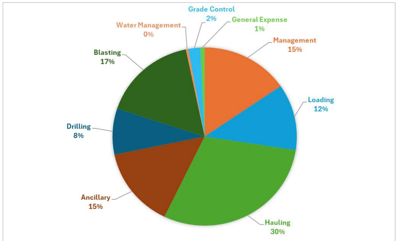
Figure 21-2: LoMp Apportionment of Open Pit Operating Costs
