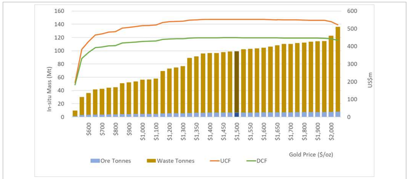
Figure 15 11: Massawa NZ Optimisation Results
