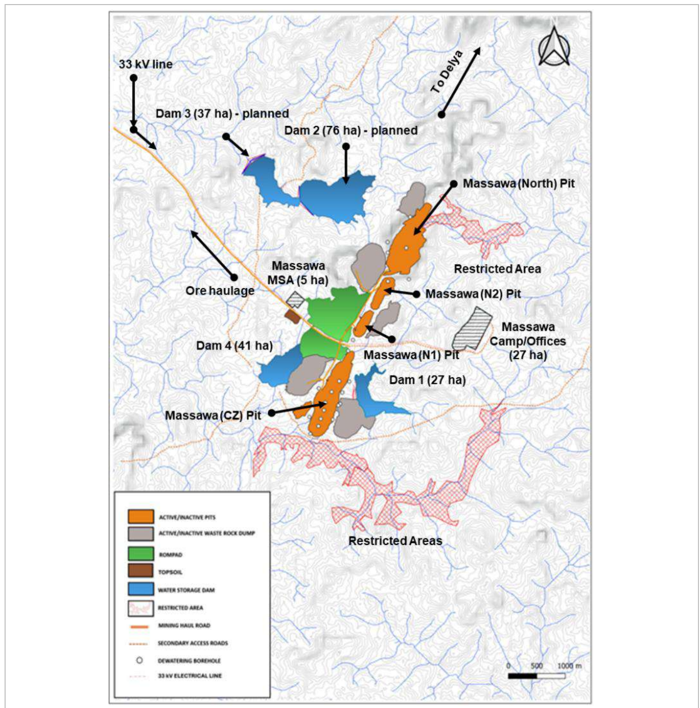
Figure 18-3: Massawa Infrastructure GA (EDV, 2025)
