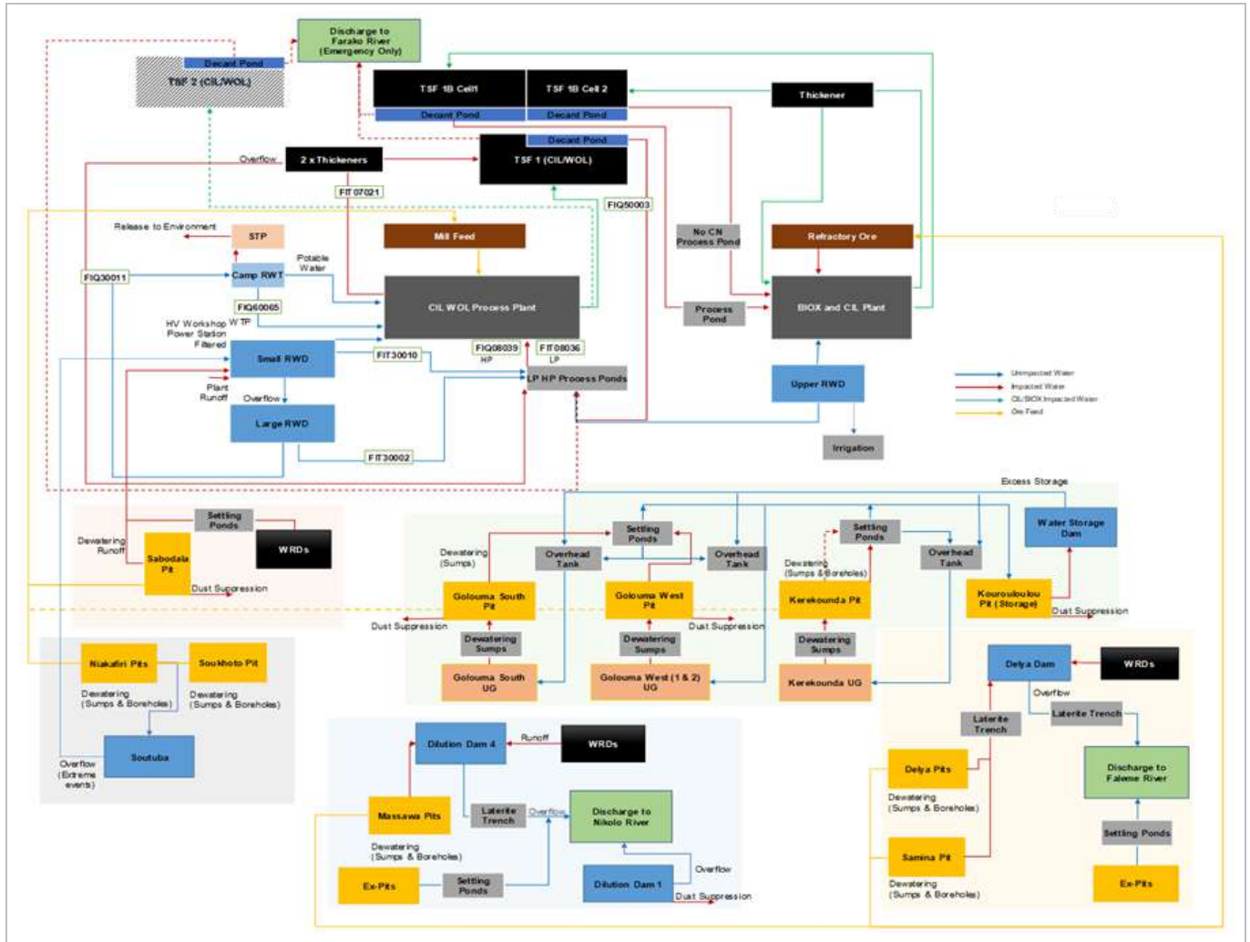
Figure 20-2: Sabodala MC Water BFD with “PI” Tags for Key Monitoring Locations
