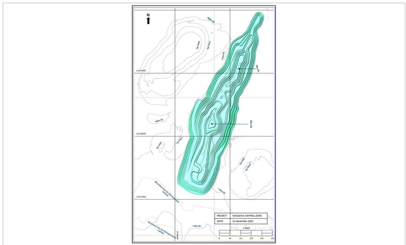
Figure 15-22: MCZ Pit Design Stages (EDV, 2025)
