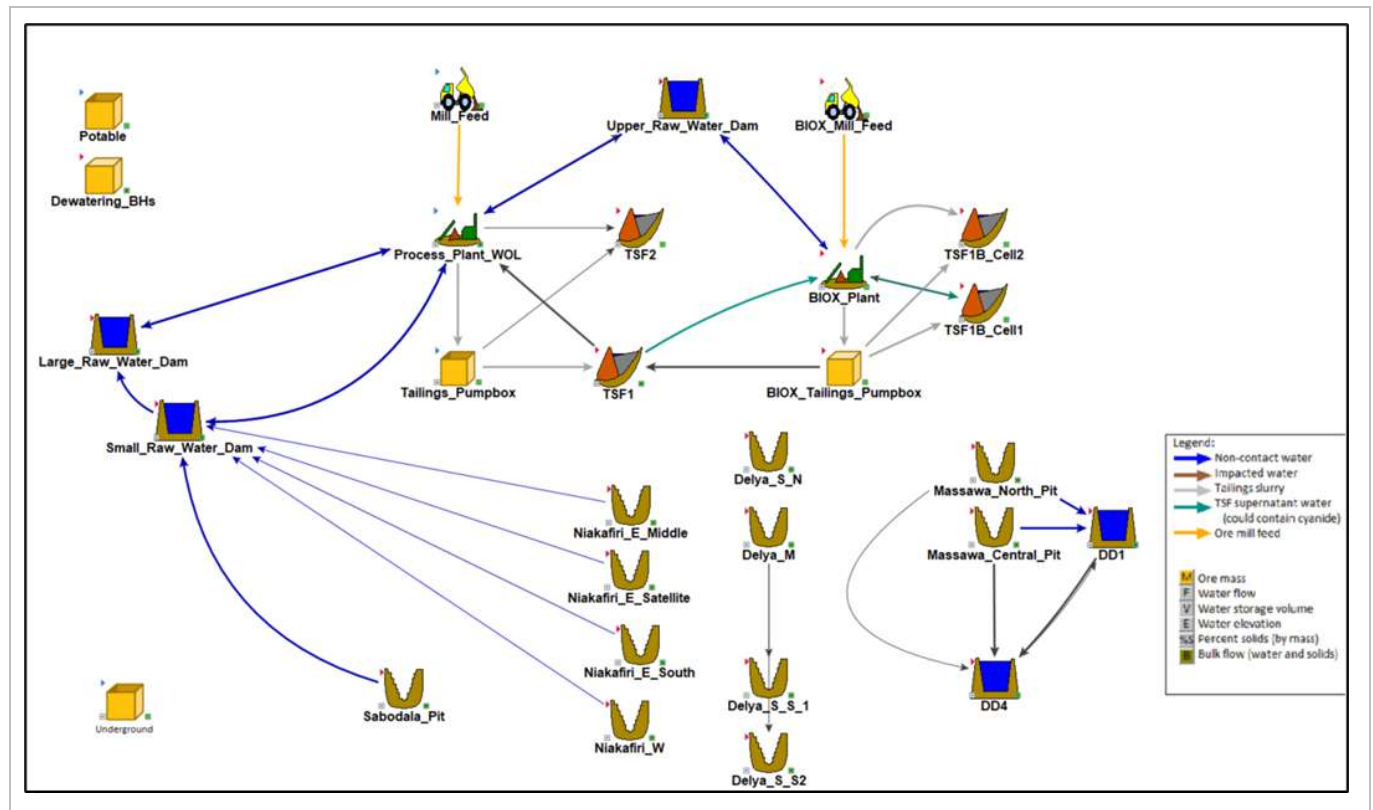
Figure 18-7: Uppermost level of the Sabodala GoldSim model
