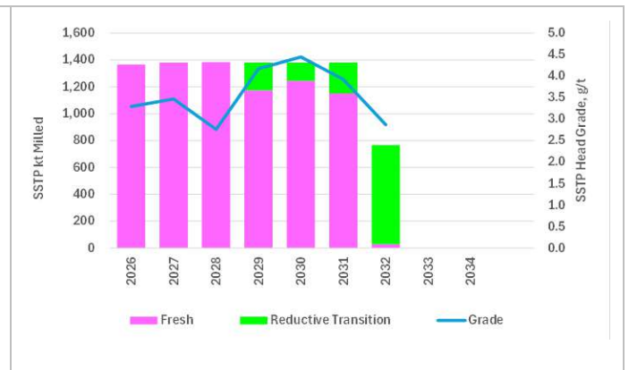
Figure 17-4: SSTP LoM Mill Feed by Weathering
