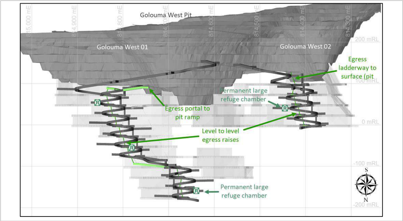
Figure 16-10: Golouma West 01 and 02 Egress System Schematic
