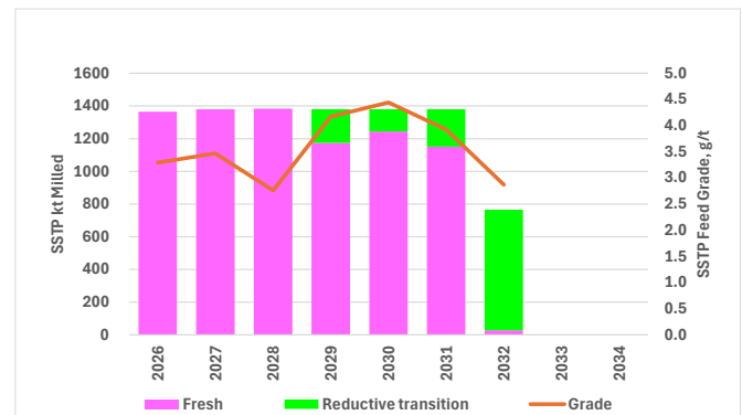
Figure 13-3: SSTP LoM Mill Feed by Weathering
