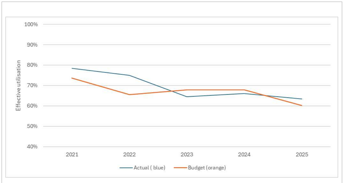
Figure 16-3: Excavator PC3000 Effective Utilisation - Planned (Orange) vs Actual (Blue)
