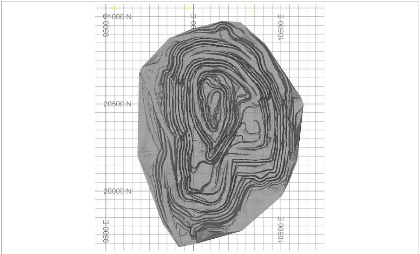
Figure 14-48: Sabodala Open Pit Depletion as of 31 December 2025 (Local Grid) (EDV 2025)
