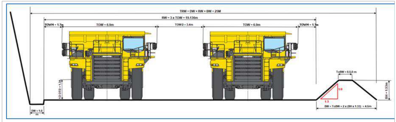
Figure 15-12: Dual Lane Haul Road Width
