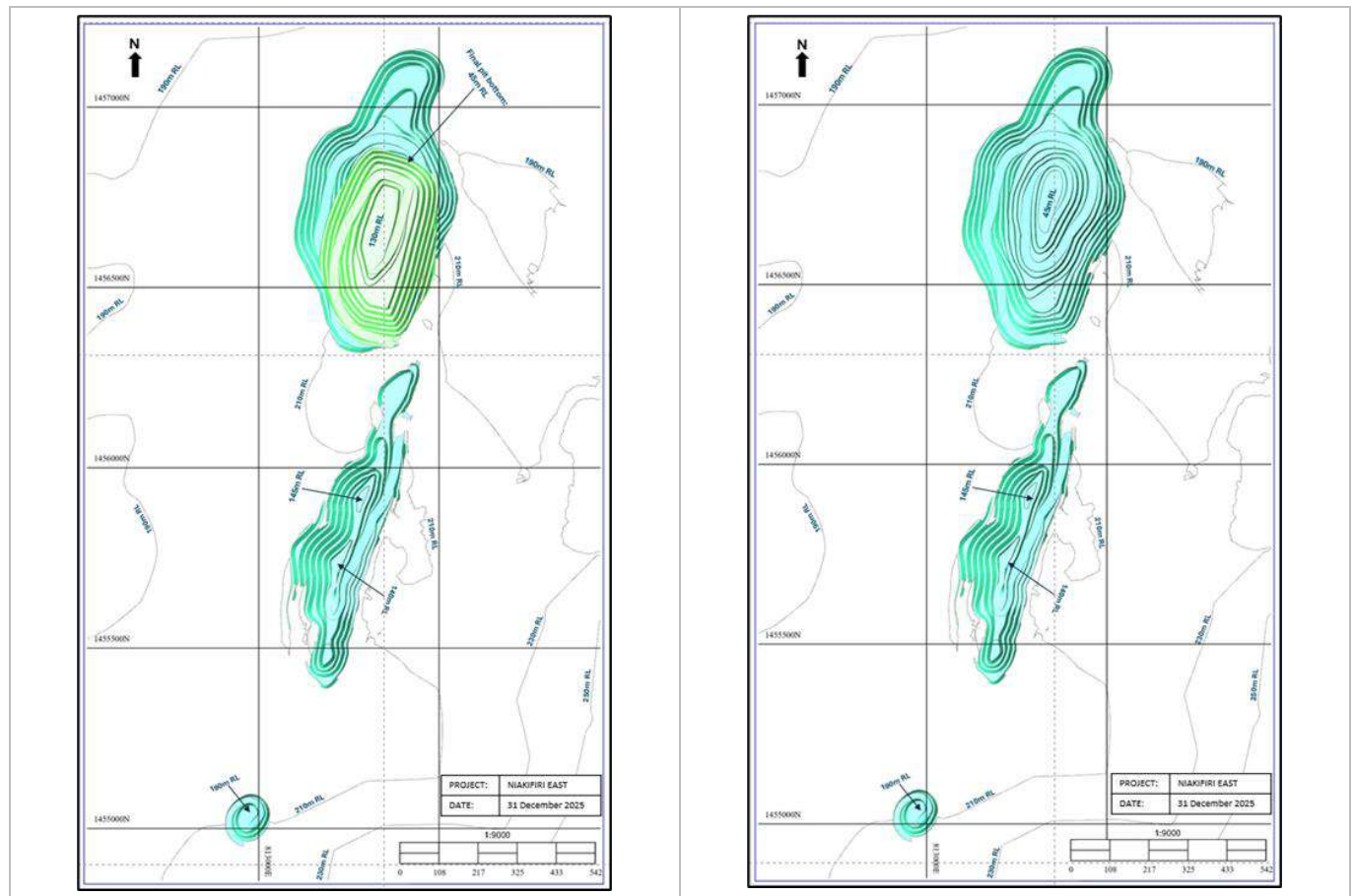
Figure 15-18: Niakifiri East Stage and Final Pit Designs (EDV, 2025)
