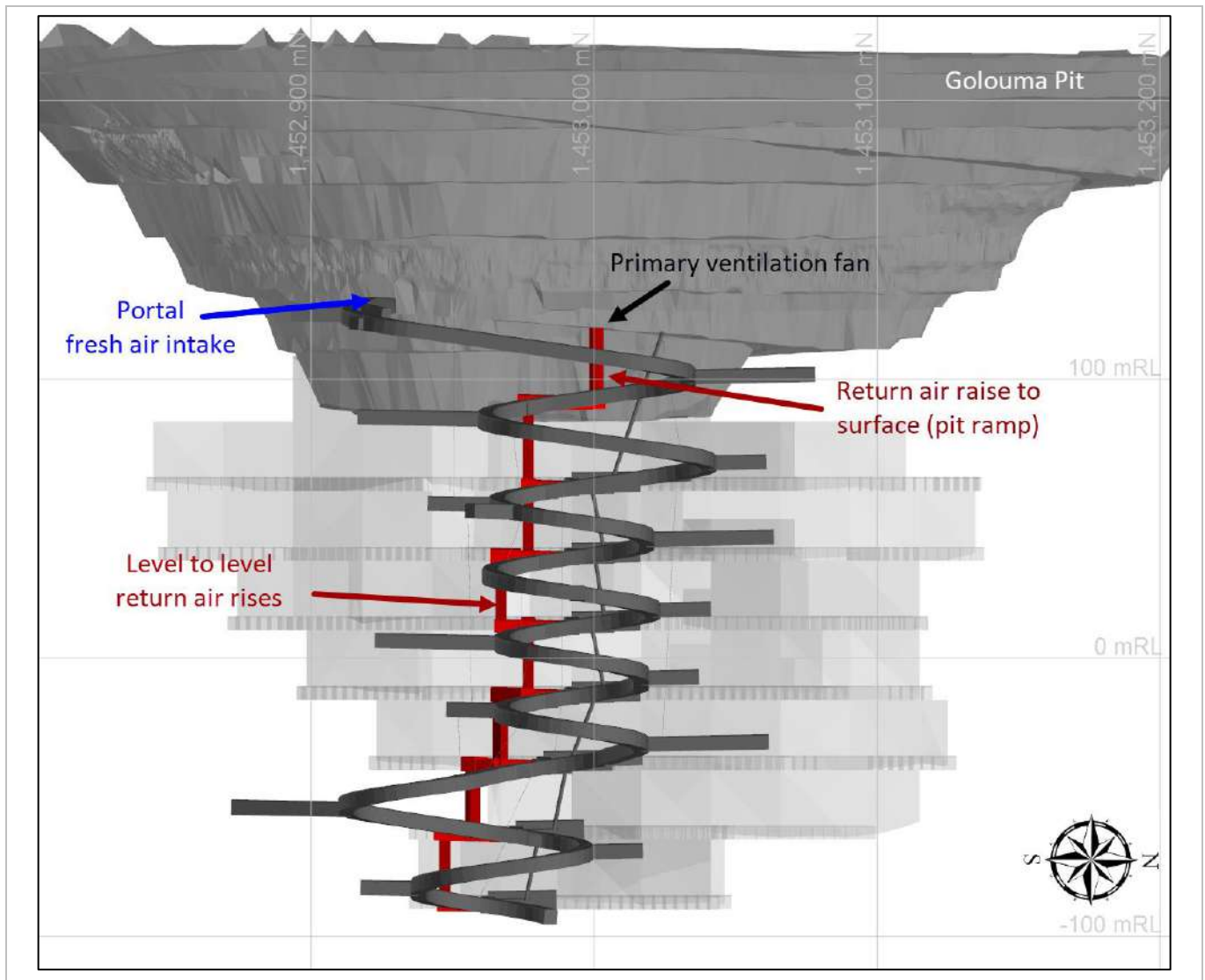
Figure 16-8: Golouma South Primary Ventilation System Schematic
