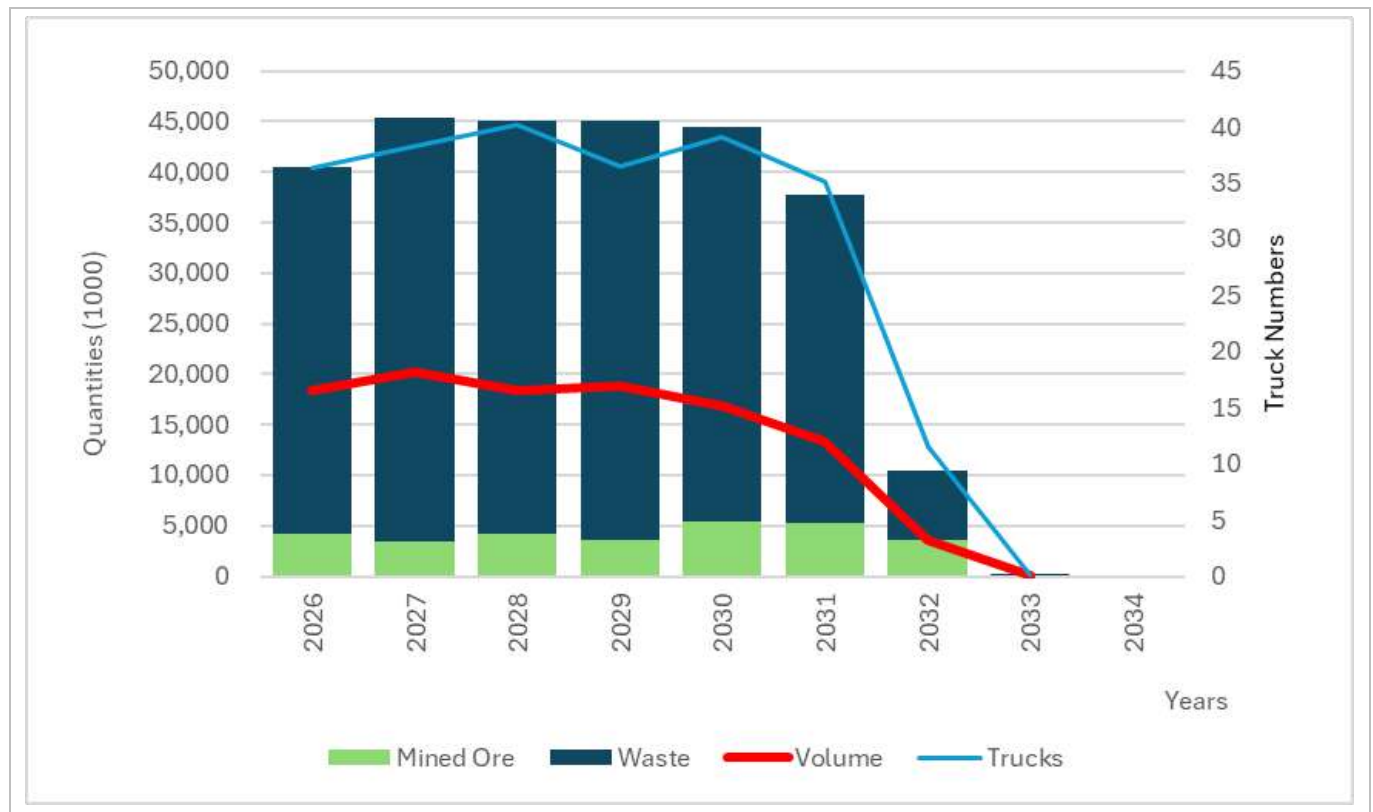
Figure 16-19: Annual Material Movement and Trucks Requirement
