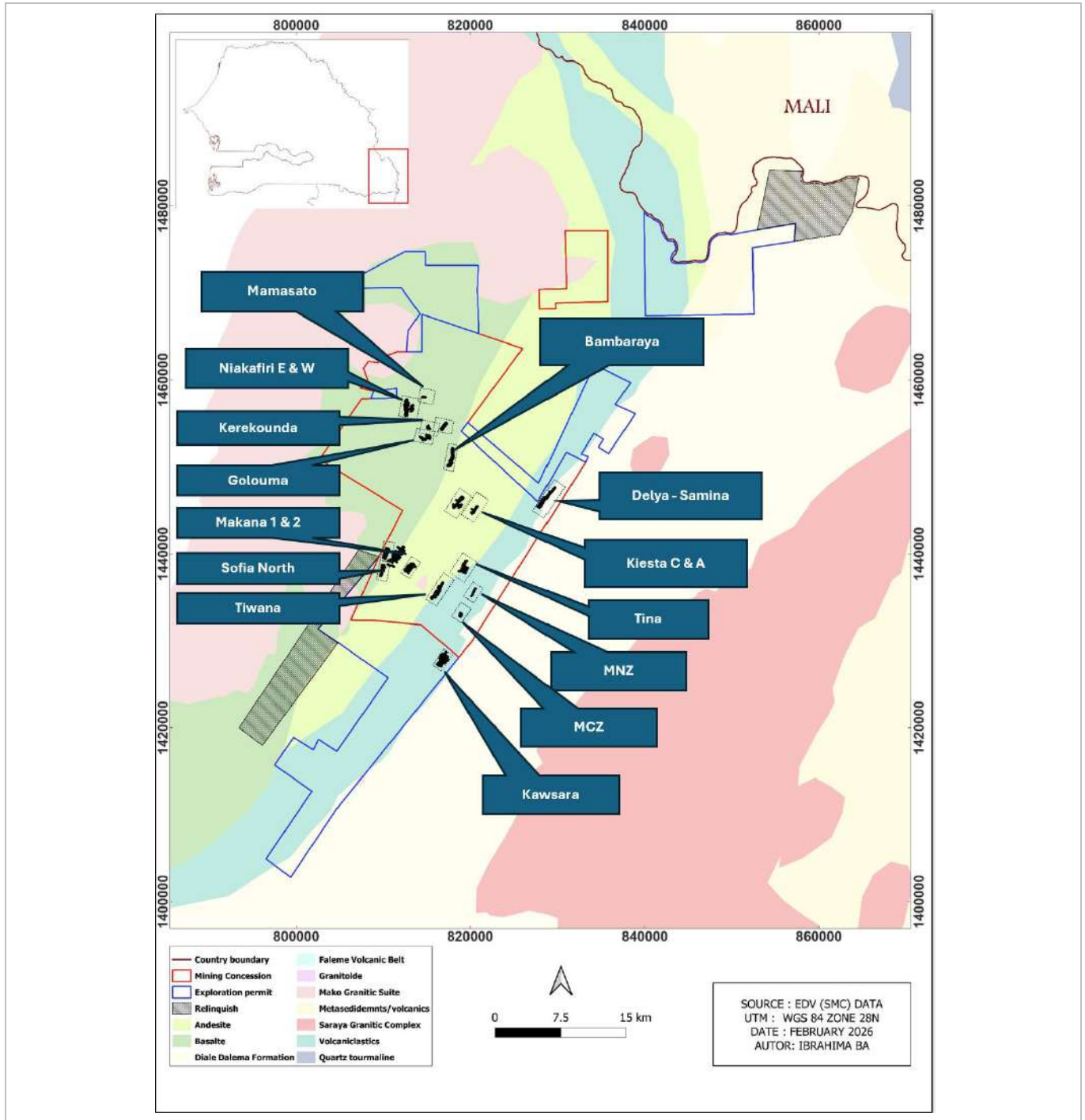
Figure 10-1: Resource Drill Hole Locations 2021 to 2025
