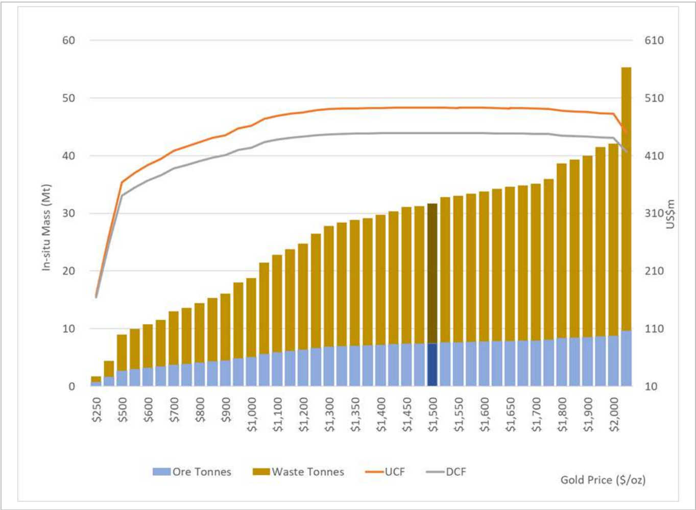
Figure 15-10: Massawa CZ Optimisation Results
