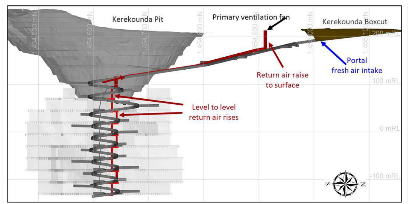
Figure 16-6: Kerekounda Primary Ventilation System Schematic
