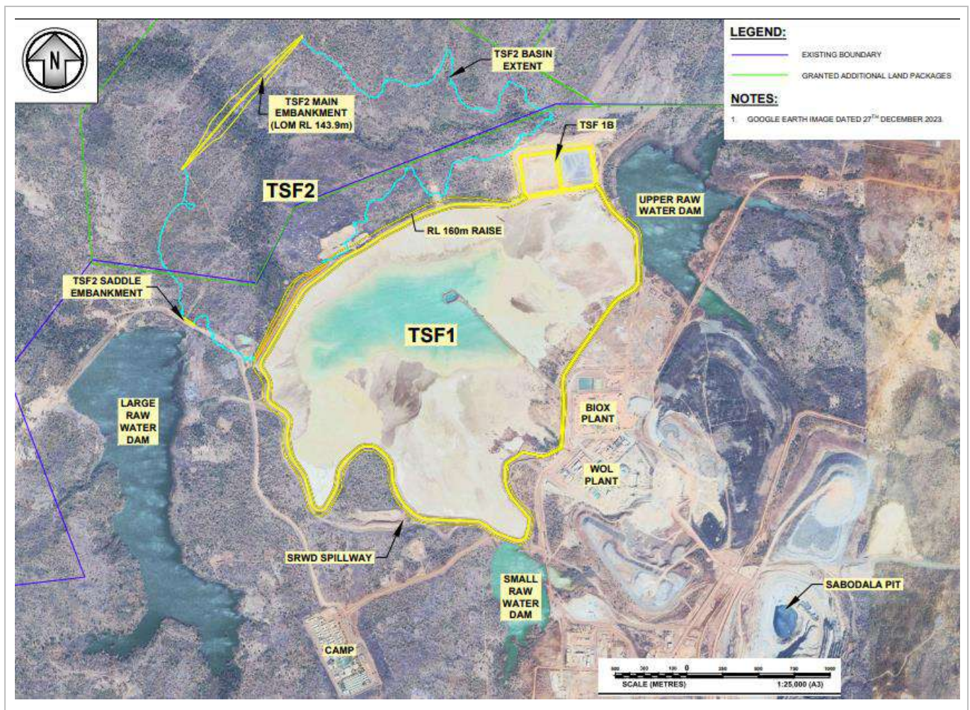
Figure 18-16 Layout Drawing for TSF1, TSF 1B and TS2 (KP, 2026)
