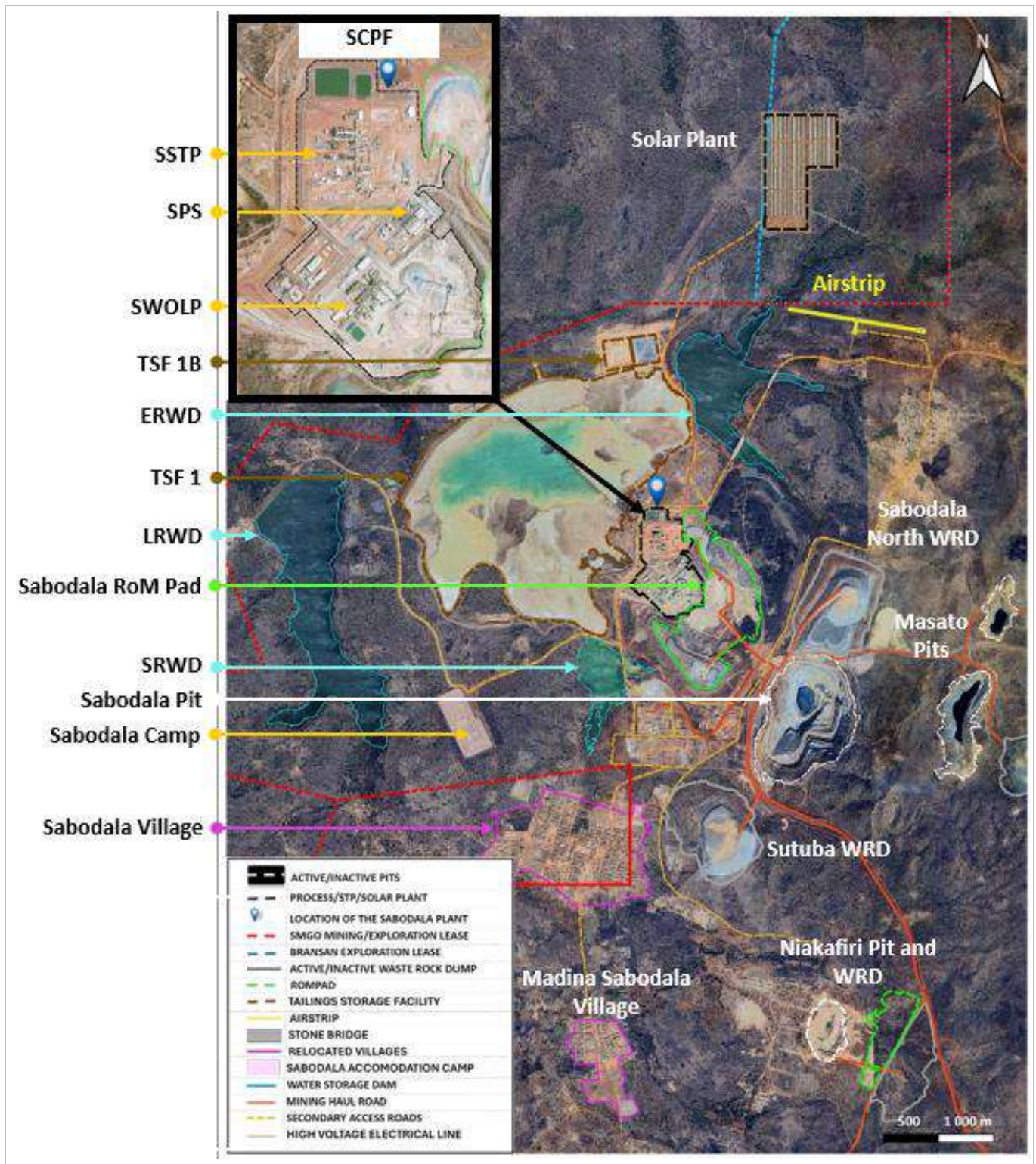
Figure 18-2: Sabodala Lot A GA (EDV, 2025)
