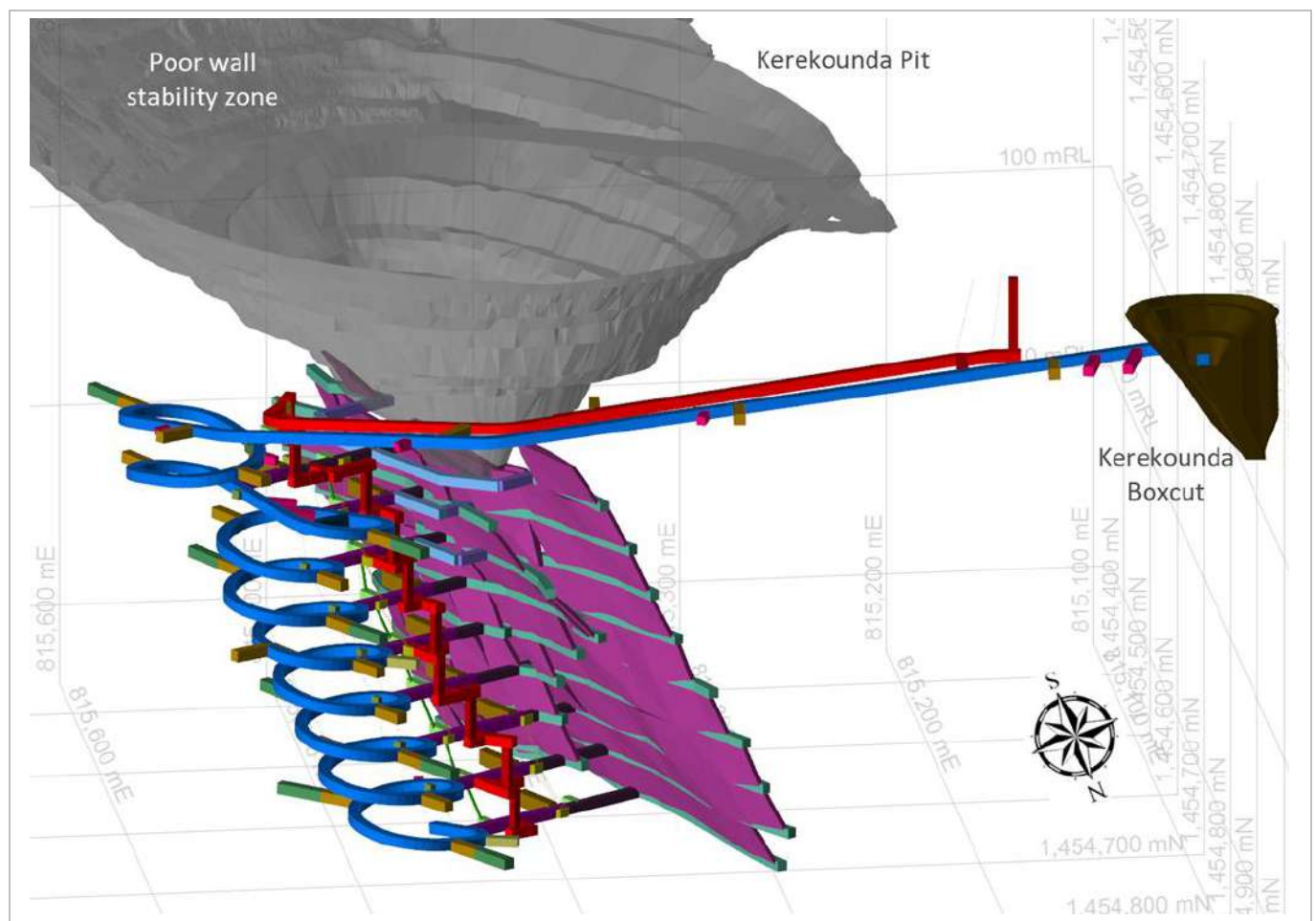
Figure 16-15: Kerekounda Underground Mineral Reserve Design
