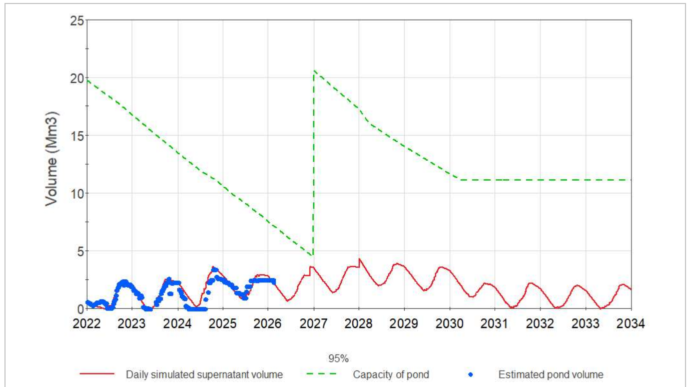
Figure 18-11: TSF 1 Simulated 1:100 Year Rainfall Events (95 th percentile, 100 realisations)
