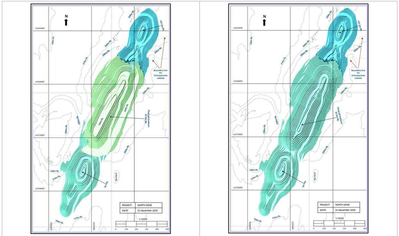
Figure 15-23: MNZ Pit Designs With the Central Initial Stage and Final Pit (EDV, 2025)
