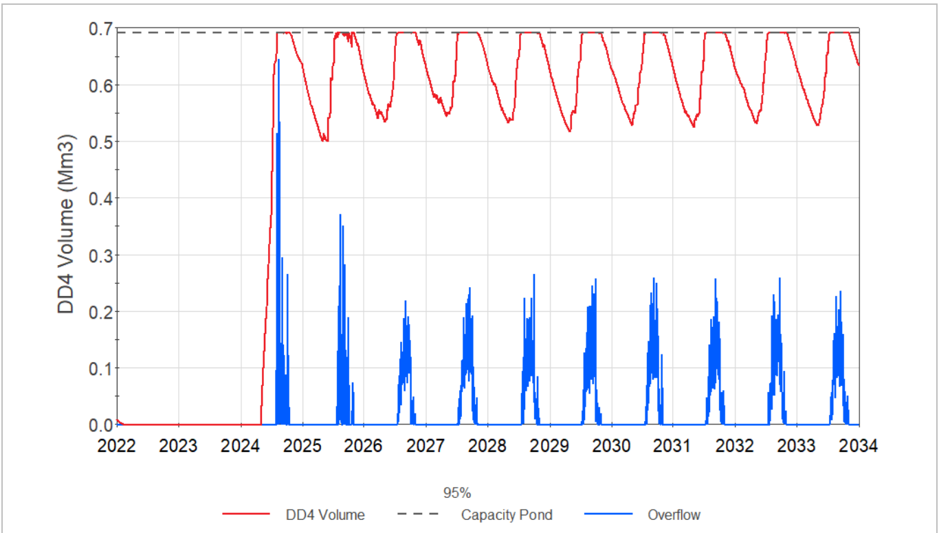
Figure 18-13: DD4 Modelled Volume and Discharge (95 th Percentile)
