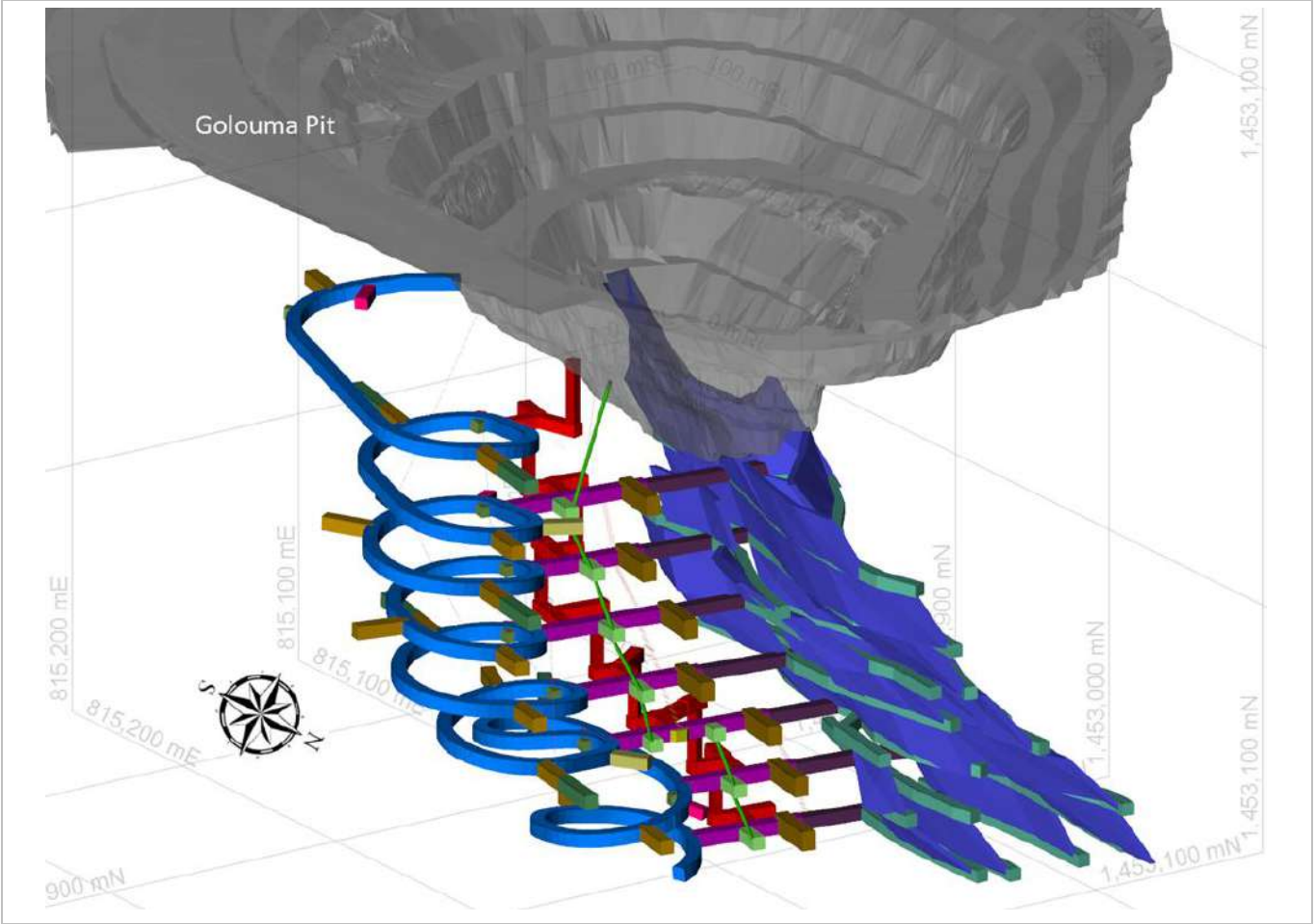
Figure 16-17: Golouma South Underground Mineral Reserve Design
