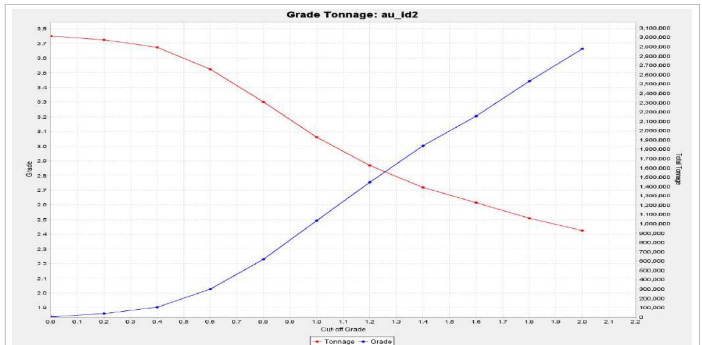
Figure 14-95: Kiesta C Grade-Tonnage Curve Constrained by USD 2100/oz Whittle Pit (EDV, 2025)
