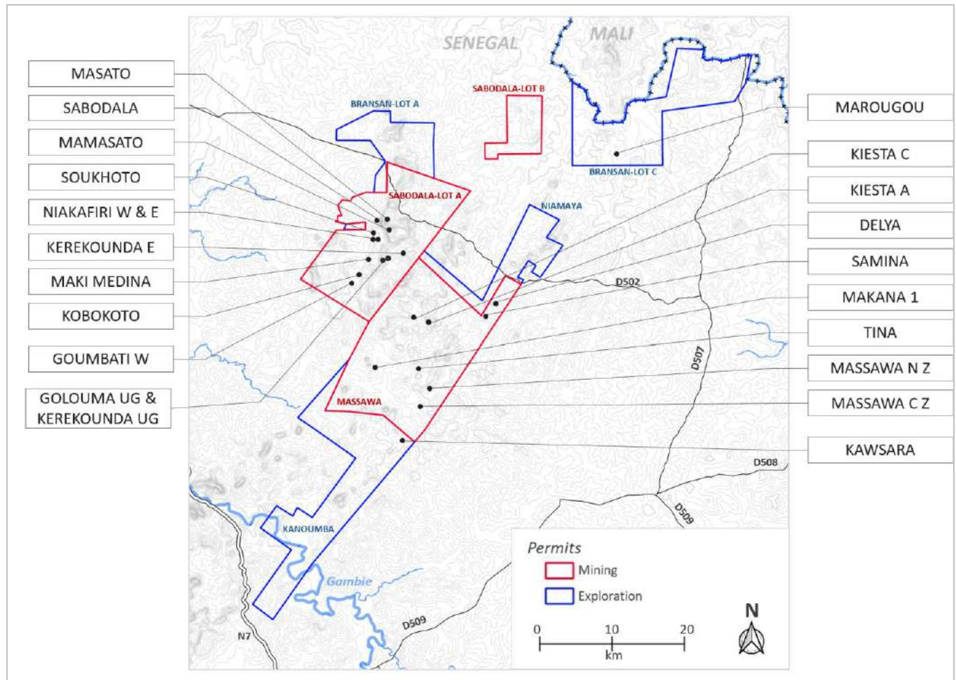
Figure 14-1: Location of Deposits with Current Mineral Resources
