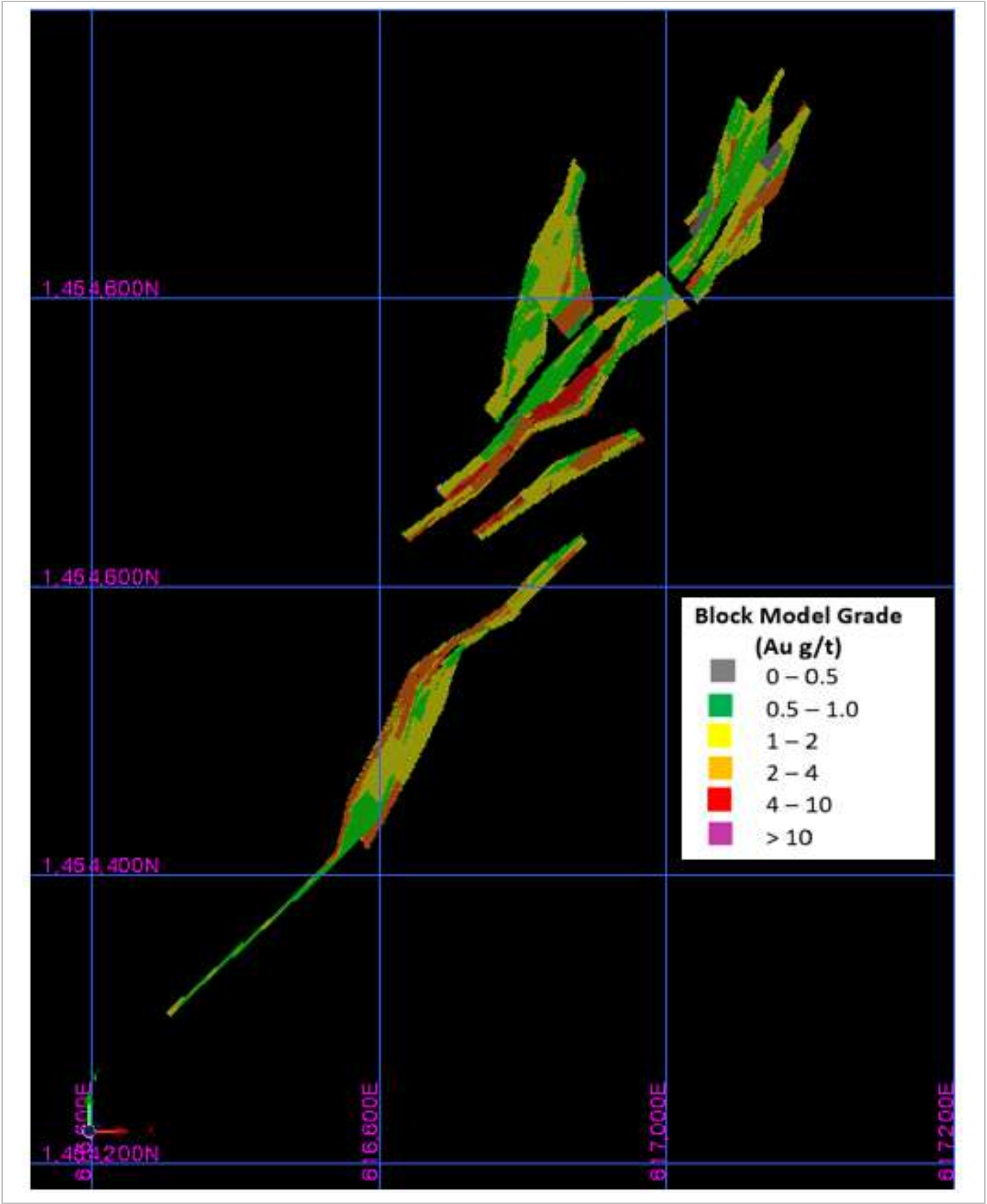
Figure 14-75: Kerekounda East Grade Block Model Plan View (EDV 2025)
