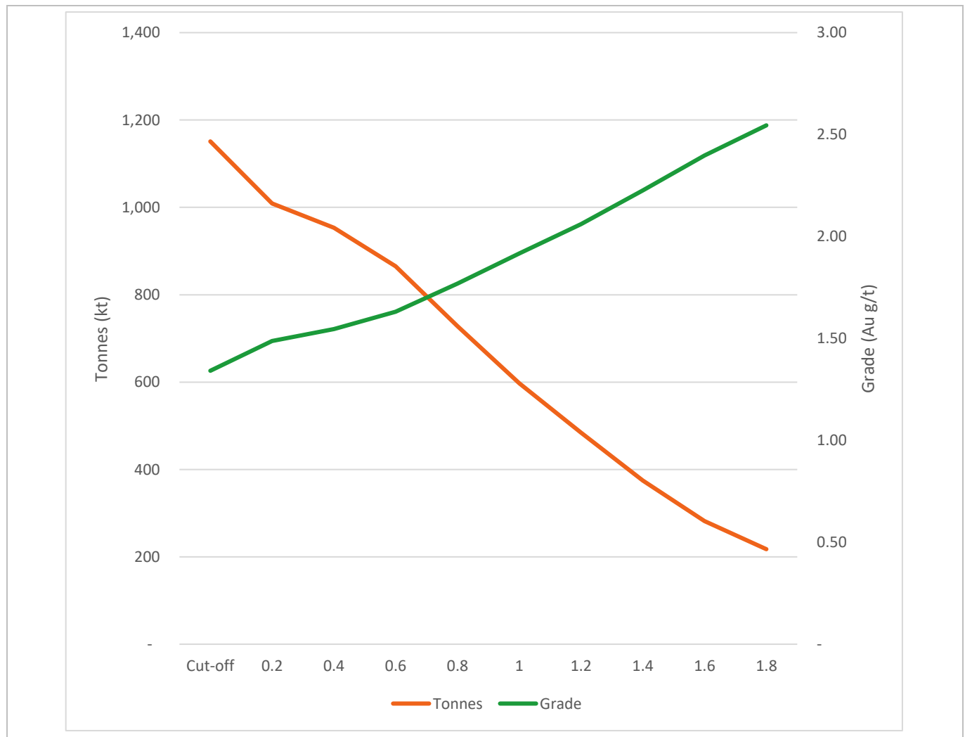
Figure 14-97: Maki Medina Grade-Tonnage Curve Within USD 2100 Whittle Pit (EDV 2025)
