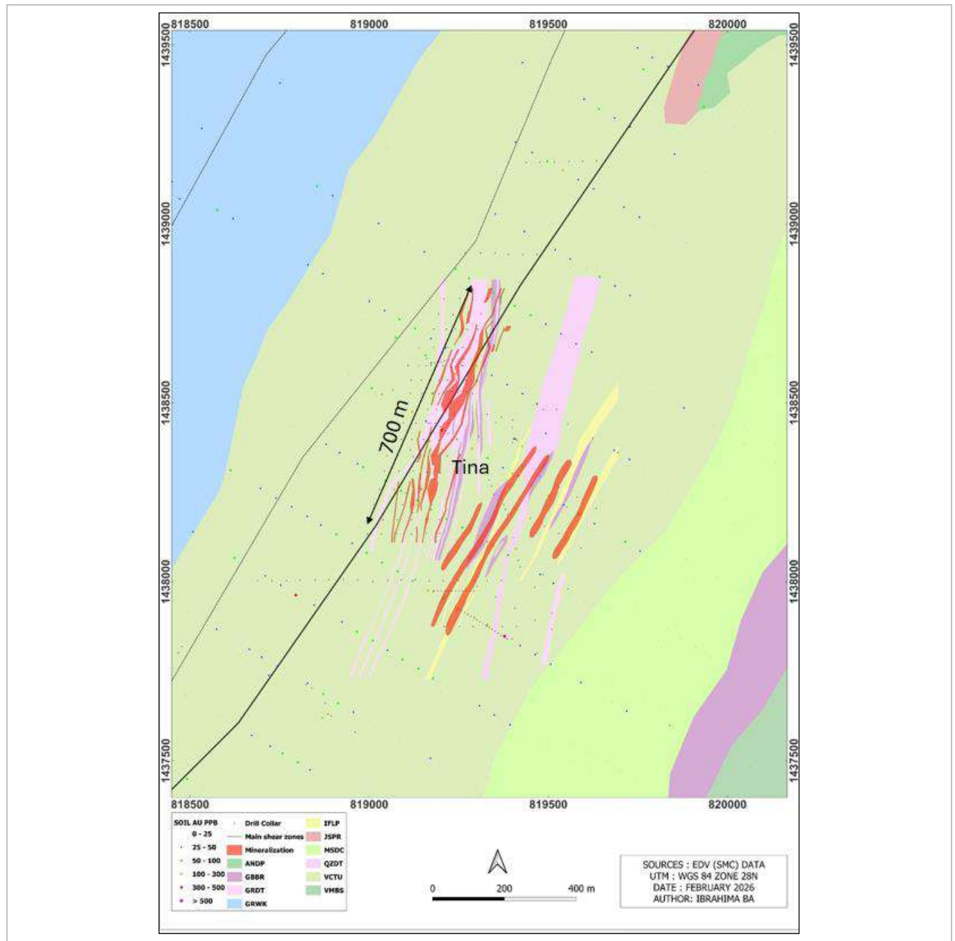
Figure 7-18: Tina Geological Map with Mineralisation Zones (EDV, 2025a)
