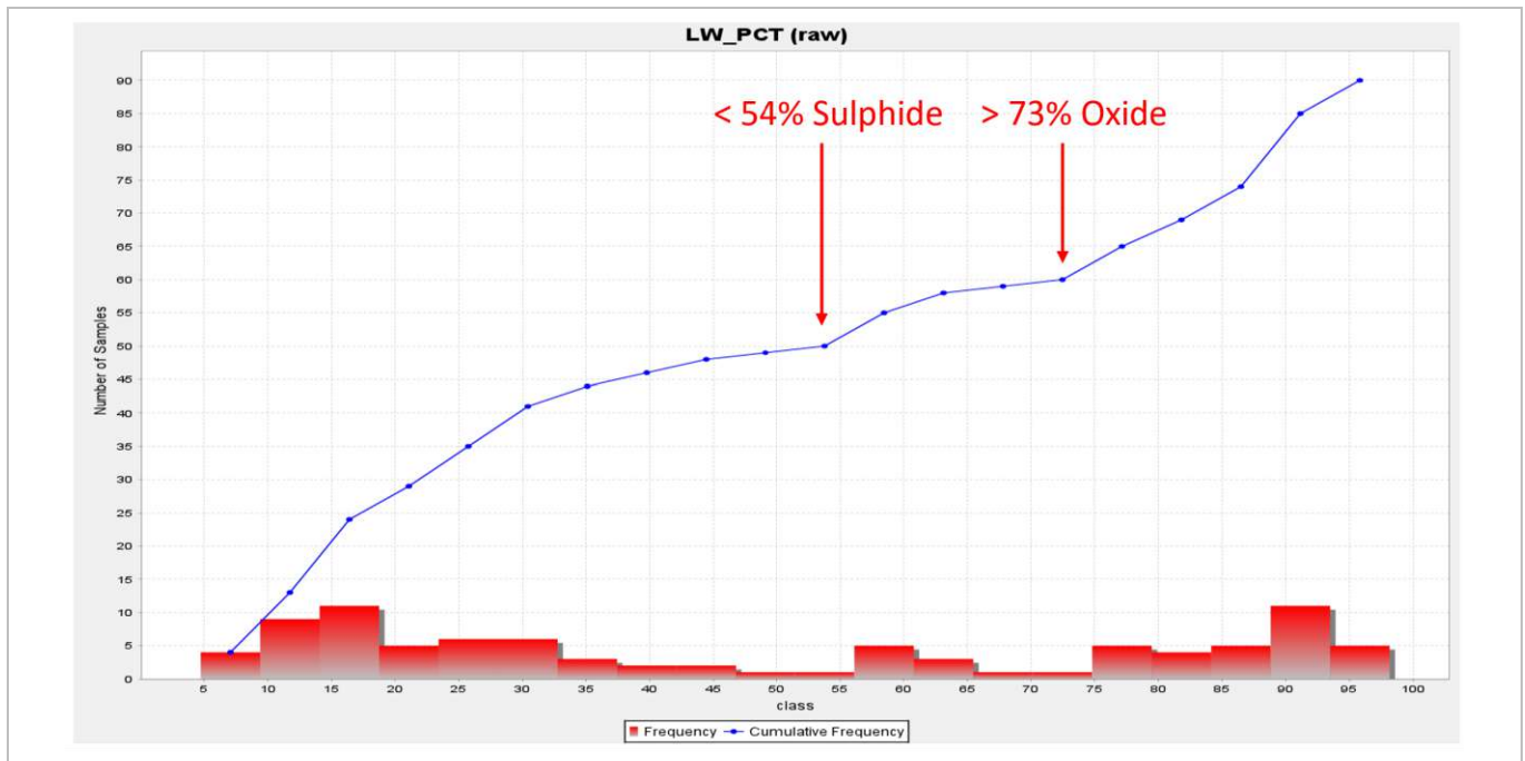
Figure 14-2: Tina LW% by RedOx Zone (EDV, 2025)
