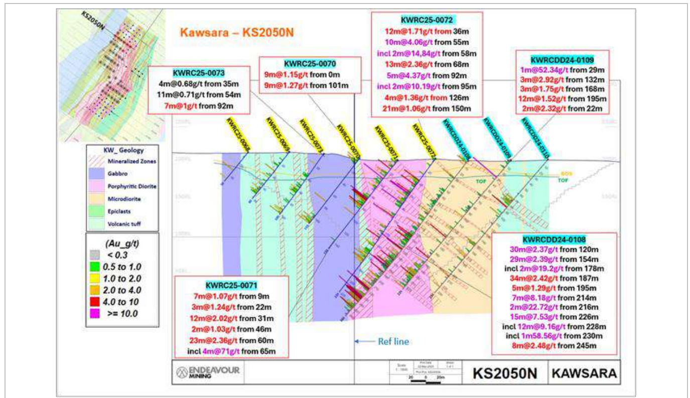
Figure 10-12: Kawsara Cross-Section KS2050N with Geology and Assay Results
