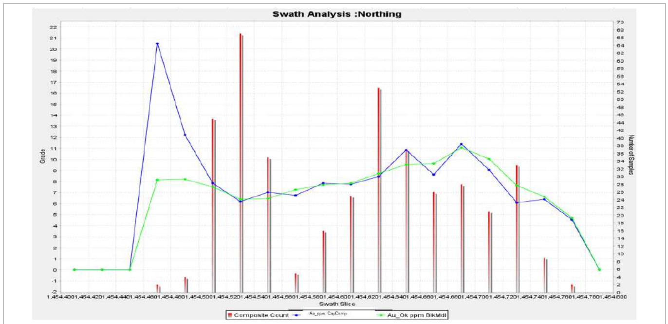
Figure 14-47: Example of a Swath Plot (EDV 2023)
