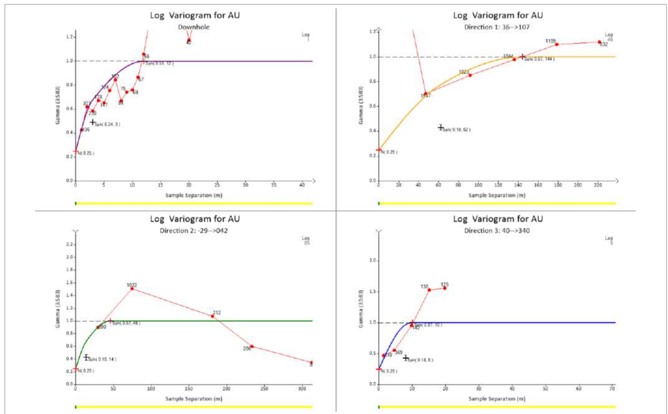
Figure 14-42: Mamasato Semi-Variograms (EDV, 2025)
