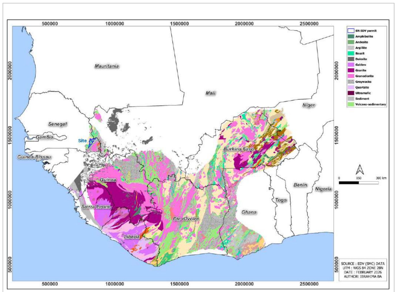
Figure 8-1: Geology of the West African Craton (EDV, 2026)
