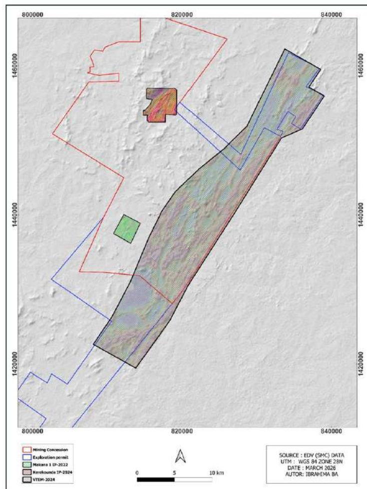
Figure 9-1: IP and EM -Geophysical Surveys 2022-2025
