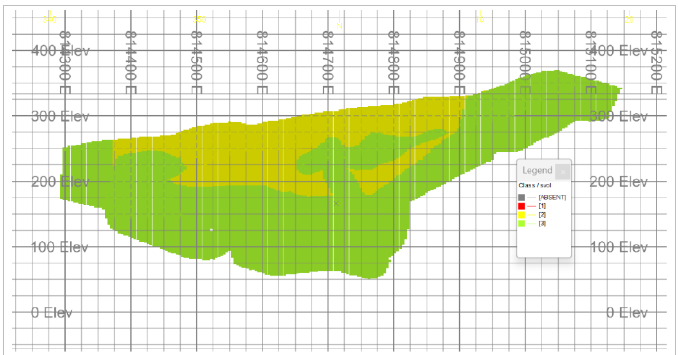
Figure 14-62: Mamasato Mineral Resource Classification (EDV 2025)
