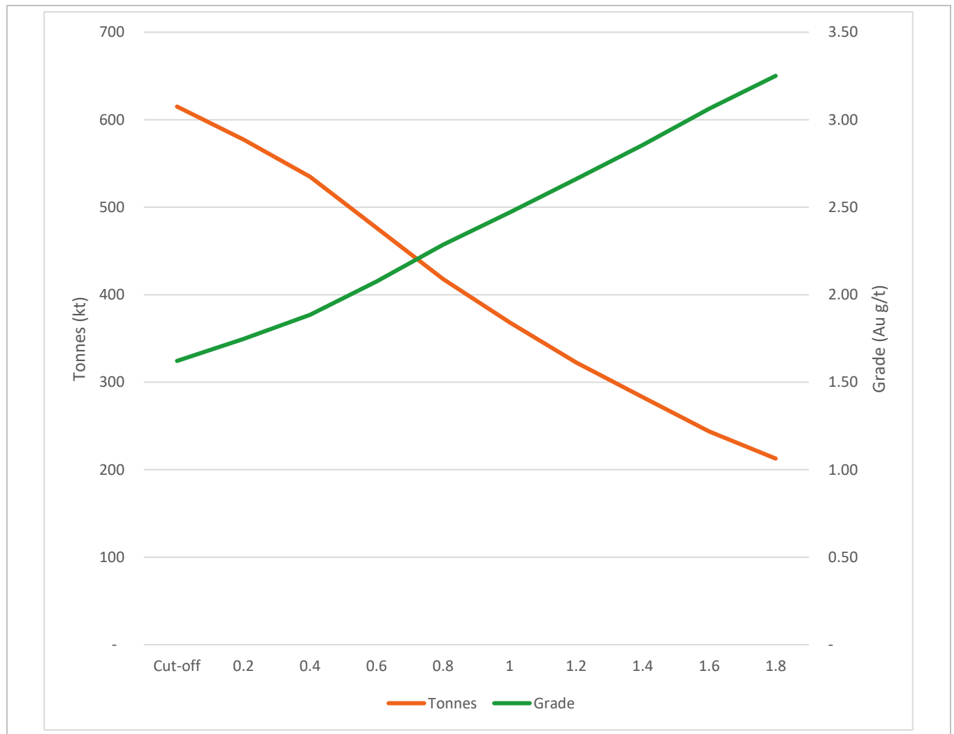
Figure 14-98: Mamasato Grade-Tonnage Curve Within USD 2100/oz Whittle Pit (EDV 2025)
