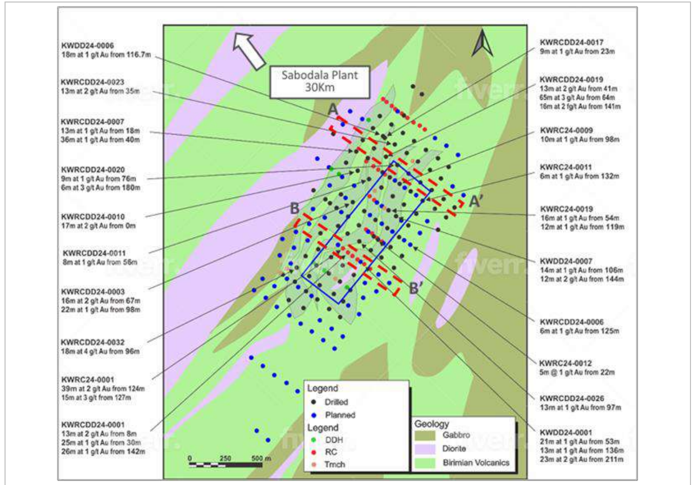
Figure 10-11: Kawsara Drill Hole Collar Locations with Selected Results
