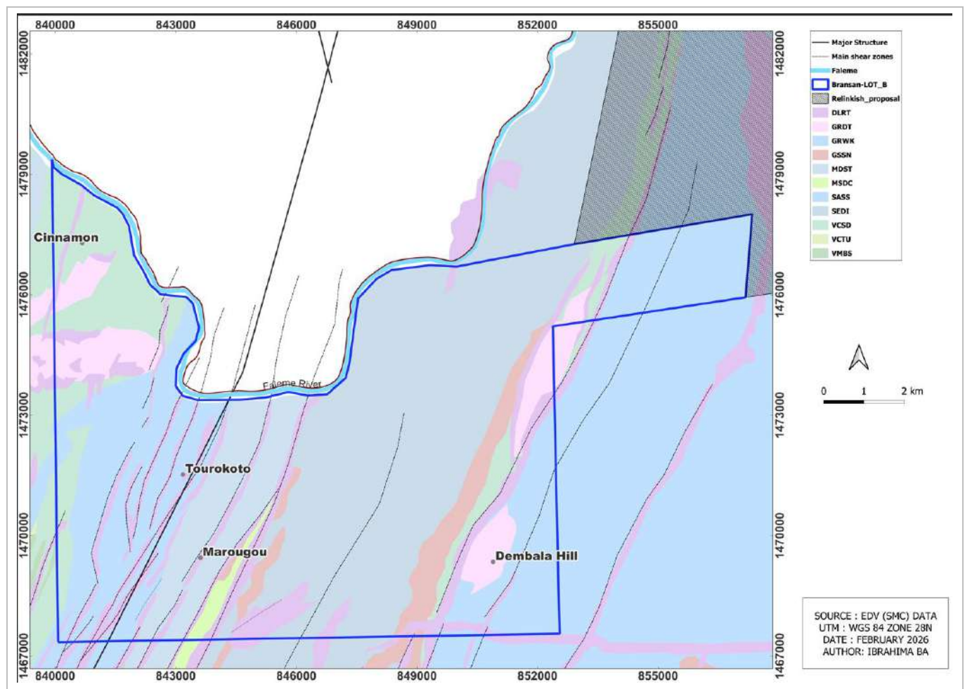
Figure 7-9: Branson Lot C Geology and Prospects (EDV, 2025a)
