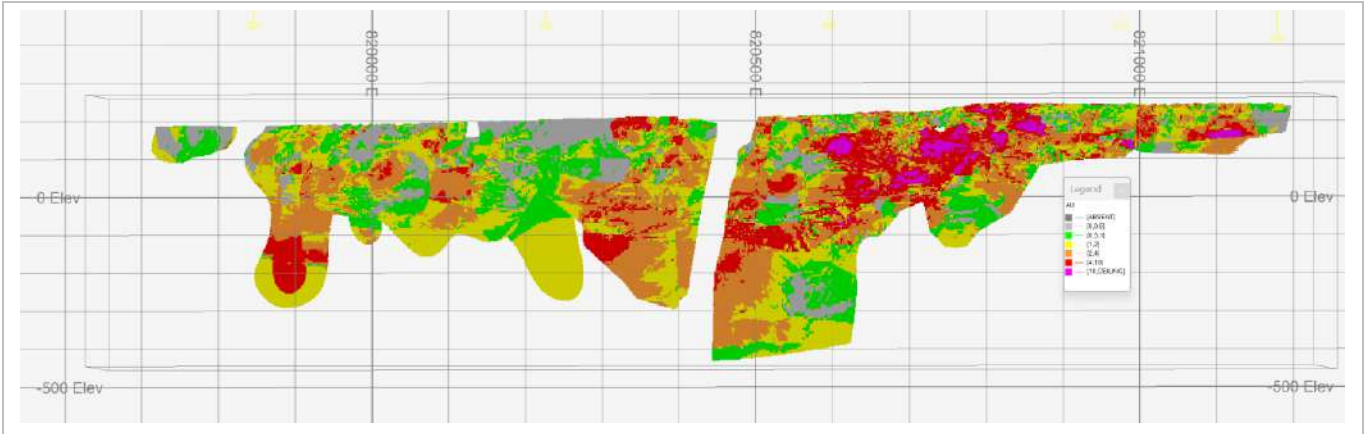
Figure 14-82: MNZ Grade Block Model (EDV 2025)
