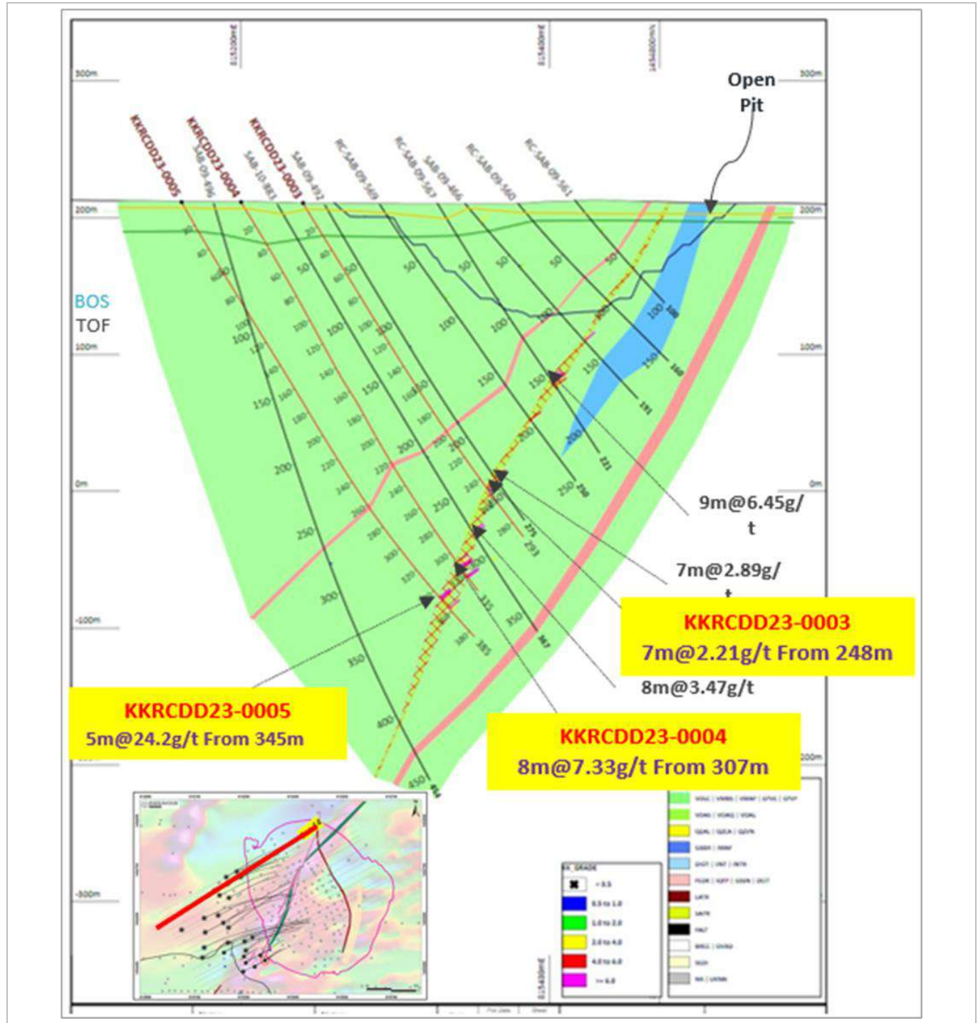
Figure 10-6: Kerekounda Drilling Cross-Section with Selected Assay Results
