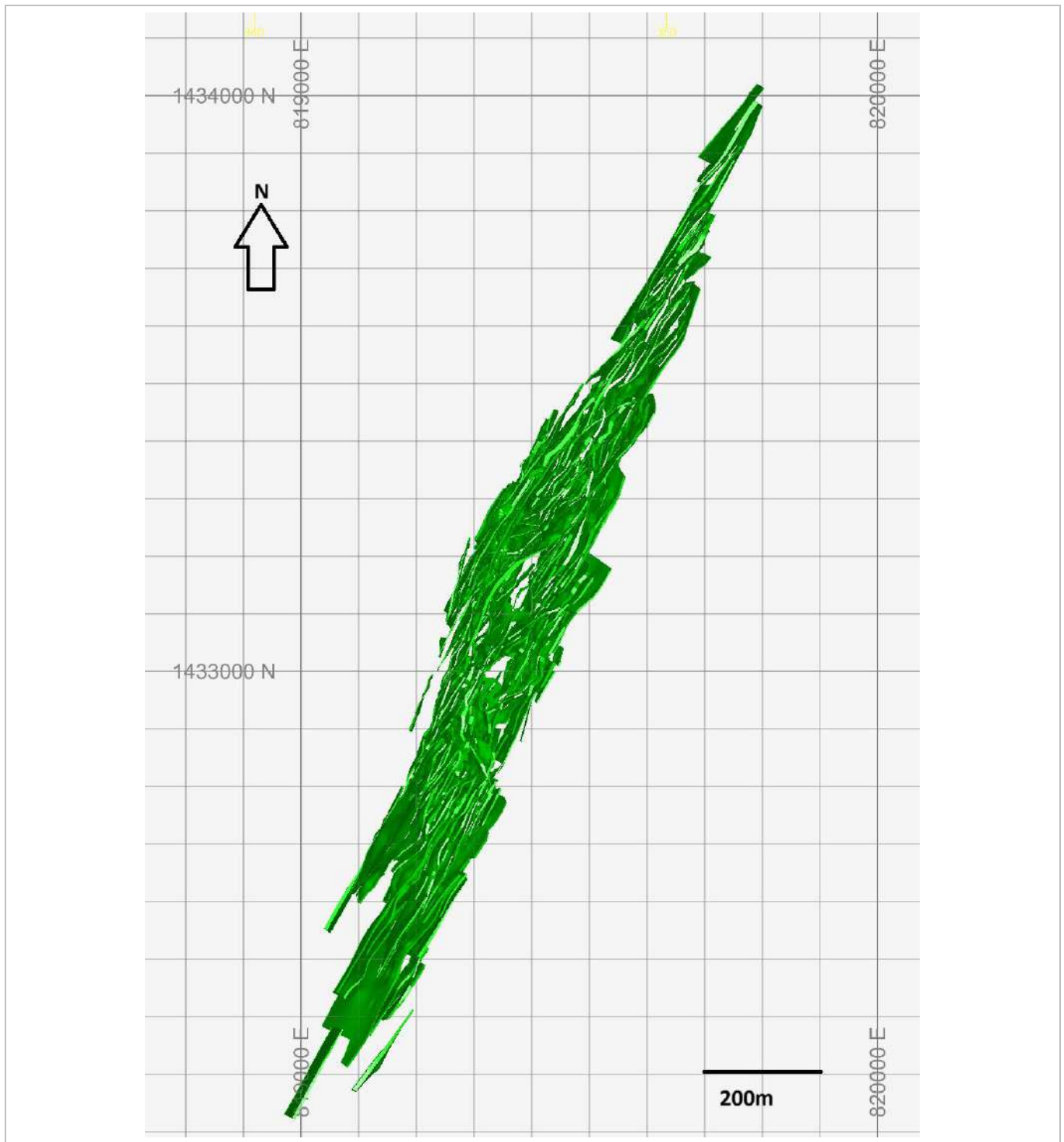
Figure 14-29: MCZ Mineralisation, Plan View (EDV, 2025)
