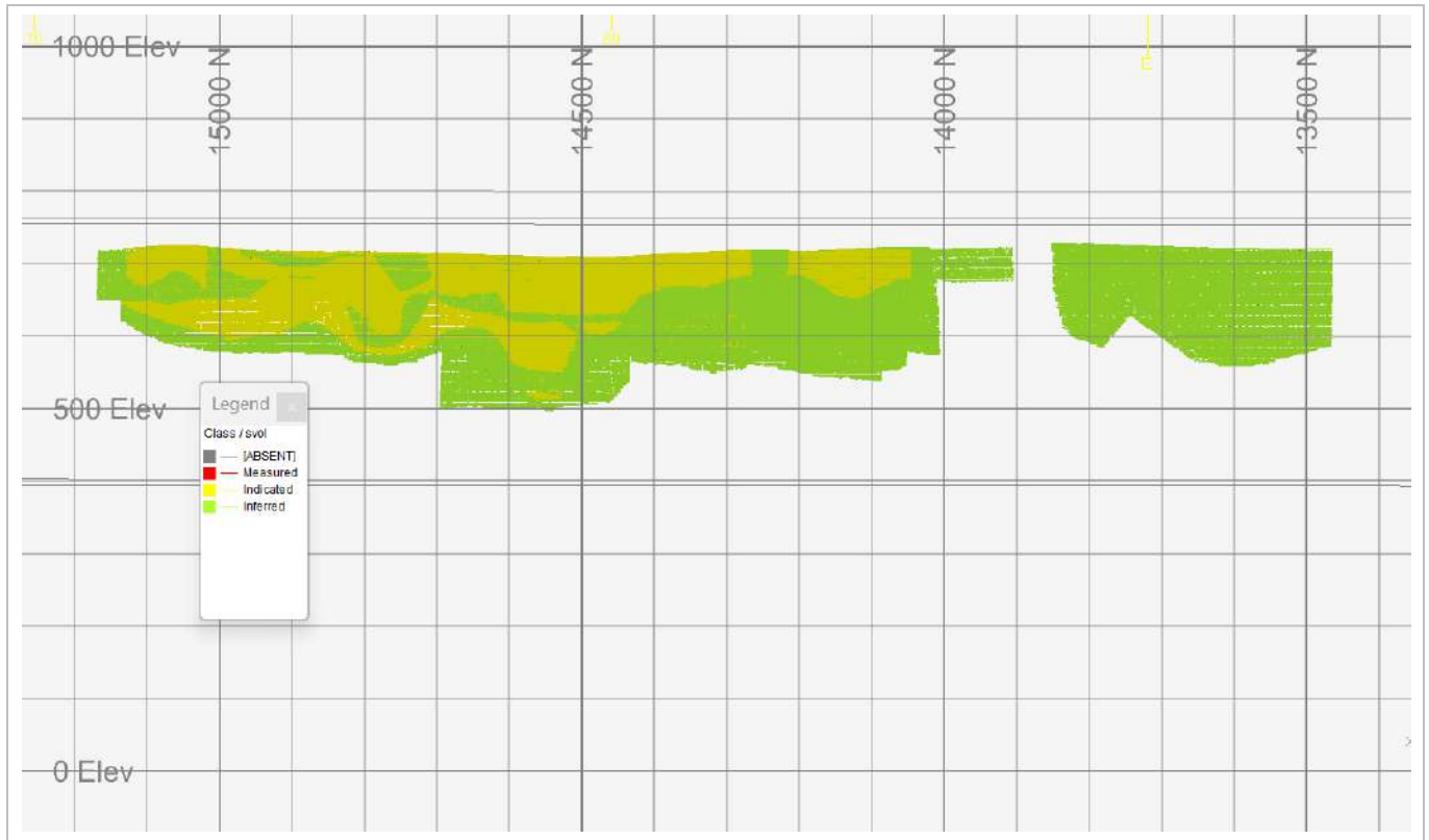
Figure 14-61: Maki Medina Mineral Resource Classification Long Section (EDV 2025)
