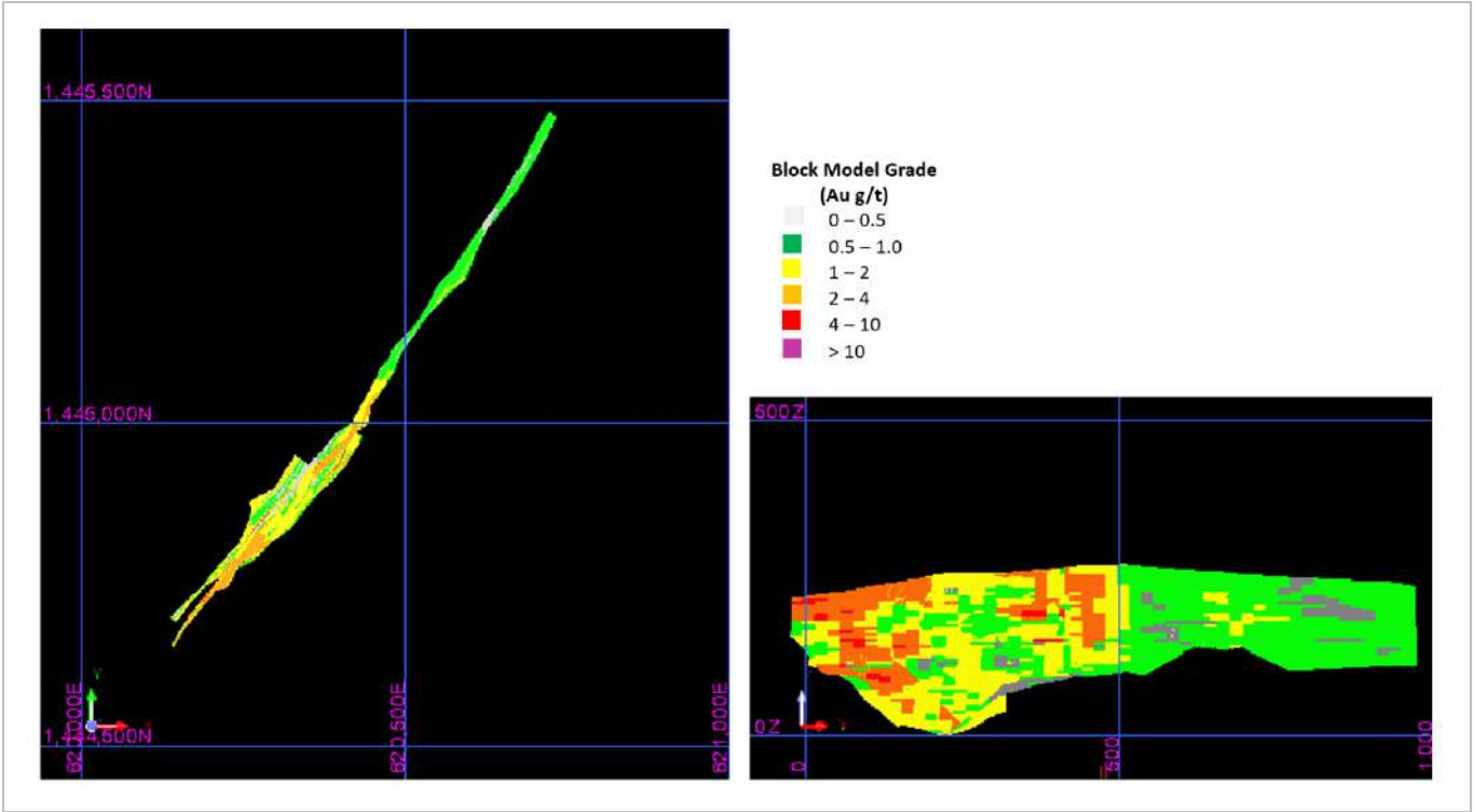
Figure 14-76: Kiesta A Grade Block Model Plan and SE-NW Long Section Views (EDV 2025)
