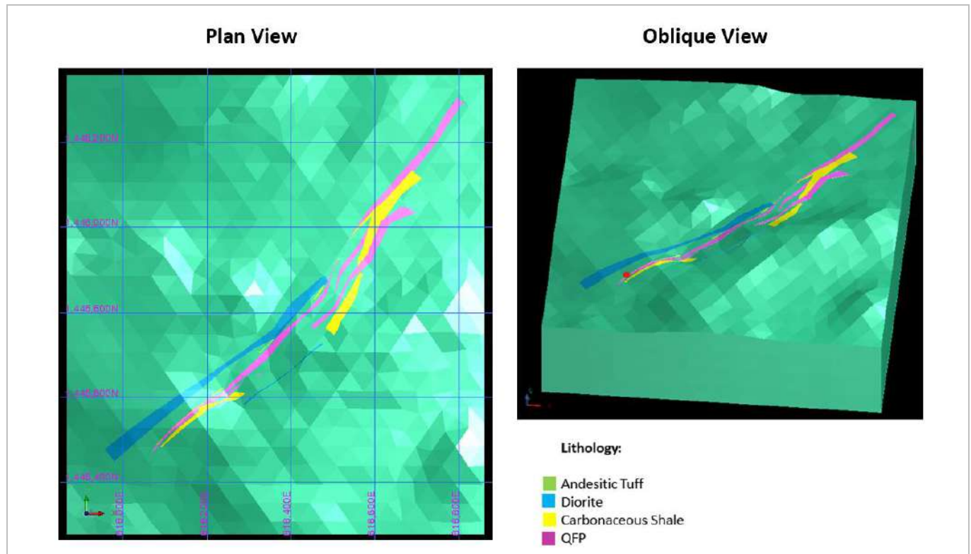
Figure 14-7: Kiesta C Lithological Model (EDV, 2025)
