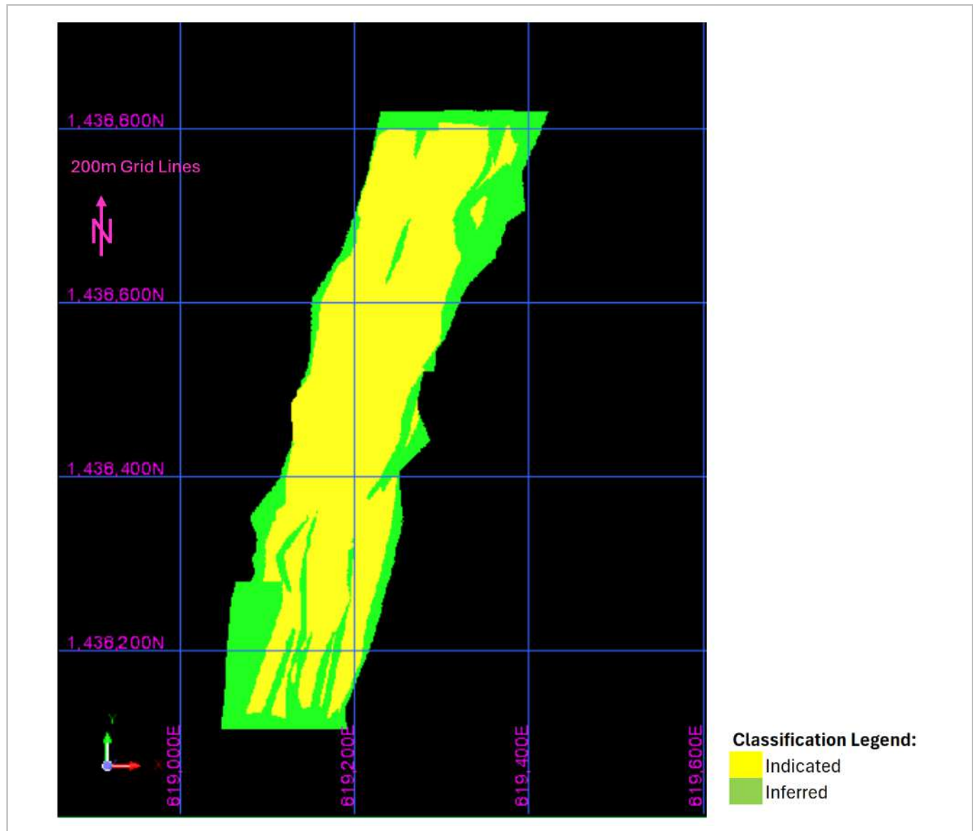
Figure 14-69: Tina Mineral Resource Classification
