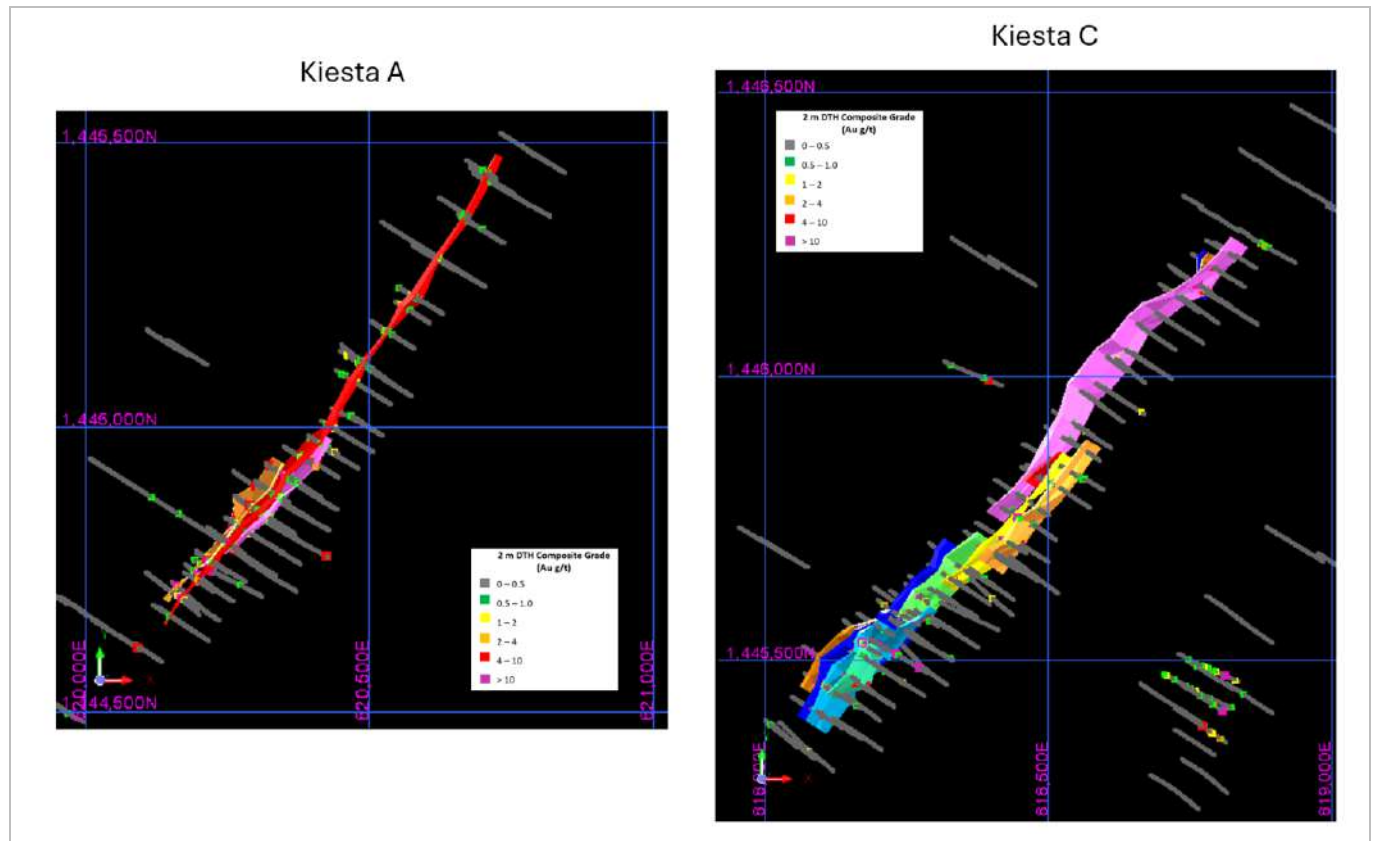
Figure 14-24: Kiesta A and Kiesta C Mineralisation, Plan View (EDV, 2025)
