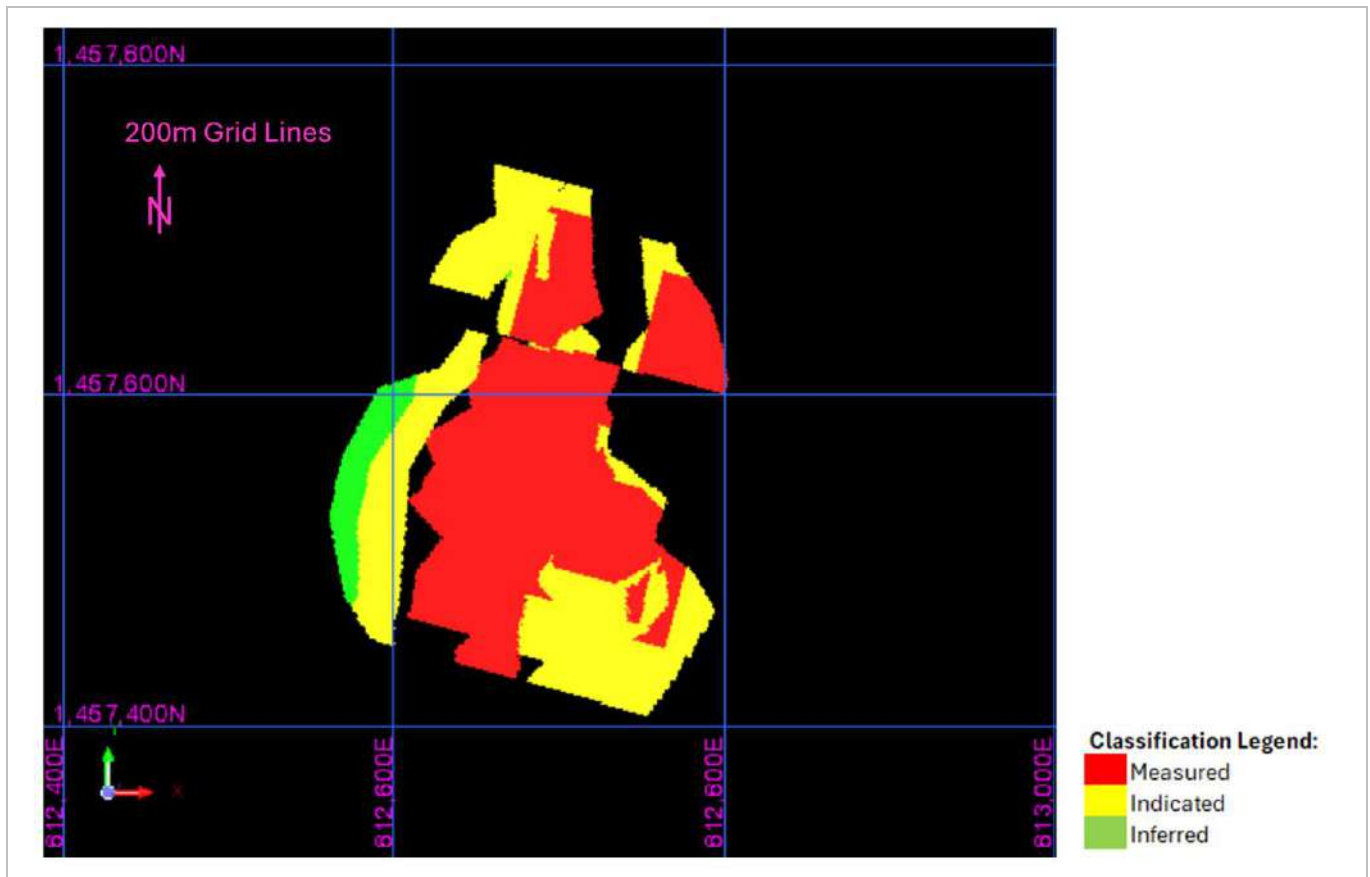
Figure 14-68: Soukhoto Mineral Resource Classification Plan View (EDV 2025)
