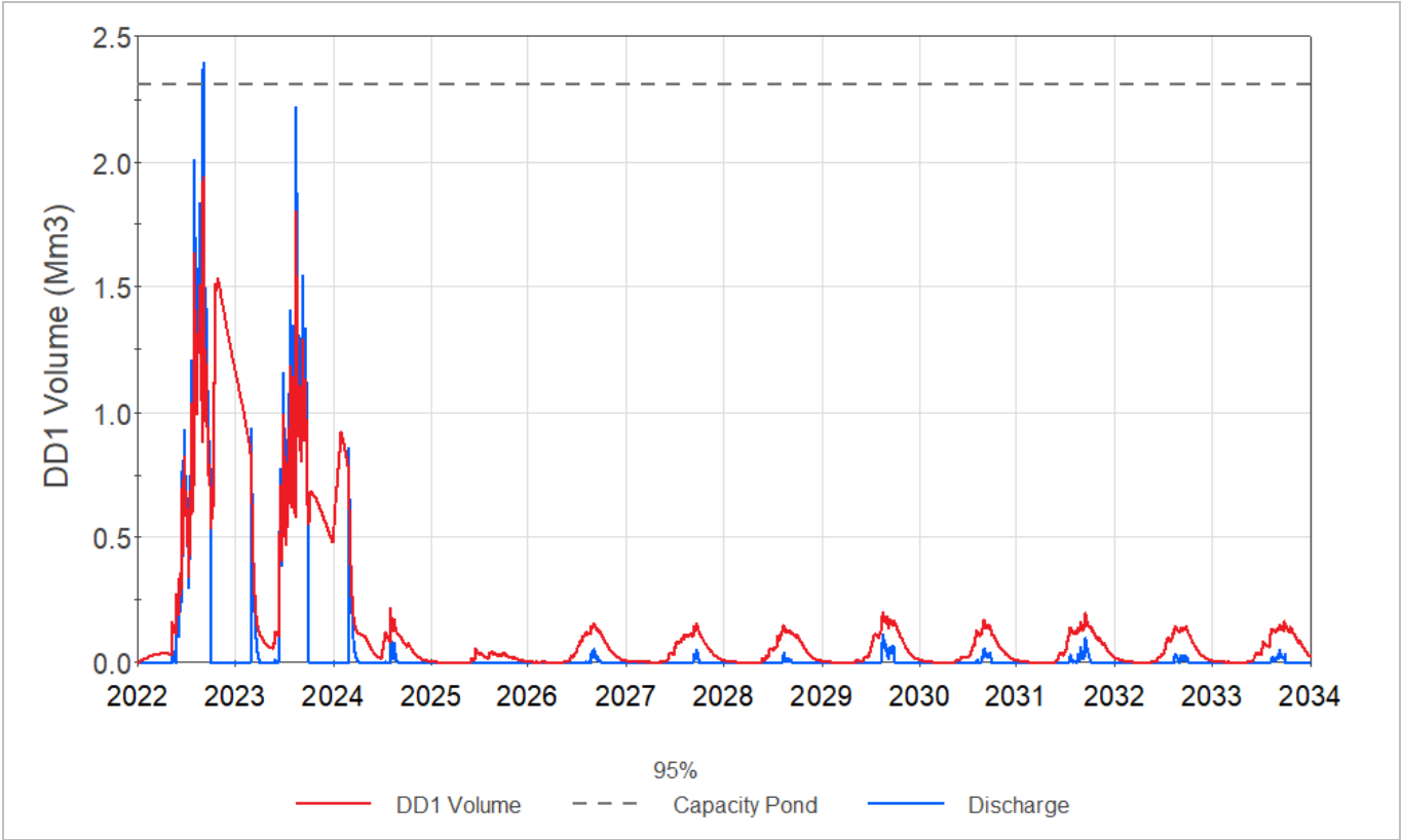
Figure 18-12: DD1 Modelled Volume and Discharge (95 th Percentile)
