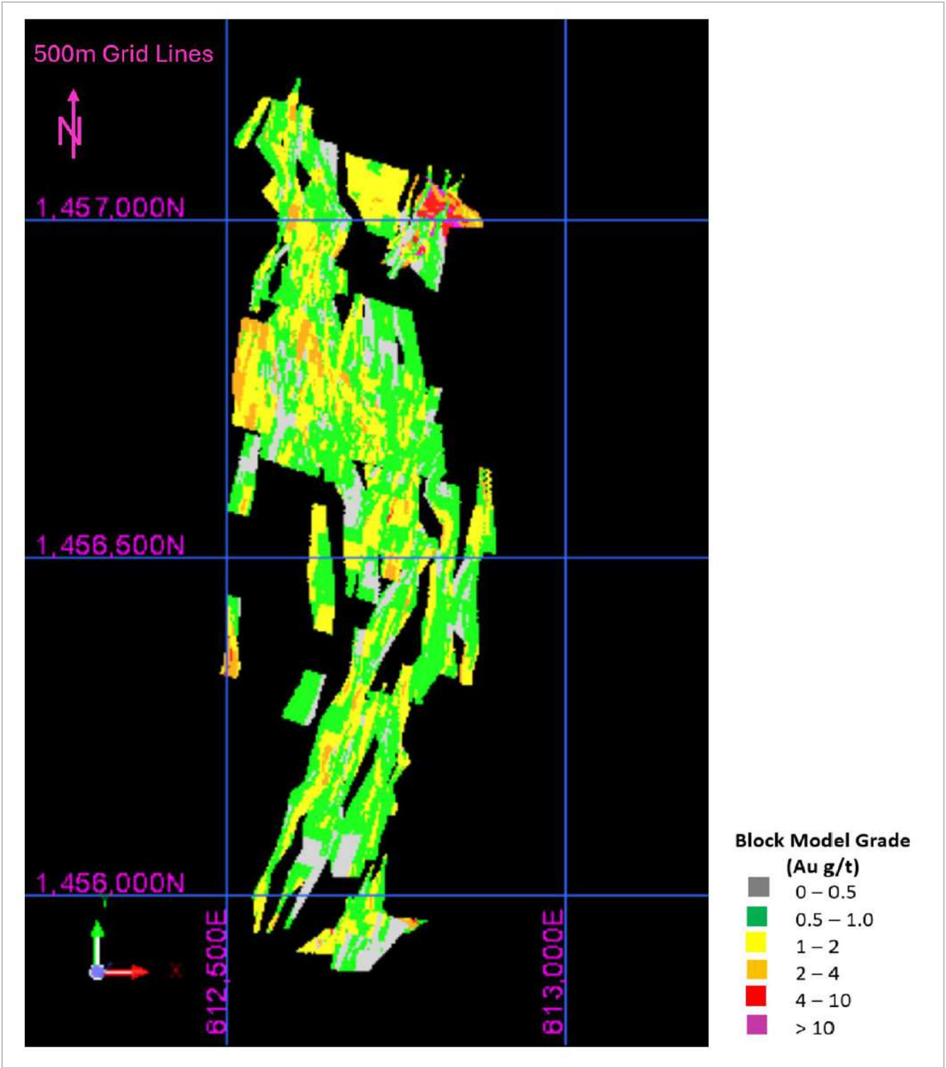
Figure 14-85: Niakafiri West Grade Block Model Plan View (EDV 2025)
