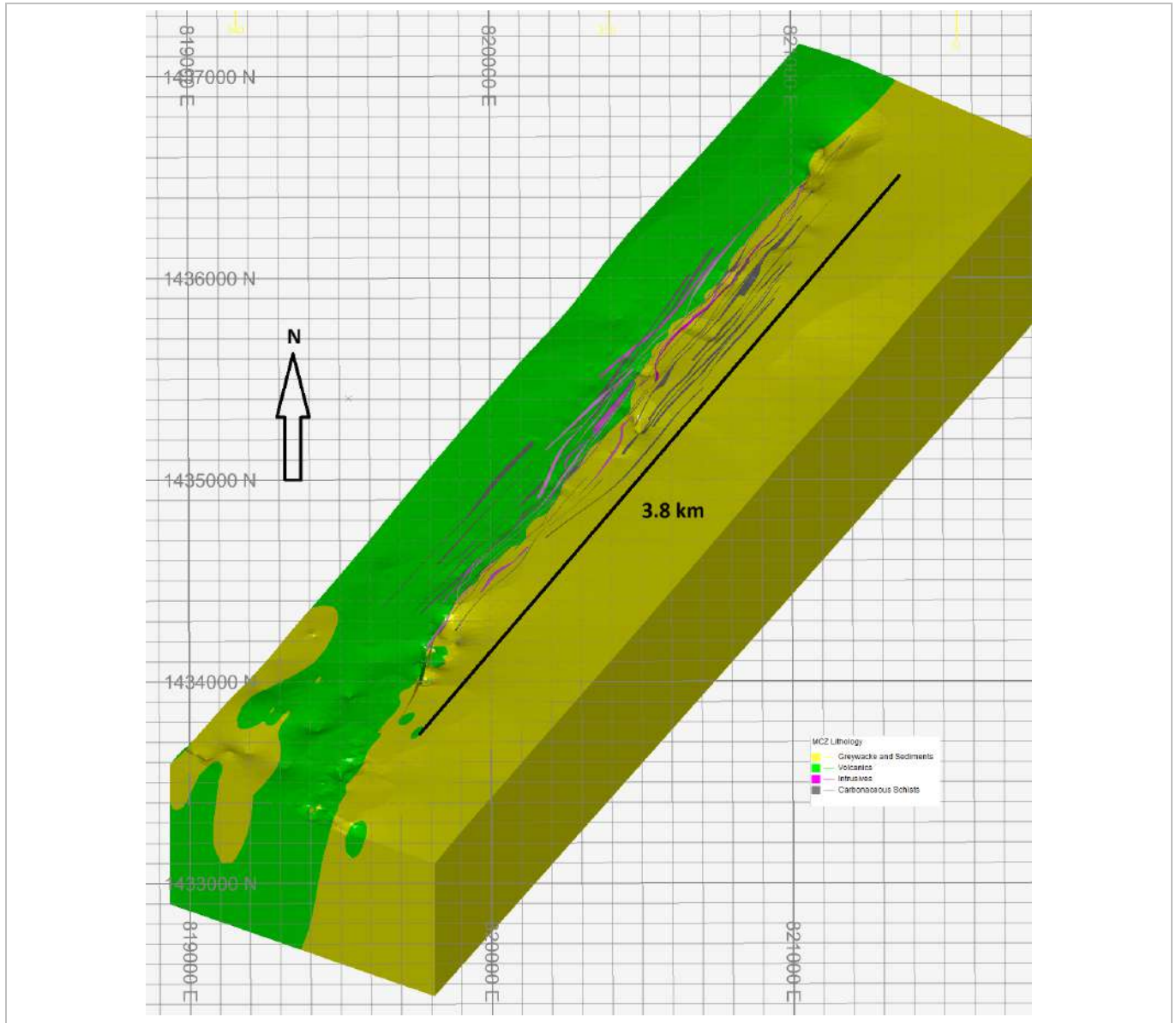
Figure 14-13: MNZ Lithological Model, Oblique View (EDV, 2025)
