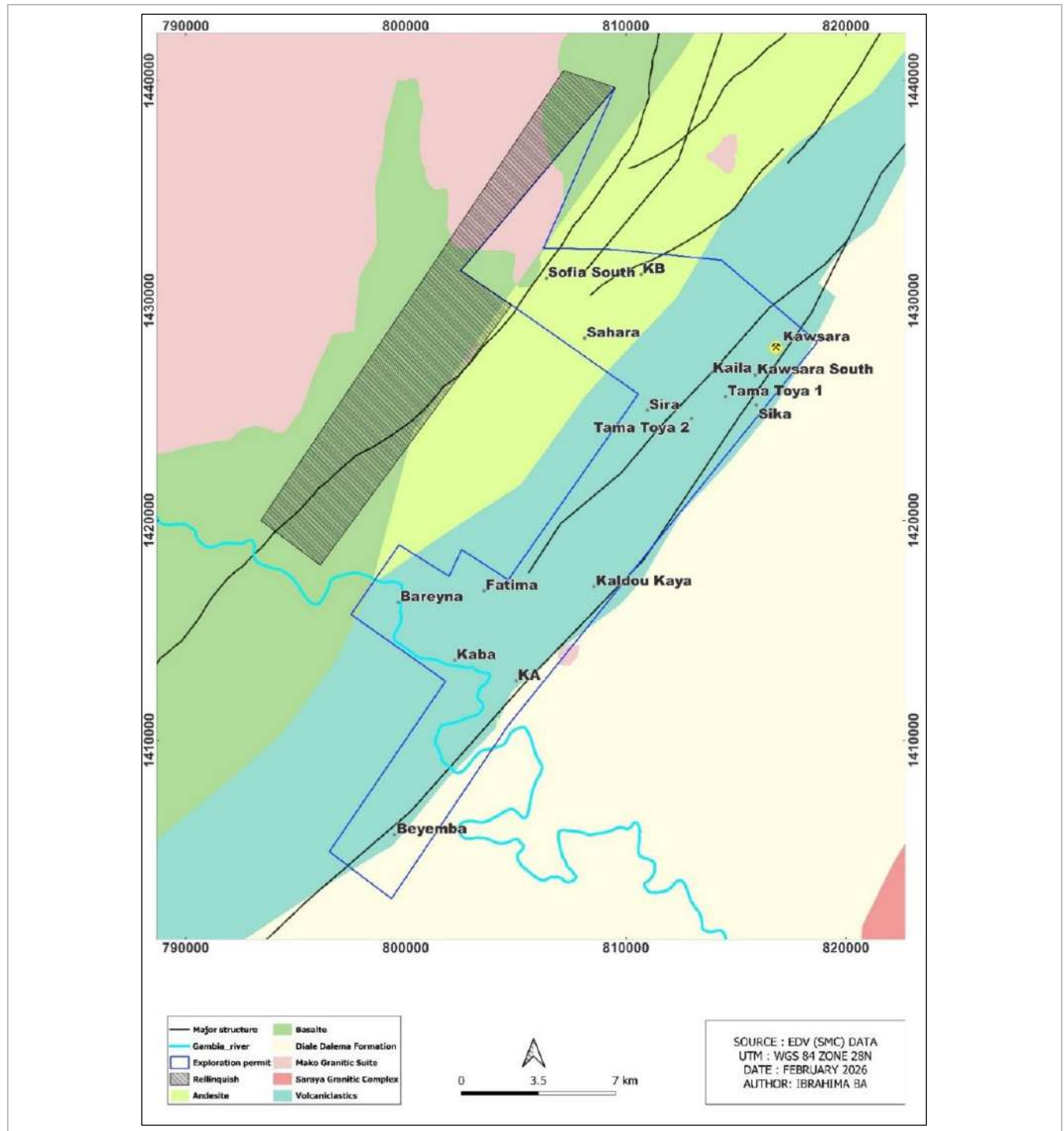
Figure 7-19: Kanoumba Geological Map with Deposits and Prospects (EDV, 2025a)
