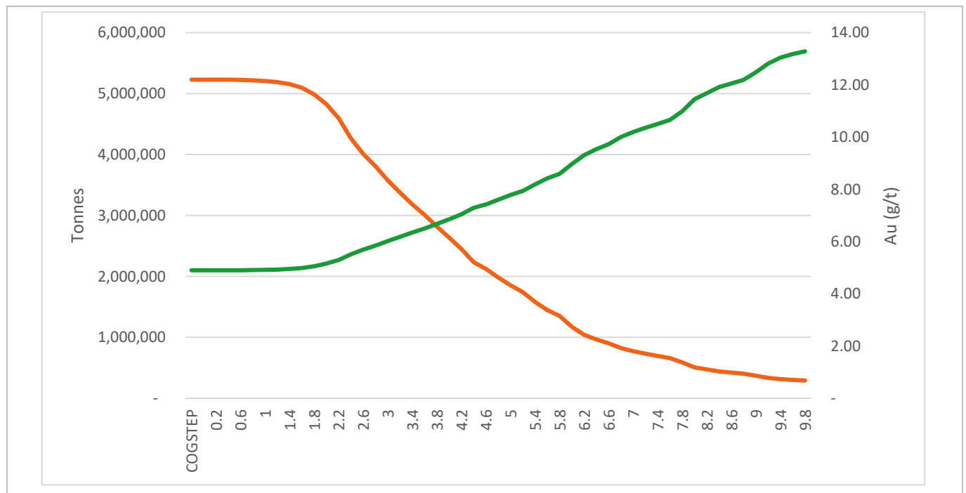
Figure 14-89: Golouma Underground Grade-Tonnage Curve (EDV 2025)
