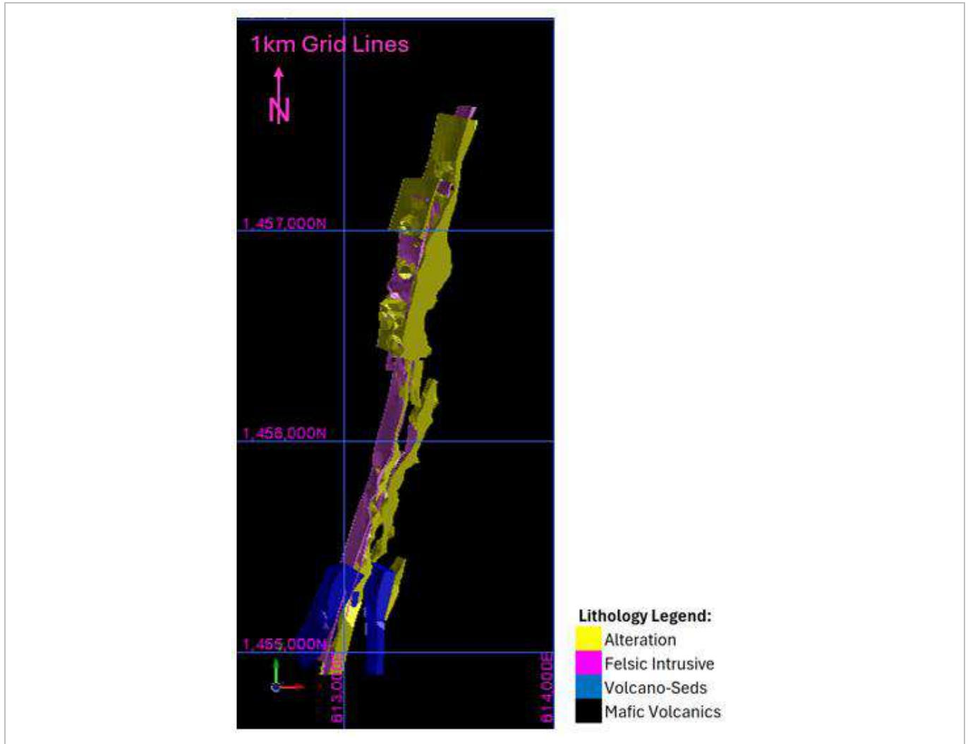
Figure 14-14: Niakafiri East Lithological Model Plan View (EDV, 2025)
