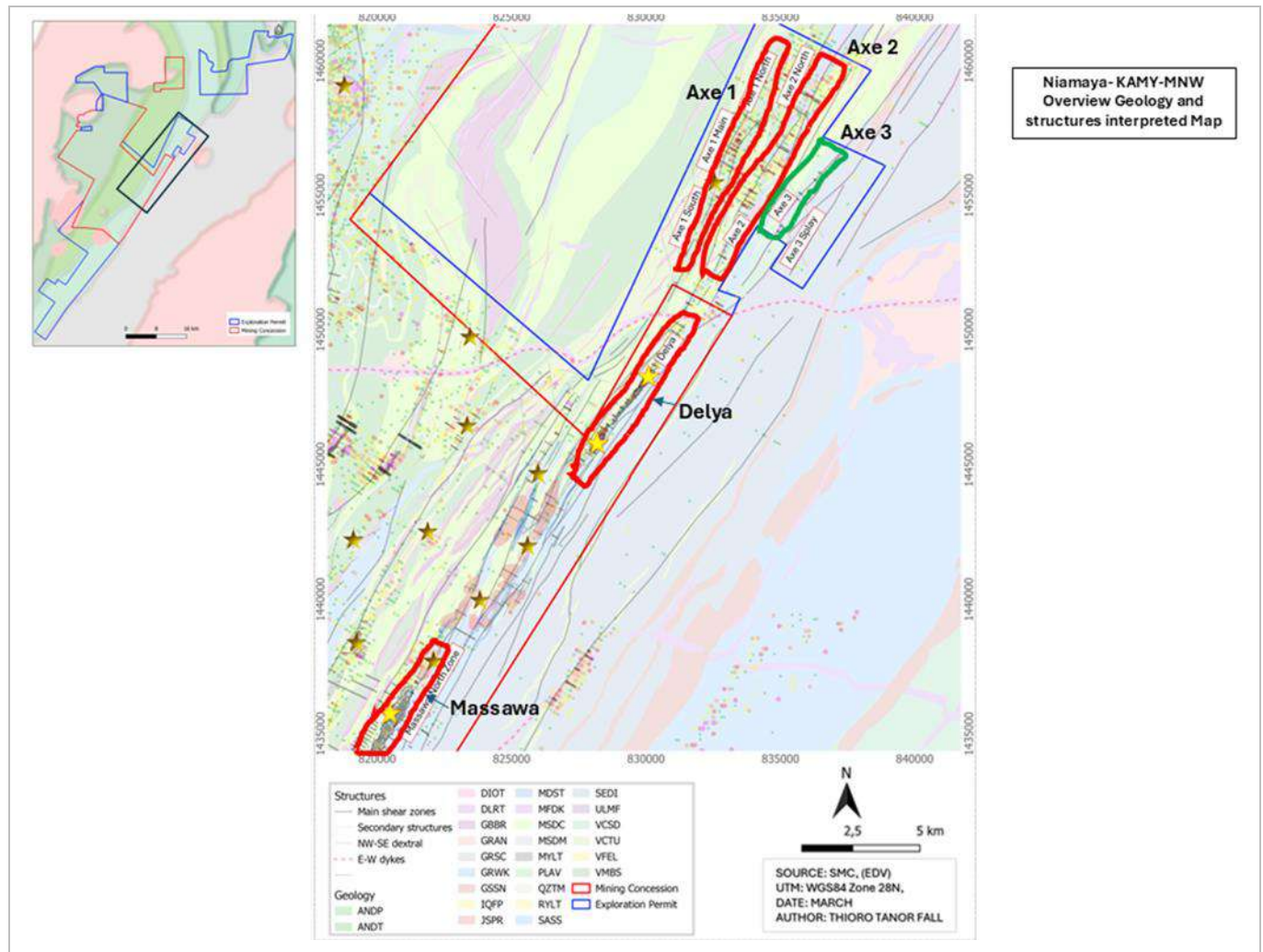
Figure 9-5: Niamaya Geology and Exploration Activities (2022 -2025)
