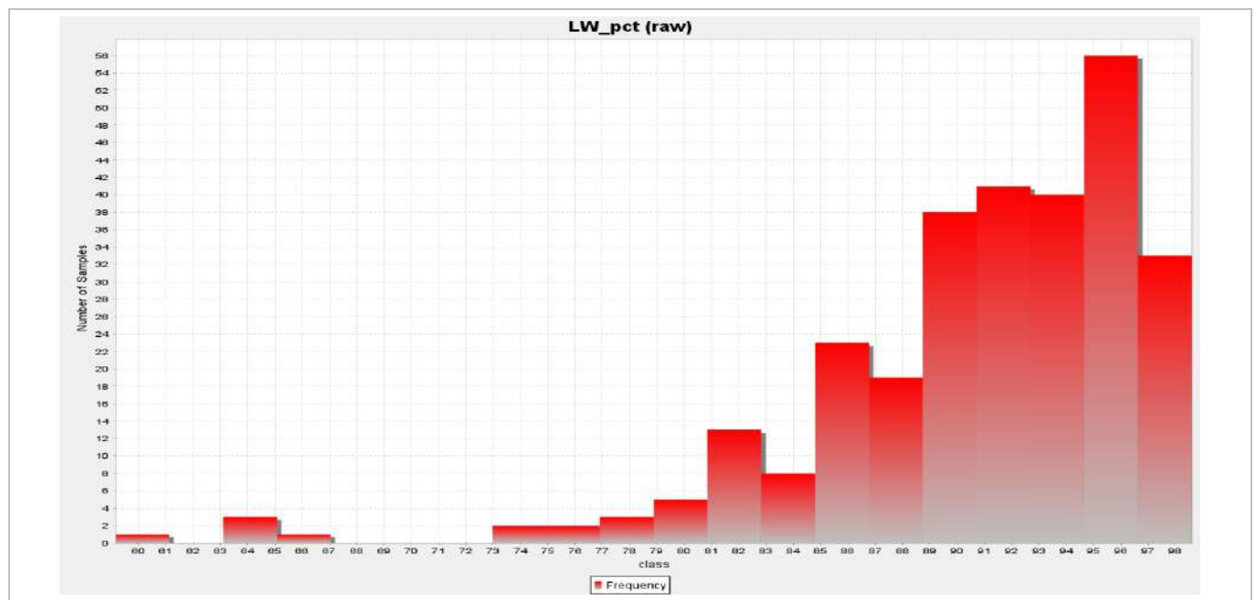
Figure 14-36: Plot of Samina Exploration LeachWell % Results (> 0.2 g/t Au), (EDV, 2025)
