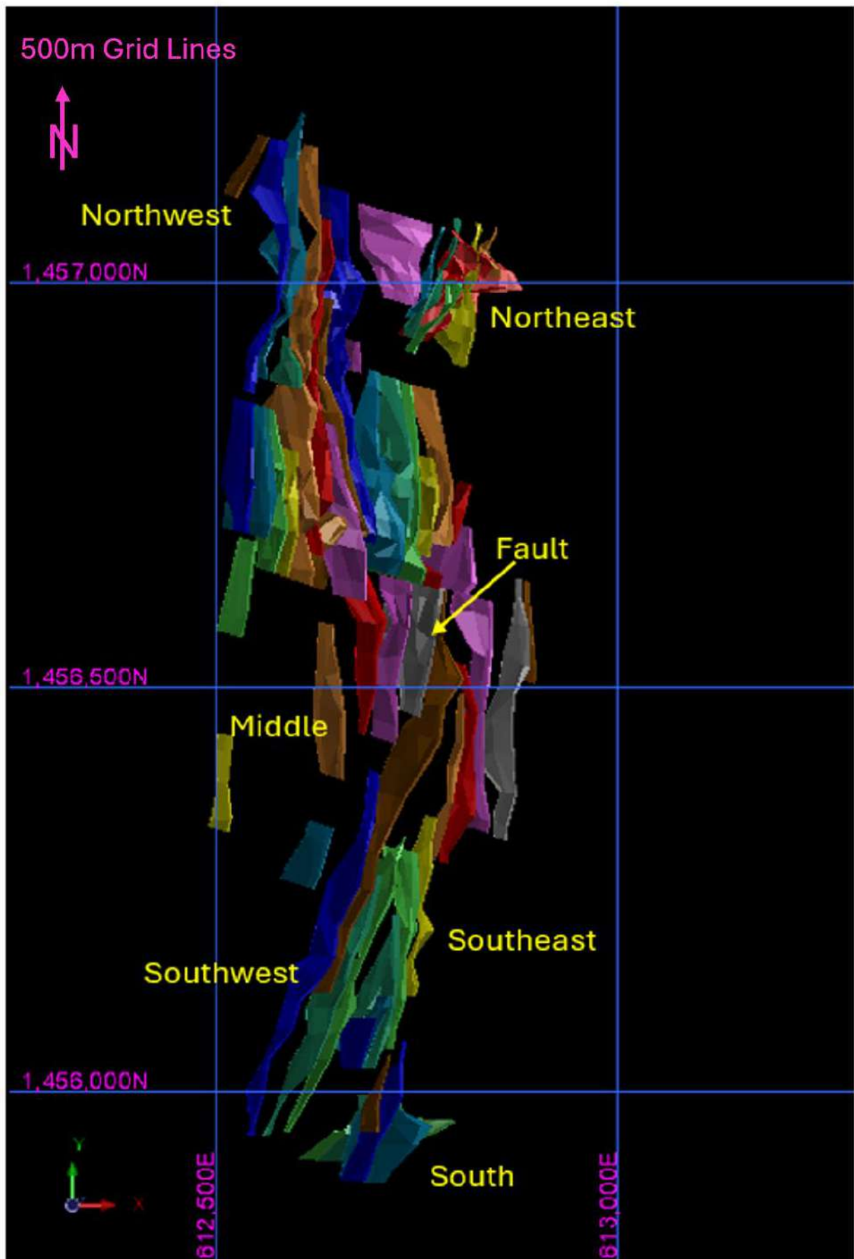
Figure 14-32: Niakafiri West Mineralisation Zones and Domains, Plan View (EDV, 2025)
