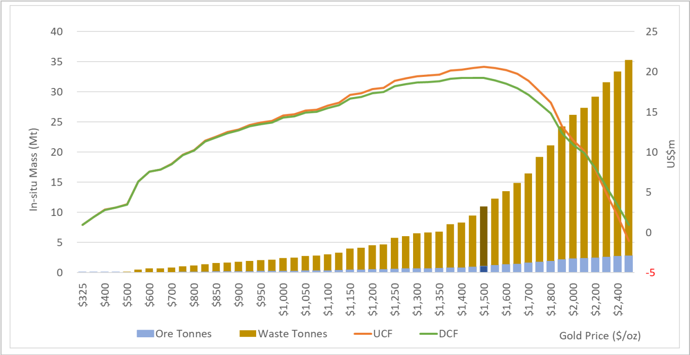
Figure 15-9: Goumbati West Optimisation Results
