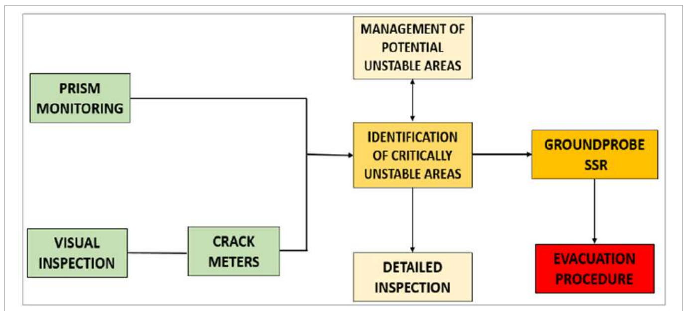
Figure 16-1: Slope Monitoring Strategy Across the Open-Pits at the Mine
