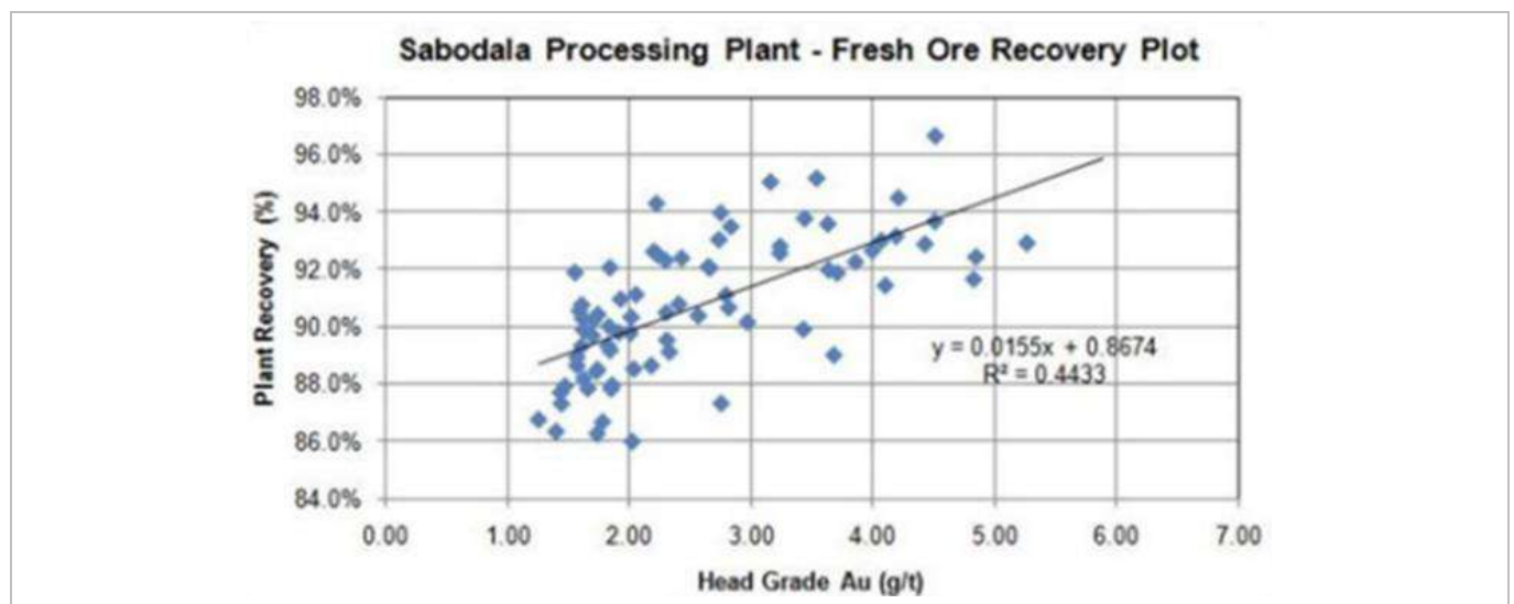
Figure 13-8: April-July 2010 Operational Data Supporting Sabodala Fresh Recovery Modelling
