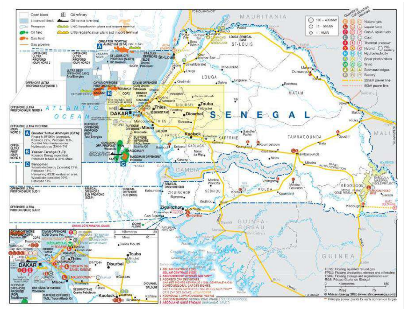
Figure 18-4: The National Electricity Grid of Senegal (ECG, 2025)
