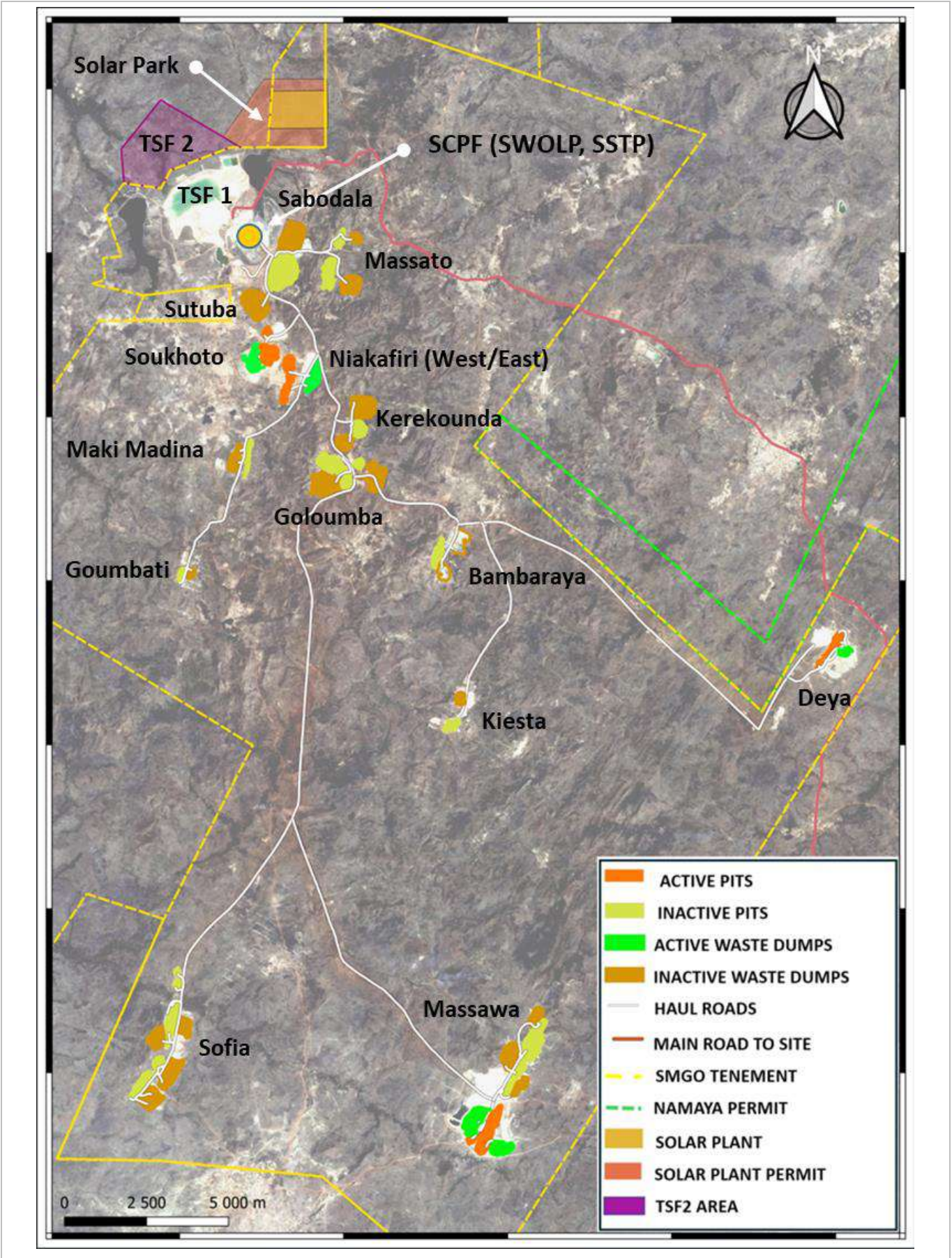
Figure 18-1: Sabodala MC Infrastructure GA (EDV, 2025)
