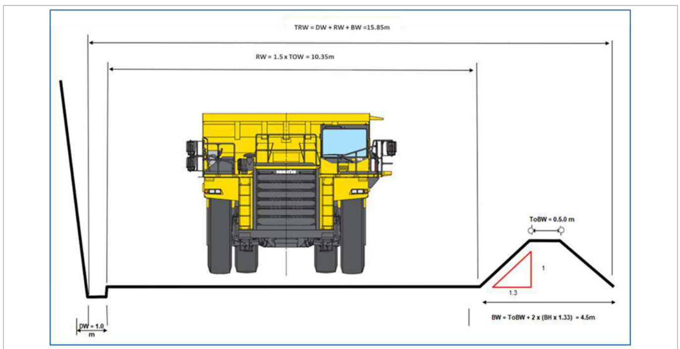
Figure 15-13: Single Lane Haul Road Width
