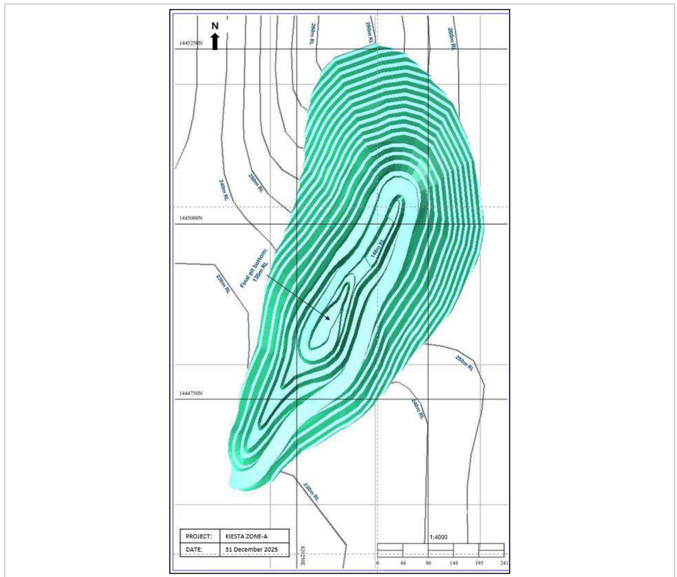
Figure 15-15: Kiesta A Pit Design (EDV, 2025)
