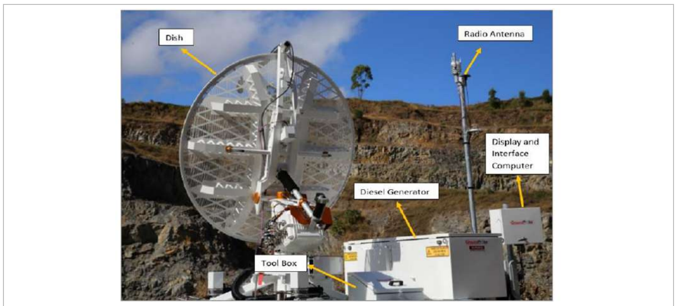
Figure 16-2: Ground Probe Slope Stability Radar – XT (SGO, 2025)
