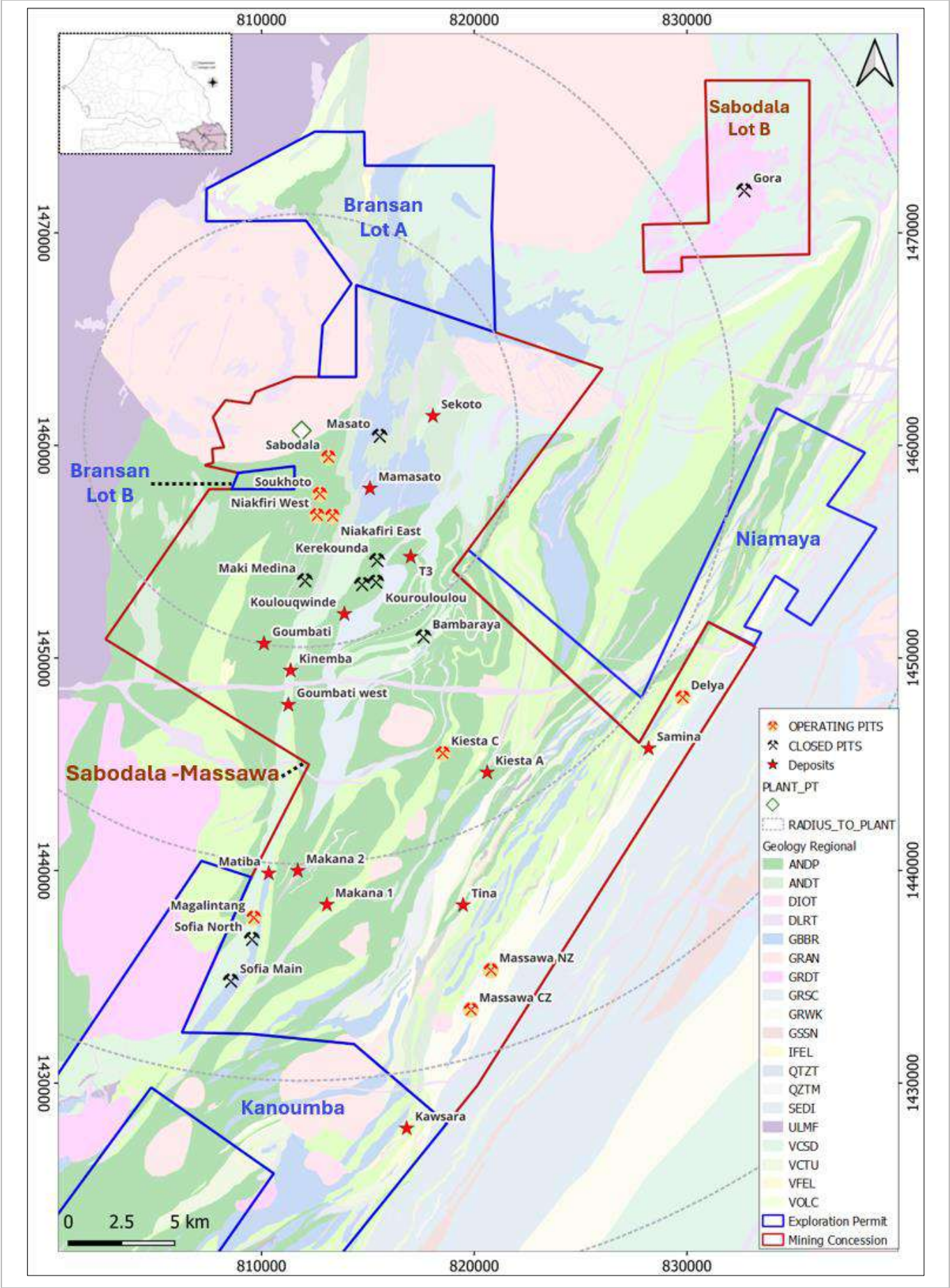
Figure 15-1: Sabodala MC Site Layout Map (EDV, 2025)
