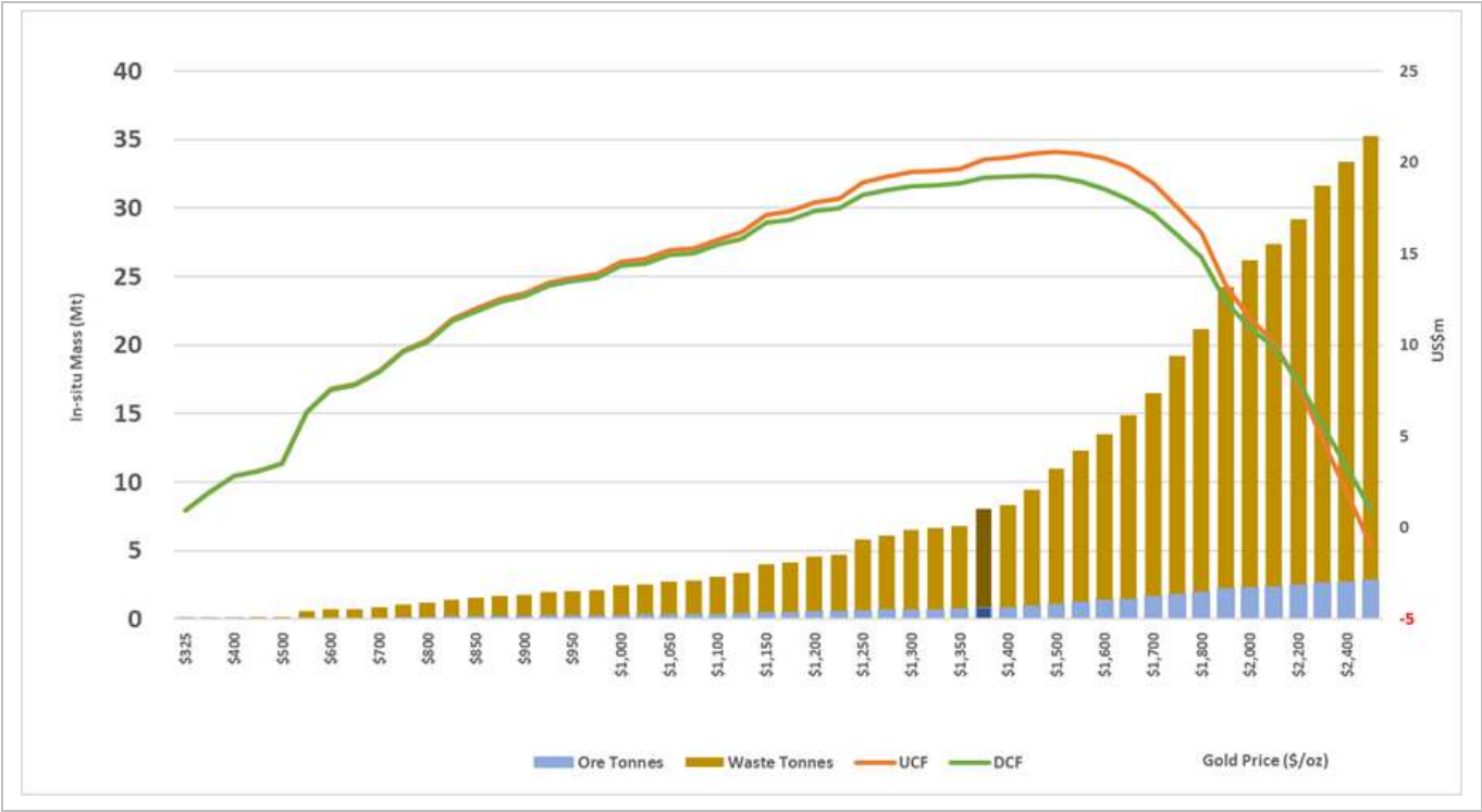
Figure 15-6: Goumbati West Optimisation Results
