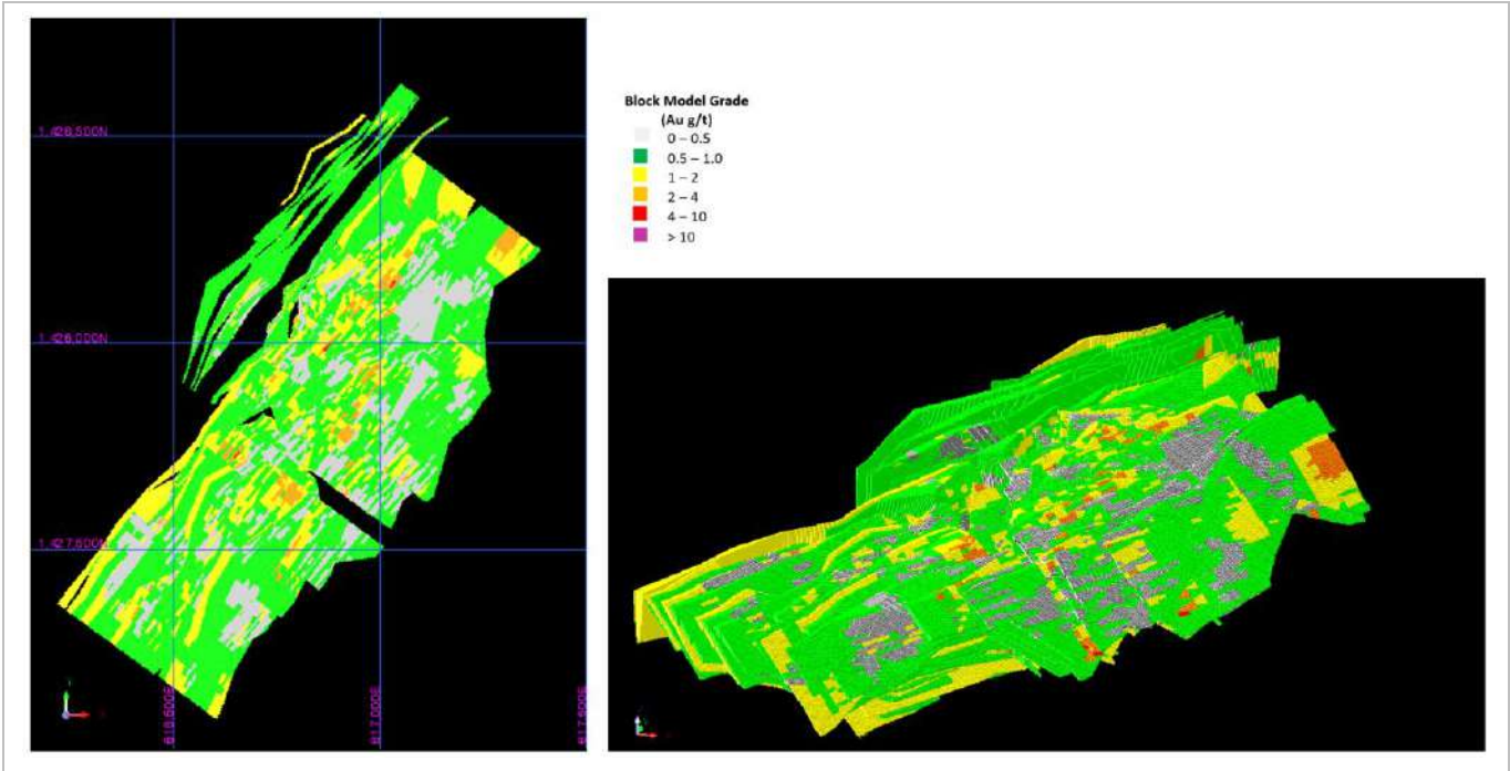
Figure 14-73: Kawsara Grade Block Model Plan and Oblique Views (EDV 2025)
