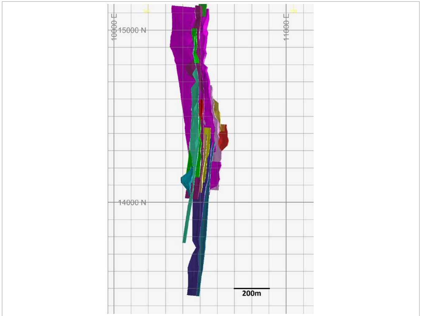
Figure 14-26: Maki Medina Mineralisation, Plan View (EDV, 2025)
