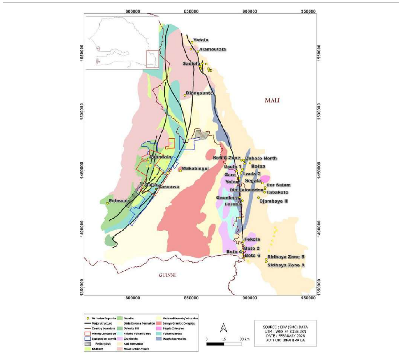
Figure 7-2: Schematic Geology of the Kédougou-Kenieba Inlier (EDV, 2025a)
