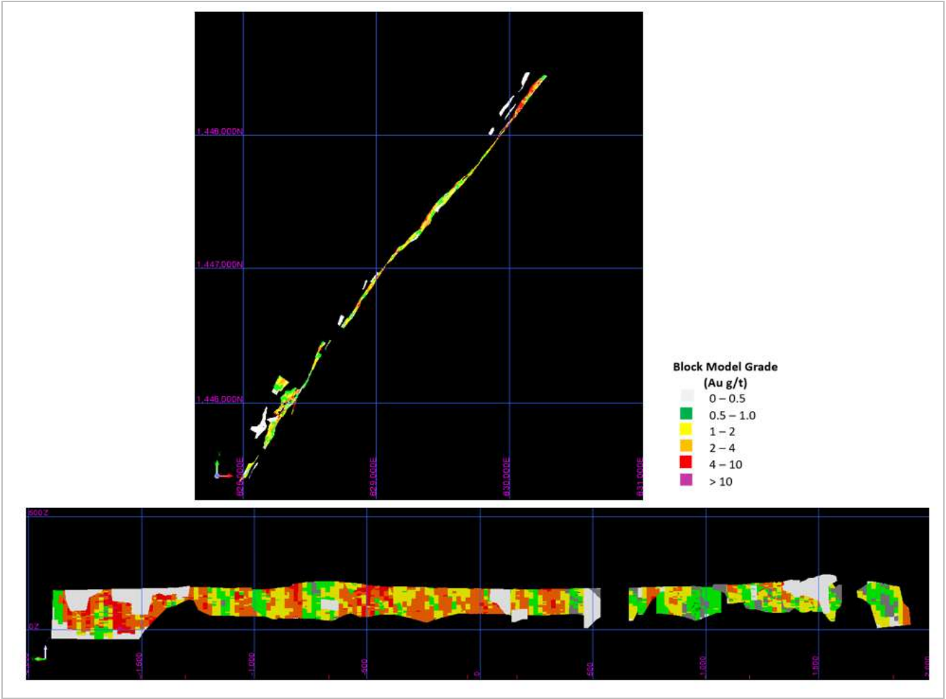
Figure 14-70: Delya-Samina Grade Block Model Plan and Long Section Views (EDV 2025)
