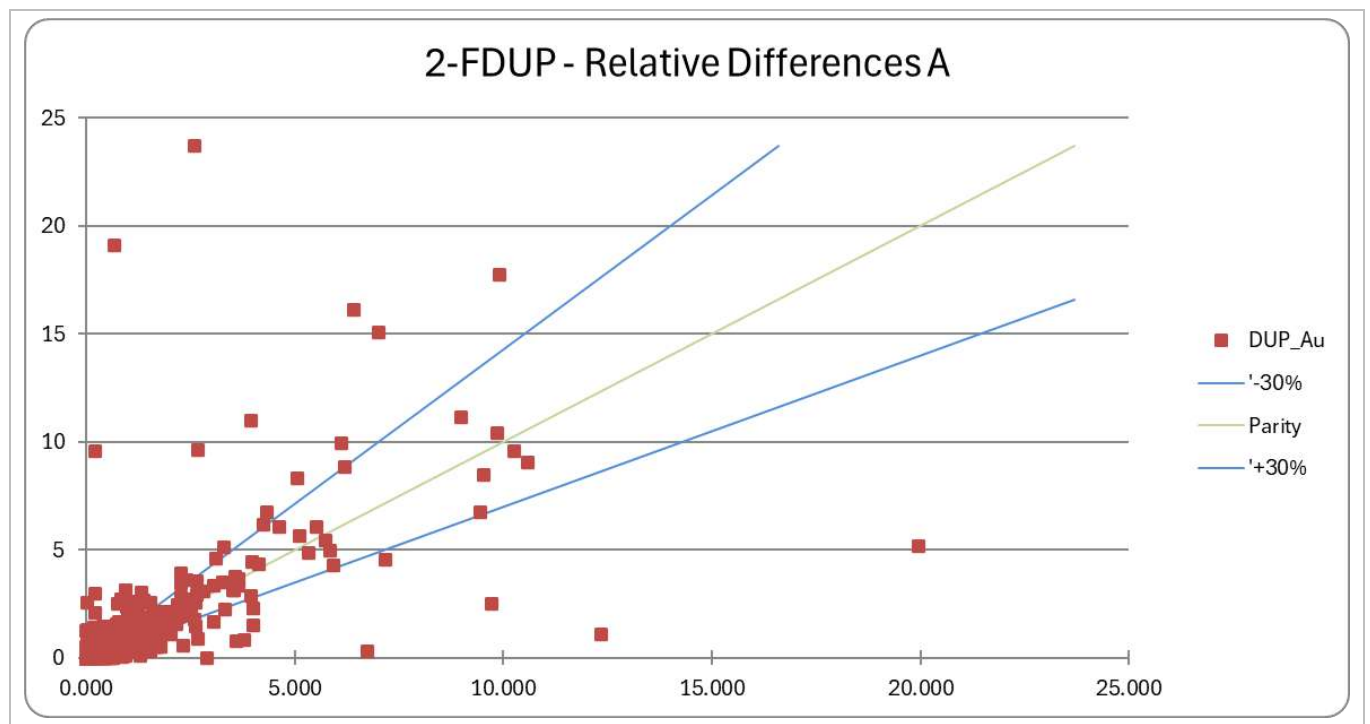
Figure 11-6: Example of X-Y Scatterplot of Original v Field Duplicate (ALSKU, Massawa)
