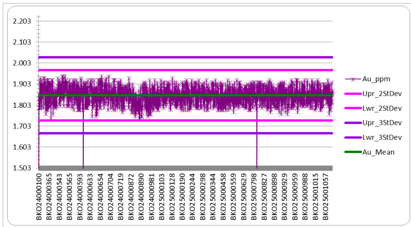
Figure 11-9: Example of a CRM Control Chart (BV-Bk, Massawa, OREAS236 (1.85 ppm Au))
