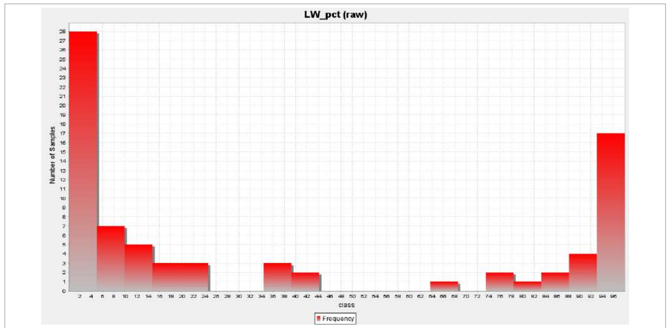
Figure 14-35: Plot of Delya South Exploration LeachWell % Results (> 0.2 g/t Au), (EDV, 2025)
