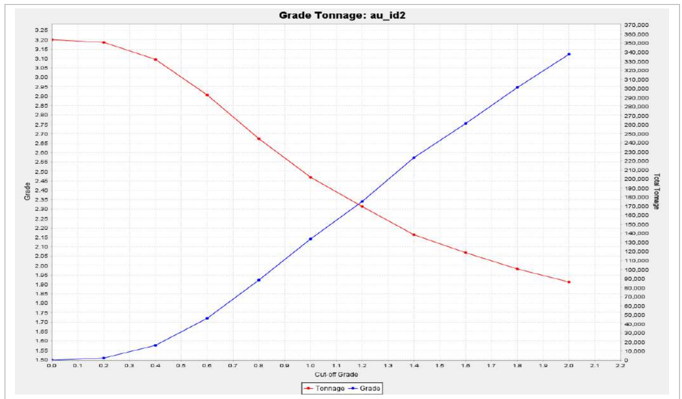
Figure 14-104: Soukhoto Grade-Tonnage Curve Within USD 2100 Pit Shell (Un-depleted) (EDV2025)
