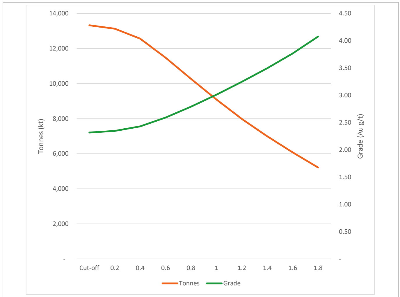
Figure 14-100: MCZ Grade-Tonnage Curve Within USD 2100/oz Whittle Pit (EDV 2025)
