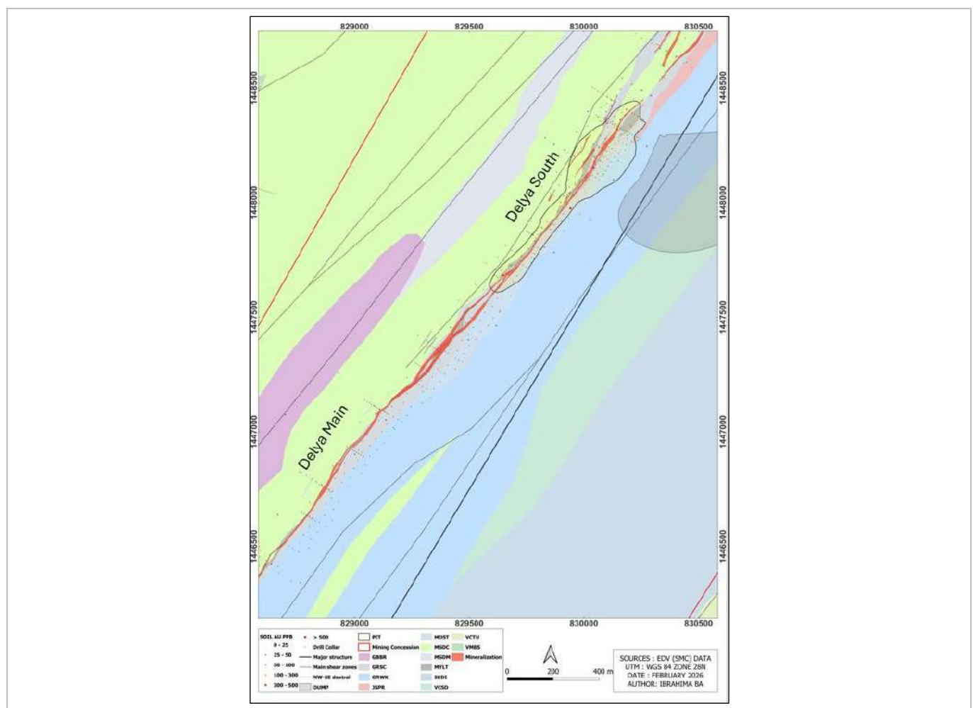
Figure 7-17: Delya Geological Map (EDV, 2025a)
