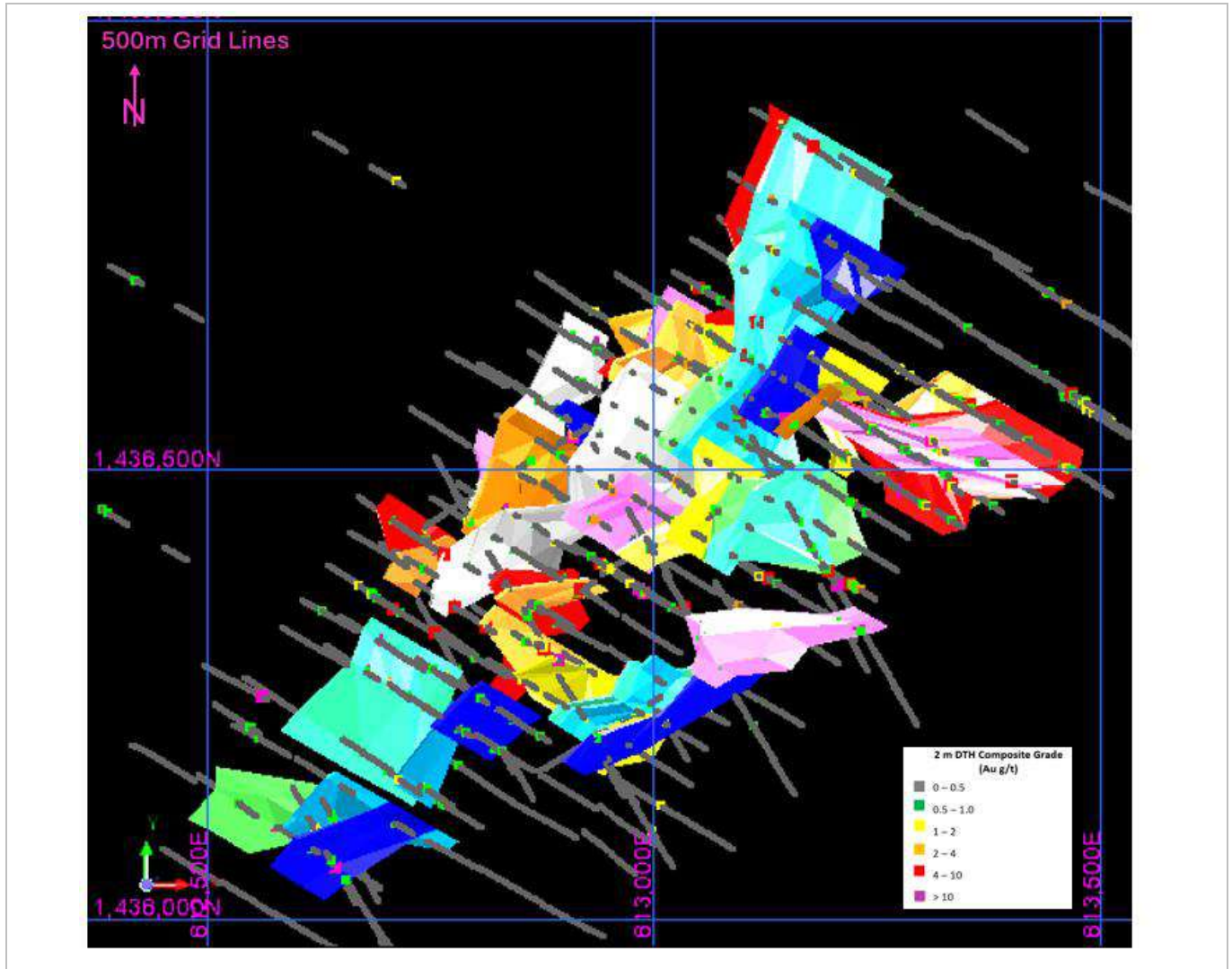
Figure 14-25: Makana 1 Mineralisation, Plan View (EDV, 2025)
