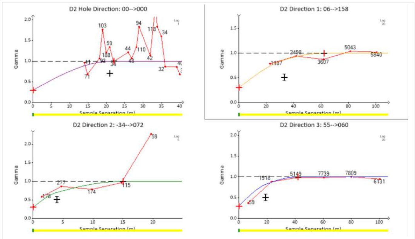
Figure 14-40: Kerekounda Mineral Zone 4 Variogram (EDV, 2025)
