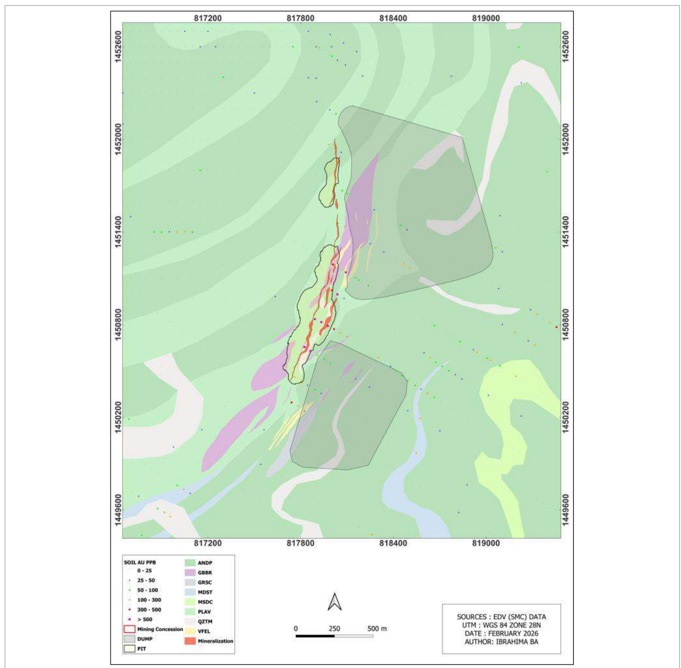
Figure 7-12: Geological Map of the Bambaraya Deposit (EDV, 2025a)
