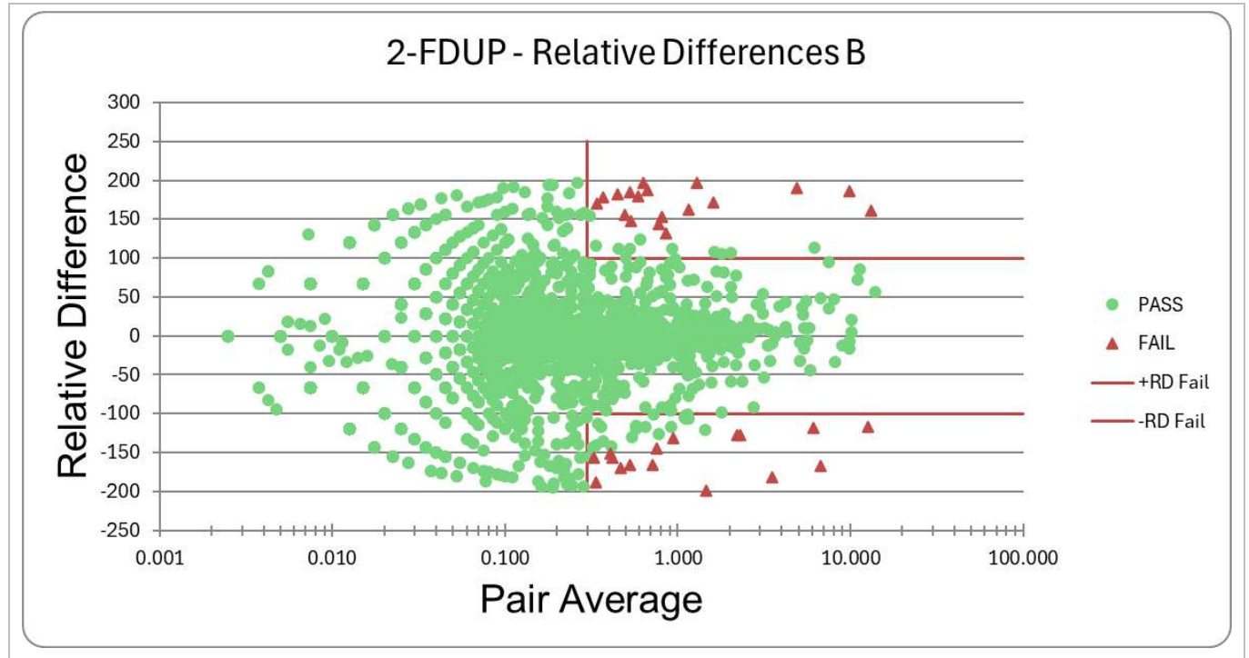
Figure 11-7: Example of a Sample Pair Average versus Log Relative Difference Chart (ALSKU, Massawa)
