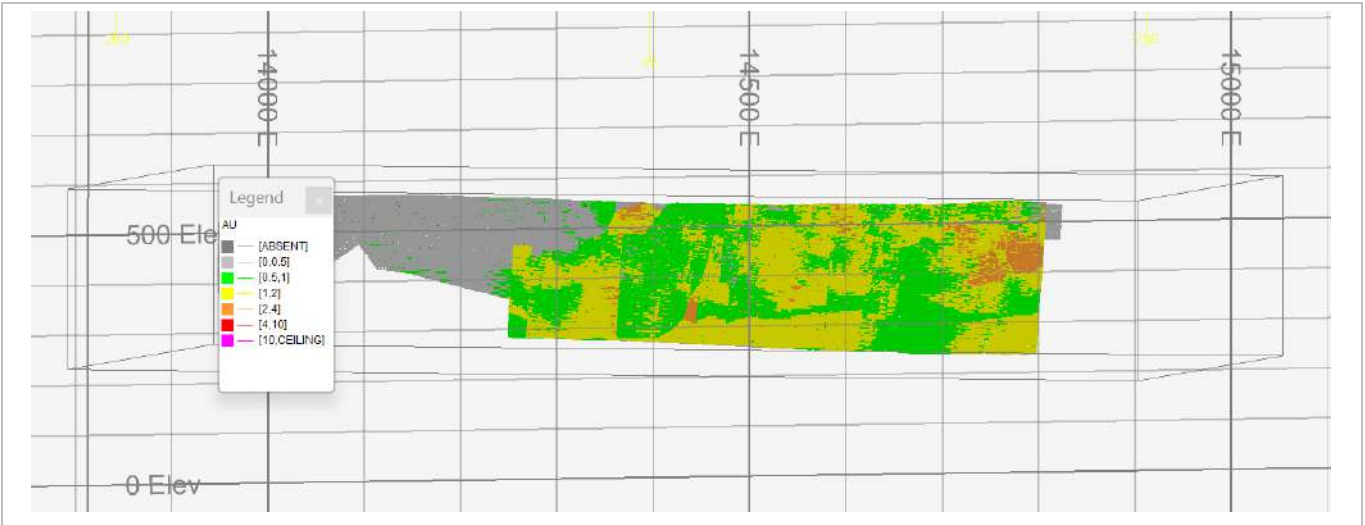
Figure 14-79: Maki Medina Grade Block Model (EDV 2025)
