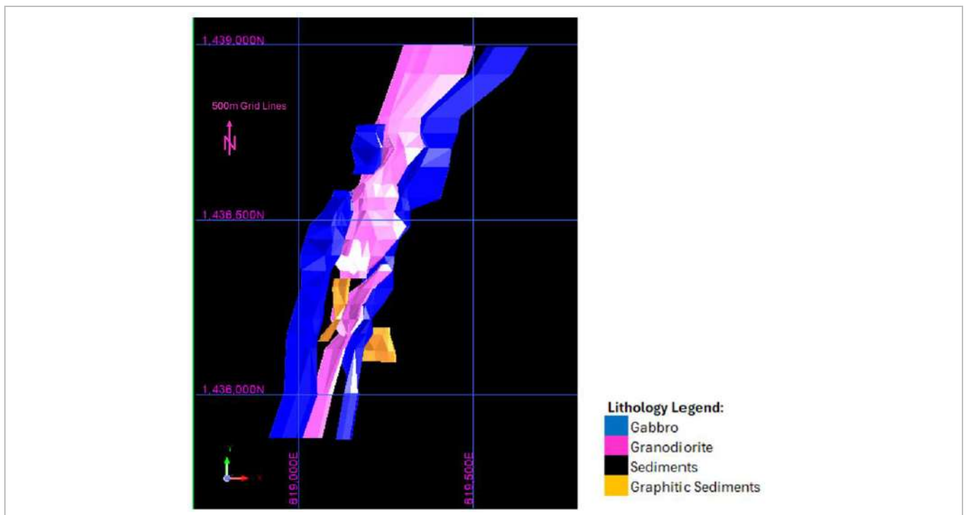
Figure 14-17: Tina Lithological Model, Plan View (EDV, 2025)
