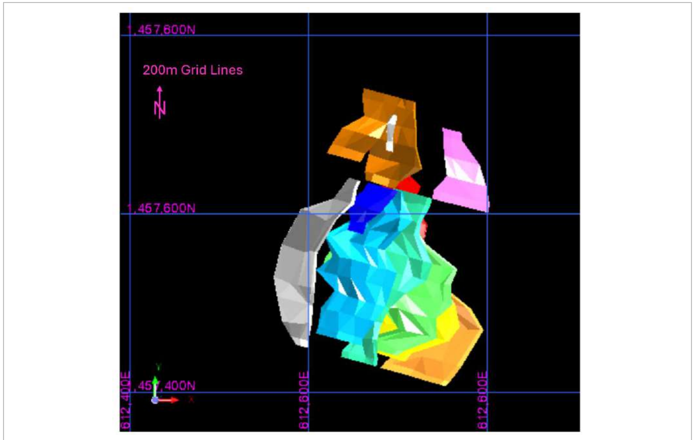
Figure 14-33: Soukhoto Mineralisation Zones, Plan View (EDV, 2025)
