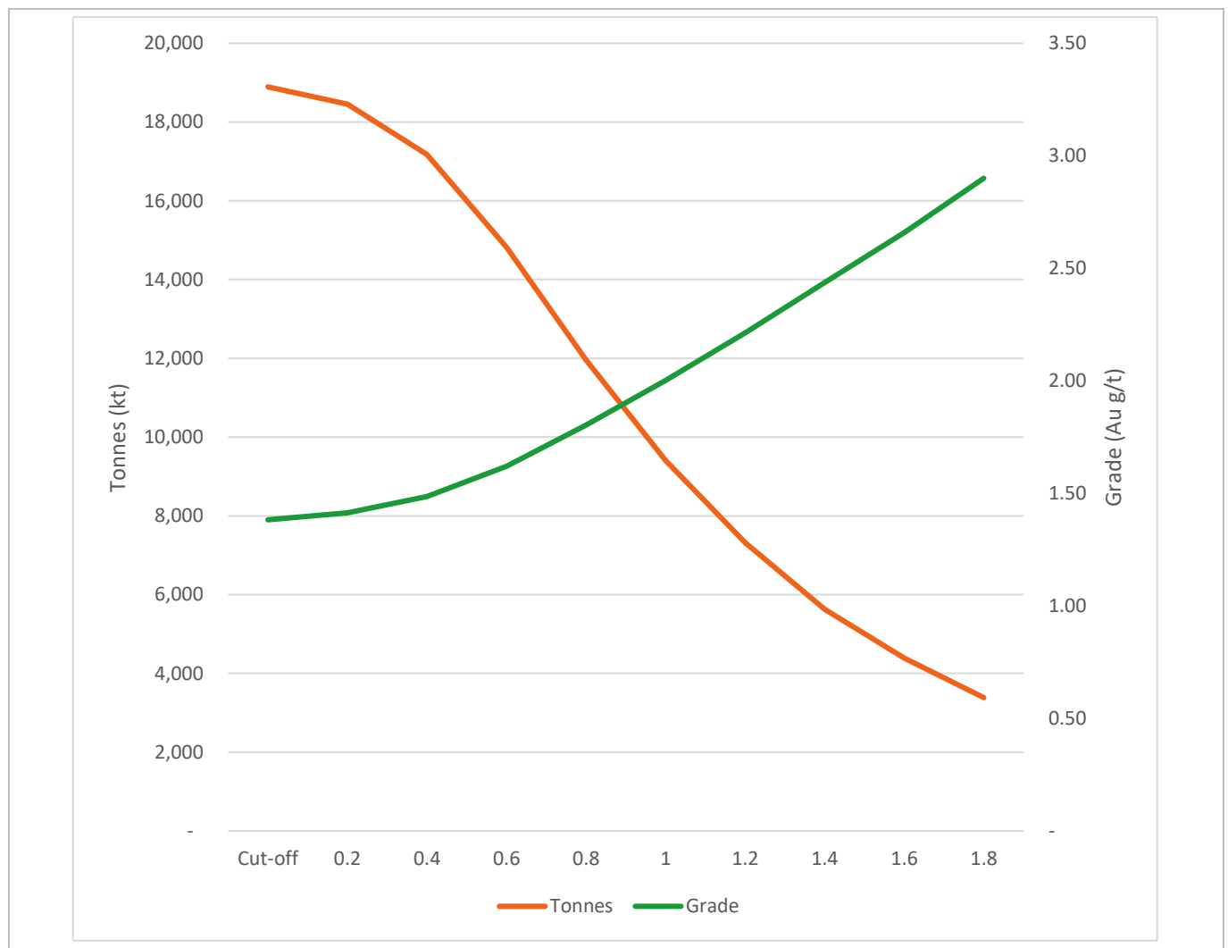
Figure 14-99: Masato Grade-Tonnage Curve Within USD 2100/oz Whittle Pit (EDV 2025)
