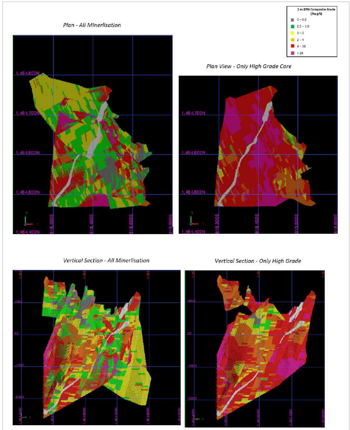
Figure 14-74: Kerekounda Grade Block Model Plan and Vertical Section Views (EDV 2025)
