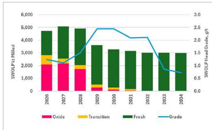
Figure 17-3: SWOLP LoM Mill Feed by Weathering
