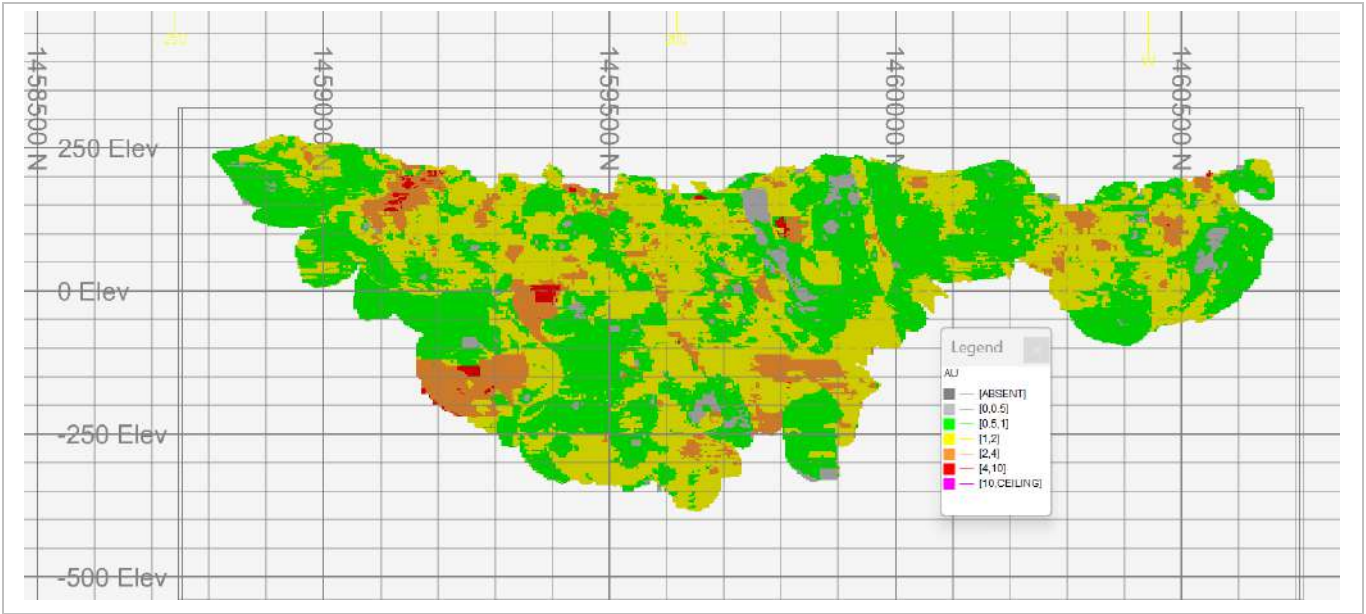
Figure 14-81: Masato Grade Block Model (EDV 2025)
