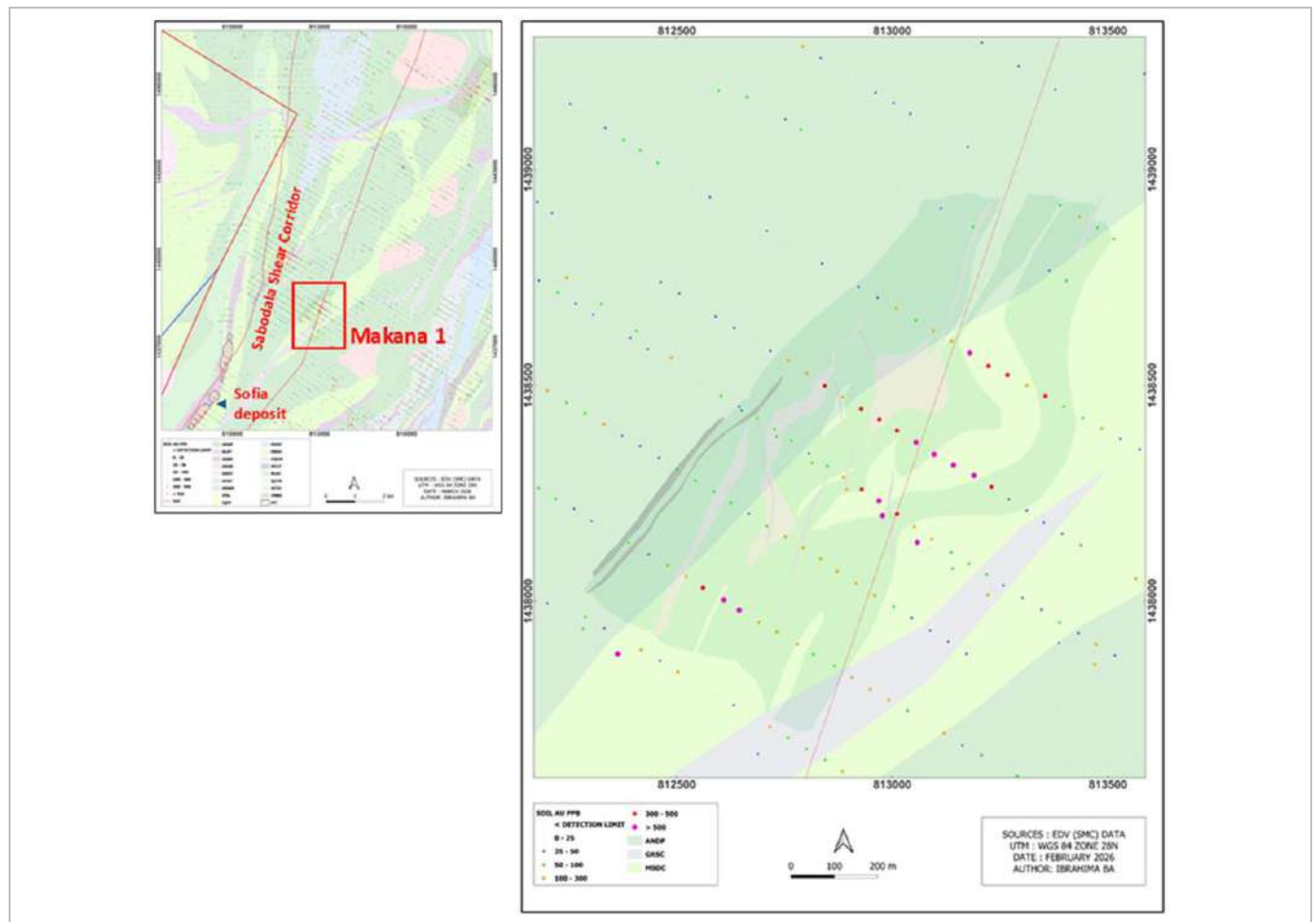
Figure 9-2: Makana 1 Location and Historical Soil Sampling Results
