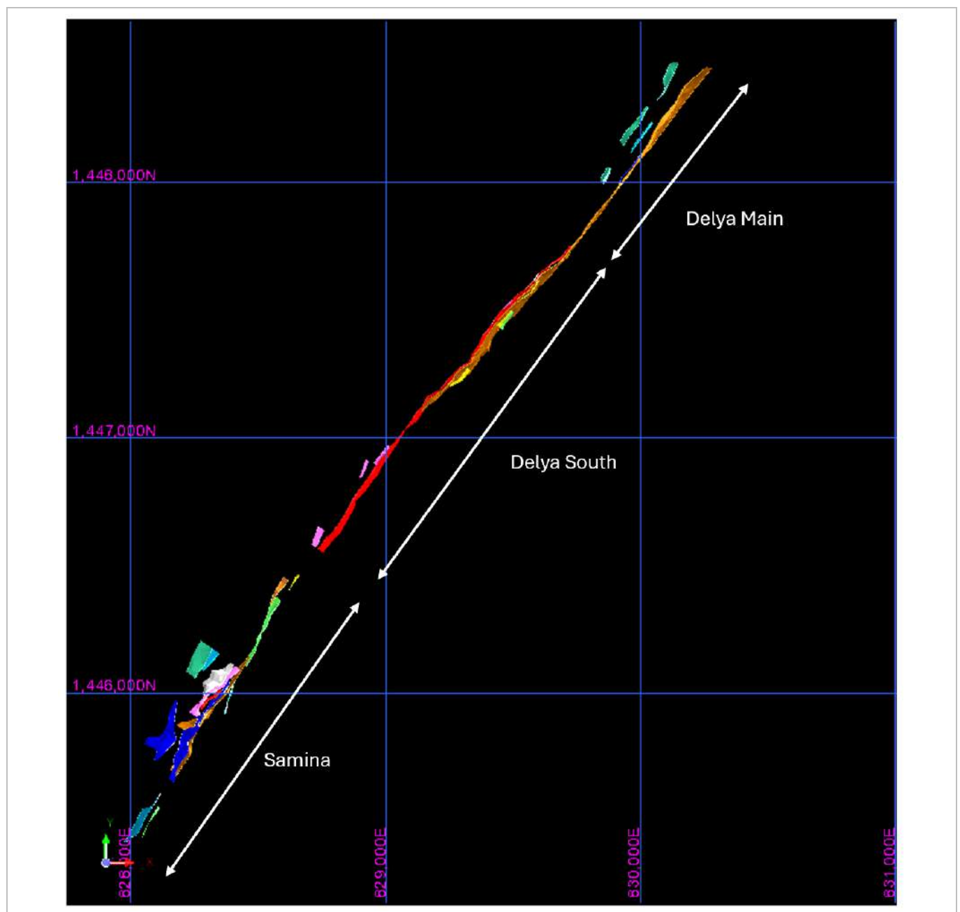
Figure 14-18: Delya-Samina Mineralisation, Plan View (EDV, 2025)
