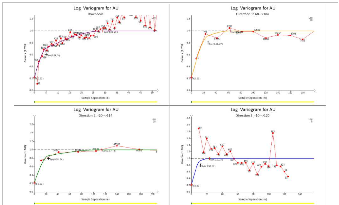
Figure 14-43: Masato Semi-Variograms (EDV, 2023)
