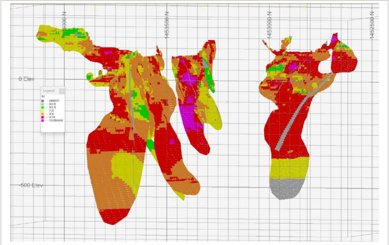
Figure 14-71: Golouma Grade Block Model (EDV 2025)
