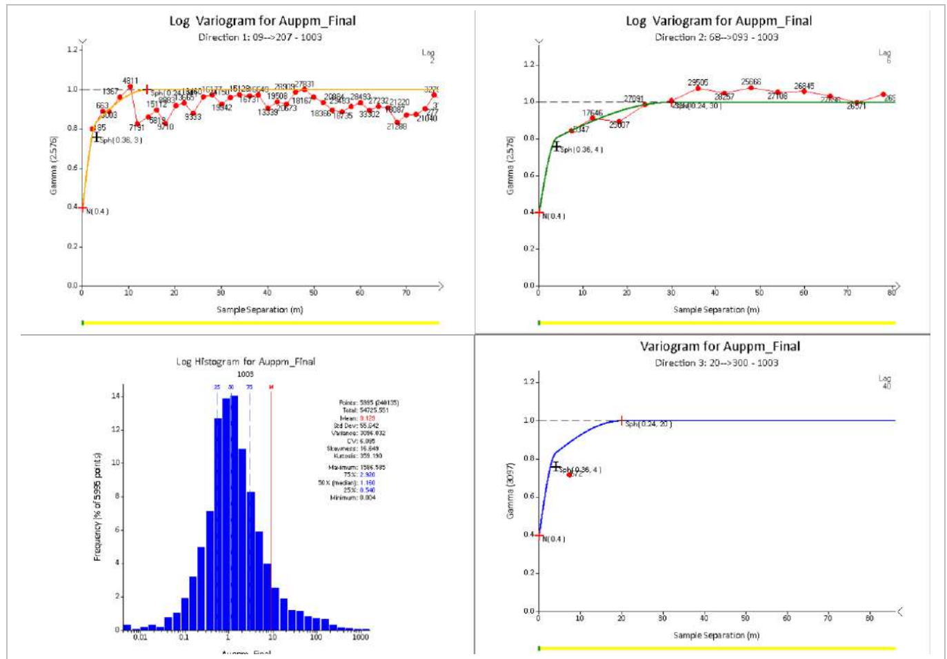
Figure 14-44: MCZ Semi-Variograms Example - Zone 1003 (EDV, 2023)
