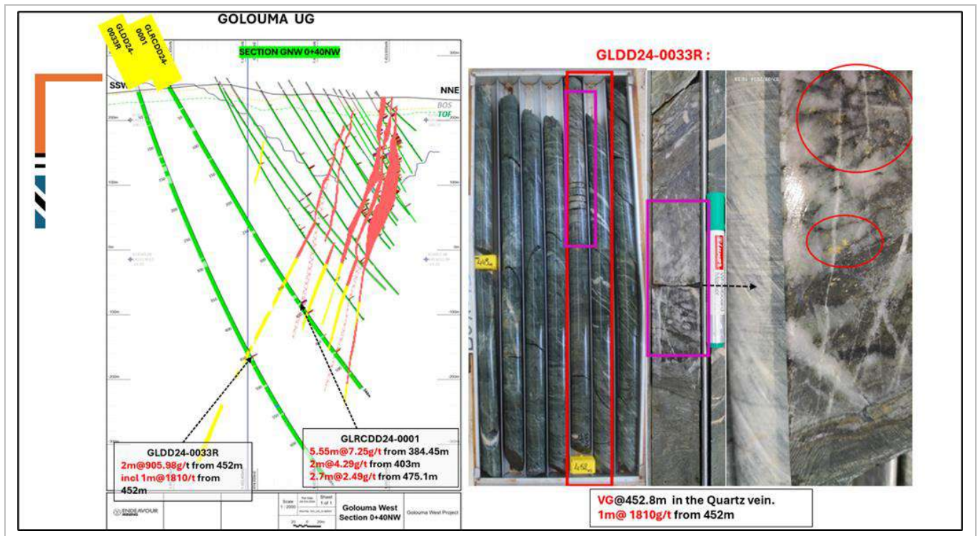
Figure 10-4: Golouma West Cross Section (0+40) Northwest and Drill Core Images
