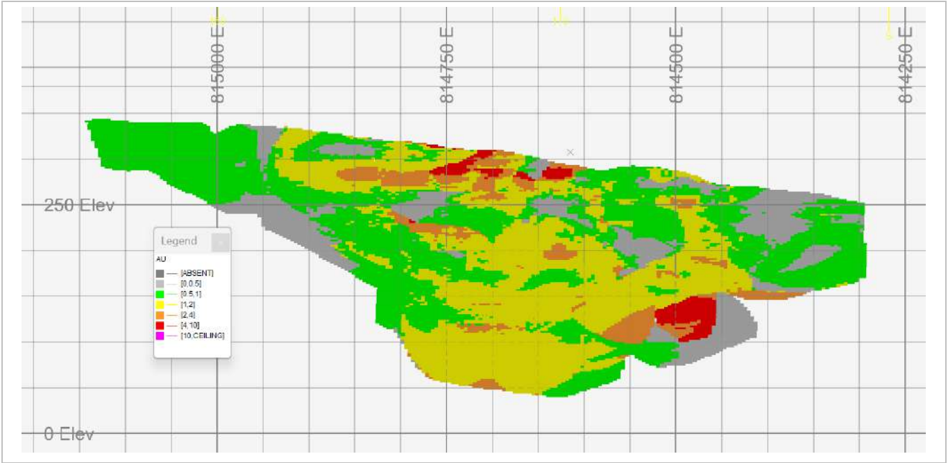
Figure 14-80: Mamasato Grade Block Model (EDV 2025)
