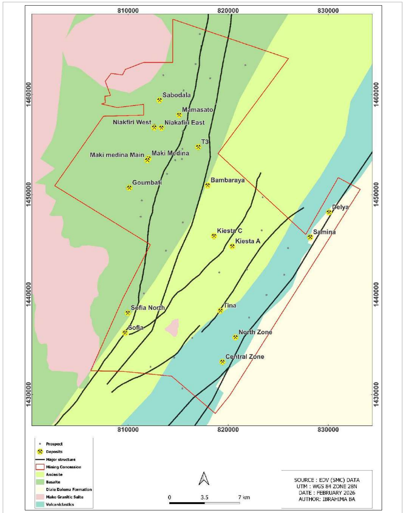
Figure 7-4: Sabodala Mining Concession Geology with Major Gold Deposits (EDV, 2025a)
