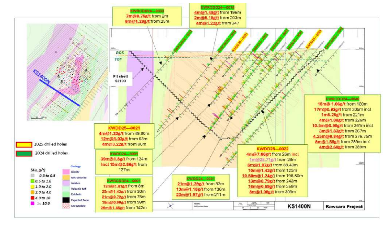
Figure 10-13: Kawsara Cross-Section KS1400N with Geology and Assay Results
