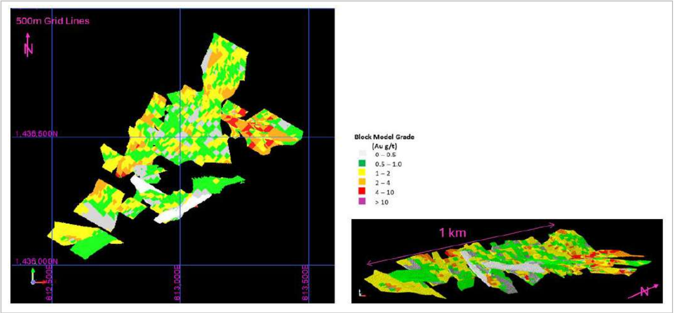
Figure 14-78: Makana 1 Grade Block Model Plan and Oblique View (EDV 2025)
