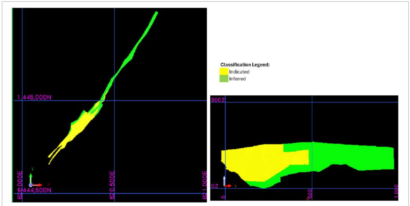
Figure 14-58: Kiesta A Mineral Resource Classification Plan View & S-N Long Section Looking W (EDV 2025)
