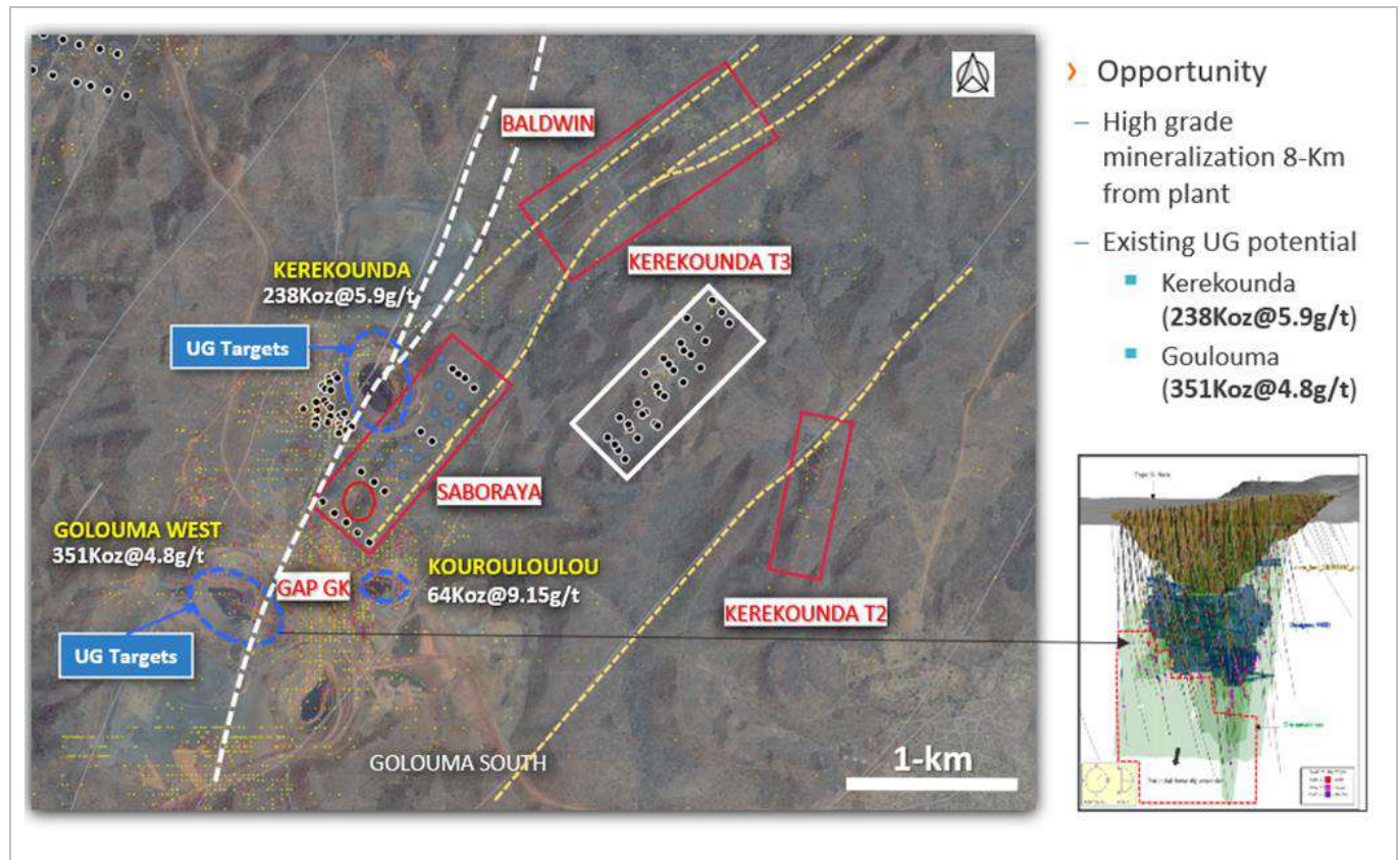
Figure 10-2: Kerekounda and Golouma Area with 2024-25 DH Collars and Exploration Targets
