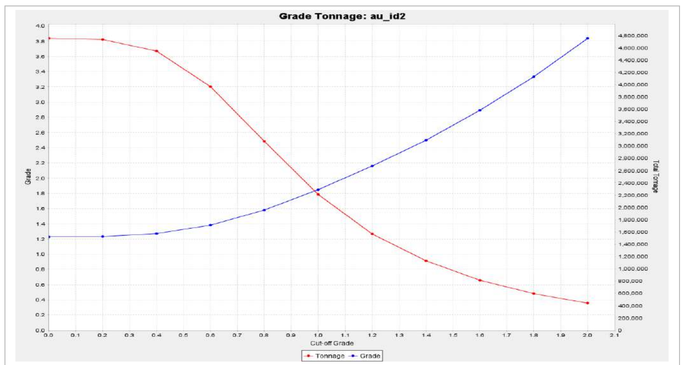
Figure 14-103: Niakafiri West Grade-Tonnage Curve Within USD 2100 Pit Shell (Un-depleted) (EDV 2025)
