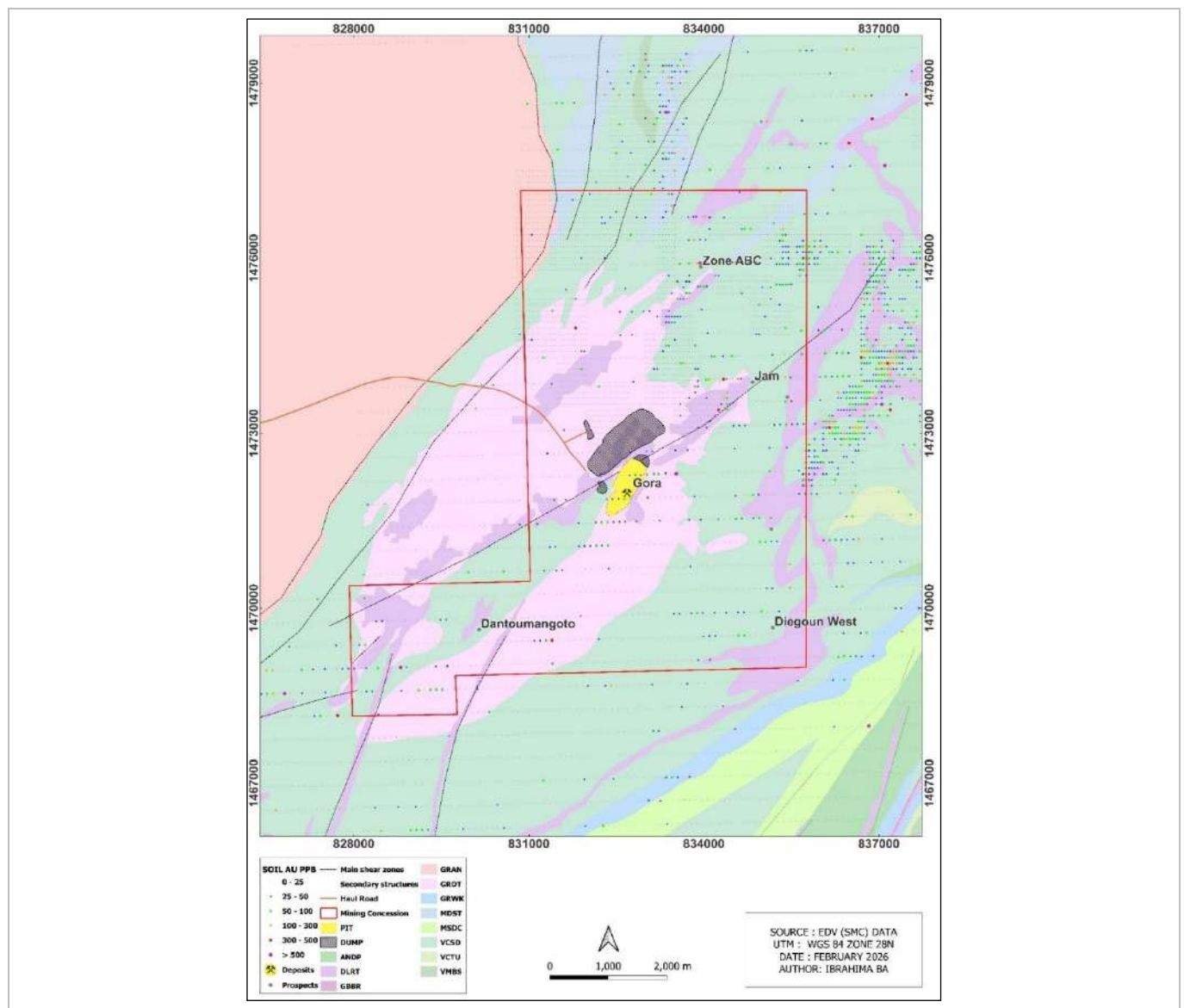
Figure 7-5: Sabodala Lot B ( Gora) Geology, Deposits and Prospects (EDV, 2025a)
