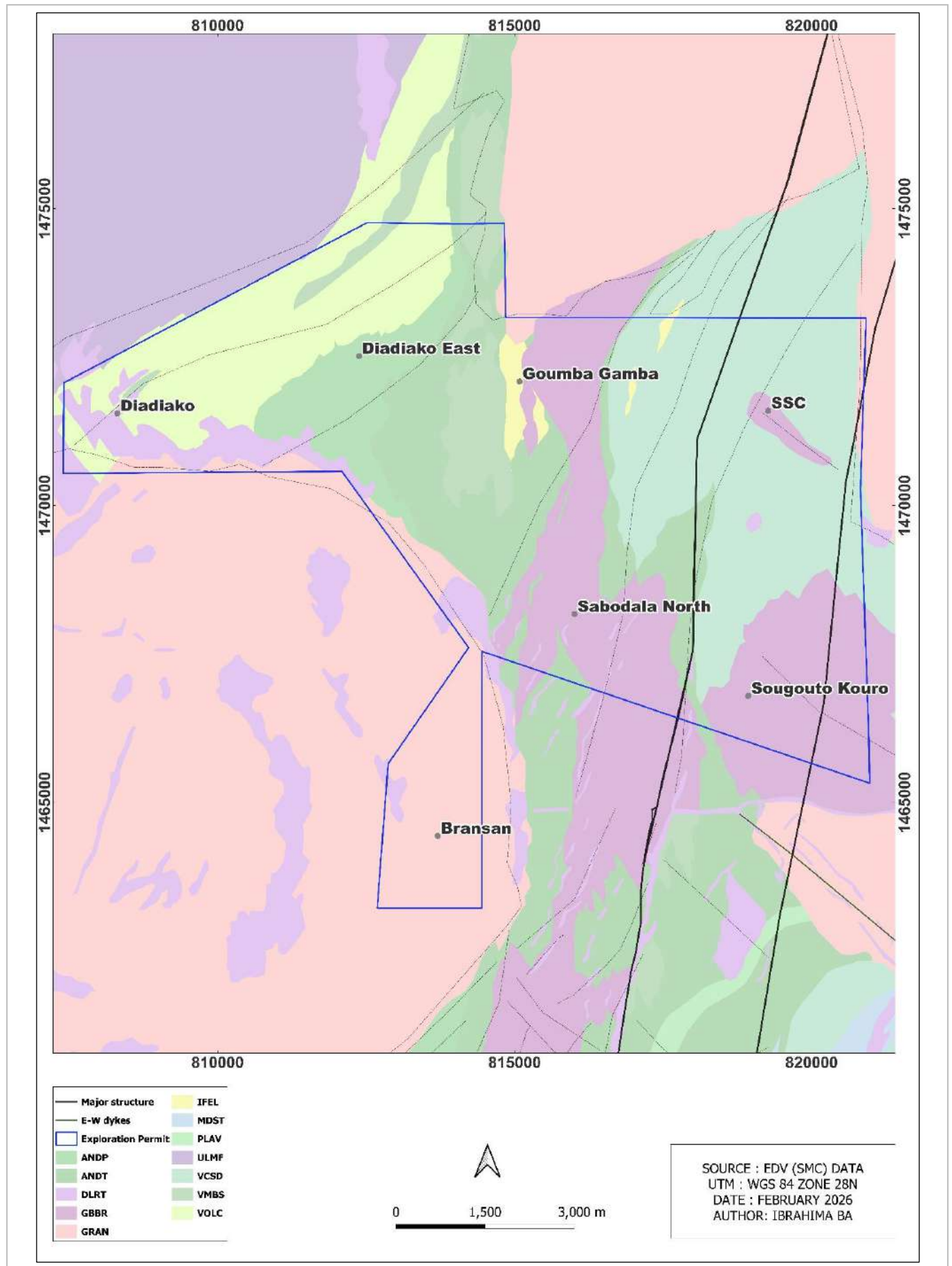
Figure 7-7: Bransan Lot A Geology and Prospects (EDV, 2025a)
