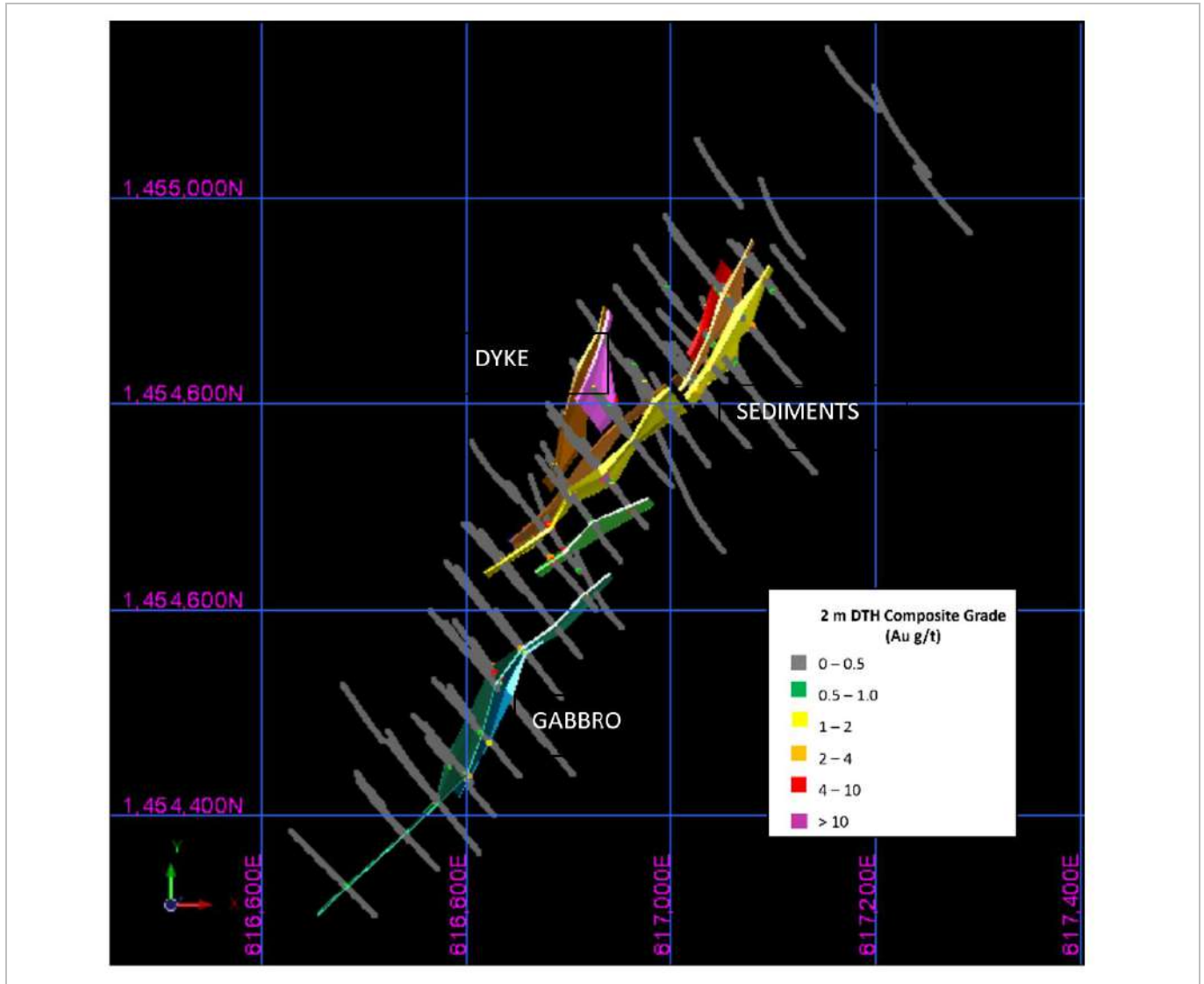
Figure 14-23: Kerekounda East Mineralisation, Plan View (EDV, 2025)
