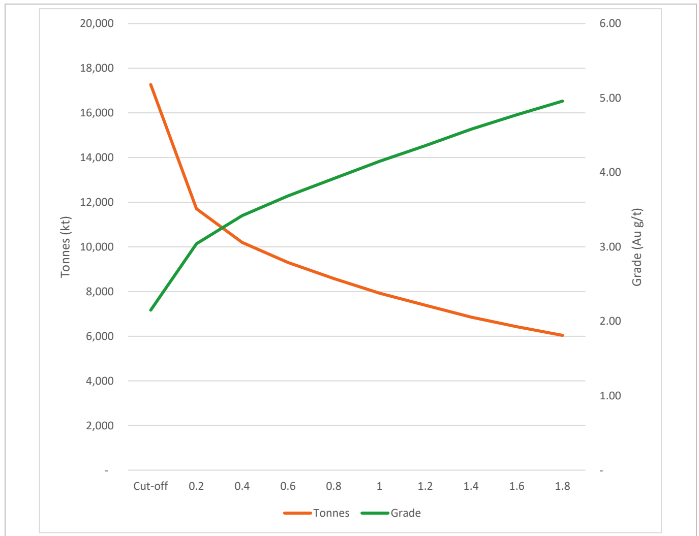
Figure 14-101: MNZ Grade-Tonnage Curve Within USD 2100/oz Whittle Pit (EDV 2025)
