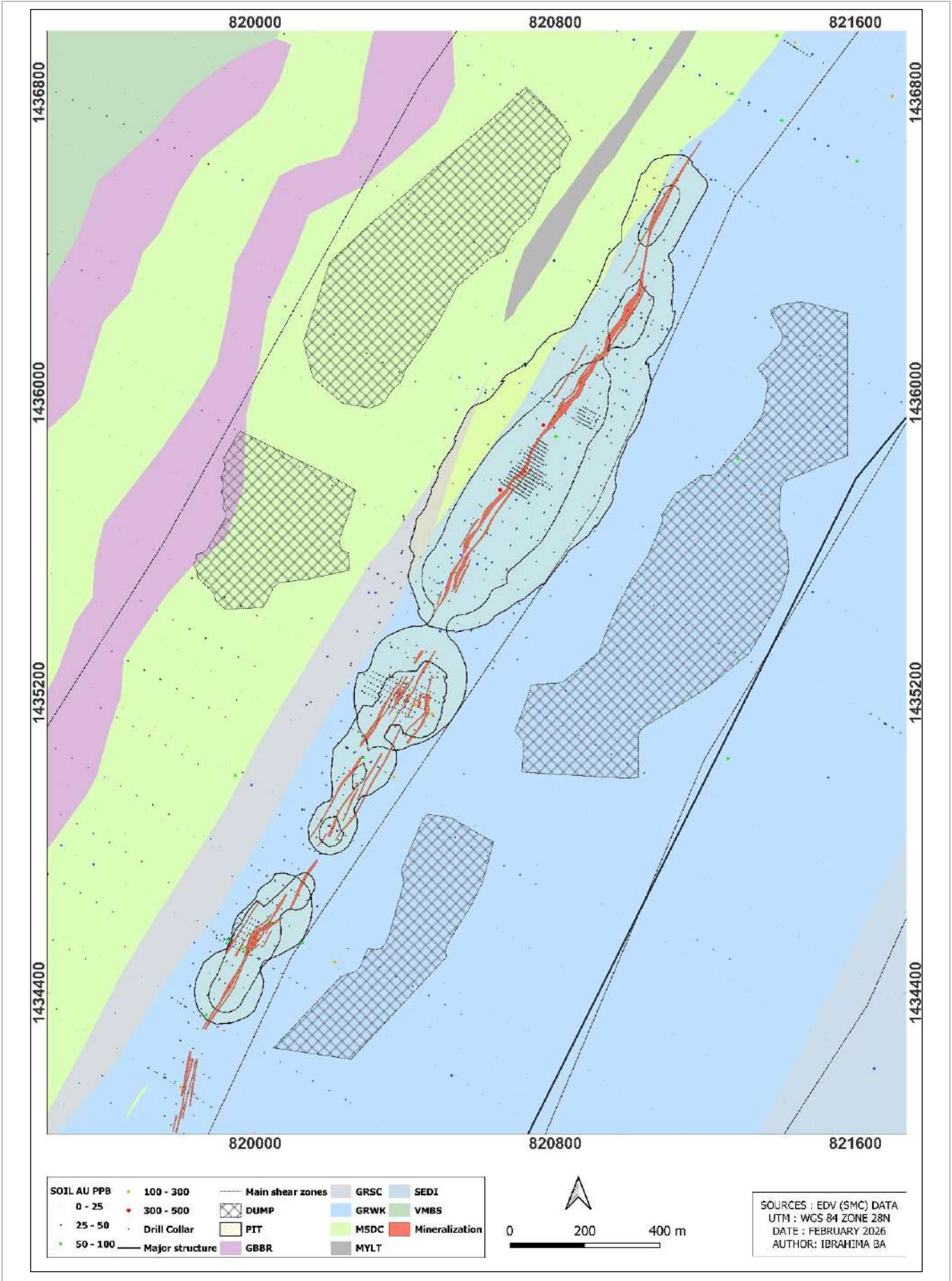
Figure 7-16: MNZ Geological Map Showing Mineralised Zones (EDV, 2025a)
