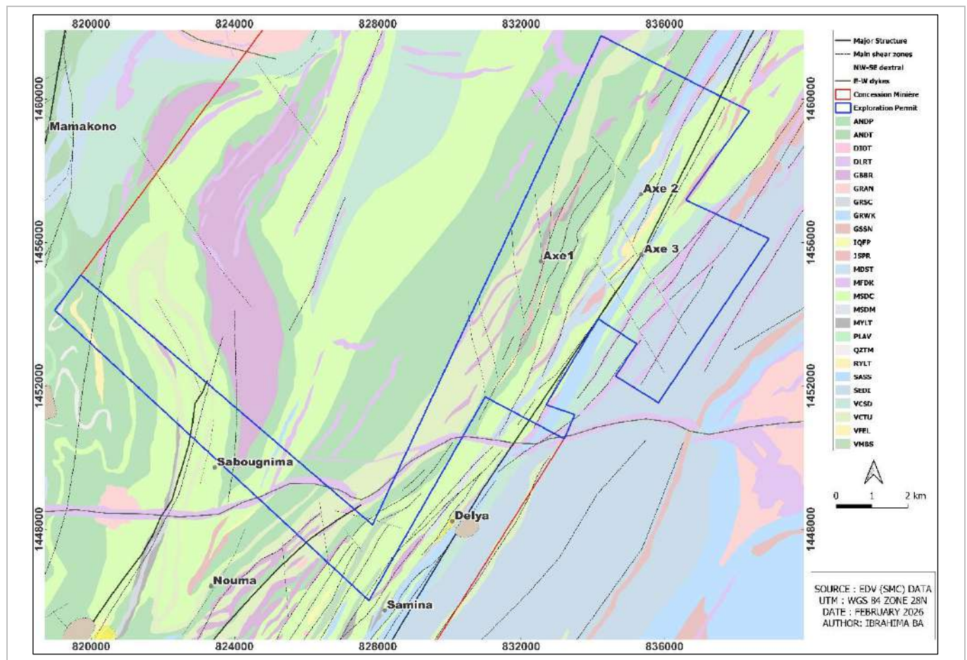
Figure 7-10: Niamaya Geology and Prospects (EDV, 2025a)
