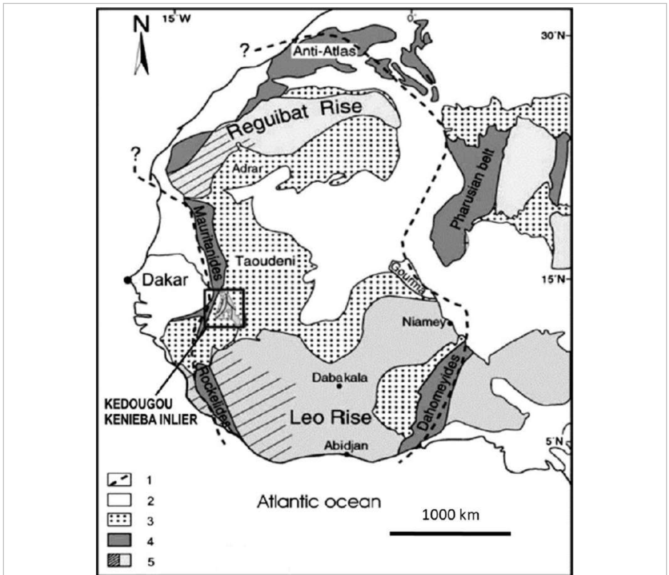
Figure 7-1: Location of the Kédougou-Kenieba-Inlier in the West African Craton (Gueye, 2008)
