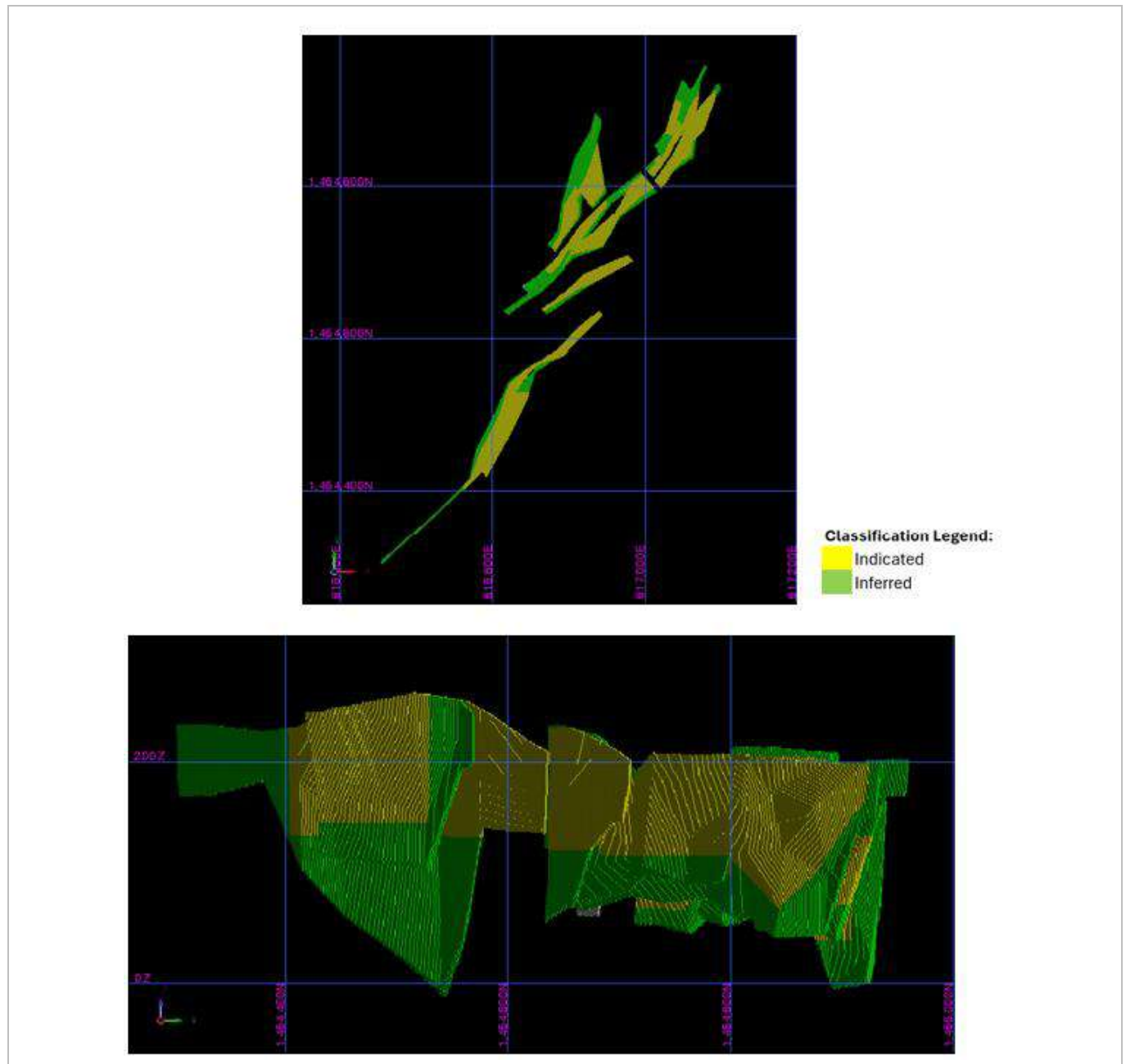
Figure 14-57: Kerekounda East Mineral Resource Classification Plan & N-S Long Sections (EDV 2025)
