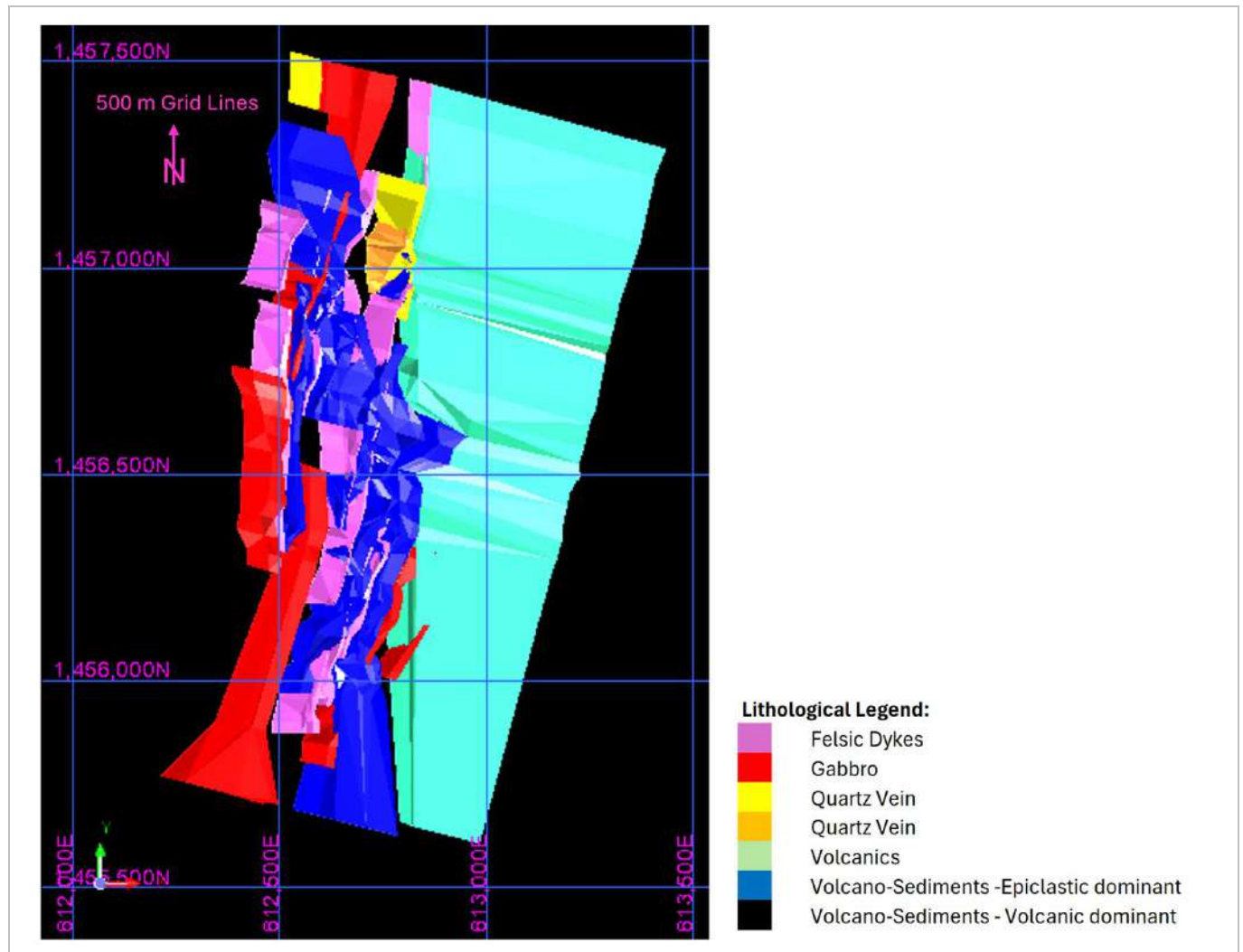
Figure 14-15: Niakafiri West Lithological Model, Plan View (EDV, 2025)
