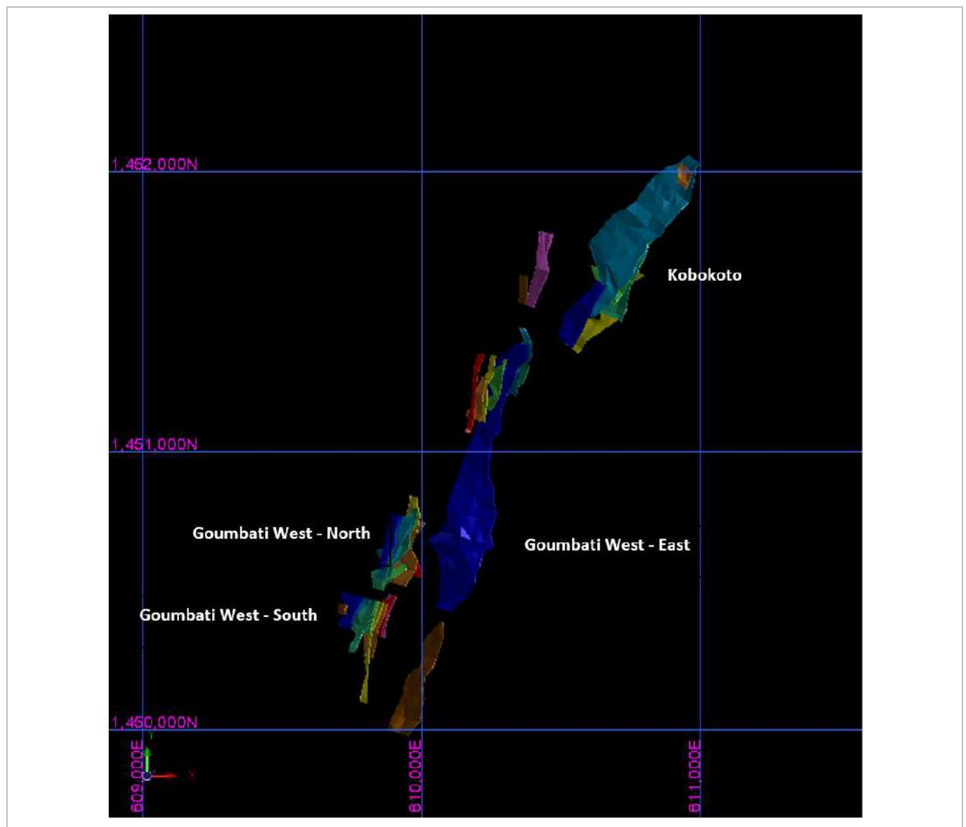
Figure 14-20: Goumbati West - Kobokoto Mineralisation, Plan View (EDV, 2025)
