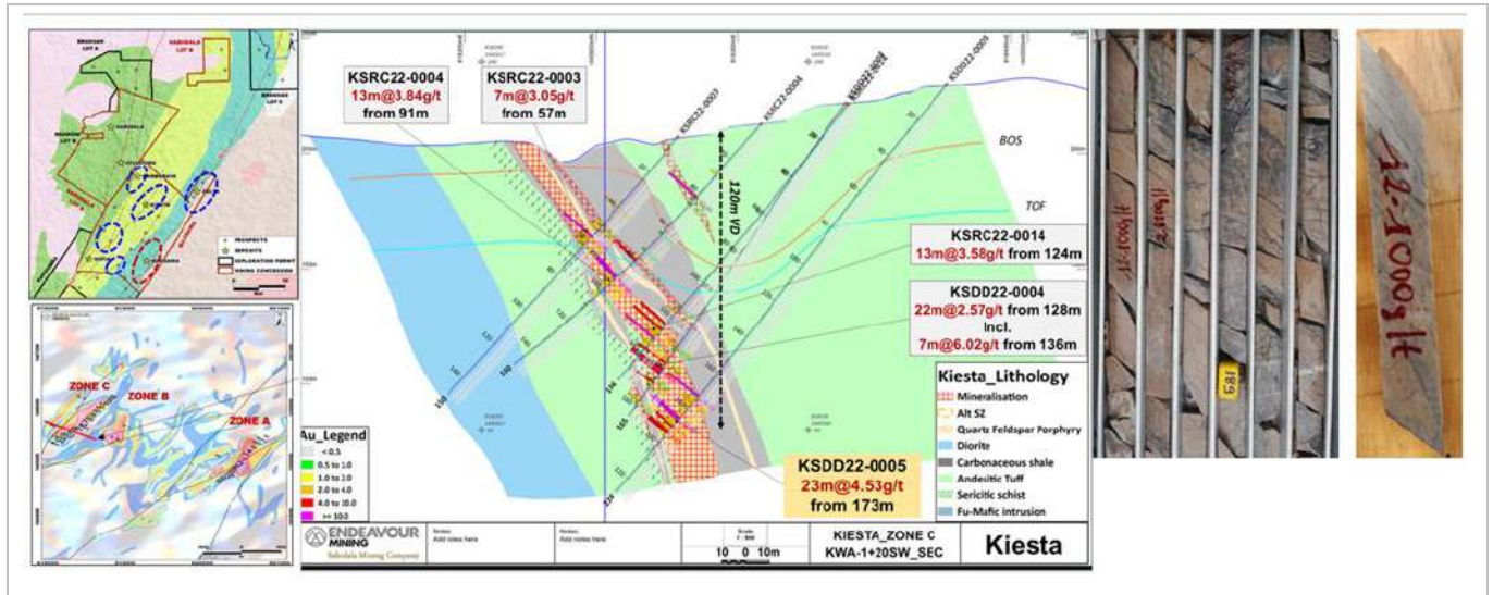
Figure 10-8: Kiesta C Cross-Section Example
