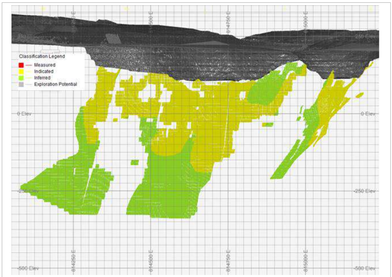
Figure 14-53: Longitudinal Section of Golouma Classification MSO Constrained (EDV 2025)
