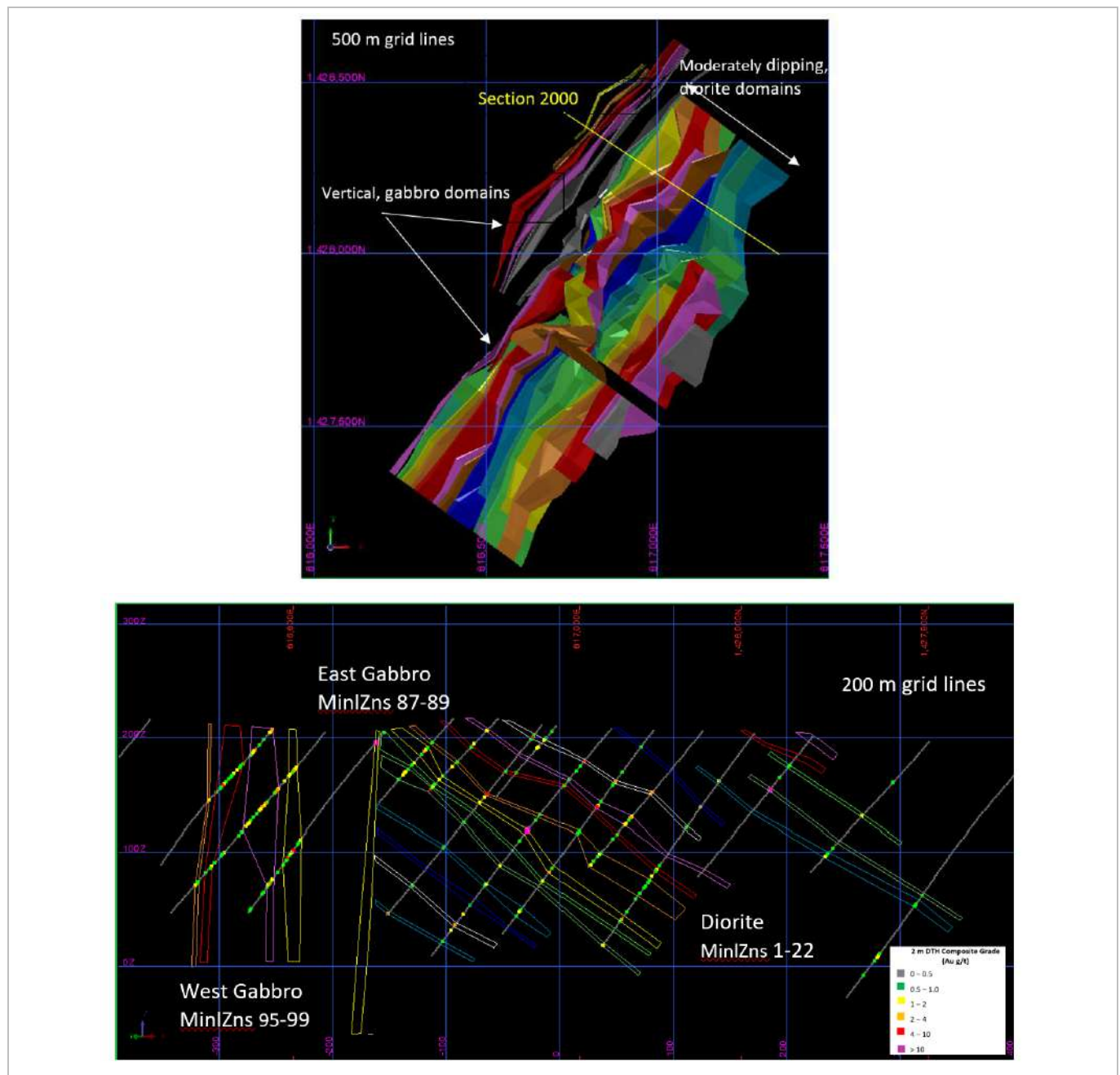
Figure 14-21: Kawsara Mineralisation, Plan and Cross-Section View (EDV, 2025)
