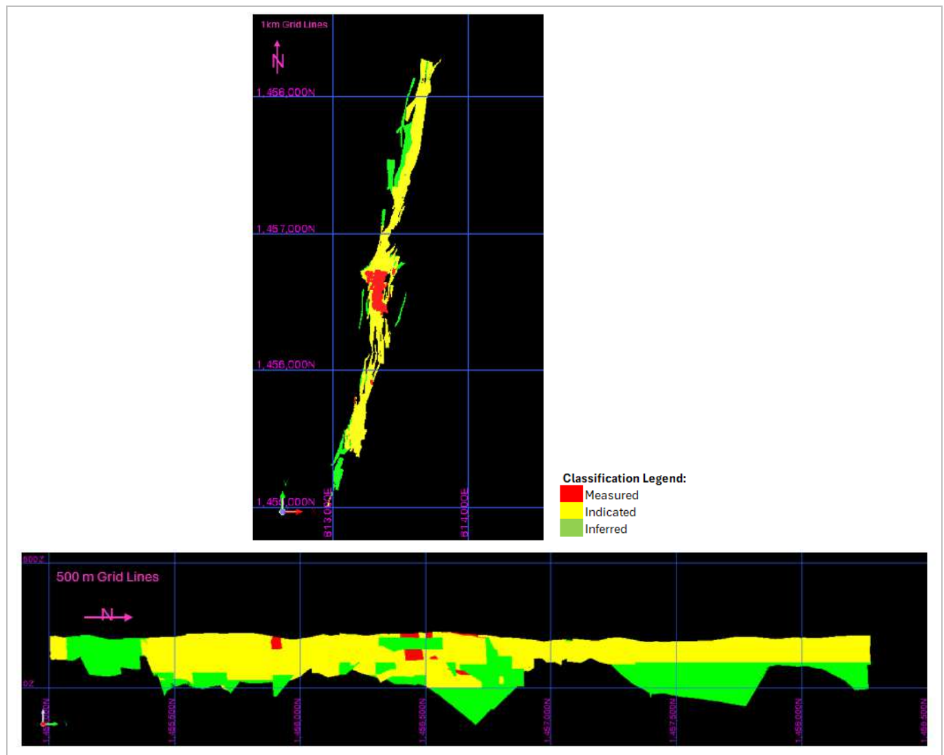
Figure 14-66: Niakafiri East Mineral Resource Classification Plan and N-S Long Section Views (EDV 2025)
