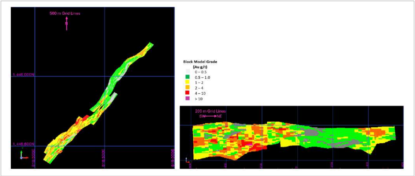
Figure 14-77: Kiesta C Grade Block Model Plan and SW-NE Long Section Views (EDV 2025)
