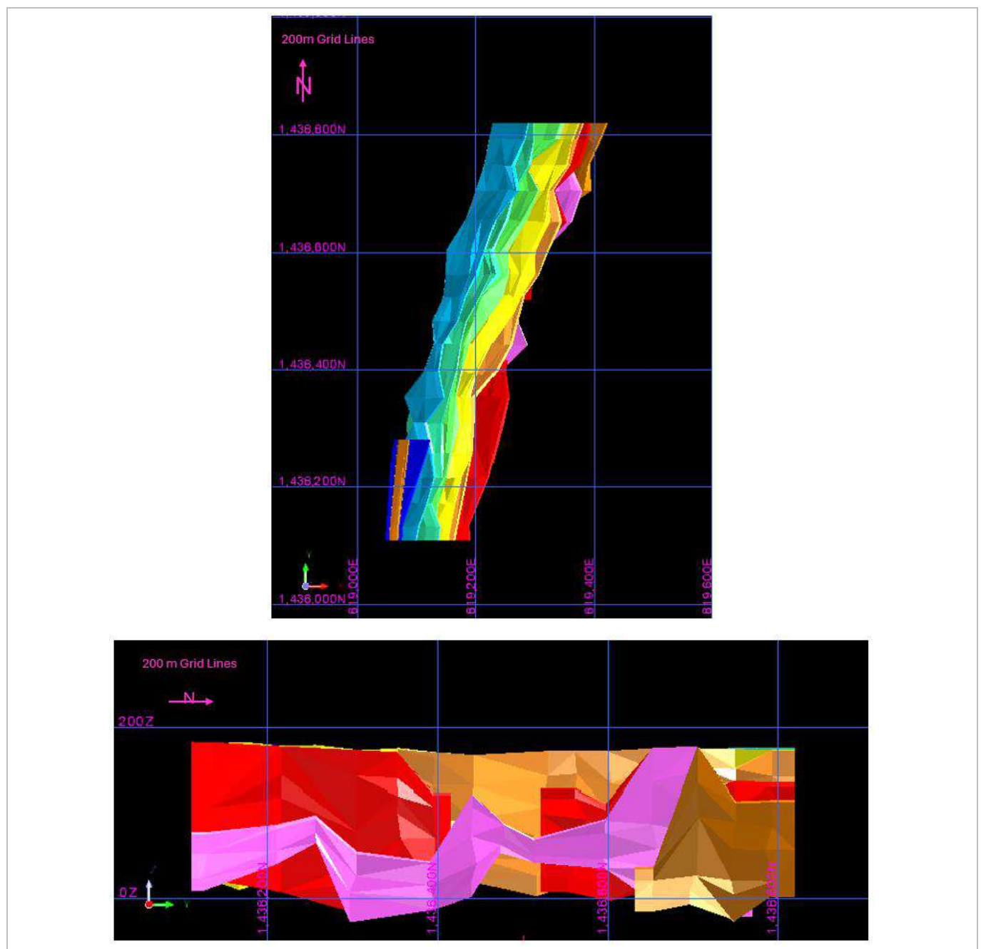
Figure 14-34: Tina Mineralisation Zones, Plan and N-S Long Section looking West Views (EDV, 2025)
