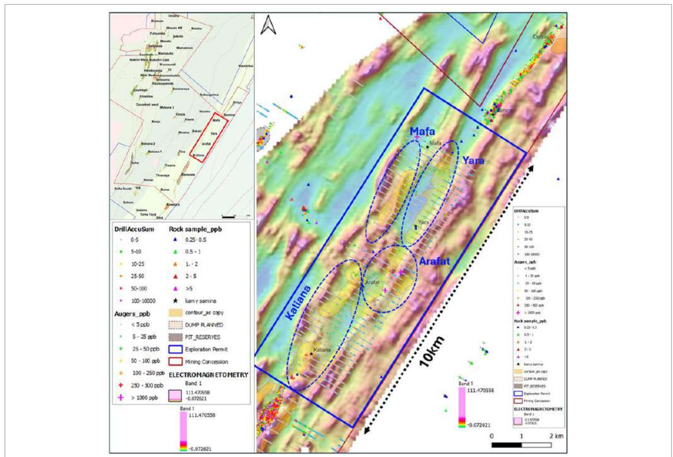
Figure 9-3: Kamy Corridor Target Locations Superimposed on EM Data
