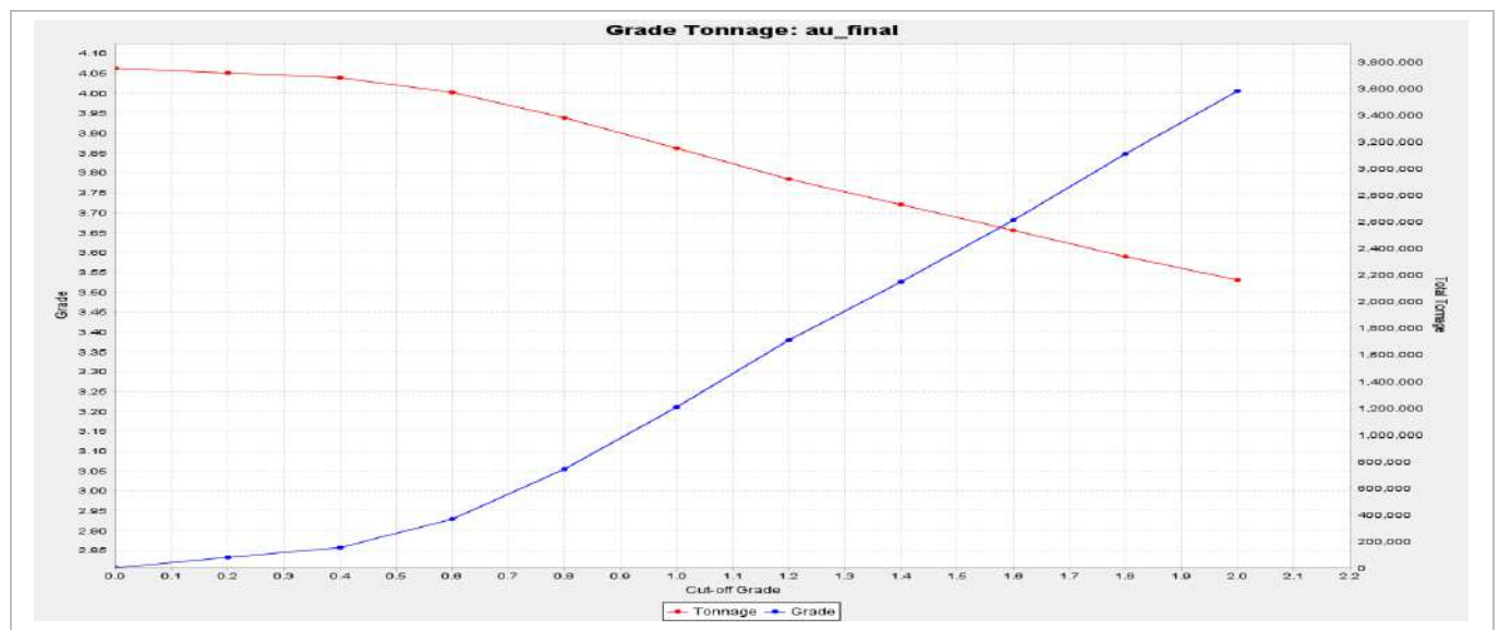
Figure 14-88: Delya-Samina Grade-Tonnage Curve Within USD 2100 Pit Shell (Un-depleted) (EDV 2025)
