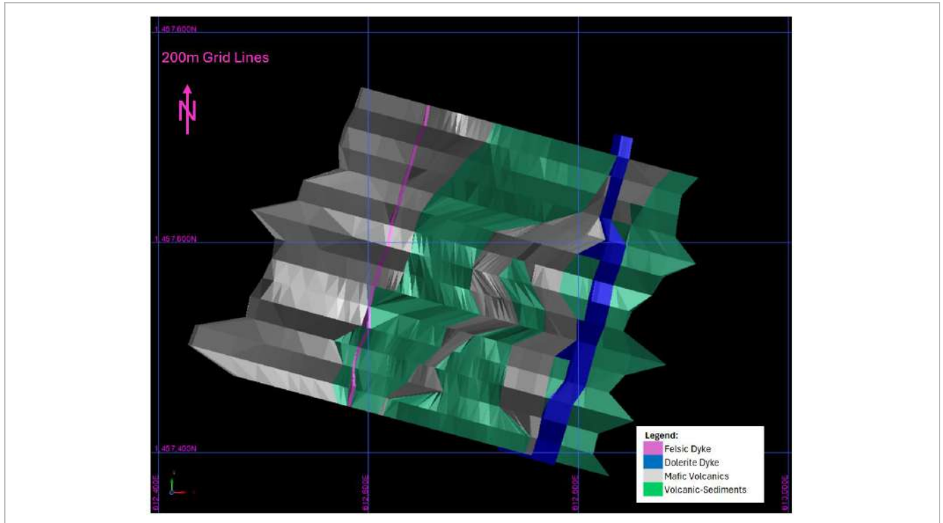
Figure 14-16: Soukhoto Lithological Model, Plan View (EDV, 2025)
