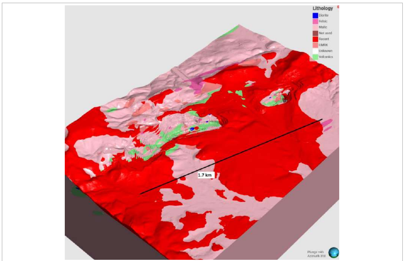
Figure 14-11: Masato Isometric Lithological Model Looking Northwest (EDV, 2022)
