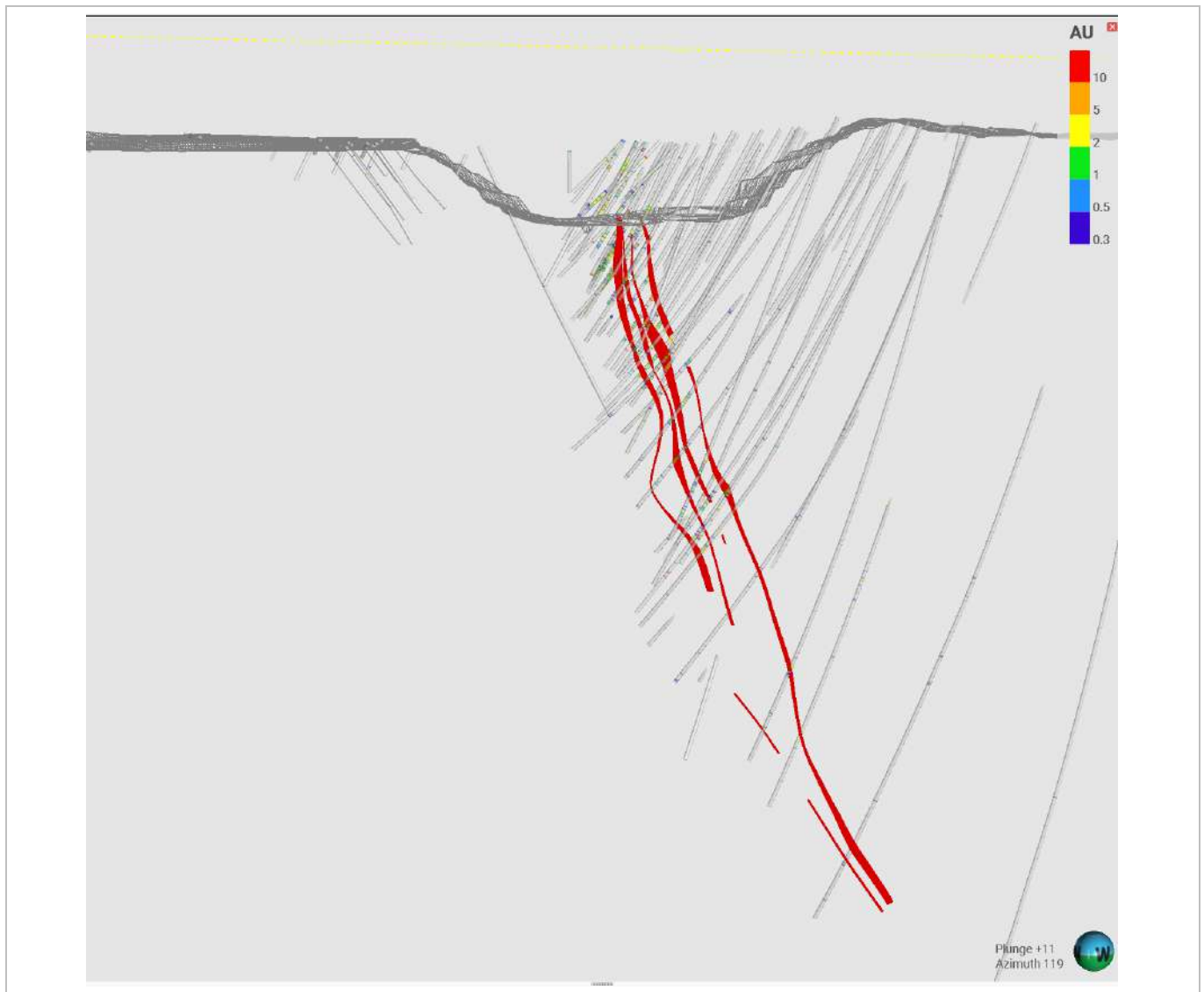
Figure 14-19: Golouma Mineralisation Cross Section (EDV, 2025)
