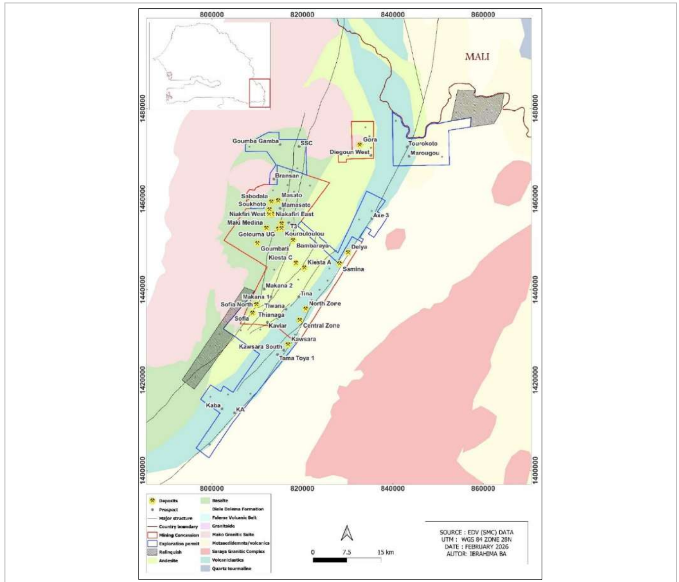
Figure 7-3: Site Permits, Geology, Deposits and Prospects (EDV, 2025a)
