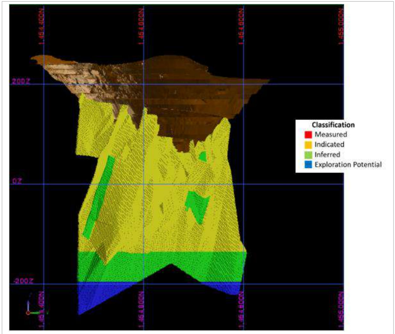
Figure 14-56: Kerekounda Classification Longitudinal Section View (EDV 2025)
