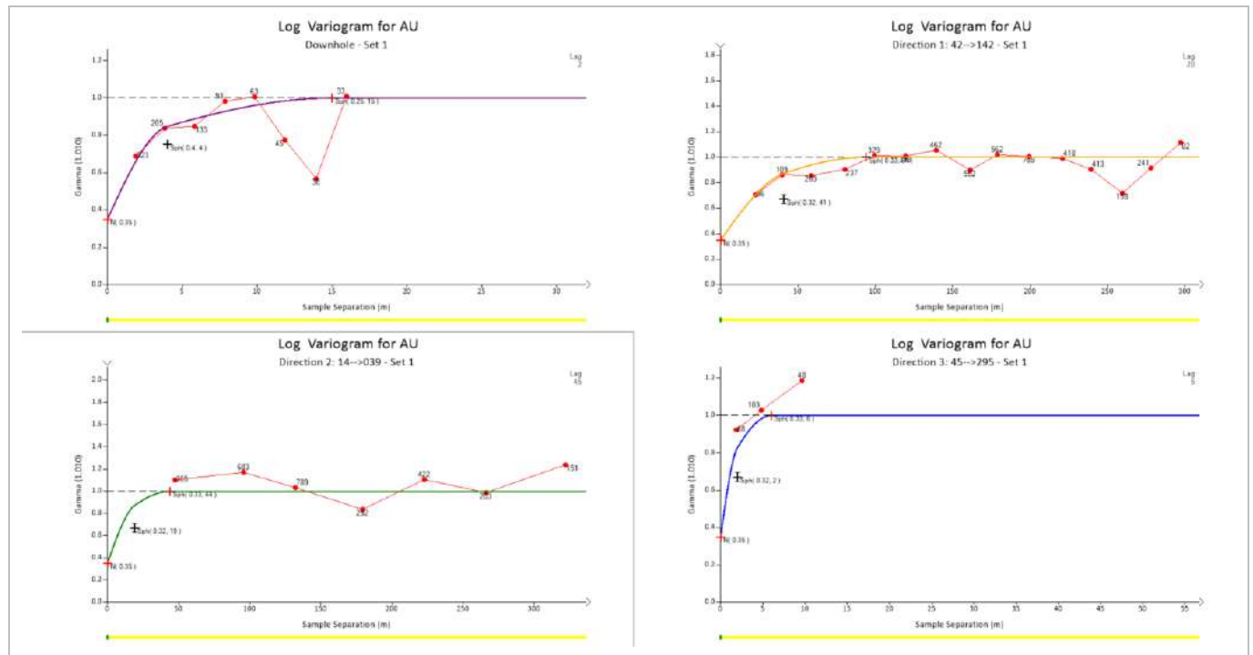
Figure 14-38: Golouma Set 1 Variogram (EDV, 2025)
