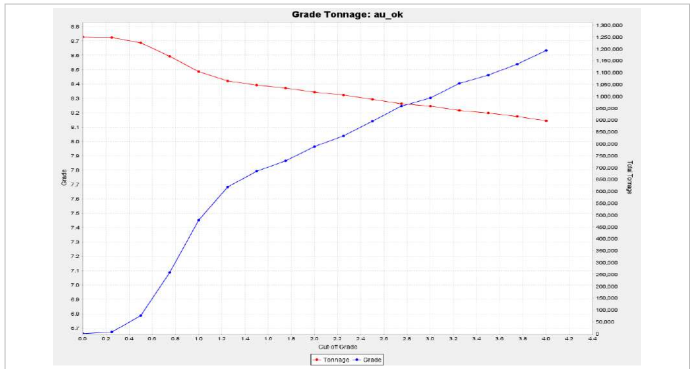
Figure 14-92: Kerekounda Underground Grade-Tonnage Curve (EDV 2025)
