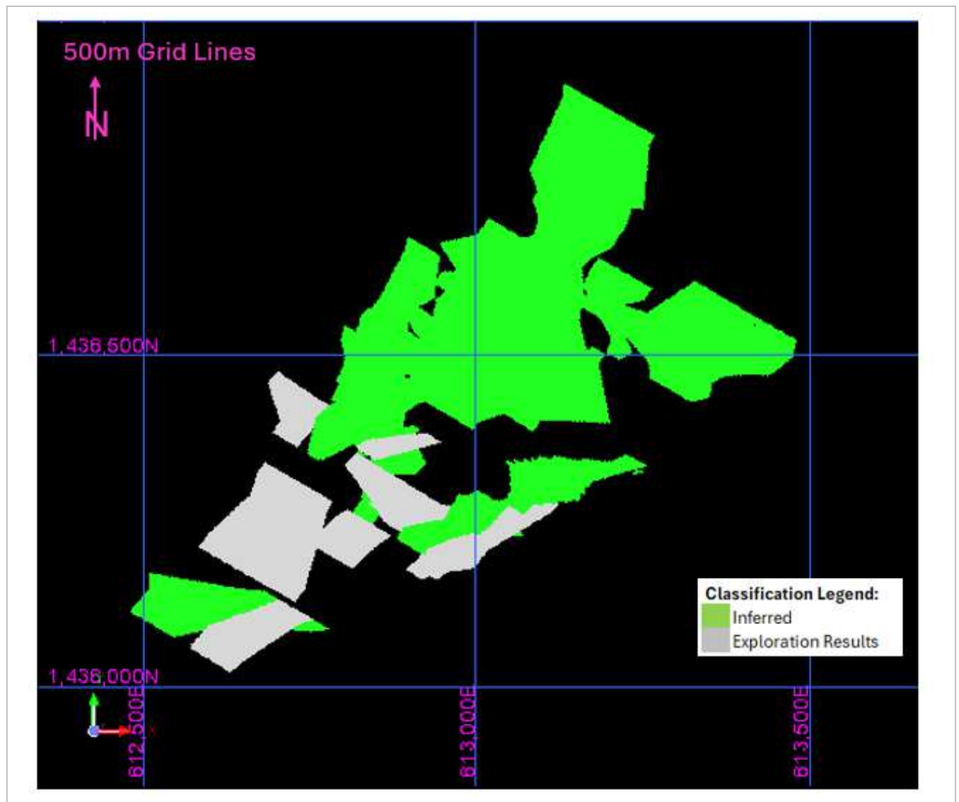
Figure 14-60: Makana 1 Mineral Resource Classification (EDV 2025)
