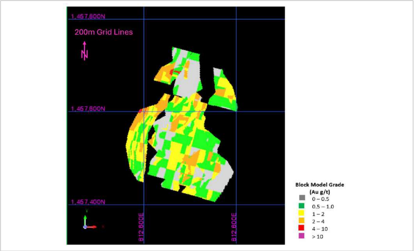
Figure 14-86: Soukhoto Grade Block Model Plan View (EDV 2025)
