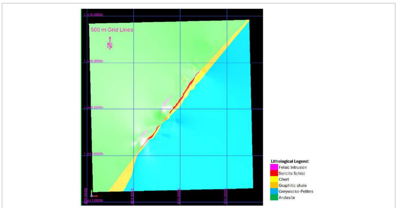
Figure 14-3: Delya Lithological Model Cross Section (Endeavour, 2025)
