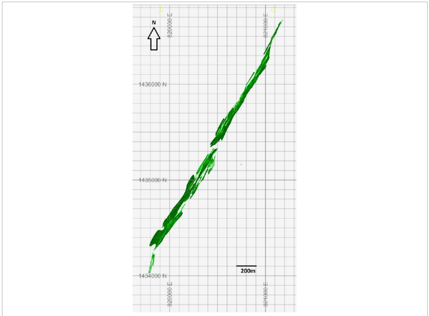
Figure 14-30: MNZ Mineralisation Plan View (EDV, 2025)
