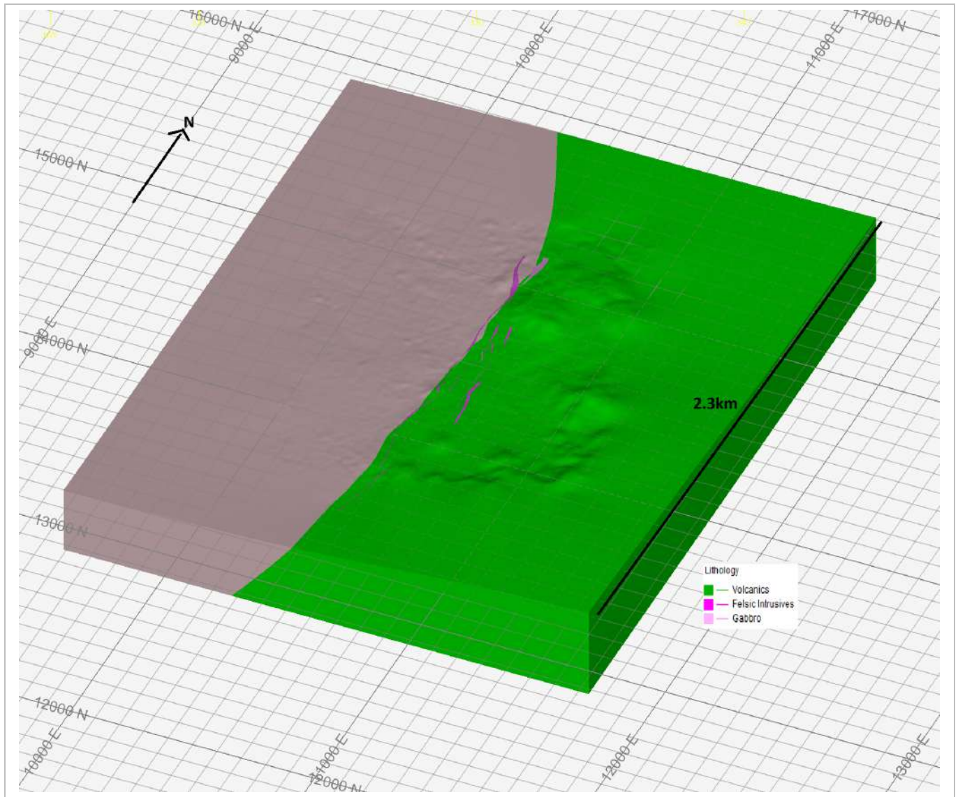
Figure 14-9: Maki Medina Lithological Model Oblique View (EDV, 2025)
