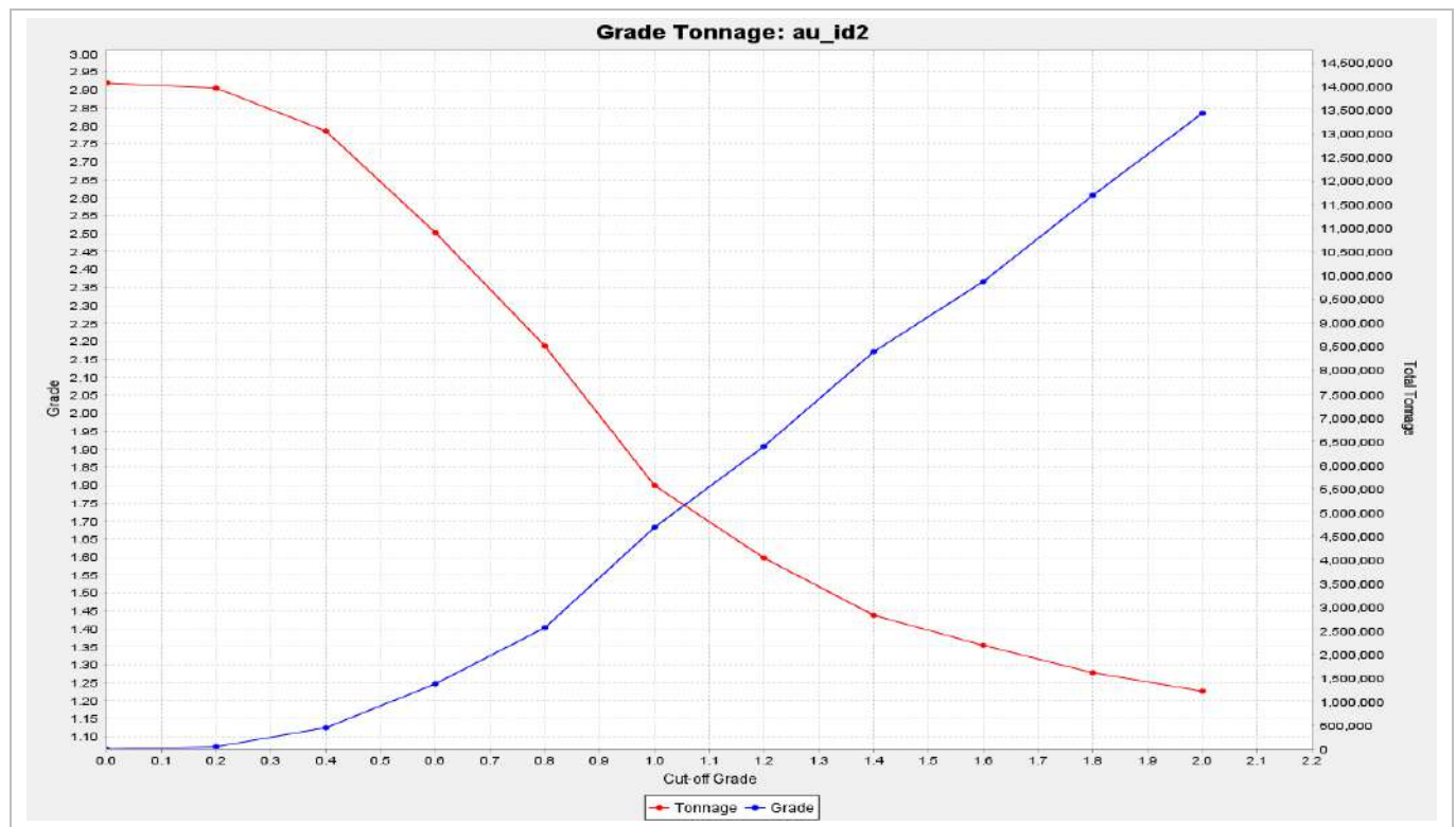
Figure 14-91: Kawsara Grade-Tonnage Curve Within USD 2100 Pit Shell (EDV 2025)
