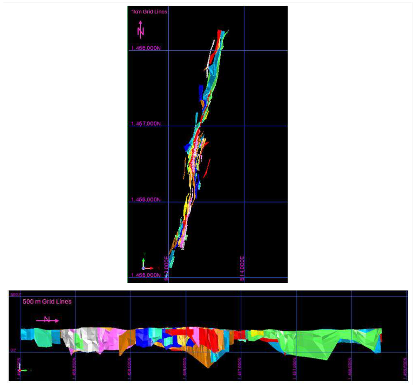
Figure 14-31: Niakafiri East Mineralisation Zones, Plan and N-S Section Looking West Views (EDV, 2025)
