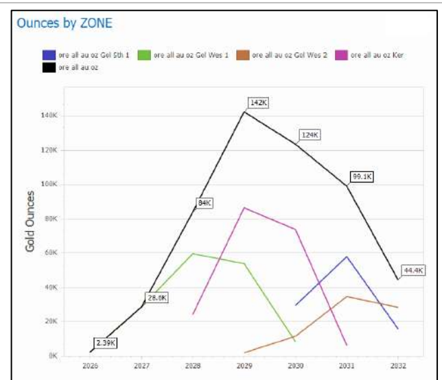
Figure 16-30: K&G Underground Gold Ounce Profile
