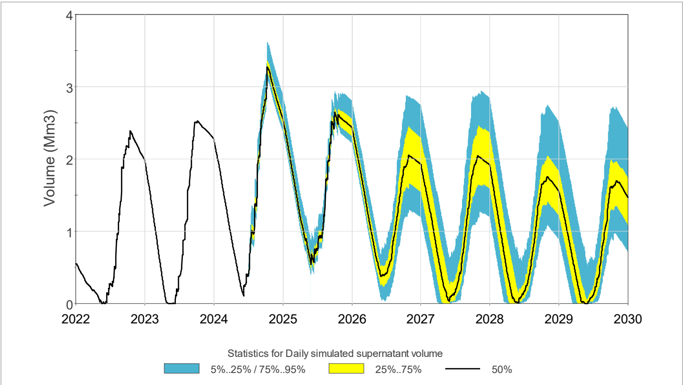
Figure 18-10: TSF 1 Probabilistic Simulation of Tailings Supernatant Pond Volume (100 Realisations)
