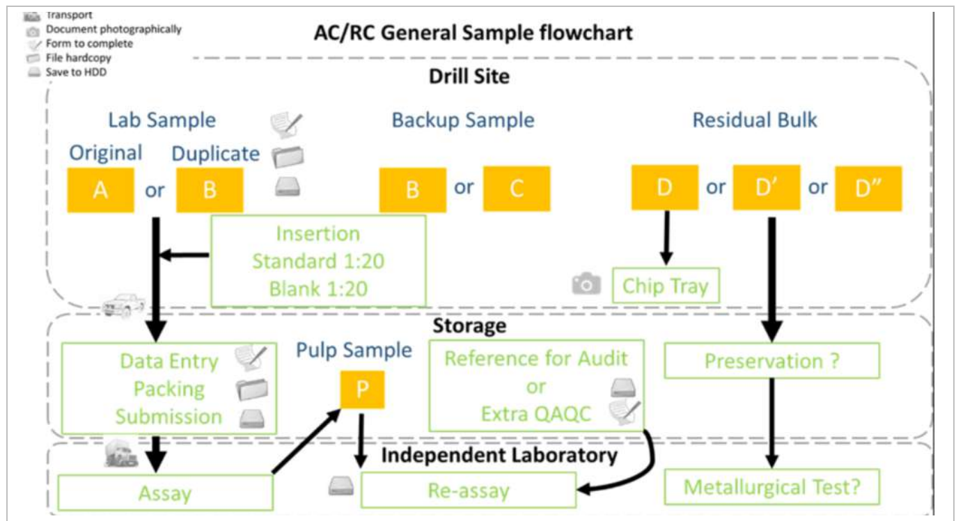
Figure 11-3: RC Sampling Flowchart
