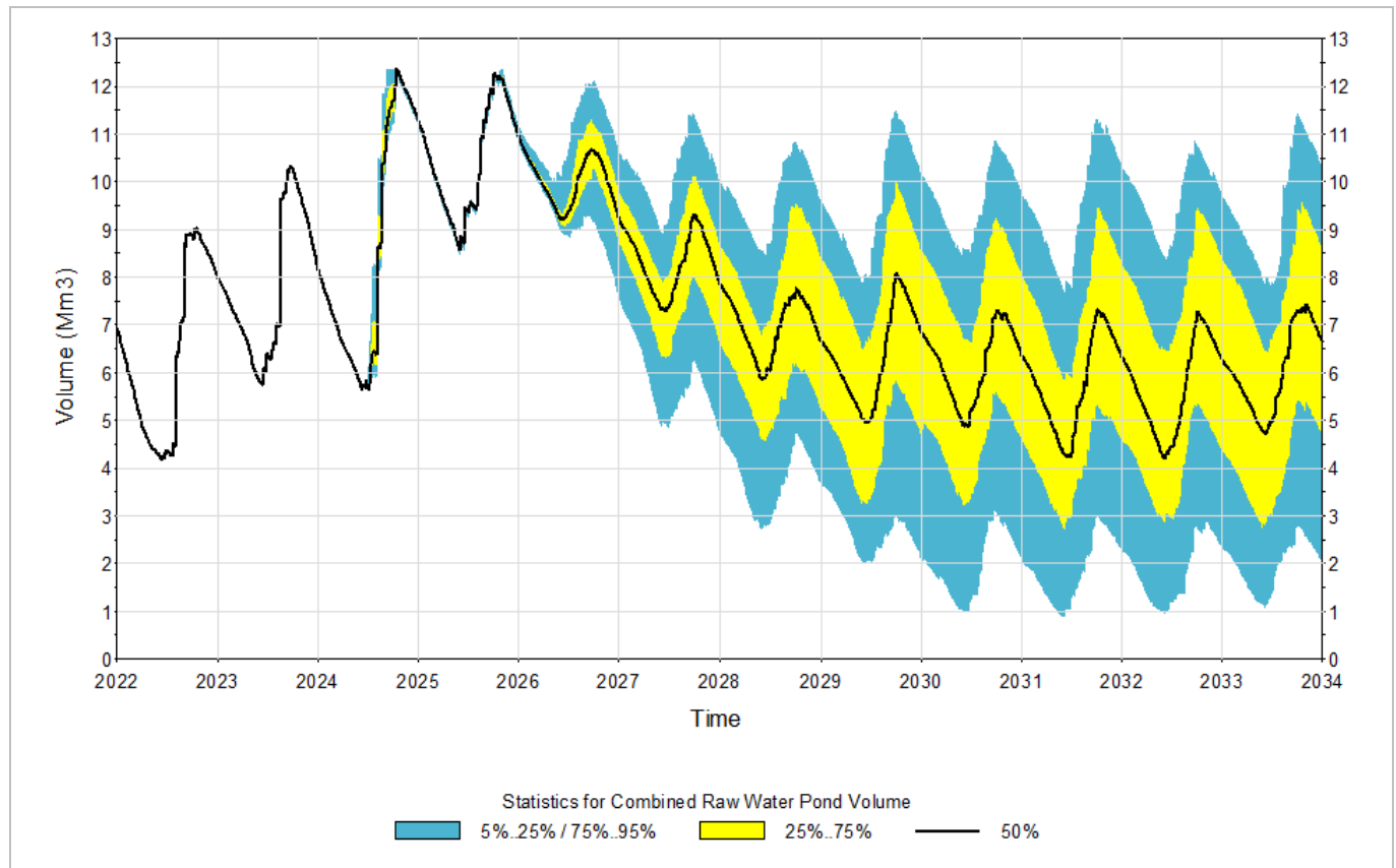
Figure 18-8: Projected Combined SRWD, LRWD and URWD/ERWD Raw water Storage Volume
