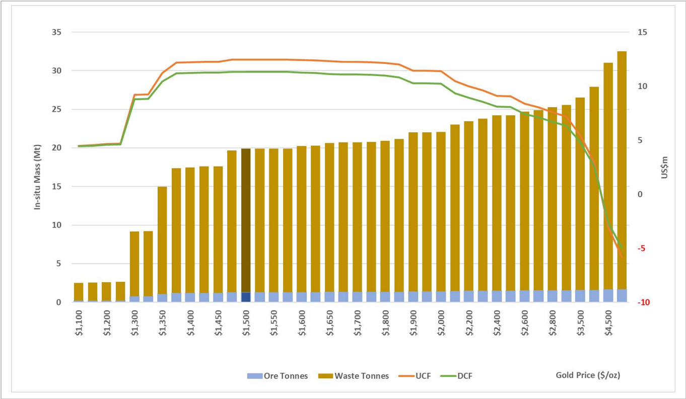
Figure 15-5: Kiesta Zone C (KIC) Optimisation Results
