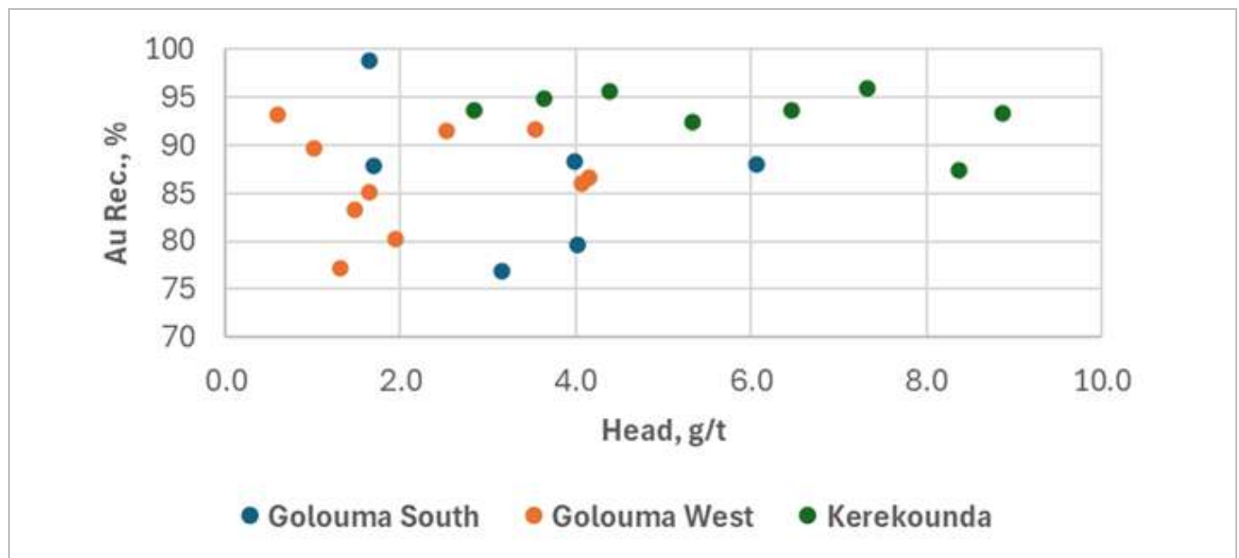
Figure 13-9: K&G UG Variability Gravity/Leach Recoveries
