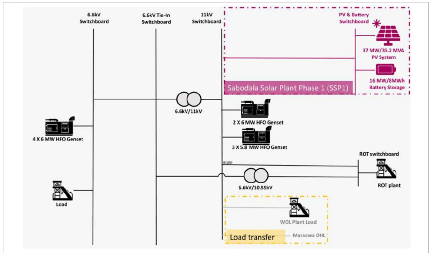
Figure 18-5 SPS Power Supply Configuration (QGE, 2025)
