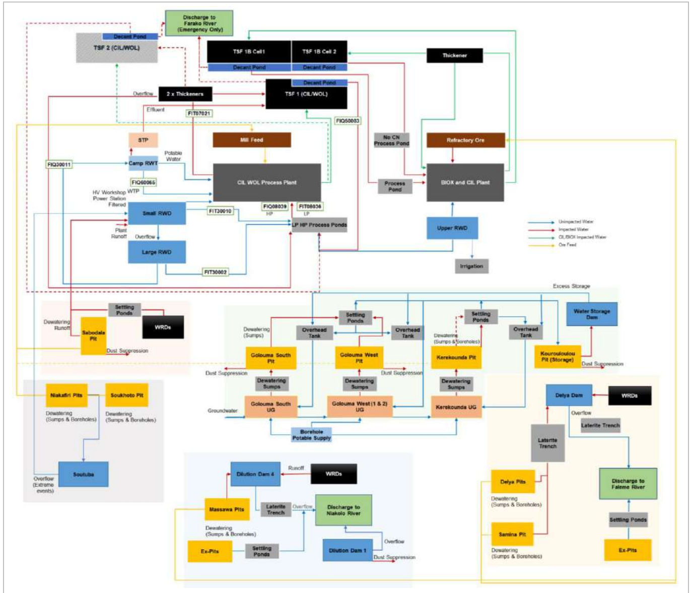
Figure 18-6: Mine Site-Wide Block Flow Diagram
