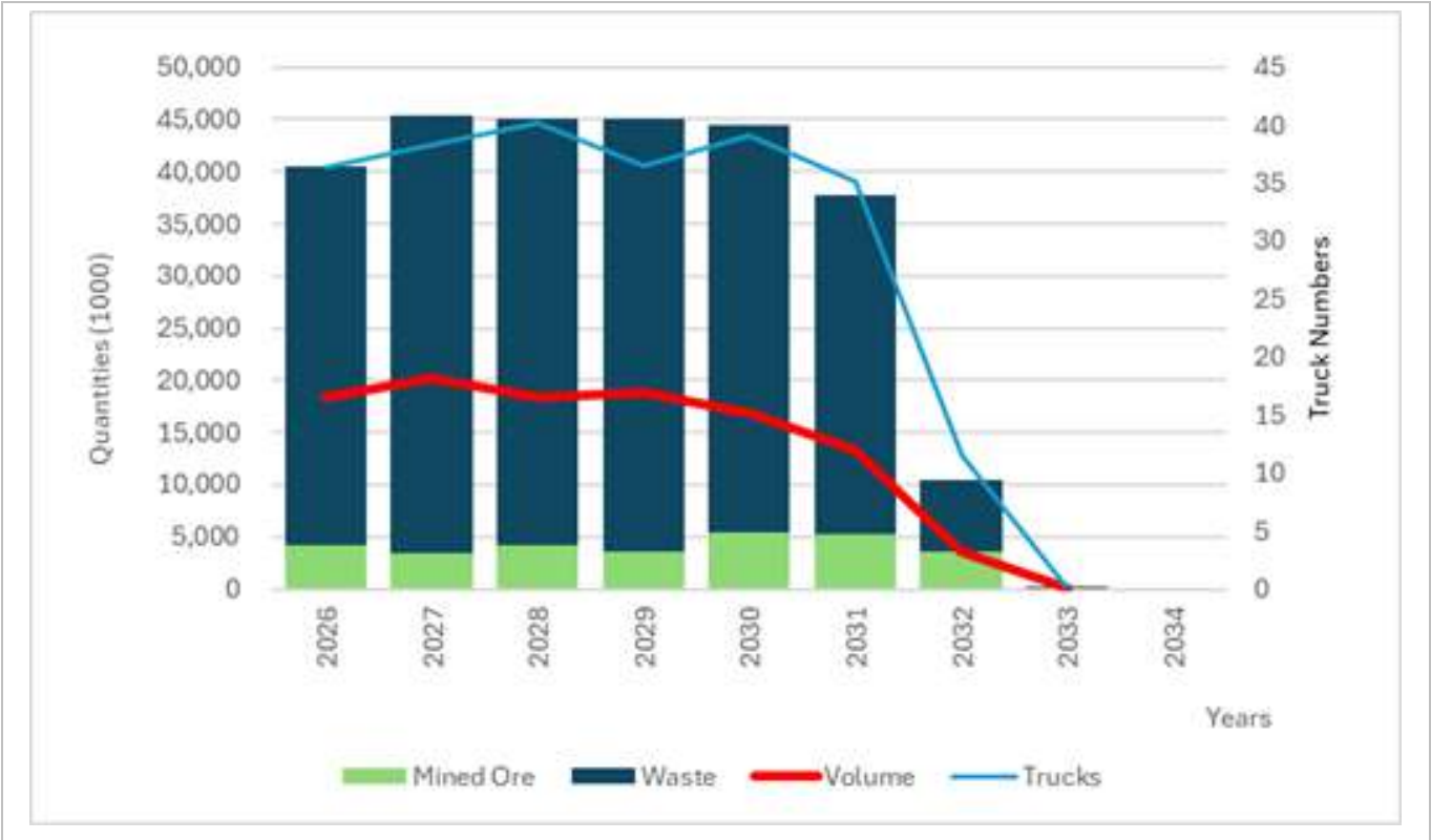
Figure 16-20: Annual Material Movement and Trucks Requirement
