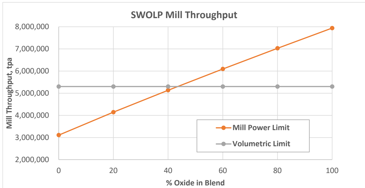
Figure 13-13: Modelled SWOLP Mill Throughput
