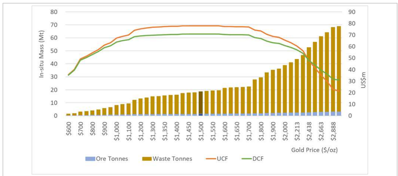
Figure 15-11: Delya Optimisation Results for (Delya Main/Delya South/Samina) Pits
