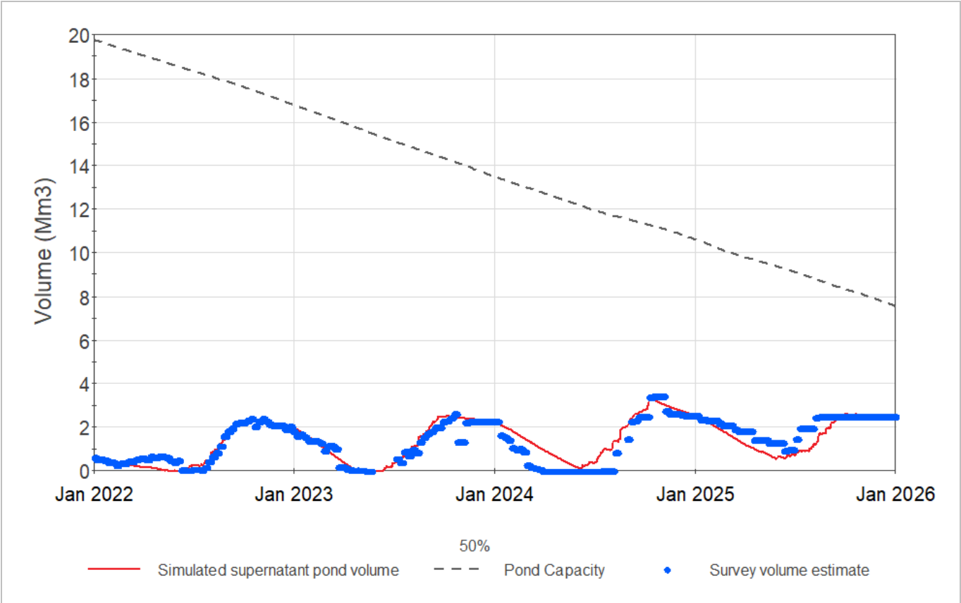
Figure 18-9: TSF 1 Calibration (2022 to October 2025)
